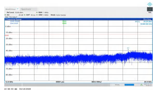
NTNV-DC_2A-n66A-PC3-15-5+20-M+L-QPSK-IDLE-DFT-BPSK-Inner_1RB_Left-12000-20000-PASS
