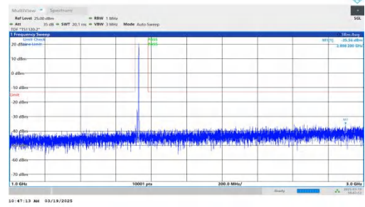
NTNV-DC_2A-n66A-PC3-15-5+20-M+L-QPSK-IDLE-DFT-BPSK-Inner_1RB_Right-1000-3000-PASS
