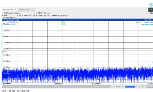
NTNV-DC_2A-n66A-PC3-15-5+10-M+L-QPSK-IDLE-DFT-QPSK-Inner_1RB_Left-30-1000-PASS
