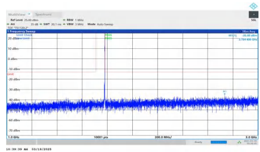
NTNV-DC_2A-n66A-PC3-15-5+10-M+H-QPSK-IDLE-DFT-QPSK-In ner_1RB_Right-1000-3000-PASS
