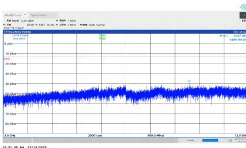
NTNV-DC_2A-n66A-PC3-15-5+20-M+H-QPSK-IDLE-DFT-BPSK-Inner_1RB_Left-3000-12000-PASS
