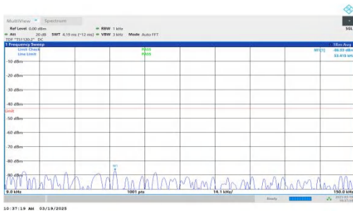
NTNV-DC_2A-n66A-PC3-15-5+10-M+M-QPSK-IDLE-DFT-QPSK-Inner_1RB_Right-0.009-0.15-PASS
