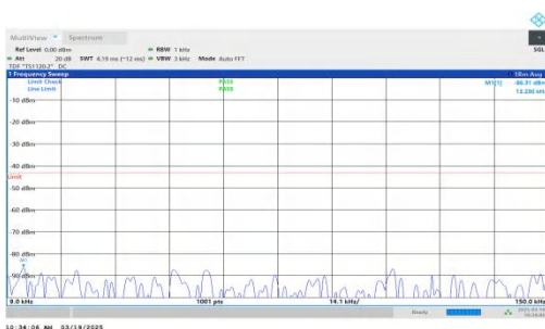
NTNV-DC_2A-n66A-PC3-15-5+10-M+L-QPSK-IDLE-DFT-BPSK-Inner_1RB_Right-0.009-0.15-PASS
