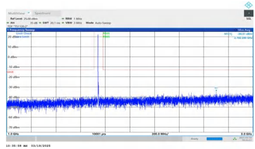
NTNV-DC_2A-n66A-PC3-15-5+10-M+M-QPSK-IDLE-DFT-BPSK-In ner_1RB_Left-1000-3000-PASS
