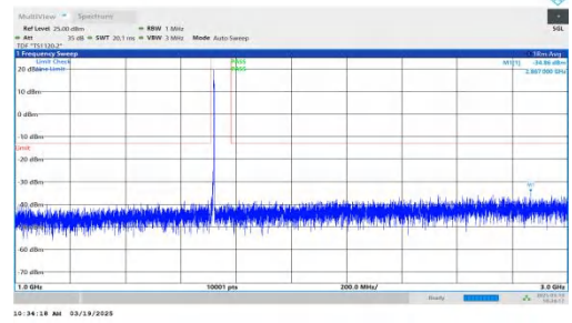
NTNV-DC_2A-n66A-PC3-15-5+10-M+L-QPSK-IDLE-DFT-BPSK-Inner_1RB_Right-1000-3000-PASS
