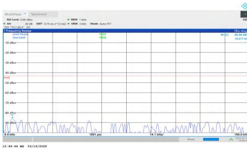
NTNV-DC_2A-n66A-PC3-15-5+20-M+M-QPSK-IDLE-DFT-QPSK-I nner_1RB_Left-0.009-0.15-PASS
