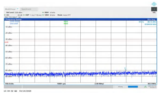
NTNV-DC_2A-n66A-PC3-15-5+10-M+H-QPSK-IDLE-DFT-QPSK-In ner_1RB_Right-0.15-30-PASS
