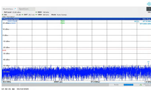
NTNV-DC_2A-n66A-PC3-15-5+15-M+M-QPSK-IDLE-DFT-BPSK-In ner_1RB_Left-30-1000-PASS
