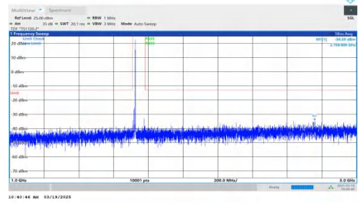
NTNV-DC_2A-n66A-PC3-15-5+15-M+L-QPSK-IDLE-DFT-BPSK-Inner_1RB_Right-1000-3000-PASS
