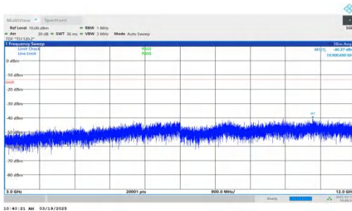
NTNV-DC_2A-n66A-PC3-15-5+15-M+L-QPSK-IDLE-DFT-BPSK-Inner_1RB_Left-3000-12000-PASS
