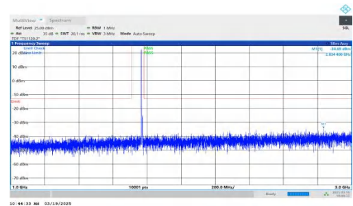
NTNV-DC_2A-n66A-PC3-15-5+15-M+H-QPSK-IDLE-DFT-BPSK-Inner_1RB_Left-1000-3000-PASS
