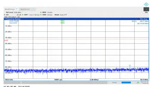
NTNV-DC_2A-n66A-PC3-15-5+15-M+L-QPSK-IDLE-DFT-BPSK-Inner_1RB_Right-0.15-30-PASS
