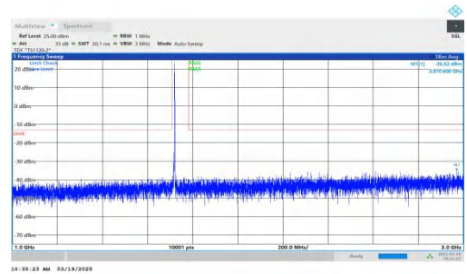
NTNV-DC_2A-n66A-PC3-15-5+10-M+L-QPSK-IDLE-DFT-QPSK-Inner_1RB_Right-1000-3000-PASS
