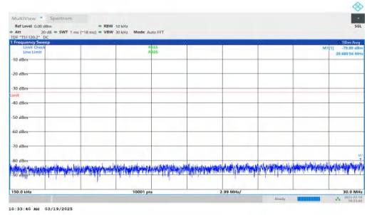
NTNV-DC_2A-n66A-PC3-15-5+10-M+L-QPSK-IDLE-DFT-BPSK-Inner_1RB_Left-0.15-30-PASS
