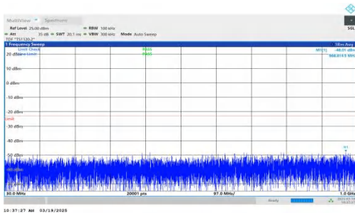
NTNV-DC_2A-n66A-PC3-15-5+10-M+M-QPSK-IDLE-DFT-QPSK-Inner_1RB_Right-30-1000-PASS
