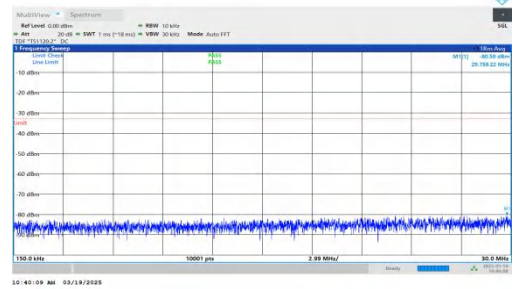
NTNV-DC_2A-n66A-PC3-15-5+15-M+L-QPSK-IDLE-DFT-BPSK-Inner_1RB_Left-0.15-30-PASS
