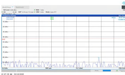
NTNV-DC_2A-n66A-PC3-15-5+20-M+L-QPSK-IDLE-DFT-QPSK-Inner_1RB_Left-0.009-0.15-PASS
