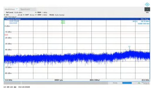
NTNV-DC_2A-n66A-PC3-15-5+20-M+L-QPSK-IDLE-DFT-QPSK-Inner_1RB_Right-12000-20000-PASS
