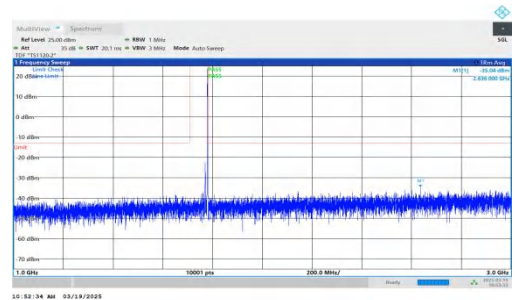
NTNV-DC_2A-n66A-PC3-15-5+20-M+H-QPSK-IDLE-DFT-QPSK-In ner_1RB_Right-1000-3000-PASS
