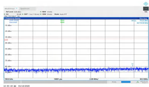
NTNV-DC_2A-n66A-PC3-15-5+20-M+M-QPSK-IDLE-DFT-QPSK-In ner_1RB_Right-0.15-30-PASS
