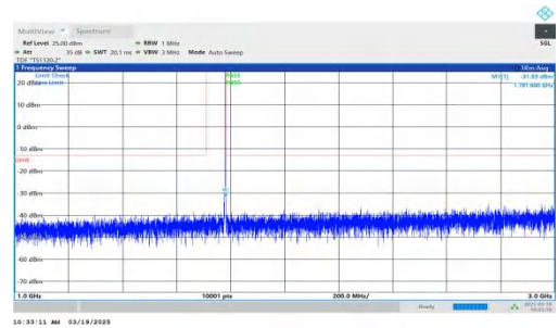
NTNV-DC_2A-n66A-PC3-15-5+5-M+H-QPSK-IDLE-DFT-QPSK-Inner_1RB_Right-1000-3000-PASS
