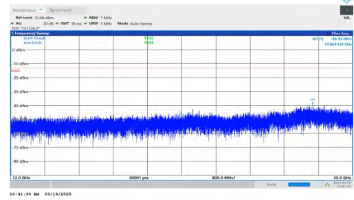
NTNV-DC_2A-n66A-PC3-15-5+15-M+L-QPSK-IDLE-DFT-QPSK-Inner_1RB_Left-12000-20000-PASS
