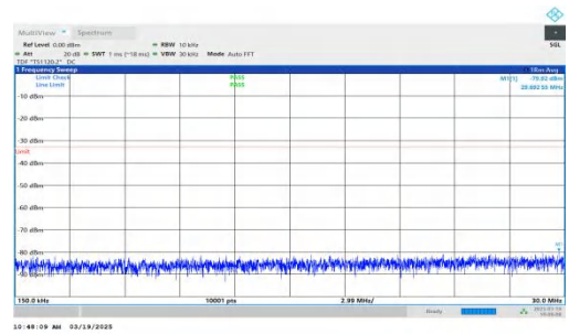
NTNV-DC_2A-n66A-PC3-15-5+20-M+L-QPSK-IDLE-DFT-QPSK-Inner_1RB_Right-0.15-30-PASS
