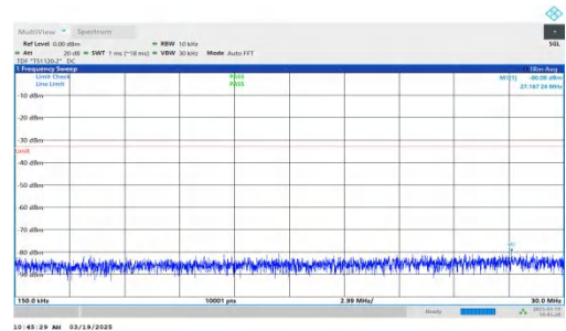
NTNV-DC_2A-n66A-PC3-15-5+15-M+H-QPSK-IDLE-DFT-QPSK-Inner_1RB_Left-0.15-30-PASS
