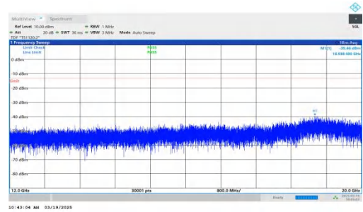
NTNV-DC_2A-n66A-PC3-15-5+15-M+M-QPSK-IDLE-DFT-BPSK-In ner_1RB_Right-12000-20000-PASS
