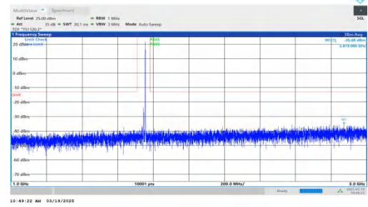
NTNV-DC_2A-n66A-PC3-15-5+20-M+M-QPSK-IDLE-DFT-BPSK-In ner_1RB_Right-1000-3000-PASS
