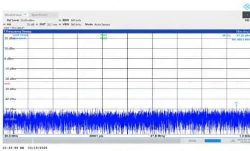
NTNV-DC_2A-n66A-PC3-15-5+10-M+L-QPSK-IDLE-DFT-BPSK-Inner_1RB_Left-30-1000-PASS
