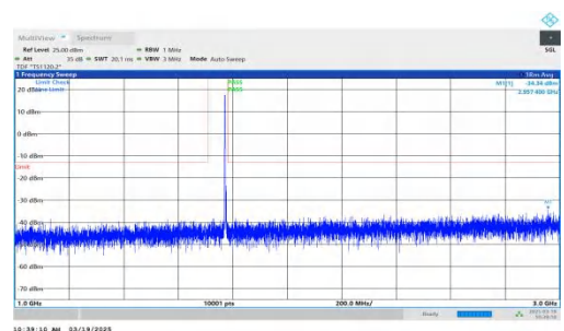
NTNV-DC_2A-n66A-PC3-15-5+10-M+H-QPSK-IDLE-DFT-QPSK-Inner_1RB_Left-1000-3000-PASS
