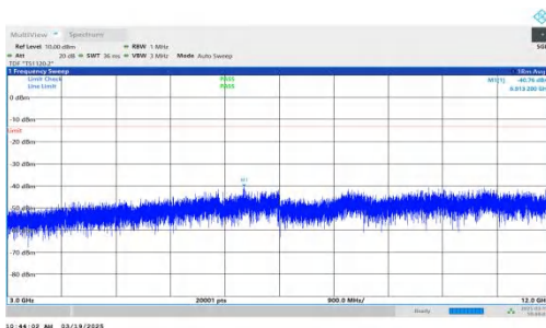
NTNV-DC_2A-n66A-PC3-15-5+15-M+M-QPSK-IDLE-DFT-QPSK-Inner_1RB_Right-3000-12000-PASS
