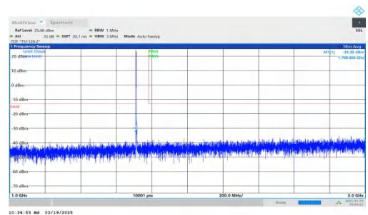
NTNV-DC_2A-n66A-PC3-15-5+10-M+L-QPSK-IDLE-DFT-QPSK-Inner_1RB_Left-1000-3000-PASS
