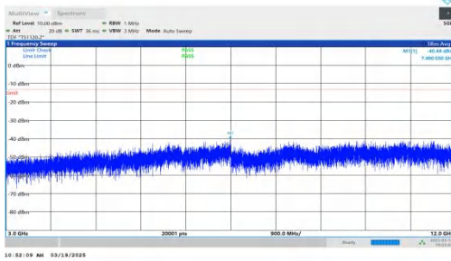
NTNV-DC_2A-n66A-PC3-15-5+20-M+H-QPSK-IDLE-DFT-QPSK-In ner_1RB_Left-3000-12000-PASS
