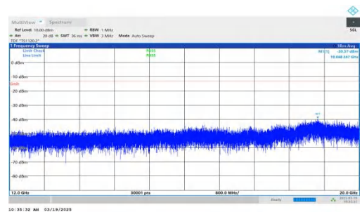
NTNV-DC_2A-n66A-PC3-15-5+10-M+L-QPSK-IDLE-DFT-QPSK-Inner_1RB_Right-12000-20000-PASS
