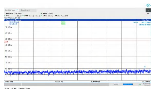
NTNV-DC_2A-n66A-PC3-15-5+10-M+L-QPSK-IDLE-DFT-BPSK-Inner_1RB_Right-0.15-30-PASS
