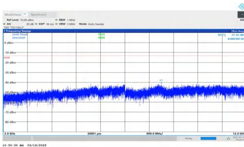
NTNV-DC_2A-n66A-PC3-15-5+20-M+M-QPSK-IDLE-DFT-QPSK-I nner_1RB_Right-3000-12000-PASS
