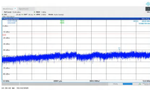
NTNV-DC_2A-n66A-PC3-15-5+10-M+L-QPSK-IDLE-DFT-BPSK-Inner_1RB_Right-3000-12000-PASS
