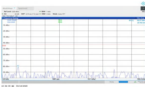
NTNV-DC_2A-n66A-PC3-15-5+5-M+H-QPSK-IDLE-DFT-QPSK-Inner_1RB_Left-0.009-0.15-PASS
