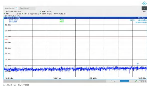
NTNV-DC_2A-n66A-PC3-15-5+10-M+L-QPSK-IDLE-DFT-QPSK-Inner_1RB_Left-0.15-30-PASS
