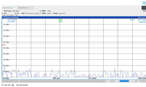
NTNV-DC_2A-n66A-PC3-15-5+15-M+H-QPSK-IDLE-DFT-QPSK-In ner_1RB_Right-0.009-0.15-PASS
