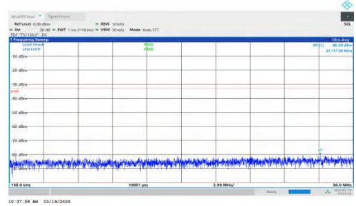
NTNV-DC_2A-n66A-PC3-15-5+10-M+H-QPSK-IDLE-DFT-BPSK-Inner_1RB_Left-0.15-30-PASS
