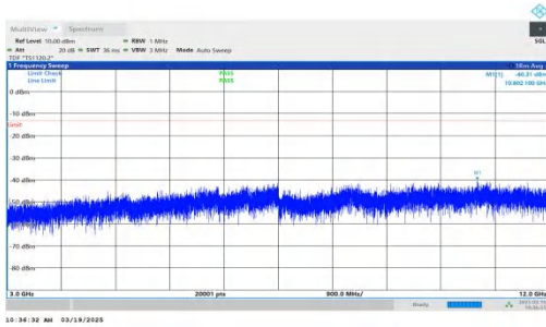
NTNV-DC_2A-n66A-PC3-15-5+10-M+M-QPSK-IDLE-DFT-BPSK-Inner_1RB_Right-3000-12000-PASS
