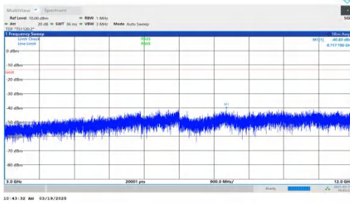
NTNV-DC_2A-n66A-PC3-15-5+15-M+M-QPSK-IDLE-DFT-QPSK-Inner_1RB_Left-3000-12000-PASS
