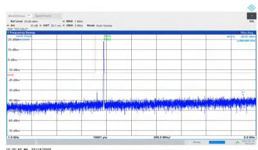
NTNV-DC_2A-n66A-PC3-15-5+5-M+H-QPSK-IDLE-DFT-QPSK-Inner_1RB_Left-1000-3000-PASS
