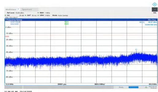
NTNV-DC_2A-n66A-PC3-15-5+15-M+H-QPSK-IDLE-DFT-BPSK-Inner_1RB_Left-12000-20000-PASS
