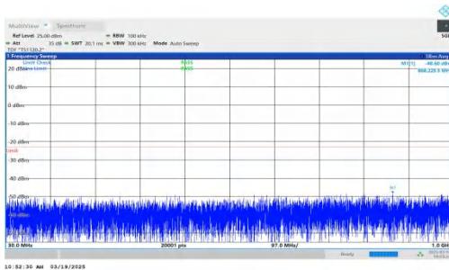
NTNV-DC_2A-n66A-PC3-15-5+20-M+H-QPSK-IDLE-DFT-QPSK-In ner_1RB_Right-30-1000-PASS
