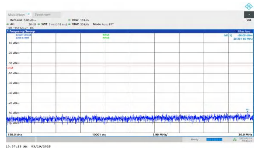
NTNV-DC_2A-n66A-PC3-15-5+10-M+M-QPSK-IDLE-DFT-QPSK-Inner_1RB_Right-0.15-30-PASS
