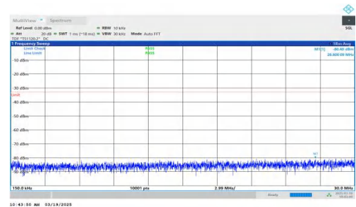
NTNV-DC_2A-n66A-PC3-15-5+15-M+M-QPSK-IDLE-DFT-QPSK-Inner_1RB_Right-0.15-30-PASS
