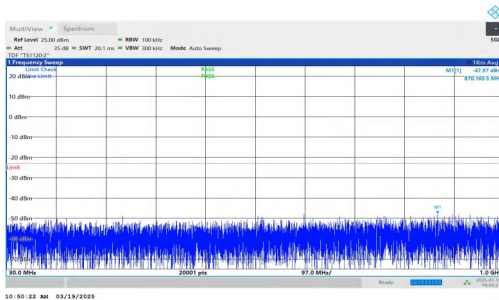
NTNV-DC_2A-n66A-PC3-15-5+20-M+M-QPSK-IDLE-DFT-QPSK-I nner_1RB_Right-30-1000-PASS
