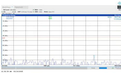
NTNV-DC_2A-n66A-PC3-15-5+5-M+H-QPSK-IDLE-DFT-QPSK-Inner_1RB_Right-0.009-0.15-PASS
