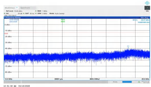
NTNV-DC_2A-n66A-PC3-15-5+20-M+H-QPSK-IDLE-DFT-BPSK-Inner_1RB_Right-12000-20000-PASS
