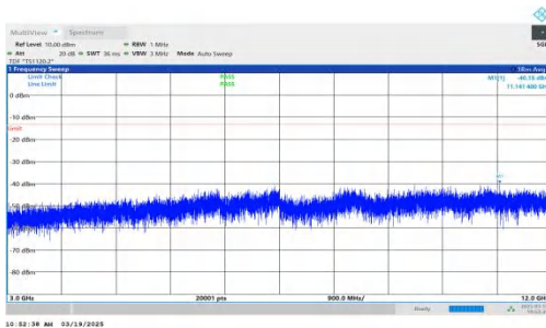
NTNV-DC_2A-n66A-PC3-15-5+20-M+H-QPSK-IDLE-DFT-QPSK-In ner_1RB_Right-3000-12000-PASS
