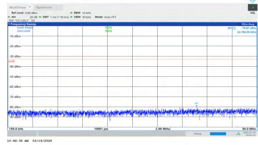
NTNV-DC_2A-n66A-PC3-15-5+20-M+L-QPSK-IDLE-DFT-BPSK-Inner_1RB_Left-0.15-30-PASS
