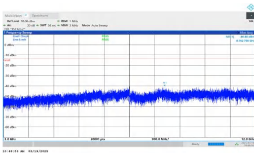
NTNV-DC_2A-n66A-PC3-15-5+20-M+M-QPSK-IDLE-DFT-BPSK-In ner_1RB_Left-3000-12000-PASS
