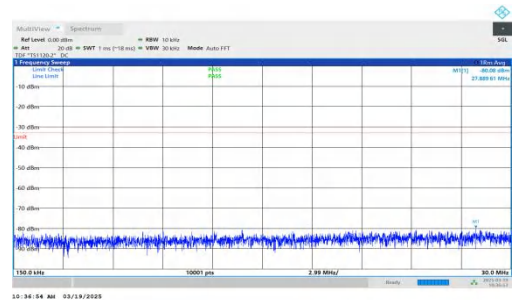
NTNV-DC_2A-n66A-PC3-15-5+10-M+M-QPSK-IDLE-DFT-QPSK-Inner_1RB_Left-0.15-30-PASS
