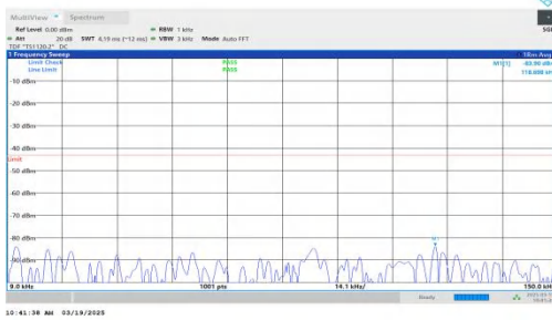
NTNV-DC_2A-n66A-PC3-15-5+15-M+L-QPSK-IDLE-DFT-QPSK-Inner_1RB_Right-0.009-0.15-PASS
