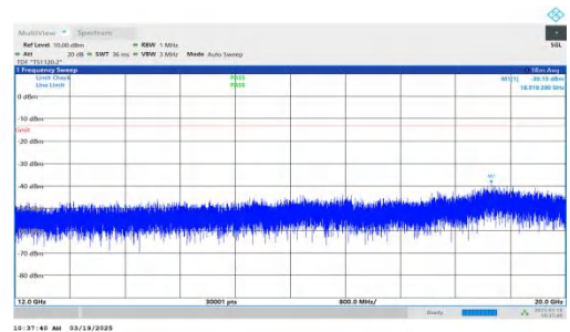
NTNV-DC_2A-n66A-PC3-15-5+10-M+M-QPSK-IDLE-DFT-QPSK-Inner_1RB_Right-12000-20000-PASS
