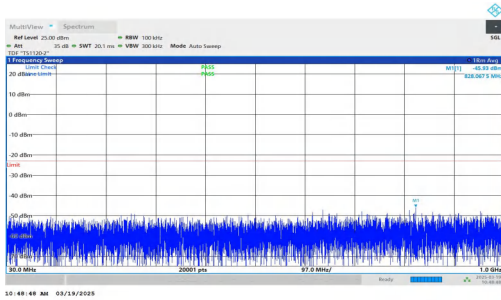
NTNV-DC_2A-n66A-PC3-15-5+20-M+M-QPSK-IDLE-DFT-BPSK-In ner_1RB_Left-30-1000-PASS
