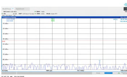
NTNV-DC_2A-n66A-PC3-15-5+20-M+L-QPSK-IDLE-DFT-BPSK-Inner_1RB_Right-0.009-0.15-PASS
