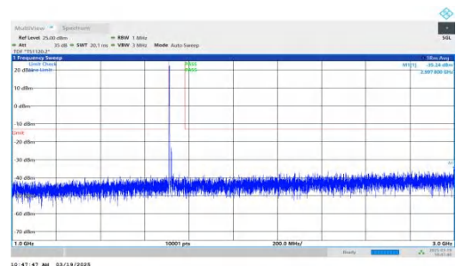
NTNV-DC_2A-n66A-PC3-15-5+20-M+L-QPSK-IDLE-DFT-QPSK-Inner_1RB_Left-1000-3000-PASS
