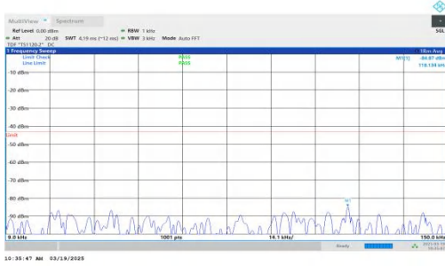
NTNV-DC_2A-n66A-PC3-15-5+10-M+M-QPSK-IDLE-DFT-BPSK-In ner_1RB_Left-0.009-0.15-PASS
