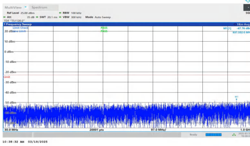
NTNV-DC_2A-n66A-PC3-15-5+10-M+H-QPSK-IDLE-DFT-BPSK-Inner_1RB_Right-30-1000-PASS
