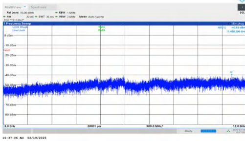
NTNV-DC_2A-n66A-PC3-15-5+10-M+M-QPSK-IDLE-DFT-QPSK-Inner_1RB_Left-3000-12000-PASS
