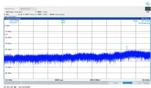
NTNV-DC_2A-n66A-PC3-15-5+20-M+M-QPSK-IDLE-DFT-QPSK-In ner_1RB_Right-12000-20000-PASS
