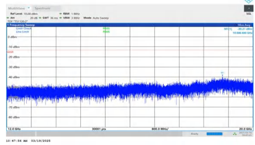
NTNV-DC_2A-n66A-PC3-15-5+20-M+L-QPSK-IDLE-DFT-QPSK-Inner_1RB_Left-12000-20000-PASS
