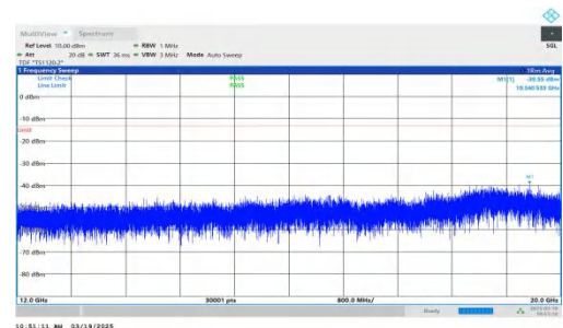
NTNV-DC_2A-n66A-PC3-15-5+20-M+H-QPSK-IDLE-DFT-BPSK-Inner_1RB_Left-12000-20000-PASS
