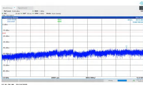
NTNV-DC_2A-n66A-PC3-15-5+15-M+L-QPSK-IDLE-DFT-QPSK-Inner_1RB_Right-3000-12000-PASS
