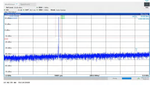
NTNV-DC_2A-n66A-PC3-15-5+15-M+M-QPSK-IDLE-DFT-BPSK-In ner_1RB_Right-1000-3000-PASS
