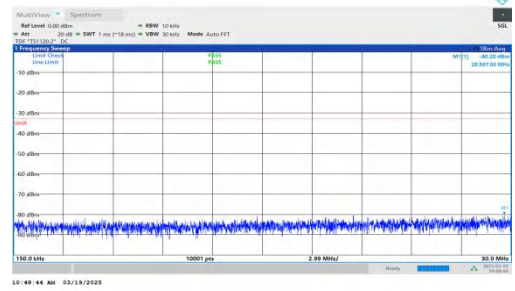
NTNV-DC_2A-n66A-PC3-15-5+20-M+M-QPSK-IDLE-DFT-BPSK-In ner_1RB_Left-0.15-30-PASS
