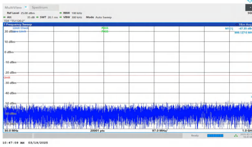
NTNV-DC_2A-n66A-PC3-15-5+20-M+L-QPSK-IDLE-DFT-BPSK-Inner_1RB_Right-30-1000-PASS
