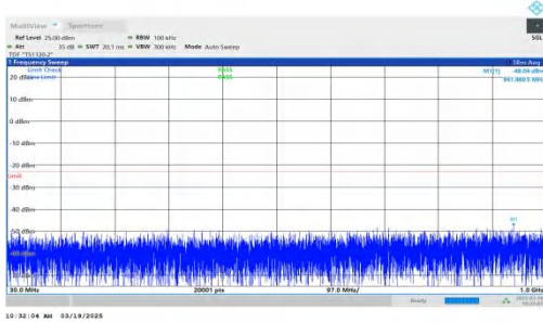
NTNV-DC_2A-n66A-PC3-15-5+5-M+H-QPSK-IDLE-DFT-BPSK-Inner_1RB_Right-30-1000-PASS
