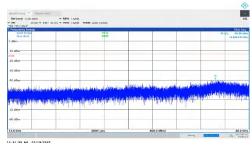
NTNV-DC_2A-n66A-PC3-15-5+15-M+L-QPSK-IDLE-DFT-QPSK-Inner_1RB_Right-12000-20000-PASS
