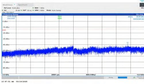
NTNV-DC_2A-n66A-PC3-15-5+20-M+L-QPSK-IDLE-DFT-QPSK-Inner_1RB_Left-3000-12000-PASS
