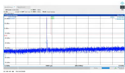
NTNV-DC_2A-n66A-PC3-15-5+20-M+L-QPSK-IDLE-DFT-BPSK-Inner_1RB_Left-1000-3000-PASS
