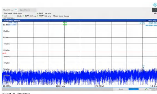
NTNV-DC_2A-n66A-PC3-15-5+5-M+H-QPSK-IDLE-DFT-QPSK-Inner_1RB_Left-30-1000-PASS
