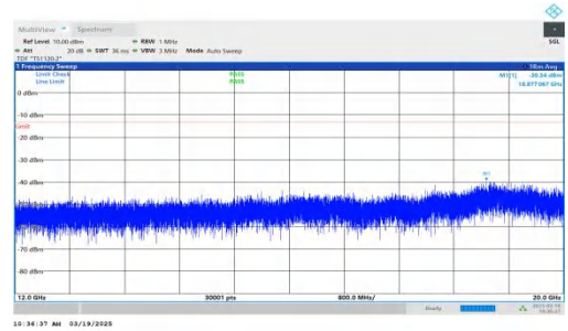
NTNV-DC_2A-n66A-PC3-15-5+10-M+M-QPSK-IDLE-DFT-BPSK-Inner_1RB_Right-12000-20000-PASS
