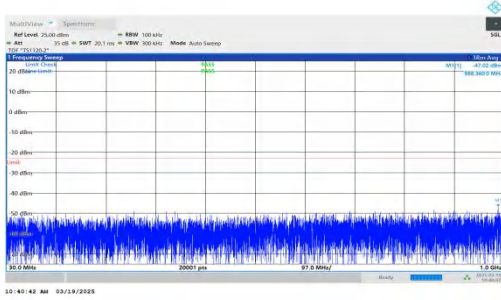
NTNV-DC_2A-n66A-PC3-15-5+15-M+L-QPSK-IDLE-DFT-BPSK-Inner_1RB_Right-30-1000-PASS
