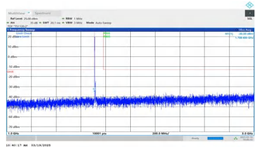
NTNV-DC_2A-n66A-PC3-15-5+15-M+L-QPSK-IDLE-DFT-BPSK-Inner_1RB_Left-1000-3000-PASS
