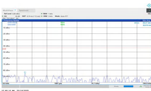
NTNV-DC_2A-n66A-PC3-15-5+20-M+M-QPSK-IDLE-DFT-BPSK-In ner_1RB_Right-0.009-0.15-PASS
