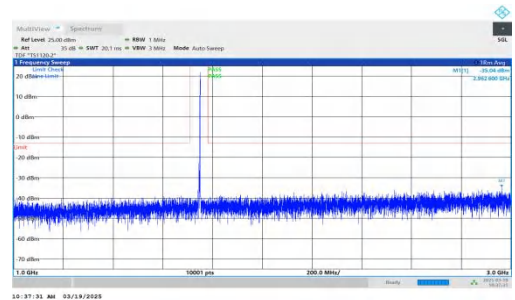
NTNV-DC_2A-n66A-PC3-15-5+10-M+M-QPSK-IDLE-DFT-QPSK-Inner_1RB_Right-1000-3000-PASS
