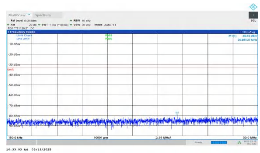
NTNV-DC_2A-n66A-PC3-15-5+5-M+H-QPSK-IDLE-DFT-QPSK-Inner_1RB_Right-0.15-30-PASS
