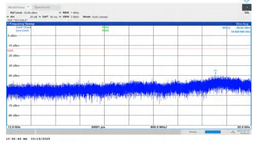
NTNV-DC_2A-n66A-PC3-15-5+15-M+H-QPSK-IDLE-DFT-QPSK-In ner_1RB_Left-12000-20000-PASS
