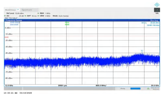
NTNV-DC_2A-n66A-PC3-15-5+5-M+H-QPSK-IDLE-DFT-QPSK-Inner_1RB_Right-12000-20000-PASS
