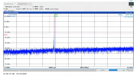
NTNV-DC_2A-n66A-PC3-15-5+15-M+H-QPSK-IDLE-DFT-BPSK-Inner_1RB_Right-1000-3000-PASS
