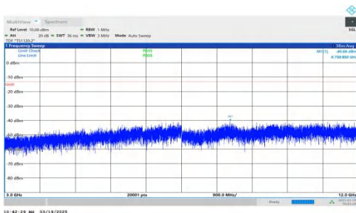
NTNV-DC_2A-n66A-PC3-15-5+15-M+M-QPSK-IDLE-DFT-BPSK-In ner_1RB_Left-3000-12000-PASS
