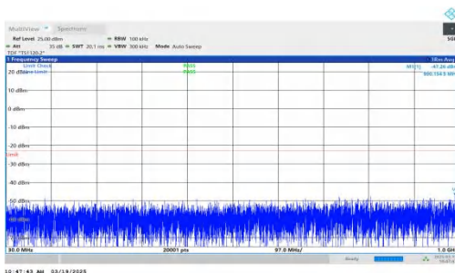
NTNV-DC_2A-n66A-PC3-15-5+20-M+L-QPSK-IDLE-DFT-QPSK-Inner_1RB_Left-30-1000-PASS
