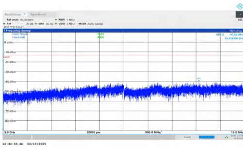
NTNV-DC_2A-n66A-PC3-15-5+15-M+L-QPSK-IDLE-DFT-BPSK-Inner_1RB_Right-3000-12000-PASS
