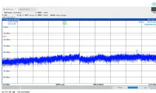
NTNV-DC_2A-n66A-PC3-15-5+10-M+M-QPSK-IDLE-DFT-QPSK-Inner_1RB_Right-3000-12000-PASS
