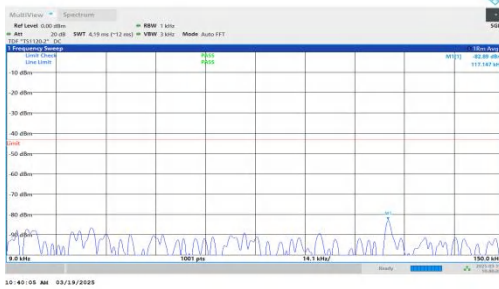
NTNV-DC_2A-n66A-PC3-15-5+15-M+L-QPSK-IDLE-DFT-BPSK-Inner_1RB_Left-0.009-0.15-PASS
