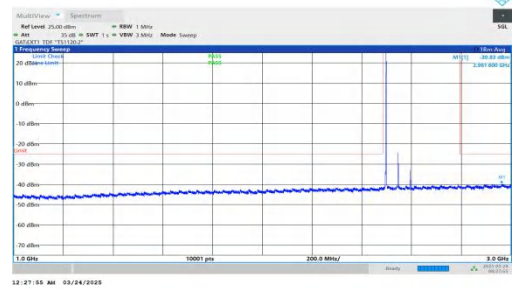
NTNV-DC_2A-n41A-PC2-30-5+100-M+L-QPSK-IDLE-DFT-BPSK-In ner_1RB_Left-1000-3000-PASS
