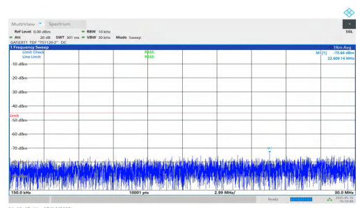
NTNV-DC_2A-n41A-PC2-30-5+80-M+H-QPSK-IDLE-DFT-BPSK-Inner_1RB_Right-0.15-30-PASS
