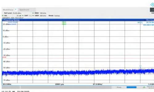
NTNV-DC_2A-n41A-PC2-30-5+80-M+H-QPSK-IDLE-DFT-QPSK-Inner_1RB_Left-30-1000-PASS
