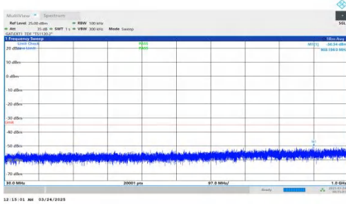
NTNV-DC_2A-n41A-PC2-30-5+90-M+L-QPSK-IDLE-DFT-BPSK-Inner_1RB_Left-30-1000-PASS
