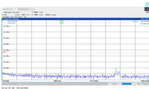
NTNV-DC_2A-n41A-PC2-30-5+100-M+M-QPSK-IDLE-DFT-QPSK-I Inner_1RB_Left-0.009-0.15-PASS
