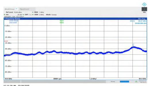
NTNV-DC_2A-n41A-PC2-30-5+80-M+M-QPSK-IDLE-DFT-QPSK-Inner_1RB_Right-18000-30000-PASS
