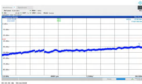
NTNV-DC_2A-n41A-PC2-30-5+90-M+H-QPSK-IDLE-DFT-BPSK-Inner_1RB_Right-3000-18000-PASS
