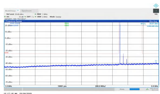
NTNV-DC_2A-n41A-PC2-30-5+90-M+L-QPSK-IDLE-DFT-QPSK-Inner_1RB_Left-1000-3000-PASS
