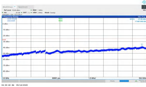
NTNV-DC_2A-n41A-PC2-30-5+90-M+M-QPSK-IDLE-DFT-QPSK-Inner_1RB_Left-3000-18000-PASS
