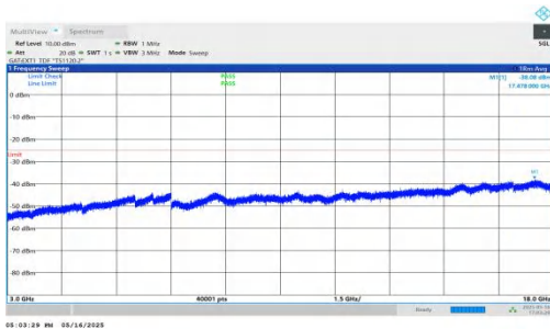
NTNV-DC_2A-n41A-PC2-30-5+100-M+M-QPSK-IDLE-DFT-BPSK-I nner_1RB_Left-3000-18000-PASS
