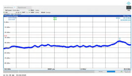
NTNV-DC_2A-n41A-PC2-30-5+100-M+L-QPSK-IDLE-DFT-QPSK-Inner_1RB_Right-18000-30000-PASS
