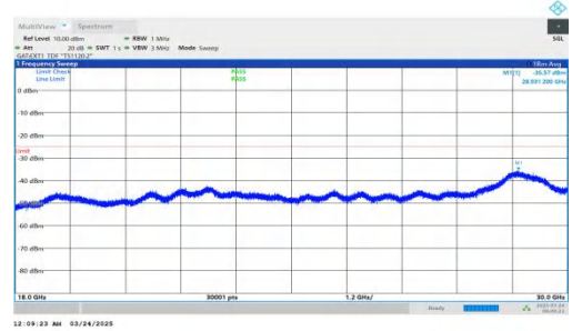
NTNV-DC_2A-n41A-PC2-30-5+80-M+M-QPSK-IDLE-DFT-QPSK-Inner_1RB_Left-18000-30000-PASS
