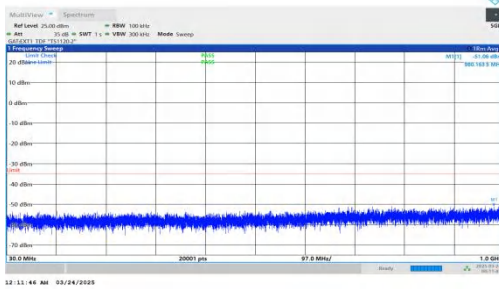
NTNV-DC_2A-n41A-PC2-30-5+80-M+H-QPSK-IDLE-DFT-BPSK-Inner_1RB_Right-30-1000-PASS
