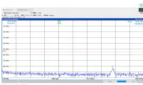
NTNV-DC_2A-n41A-PC2-30-5+80-M+H-QPSK-IDLE-DFT-BPSK-Inner_1RB_Right-0.009-0.15-PASS
