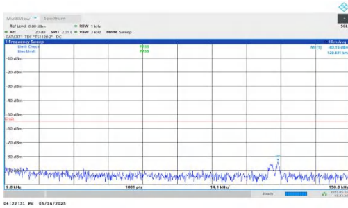
NTNV-DC_2A-n41A-PC2-30-5+100-M+M-QPSK-IDLE-DFT-QPSK-Inner_1RB_Right-0.009-0.15-PASS
