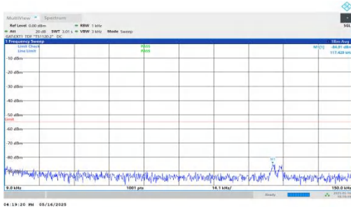
NTNV-DC_2A-n41A-PC2-30-5+100-M+L-QPSK-IDLE-DFT-BPSK-I nner_1RB_Right-0.009-0.15-PASS
