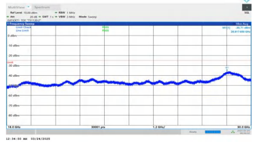
NTNV-DC_2A-n41A-PC2-30-5+100-M+M-QPSK-IDLE-DFT-QPSK-Inner_1RB_Left-18000-30000-PASS
