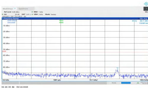
NTNV-DC_2A-n41A-PC2-30-5+100-M+H-QPSK-IDLE-DFT-QPSK-I nner_1RB_Right-0.009-0.15-PASS
