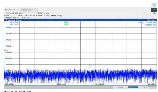
NTNV-DC_2A-n41A-PC2-30-5+90-M+H-QPSK-IDLE-DFT-BPSK-Inner_1RB_Right-0.15-30-PASS
