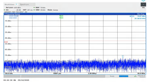
NTNV-DC_2A-n41A-PC2-30-5+100-M+M-QPSK-IDLE-DFT-QPSK-Inner_1RB_Right-0.15-30-PASS
