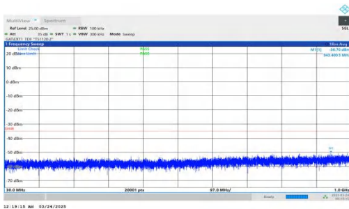
NTNV-DC_2A-n41A-PC2-30-5+90-M+M-QPSK-IDLE-DFT-BPSK-In ner_1RB_Left-30-1000-PASS
