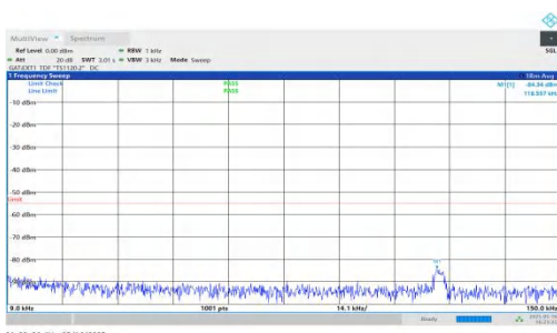
NTNV-DC_2A-n41A-PC2-30-5+100-M+H-QPSK-IDLE-DFT-BPSK-I nner_1RB_Right-0.009-0.15-PASS
