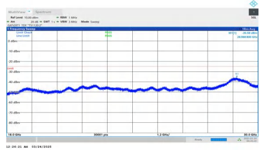
NTNV-DC_2A-n41A-PC2-30-5+90-M+H-QPSK-IDLE-DFT-QPSK-In ner_1RB_Left-18000-30000-PASS
