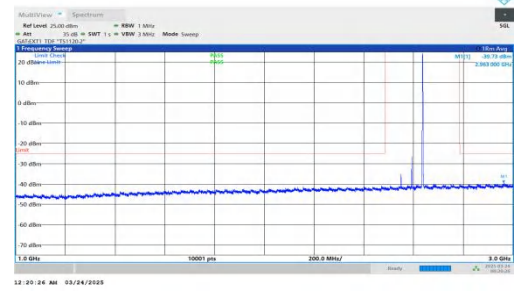
NTNV-DC_2A-n41A-PC2-30-5+90-M+M-QPSK-IDLE-DFT-BPSK-In ner_1RB_Right-1000-3000-PASS
