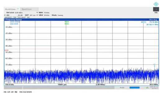
NTNV-DC_2A-n41A-PC2-30-5+90-M+H-QPSK-IDLE-DFT-QPSK-In ner_1RB_Right-0.15-30-PASS
