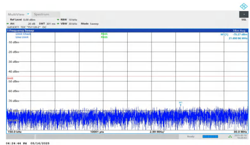
NTNV-DC_2A-n41A-PC2-30-5+100-M+H-QPSK-IDLE-DFT-QPSK-I nner_1RB_Right-0.15-30-PASS
