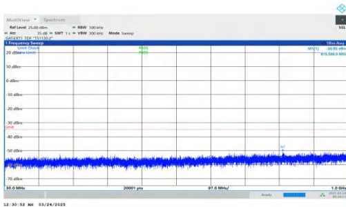
NTNV-DC_2A-n41A-PC2-30-5+100-M+L-QPSK-IDLE-DFT-QPSK-Inner_1RB_Right-30-1000-PASS
