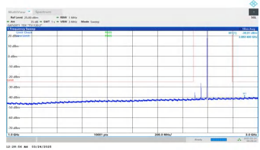
NTNV-DC_2A-n41A-PC2-30-5+100-M+L-QPSK-IDLE-DFT-BPSK-Inner_1RB_Right-1000-3000-PASS
