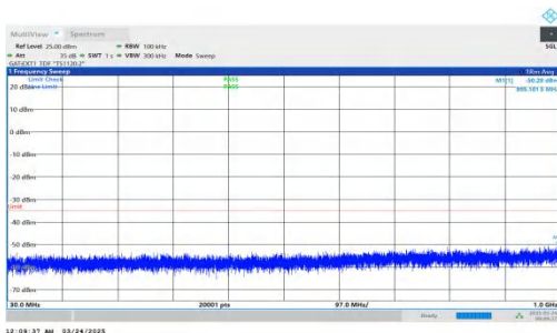
NTNV-DC_2A-n41A-PC2-30-5+80-M+M-QPSK-IDLE-DFT-QPSK-Inner_1RB_Right-30-1000-PASS
