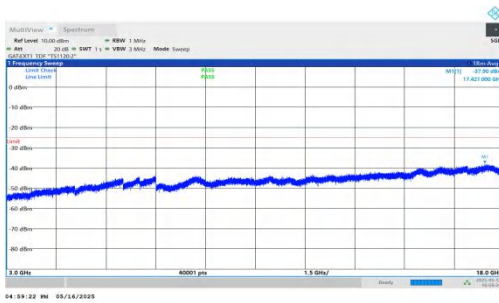
NTNV-DC_2A-n41A-PC2-30-5+90-M+M-QPSK-IDLE-DFT-BPSK-In ner_1RB_Right-3000-18000-PASS
