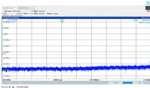
NTNV-DC_2A-n41A-PC2-30-5+80-M+H-QPSK-IDLE-DFT-BPSK-Inner_1RB_Left-30-1000-PASS
