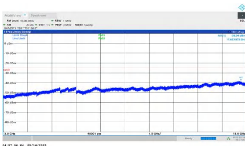
NTNV-DC_2A-n41A-PC2-30-5+80-M+H-QPSK-IDLE-DFT-QPSK-In ner_1RB_Right-3000-18000-PASS
