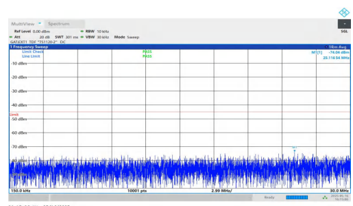
NTNV-DC_2A-n41A-PC2-30-5+90-M+M-QPSK-IDLE-DFT-BPSK-In ner_1RB_Right-0.15-30-PASS
