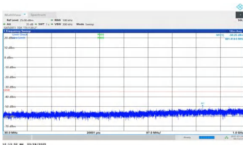
NTNV-DC_2A-n41A-PC2-30-5+80-M+H-QPSK-IDLE-DFT-QPSK-In ner_1RB_Right-30-1000-PASS
