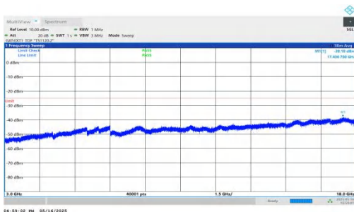
NTNV-DC_2A-n41A-PC2-30-5+90-M+M-QPSK-IDLE-DFT-BPSK-In ner_1RB_Left-3000-18000-PASS
