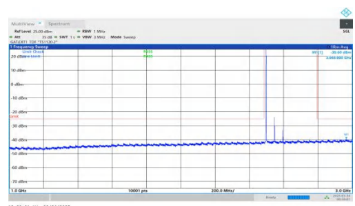
NTNV-DC_2A-n41A-PC2-30-5+100-M+L-QPSK-IDLE-DFT-QPSK-Inner_1RB_Left-1000-3000-PASS
