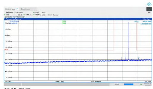
NTNV-DC_2A-n41A-PC2-30-5+100-M+H-QPSK-IDLE-DFT-QPSK-I nner_1RB_Right-1000-3000-PASS
