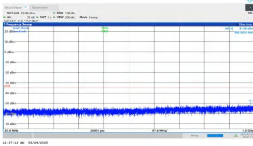
NTNV-DC_2A-n41A-PC2-30-5+100-M+H-QPSK-IDLE-DFT-BPSK-I nner_1RB_Right-30-1000-PASS
