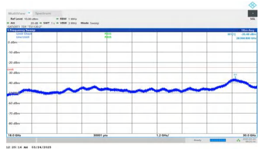
NTNV-DC_2A-n41A-PC2-30-5+90-M+H-QPSK-IDLE-DFT-BPSK-Inner_1RB_Right-18000-30000-PASS
