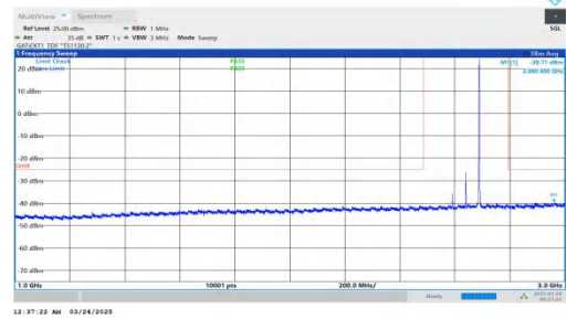
NTNV-DC_2A-n41A-PC2-30-5+100-M+H-QPSK-IDLE-DFT-BPSK-In ner_1RB_Right-1000-3000-PASS
