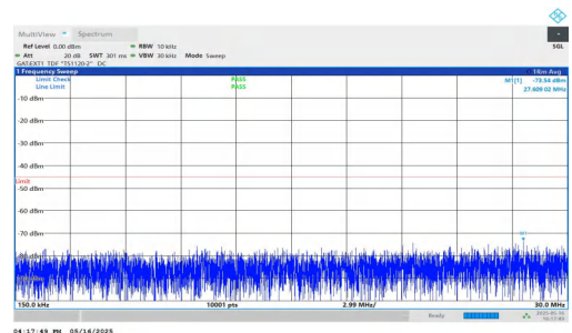
NTNV-DC_2A-n41A-PC2-30-5+90-M+H-QPSK-IDLE-DFT-QPSK-Inner_1RB_Left-0.15-30-PASS
