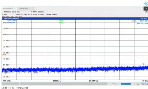
NTNV-DC_2A-n41A-PC2-30-5+100-M+M-QPSK-IDLE-DFT-QPSK-Inner_1RB_Right-30-1000-PASS
