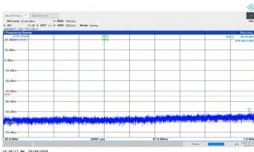
NTNV-DC_2A-n41A-PC2-30-5+100-M+H-QPSK-IDLE-DFT-QPSK-I nner_1RB_Right-30-1000-PASS
