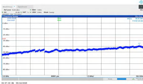
NTNV-DC_2A-n41A-PC2-30-5+90-M+L-QPSK-IDLE-DFT-BPSK-Inner_1RB_Left-3000-18000-PASS
