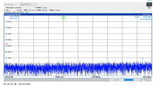
NTNV-DC_2A-n41A-PC2-30-5+100-M+L-QPSK-IDLE-DFT-BPSK-In ner_1RB_Left-0.15-30-PASS
