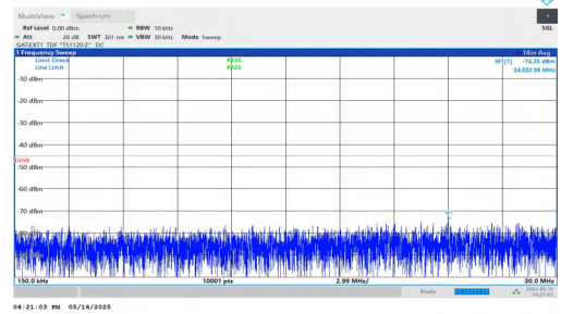
NTNV-DC_2A-n41A-PC2-30-5+100-M+M-QPSK-IDLE-DFT-BPSK-I nner_1RB_Left-0.15-30-PASS
