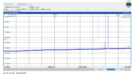
NTNV-DC_2A-n41A-PC2-30-5+100-M+M-QPSK-IDLE-DFT-QPSK-Inner_1RB_Right-1000-3000-PASS
