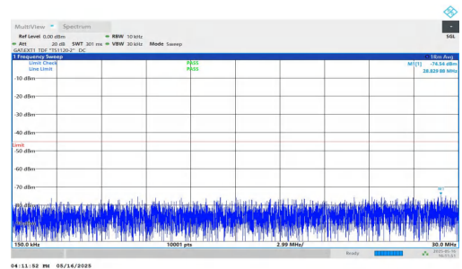
NTNV-DC_2A-n41A-PC2-30-5+80-M+H-QPSK-IDLE-DFT-QPSK-In ner_1RB_Right-0.15-30-PASS
