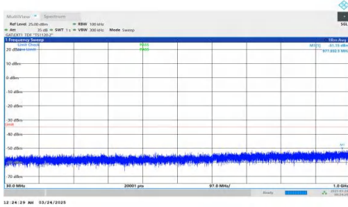
NTNV-DC_2A-n41A-PC2-30-5+90-M+H-QPSK-IDLE-DFT-BPSK-Inner_1RB_Right-30-1000-PASS
