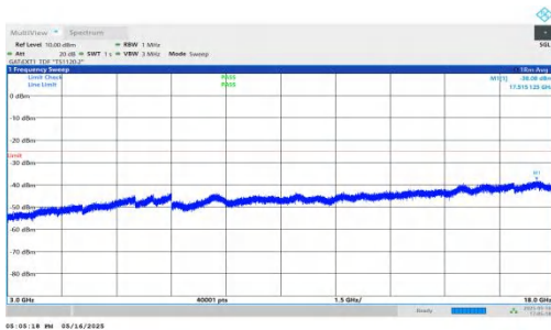
NTNV-DC_2A-n41A-PC2-30-5+100-M+H-QPSK-IDLE-DFT-BPSK-I nner_1RB_Right-3000-18000-PASS
