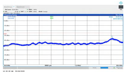
NTNV-DC_2A-n41A-PC2-30-5+100-M+M-QPSK-IDLE-DFT-BPSK-I nner_1RB_Left-18000-30000-PASS
