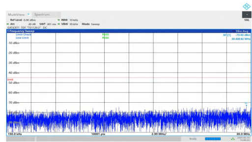
NTNV-DC_2A-n41A-PC2-30-5+80-M+L-QPSK-IDLE-DFT-BPSK-Inner_1RB_Right-0.15-30-PASS
