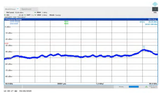
NTNV-DC_2A-n41A-PC2-30-5+80-M+M-QPSK-IDLE-DFT-BPSK-In ner_1RB_Right-18000-30000-PASS
