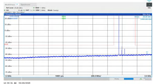
NTNV-DC_2A-n41A-PC2-30-5+80-M+M-QPSK-IDLE-DFT-BPSK-In ner_1RB_Left-1000-3000-PASS
