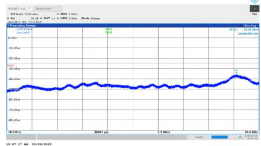
NTNV-DC_2A-n41A-PC2-30-5+80-M+M-QPSK-IDLE-DFT-BPSK-In ner_1RB_Left-18000-30000-PASS
