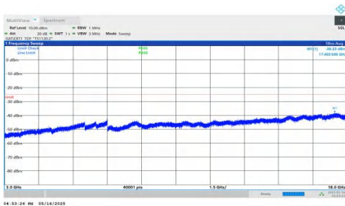
NTNV-DC_2A-n41A-PC2-30-5+80-M+L-QPSK-IDLE-DFT-BPSK-Inner_1RB_Right-3000-18000-PASS
