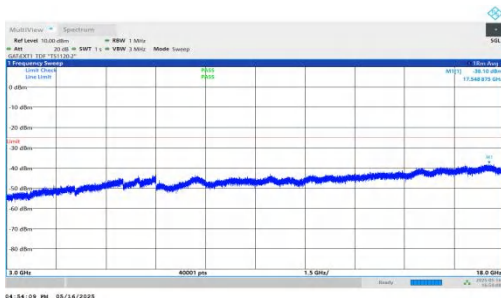
NTNV-DC_2A-n41A-PC2-30-5+80-M+L-QPSK-IDLE-DFT-QPSK-Inner_1RB_Right-3000-18000-PASS
