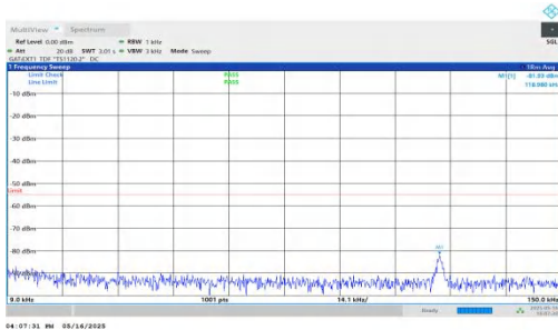
NTNV-DC_2A-n41A-PC2-30-5+80-M+L-QPSK-IDLE-DFT-QPSK-Inner_1RB_Right-0.009-0.15-PASS
