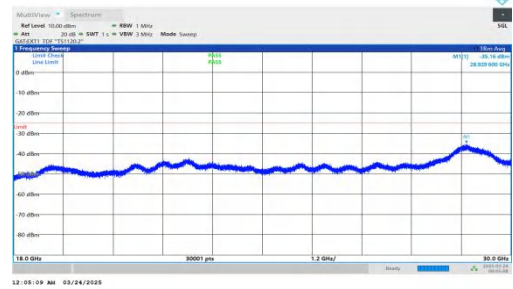
NTNV-DC_2A-n41A-PC2-30-5+80-M+L-QPSK-IDLE-DFT-QPSK-Inner_1RB_Left-18000-30000-PASS
