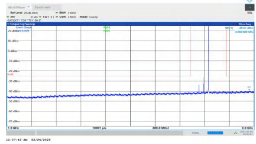
NTNV-DC_2A-n41A-PC2-30-5+80-M+M-QPSK-IDLE-DFT-BPSK-In ner_1RB_Right-1000-3000-PASS
