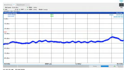
NTNV-DC_2A-n41A-PC2-30-5+80-M+L-QPSK-IDLE-DFT-BPSK-Inner_1RB_Left-18000-30000-PASS
