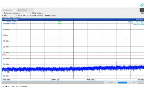
NTNV-DC_2A-n41A-PC2-30-5+80-M+L-QPSK-IDLE-DFT-QPSK-Inner_1RB_Left-30-1000-PASS
