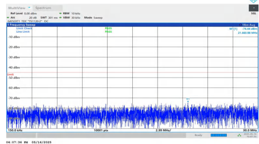
NTNV-DC_2A-n41A-PC2-30-5+80-M+L-QPSK-IDLE-DFT-QPSK-Inner_1RB_Right-0.15-30-PASS
