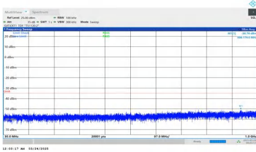
NTNV-DC_2A-n41A-PC2-30-5+80-M+L-QPSK-IDLE-DFT-BPSK-Inner_1RB_Right-30-1000-PASS
