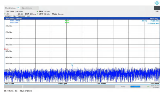
NTNV-DC_2A-n41A-PC2-30-5+80-M+M-QPSK-IDLE-DFT-BPSK-In ner_1RB_Right-0.15-30-PASS
