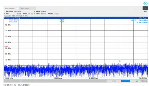
NTNV-DC_2A-n41A-PC2-30-5+80-M+L-QPSK-IDLE-DFT-QPSK-Inner_1RB_Left-0.15-30-PASS
