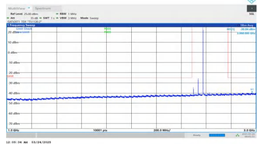
NTNV-DC_2A-n41A-PC2-30-5+80-M+L-QPSK-IDLE-DFT-QPSK-Inner_1RB_Right-1000-3000-PASS
