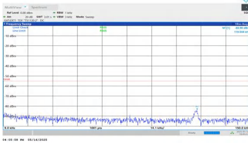
NTNV-DC_2A-n41A-PC2-30-5+80-M+L-QPSK-IDLE-DFT-BPSK-Inner_1RB_Left-0.009-0.15-PASS
