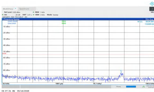
NTNV-DC_2A-n41A-PC2-30-5+80-M+L-QPSK-IDLE-DFT-QPSK-Inner_1RB_Left-0.009-0.15-PASS
