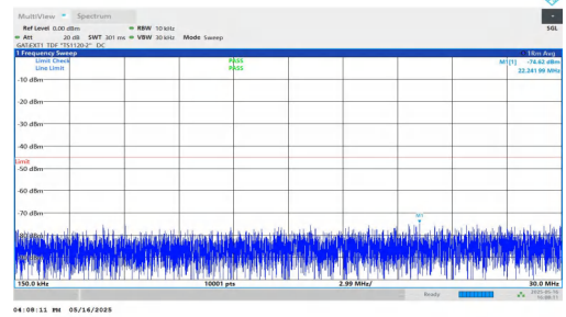
NTNV-DC_2A-n41A-PC2-30-5+80-M+M-QPSK-IDLE-DFT-BPSK-In ner_1RB_Left-0.15-30-PASS
