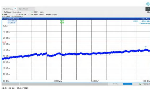
NTNV-DC_2A-n41A-PC2-30-5+80-M+M-QPSK-IDLE-DFT-BPSK-In ner_1RB_Right-3000-18000-PASS
