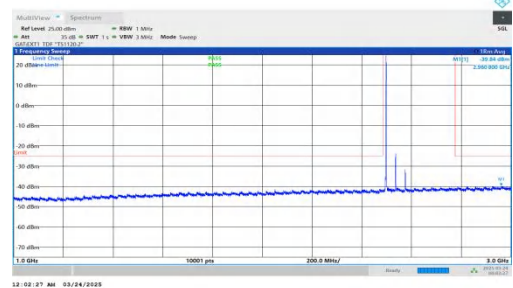
NTNV-DC_2A-n41A-PC2-30-5+80-M+L-QPSK-IDLE-DFT-BPSK-Inner_1RB_Left-1000-3000-PASS
