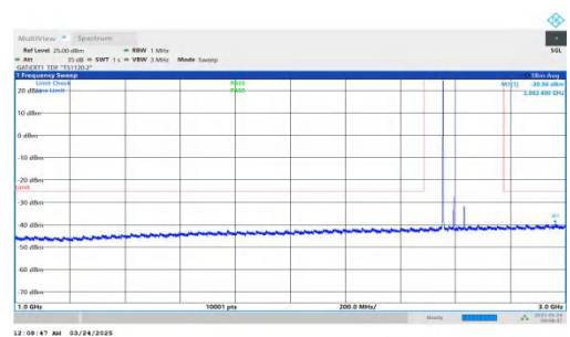
NTNV-DC_2A-n41A-PC2-30-5+80-M+M-QPSK-IDLE-DFT-QPSK-In ner_1RB_Left-1000-3000-PASS
