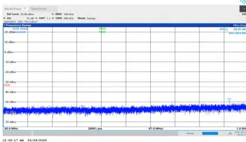
NTNV-DC_2A-n41A-PC2-30-5+80-M+L-QPSK-IDLE-DFT-BPSK-Inner_1RB_Left-30-1000-PASS
