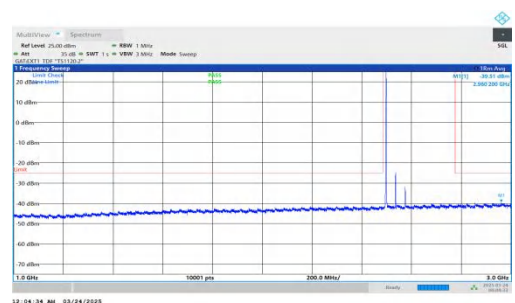
NTNV-DC_2A-n41A-PC2-30-5+80-M+L-QPSK-IDLE-DFT-QPSK-Inner_1RB_Left-1000-3000-PASS
