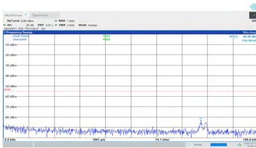
NTNV-DC_2A-n41A-PC2-30-5+80-M+L-QPSK-IDLE-DFT-BPSK-Inner_1RB_Right-0.009-0.15-PASS
