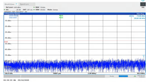
NTNV-DC_2A-n41A-PC2-30-5+80-M+L-QPSK-IDLE-DFT-BPSK-Inner_1RB_Left-0.15-30-PASS
