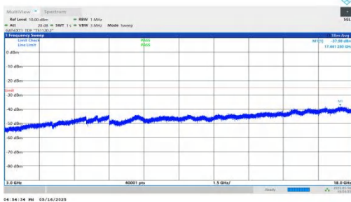
NTNV-DC_2A-n41A-PC2-30-5+80-M+M-QPSK-IDLE-DFT-BPSK-In ner_1RB_Left-3000-18000-PASS
