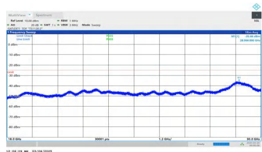
NTNV-DC_2A-n41A-PC2-30-5+80-M+L-QPSK-IDLE-DFT-QPSK-Inner_1RB_Right-18000-30000-PASS
