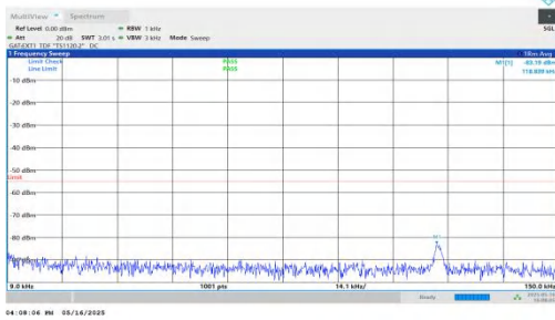
NTNV-DC_2A-n41A-PC2-30-5+80-M+M-QPSK-IDLE-DFT-BPSK-In ner_1RB_Left-0.009-0.15-PASS
