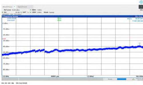
NTNV-DC_2A-n41A-PC2-30-5+80-M+L-QPSK-IDLE-DFT-QPSK-Inner_1RB_Left-3000-18000-PASS
