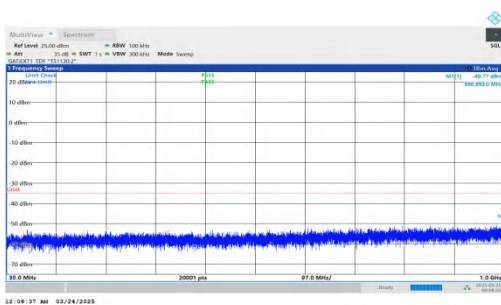
NTNV-DC_2A-n41A-PC2-30-5+80-M+M-QPSK-IDLE-DFT-QPSK-I nner_1RB_Left-30-1000-PASS
