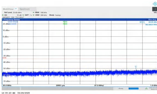
NTNV-DC_2A-n41A-PC2-30-5+80-M+L-QPSK-IDLE-DFT-QPSK-Inner_1RB_Right-30-1000-PASS
