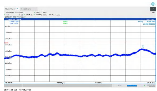
NTNV-DC_2A-n41A-PC2-30-5+80-M+L-QPSK-IDLE-DFT-BPSK-Inner_1RB_Right-18000-30000-PASS
