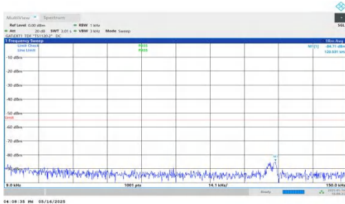
NTNV-DC_2A-n41A-PC2-30-5+80-M+M-QPSK-IDLE-DFT-BPSK-In ner_1RB_Right-0.009-0.15-PASS
