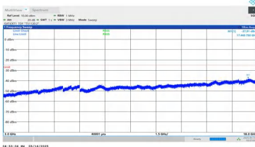
NTNV-DC_2A-n41A-PC2-30-5+80-M+L-QPSK-IDLE-DFT-BPSK-Inner_1RB_Left-3000-18000-PASS
