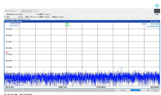
NTNV-DC_2A-n41A-PC2-30-5+40-M+M-QPSK-IDLE-DFT-BPSK-In ner_1RB_Right-0.15-30-PASS
