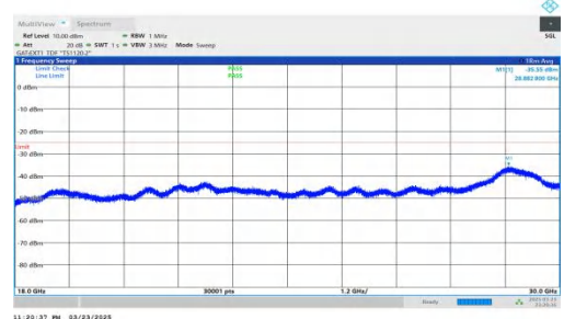
NTNV-DC_2A-n41A-PC2-30-5+40-M+H-QPSK-IDLE-DFT-BPSK-Inner_1RB_Left-18000-30000-PASS
