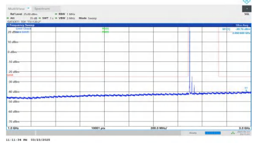
NTNV-DC_2A-n41A-PC2-30-5+40-M+L-QPSK-IDLE-DFT-BPSK-Inner_1RB_Left-1000-3000-PASS
