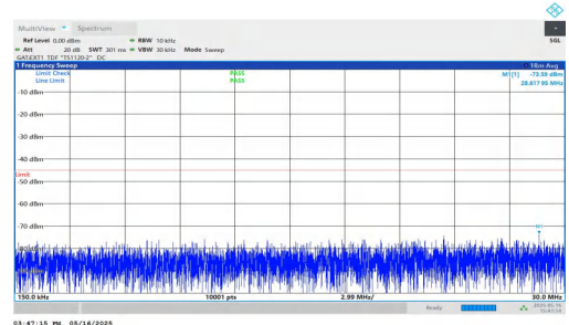
NTNV-DC_2A-n41A-PC2-30-5+50-M+L-QPSK-IDLE-DFT-BPSK-Inner_1RB_Right-0.15-30-PASS
