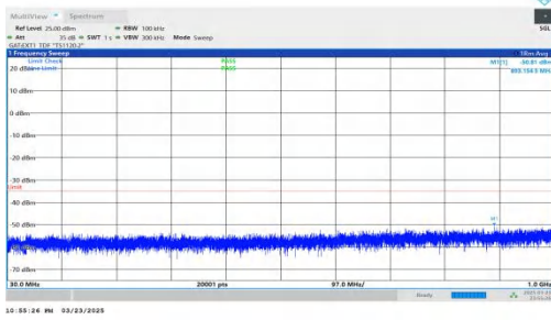
NTNV-DC_2A-n41A-PC2-30-5+20-M+H-QPSK-IDLE-DFT-BPSK-Inner_1RB_Right-30-1000-PASS
