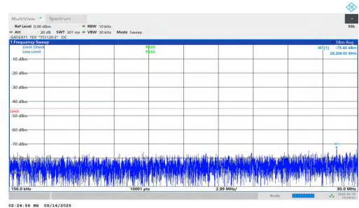
NTNV-DC_2A-n41A-PC2-30-5+20-M+M-QPSK-IDLE-DFT-QPSK-Inner_1RB_Right-0.15-30-PASS
