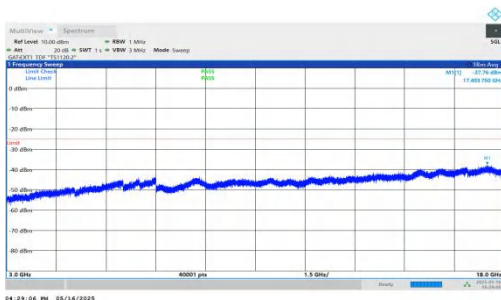
NTNV-DC_2A-n41A-PC2-30-5+20-M+M-QPSK-IDLE-DFT-BPSK-In ner_1RB_Left-3000-18000-PASS
