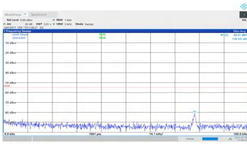
NTNV-DC_2A-n41A-PC2-30-5+40-M+L-QPSK-IDLE-DFT-BPSK-Inner_1RB_Right-0.009-0.15-PASS
