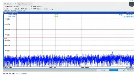
NTNV-DC_2A-n41A-PC2-30-5+30-M+H-QPSK-IDLE-DFT-BPSK-Inner_1RB_Left-0.15-30-PASS
