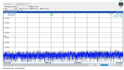
NTNV-DC_2A-n41A-PC2-30-5+30-M+M-QPSK-IDLE-DFT-BPSK-In ner_1RB_Left-0.15-30-PASS
