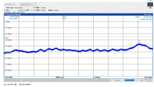
NTNV-DC_2A-n41A-PC2-30-5+40-M+M-QPSK-IDLE-DFT-QPSK-Inner_1RB_Left-18000-30000-PASS
