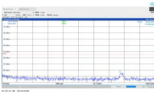
NTNV-DC_2A-n41A-PC2-30-5+20-M+H-QPSK-IDLE-DFT-QPSK-In ner_1RB_Right-0.009-0.15-PASS
