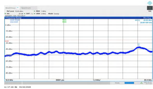
NTNV-DC_2A-n41A-PC2-30-5+40-M+M-QPSK-IDLE-DFT-BPSK-In ner_1RB_Right-18000-30000-PASS
