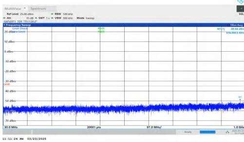
NTNV-DC_2A-n41A-PC2-30-5+40-M+L-QPSK-IDLE-DFT-BPSK-Inner_1RB_Left-30-1000-PASS
