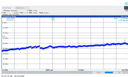
NTNV-DC_2A-n41A-PC2-30-5+30-M+H-QPSK-IDLE-DFT-BPSK-Inner_1RB_Left-3000-18000-PASS
