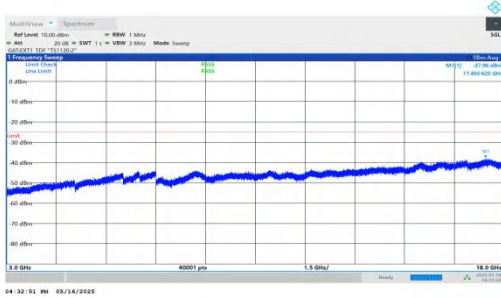
NTNV-DC_2A-n41A-PC2-30-5+30-M+M-QPSK-IDLE-DFT-QPSK-Inner_1RB_Left-3000-18000-PASS
