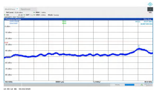
NTNV-DC_2A-n41A-PC2-30-5+20-M+H-QPSK-IDLE-DFT-BPSK-Inner_1RB_Left-18000-30000-PASS
