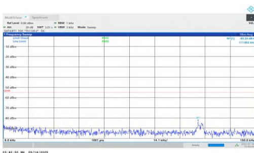
NTNV-DC_2A-n41A-PC2-30-5+40-M+M-QPSK-IDLE-DFT-BPSK-In ner_1RB_Right-0.009-0.15-PASS
