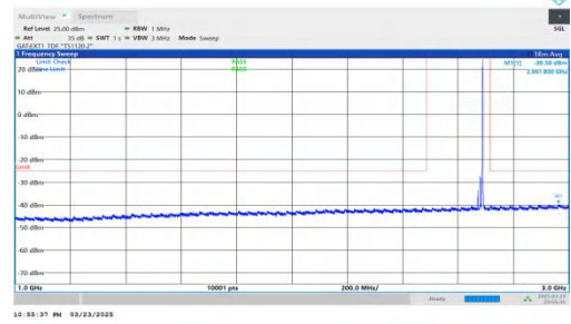
NTNV-DC_2A-n41A-PC2-30-5+20-M+H-QPSK-IDLE-DFT-BPSK-Inner_1RB_Right-1000-3000-PASS
