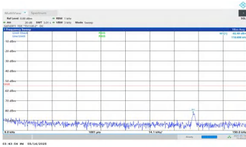
NTNV-DC_2A-n41A-PC2-30-5+40-M+M-QPSK-IDLE-DFT-QPSK-Inner_1RB_Right-0.009-0.15-PASS
