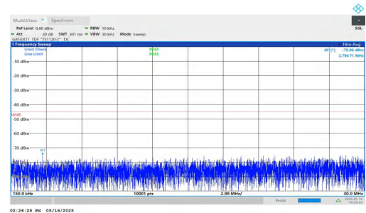
NTNV-DC_2A-n41A-PC2-30-5+20-M+M-QPSK-IDLE-DFT-QPSK-In ner_1RB_Left-0.15-30-PASS
