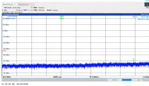
NTNV-DC_2A-n41A-PC2-30-5+30-M+M-QPSK-IDLE-DFT-BPSK-In ner_1RB_Right-30-1000-PASS
