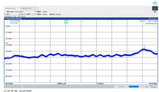
NTNV-DC_2A-n41A-PC2-30-5+30-M+H-QPSK-IDLE-DFT-BPSK-Inner_1RB_Right-18000-30000-PASS
