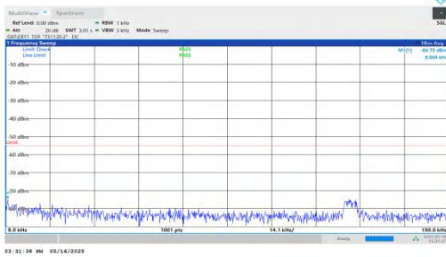
NTNV-DC_2A-n41A-PC2-30-5+20-M+H-QPSK-IDLE-DFT-BPSK-Inner_1RB_Left-0.009-0.15-PASS
