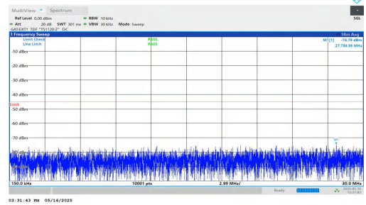
NTNV-DC_2A-n41A-PC2-30-5+20-M+H-QPSK-IDLE-DFT-BPSK-Inner_1RB_Left-0.15-30-PASS
