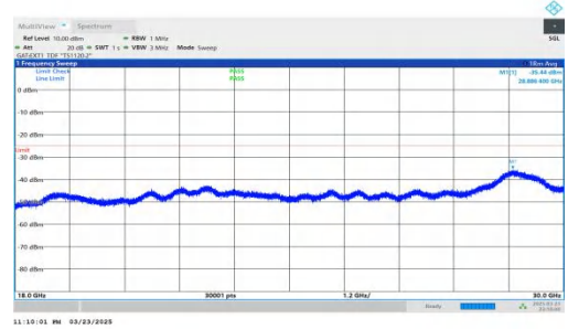
NTNV-DC_2A-n41A-PC2-30-5+30-M+H-QPSK-IDLE-DFT-QPSK-In ner_1RB_Left-18000-30000-PASS
