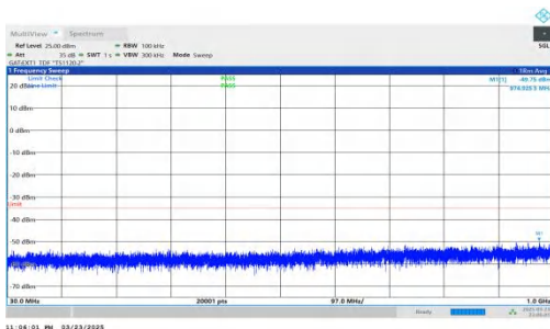
NTNV-DC_2A-n41A-PC2-30-5+30-M+M-QPSK-IDLE-DFT-QPSK-Inner_1RB_Right-30-1000-PASS
