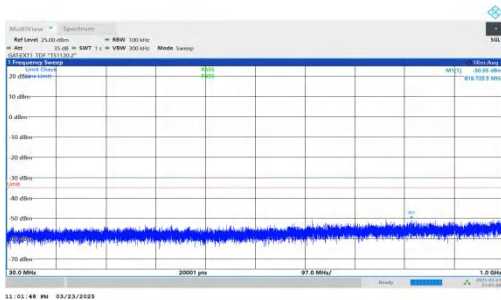
NTNV-DC_2A-n41A-PC2-30-5+30-M+L-QPSK-IDLE-DFT-QPSK-Inner_1RB_Right-30-1000-PASS
