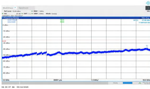
NTNV-DC_2A-n41A-PC2-30-5+30-M+L-QPSK-IDLE-DFT-BPSK-Inner_1RB_Right-3000-18000-PASS
