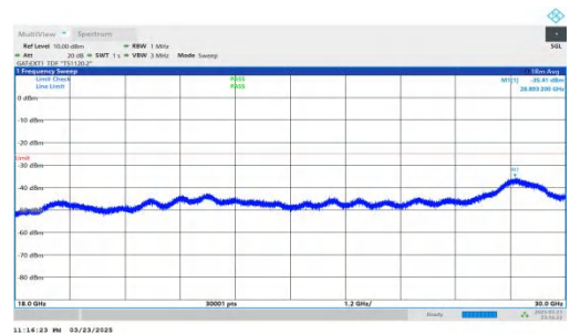
NTNV-DC_2A-n41A-PC2-30-5+40-M+M-QPSK-IDLE-DFT-BPSK-In ner_1RB_Left-18000-30000-PASS
