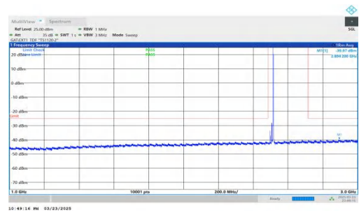
NTNV-DC_2A-n41A-PC2-30-5+20-M+L-QPSK-IDLE-DFT-QPSK-Inner_1RB_Right-1000-3000-PASS
