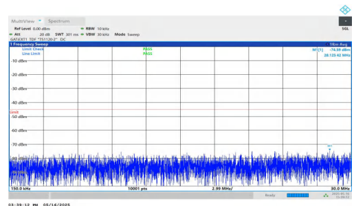
NTNV-DC_2A-n41A-PC2-30-5+30-M+H-QPSK-IDLE-DFT-QPSK-Inner_1RB_Left-0.15-30-PASS
