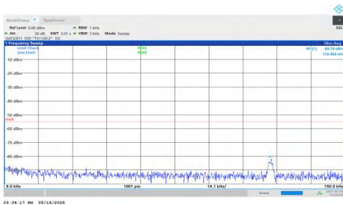
NTNV-DC_2A-n41A-PC2-30-5+30-M+L-QPSK-IDLE-DFT-BPSK-Inner_1RB_Right-0.009-0.15-PASS
