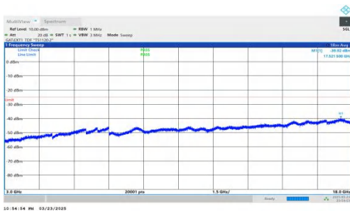
NTNV-DC_2A-n41A-PC2-30-5+20-M+H-QPSK-IDLE-DFT-BPSK-Inner_1RB_Left-3000-18000-PASS
