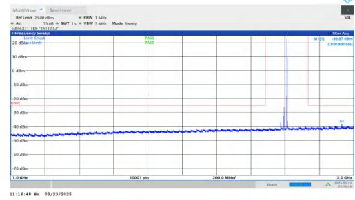
NTNV-DC_2A-n41A-PC2-30-5+40-M+M-QPSK-IDLE-DFT-BPSK-In ner_1RB_Right-1000-3000-PASS
