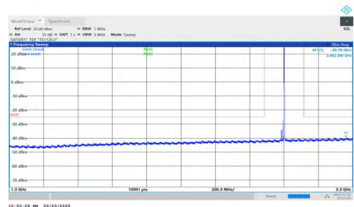
NTNV-DC_2A-n41A-PC2-30-5+20-M+M-QPSK-IDLE-DFT-QPSK-Inner_1RB_Right-1000-3000-PASS
