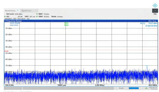
NTNV-DC_2A-n41A-PC2-30-5+20-M+M-QPSK-IDLE-DFT-BPSK-In ner_1RB_Right-0.15-30-PASS
