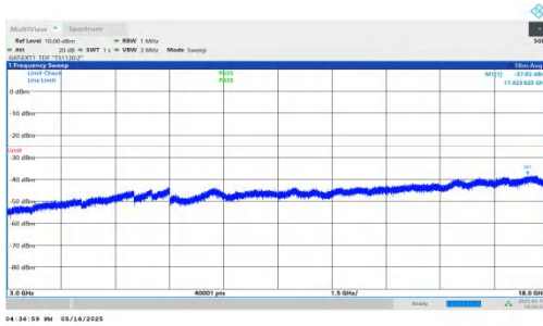
NTNV-DC_2A-n41A-PC2-30-5+40-M+M-QPSK-IDLE-DFT-BPSK-In ner_1RB_Right-3000-18000-PASS
