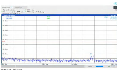
NTNV-DC_2A-n41A-PC2-30-5+20-M+H-QPSK-IDLE-DFT-BPSK-Inner_1RB_Right-0.009-0.15-PASS
