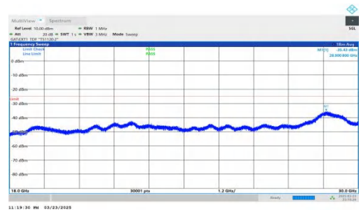
NTNV-DC_2A-n41A-PC2-30-5+40-M+M-QPSK-IDLE-DFT-QPSK-Inner_1RB_Right-18000-30000-PASS
