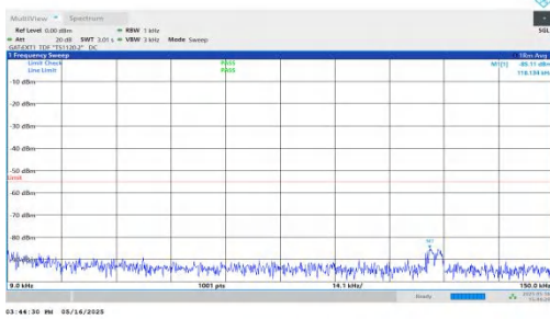
NTNV-DC_2A-n41A-PC2-30-5+40-M+H-QPSK-IDLE-DFT-BPSK-Inner_1RB_Left-0.009-0.15-PASS
