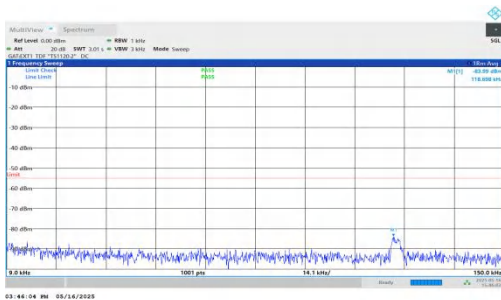
NTNV-DC_2A-n41A-PC2-30-5+40-M+H-QPSK-IDLE-DFT-QPSK-In ner_1RB_Right-0.009-0.15-PASS
