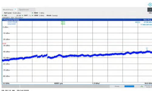
NTNV-DC_2A-n41A-PC2-30-5+40-M+H-QPSK-IDLE-DFT-QPSK-In ner_1RB_Right-3000-18000-PASS
