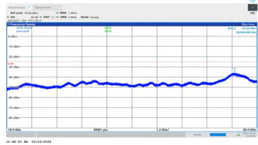
NTNV-DC_2A-n41A-PC2-30-5+20-M+L-QPSK-IDLE-DFT-QPSK-Inner_1RB_Left-18000-30000-PASS
