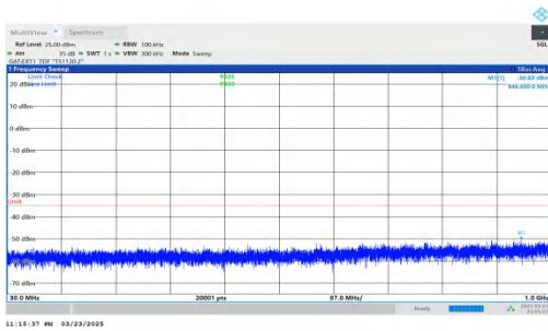
NTNV-DC_2A-n41A-PC2-30-5+40-M+M-QPSK-IDLE-DFT-BPSK-In ner_1RB_Left-30-1000-PASS
