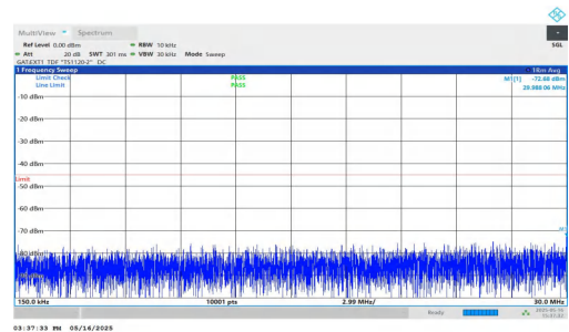
NTNV-DC_2A-n41A-PC2-30-5+30-M+M-QPSK-IDLE-DFT-QPSK-Inner_1RB_Right-0.15-30-PASS
