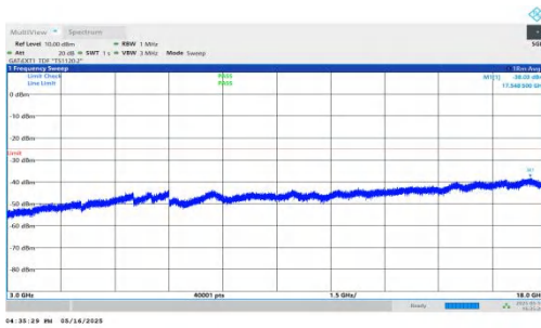
NTNV-DC_2A-n41A-PC2-30-5+40-M+L-QPSK-IDLE-DFT-BPSK-Inner_1RB_Right-3000-18000-PASS
