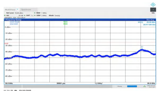
NTNV-DC_2A-n41A-PC2-30-5+30-M+H-QPSK-IDLE-DFT-QPSK-In ner_1RB_Right-18000-30000-PASS
