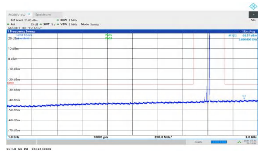
NTNV-DC_2A-n41A-PC2-30-5+40-M+M-QPSK-IDLE-DFT-QPSK-Inner_1RB_Right-1000-3000-PASS
