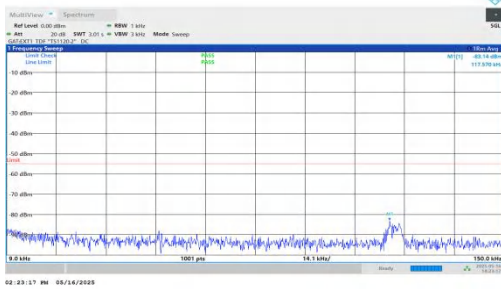
NTNV-DC_2A-n41A-PC2-30-5+20-M+M-QPSK-IDLE-DFT-BPSK-In ner_1RB_Left-0.009-0.15-PASS
