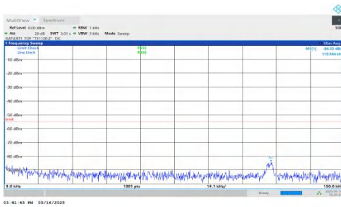
NTNV-DC_2A-n41A-PC2-30-5+40-M+L-QPSK-IDLE-DFT-QPSK-Inner_1RB_Right-0.009-0.15-PASS
