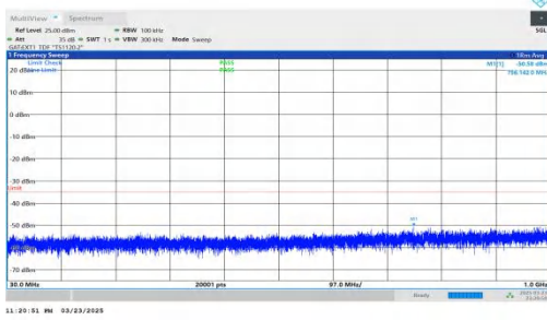
NTNV-DC_2A-n41A-PC2-30-5+40-M+H-QPSK-IDLE-DFT-BPSK-Inner_1RB_Right-30-1000-PASS
