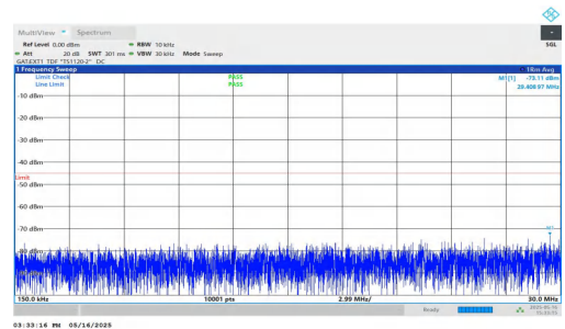
NTNV-DC_2A-n41A-PC2-30-5+20-M+H-QPSK-IDLE-DFT-QPSK-In ner_1RB_Right-0.15-30-PASS
