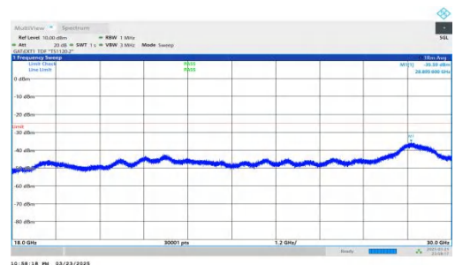
NTNV-DC_2A-n41A-PC2-30-5+20-M+H-QPSK-IDLE-DFT-QPSK-In ner_1RB_Right-18000-30000-PASS
