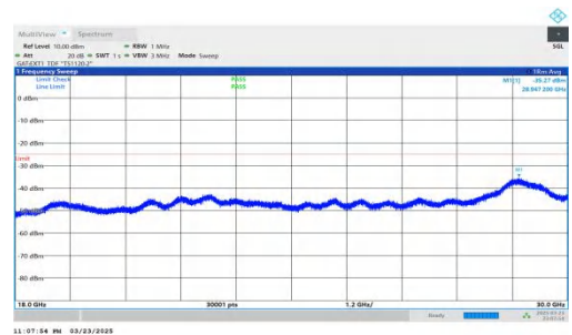
NTNV-DC_2A-n41A-PC2-30-5+30-M+H-QPSK-IDLE-DFT-BPSK-Inner_1RB_Left-18000-30000-PASS
