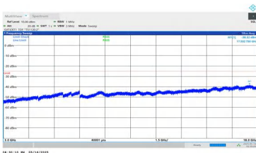
NTNV-DC_2A-n41A-PC2-30-5+20-M+M-QPSK-IDLE-DFT-QPSK-Inner_1RB_Right-3000-18000-PASS
