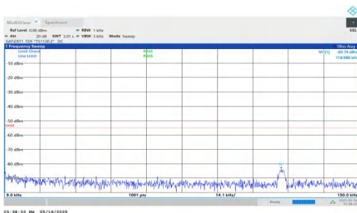
NTNV-DC_2A-n41A-PC2-30-5+30-M+H-QPSK-IDLE-DFT-BPSK-Inner_1RB_Right-0.009-0.15-PASS
