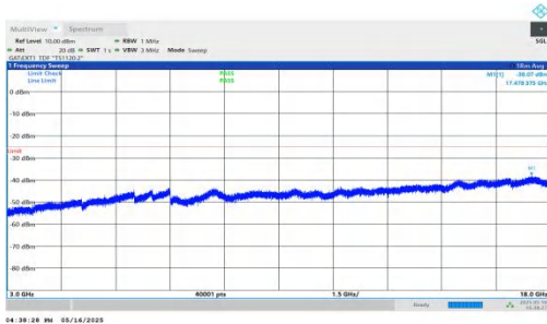
NTNV-DC_2A-n41A-PC2-30-5+40-M+H-QPSK-IDLE-DFT-BPSK-Inner_1RB_Right-3000-18000-PASS
