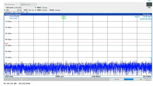
NTNV-DC_2A-n41A-PC2-30-5+40-M+M-QPSK-IDLE-DFT-BPSK-In ner_1RB_Left-0.15-30-PASS
