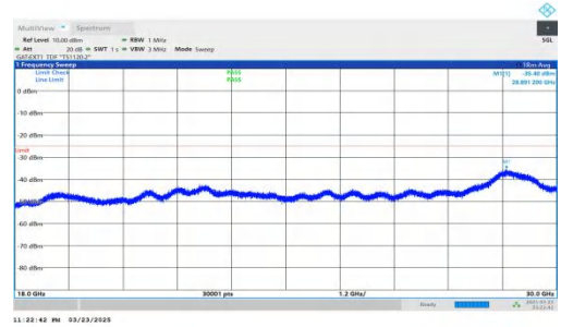
NTNV-DC_2A-n41A-PC2-30-5+40-M+H-QPSK-IDLE-DFT-QPSK-In ner_1RB_Left-18000-30000-PASS
