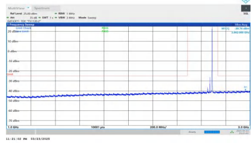
NTNV-DC_2A-n41A-PC2-30-5+40-M+H-QPSK-IDLE-DFT-BPSK-Inner_1RB_Right-1000-3000-PASS
