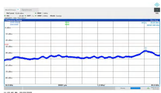
NTNV-DC_2A-n41A-PC2-30-5+40-M+H-QPSK-IDLE-DFT-QPSK-In ner_1RB_Right-18000-30000-PASS
