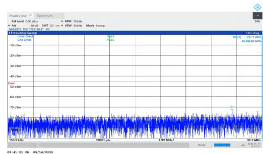
NTNV-DC_2A-n41A-PC2-30-5+40-M+L-QPSK-IDLE-DFT-QPSK-Inner_1RB_Left-0.15-30-PASS
