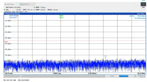
NTNV-DC_2A-n41A-PC2-30-5+20-M+M-QPSK-IDLE-DFT-BPSK-In ner_1RB_Left-0.15-30-PASS
