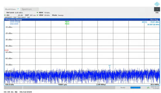
NTNV-DC_2A-n41A-PC2-30-5+30-M+H-QPSK-IDLE-DFT-QPSK-In ner_1RB_Right-0.15-30-PASS
