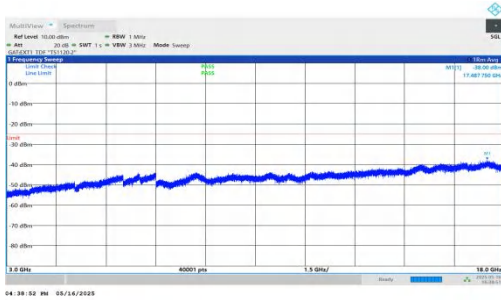
NTNV-DC_2A-n41A-PC2-30-5+40-M+H-QPSK-IDLE-DFT-QPSK-In ner_1RB_Left-3000-18000-PASS
