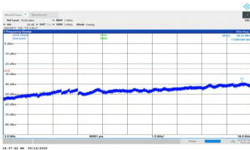
NTNV-DC_2A-n41A-PC2-30-5+40-M+M-QPSK-IDLE-DFT-QPSK-Inner_1RB_Right-3000-18000-PASS
