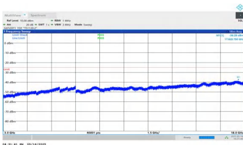
NTNV-DC_2A-n41A-PC2-30-5+30-M+L-QPSK-IDLE-DFT-QPSK-Inner_1RB_Right-3000-18000-PASS
