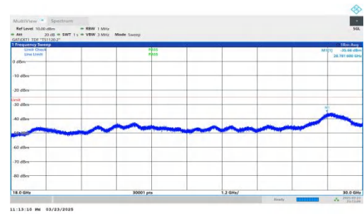
NTNV-DC_2A-n41A-PC2-30-5+40-M+L-QPSK-IDLE-DFT-BPSK-Inner_1RB_Right-18000-30000-PASS
