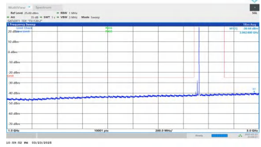
NTNV-DC_2A-n41A-PC2-30-5+30-M+L-QPSK-IDLE-DFT-BPSK-Inner_1RB_Right-1000-3000-PASS
