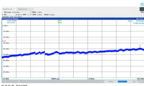
NTNV-DC_2A-n41A-PC2-30-5+30-M+H-QPSK-IDLE-DFT-QPSK-In ner_1RB_Right-3000-18000-PASS
