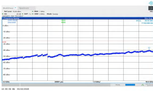
NTNV-DC_2A-n41A-PC2-30-5+20-M+H-QPSK-IDLE-DFT-BPSK-Inner_1RB_Right-3000-18000-PASS
