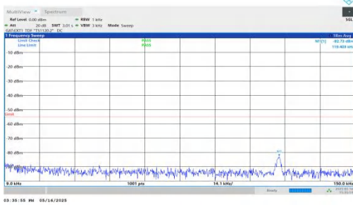
NTNV-DC_2A-n41A-PC2-30-5+30-M+M-QPSK-IDLE-DFT-BPSK-In ner_1RB_Left-0.009-0.15-PASS
