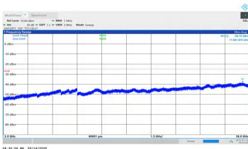
NTNV-DC_2A-n41A-PC2-30-5+30-M+M-QPSK-IDLE-DFT-BPSK-In ner_1RB_Left-3000-18000-PASS
