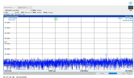
NTNV-DC_2A-n41A-PC2-30-5+30-M+M-QPSK-IDLE-DFT-QPSK-In ner_1RB_Left-0.15-30-PASS
