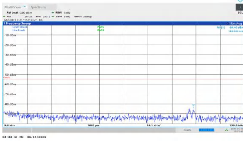
NTNV-DC_2A-n41A-PC2-30-5+30-M+L-QPSK-IDLE-DFT-BPSK-Inner_1RB_Left-0.009-0.15-PASS
