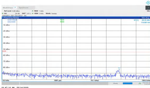
NTNV-DC_2A-n41A-PC2-30-5+50-M+L-QPSK-IDLE-DFT-BPSK-Inner_1RB_Right-0.009-0.15-PASS
