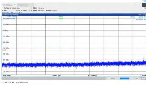
NTNV-DC_2A-n41A-PC2-30-5+40-M+L-QPSK-IDLE-DFT-BPSK-Inner_1RB_Right-30-1000-PASS
