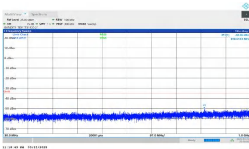
NTNV-DC_2A-n41A-PC2-30-5+40-M+M-QPSK-IDLE-DFT-QPSK-Inner_1RB_Right-30-1000-PASS
