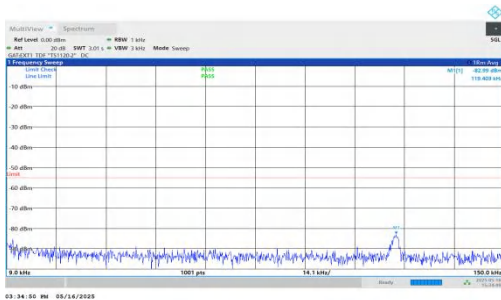
NTNV-DC_2A-n41A-PC2-30-5+30-M+L-QPSK-IDLE-DFT-QPSK-Inner_1RB_Left-0.009-0.15-PASS
