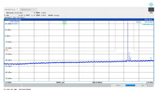
NTNV-DC_2A-n41A-PC2-30-5+40-M+H-QPSK-IDLE-DFT-QPSK-Inner_1RB_Left-1000-3000-PASS
