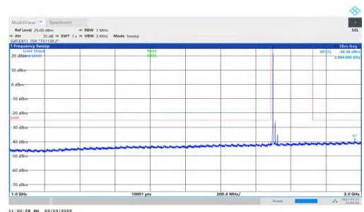
NTNV-DC_2A-n41A-PC2-30-5+30-M+L-QPSK-IDLE-DFT-QPSK-Inner_1RB_Left-1000-3000-PASS
