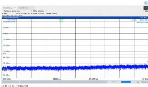
NTNV-DC_2A-n41A-PC2-30-5+20-M+M-QPSK-IDLE-DFT-BPSK-In ner_1RB_Left-30-1000-PASS
