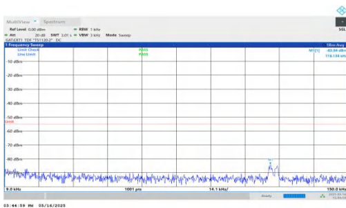
NTNV-DC_2A-n41A-PC2-30-5+40-M+H-QPSK-IDLE-DFT-BPSK-Inner_1RB_Right-0.009-0.15-PASS
