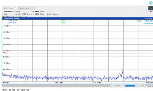
NTNV-DC_2A-n41A-PC2-30-5+30-M+L-QPSK-IDLE-DFT-QPSK-Inner_1RB_Right-0.009-0.15-PASS
