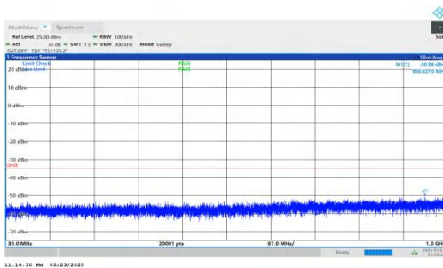
NTNV-DC_2A-n41A-PC2-30-5+40-M+L-QPSK-IDLE-DFT-QPSK-Inner_1RB_Right-30-1000-PASS
