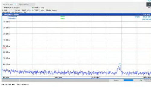
NTNV-DC_2A-n41A-PC2-30-5+30-M+H-QPSK-IDLE-DFT-BPSK-Inner_1RB_Left-0.009-0.15-PASS
