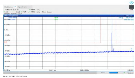
NTNV-DC_2A-n41A-PC2-30-5+30-M+H-QPSK-IDLE-DFT-BPSK-Inner_1RB_Left-1000-3000-PASS
