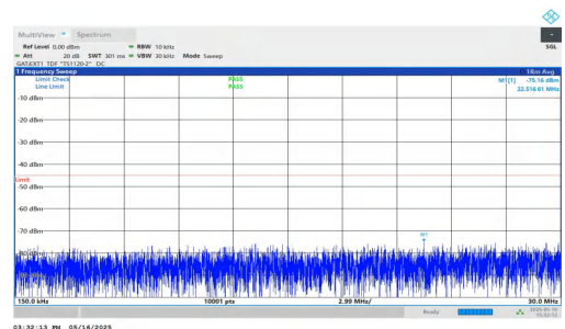
NTNV-DC_2A-n41A-PC2-30-5+20-M+H-QPSK-IDLE-DFT-BPSK-Inner_1RB_Right-0.15-30-PASS
