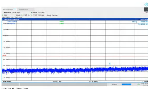
NTNV-DC_2A-n41A-PC2-30-5+40-M+M-QPSK-IDLE-DFT-QPSK-In ner_1RB_Left-30-1000-PASS
