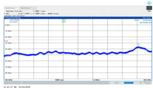
NTNV-DC_2A-n41A-PC2-30-5+40-M+H-QPSK-IDLE-DFT-BPSK-Inner_1RB_Right-18000-30000-PASS
