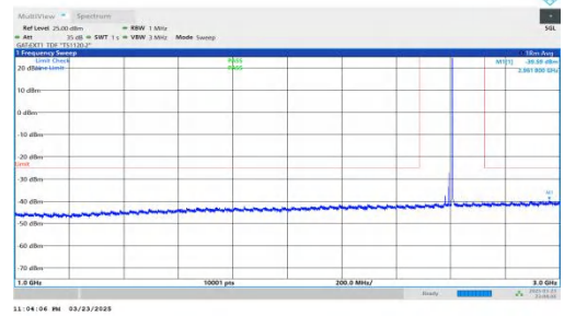
NTNV-DC_2A-n41A-PC2-30-5+30-M+M-QPSK-IDLE-DFT-BPSK-In ner_1RB_Right-1000-3000-PASS
