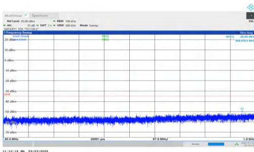
NTNV-DC_2A-n41A-PC2-30-5+30-M+H-QPSK-IDLE-DFT-QPSK-In ner_1RB_Right-30-1000-PASS
