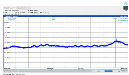
NTNV-DC_2A-n41A-PC2-30-5+30-M+L-QPSK-IDLE-DFT-QPSK-Inner_1RB_Right-18000-30000-PASS
