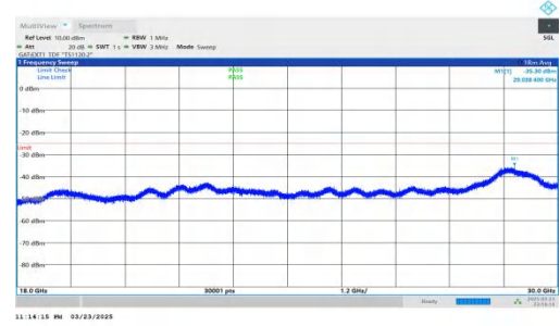
NTNV-DC_2A-n41A-PC2-30-5+40-M+L-QPSK-IDLE-DFT-QPSK-Inner_1RB_Left-18000-30000-PASS
