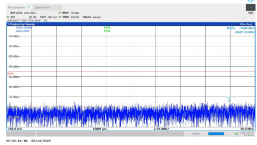
NTNV-DC_2A-n41A-PC2-30-5+50-M+L-QPSK-IDLE-DFT-BPSK-Inner_1RB_Left-0.15-30-PASS
