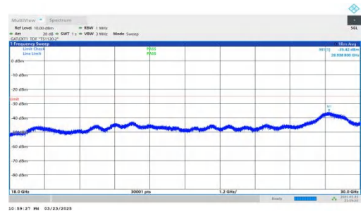
NTNV-DC_2A-n41A-PC2-30-5+30-M+L-QPSK-IDLE-DFT-BPSK-Inner_1RB_Left-18000-30000-PASS
