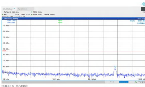
NTNV-DC_2A-n41A-PC2-30-5+40-M+L-QPSK-IDLE-DFT-QPSK-Inner_1RB_Left-0.009-0.15-PASS
