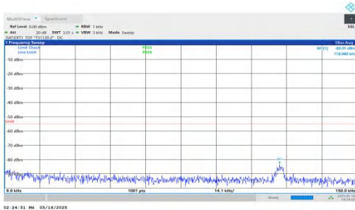
NTNV-DC_2A-n41A-PC2-30-5+20-M+M-QPSK-IDLE-DFT-QPSK-Inner_1RB_Right-0.009-0.15-PASS
