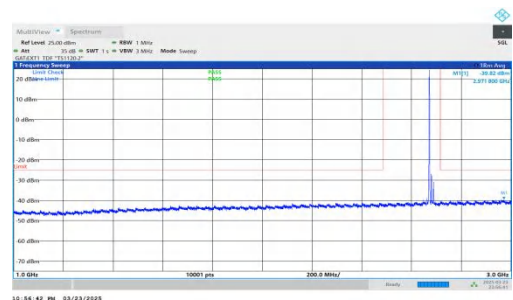
NTNV-DC_2A-n41A-PC2-30-5+20-M+H-QPSK-IDLE-DFT-QPSK-Inner_1RB_Left-1000-3000-PASS
