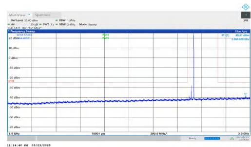
NTNV-DC_2A-n41A-PC2-30-5+40-M+L-QPSK-IDLE-DFT-QPSK-Inner_1RB_Right-1000-3000-PASS
