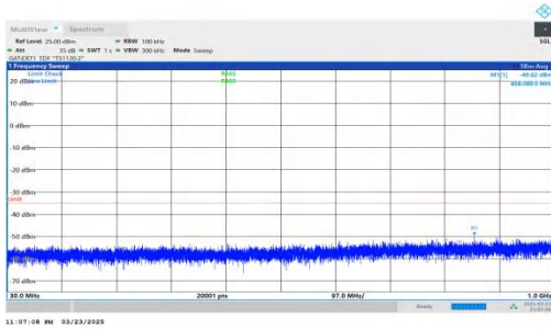
NTNV-DC_2A-n41A-PC2-30-5+30-M+H-QPSK-IDLE-DFT-BPSK-Inner_1RB_Left-30-1000-PASS
