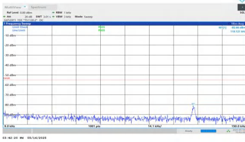
NTNV-DC_2A-n41A-PC2-30-5+40-M+M-QPSK-IDLE-DFT-BPSK-In ner_1RB_Left-0.009-0.15-PASS
