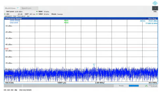
NTNV-DC_2A-n41A-PC2-30-5+40-M+M-QPSK-IDLE-DFT-QPSK-Inner_1RB_Right-0.15-30-PASS
