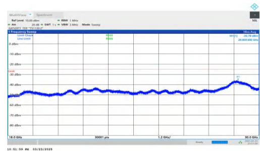
NTNV-DC_2A-n41A-PC2-30-5+20-M+M-QPSK-IDLE-DFT-BPSK-In ner_1RB_Right-18000-30000-PASS
