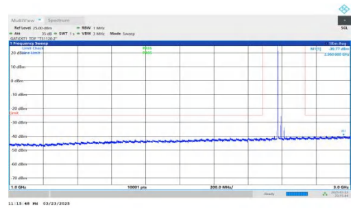
NTNV-DC_2A-n41A-PC2-30-5+40-M+M-QPSK-IDLE-DFT-BPSK-In ner_1RB_Left-1000-3000-PASS
