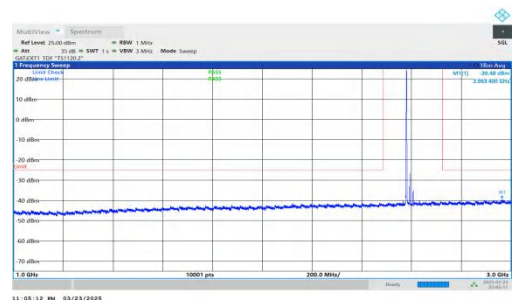
NTNV-DC_2A-n41A-PC2-30-5+30-M+M-QPSK-IDLE-DFT-QPSK-In ner_1RB_Left-1000-3000-PASS
