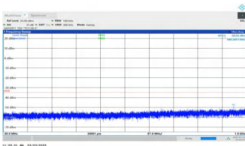
NTNV-DC_2A-n41A-PC2-30-5+30-M+M-QPSK-IDLE-DFT-QPSK-I nner_1RB_Left-30-1000-PASS
