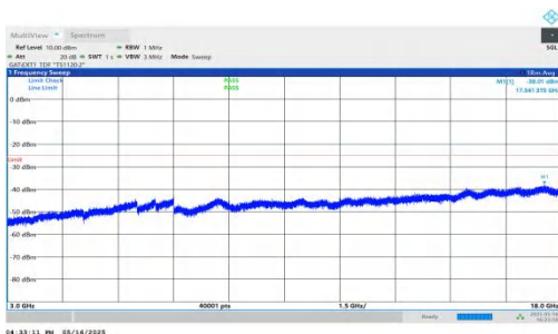
NTNV-DC_2A-n41A-PC2-30-5+30-M+M-QPSK-IDLE-DFT-QPSK-Inner_1RB_Right-3000-18000-PASS
