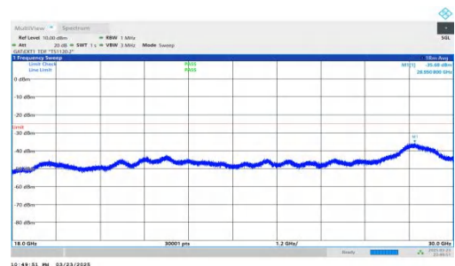
NTNV-DC_2A-n41A-PC2-30-5+20-M+L-QPSK-IDLE-DFT-QPSK-Inner_1RB_Right-18000-30000-PASS
