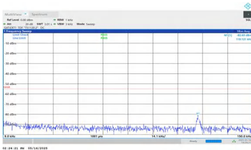
NTNV-DC_2A-n41A-PC2-30-5+20-M+M-QPSK-IDLE-DFT-QPSK-I nner_1RB_Left-0.009-0.15-PASS
