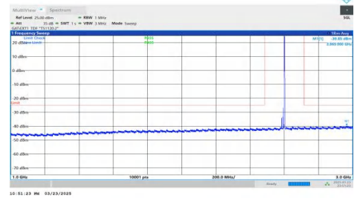
NTNV-DC_2A-n41A-PC2-30-5+20-M+M-QPSK-IDLE-DFT-BPSK-In ner_1RB_Right-1000-3000-PASS
