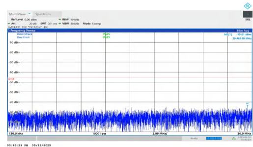
NTNV-DC_2A-n41A-PC2-30-5+40-M+M-QPSK-IDLE-DFT-QPSK-In ner_1RB_Left-0.15-30-PASS
