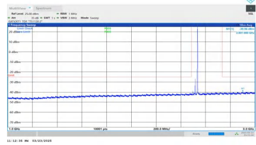
NTNV-DC_2A-n41A-PC2-30-5+40-M+L-QPSK-IDLE-DFT-BPSK-Inner_1RB_Right-1000-3000-PASS
