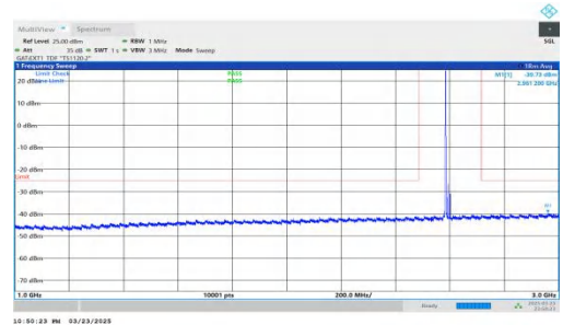
NTNV-DC_2A-n41A-PC2-30-5+20-M+M-QPSK-IDLE-DFT-BPSK-In ner_1RB_Left-1000-3000-PASS
