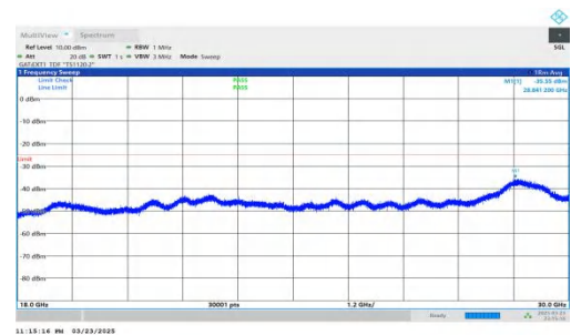
NTNV-DC_2A-n41A-PC2-30-5+40-M+L-QPSK-IDLE-DFT-QPSK-Inner_1RB_Right-18000-30000-PASS
