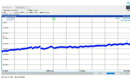
NTNV-DC_2A-n41A-PC2-30-5+30-M+L-QPSK-IDLE-DFT-BPSK-Inner_1RB_Left-3000-18000-PASS
