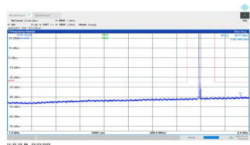
NTNV-DC_2A-n41A-PC2-30-5+20-M+M-QPSK-IDLE-DFT-QPSK-In ner_1RB_Left-1000-3000-PASS
