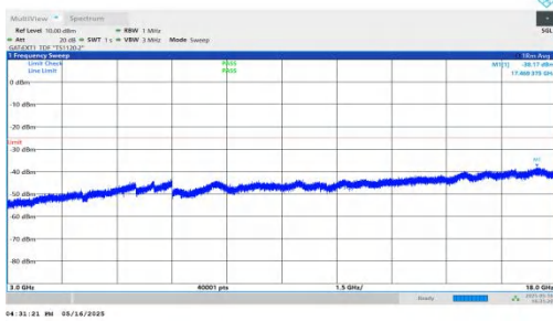
NTNV-DC_2A-n41A-PC2-30-5+30-M+L-QPSK-IDLE-DFT-QPSK-Inner_1RB_Left-3000-18000-PASS
