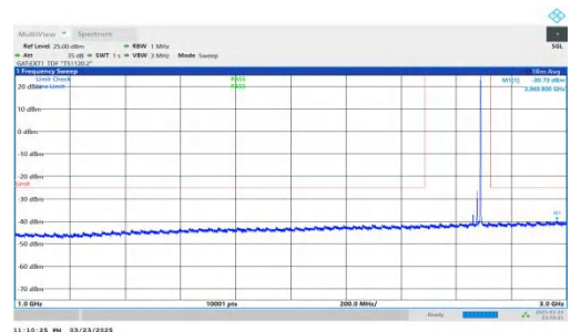
NTNV-DC_2A-n41A-PC2-30-5+30-M+H-QPSK-IDLE-DFT-QPSK-In ner_1RB_Right-1000-3000-PASS
