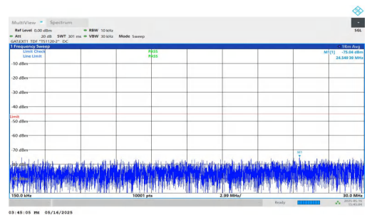
NTNV-DC_2A-n41A-PC2-30-5+40-M+H-QPSK-IDLE-DFT-BPSK-Inner_1RB_Right-0.15-30-PASS
