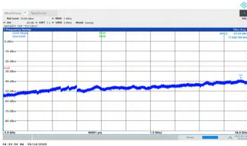
NTNV-DC_2A-n41A-PC2-30-5+30-M+H-QPSK-IDLE-DFT-BPSK-Inner_1RB_Right-3000-18000-PASS
