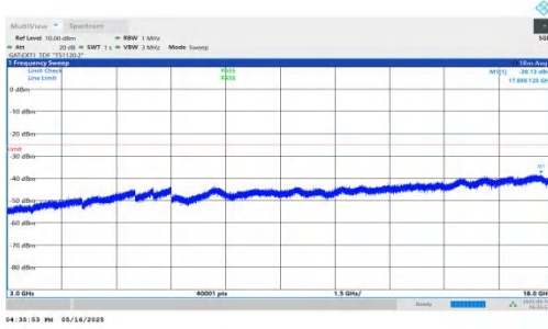
NTNV-DC_2A-n41A-PC2-30-5+40-M+L-QPSK-IDLE-DFT-QPSK-Inner_1RB_Left-3000-18000-PASS
