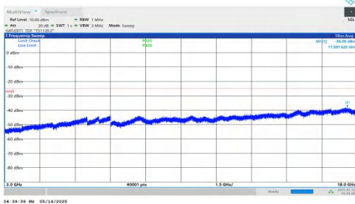
NTNV-DC_2A-n41A-PC2-30-5+50-M+L-QPSK-IDLE-DFT-BPSK-Inner_1RB_Left-3000-18000-PASS
