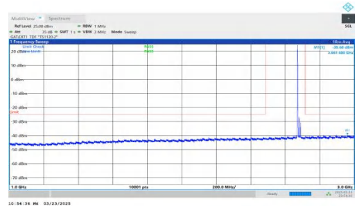
NTNV-DC_2A-n41A-PC2-30-5+20-M+H-QPSK-IDLE-DFT-BPSK-Inner_1RB_Left-1000-3000-PASS
