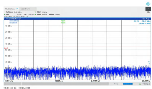
NTNV-DC_2A-n41A-PC2-30-5+30-M+L-QPSK-IDLE-DFT-BPSK-Inner_1RB_Right-0.15-30-PASS
