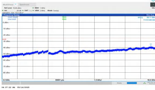
NTNV-DC_2A-n41A-PC2-30-5+40-M+M-QPSK-IDLE-DFT-QPSK-Inner_1RB_Left-3000-18000-PASS
