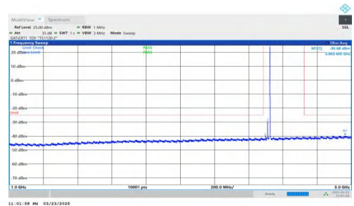
NTNV-DC_2A-n41A-PC2-30-5+30-M+L-QPSK-IDLE-DFT-QPSK-Inner_1RB_Right-1000-3000-PASS
