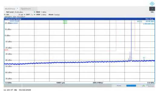
NTNV-DC_2A-n41A-PC2-30-5+40-M+H-QPSK-IDLE-DFT-QPSK-In ner_1RB_Right-1000-3000-PASS
