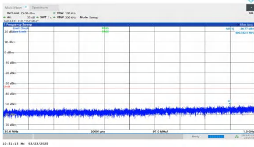
NTNV-DC_2A-n41A-PC2-30-5+20-M+M-QPSK-IDLE-DFT-BPSK-In ner_1RB_Right-30-1000-PASS
