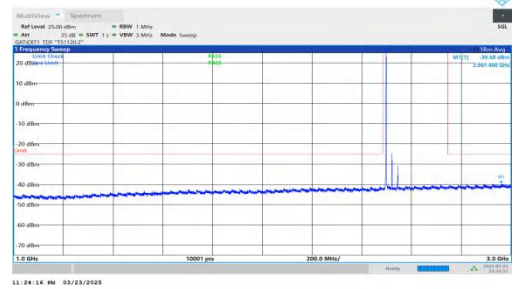
NTNV-DC_2A-n41A-PC2-30-5+50-M+L-QPSK-IDLE-DFT-BPSK-Inner_1RB_Left-1000-3000-PASS
