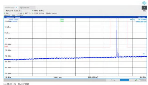
NTNV-DC_2A-n41A-PC2-30-5+30-M+M-QPSK-IDLE-DFT-BPSK-In ner_1RB_Left-1000-3000-PASS
