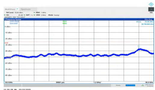
NTNV-DC_2A-n41A-PC2-30-5+20-M+M-QPSK-IDLE-DFT-BPSK-In ner_1RB_Left-18000-30000-PASS
