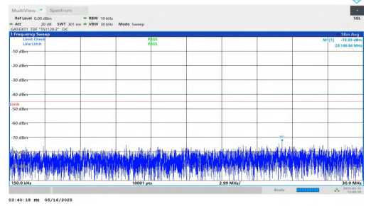
NTNV-DC_2A-n41A-PC2-30-5+40-M+L-QPSK-IDLE-DFT-BPSK-Inner_1RB_Left-0.15-30-PASS
