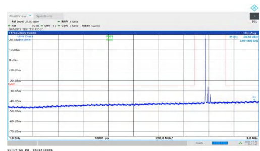
NTNV-DC_2A-n41A-PC2-30-5+40-M+M-QPSK-IDLE-DFT-QPSK-In ner_1RB_Left-1000-3000-PASS
