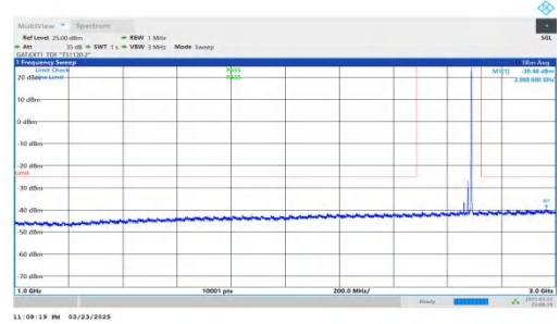
NTNV-DC_2A-n41A-PC2-30-5+30-M+H-QPSK-IDLE-DFT-BPSK-Inner_1RB_Right-1000-3000-PASS
