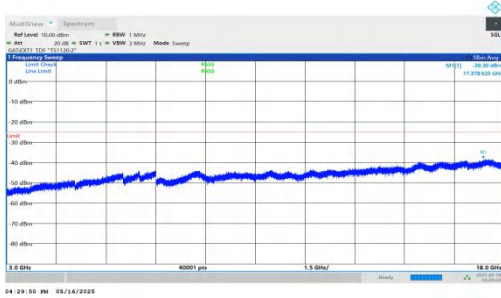
NTNV-DC_2A-n41A-PC2-30-5+20-M+M-QPSK-IDLE-DFT-QPSK-Inner_1RB_Left-3000-18000-PASS
