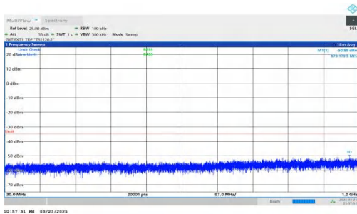
NTNV-DC_2A-n41A-PC2-30-5+20-M+H-QPSK-IDLE-DFT-QPSK-In ner_1RB_Right-30-1000-PASS
