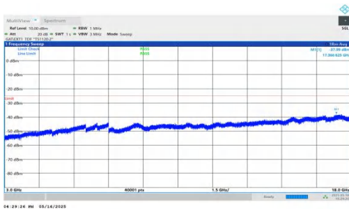
NTNV-DC_2A-n41A-PC2-30-5+20-M+M-QPSK-IDLE-DFT-BPSK-In ner_1RB_Right-3000-18000-PASS
