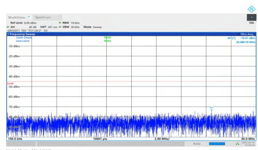
NTNV-DC_2A-n41A-PC2-30-5+30-M+M-QPSK-IDLE-DFT-BPSK-In ner_1RB_Right-0.15-30-PASS
