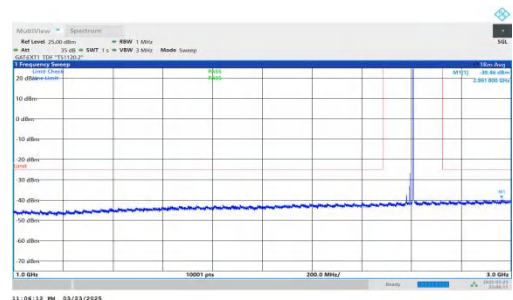
NTNV-DC_2A-n41A-PC2-30-5+30-M+M-QPSK-IDLE-DFT-QPSK-Inner_1RB_Right-1000-3000-PASS
