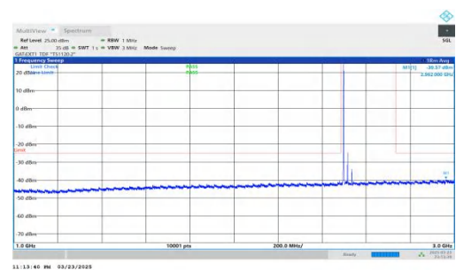
NTNV-DC_2A-n41A-PC2-30-5+40-M+L-QPSK-IDLE-DFT-QPSK-Inner_1RB_Left-1000-3000-PASS
