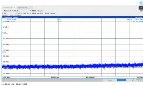
NTNV-DC_2A-n41A-PC2-30-5+30-M+L-QPSK-IDLE-DFT-BPSK-Inner_1RB_Left-30-1000-PASS
