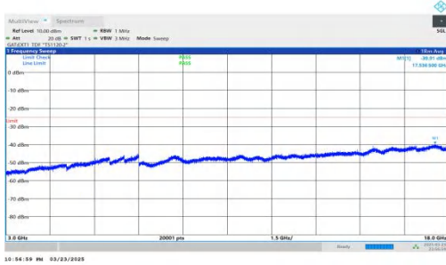
NTNV-DC_2A-n41A-PC2-30-5+20-M+H-QPSK-IDLE-DFT-QPSK-In ner_1RB_Left-3000-18000-PASS
