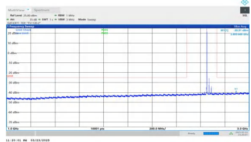
NTNV-DC_2A-n41A-PC2-30-5+40-M+H-QPSK-IDLE-DFT-BPSK-Inner_1RB_Left-1000-3000-PASS
