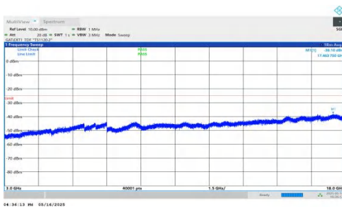
NTNV-DC_2A-n41A-PC2-30-5+40-M+L-QPSK-IDLE-DFT-QPSK-Inner_1RB_Right-3000-18000-PASS
