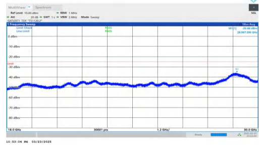
NTNV-DC_2A-n41A-PC2-30-5+20-M+M-QPSK-IDLE-DFT-QPSK-Inner_1RB_Left-18000-30000-PASS
