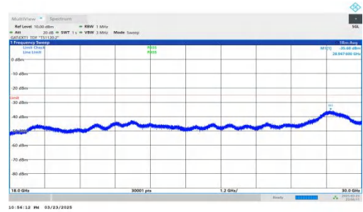
NTNV-DC_2A-n41A-PC2-30-5+20-M+H-QPSK-IDLE-DFT-BPSK-Inner_1RB_Right-18000-30000-PASS
