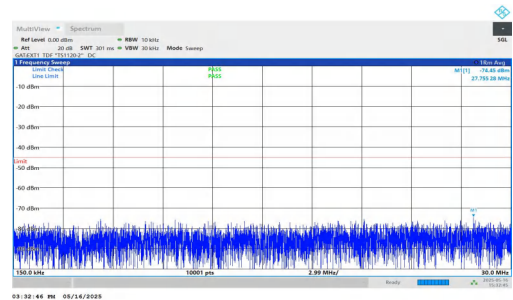
NTNV-DC_2A-n41A-PC2-30-5+20-M+H-QPSK-IDLE-DFT-QPSK-Inner_1RB_Left-0.15-30-PASS
