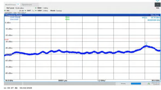
NTNV-DC_2A-n41A-PC2-30-5+30-M+M-QPSK-IDLE-DFT-QPSK-Inner_1RB_Left-18000-30000-PASS
