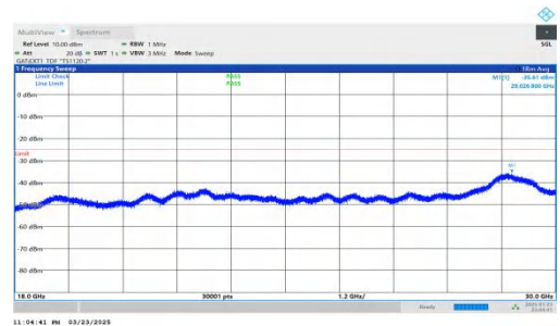
NTNV-DC_2A-n41A-PC2-30-5+30-M+M-QPSK-IDLE-DFT-BPSK-In ner_1RB_Right-18000-30000-PASS
