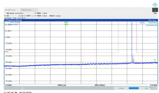
NTNV-DC_2A-n41A-PC2-30-5+30-M+H-QPSK-IDLE-DFT-QPSK-Inner_1RB_Left-1000-3000-PASS
