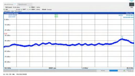
NTNV-DC_2A-n41A-PC2-30-5+30-M+L-QPSK-IDLE-DFT-QPSK-Inner_1RB_Left-18000-30000-PASS
