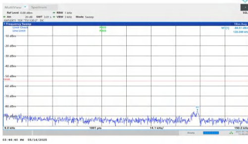
NTNV-DC_2A-n41A-PC2-30-5+50-M+L-QPSK-IDLE-DFT-BPSK-Inner_1RB_Left-0.009-0.15-PASS
