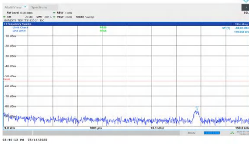
NTNV-DC_2A-n41A-PC2-30-5+40-M+L-QPSK-IDLE-DFT-BPSK-Inner_1RB_Left-0.009-0.15-PASS
