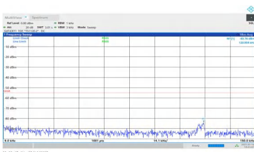
NTNV-DC_2A-n41A-PC2-30-5+20-M+M-QPSK-IDLE-DFT-BPSK-In ner_1RB_Right-0.009-0.15-PASS
