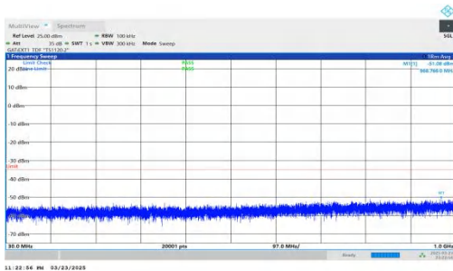
NTNV-DC_2A-n41A-PC2-30-5+40-M+H-QPSK-IDLE-DFT-QPSK-In ner_1RB_Right-30-1000-PASS
