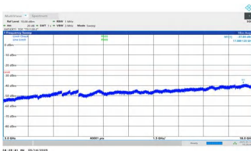
NTNV-DC_2A-n41A-PC2-30-5+20-M+L-QPSK-IDLE-DFT-QPSK-Inner_1RB_Right-3000-18000-PASS
