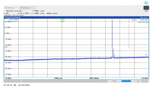
NTNV-DC_2A-n41A-PC2-30-5+30-M+L-QPSK-IDLE-DFT-BPSK-Inner_1RB_Left-1000-3000-PASS
