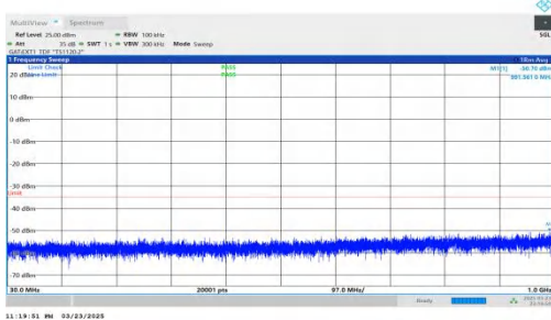
NTNV-DC_2A-n41A-PC2-30-5+40-M+H-QPSK-IDLE-DFT-BPSK-Inner_1RB_Left-30-1000-PASS
