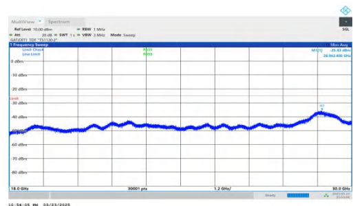
NTNV-DC_2A-n41A-PC2-30-5+20-M+M-QPSK-IDLE-DFT-QPSK-Inner_1RB_Right-18000-30000-PASS
