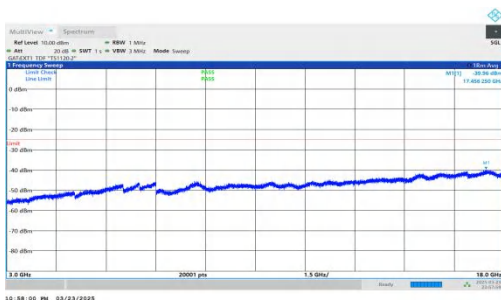
NTNV-DC_2A-n41A-PC2-30-5+20-M+H-QPSK-IDLE-DFT-QPSK-In ner_1RB_Right-3000-18000-PASS
