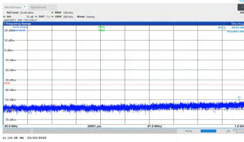
NTNV-DC_2A-n41A-PC2-30-5+40-M+M-QPSK-IDLE-DFT-BPSK-In ner_1RB_Right-30-1000-PASS
