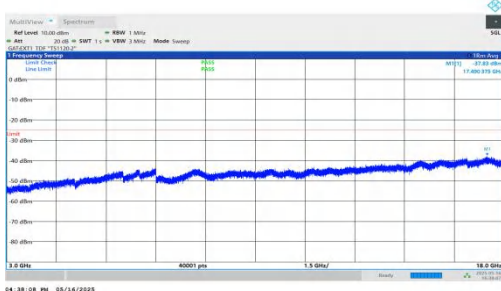
NTNV-DC_2A-n41A-PC2-30-5+40-M+H-QPSK-IDLE-DFT-BPSK-Inner_1RB_Left-3000-18000-PASS
