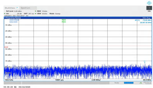
NTNV-DC_2A-n41A-PC2-30-5+30-M+L-QPSK-IDLE-DFT-QPSK-Inner_1RB_Right-0.15-30-PASS
