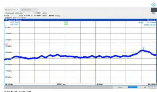
NTNV-DC_2A-n41A-PC2-30-5+30-M+M-QPSK-IDLE-DFT-QPSK-Inner_1RB_Right-18000-30000-PASS
