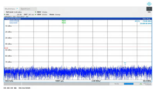
NTNV-DC_2A-n41A-PC2-30-5+40-M+H-QPSK-IDLE-DFT-QPSK-In ner_1RB_Right-0.15-30-PASS
