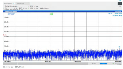
NTNV-DC_2A-n41A-PC2-30-5+30-M+L-QPSK-IDLE-DFT-BPSK-Inner_1RB_Left-0.15-30-PASS
