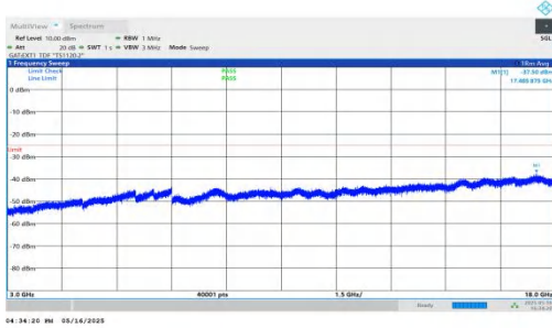
NTNV-DC_2A-n41A-PC2-30-5+30-M+H-QPSK-IDLE-DFT-QPSK-In ner_1RB_Left-3000-18000-PASS
