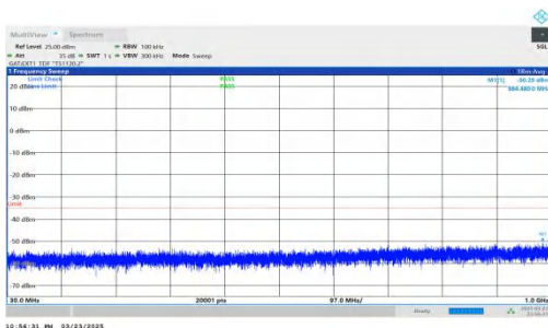
NTNV-DC_2A-n41A-PC2-30-5+20-M+H-QPSK-IDLE-DFT-QPSK-Inner_1RB_Left-30-1000-PASS
