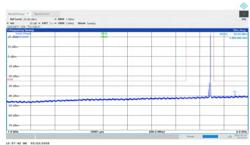
NTNV-DC_2A-n41A-PC2-30-5+20-M+H-QPSK-IDLE-DFT-QPSK-In ner_1RB_Right-1000-3000-PASS
