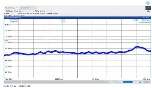
NTNV-DC_2A-n41A-PC2-30-5+30-M+L-QPSK-IDLE-DFT-BPSK-Inner_1RB_Right-18000-30000-PASS
