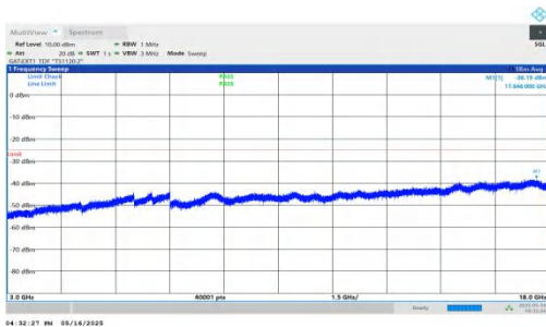
NTNV-DC_2A-n41A-PC2-30-5+30-M+M-QPSK-IDLE-DFT-BPSK-In ner_1RB_Right-3000-18000-PASS
