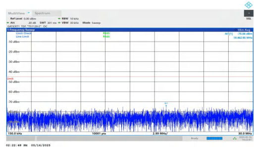
NTNV-DC_2A-n41A-PC2-30-5+20-M+L-QPSK-IDLE-DFT-QPSK-Inner_1RB_Right-0.15-30-PASS
