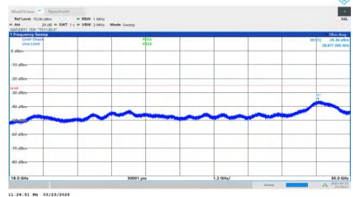
NTNV-DC_2A-n41A-PC2-30-5+50-M+L-QPSK-IDLE-DFT-BPSK-Inner_1RB_Left-18000-30000-PASS
