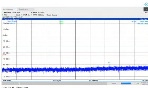
NTNV-DC_2A-n41A-PC2-30-5+40-M+H-QPSK-IDLE-DFT-QPSK-Inner_1RB_Left-30-1000-PASS
