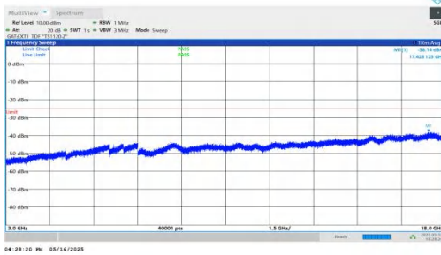
NTNV-DC_2A-n41A-PC2-30-5+20-M+L-QPSK-IDLE-DFT-QPSK-Inner_1RB_Left-3000-18000-PASS
