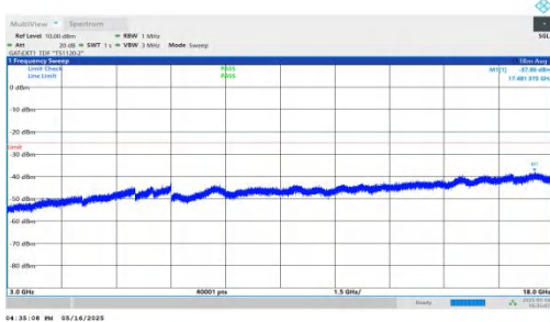
NTNV-DC_2A-n41A-PC2-30-5+40-M+L-QPSK-IDLE-DFT-BPSK-Inner_1RB_Left-3000-18000-PASS
