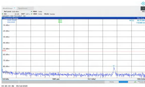
NTNV-DC_2A-n41A-PC2-30-5+40-M+H-QPSK-IDLE-DFT-QPSK-Inner_1RB_Left-0.009-0.15-PASS
