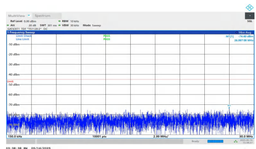
NTNV-DC_2A-n41A-PC2-30-5+30-M+H-QPSK-IDLE-DFT-BPSK-Inner_1RB_Right-0.15-30-PASS
