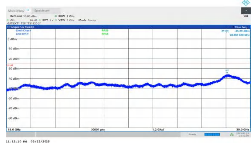
NTNV-DC_2A-n41A-PC2-30-5+40-M+L-QPSK-IDLE-DFT-BPSK-Inner_1RB_Left-18000-30000-PASS
