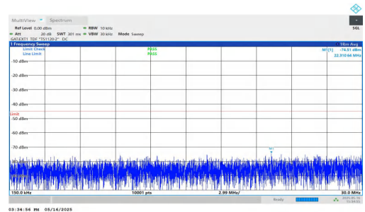
NTNV-DC_2A-n41A-PC2-30-5+30-M+L-QPSK-IDLE-DFT-QPSK-Inner_1RB_Left-0.15-30-PASS
