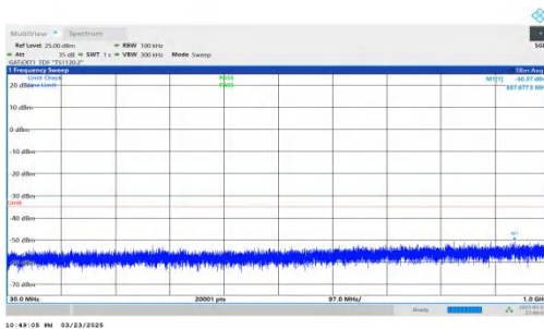
NTNV-DC_2A-n41A-PC2-30-5+20-M+L-QPSK-IDLE-DFT-QPSK-Inner_1RB_Right-30-1000-PASS
