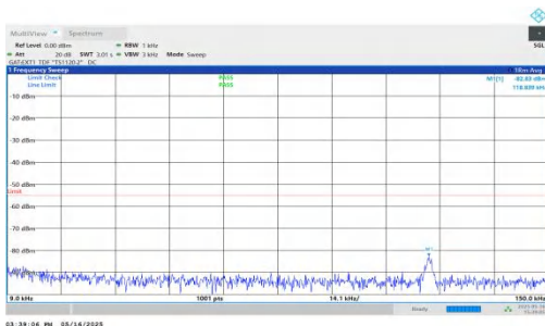
NTNV-DC_2A-n41A-PC2-30-5+30-M+H-QPSK-IDLE-DFT-QPSK-Inner_1RB_Left-0.009-0.15-PASS
