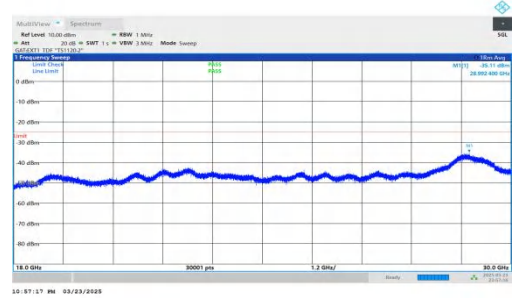
NTNV-DC_2A-n41A-PC2-30-5+20-M+H-QPSK-IDLE-DFT-QPSK-In ner_1RB_Left-18000-30000-PASS
