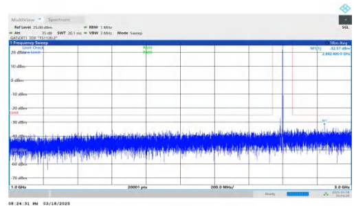
NTNV-DC_2A-n38A-PC3-30-5+30-M+L-QPSK-IDLE-DFT-QPSK-Inner_1RB_Right-1000-3000-PASS
