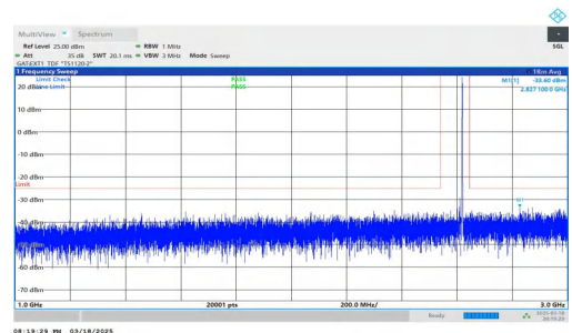
NTNV-DC_2A-n38A-PC3-30-5+20-M+H-QPSK-IDLE-DFT-QPSK-In ner_1RB_Right-1000-3000-PASS
