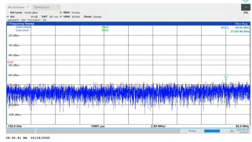
NTNV-DC_2A-n38A-PC3-30-5+30-M+H-QPSK-IDLE-DFT-BPSK-Inner_1RB_Left-0.15-30-PASS
