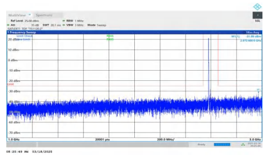
NTNV-DC_2A-n38A-PC3-30-5+30-M+M-QPSK-IDLE-DFT-BPSK-In ner_1RB_Left-1000-3000-PASS
