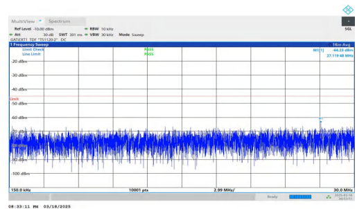
NTNV-DC_2A-n38A-PC3-30-5+30-M+H-QPSK-IDLE-DFT-QPSK-Inner_1RB_Left-0.15-30-PASS
