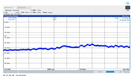
NTNV-DC_2A-n38A-PC3-30-5+40-M+L-QPSK-IDLE-DFT-BPSK-Inner_1RB_Right-12000-26500-PASS
