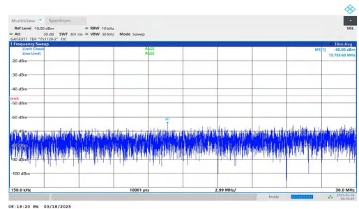
NTNV-DC_2A-n38A-PC3-30-5+20-M+H-QPSK-IDLE-DFT-QPSK-In ner_1RB_Right-0.15-30-PASS
