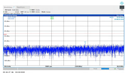
NTNV-DC_2A-n38A-PC3-30-5+40-M+M-QPSK-IDLE-DFT-QPSK-Inner_1RB_Right-0.15-30-PASS
