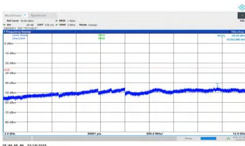
NTNV-DC_2A-n38A-PC3-30-5+40-M+M-QPSK-IDLE-DFT-QPSK-Inner_1RB_Right-3000-12000-PASS
