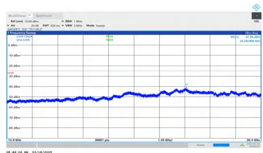
NTNV-DC_2A-n38A-PC3-30-5+40-M+H-QPSK-IDLE-DFT-BPSK-Inner_1RB_Left-12000-26500-PASS
