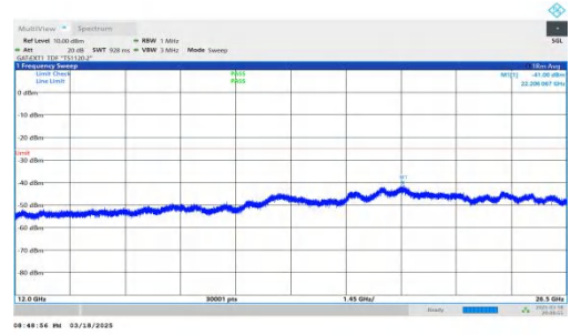
NTNV-DC_2A-n38A-PC3-30-5+40-M+H-QPSK-IDLE-DFT-QPSK-In ner_1RB_Left-12000-26500-PASS
