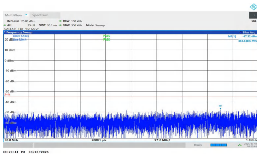
NTNV-DC_2A-n38A-PC3-30-5+30-M+L-QPSK-IDLE-DFT-BPSK-Inner_1RB_Left-30-1000-PASS
