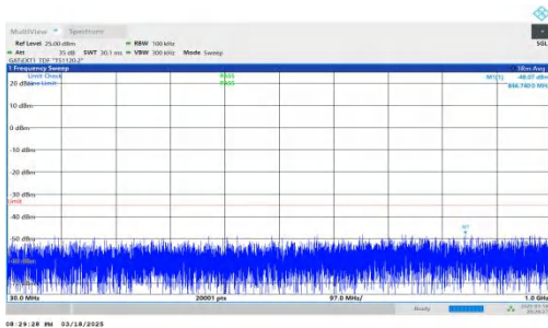
NTNV-DC_2A-n38A-PC3-30-5+30-M+M-QPSK-IDLE-DFT-QPSK-Inner_1RB_Right-30-1000-PASS
