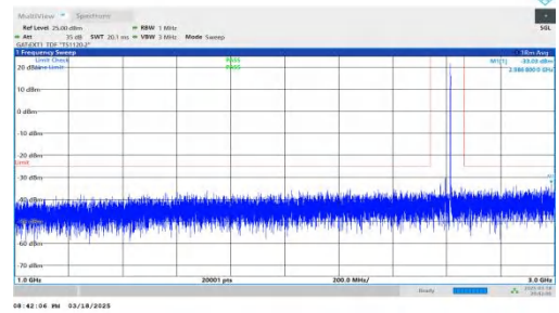
NTNV-DC_2A-n38A-PC3-30-5+40-M+M-QPSK-IDLE-DFT-BPSK-In ner_1RB_Right-1000-3000-PASS
