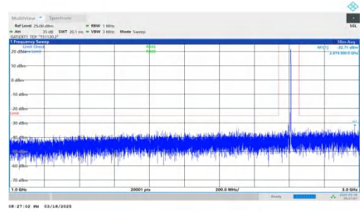
NTNV-DC_2A-n38A-PC3-30-5+30-M+M-QPSK-IDLE-DFT-BPSK-In ner_1RB_Right-1000-3000-PASS
