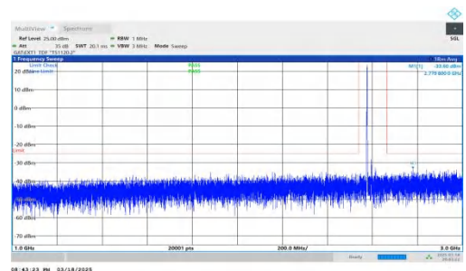
NTNV-DC_2A-n38A-PC3-30-5+40-M+M-QPSK-IDLE-DFT-QPSK-In ner_1RB_Left-1000-3000-PASS
