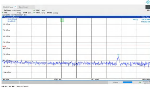
NTNV-DC_2A-n38A-PC3-30-5+20-M+H-QPSK-IDLE-DFT-BPSK-Inner_1RB_Left-0.009-0.15-PASS
