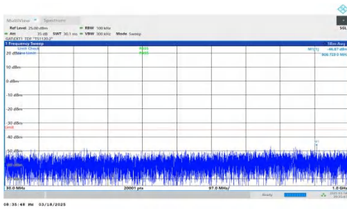
NTNV-DC_2A-n38A-PC3-30-5+40-M+L-QPSK-IDLE-DFT-BPSK-Inner_1RB_Left-30-1000-PASS
