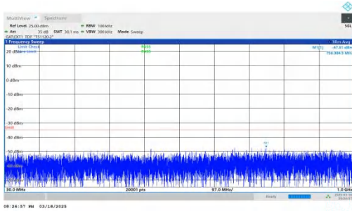
NTNV-DC_2A-n38A-PC3-30-5+30-M+M-QPSK-IDLE-DFT-BPSK-In ner_1RB_Right-30-1000-PASS
