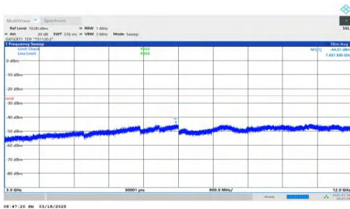
NTNV-DC_2A-n38A-PC3-30-5+40-M+H-QPSK-IDLE-DFT-BPSK-Inner_1RB_Right-3000-12000-PASS
