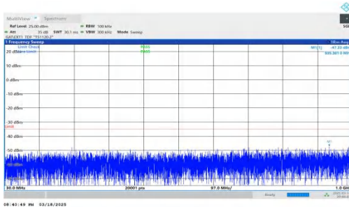
NTNV-DC_2A-n38A-PC3-30-5+40-M+M-QPSK-IDLE-DFT-BPSK-In ner_1RB_Left-30-1000-PASS
