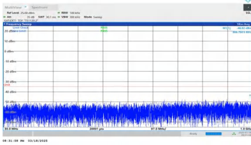
NTNV-DC_2A-n38A-PC3-30-5+30-M+H-QPSK-IDLE-DFT-BPSK-Inner_1RB_Right-30-1000-PASS
