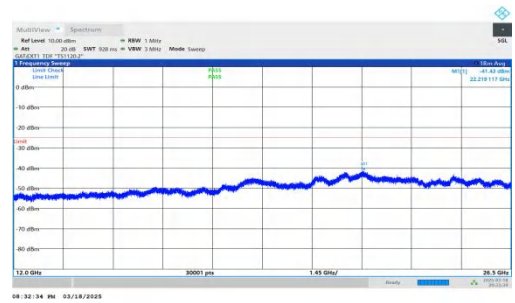
NTNV-DC_2A-n38A-PC3-30-5+30-M+H-QPSK-IDLE-DFT-BPSK-Inner_1RB_Right-12000-26500-PASS
