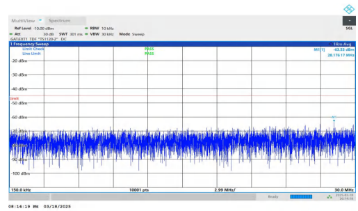
NTNV-DC_2A-n38A-PC3-30-5+20-M+M-QPSK-IDLE-DFT-QPSK-Inner_1RB_Right-0.15-30-PASS
