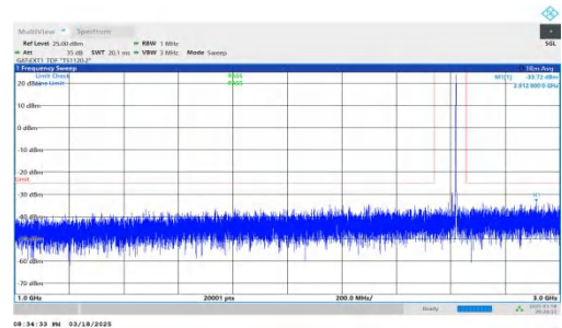
NTNV-DC_2A-n38A-PC3-30-5+30-M+H-QPSK-IDLE-DFT-QPSK-In ner_1RB_Right-1000-3000-PASS
