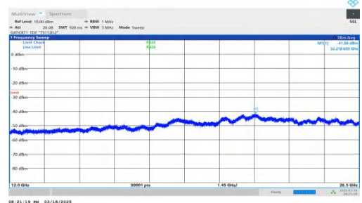
NTNV-DC_2A-n38A-PC3-30-5+30-M+L-QPSK-IDLE-DFT-BPSK-Inner_1RB_Left-12000-26500-PASS
