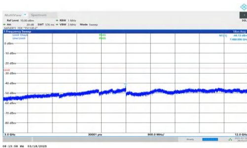
NTNV-DC_2A-n38A-PC3-30-5+20-M+H-QPSK-IDLE-DFT-BPSK-Inner_1RB_Left-3000-12000-PASS
