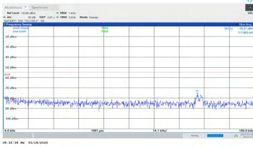
NTNV-DC_2A-n38A-PC3-30-5+40-M+L-QPSK-IDLE-DFT-BPSK-Inner_1RB_Left-0.009-0.15-PASS
