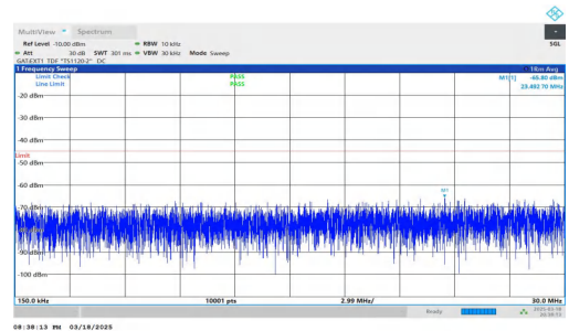
NTNV-DC_2A-n38A-PC3-30-5+40-M+L-QPSK-IDLE-DFT-QPSK-Inner_1RB_Left-0.15-30-PASS
