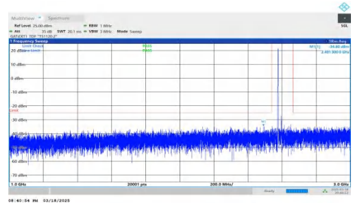
NTNV-DC_2A-n38A-PC3-30-5+40-M+M-QPSK-IDLE-DFT-BPSK-In ner_1RB_Left-1000-3000-PASS
