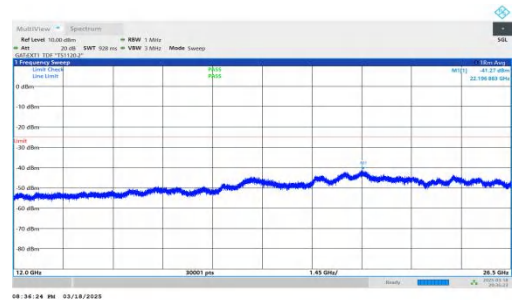
NTNV-DC_2A-n38A-PC3-30-5+40-M+L-QPSK-IDLE-DFT-BPSK-Inner_1RB_Left-12000-26500-PASS
