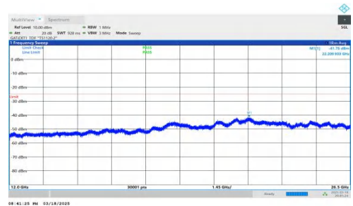
NTNV-DC_2A-n38A-PC3-30-5+40-M+M-QPSK-IDLE-DFT-BPSK-In ner_1RB_Left-12000-26500-PASS
