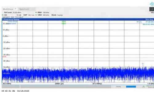
NTNV-DC_2A-n38A-PC3-30-5+40-M+H-QPSK-IDLE-DFT-BPSK-Inner_1RB_Left-30-1000-PASS
