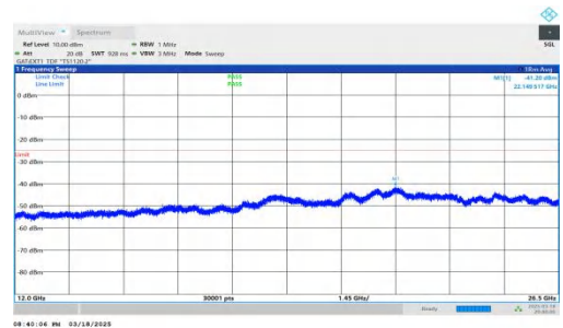
NTNV-DC_2A-n38A-PC3-30-5+40-M+L-QPSK-IDLE-DFT-QPSK-Inner_1RB_Right-12000-26500-PASS
