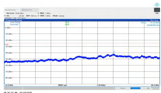
NTNV-DC_2A-n38A-PC3-30-5+30-M+M-QPSK-IDLE-DFT-QPSK-Inner_1RB_Right-12000-26500-PASS
