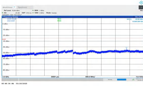
NTNV-DC_2A-n38A-PC3-30-5+40-M+H-QPSK-IDLE-DFT-QPSK-In ner_1RB_Left-3000-12000-PASS
