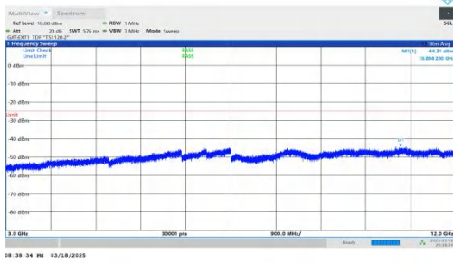
NTNV-DC_2A-n38A-PC3-30-5+40-M+L-QPSK-IDLE-DFT-QPSK-Inner_1RB_Left-3000-12000-PASS
