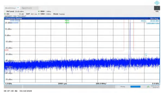
NTNV-DC_2A-n38A-PC3-30-5+40-M+H-QPSK-IDLE-DFT-BPSK-Inner_1RB_Right-1000-3000-PASS
