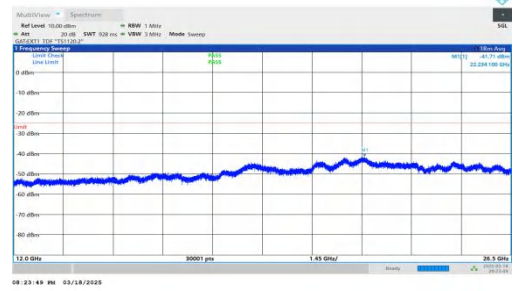
NTNV-DC_2A-n38A-PC3-30-5+30-M+L-QPSK-IDLE-DFT-QPSK-Inner_1RB_Left-12000-26500-PASS
