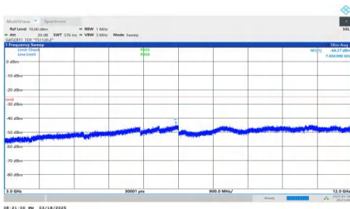
NTNV-DC_2A-n38A-PC3-30-5+30-M+L-QPSK-IDLE-DFT-BPSK-Inner_1RB_Left-3000-12000-PASS
