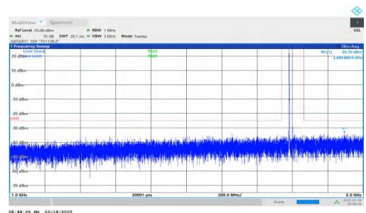
NTNV-DC_2A-n38A-PC3-30-5+40-M+H-QPSK-IDLE-DFT-QPSK-Inner_1RB_Left-1000-3000-PASS
