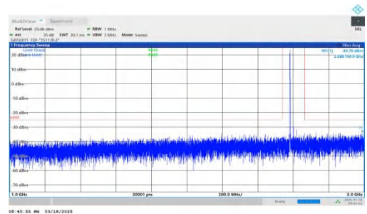
NTNV-DC_2A-n38A-PC3-30-5+40-M+H-QPSK-IDLE-DFT-BPSK-Inner_1RB_Left-1000-3000-PASS
