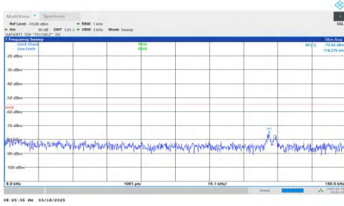
NTNV-DC_2A-n38A-PC3-30-5+30-M+M-QPSK-IDLE-DFT-BPSK-In ner_1RB_Left-0.009-0.15-PASS
