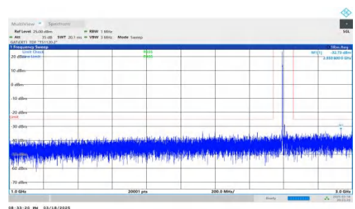
NTNV-DC_2A-n38A-PC3-30-5+30-M+H-QPSK-IDLE-DFT-QPSK-Inner_1RB_Left-1000-3000-PASS
