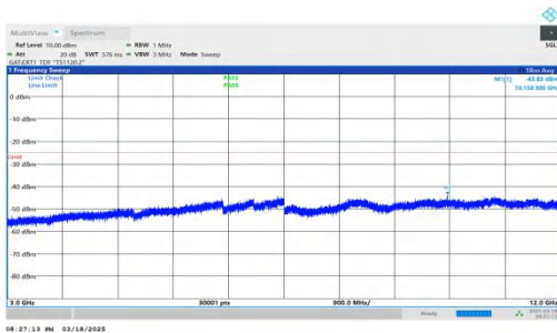
NTNV-DC_2A-n38A-PC3-30-5+30-M+M-QPSK-IDLE-DFT-BPSK-In ner_1RB_Right-3000-12000-PASS
