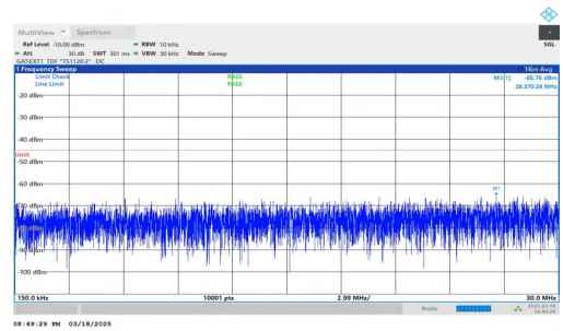
NTNV-DC_2A-n38A-PC3-30-5+40-M+H-QPSK-IDLE-DFT-QPSK-In ner_1RB_Right-0.15-30-PASS
