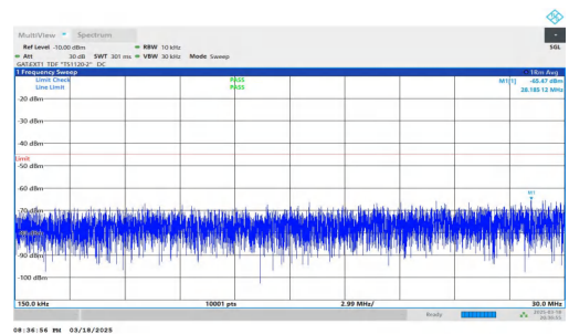
NTNV-DC_2A-n38A-PC3-30-5+40-M+L-QPSK-IDLE-DFT-BPSK-Inner_1RB_Right-0.15-30-PASS
