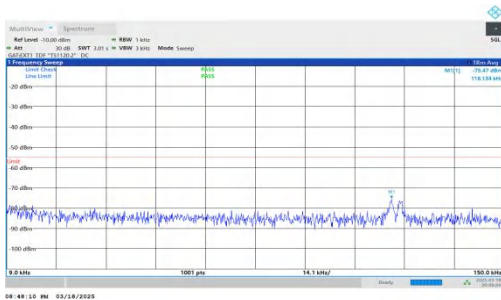
NTNV-DC_2A-n38A-PC3-30-5+40-M+H-QPSK-IDLE-DFT-QPSK-Inner_1RB_Left-0.009-0.15-PASS
