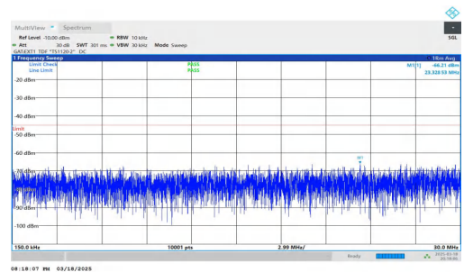
NTNV-DC_2A-n38A-PC3-30-5+20-M+H-QPSK-IDLE-DFT-QPSK-Inner_1RB_Left-0.15-30-PASS
