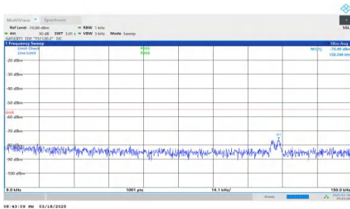
NTNV-DC_2A-n38A-PC3-30-5+40-M+M-QPSK-IDLE-DFT-QPSK-I nner_1RB_Left-0.009-0.15-PASS
