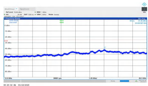
NTNV-DC_2A-n38A-PC3-30-5+30-M+L-QPSK-IDLE-DFT-QPSK-Inner_1RB_Right-12000-26500-PASS
