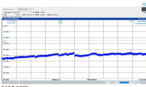
NTNV-DC_2A-n38A-PC3-30-5+20-M+H-QPSK-IDLE-DFT-QPSK-In ner_1RB_Right-3000-12000-PASS
