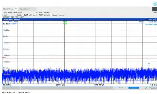
NTNV-DC_2A-n38A-PC3-30-5+20-M+M-QPSK-IDLE-DFT-QPSK-Inner_1RB_Right-30-1000-PASS
