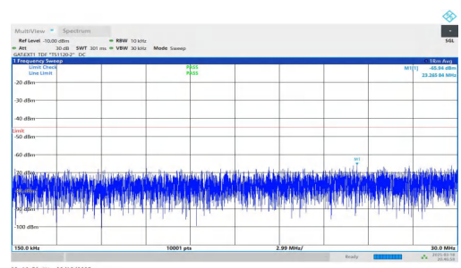
NTNV-DC_2A-n38A-PC3-30-5+40-M+H-QPSK-IDLE-DFT-BPSK-Inner_1RB_Right-0.15-30-PASS
