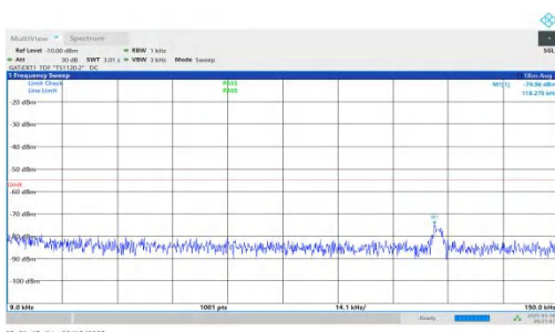
NTNV-DC_2A-n38A-PC3-30-5+30-M+L-QPSK-IDLE-DFT-BPSK-Inner_1RB_Right-0.009-0.15-PASS
