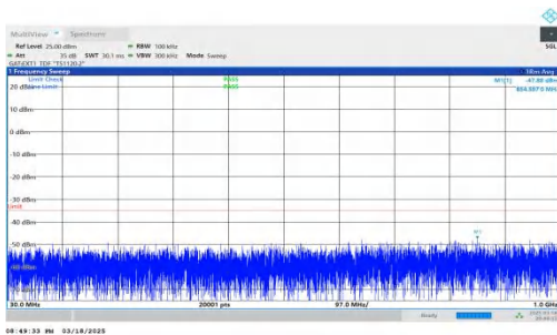
NTNV-DC_2A-n38A-PC3-30-5+40-M+H-QPSK-IDLE-DFT-QPSK-In ner_1RB_Right-30-1000-PASS
