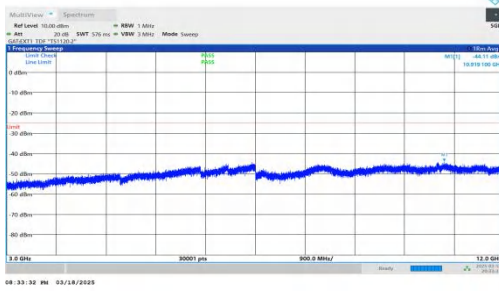
NTNV-DC_2A-n38A-PC3-30-5+30-M+H-QPSK-IDLE-DFT-QPSK-In ner_1RB_Left-3000-12000-PASS
