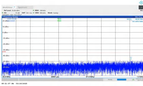
NTNV-DC_2A-n38A-PC3-30-5+30-M+L-QPSK-IDLE-DFT-BPSK-Inner_1RB_Right-30-1000-PASS
