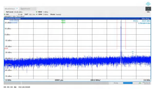
NTNV-DC_2A-n38A-PC3-30-5+30-M+H-QPSK-IDLE-DFT-BPSK-Inner_1RB_Left-1000-3000-PASS
