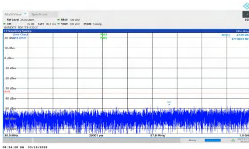
NTNV-DC_2A-n38A-PC3-30-5+30-M+H-QPSK-IDLE-DFT-QPSK-In ner_1RB_Right-30-1000-PASS
