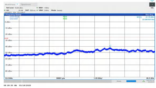
NTNV-DC_2A-n38A-PC3-30-5+30-M+M-QPSK-IDLE-DFT-QPSK-Inner_1RB_Left-12000-26500-PASS
