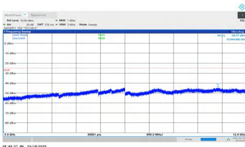
NTNV-DC_2A-n38A-PC3-30-5+40-M+H-QPSK-IDLE-DFT-BPSK-Inner_1RB_Left-3000-12000-PASS
