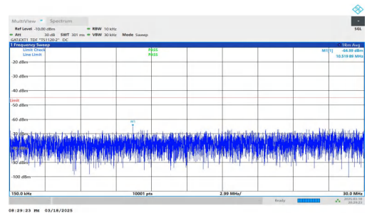
NTNV-DC_2A-n38A-PC3-30-5+30-M+M-QPSK-IDLE-DFT-QPSK-Inner_1RB_Right-0.15-30-PASS
