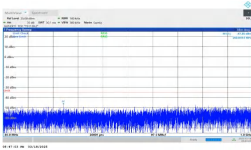
NTNV-DC_2A-n38A-PC3-30-5+40-M+H-QPSK-IDLE-DFT-BPSK-Inner_1RB_Right-30-1000-PASS
