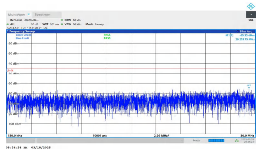
NTNV-DC_2A-n38A-PC3-30-5+30-M+H-QPSK-IDLE-DFT-QPSK-In ner_1RB_Right-0.15-30-PASS
