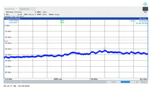
NTNV-DC_2A-n38A-PC3-30-5+20-M+H-QPSK-IDLE-DFT-BPSK-Inner_1RB_Left-12000-26500-PASS
