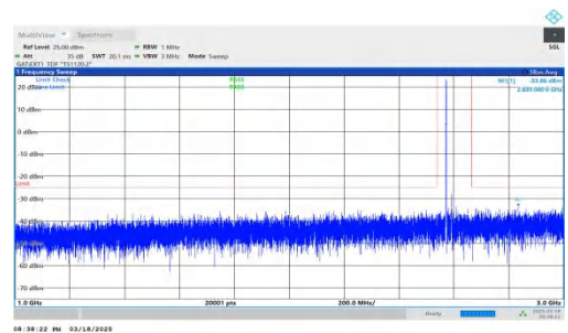
NTNV-DC_2A-n38A-PC3-30-5+40-M+L-QPSK-IDLE-DFT-QPSK-Inner_1RB_Left-1000-3000-PASS
