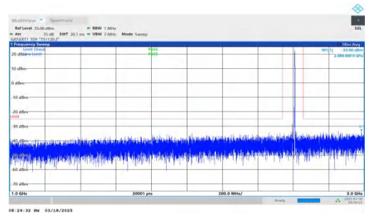
NTNV-DC_2A-n38A-PC3-30-5+30-M+M-QPSK-IDLE-DFT-QPSK-Inner_1RB_Right-1000-3000-PASS
