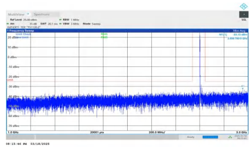
NTNV-DC_2A-n38A-PC3-30-5+20-M+H-QPSK-IDLE-DFT-BPSK-Inner_1RB_Left-1000-3000-PASS
