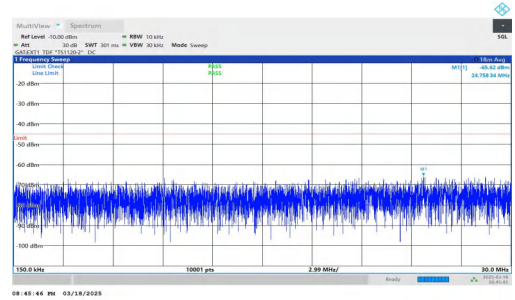
NTNV-DC_2A-n38A-PC3-30-5+40-M+H-QPSK-IDLE-DFT-BPSK-Inner_1RB_Left-0.15-30-PASS
