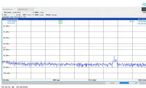
NTNV-DC_2A-n38A-PC3-30-5+40-M+L-QPSK-IDLE-DFT-BPSK-Inner_1RB_Right-0.009-0.15-PASS
