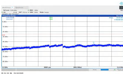
NTNV-DC_2A-n38A-PC3-30-5+30-M+H-QPSK-IDLE-DFT-BPSK-Inner_1RB_Left-3000-12000-PASS
