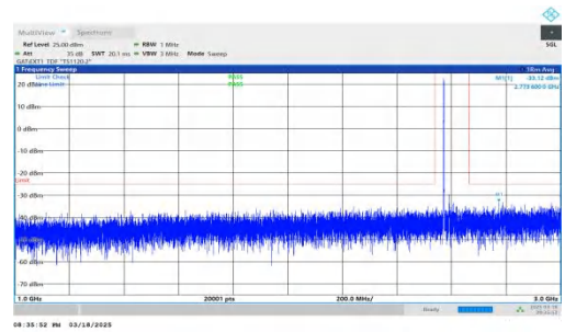
NTNV-DC_2A-n38A-PC3-30-5+40-M+L-QPSK-IDLE-DFT-BPSK-Inner_1RB_Left-1000-3000-PASS
