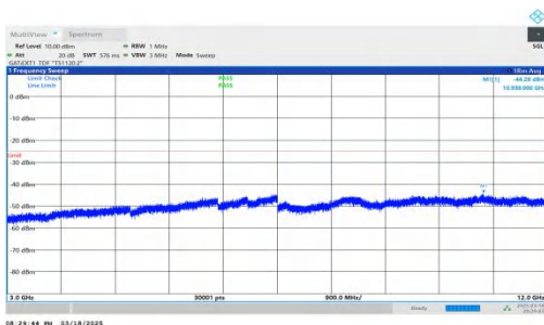
NTNV-DC_2A-n38A-PC3-30-5+30-M+M-QPSK-IDLE-DFT-QPSK-Inner_1RB_Right-3000-12000-PASS
