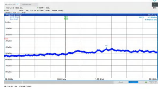
NTNV-DC_2A-n38A-PC3-30-5+30-M+H-QPSK-IDLE-DFT-QPSK-In ner_1RB_Left-12000-26500-PASS
