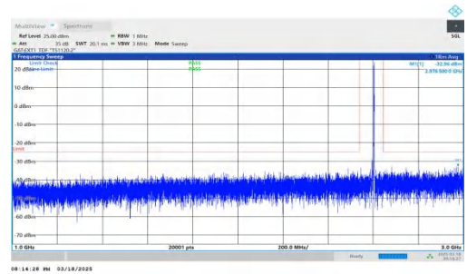
NTNV-DC_2A-n38A-PC3-30-5+20-M+M-QPSK-IDLE-DFT-QPSK-Inner_1RB_Right-1000-3000-PASS
