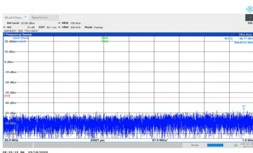
NTNV-DC_2A-n38A-PC3-30-5+30-M+H-QPSK-IDLE-DFT-QPSK-Inner_1RB_Left-30-1000-PASS
