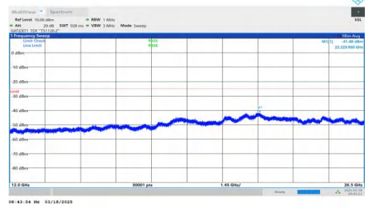
NTNV-DC_2A-n38A-PC3-30-5+40-M+M-QPSK-IDLE-DFT-QPSK-Inner_1RB_Left-12000-26500-PASS
