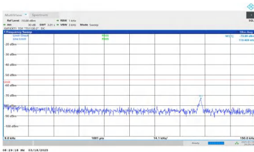
NTNV-DC_2A-n38A-PC3-30-5+30-M+M-QPSK-IDLE-DFT-QPSK-Inner_1RB_Right-0.009-0.15-PASS
