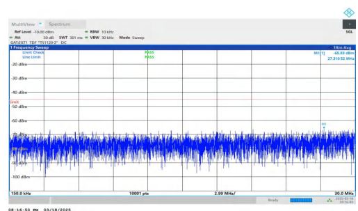
NTNV-DC_2A-n38A-PC3-30-5+20-M+H-QPSK-IDLE-DFT-BPSK-Inner_1RB_Right-0.15-30-PASS
