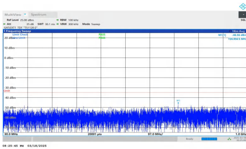
NTNV-DC_2A-n38A-PC3-30-5+30-M+M-QPSK-IDLE-DFT-BPSK-In ner_1RB_Left-30-1000-PASS
