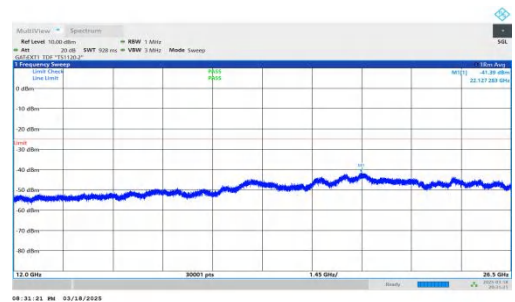
NTNV-DC_2A-n38A-PC3-30-5+30-M+H-QPSK-IDLE-DFT-BPSK-Inner_1RB_Left-12000-26500-PASS
