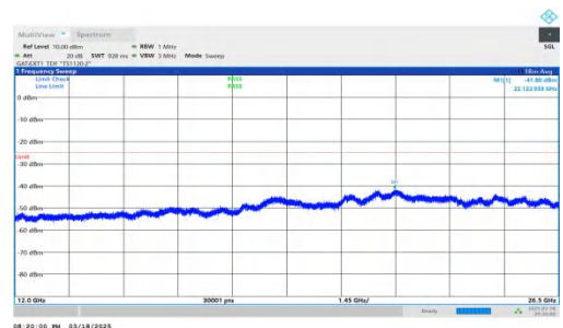
NTNV-DC_2A-n38A-PC3-30-5+20-M+H-QPSK-IDLE-DFT-QPSK-In ner_1RB_Right-12000-26500-PASS
