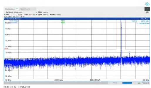
NTNV-DC_2A-n38A-PC3-30-5+40-M+M-QPSK-IDLE-DFT-QPSK-Inner_1RB_Right-1000-3000-PASS
