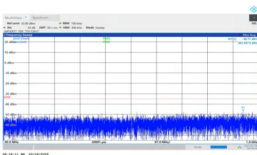
NTNV-DC_2A-n38A-PC3-30-5+20-M+H-QPSK-IDLE-DFT-QPSK-Inner_1RB_Left-30-1000-PASS
