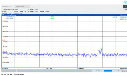
NTNV-DC_2A-n38A-PC3-30-5+30-M+L-QPSK-IDLE-DFT-BPSK-Inner_1RB_Left-0.009-0.15-PASS
