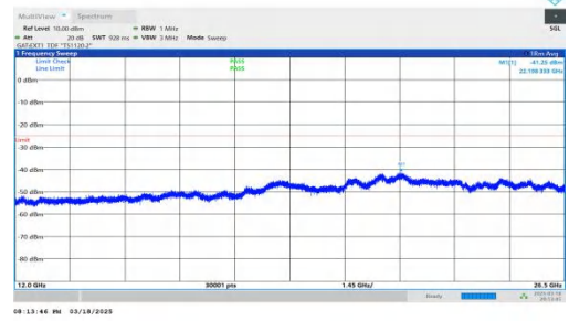
NTNV-DC_2A-n38A-PC3-30-5+20-M+M-QPSK-IDLE-DFT-QPSK-Inner_1RB_Left-12000-26500-PASS
