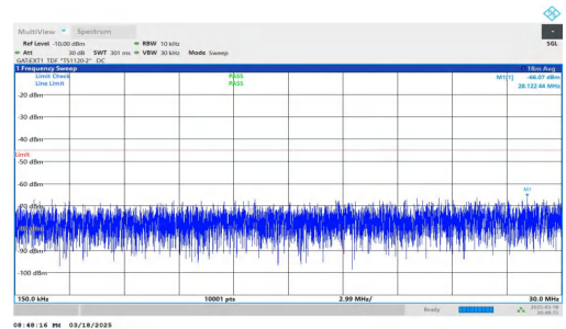
NTNV-DC_2A-n38A-PC3-30-5+40-M+H-QPSK-IDLE-DFT-QPSK-Inner_1RB_Left-0.15-30-PASS
