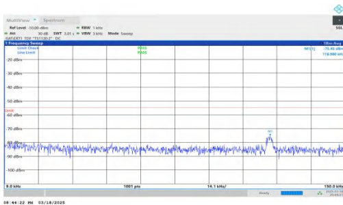
NTNV-DC_2A-n38A-PC3-30-5+40-M+M-QPSK-IDLE-DFT-QPSK-Inner_1RB_Right-0.009-0.15-PASS
