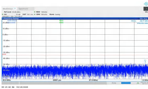
NTNV-DC_2A-n38A-PC3-30-5+20-M+H-QPSK-IDLE-DFT-BPSK-Inner_1RB_Left-30-1000-PASS
