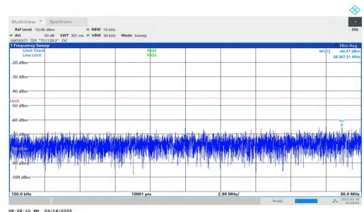
NTNV-DC_2A-n38A-PC3-30-5+30-M+M-QPSK-IDLE-DFT-QPSK-In ner_1RB_Left-0.15-30-PASS
