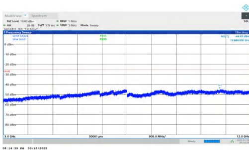
NTNV-DC_2A-n38A-PC3-30-5+20-M+M-QPSK-IDLE-DFT-QPSK-Inner_1RB_Right-3000-12000-PASS
