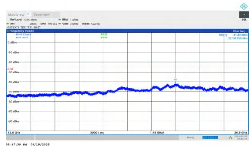
NTNV-DC_2A-n38A-PC3-30-5+40-M+H-QPSK-IDLE-DFT-BPSK-Inner_1RB_Right-12000-26500-PASS
