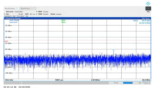
NTNV-DC_2A-n38A-PC3-30-5+40-M+M-QPSK-IDLE-DFT-QPSK-In ner_1RB_Left-0.15-30-PASS
