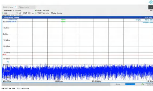
NTNV-DC_2A-n38A-PC3-30-5+20-M+H-QPSK-IDLE-DFT-BPSK-Inner_1RB_Right-30-1000-PASS
