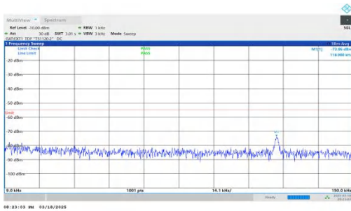
NTNV-DC_2A-n38A-PC3-30-5+30-M+L-QPSK-IDLE-DFT-QPSK-Inner_1RB_Left-0.009-0.15-PASS
