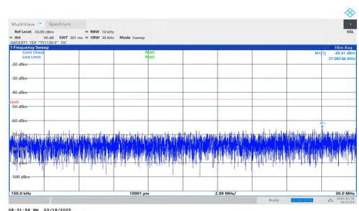
NTNV-DC_2A-n38A-PC3-30-5+30-M+H-QPSK-IDLE-DFT-BPSK-Inner_1RB_Right-0.15-30-PASS
