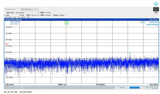
NTNV-DC_2A-n38A-PC3-30-5+40-M+L-QPSK-IDLE-DFT-QPSK-Inner_1RB_Right-0.15-30-PASS
