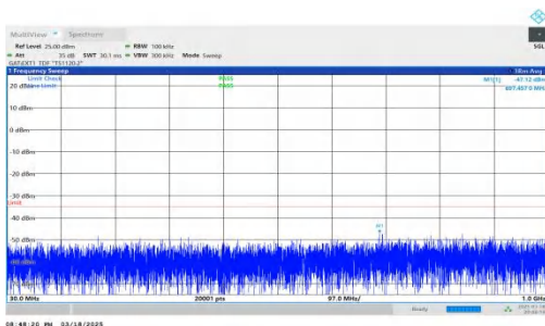
NTNV-DC_2A-n38A-PC3-30-5+40-M+H-QPSK-IDLE-DFT-QPSK-Inner_1RB_Left-30-1000-PASS
