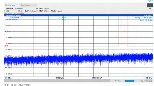
NTNV-DC_2A-n38A-PC3-30-5+30-M+L-QPSK-IDLE-DFT-BPSK-Inner_1RB_Left-1000-3000-PASS
