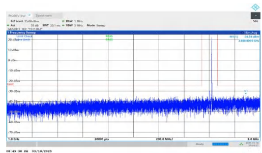
NTNV-DC_2A-n38A-PC3-30-5+40-M+H-QPSK-IDLE-DFT-QPSK-In ner_1RB_Right-1000-3000-PASS
