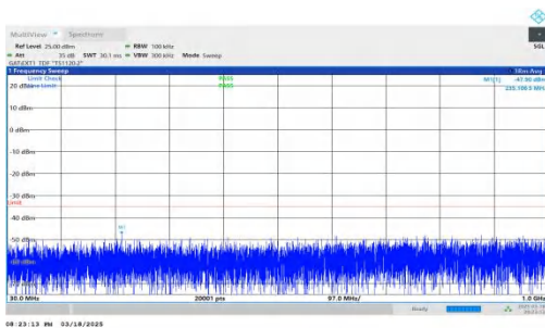
NTNV-DC_2A-n38A-PC3-30-5+30-M+L-QPSK-IDLE-DFT-QPSK-Inner_1RB_Left-30-1000-PASS
