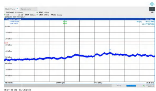
NTNV-DC_2A-n38A-PC3-30-5+30-M+M-QPSK-IDLE-DFT-BPSK-In ner_1RB_Right-12000-26500-PASS
