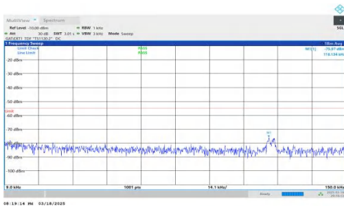
NTNV-DC_2A-n38A-PC3-30-5+20-M+H-QPSK-IDLE-DFT-QPSK-In ner_1RB_Right-0.009-0.15-PASS
