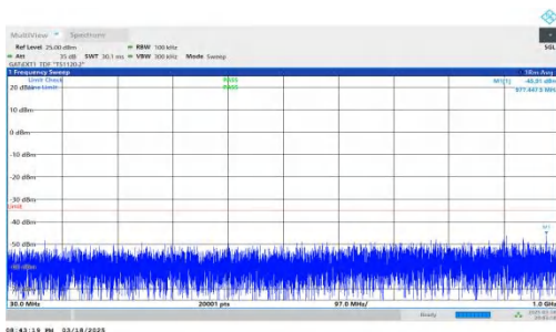
NTNV-DC_2A-n38A-PC3-30-5+40-M+M-QPSK-IDLE-DFT-QPSK-I nner_1RB_Left-30-1000-PASS
