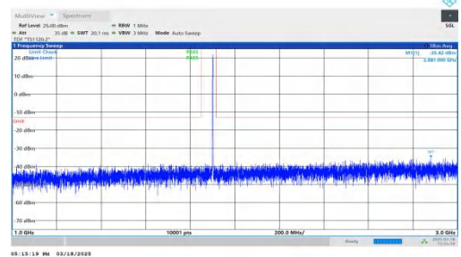
NTNV-DC_7A-n25A-PC3-15-5+15-M+H-QPSK-IDLE-DFT-BPSK-Inner_1RB_Left-1000-3000-PASS
