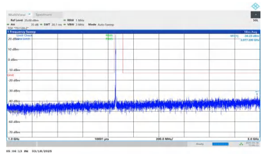
NTNV-DC_7A-n25A-PC3-15-5+10-M+L-QPSK-IDLE-DFT-QPSK-Inner_1RB_Right-1000-3000-PASS
