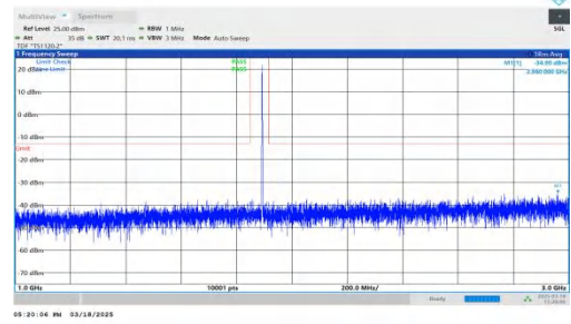
NTNV-DC_7A-n25A-PC3-15-5+20-M+M-QPSK-IDLE-DFT-BPSK-In ner_1RB_Right-1000-3000-PASS
