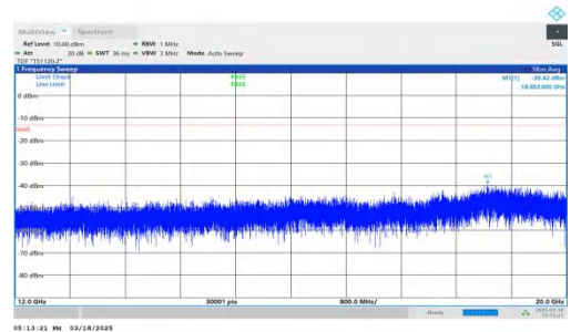
NTNV-DC_7A-n25A-PC3-15-5+15-M+M-QPSK-IDLE-DFT-BPSK-In ner_1RB_Left-12000-20000-PASS
