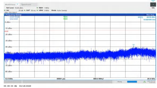
NTNV-DC_7A-n25A-PC3-15-5+10-M+M-QPSK-IDLE-DFT-QPSK-Inner_1RB_Left-12000-20000-PASS
