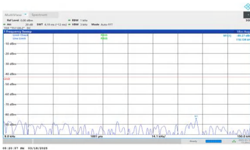
NTNV-DC_7A-n25A-PC3-15-5+20-M+M-QPSK-IDLE-DFT-QPSK-Inner_1RB_Right-0.009-0.15-PASS
