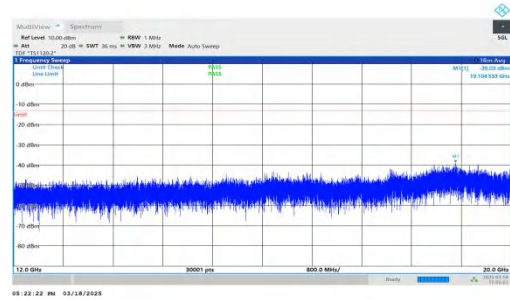
NTNV-DC_7A-n25A-PC3-15-5+20-M+H-QPSK-IDLE-DFT-BPSK-Inner_1RB_Right-12000-20000-PASS
