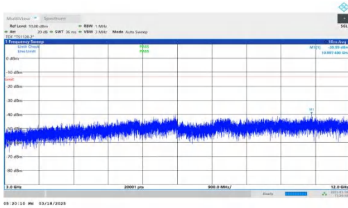
NTNV-DC_7A-n25A-PC3-15-5+20-M+M-QPSK-IDLE-DFT-BPSK-In ner_1RB_Right-3000-12000-PASS
