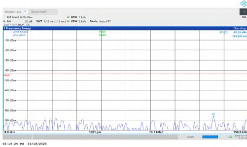
NTNV-DC_7A-n25A-PC3-15-5+20-M+M-QPSK-IDLE-DFT-BPSK-In ner_1RB_Left-0.009-0.15-PASS
