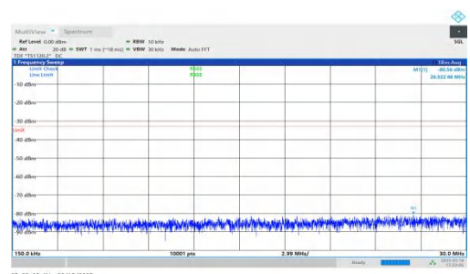
NTNV-DC_7A-n25A-PC3-15-5+20-M+H-QPSK-IDLE-DFT-BPSK-Inner_1RB_Right-0.15-30-PASS
