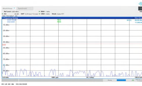
NTNV-DC_7A-n25A-PC3-15-5+20-M+L-QPSK-IDLE-DFT-QPSK-Inner_1RB_Right-0.009-0.15-PASS
