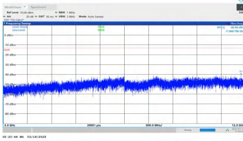
NTNV-DC_7A-n25A-PC3-15-5+20-M+M-QPSK-IDLE-DFT-QPSK-Inner_1RB_Left-3000-12000-PASS
