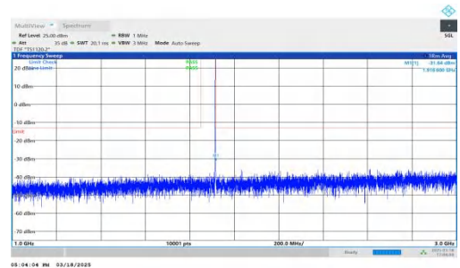
NTNV-DC_7A-n25A-PC3-15-5+5-M+H-QPSK-IDLE-DFT-QPSK-Inner_1RB_Right-1000-3000-PASS
