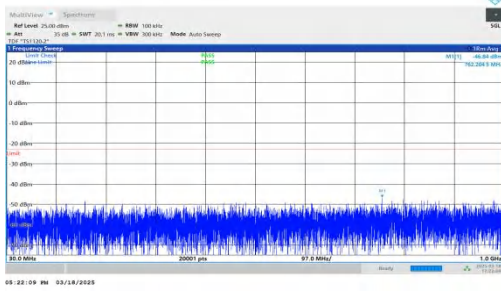
NTNV-DC_7A-n25A-PC3-15-5+20-M+H-QPSK-IDLE-DFT-BPSK-Inner_1RB_Right-30-1000-PASS
