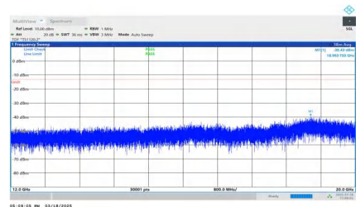
NTNV-DC_7A-n25A-PC3-15-5+10-M+H-QPSK-IDLE-DFT-BPSK-Inner_1RB_Left-12000-20000-PASS
