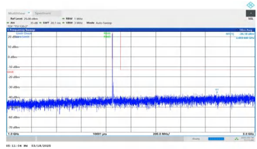
NTNV-DC_7A-n25A-PC3-15-5+15-M+L-QPSK-IDLE-DFT-BPSK-Inner_1RB_Left-1000-3000-PASS
