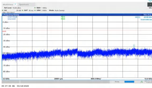
NTNV-DC_7A-n25A-PC3-15-5+10-M+M-QPSK-IDLE-DFT-QPSK-Inner_1RB_Left-3000-12000-PASS
