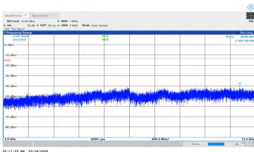
NTNV-DC_7A-n25A-PC3-15-5+20-M+L-QPSK-IDLE-DFT-BPSK-Inner_1RB_Left-3000-12000-PASS
