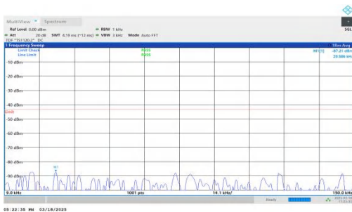
NTNV-DC_7A-n25A-PC3-15-5+20-M+H-QPSK-IDLE-DFT-QPSK-Inner_1RB_Left-0.009-0.15-PASS
