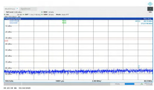
NTNV-DC_7A-n25A-PC3-15-5+20-M+H-QPSK-IDLE-DFT-QPSK-In ner_1RB_Right-0.15-30-PASS
