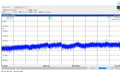
NTNV-DC_7A-n25A-PC3-15-5+10-M+L-QPSK-IDLE-DFT-BPSK-Inner_1RB_Left-3000-12000-PASS
