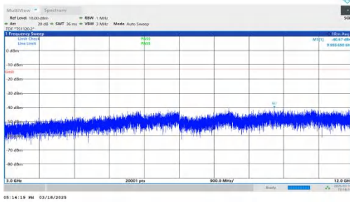
NTNV-DC_7A-n25A-PC3-15-5+15-M+M-QPSK-IDLE-DFT-QPSK-Inner_1RB_Left-3000-12000-PASS
