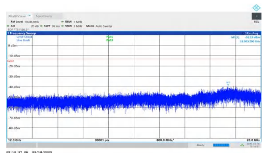
NTNV-DC_7A-n25A-PC3-15-5+10-M+H-QPSK-IDLE-DFT-QPSK-In ner_1RB_Right-12000-20000-PASS
