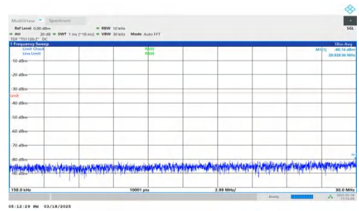
NTNV-DC_7A-n25A-PC3-15-5+15-M+L-QPSK-IDLE-DFT-QPSK-Inner_1RB_Right-0.15-30-PASS
