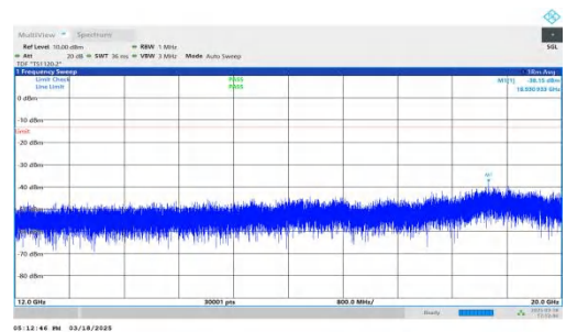
NTNV-DC_7A-n25A-PC3-15-5+15-M+L-QPSK-IDLE-DFT-QPSK-Inner_1RB_Right-12000-20000-PASS
