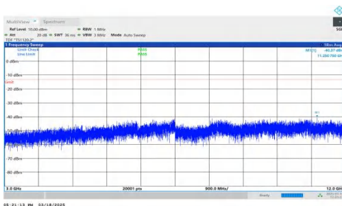
NTNV-DC_7A-n25A-PC3-15-5+20-M+M-QPSK-IDLE-DFT-QPSK-Inner_1RB_Right-3000-12000-PASS
