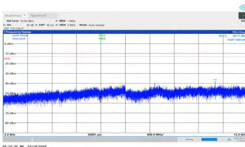
NTNV-DC_7A-n25A-PC3-15-5+10-M+H-QPSK-IDLE-DFT-QPSK-In ner_1RB_Right-3000-12000-PASS
