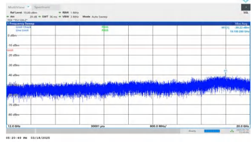
NTNV-DC_7A-n25A-PC3-15-5+20-M+M-QPSK-IDLE-DFT-QPSK-Inner_1RB_Left-12000-20000-PASS
