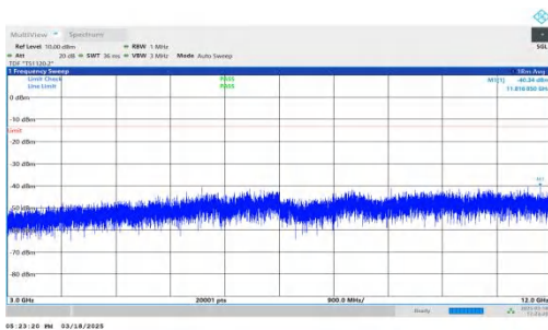
NTNV-DC_7A-n25A-PC3-15-5+20-M+H-QPSK-IDLE-DFT-QPSK-In ner_1RB_Right-3000-12000-PASS
