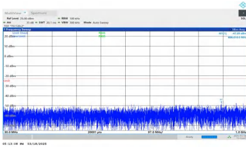
NTNV-DC_7A-n25A-PC3-15-5+15-M+M-QPSK-IDLE-DFT-BPSK-In ner_1RB_Left-30-1000-PASS
