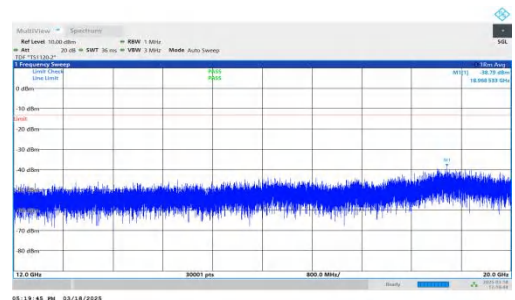
NTNV-DC_7A-n25A-PC3-15-5+20-M+M-QPSK-IDLE-DFT-BPSK-In ner_1RB_Left-12000-20000-PASS
