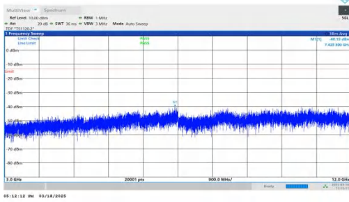
NTNV-DC_7A-n25A-PC3-15-5+15-M+L-QPSK-IDLE-DFT-QPSK-Inner_1RB_Left-3000-12000-PASS
