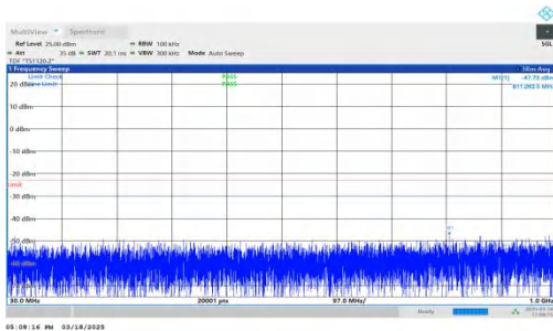
NTNV-DC_7A-n25A-PC3-15-5+10-M+M-QPSK-IDLE-DFT-QPSK-Inner_1RB_Right-30-1000-PASS
