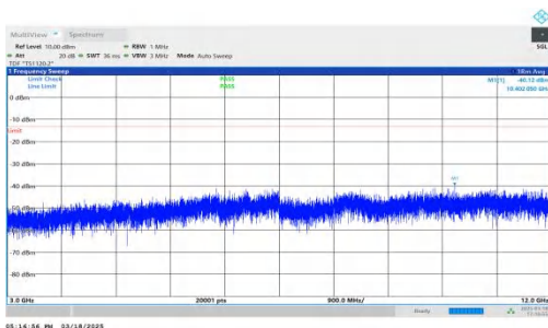
NTNV-DC_7A-n25A-PC3-15-5+15-M+H-QPSK-IDLE-DFT-QPSK-In ner_1RB_Right-3000-12000-PASS
