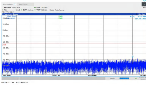
NTNV-DC_7A-n25A-PC3-15-5+10-M+H-QPSK-IDLE-DFT-BPSK-Inner_1RB_Right-30-1000-PASS
