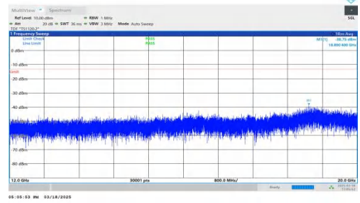
NTNV-DC_7A-n25A-PC3-15-5+10-M+L-QPSK-IDLE-DFT-QPSK-Inner_1RB_Left-12000-20000-PASS
