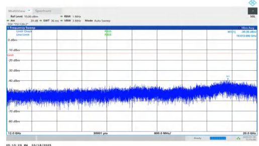
NTNV-DC_7A-n25A-PC3-15-5+15-M+H-QPSK-IDLE-DFT-BPSK-Inner_1RB_Left-12000-20000-PASS
