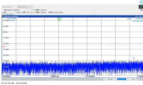
NTNV-DC_7A-n25A-PC3-15-5+10-M+L-QPSK-IDLE-DFT-BPSK-Inner_1RB_Right-30-1000-PASS
