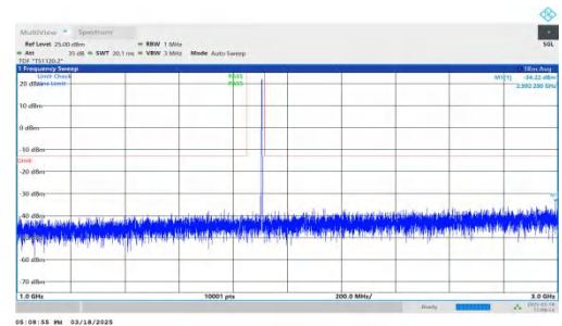
NTNV-DC_7A-n25A-PC3-15-5+10-M+H-QPSK-IDLE-DFT-BPSK-Inner_1RB_Left-1000-3000-PASS
