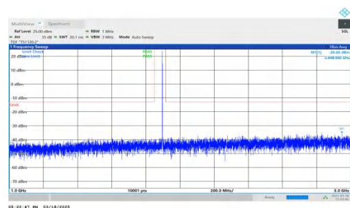
NTNV-DC_7A-n25A-PC3-15-5+20-M+H-QPSK-IDLE-DFT-QPSK-Inner_1RB_Left-1000-3000-PASS
