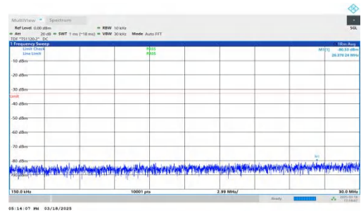
NTNV-DC_7A-n25A-PC3-15-5+15-M+M-QPSK-IDLE-DFT-QPSK-In ner_1RB_Left-0.15-30-PASS
