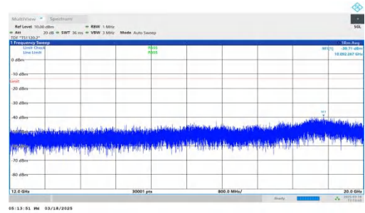
NTNV-DC_7A-n25A-PC3-15-5+15-M+M-QPSK-IDLE-DFT-BPSK-In ner_1RB_Right-12000-20000-PASS
