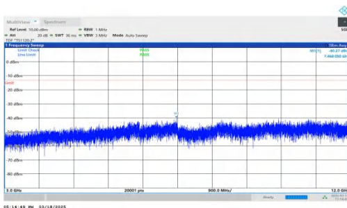
NTNV-DC_7A-n25A-PC3-15-5+15-M+M-QPSK-IDLE-DFT-QPSK-Inner_1RB_Right-3000-12000-PASS
