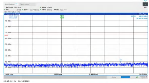
NTNV-DC_7A-n25A-PC3-15-5+15-M+H-QPSK-IDLE-DFT-BPSK-Inner_1RB_Left-0.15-30-PASS
