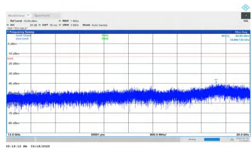
NTNV-DC_7A-n25A-PC3-15-5+20-M+L-QPSK-IDLE-DFT-QPSK-Inner_1RB_Right-12000-20000-PASS
