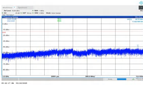
NTNV-DC_7A-n25A-PC3-15-5+20-M+H-QPSK-IDLE-DFT-BPSK-Inner_1RB_Right-3000-12000-PASS
