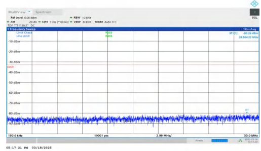
NTNV-DC_7A-n25A-PC3-15-5+20-M+L-QPSK-IDLE-DFT-BPSK-Inner_1RB_Left-0.15-30-PASS
