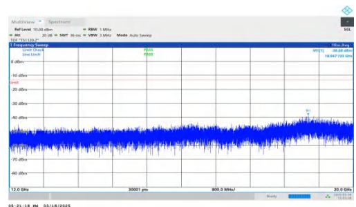
NTNV-DC_7A-n25A-PC3-15-5+20-M+M-QPSK-IDLE-DFT-QPSK-Inner_1RB_Right-12000-20000-PASS
