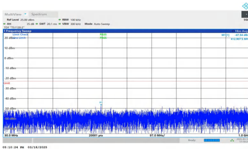
NTNV-DC_7A-n25A-PC3-15-5+10-M+H-QPSK-IDLE-DFT-QPSK-In ner_1RB_Right-30-1000-PASS
