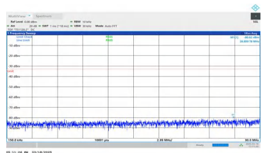
NTNV-DC_7A-n25A-PC3-15-5+15-M+L-QPSK-IDLE-DFT-BPSK-Inner_1RB_Right-0.15-30-PASS
