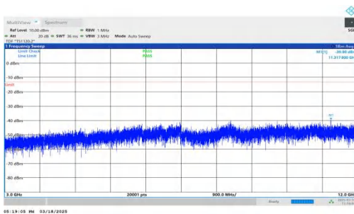
NTNV-DC_7A-n25A-PC3-15-5+20-M+L-QPSK-IDLE-DFT-QPSK-Inner_1RB_Right-3000-12000-PASS
