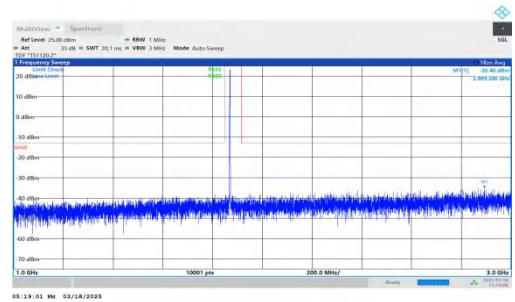
NTNV-DC_7A-n25A-PC3-15-5+20-M+L-QPSK-IDLE-DFT-QPSK-Inner_1RB_Right-1000-3000-PASS
