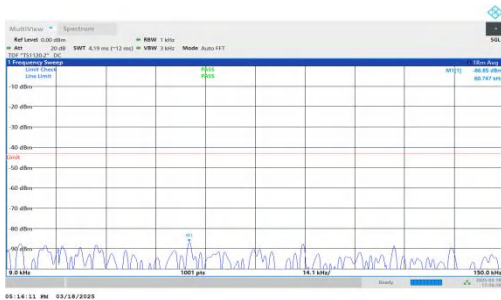
NTNV-DC_7A-n25A-PC3-15-5+15-M+H-QPSK-IDLE-DFT-QPSK-Inner_1RB_Left-0.009-0.15-PASS
