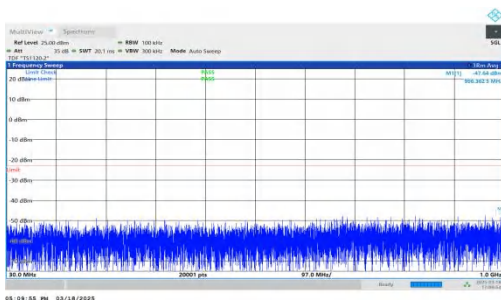
NTNV-DC_7A-n25A-PC3-15-5+10-M+H-QPSK-IDLE-DFT-QPSK-Inner_1RB_Left-30-1000-PASS
