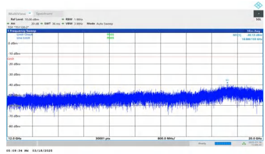
NTNV-DC_7A-n25A-PC3-15-5+10-M+H-QPSK-IDLE-DFT-BPSK-Inner_1RB_Right-12000-20000-PASS
