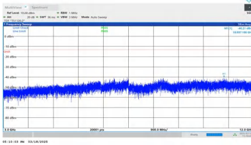
NTNV-DC_7A-n25A-PC3-15-5+10-M+H-QPSK-IDLE-DFT-QPSK-In ner_1RB_Left-3000-12000-PASS
