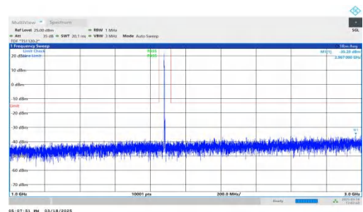
NTNV-DC_7A-n25A-PC3-15-5+10-M+M-QPSK-IDLE-DFT-QPSK-In ner_1RB_Left-1000-3000-PASS
