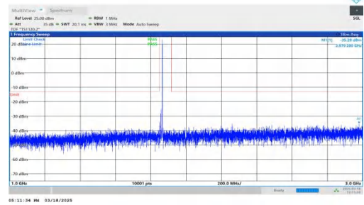
NTNV-DC_7A-n25A-PC3-15-5+15-M+L-QPSK-IDLE-DFT-BPSK-Inner_1RB_Right-1000-3000-PASS
