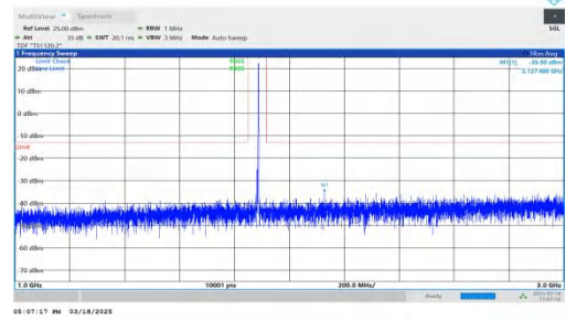
NTNV-DC_7A-n25A-PC3-15-5+10-M+M-QPSK-IDLE-DFT-BPSK-In ner_1RB_Right-1000-3000-PASS
