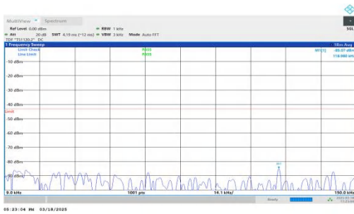
NTNV-DC_7A-n25A-PC3-15-5+20-M+H-QPSK-IDLE-DFT-QPSK-In ner_1RB_Right-0.009-0.15-PASS
