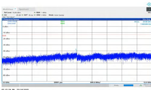
NTNV-DC_7A-n25A-PC3-15-5+15-M+H-QPSK-IDLE-DFT-BPSK-Inner_1RB_Left-3000-12000-PASS
