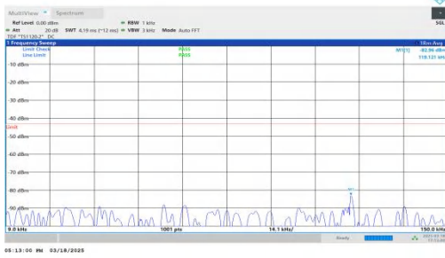
NTNV-DC_7A-n25A-PC3-15-5+15-M+M-QPSK-IDLE-DFT-BPSK-In ner_1RB_Left-0.009-0.15-PASS
