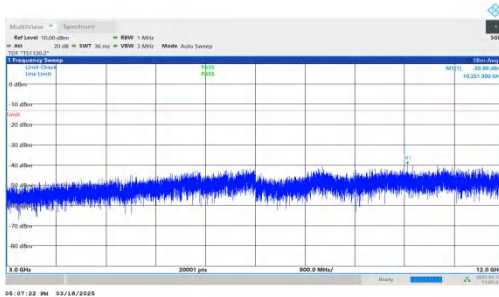
NTNV-DC_7A-n25A-PC3-15-5+10-M+M-QPSK-IDLE-DFT-BPSK-In ner_1RB_Right-3000-12000-PASS
