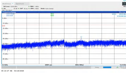
NTNV-DC_7A-n25A-PC3-15-5+15-M+H-QPSK-IDLE-DFT-QPSK-In ner_1RB_Left-3000-12000-PASS
