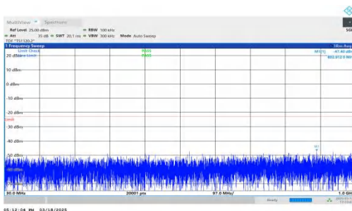
NTNV-DC_7A-n25A-PC3-15-5+15-M+L-QPSK-IDLE-DFT-QPSK-Inner_1RB_Left-30-1000-PASS
