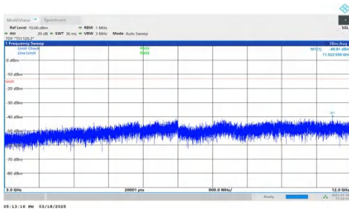
NTNV-DC_7A-n25A-PC3-15-5+15-M+M-QPSK-IDLE-DFT-BPSK-In ner_1RB_Left-3000-12000-PASS
