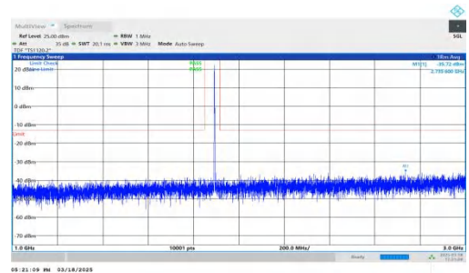
NTNV-DC_7A-n25A-PC3-15-5+20-M+M-QPSK-IDLE-DFT-QPSK-Inner_1RB_Right-1000-3000-PASS
