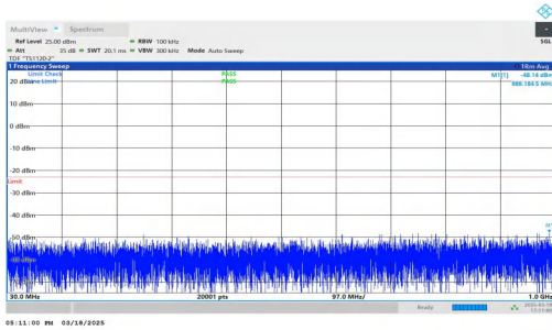
NTNV-DC_7A-n25A-PC3-15-5+15-M+L-QPSK-IDLE-DFT-BPSK-Inner_1RB_Left-30-1000-PASS
