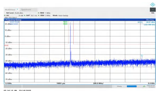
NTNV-DC_7A-n25A-PC3-15-5+15-M+M-QPSK-IDLE-DFT-QPSK-In ner_1RB_Left-1000-3000-PASS
