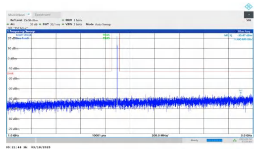
NTNV-DC_7A-n25A-PC3-15-5+20-M+H-QPSK-IDLE-DFT-BPSK-Inner_1RB_Left-1000-3000-PASS
