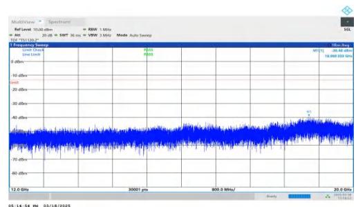
NTNV-DC_7A-n25A-PC3-15-5+15-M+M-QPSK-IDLE-DFT-QPSK-Inner_1RB_Right-12000-20000-PASS
