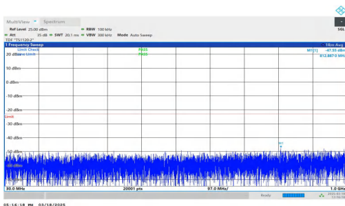
NTNV-DC_7A-n25A-PC3-15-5+15-M+H-QPSK-IDLE-DFT-QPSK-Inner_1RB_Left-30-1000-PASS
