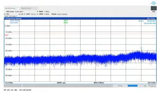
NTNV-DC_7A-n25A-PC3-15-5+20-M+M-QPSK-IDLE-DFT-BPSK-In ner_1RB_Right-12000-20000-PASS
