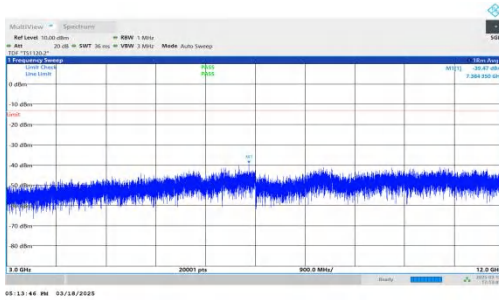
NTNV-DC_7A-n25A-PC3-15-5+15-M+M-QPSK-IDLE-DFT-BPSK-In ner_1RB_Right-3000-12000-PASS
