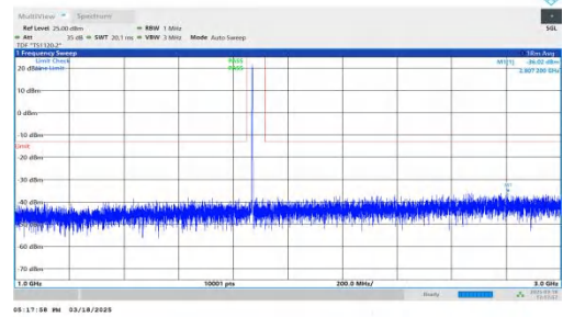
NTNV-DC_7A-n25A-PC3-15-5+20-M+L-QPSK-IDLE-DFT-BPSK-Inner_1RB_Right-1000-3000-PASS
