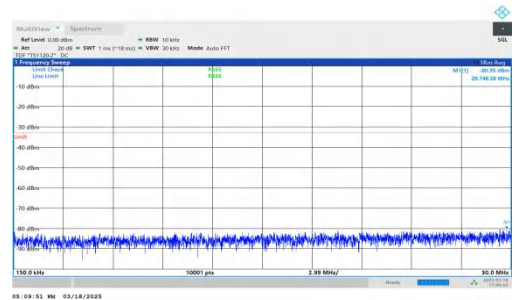
NTNV-DC_7A-n25A-PC3-15-5+10-M+H-QPSK-IDLE-DFT-QPSK-Inner_1RB_Left-0.15-30-PASS
