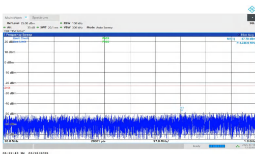
NTNV-DC_7A-n25A-PC3-15-5+20-M+H-QPSK-IDLE-DFT-QPSK-Inner_1RB_Left-30-1000-PASS
