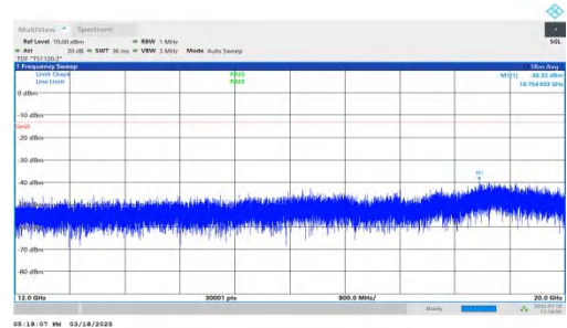
NTNV-DC_7A-n25A-PC3-15-5+20-M+L-QPSK-IDLE-DFT-BPSK-Inner_1RB_Right-12000-20000-PASS
