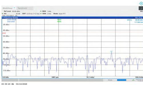
NTNV-DC_7A-n2A-PC3-15-5+5-M+H-QPSK-IDLE-DFT-QPSK-Inner r_1RB_Left-0.009-0.15-PASS
