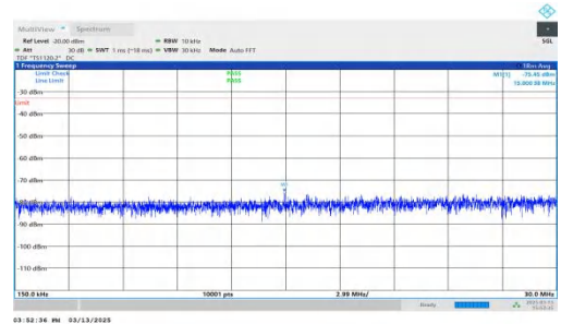
NTNV-DC_7A-n2A-PC3-15-5+15-M+H-QPSK-IDLE-DFT-QPSK-Inner_1RB_Right-0.15-30-PASS
