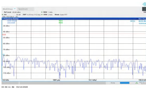
NTNV-DC_7A-n2A-PC3-15-5+20-M+L-QPSK-IDLE-DFT-QPSK-Inner_1RB_Left-0.009-0.15-PASS
