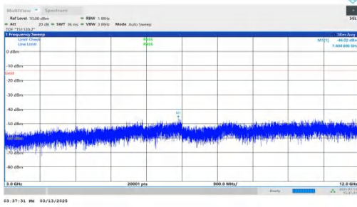
NTNV-DC_7A-n2A-PC3-15-5+5-M+M-QPSK-IDLE-DFT-QPSK-Inner_1RB_Left-3000-12000-PASS
