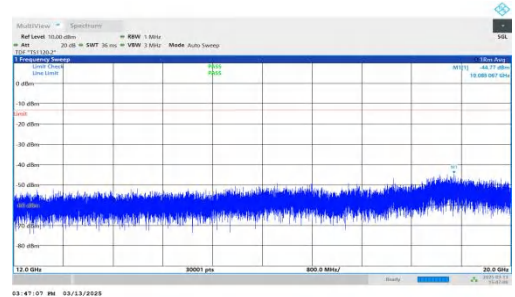
NTNV-DC_7A-n2A-PC3-15-5+15-M+L-QPSK-IDLE-DFT-BPSK-Inner_1RB_Left-12000-20000-PASS
