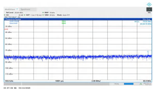
NTNV-DC_7A-n2A-PC3-15-5+20-M+H-QPSK-IDLE-DFT-BPSK-Inner_1RB_Right-0.15-30-PASS
