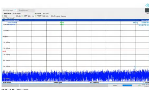
NTNV-DC_7A-n2A-PC3-15-5+20-M+L-QPSK-IDLE-DFT-QPSK-Inner_1RB_Left-30-1000-PASS
