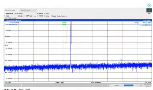
NTNV-DC_7A-n2A-PC3-15-5+10-M+H-QPSK-IDLE-DFT-QPSK-Inner_1RB_Left-1000-3000-PASS
