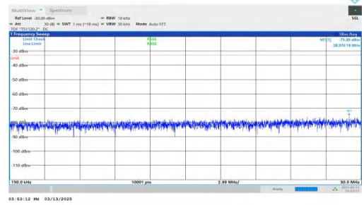
NTNV-DC_7A-n2A-PC3-15-5+20-M+L-QPSK-IDLE-DFT-BPSK-Inner_1RB_Left-0.15-30-PASS
