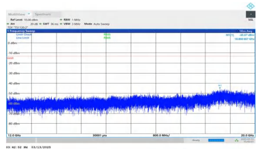
NTNV-DC_7A-n2A-PC3-15-5+10-M+M-QPSK-IDLE-DFT-BPSK-Inner_1RB_Left-12000-20000-PASS
