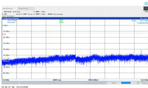
NTNV-DC_7A-n2A-PC3-15-5+10-M+M-QPSK-IDLE-DFT-BPSK-Inner_1RB_Left-3000-12000-PASS
