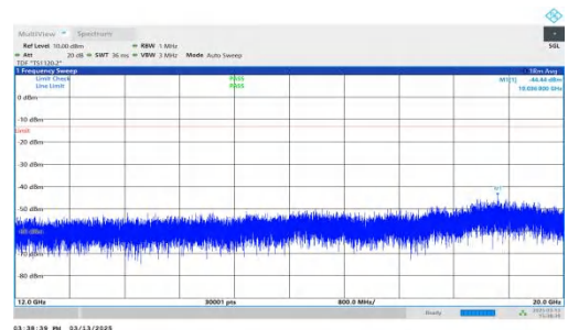
NTNV-DC_7A-n2A-PC3-15-5+5-M+H-QPSK-IDLE-DFT-BPSK-Inner _1RB_Left-12000-20000-PASS
