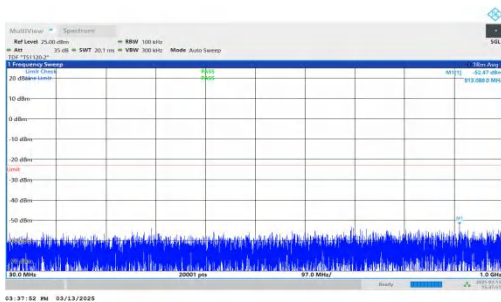
NTNV-DC_7A-n2A-PC3-15-5+5-M+M-QPSK-IDLE-DFT-QPSK-Inner_1RB_Right-30-1000-PASS
