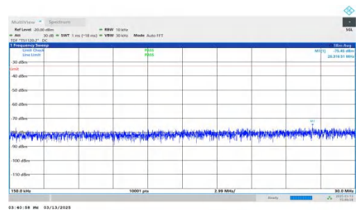
NTNV-DC_7A-n2A-PC3-15-5+10-M+L-QPSK-IDLE-DFT-BPSK-Inner_1RB_Right-0.15-30-PASS
