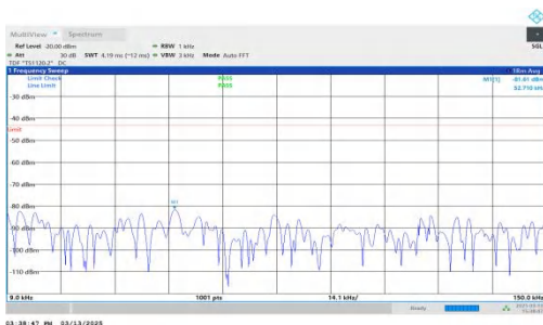
NTNV-DC_7A-n2A-PC3-15-5+5-M+H-QPSK-IDLE-DFT-BPSK-Inner r_1RB_Right-0.009-0.15-PASS
