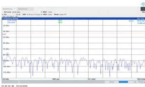
NTNV-DC_7A-n2A-PC3-15-5+10-M+H-QPSK-IDLE-DFT-QPSK-Inner_1RB_Left-0.009-0.15-PASS
