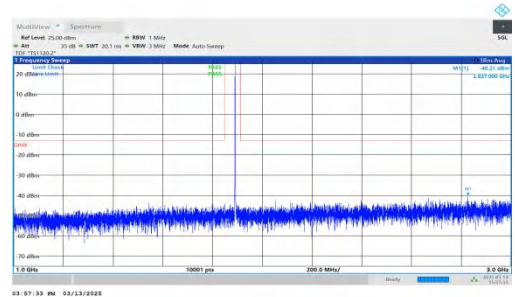
NTNV-DC_7A-n2A-PC3-15-5+20-M+H-QPSK-IDLE-DFT-BPSK-Inner_1RB_Left-1000-3000-PASS
