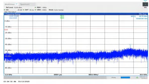
NTNV-DC_7A-n2A-PC3-15-5+20-M+L-QPSK-IDLE-DFT-QPSK-Inner_1RB_Left-12000-20000-PASS
