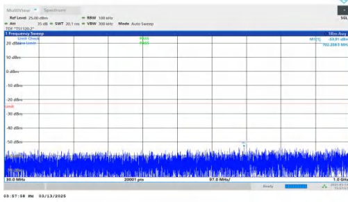
NTNV-DC_7A-n2A-PC3-15-5+20-M+H-QPSK-IDLE-DFT-BPSK-Inner_1RB_Right-30-1000-PASS
