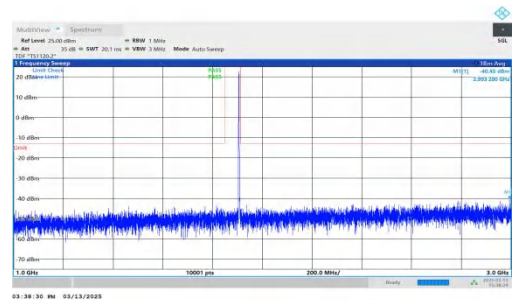
NTNV-DC_7A-n2A-PC3-15-5+5-M+H-QPSK-IDLE-DFT-BPSK-Inner _1RB_Left-1000-3000-PASS
