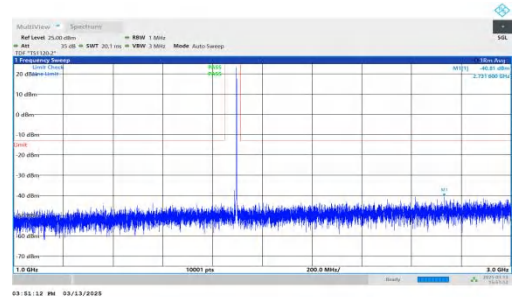
NTNV-DC_7A-n2A-PC3-15-5+15-M+H-QPSK-IDLE-DFT-BPSK-Inner_1RB_Left-1000-3000-PASS
