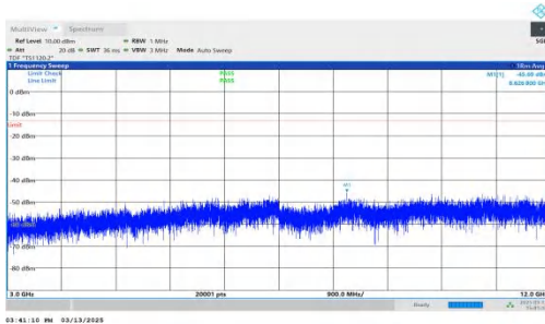
NTNV-DC_7A-n2A-PC3-15-5+10-M+L-QPSK-IDLE-DFT-BPSK-Inner_1RB_Right-3000-12000-PASS
