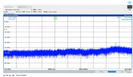
NTNV-DC_7A-n2A-PC3-15-5+15-M+M-QPSK-IDLE-DFT-BPSK-Inner_1RB_Right-12000-20000-PASS
