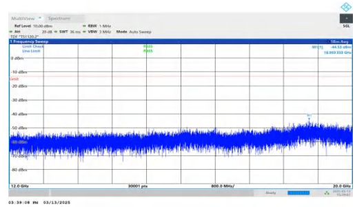
NTNV-DC_7A-n2A-PC3-15-5+5-M+H-QPSK-IDLE-DFT-BPSK-Inner _1RB_Right-12000-20000-PASS
