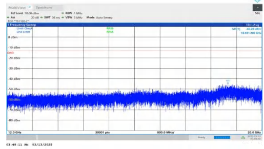
NTNV-DC_7A-n2A-PC3-15-5+15-M+L-QPSK-IDLE-DFT-QPSK-Inner_1RB_Left-12000-20000-PASS
