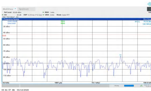
NTNV-DC_7A-n2A-PC3-15-5+10-M+L-QPSK-IDLE-DFT-QPSK-Inner_1RB_Right-0.009-0.15-PASS
