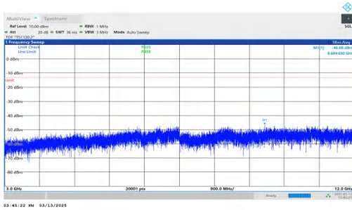
NTNV-DC_7A-n2A-PC3-15-5+10-M+H-QPSK-IDLE-DFT-BPSK-Inner_1RB_Right-3000-12000-PASS
