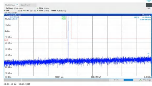
NTNV-DC_7A-n2A-PC3-15-5+20-M+L-QPSK-IDLE-DFT-BPSK-Inner_1RB_Right-1000-3000-PASS
