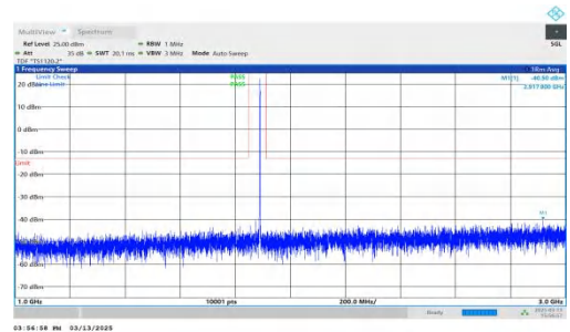
NTNV-DC_7A-n2A-PC3-15-5+20-M+M-QPSK-IDLE-DFT-QPSK-Inner_1RB_Right-1000-3000-PASS
