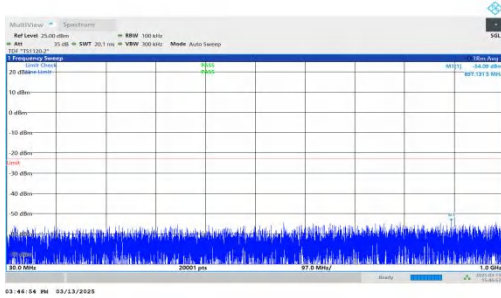
NTNV-DC_7A-n2A-PC3-15-5+15-M+L-QPSK-IDLE-DFT-BPSK-Inner_1RB_Left-30-1000-PASS
