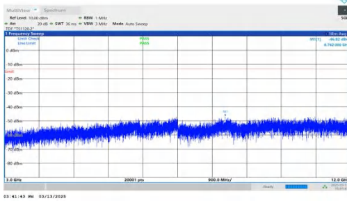
NTNV-DC_7A-n2A-PC3-15-5+10-M+L-QPSK-IDLE-DFT-QPSK-Inner_1RB_Left-3000-12000-PASS
