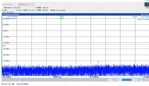
NTNV-DC_7A-n2A-PC3-15-5+15-M+H-QPSK-IDLE-DFT-BPSK-Inner_1RB_Right-30-1000-PASS
