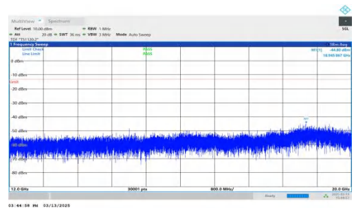
NTNV-DC_7A-n2A-PC3-15-5+10-M+H-QPSK-IDLE-DFT-BPSK-Inner_1RB_Left-12000-20000-PASS
