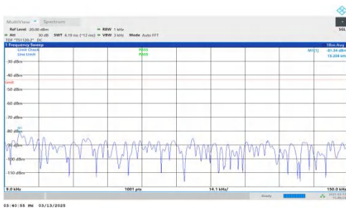
NTNV-DC_7A-n2A-PC3-15-5+10-M+L-QPSK-IDLE-DFT-BPSK-Inner_1RB_Right-0.009-0.15-PASS
