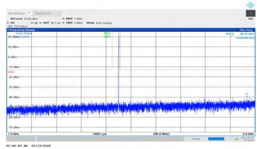
NTNV-DC_7A-n2A-PC3-15-5+10-M+H-QPSK-IDLE-DFT-BPSK-Inner_1RB_Left-1000-3000-PASS
