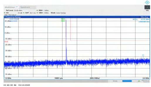
NTNV-DC_7A-n2A-PC3-15-5+15-M+L-QPSK-IDLE-DFT-BPSK-Inner_1RB_Left-1000-3000-PASS
