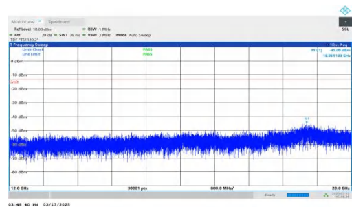
NTNV-DC_7A-n2A-PC3-15-5+15-M+L-QPSK-IDLE-DFT-QPSK-Inner_1RB_Right-12000-20000-PASS
