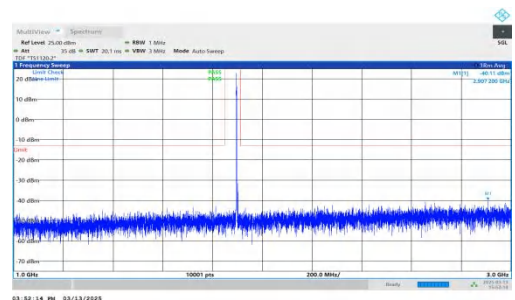
NTNV-DC_7A-n2A-PC3-15-5+15-M+H-QPSK-IDLE-DFT-QPSK-Inner_1RB_Left-1000-3000-PASS
