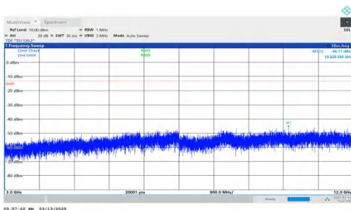
NTNV-DC_7A-n2A-PC3-15-5+20-M+M-QPSK-IDLE-DFT-QPSK-Inner_1RB_Right-3000-12000-PASS
