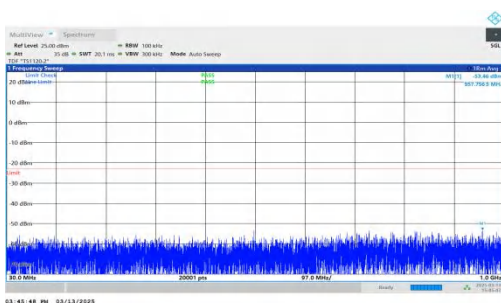
NTNV-DC_7A-n2A-PC3-15-5+10-M+H-QPSK-IDLE-DFT-QPSK-Inner_1RB_Left-30-1000-PASS
