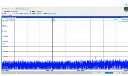
NTNV-DC_7A-n2A-PC3-15-5+20-M+M-QPSK-IDLE-DFT-QPSK-Inner_1RB_Left-30-1000-PASS
