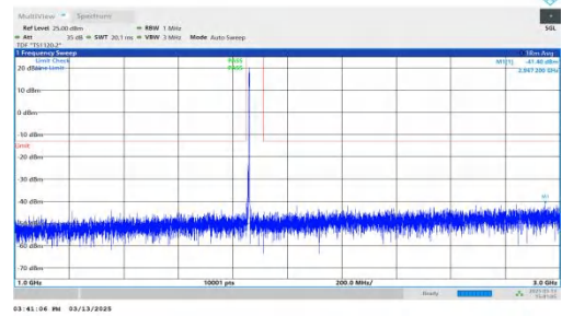
NTNV-DC_7A-n2A-PC3-15-5+10-M+L-QPSK-IDLE-DFT-BPSK-Inner_1RB_Right-1000-3000-PASS
