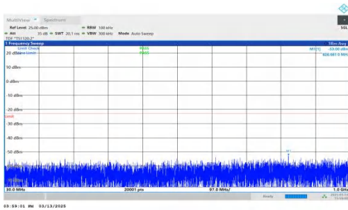
NTNV-DC_7A-n2A-PC3-15-5+20-M+H-QPSK-IDLE-DFT-QPSK-Inner_1RB_Right-30-1000-PASS
