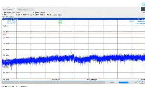
NTNV-DC_7A-n2A-PC3-15-5+10-M+L-QPSK-IDLE-DFT-QPSK-Inner_1RB_Right-3000-12000-PASS
