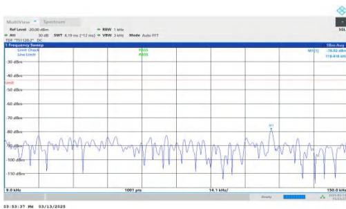
NTNV-DC_7A-n2A-PC3-15-5+20-M+L-QPSK-IDLE-DFT-BPSK-Inner_1RB_Right-0.009-0.15-PASS
