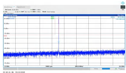
NTNV-DC_7A-n2A-PC3-15-5+10-M+H-QPSK-IDLE-DFT-QPSK-Inner_1RB_Right-1000-3000-PASS
