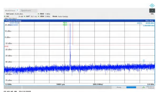
NTNV-DC_7A-n2A-PC3-15-5+10-M+M-QPSK-IDLE-DFT-QPSK-Inner_1RB_Left-1000-3000-PASS
