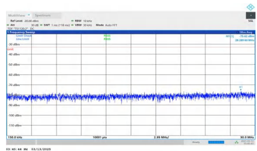
NTNV-DC_7A-n2A-PC3-15-5+10-M+H-QPSK-IDLE-DFT-QPSK-Inner_1RB_Left-0.15-30-PASS
