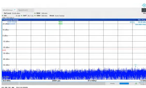
NTNV-DC_7A-n2A-PC3-15-5+20-M+H-QPSK-IDLE-DFT-QPSK-Inner_1RB_Left-30-1000-PASS
