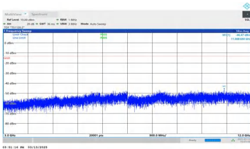
NTNV-DC_7A-n2A-PC3-15-5+15-M+H-QPSK-IDLE-DFT-BPSK-Inner_1RB_Left-3000-12000-PASS
