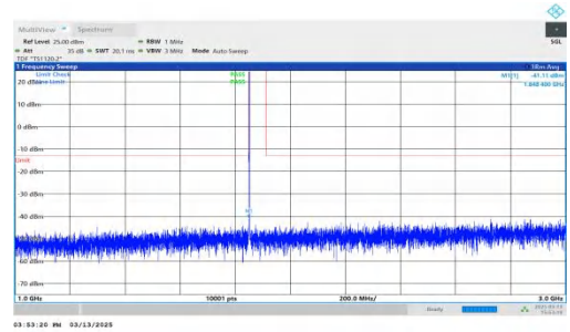
NTNV-DC_7A-n2A-PC3-15-5+20-M+L-QPSK-IDLE-DFT-BPSK-Inner_1RB_Left-1000-3000-PASS
