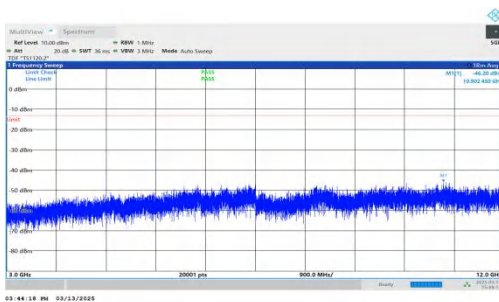
NTNV-DC_7A-n2A-PC3-15-5+10-M+M-QPSK-IDLE-DFT-QPSK-Inner_1RB_Right-3000-12000-PASS
