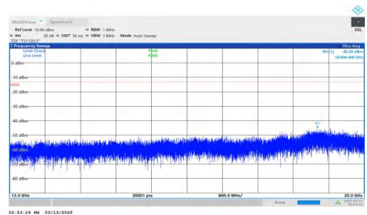
NTNV-DC_7A-n2A-PC3-15-5+20-M+L-QPSK-IDLE-DFT-BPSK-Inner_1RB_Left-12000-20000-PASS
