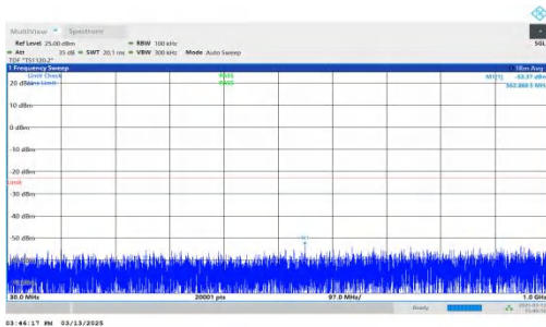
NTNV-DC_7A-n2A-PC3-15-5+10-M+H-QPSK-IDLE-DFT-QPSK-Inner_1RB_Right-30-1000-PASS
