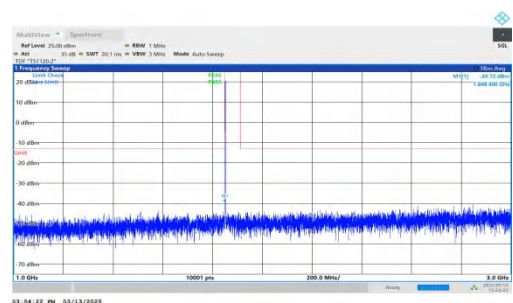
NTNV-DC_7A-n2A-PC3-15-5+20-M+L-QPSK-IDLE-DFT-QPSK-Inner_1RB_Left-1000-3000-PASS
