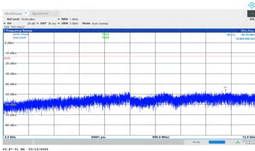
NTNV-DC_7A-n2A-PC3-15-5+15-M+L-QPSK-IDLE-DFT-BPSK-Inner_1RB_Right-3000-12000-PASS
