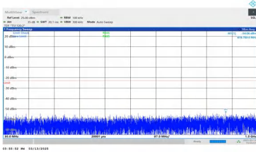
NTNV-DC_7A-n2A-PC3-15-5+20-M+M-QPSK-IDLE-DFT-BPSK-Inner_1RB_Right-30-1000-PASS
