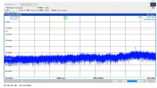
NTNV-DC_7A-n2A-PC3-15-5+15-M+H-QPSK-IDLE-DFT-QPSK-Inner_1RB_Left-12000-20000-PASS
