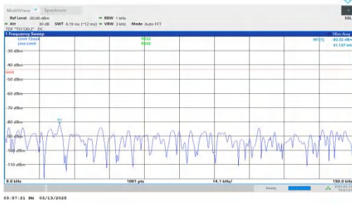
NTNV-DC_7A-n2A-PC3-15-5+20-M+H-QPSK-IDLE-DFT-BPSK-Inner_1RB_Left-0.009-0.15-PASS
