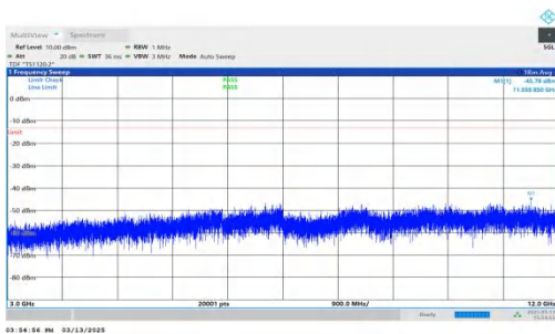
NTNV-DC_7A-n2A-PC3-15-5+20-M+L-QPSK-IDLE-DFT-QPSK-Inner_1RB_Right-3000-12000-PASS
