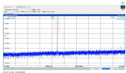
NTNV-DC_7A-n2A-PC3-15-5+15-M+M-QPSK-IDLE-DFT-QPSK-Inner_1RB_Right-1000-3000-PASS
