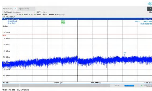
NTNV-DC_7A-n2A-PC3-15-5+20-M+M-QPSK-IDLE-DFT-BPSK-Inner_1RB_Left-3000-12000-PASS
