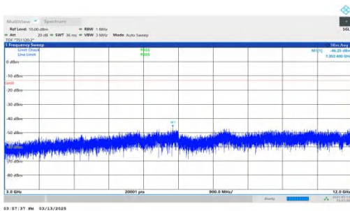
NTNV-DC_7A-n2A-PC3-15-5+20-M+H-QPSK-IDLE-DFT-BPSK-Inner_1RB_Left-3000-12000-PASS
