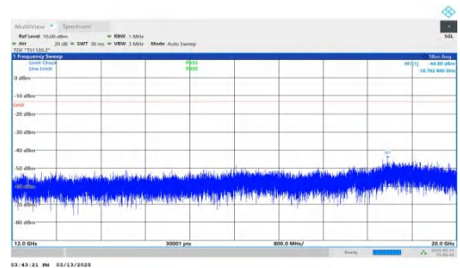
NTNV-DC_7A-n2A-PC3-15-5+10-M+M-QPSK-IDLE-DFT-BPSK-Inner_1RB_Right-12000-20000-PASS
