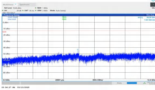
NTNV-DC_7A-n2A-PC3-15-5+20-M+L-QPSK-IDLE-DFT-QPSK-Inner_1RB_Left-3000-12000-PASS
