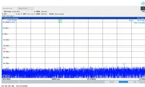
NTNV-DC_7A-n2A-PC3-15-5+20-M+M-QPSK-IDLE-DFT-QPSK-Inner_1RB_Right-30-1000-PASS
