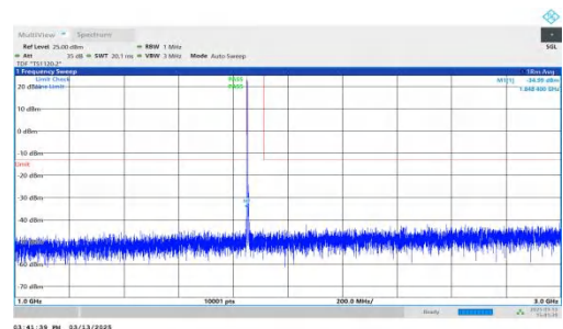
NTNV-DC_7A-n2A-PC3-15-5+10-M+L-QPSK-IDLE-DFT-QPSK-Inner_1RB_Left-1000-3000-PASS
