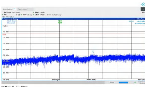
NTNV-DC_7A-n2A-PC3-15-5+10-M+H-QPSK-IDLE-DFT-QPSK-Inner_1RB_Right-3000-12000-PASS
