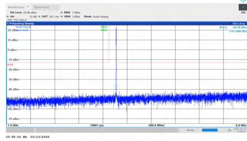
NTNV-DC_7A-n2A-PC3-15-5+20-M+H-QPSK-IDLE-DFT-BPSK-Inner_1RB_Right-1000-3000-PASS
