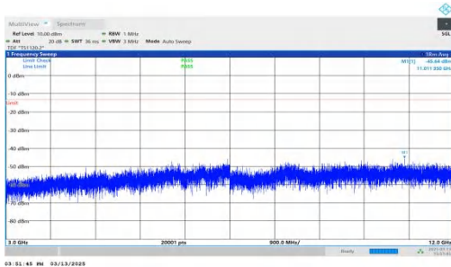
NTNV-DC_7A-n2A-PC3-15-5+15-M+H-QPSK-IDLE-DFT-BPSK-Inner_1RB_Right-3000-12000-PASS
