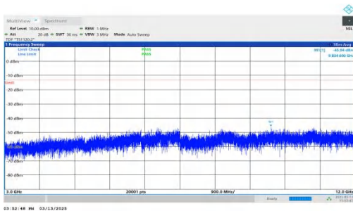
NTNV-DC_7A-n2A-PC3-15-5+15-M+H-QPSK-IDLE-DFT-QPSK-Inner_1RB_Right-3000-12000-PASS
