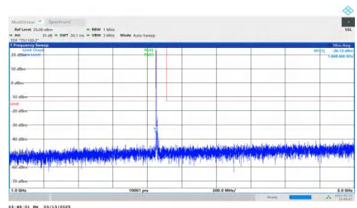
NTNV-DC_7A-n2A-PC3-15-5+15-M+L-QPSK-IDLE-DFT-QPSK-Inner_1RB_Left-1000-3000-PASS
