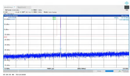
NTNV-DC_7A-n2A-PC3-15-5+20-M+H-QPSK-IDLE-DFT-QPSK-Inner_1RB_Right-1000-3000-PASS
