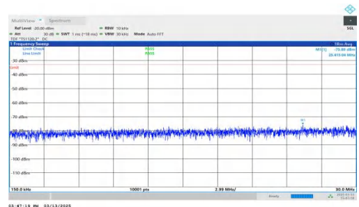
NTNV-DC_7A-n2A-PC3-15-5+15-M+L-QPSK-IDLE-DFT-BPSK-Inner_1RB_Right-0.15-30-PASS
