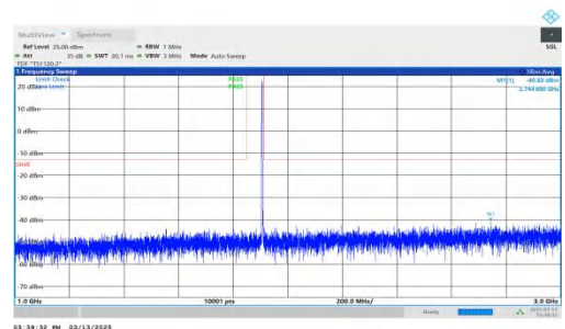
NTNV-DC_7A-n2A-PC3-15-5+5-M+H-QPSK-IDLE-DFT-QPSK-Inner _1RB_Left-1000-3000-PASS
