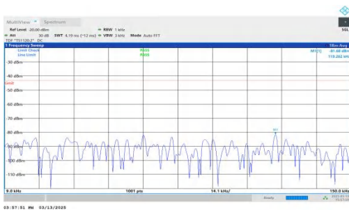
NTNV-DC_7A-n2A-PC3-15-5+20-M+H-QPSK-IDLE-DFT-BPSK-Inner_1RB_Right-0.009-0.15-PASS
