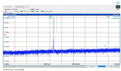
NTNV-DC_7A-n2A-PC3-15-5+15-M+L-QPSK-IDLE-DFT-QPSK-Inner_1RB_Right-1000-3000-PASS
