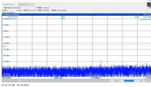
NTNV-DC_7A-n2A-PC3-15-5+10-M+L-QPSK-IDLE-DFT-BPSK-Inner_1RB_Right-30-1000-PASS
