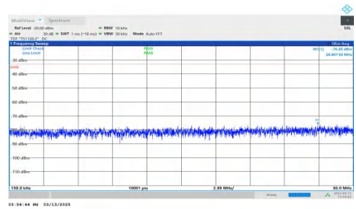
NTNV-DC_7A-n2A-PC3-15-5+20-M+L-QPSK-IDLE-DFT-QPSK-Inner_1RB_Right-0.15-30-PASS
