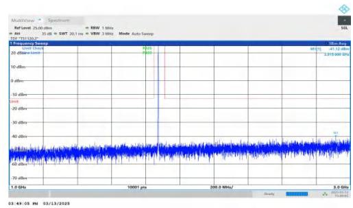
NTNV-DC_7A-n2A-PC3-15-5+15-M+M-QPSK-IDLE-DFT-BPSK-Inner_1RB_Left-1000-3000-PASS
