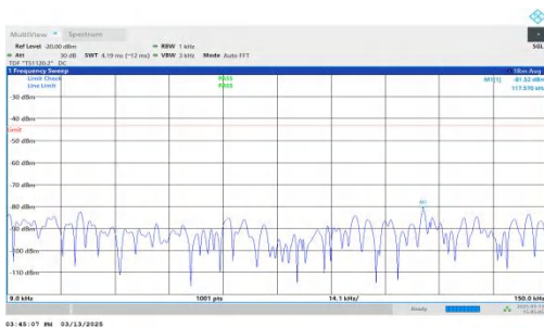
NTNV-DC_7A-n2A-PC3-15-5+10-M+H-QPSK-IDLE-DFT-BPSK-Inner_1RB_Right-0.009-0.15-PASS
