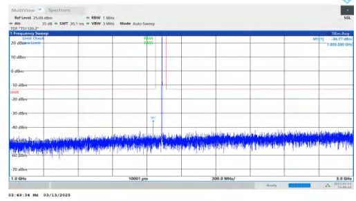
NTNV-DC_7A-n2A-PC3-15-5+15-M+M-QPSK-IDLE-DFT-BPSK-Inner_1RB_Right-1000-3000-PASS
