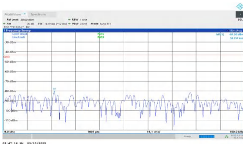
NTNV-DC_7A-n2A-PC3-15-5+15-M+L-QPSK-IDLE-DFT-BPSK-Inner_1RB_Right-0.009-0.15-PASS
