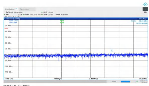
NTNV-DC_7A-n2A-PC3-15-5+20-M+M-QPSK-IDLE-DFT-BPSK-Inner_1RB_Right-0.15-30-PASS
