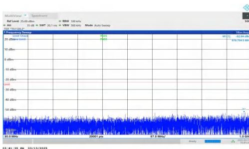
NTNV-DC_7A-n2A-PC3-15-5+10-M+L-QPSK-IDLE-DFT-QPSK-Inner_1RB_Left-30-1000-PASS
