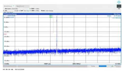
NTNV-DC_7A-n2A-PC3-15-5+5-M+H-QPSK-IDLE-DFT-BPSK-Inner _1RB_Right-1000-3000-PASS
