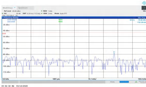
NTNV-DC_7A-n2A-PC3-15-5+15-M+H-QPSK-IDLE-DFT-QPSK-Inner_1RB_Right-0.009-0.15-PASS
