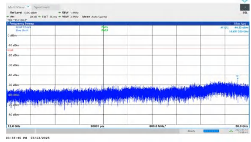
NTNV-DC_7A-n2A-PC3-15-5+20-M+H-QPSK-IDLE-DFT-QPSK-Inner_1RB_Left-12000-20000-PASS
