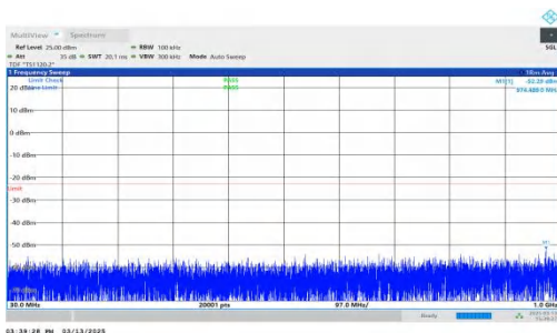
NTNV-DC_7A-n2A-PC3-15-5+5-M+H-QPSK-IDLE-DFT-QPSK-Inner r_1RB_Left-30-1000-PASS
