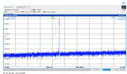
NTNV-DC_7A-n2A-PC3-15-5+15-M+H-QPSK-IDLE-DFT-QPSK-Inner_1RB_Right-1000-3000-PASS
