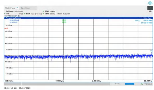
NTNV-DC_7A-n2A-PC3-15-5+10-M+H-QPSK-IDLE-DFT-QPSK-Inner_1RB_Right-0.15-30-PASS
