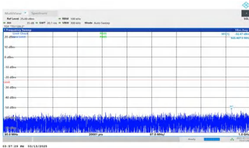
NTNV-DC_7A-n2A-PC3-15-5+20-M+H-QPSK-IDLE-DFT-BPSK-Inner_1RB_Left-30-1000-PASS
