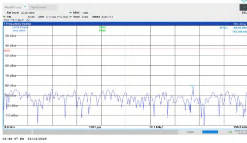
NTNV-DC_7A-n2A-PC3-15-5+10-M+H-QPSK-IDLE-DFT-BPSK-Inner_1RB_Left-0.009-0.15-PASS
