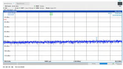
NTNV-DC_7A-n2A-PC3-15-5+15-M+L-QPSK-IDLE-DFT-BPSK-Inner_1RB_Left-0.15-30-PASS
