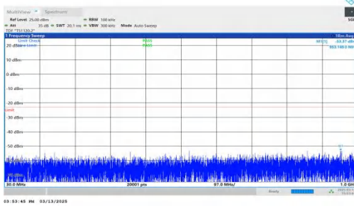
NTNV-DC_7A-n2A-PC3-15-5+20-M+L-QPSK-IDLE-DFT-BPSK-Inner_1RB_Right-30-1000-PASS
