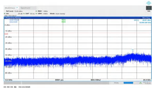
NTNV-DC_7A-n2A-PC3-15-5+20-M+M-QPSK-IDLE-DFT-BPSK-Inner_1RB_Right-12000-20000-PASS
