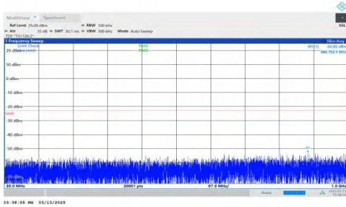
NTNV-DC_7A-n2A-PC3-15-5+5-M+H-QPSK-IDLE-DFT-BPSK-Inner r_1RB_Right-30-1000-PASS
