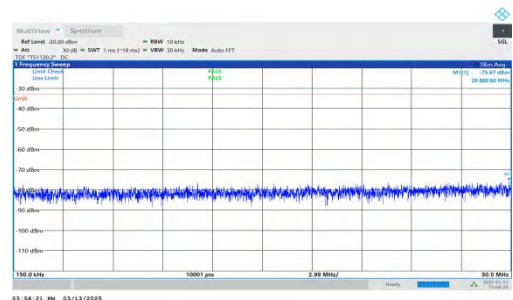
NTNV-DC_7A-n2A-PC3-15-5+20-M+M-QPSK-IDLE-DFT-QPSK-Inner_1RB_Left-0.15-30-PASS
