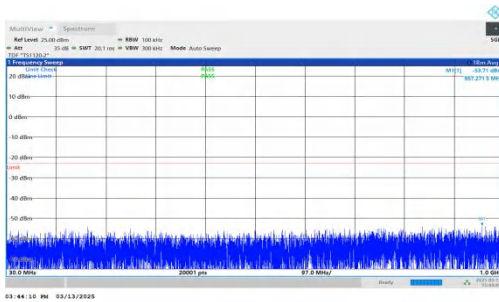
NTNV-DC_7A-n2A-PC3-15-5+10-M+M-QPSK-IDLE-DFT-QPSK-Inner_1RB_Right-30-1000-PASS
