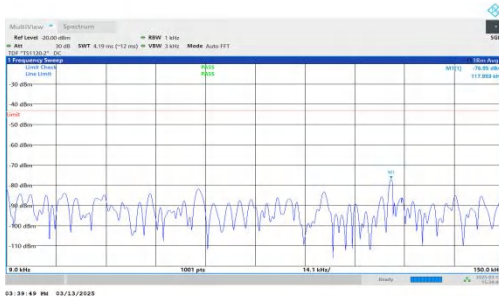
NTNV-DC_7A-n2A-PC3-15-5+5-M+H-QPSK-IDLE-DFT-QPSK-Inner_r_1RB_Right-0.009-0.15-PASS
