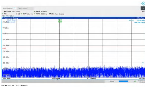
NTNV-DC_7A-n2A-PC3-15-5+15-M+L-QPSK-IDLE-DFT-QPSK-Inner_1RB_Right-30-1000-PASS
