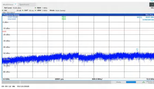
NTNV-DC_7A-n2A-PC3-15-5+15-M+M-QPSK-IDLE-DFT-QPSK-Inner_1RB_Left-3000-12000-PASS
