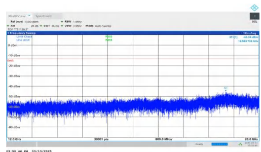
NTNV-DC_7A-n2A-PC3-15-5+15-M+M-QPSK-IDLE-DFT-QPSK-Inner_1RB_Right-12000-20000-PASS
