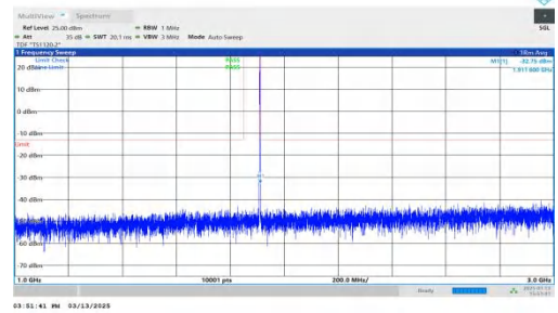
NTNV-DC_7A-n2A-PC3-15-5+15-M+H-QPSK-IDLE-DFT-BPSK-Inner_1RB_Right-1000-3000-PASS
