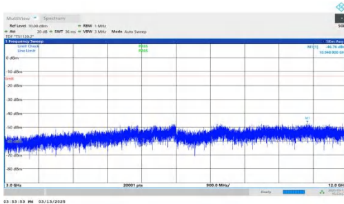
NTNV-DC_7A-n2A-PC3-15-5+20-M+L-QPSK-IDLE-DFT-BPSK-Inner_1RB_Right-3000-12000-PASS
