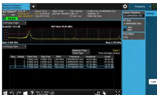
NTNV-n78(3700-3800)-PC2-30-50-L-CP-QPSK-Edge_1RB_Left-PAS
