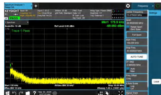
NTNV-n78(3700-3800)-PC2-30-50-H-CP-QPSK-Inner_1RB_Left-0. 15-30-PASS
