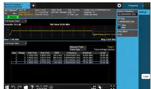
NTNV-n78(3700-3800)-PC2-30-40-H-CP-QPSK-Outer_Full-PA
