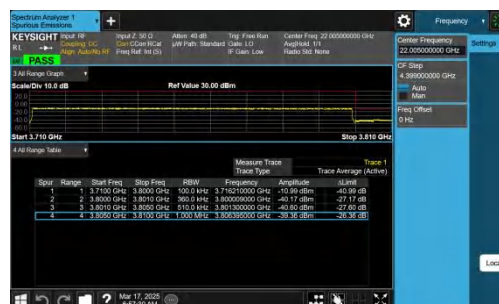
NTNV-n78(3700-3800)-PC2-30-90-H-CP-QPSK-Outer_Full-PA SS
