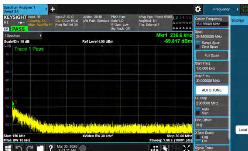
NTNV-n78(3700-3800)-PC2-30-30-L-CP-QPSK-Inner_1RB_Right- 0.15-30-PASS
