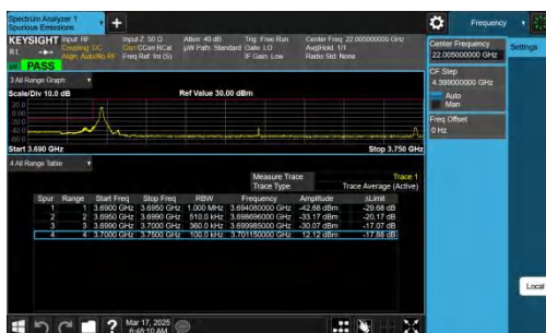
NTNV-n78(3700-3800)-PC2-30-50-L-CP-QPSK-Edge_1RB_Left-PAS
