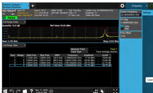
NTNV-n78(3700-3800)-PC2-30-80-H-CP-QPSK-Edge_1RB_Right-PA
