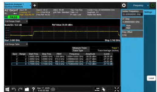
NTNV-n78(3700-3800)-PC2-30-40-L-CP-QPSK-Outer_Full-PAS
