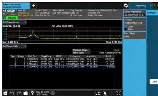
NTNV-n78(3700-3800)-PC2-30-40-L-CP-QPSK-Edge_1RB_Left-PAS
