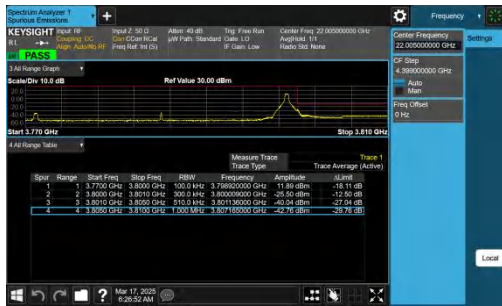
NTNV-n78(3700-3800)-PC2-30-30-H-CP-QPSK-Edge_1RB_Right-PA
