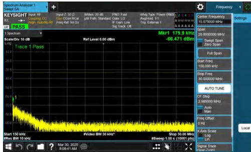
NTNV-n78(3700-3800)-PC2-30-30-H-CP-QPSK-Inner_1RB_Right -0.15-30-PASS
