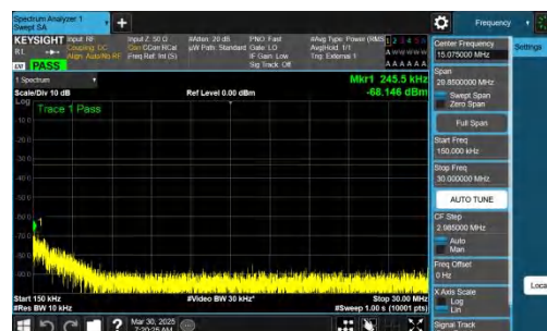
NTNV-n78(3700-3800)-PC2-30-20-L-CP-QPSK-Inner_1RB_Left-0.15-30-PASS
