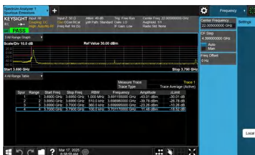
NTNV-n78(3700-3800)-PC2-30-90-L-CP-QPSK-Edge_1RB_Left-PAS
