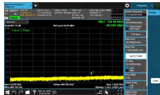
NTNV-n78(3700-3800)-PC2-30-40-H-CP-QPSK-Inner_1RB_Right- 30-1000-PASS
