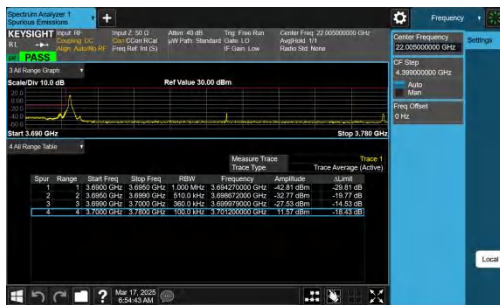
NTNV-n78(3700-3800)-PC2-30-80-L-CP-QPSK-Edge_1RB_Left-PAS
