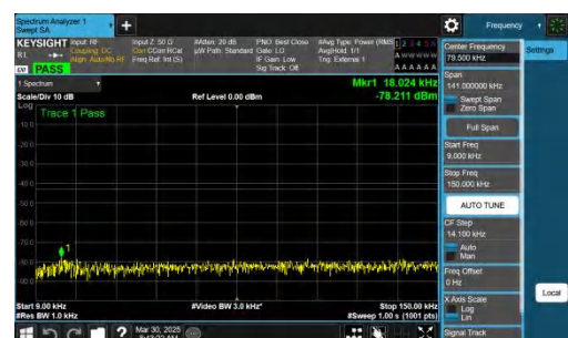
NTNV-n78(3700-3800)-PC2-30-50-L-CP-QPSK-Inner_1RB_Right-0.009-0.15-PASS
