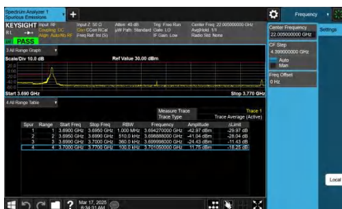
NTNV-n78(3700-3800)-PC2-30-70-L-CP-QPSK-Edge_1RB_Left-PAS
