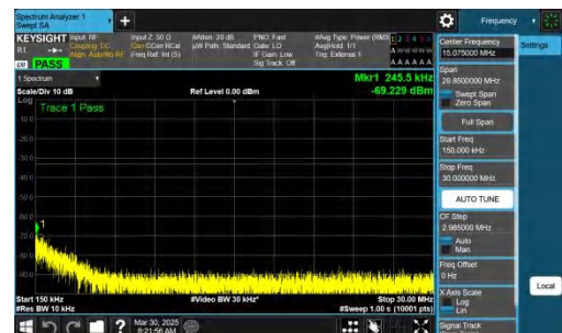
NTNV-n78(3700-3800)-PC2-30-40-M-CP-QPSK-Inner_1RB_Left-0.15-30-PASS
