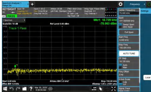
NTNV-n78(3700-3800)-PC2-30-50-L-CP-QPSK-Inner_1RB_Left-0.009-0.15-PASS
