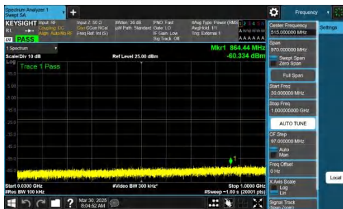
NTNV-n78(3700-3800)-PC2-30-30-H-CP-QPSK-Inner_1RB_Left-30-1000-PASS
