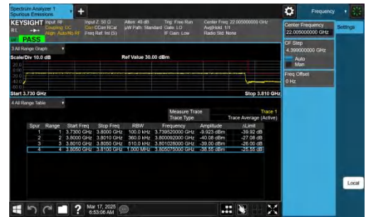
NTNV-n78(3700-3800)-PC2-30-70-H-CP-QPSK-Outer_Full-PA
