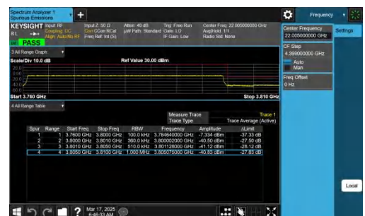
NTNV-n78(3700-3800)-PC2-30-40-H-CP-QPSK-Outer_Full-PA
