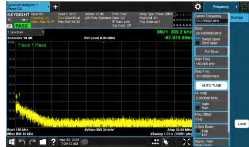
NTNV-n78(3700-3800)-PC2-30-20-M-CP-QPSK-Inner_1RB_Left-0.15-30-PASS
