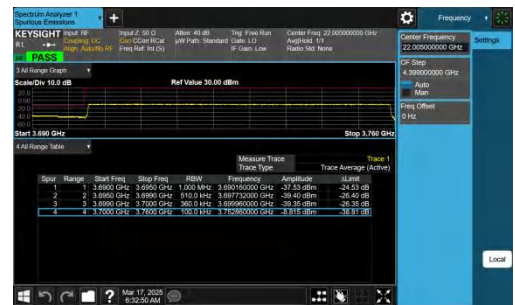
NTNV-n78(3700-3800)-PC2-30-60-L-CP-QPSK-Outer_Full-PAS
