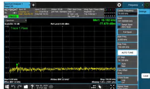
NTNV-n78(3700-3800)-PC2-30-40-L-CP-QPSK-Inner_1RB_Right-0 .009-0.15-PASS
