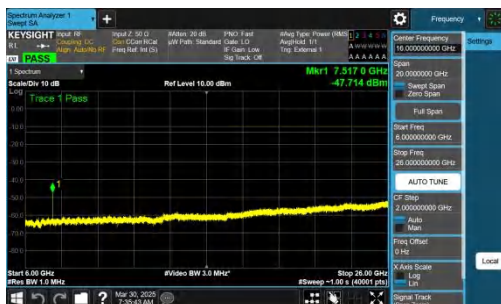
NTNV-n78(3700-3800)-PC2-30-20-M-CP-QPSK-Inner_1RB_Right -6000-26000-PASS
