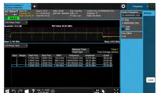
NTNV-n78(3700-3800)-PC2-30-60-H-CP-QPSK-Outer_Full-PA
