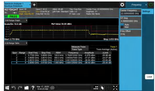
NTNV-n78(3700-3800)-PC2-30-30-H-CP-QPSK-Outer_Full-PA
