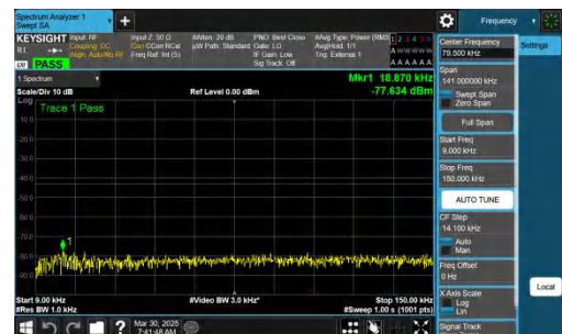
NTNV-n78(3700-3800)-PC2-30-20-H-CP-QPSK-Inner_1RB_Right- 0.009-0.15-PASS
