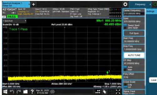
NTNV-n78(3700-3800)-PC2-30-40-L-CP-QPSK-Inner_1RB_Left-3 0-1000-PASS
