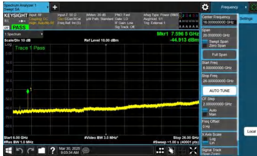
NTNV-n78(3700-3800)-PC2-30-50-H-CP-QPSK-Inner_1RB_Right -6000-26000-PASS
