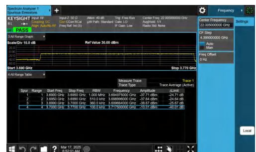
NTNV-n78(3700-3800)-PC2-30-70-L-CP-QPSK-Outer_Full-PAS
