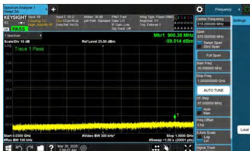
NTNV-n78(3700-3800)-PC2-30-30-M-CP-QPSK-Inner_1RB_Left-30-1000-PASS
