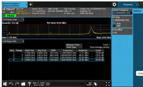
NTNV-n78(3700-3800)-PC2-30-50-H-CP-QPSK-Edge_1RB_Right-PA
