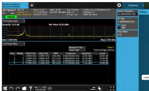
NTNV-n78(3700-3800)-PC2-30-60-L-CP-QPSK-Edge_1RB_Left-PAS
