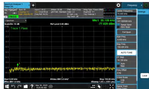
NTNV-n78(3700-3800)-PC2-30-40-M-CP-QPSK-Inner_1RB_Right-0.009-0.15-PASS
