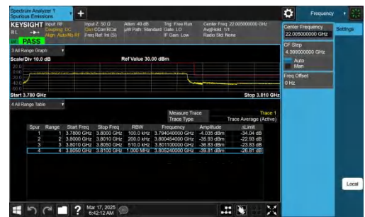
NTNV-n78(3700-3800)-PC2-30-20-H-CP-QPSK-Outer_Full-PA
