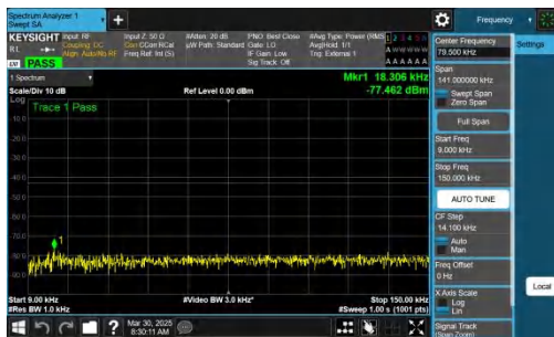
NTNV-n78(3700-3800)-PC2-30-40-H-CP-QPSK-Inner_1RB_Left-0 .009-0.15-PASS
