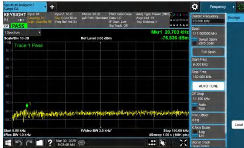
NTNV-n78(3700-3800)-PC2-30-30-H-CP-QPSK-Inner_1RB_Left-0.009-0.15-PASS
