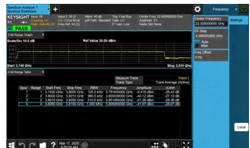
NTNV-n78(3700-3800)-PC2-30-60-H-CP-QPSK-Outer_Full-PA
