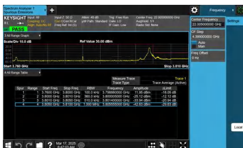
NTNV-n78(3700-3800)-PC2-30-40-H-CP-QPSK-Edge_1RB_Right-PA
