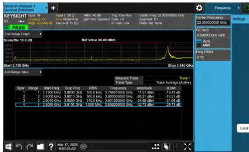
NTNV-n78(3700-3800)-PC2-30-70-H-CP-QPSK-Edge_1RB_Right-PA
