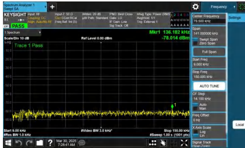
NTNV-n78(3700-3800)-PC2-30-20-M-CP-QPSK-Inner_1RB_Left-0.009-0.15-PASS
