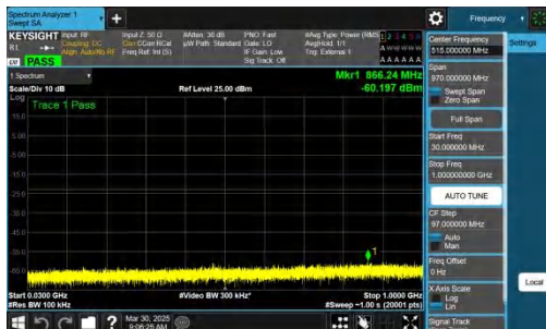
NTNV-n78(3700-3800)-PC2-30-60-L-CP-QPSK-Inner_1RB_Left-3 0-1000-PASS
