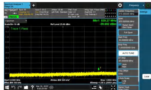
NTNV-n78(3700-3800)-PC2-30-30-M-CP-QPSK-Inner_1RB_Right- 30-1000-PASS
