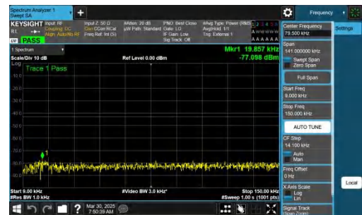
NTNV-n78(3700-3800)-PC2-30-30-L-CP-QPSK-Inner_1RB_Right-0 .009-0.15-PASS
