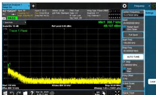
NTNV-n78(3700-3800)-PC2-30-40-M-CP-QPSK-Inner_1RB_Right-0.15-30-PASS
