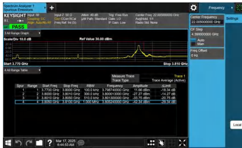
NTNV-n78(3700-3800)-PC2-30-30-H-CP-QPSK-Edge_1RB_Right-PA
