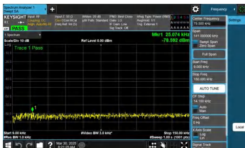
NTNV-n78(3700-3800)-PC2-30-40-M-CP-QPSK-Inner_1RB_Left-0.009-0.15-PASS
