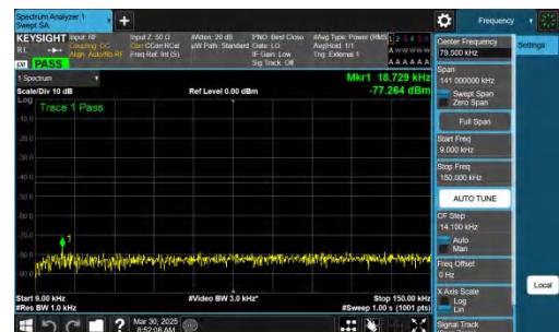
NTNV-n78(3700-3800)-PC2-30-50-M-CP-QPSK-Inner_1RB_Right-0.009-0.15-PASS
