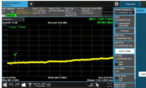
NTNV-n78(3700-3800)-PC2-30-30-L-CP-QPSK-Inner_1RB_Right-6000-26000-PASS
