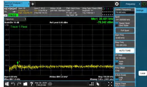
NTNV-n78(3700-3800)-PC2-30-30-M-CP-QPSK-Inner_1RB_Right- 0.009-0.15-PASS
