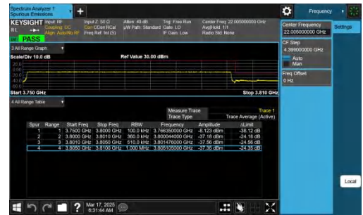
NTNV-n78(3700-3800)-PC2-30-50-H-CP-QPSK-Outer_Full-PA
