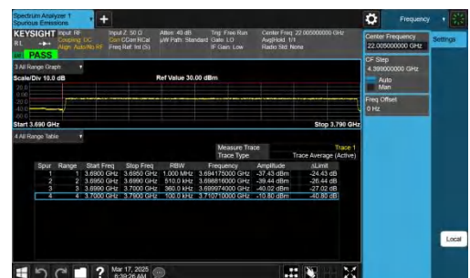
NTNV-n78(3700-3800)-PC2-30-90-L-CP-QPSK-Outer_Full-PAS
