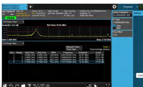
NTNV-n78(3700-3800)-PC2-30-30-L-CP-QPSK-Edge_1RB_Left-PAS
