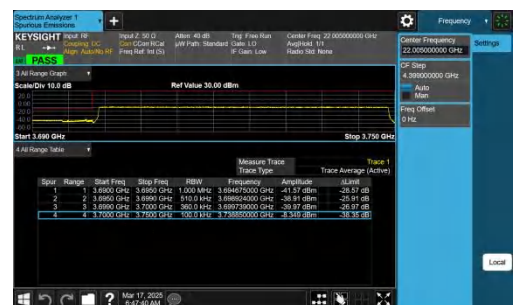
NTNV-n78(3700-3800)-PC2-30-50-L-CP-QPSK-Outer_Full-PAS
