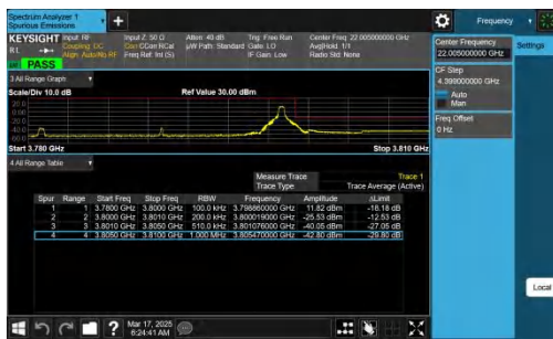
NTNV-n78(3700-3800)-PC2-30-20-H-CP-QPSK-Edge_1RB_Right-PA
