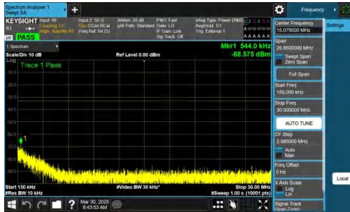
NTNV-n78(3700-3800)-PC2-30-50-L-CP-QPSK-Inner_1RB_Right-0.15-30-PASS
