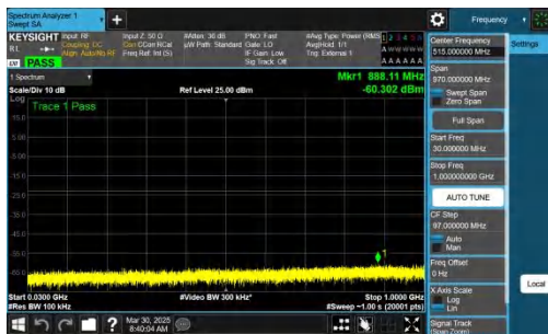
NTNV-n78(3700-3800)-PC2-30-50-L-CP-QPSK-Inner_1RB_Left-30-1000-PASS
