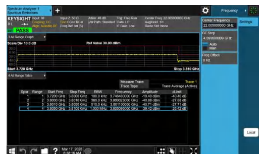
NTNV-n78(3700-3800)-PC2-30-80-H-CP-QPSK-Outer_Full-PA
