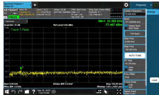
NTNV-n78(3700-3800)-PC2-30-20-L-CP-QPSK-Inner_1RB_Right-0 .009-0.15-PASS
