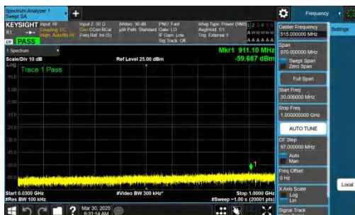
NTNV-n78(3700-3800)-PC2-30-40-H-CP-QPSK-Inner_1RB_Left-3 0-1000-PASS
