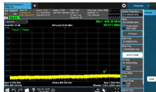
NTNV-n78(3700-3800)-PC2-30-30-L-CP-QPSK-Inner_1RB_Right-3 0-1000-PASS
