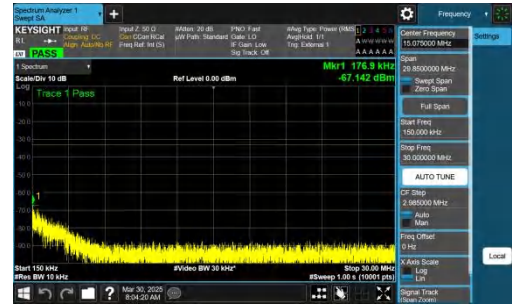
NTNV-n78(3700-3800)-PC2-30-30-H-CP-QPSK-Inner_1RB_Left-0.15-30-PASS
