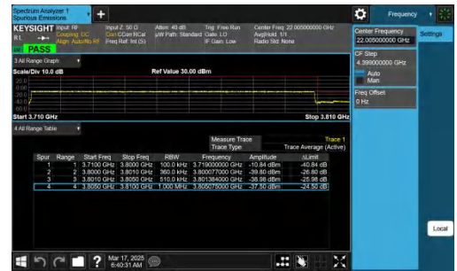
NTNV-n78(3700-3800)-PC2-30-90-H-CP-QPSK-Outer_Full-PA SS
