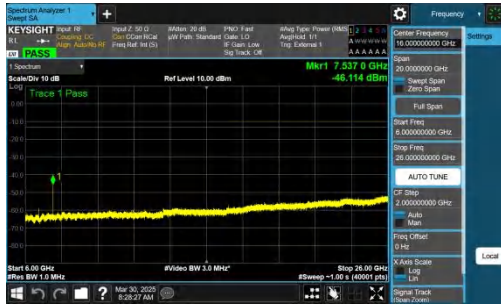
NTNV-n78(3700-3800)-PC2-30-40-M-CP-QPSK-Inner_1RB_Right -6000-26000-PASS
