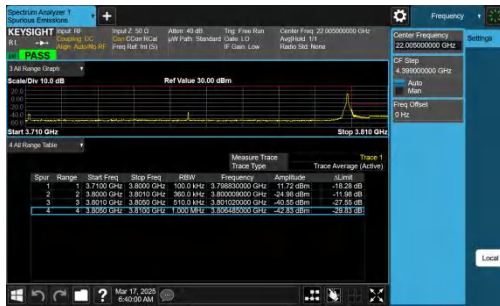
NTNV-n78(3700-3800)-PC2-30-90-H-CP-QPSK-Edge_1RB_Right-PA SS
