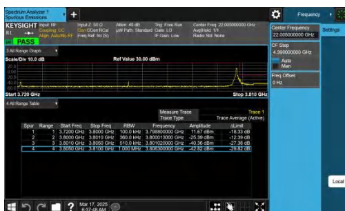
NTNV-n78(3700-3800)-PC2-30-80-H-CP-QPSK-Edge_1RB_Right-PA
