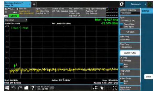
NTNV-n78(3700-3800)-PC2-30-40-H-CP-QPSK-Inner_1RB_Right- 0.009-0.15-PASS
