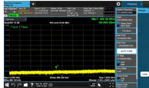
NTNV-n78(3700-3800)-PC2-30-30-H-CP-QPSK-Inner_1RB_Right- 30-1000-PASS
