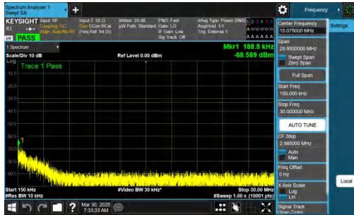
NTNV-n78(3700-3800)-PC2-30-20-M-CP-QPSK-Inner_1RB_Right -0.15-30-PASS
