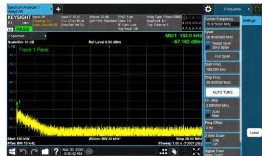
NTNV-n78(3700-3800)-PC2-30-40-H-CP-QPSK-Inner_1RB_Left-0. 15-30-PASS
