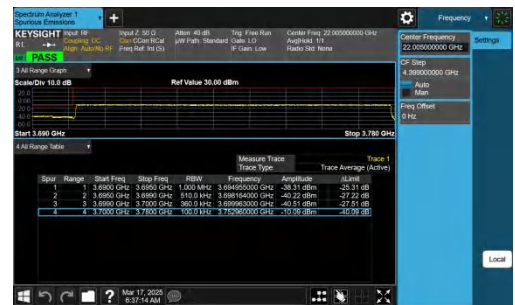
NTNV-n78(3700-3800)-PC2-30-80-L-CP-QPSK-Outer_Full-PAS
