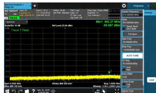
NTNV-n78(3700-3800)-PC2-30-40-M-CP-QPSK-Inner_1RB_Right-30-1000-PASS
