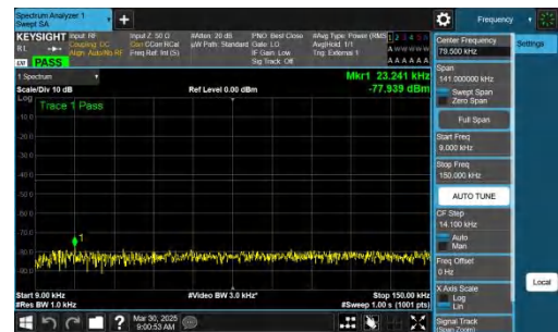
NTNV-n78(3700-3800)-PC2-30-50-H-CP-QPSK-Inner_1RB_Right- 0.009-0.15-PASS
