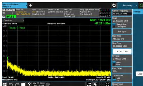
NTNV-n78(3700-3800)-PC2-30-50-H-CP-QPSK-Inner_1RB_Right -0.15-30-PASS
