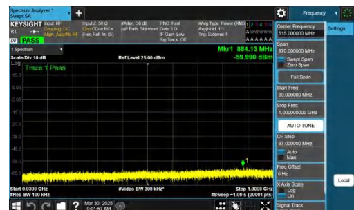
NTNV-n78(3700-3800)-PC2-30-50-H-CP-QPSK-Inner_1RB_Right- 30-1000-PASS
