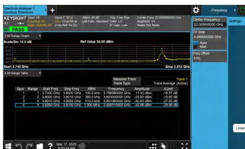
NTNV-n78(3700-3800)-PC2-30-60-H-CP-QPSK-Edge_1RB_Right-PA
