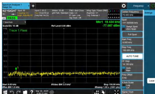
NTNV-n78(3700-3800)-PC2-30-50-H-CP-QPSK-Inner_1RB_Left-0 .009-0.15-PASS
