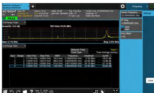
NTNV-n78(3700-3800)-PC2-30-90-H-CP-QPSK-Edge_1RB_Right-PA SS
