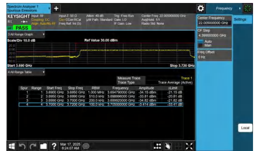
NTNV-n78(3700-3800)-PC2-30-20-L-CP-QPSK-Outer_Full-PAS
