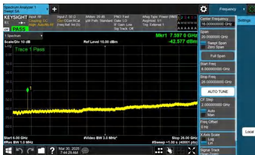
NTNV-n78(3700-3800)-PC2-30-20-H-CP-QPSK-Inner_1RB_Right -6000-26000-PASS
