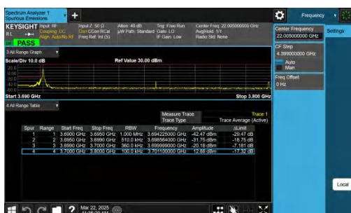
NTNV-n78(3700-3800)-PC2-30-100-L-CP-QPSK-Edge_1RB_Left-PA SS
