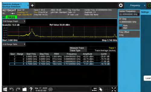
NTNV-n78(3700-3800)-PC2-30-40-L-CP-QPSK-Edge_1RB_Left-PAS
