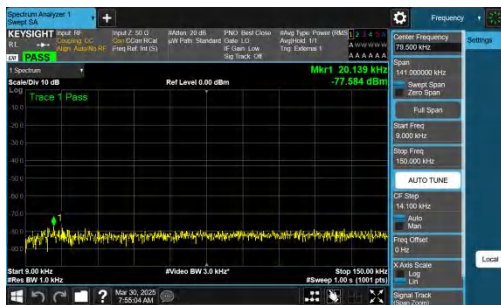
NTNV-n78(3700-3800)-PC2-30-30-M-CP-QPSK-Inner_1RB_Left-0.009-0.15-PASS
