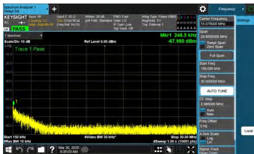
NTNV-n78(3700-3800)-PC2-30-40-H-CP-QPSK-Inner_1RB_Right -0.15-30-PASS
