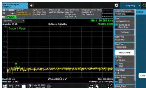
NTNV-n78(3700-3800)-PC2-30-30-L-CP-QPSK-Inner_1RB_Left-0 .009-0.15-PASS
