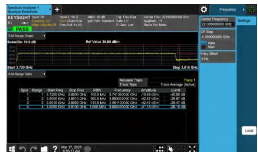
NTNV-n78(3700-3800)-PC2-30-80-H-CP-QPSK-Outer_Full-PA
