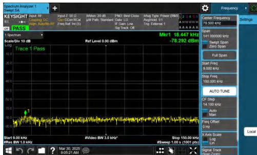
NTNV-n78(3700-3800)-PC2-30-60-L-CP-QPSK-Inner_1RB_Left-0 .009-0.15-PASS
