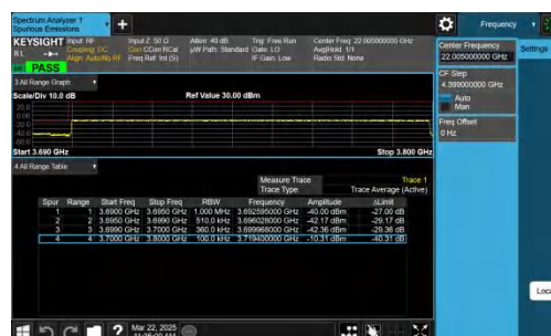
NTNV-n78(3700-3800)-PC2-30-100-L-CP-QPSK-Outer_Full-PA SS
