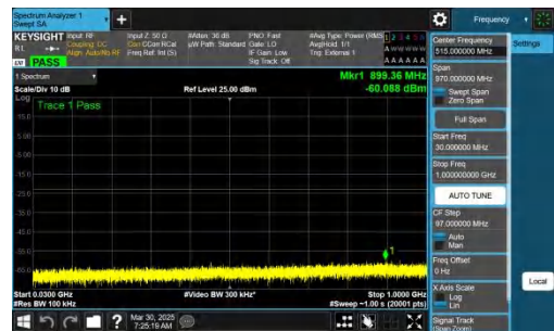
NTNV-n78(3700-3800)-PC2-30-20-L-CP-QPSK-Inner_1RB_Right-3 0-1000-PASS
