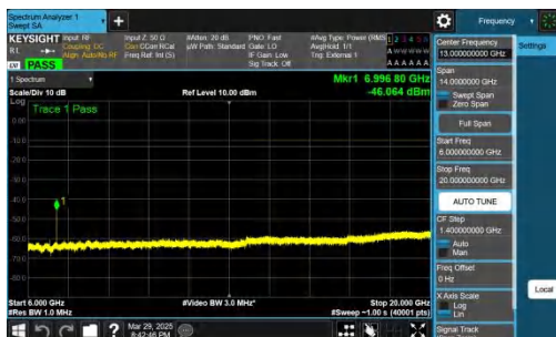
NTNV-n78(3450-3550)-PC2-30-50-L-CP-QPSK-Inner_1RB_Right-6000-20000-PASS
