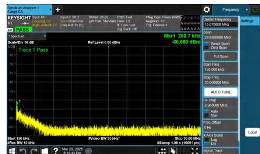
NTNV-n78(3450-3550)-PC2-30-40-M-CP-QPSK-Inner_1RB_Left-0.15-30-PASS
