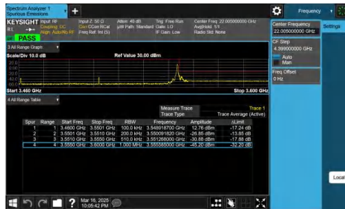
NTNV-n78(3450-3550)-PC2-30-90-H-CP-QPSK-Edge_1RB_Right -PASS
