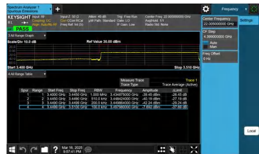
NTNV-n78(3450-3550)-PC2-30-60-L-CP-QPSK-Outer_Full-PASS
