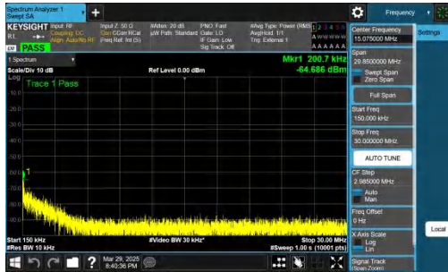
NTNV-n78(3450-3550)-PC2-30-50-L-CP-QPSK-Inner_1RB_Right-0.15-30-PASS
