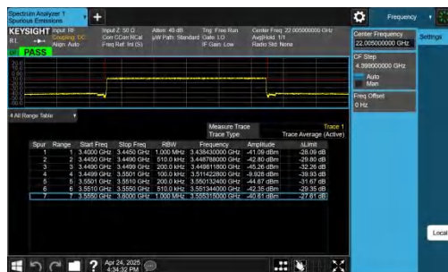
NTNV-n78(3450-3550)-PC2-30-100-L-CP-QPSK-Outer_Full-PASS
