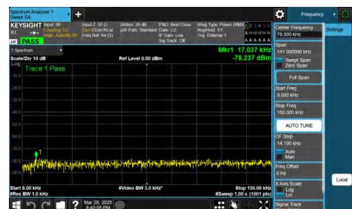
NTNV-n78(3450-3550)-PC2-30-50-L-CP-QPSK-Inner_1RB_Right-0.009-0.15-PASS
