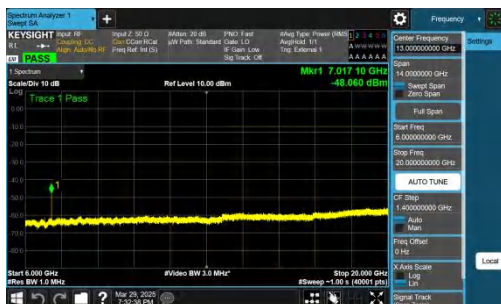
NTNV-n78(3450-3550)-PC2-30-20-M-CP-QPSK-Inner_1RB_Right -6000-20000-PASS
