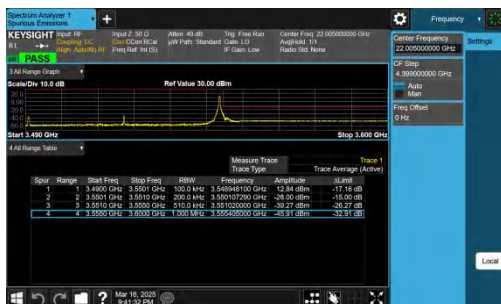
NTNV-n78(3450-3550)-PC2-30-60-H-CP-QPSK-Edge_1RB_Right -PASS
