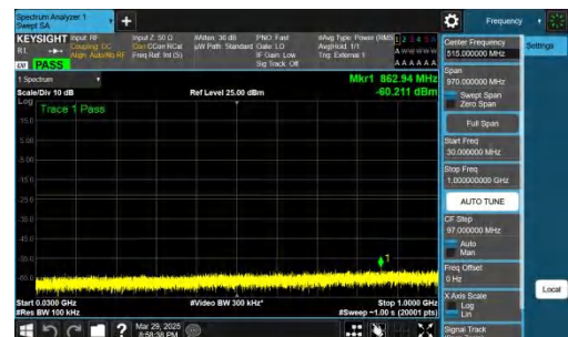
NTNV-n78(3450-3550)-PC2-30-50-H-CP-QPSK-Inner_1RB_Right- 30-1000-PASS
