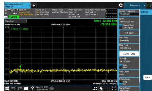
NTNV-n78(3450-3550)-PC2-30-50-H-CP-QPSK-Inner_1RB_Right- 0.009-0.15-PASS
