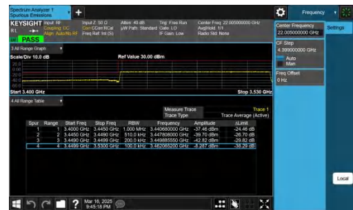
NTNV-n78(3450-3550)-PC2-30-80-L-CP-QPSK-Outer_Full-PASS
