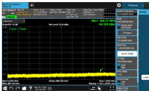
NTNV-n78(3450-3550)-PC2-30-30-H-CP-QPSK-Inner_1RB_Left-30-1000-PASS
