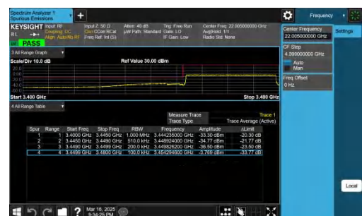
NTNV-n78(3450-3550)-PC2-30-30-L-CP-QPSK-Outer_Full-PASS
