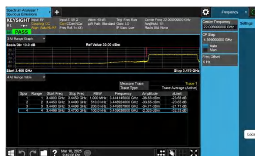
NTNV-n78(3450-3550)-PC2-30-20-L-CP-QPSK-Outer_Full-PASS
