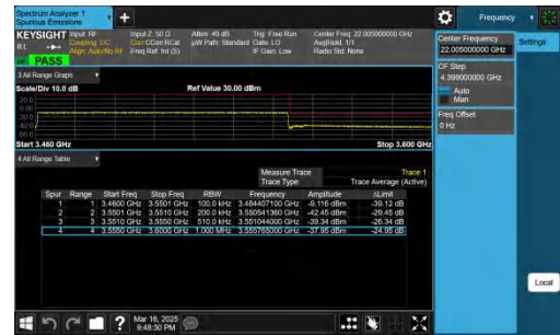
NTNV-n78(3450-3550)-PC2-30-90-H-CP-QPSK-Outer_Full-PASS
