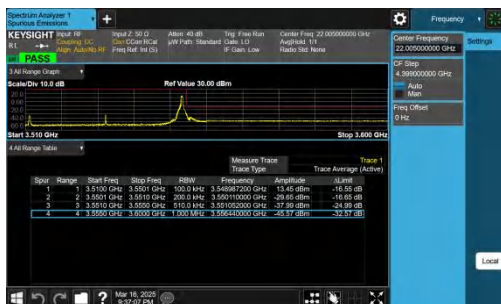
NTNV-n78(3450-3550)-PC2-30-40-H-CP-QPSK-Edge_1RB_Right -PASS
