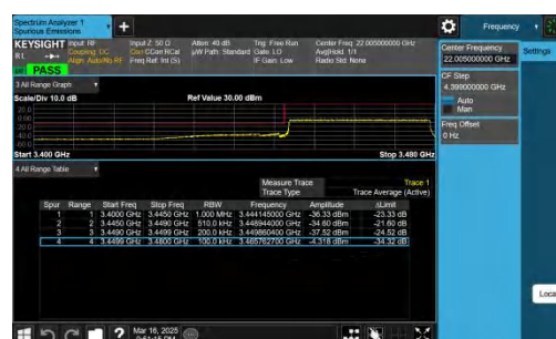
NTNV-n78(3450-3550)-PC2-30-30-L-CP-QPSK-Outer_Full-PASS
