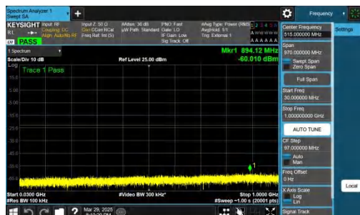
NTNV-n78(3450-3550)-PC2-30-40-L-CP-QPSK-Inner_1RB_Left-3 0-1000-PASS
