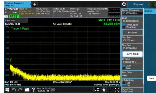
NTNV-n78(3450-3550)-PC2-30-30-H-CP-QPSK-Inner_1RB_Left-0.15-30-PASS
