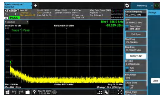
NTNV-n78(3450-3550)-PC2-30-30-M-CP-QPSK-Inner_1RB_Left-0.15-30-PASS
