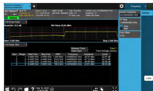
NTNV-n78(3450-3550)-PC2-30-50-L-CP-QPSK-Outer_Full-PASS
