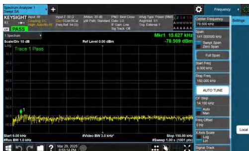
NTNV-n78(3450-3550)-PC2-30-50-H-CP-QPSK-Inner_1RB_Left-0 .009-0.15-PASS
