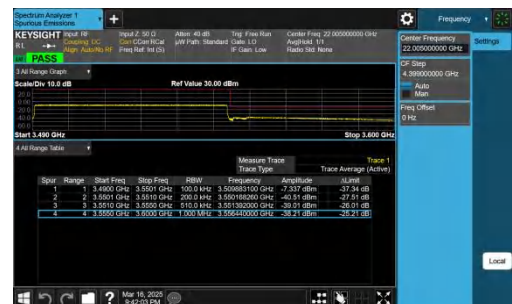
NTNV-n78(3450-3550)-PC2-30-60-H-CP-QPSK-Outer_Full-PASS
