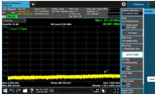
NTNV-n78(3450-3550)-PC2-30-50-M-CP-QPSK-Inner_1RB_Left-30-1000-PASS
