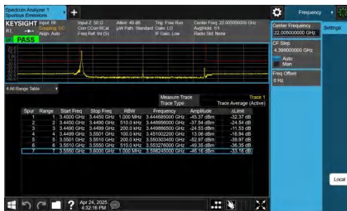
NTNV-n78(3450-3550)-PC2-30-100-L-CP-QPSK-Edge_1RB_Left PASS
