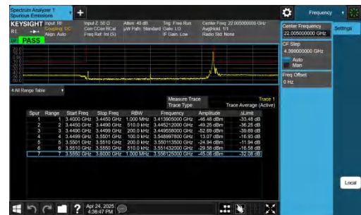
NTNV-n78(3450-3550)-PC2-30-100-L-CP-QPSK-Edge_1RB_Right -PASS
