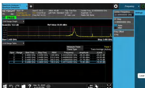
NTNV-n78(3450-3550)-PC2-30-30-L-CP-QPSK-Edge_1RB_Left-P ASS
