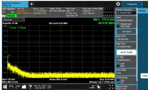
NTNV-n78(3450-3550)-PC2-30-30-H-CP-QPSK-Inner_1RB_Right -0.15-30-PASS
