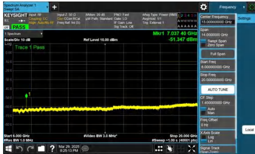
NTNV-n78(3450-3550)-PC2-30-40-M-CP-QPSK-Inner_1RB_Right -6000-20000-PASS
