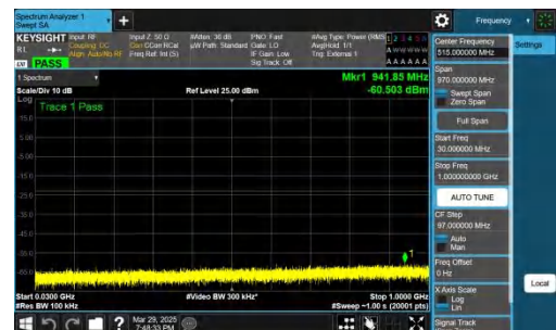
NTNV-n78(3450-3550)-PC2-30-30-L-CP-QPSK-Inner_1RB_Right-3 0-1000-PASS
