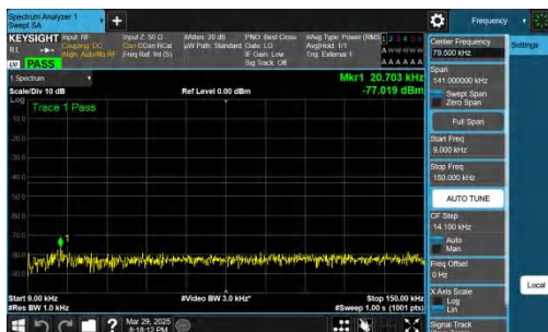
NTNV-n78(3450-3550)-PC2-30-40-M-CP-QPSK-Inner_1RB_Left-0.009-0.15-PASS
