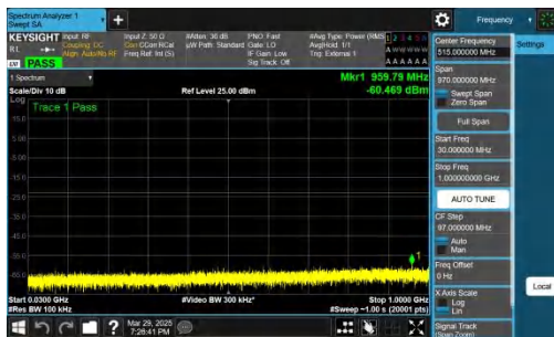
NTNV-n78(3450-3550)-PC2-30-20-M-CP-QPSK-Inner_1RB_Left-30-1000-PASS
