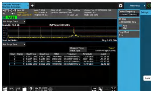
NTNV-n78(3450-3550)-PC2-30-80-H-CP-QPSK-Edge_1RB_Right -PASS
