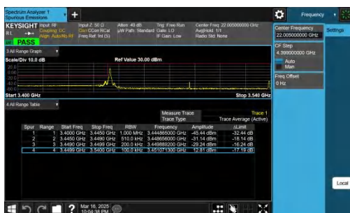
NTNV-n78(3450-3550)-PC2-30-90-L-CP-QPSK-Edge_1RB_Left-PASS
