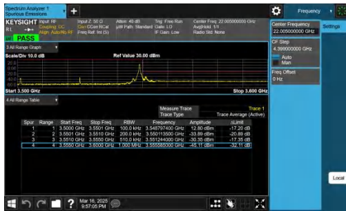
NTNV-n78(3450-3550)-PC2-30-50-H-CP-QPSK-Edge_1RB_Right -PASS
