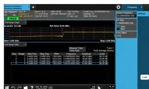
NTNV-n78(3450-3550)-PC2-30-50-L-CP-QPSK-Outer_Full-PASS
