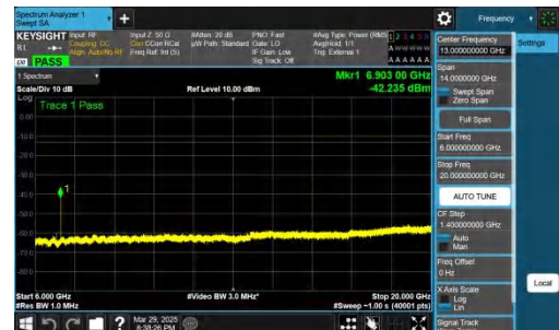
NTNV-n78(3450-3550)-PC2-30-50-L-CP-QPSK-Inner_1RB_Left-6000-20000-PASS
