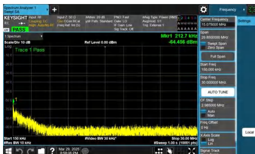
NTNV-n78(3450-3550)-PC2-30-50-H-CP-QPSK-Inner_1RB_Right -0.15-30-PASS
