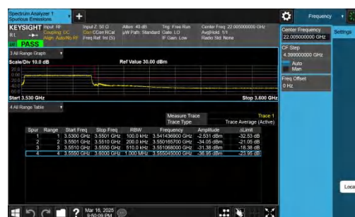
NTNV-n78(3450-3550)-PC2-30-20-H-CP-QPSK-Outer_Full-PASS
