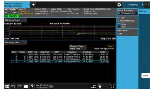
NTNV-n78(3450-3550)-PC2-30-90-H-CP-QPSK-Outer_Full-PASS
