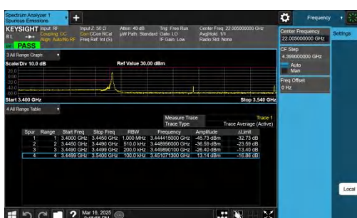
NTNV-n78(3450-3550)-PC2-30-90-L-CP-QPSK-Edge_1RB_Left-PASS
