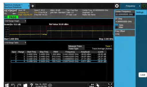
NTNV-n78(3450-3550)-PC2-30-90-L-CP-QPSK-Outer_Full-PASS
