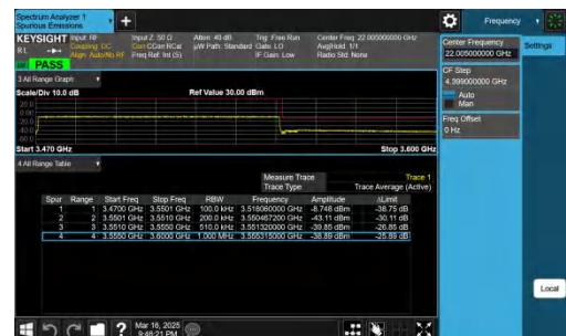
NTNV-n78(3450-3550)-PC2-30-80-H-CP-QPSK-Outer_Full-PASS
