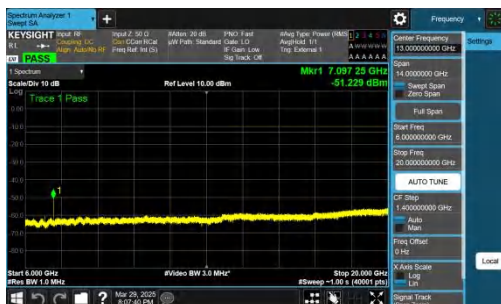
NTNV-n78(3450-3550)-PC2-30-30-H-CP-QPSK-Inner_1RB_Right -6000-20000-PASS
