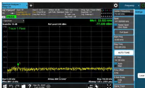
NTNV-n78(3450-3550)-PC2-30-30-L-CP-QPSK-Inner_1RB_Left-0 .009-0.15-PASS
