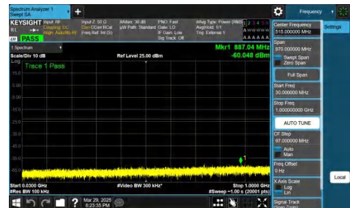
NTNV-n78(3450-3550)-PC2-30-40-M-CP-QPSK-Inner_1RB_Right-30-1000-PASS
