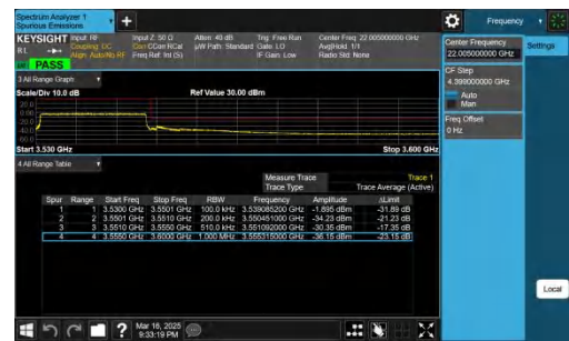
NTNV-n78(3450-3550)-PC2-30-20-H-CP-QPSK-Outer_Full-PASS
