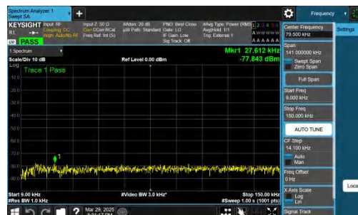
NTNV-n78(3450-3550)-PC2-30-40-H-CP-QPSK-Inner_1RB_Right- 0.009-0.15-PASS
