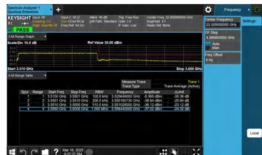
NTNV-n78(3450-3550)-PC2-30-40-H-CP-QPSK-Outer_Full-PASS
