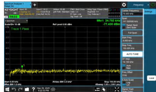
NTNV-n78(3450-3550)-PC2-30-40-M-CP-QPSK-Inner_1RB_Right-0.009-0.15-PASS
