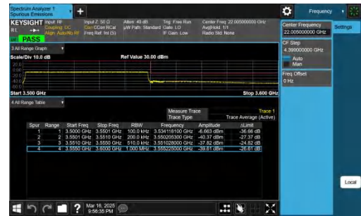
NTNV-n78(3450-3550)-PC2-30-50-H-CP-QPSK-Outer_Full-PASS
