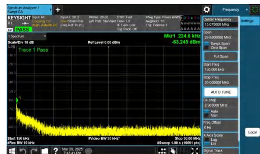
NTNV-n78(3450-3550)-PC2-30-30-L-CP-QPSK-Inner_1RB_Left-0. 15-30-PASS
