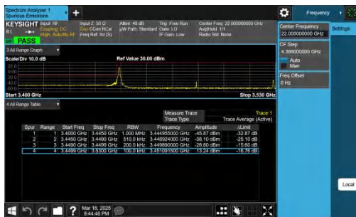
NTNV-n78(3450-3550)-PC2-30-80-L-CP-QPSK-Edge_1RB_Left-PASS
