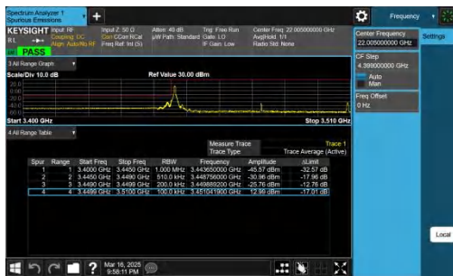
NTNV-n78(3450-3550)-PC2-30-60-L-CP-QPSK-Edge_1RB_Left-P ASS
