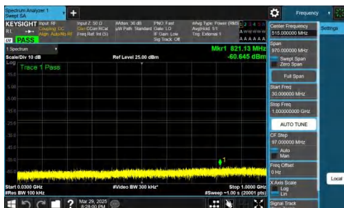
NTNV-n78(3450-3550)-PC2-30-40-H-CP-QPSK-Inner_1RB_Left-3 0-1000-PASS
