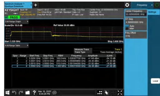
NTNV-n78(3450-3550)-PC2-30-30-H-CP-QPSK-Outer_Full-PASS
