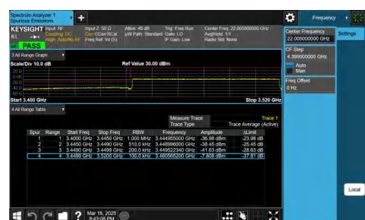
NTNV-n78(3450-3550)-PC2-30-70-L-CP-QPSK-Outer_Full-PASS
