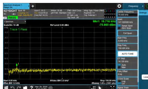
NTNV-n78(3450-3550)-PC2-30-40-L-CP-QPSK-Inner_1RB_Right-0 .009-0.15-PASS
