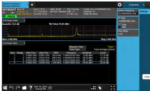
NTNV-n78(3450-3550)-PC2-30-90-H-CP-QPSK-Edge_1RB_Right -PASS
