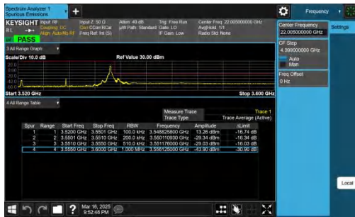
NTNV-n78(3450-3550)-PC2-30-30-H-CP-QPSK-Edge_1RB_Right -PASS
