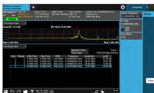
NTNV-n78(3450-3550)-PC2-30-30-L-CP-QPSK-Edge_1RB_Left-P ASS
