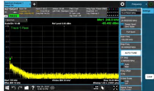
NTNV-n78(3450-3550)-PC2-30-50-L-CP-QPSK-Inner_1RB_Left-0.15-30-PASS
