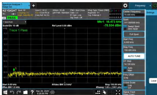
NTNV-n78(3450-3550)-PC2-30-40-H-CP-QPSK-Inner_1RB_Left-0 .009-0.15-PASS
