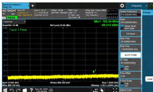
NTNV-n78(3450-3550)-PC2-30-30-M-CP-QPSK-Inner_1RB_Left-30-1000-PASS
