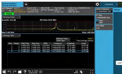
NTNV-n78(3450-3550)-PC2-30-40-L-CP-QPSK-Edge_1RB_Left-PASS
