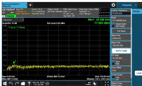
NTNV-n78(3450-3550)-PC2-30-30-M-CP-QPSK-Inner_1RB_Left-0.009-0.15-PASS
