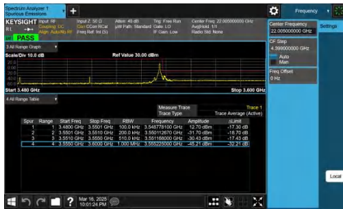
NTNV-n78(3450-3550)-PC2-30-70-H-CP-QPSK-Edge_1RB_Right -PASS
