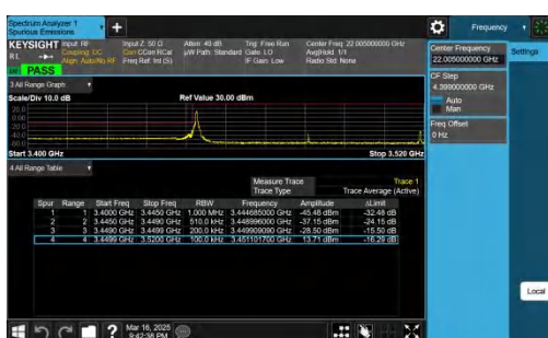
NTNV-n78(3450-3550)-PC2-30-70-L-CP-QPSK-Edge_1RB_Left-P ASS
