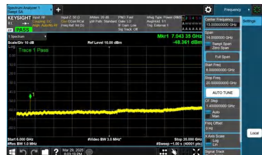
NTNV-n78(3450-3550)-PC2-30-30-H-CP-QPSK-Inner_1RB_Left-6000-20000-PASS
