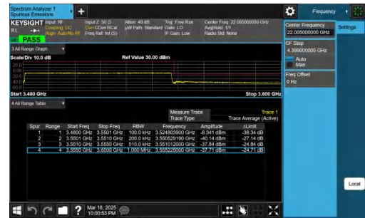
NTNV-n78(3450-3550)-PC2-30-70-H-CP-QPSK-Outer_Full-PASS
