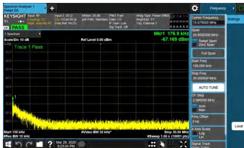
NTNV-n78(3450-3550)-PC2-30-40-M-CP-QPSK-Inner_1RB_Right-0.15-30-PASS
