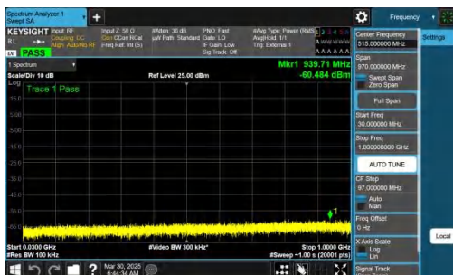
NTNV-n77(3700-3980)-PC2-30-80-L-CP-QPSK-Inner_1RB_Left-3 0-1000-PASS
