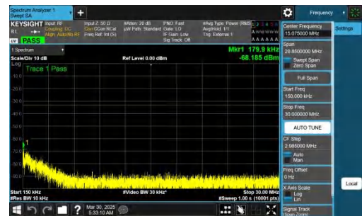
NTNV-n77(3700-3980)-PC2-30-30-M-CP-QPSK-Inner_1RB_Left-0-15-30-PASS
