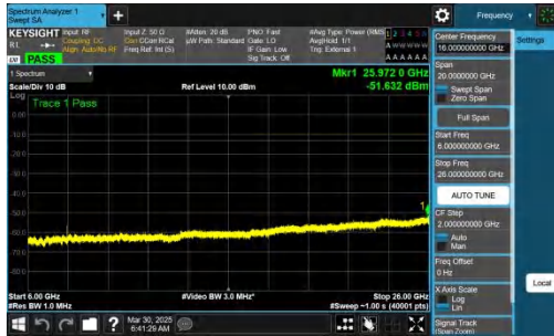
NTNV-n77(3700-3980)-PC2-30-60-H-CP-QPSK-Inner_1RB_Right -6000-26000-PASS
