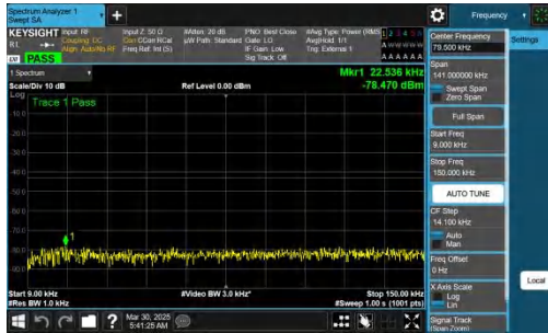
NTNV-n77(3700-3980)-PC2-30-30-H-CP-QPSK-Inner_1RB_Left-0.009-0.15-PASS
