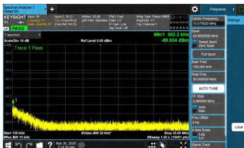
NTNV-n77(3700-3980)-PC2-30-100-L-CP-QPSK-Inner_1RB_Right-0.15-30-PASS
