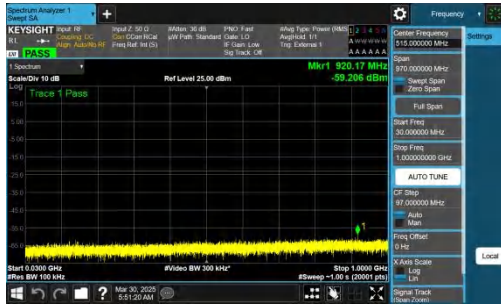
NTNV-n77(3700-3980)-PC2-30-40-L-CP-QPSK-Inner_1RB_Left-3 0-1000-PASS
