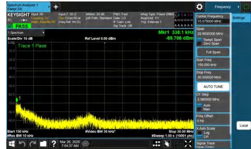
NTNV-n77(3700-3980)-PC2-30-100-H-CP-QPSK-Inner_1RB_Left-0.15-30-PASS
