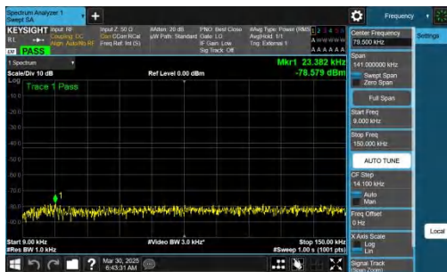
NTNV-n77(3700-3980)-PC2-30-80-L-CP-QPSK-Inner_1RB_Left-0 .009-0.15-PASS
