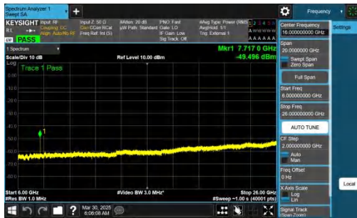
NTNV-n77(3700-3980)-PC2-30-40-M-CP-QPSK-Inner_1RB_Right -6000-26000-PASS
