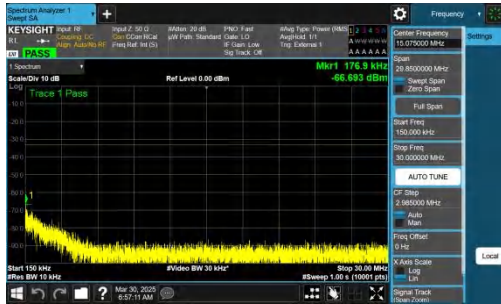
NTNV-n77(3700-3980)-PC2-30-80-M-CP-QPSK-Inner_1RB_Right -0.15-30-PASS
