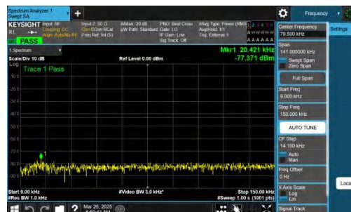
NTNV-n77(3700-3980)-PC2-30-100-M-CP-QPSK-Inner_1RB_Right -0.009-0.15-PASS
