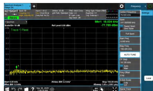
NTNV-n77(3700-3980)-PC2-30-100-H-CP-QPSK-Inner_1RB_Right-0.009-0.15-PASS
