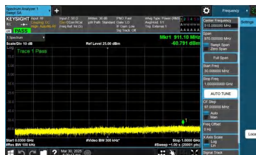
NTNV-n77(3700-3980)-PC2-30-30-L-CP-QPSK-Inner_1RB_Right-3 0-1000-PASS
