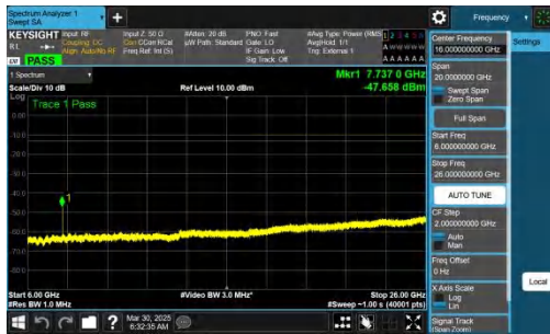
NTNV-n77(3700-3980)-PC2-30-60-M-CP-QPSK-Inner_1RB_Right -6000-26000-PASS
