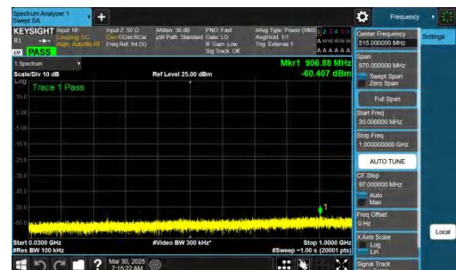
NTNV-n77(3700-3980)-PC2-30-100-L-CP-QPSK-Inner_1RB_Right-30-1000-PASS
