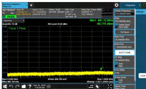
NTNV-n77(3700-3980)-PC2-30-100-H-CP-QPSK-Inner_1RB_Left-30-1000-PASS
