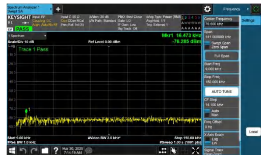
NTNV-n77(3700-3980)-PC2-30-100-L-CP-QPSK-Inner_1RB_Right-0.009-0.15-PASS
