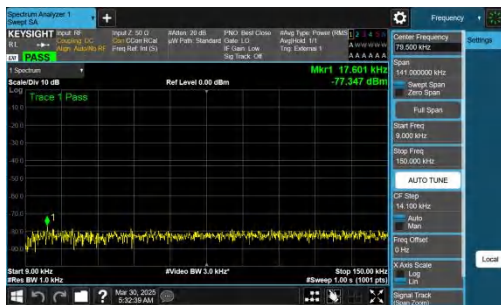
NTNV-n77(3700-3980)-PC2-30-30-M-CP-QPSK-Inner_1RB_Left-0.009-0.15-PASS
