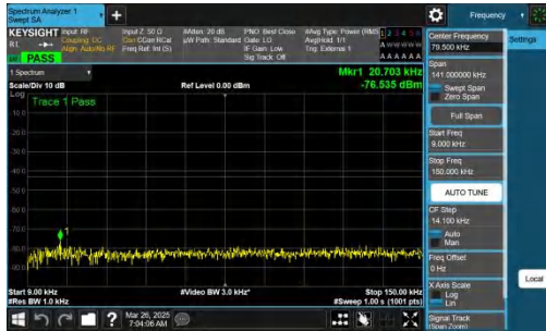
NTNV-n77(3700-3980)-PC2-30-100-H-CP-QPSK-Inner_1RB_Left-0.009-0.15-PASS
