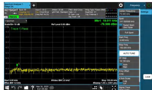
NTNV-n77(3700-3980)-PC2-30-60-L-CP-QPSK-Inner_1RB_Right-0.009-0.15-PASS
