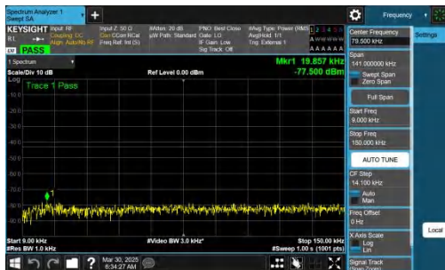
NTNV-n77(3700-3980)-PC2-30-60-H-CP-QPSK-Inner_1RB_Left-0 .009-0.15-PASS
