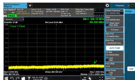
NTNV-n77(3700-3980)-PC2-30-40-L-CP-QPSK-Inner_1RB_Right-3 0-1000-PASS
