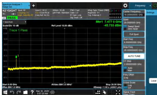
NTNV-n77(3700-3980)-PC2-30-40-L-CP-QPSK-Inner_1RB_Right-6000-26000-PASS
