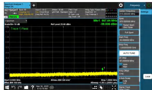
NTNV-n77(3700-3980)-PC2-30-40-H-CP-QPSK-Inner_1RB_Right- 30-1000-PASS
