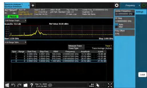
NTNV-n77(3450-3550)-PC2-30-20-H-CP-QPSK-Edge_1RB_Right- PASS
