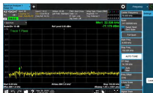
NTNV-n77(3450-3550)-PC2-30-30-L-CP-QPSK-Inner_1RB_Right-0 .009-0.15-PASS
