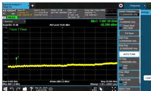
NTNV-n77(3450-3550)-PC2-30-30-H-CP-QPSK-Inner_1RB_Right -6000-20000-PASS
