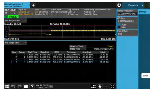
NTNV-n77(3450-3550)-PC2-30-80-L-CP-QPSK-Outer_Full-PASS
