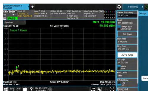
NTNV-n77(3450-3550)-PC2-30-80-M-CP-QPSK-Inner_1RB_Right-0.009-0.15-PASS
