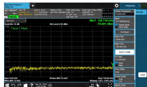
NTNV-n77(3450-3550)-PC2-30-40-M-CP-QPSK-Inner_1RB_Right-0.009-0.15-PASS
