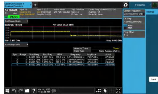
NTNV-n77(3450-3550)-PC2-30-60-H-CP-QPSK-Outer_Full-PASS
