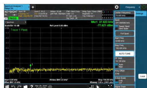
NTNV-n77(3450-3550)-PC2-30-20-M-CP-QPSK-Inner_1RB_Right-0.009-0.15-PASS
