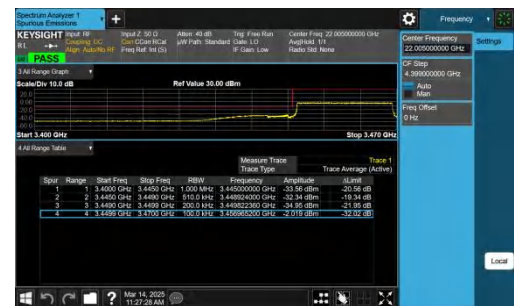
NTNV-n77(3450-3550)-PC2-30-20-L-CP-QPSK-Outer_Full-PASS
