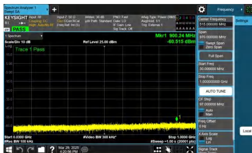
NTNV-n77(3450-3550)-PC2-30-80-L-CP-QPSK-Inner_1RB_Left-3 0-1000-PASS
