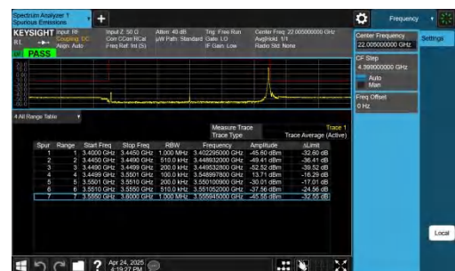
NTNV-n77(3450-3550)-PC2-30-100-L-CP-QPSK-Edge_1RB_Right -PASS
