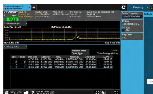
NTNV-n77(3450-3550)-PC2-30-80-H-CP-QPSK-Edge_1RB_Right- PASS
