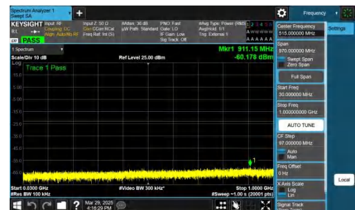
NTNV-n77(3450-3550)-PC2-30-60-H-CP-QPSK-Inner_1RB_Right- 30-1000-PASS
