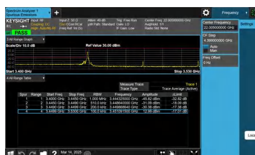
NTNV-n77(3450-3550)-PC2-30-80-L-CP-QPSK-Edge_1RB_Left-PA SS
