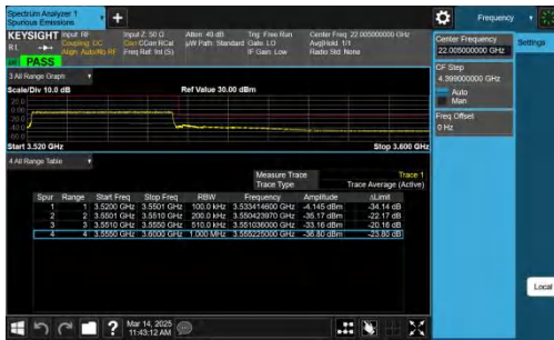
NTNV-n77(3450-3550)-PC2-30-30-H-CP-QPSK-Outer_Full-PASS
