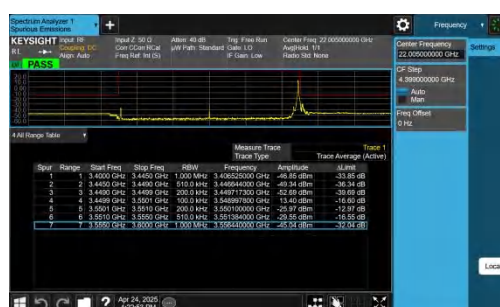
NTNV-n77(3450-3550)-PC2-30-100-L-CP-QPSK-Edge_1RB_Right-PASS
