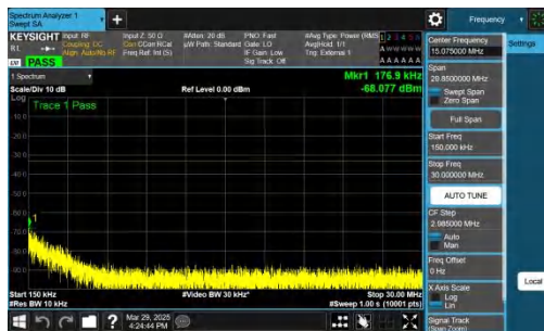
NTNV-n77(3450-3550)-PC2-30-80-L-CP-QPSK-Inner_1RB_Right- 0.15-30-PASS
