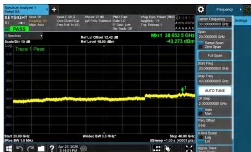
NTNV-n77(3450-3550)-PC2-30-20-H-CP-QPSK-Inner_1RB_Left-2 0000-40000-PASS
