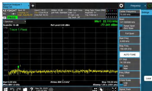
NTNV-n77(3450-3550)-PC2-30-60-L-CP-QPSK-Inner_1RB_Left-0.009-0.15-PASS
