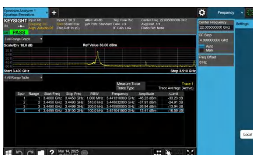
NTNV-n77(3450-3550)-PC2-30-60-L-CP-QPSK-Edge_1RB_Left-P ASS
