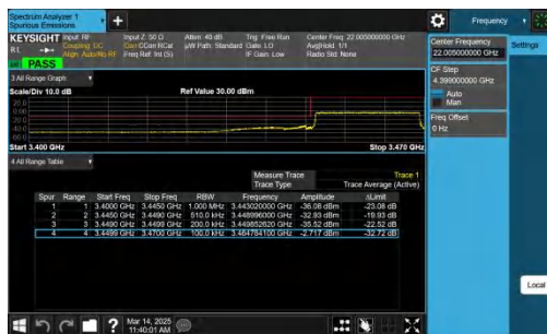
NTNV-n77(3450-3550)-PC2-30-20-L-CP-QPSK-Outer_Full-PASS
