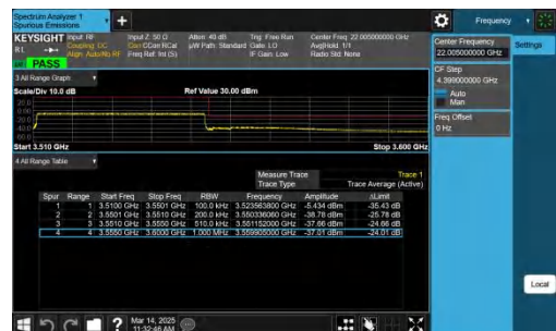
NTNV-n77(3450-3550)-PC2-30-40-H-CP-QPSK-Outer_Full-PASS
