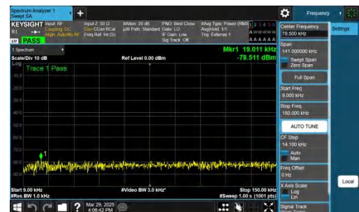
NTNV-n77(3450-3550)-PC2-30-60-M-CP-QPSK-Inner_1RB_Right-0.009-0.15-PASS
