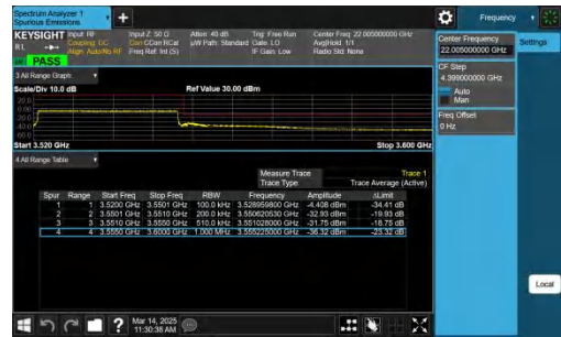
NTNV-n77(3450-3550)-PC2-30-30-H-CP-QPSK-Outer_Full-PASS
