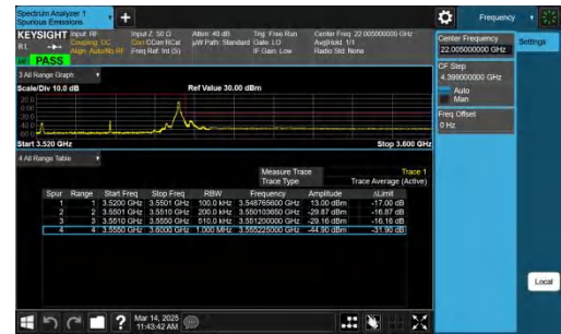
NTNV-n77(3450-3550)-PC2-30-30-H-CP-QPSK-Edge_1RB_Right-PASS
