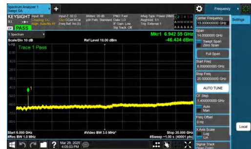
NTNV-n77(3450-3550)-PC2-30-60-M-CP-QPSK-Inner_1RB_Left-6000-20000-PASS
