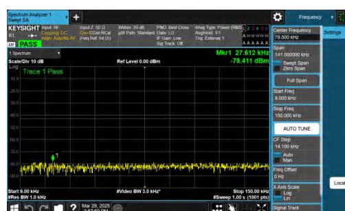
NTNV-n77(3450-3550)-PC2-30-60-L-CP-QPSK-Inner_1RB_Right-0.009-0.15-PASS
