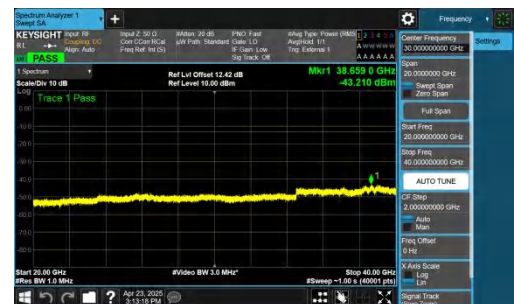
NTNV-n77(3450-3550)-PC2-30-20-M-CP-QPSK-Inner_1RB_Right- 20000-40000-PASS
