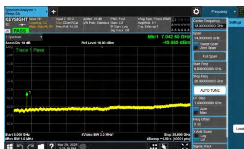
NTNV-n77(3450-3550)-PC2-30-30-H-CP-QPSK-Inner_1RB_Left-6000-20000-PASS
