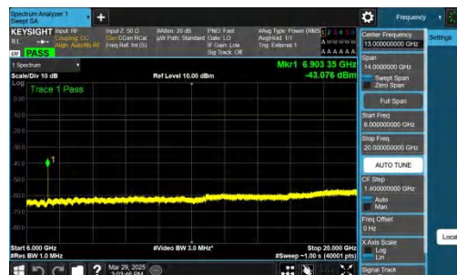
NTNV-n77(3450-3550)-PC2-30-30-L-CP-QPSK-Inner_1RB_Left-60 00-20000-PASS
