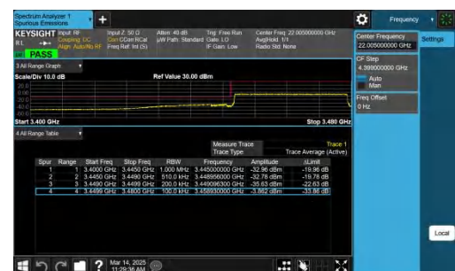
NTNV-n77(3450-3550)-PC2-30-30-L-CP-QPSK-Outer_Full-PASS
