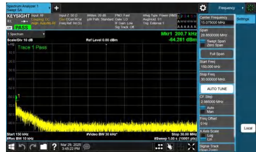
NTNV-n77(3450-3550)-PC2-30-40-H-CP-QPSK-Inner_1RB_Left-0. 15-30-PASS
