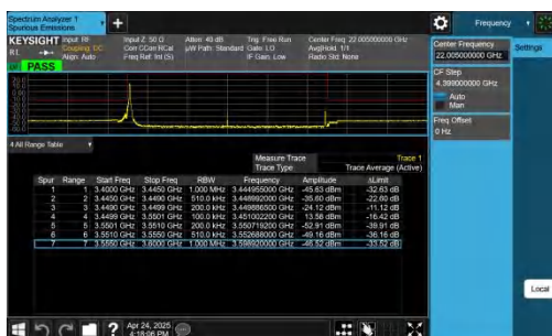
NTNV-n77(3450-3550)-PC2-30-100-L-CP-QPSK-Edge_1RB_Left- PASS
