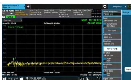
NTNV-n77(3450-3550)-PC2-30-80-H-CP-QPSK-Inner_1RB_Left-0 .009-0.15-PASS
