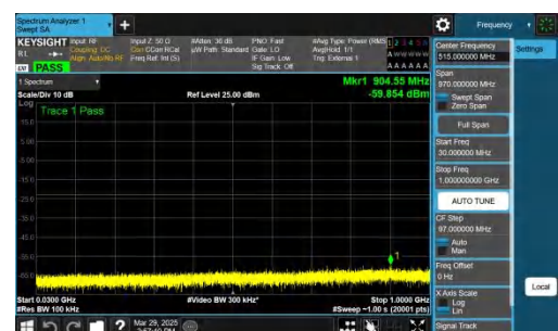
NTNV-n77(3450-3550)-PC2-30-20-H-CP-QPSK-Inner_1RB_Right- 30-1000-PASS
