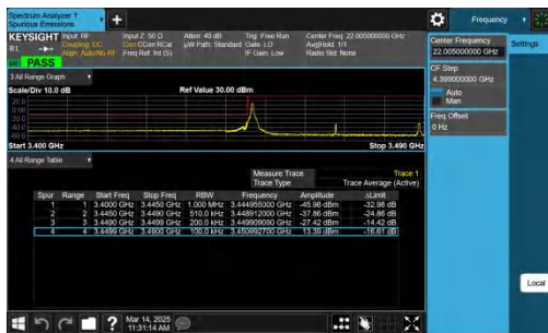
NTNV-n77(3450-3550)-PC2-30-40-L-CP-QPSK-Edge_1RB_Left-P ASS
