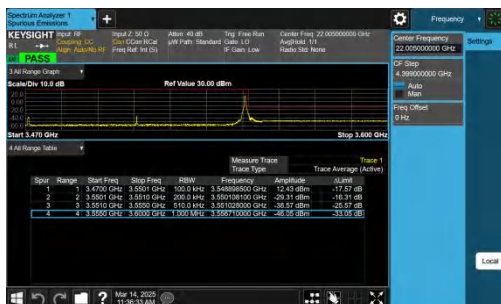
NTNV-n77(3450-3550)-PC2-30-80-H-CP-QPSK-Edge_1RB_Right -PASS
