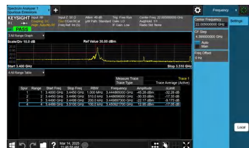
NTNV-n77(3450-3550)-PC2-30-60-L-CP-QPSK-Edge_1RB_Left-PA SS
