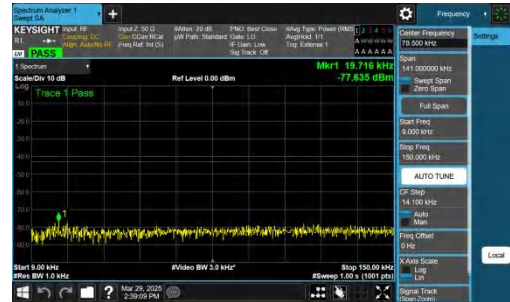
NTNV-n77(3450-3550)-PC2-30-20-L-CP-QPSK-Inner_1RB_Right-0 .009-0.15-PASS
