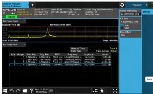
NTNV-n77(3450-3550)-PC2-30-30-H-CP-QPSK-Edge_1RB_Right -PASS
