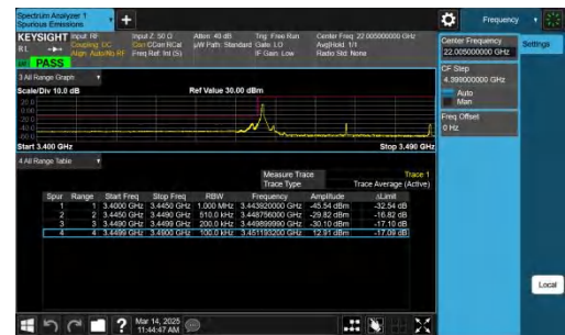
NTNV-n77(3450-3550)-PC2-30-40-L-CP-QPSK-Edge_1RB_Left-PA SS
