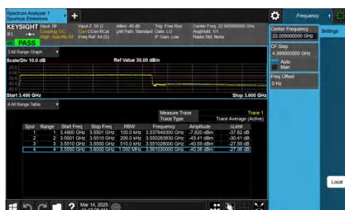
NTNV-n77(3450-3550)-PC2-30-60-H-CP-QPSK-Outer Full-PASS
