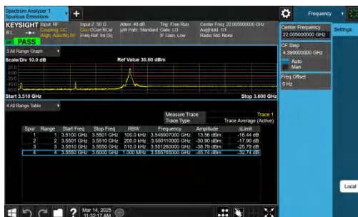
NTNV-n77(3450-3550)-PC2-30-40-H-CP-QPSK-Edge_1RB_Right -PASS
