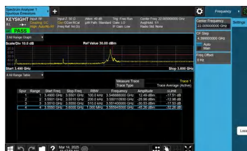
NTNV-n77(3450-3550)-PC2-30-60-H-CP-QPSK-Edge_1RB_Right- PASS
