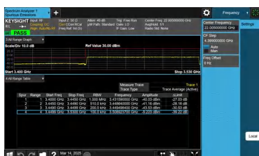
NTNV-n77(3450-3550)-PC2-30-80-L-CP-QPSK-Outer Full-PASS
