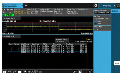
NTNV-n77(3450-3550)-PC2-30-80-H-CP-QPSK-Outer Full-PASS
