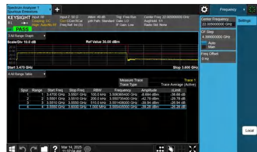
NTNV-n77(3450-3550)-PC2-30-80-H-CP-QPSK-Outer_Full-PASS
