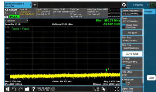
NTNV-n77(3450-3550)-PC2-30-60-L-CP-QPSK-Inner_1RB_Right-3 0-1000-PASS
