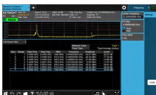
NTNV-n77(3450-3550)-PC2-30-100-L-CP-QPSK-Edge_1RB_Left- PASS
