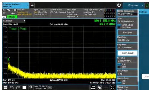
NTNV-n77(3450-3550)-PC2-30-20-L-CP-QPSK-Inner_1RB_Right- 0.15-30-PASS
