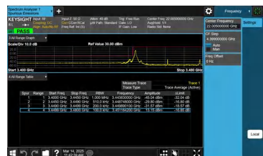
NTNV-n77(3450-3550)-PC2-30-30-L-CP-QPSK-Edge_1RB_Left-PA SS
