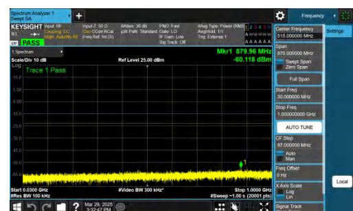
NTNV-n77(3450-3550)-PC2-30-40-L-CP-QPSK-Inner_1RB_Right-3 0-1000-PASS
