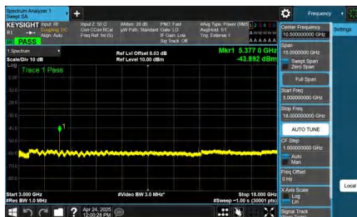
NTNV-n41-PC2-30-20-H-CP-QPSK-Inner_1RB_Right-3000-18000
