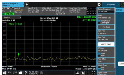
NTNV-n41-PC2-30-70-M-CP-QPSK-Inner_1RB_Left-0.009-0.15-P ASS
