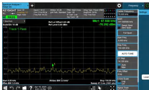
NTNV-n41-PC2-30-100-M-CP-QPSK-Inner_1RB_Right-0.009-0.1 5-PASS
