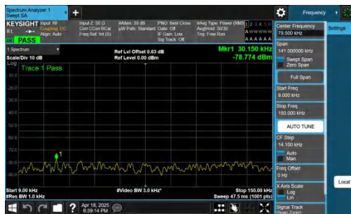
NTNV-n41-PC2-30-80-H-CP-QPSK-Inner_1RB_Left-0.009-0.15-P ASS
