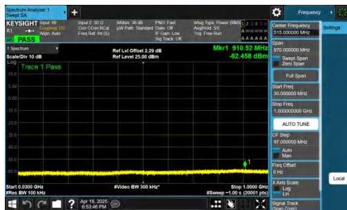
NTNV-n41-PC2-30-100-H-CP-QPSK-Inner_1RB_Right-30-1000-P ASS
