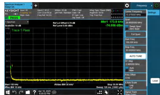
NTNV-n41-PC2-30-80-L-CP-QPSK-Inner_1RB_Left-0.15-30-PASS
