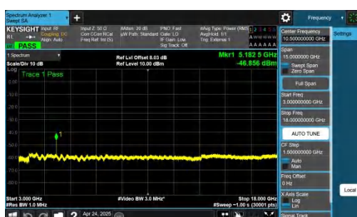
NTNV-n41-PC2-30-100-H-CP-QPSK-Inner_1RB_Left-3000-18000-PASS
