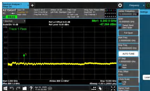
NTNV-n41-PC2-30-70-H-CP-QPSK-Inner_1RB_Left-3000-18000-
