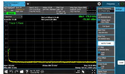
NTNV-n41-PC2-30-90-M-CP-QPSK-Inner_1RB_Right-0.15-30-PASS
