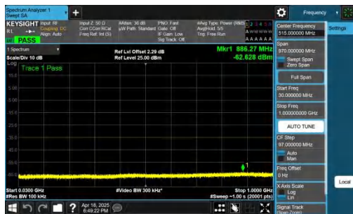
NTNV-n41-PC2-30-100-L-CP-QPSK-Inner_1RB_Right-30-1000-P ASS
