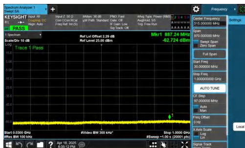
NTNV-n41-PC2-30-80-L-CP-QPSK-Inner_1RB_Left-30-1000-PASS S
