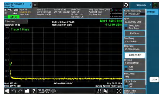
NTNV-n41-PC2-30-80-H-CP-QPSK-Inner_1RB_Right-0.15-30-PASS
