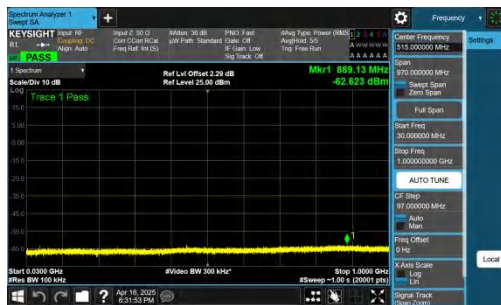
NTNV-n41-PC2-30-70-M-CP-QPSK-Inner_1RB_Right-30-1000-PASS
