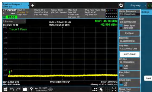
NTNV-n41-PC2-30-30-M-CP-QPSK-Inner_1RB_Right-30-1000-PASS
