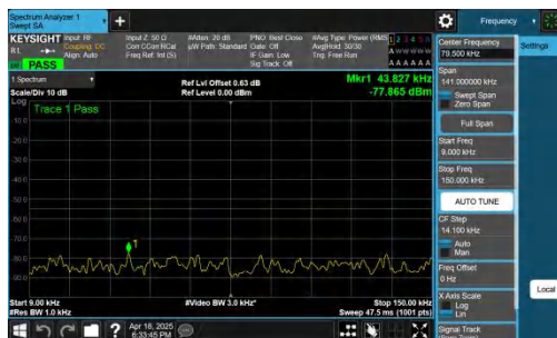
NTNV-n41-PC2-30-70-H-CP-QPSK-Inner_1RB_Right-0.009-0.15-
