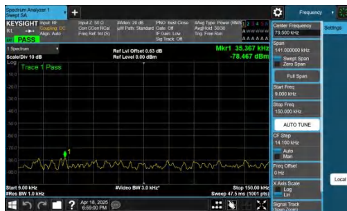
NTNV-n41-PC2-30-20-H-CP-QPSK-Inner_1RB_Left-0.009-0.15-P ASS
