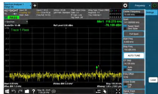
NTNV-n78(3700-3800)-PC2-30-60-M-DFT-BPSK-Inner_1RB_Right t-0.009-0.15-PASS
