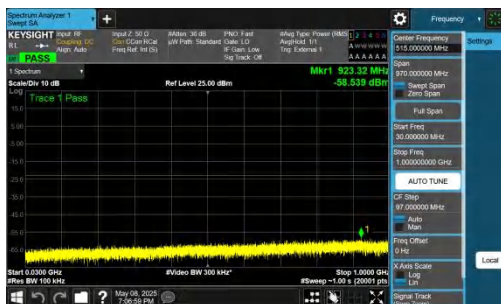
NTNV-n78(3700-3800)-PC2-30-60-M-DFT-QPSK-Inner_1RB_Lef t-30-1000-PASS
