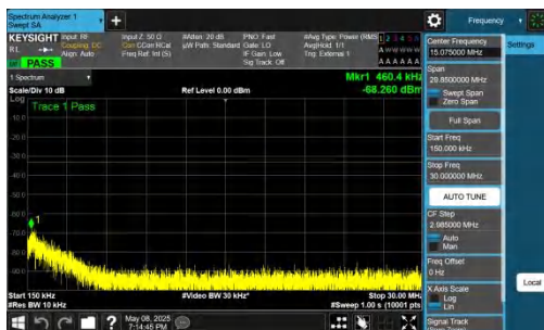
NTNV-n78(3700-3800)-PC2-30-70-L-DFT-BPSK-Inner_1RB_Rig ht-0.15-30-PASS
