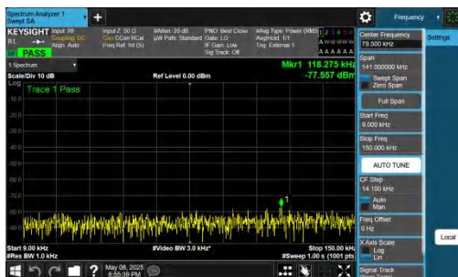
NTNV-n78(3700-3800)-PC2-30-50-H-DFT-BPSK-Inner_1RB_Left -0.009-0.15-PASS
