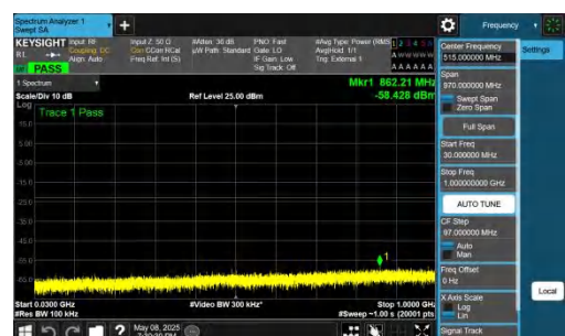
NTNV-n78(3700-3800)-PC2-30-80-L-DFT-QPSK-Inner_1RB_Right -30-1000-PASS
