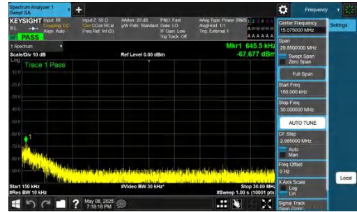
NTNV-n78(3700-3800)-PC2-30-70-M-DFT-BPSK-Inner_1RB_Left 0.15-30-PASS
