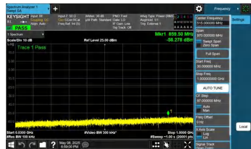
NTNV-n78(3700-3800)-PC2-30-50-H-DFT-QPSK-Inner_1RB_Right t-30-1000-PASS
