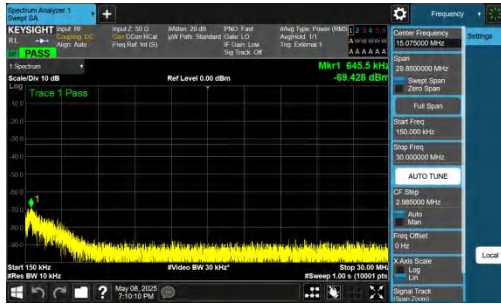
NTNV-n78(3700-3800)-PC2-30-60-H-DFT-BPSK-Inner_1RB_Rig ht-0.15-30-PASS
