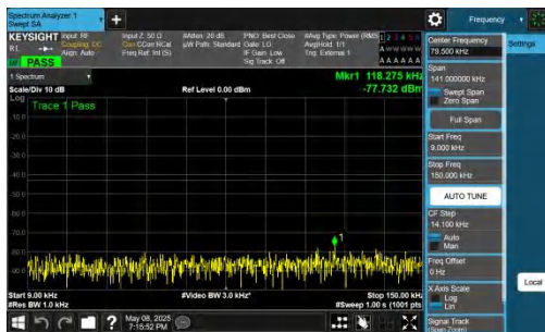
NTNV-n78(3700-3800)-PC2-30-70-L-DFT-QPSK-Inner_1RB_Left -0.009-0.15-PASS
