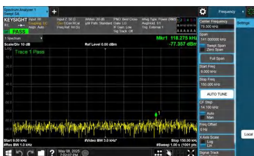
NTNV-n78(3700-3800)-PC2-30-60-L-DFT-QPSK-Inner_1RB_Left -0.009-0.15-PASS
