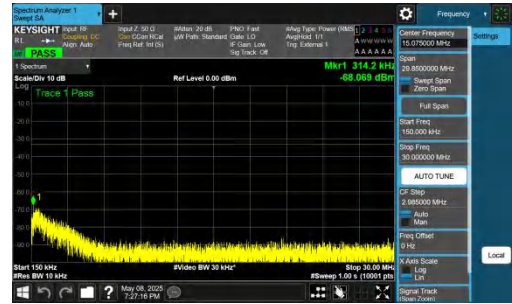
NTNV-n78(3700-3800)-PC2-30-80-L-DFT-BPSK-Inner_1RB_Left- 0.15-30-PASS
