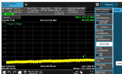
NTNV-n78(3700-3800)-PC2-30-50-H-DFT-QPSK-Inner_1RB_Left -30-1000-PASS
