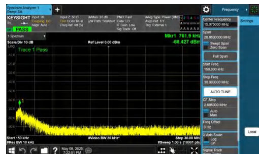
NTNV-n78(3700-3800)-PC2-30-70-H-DFT-BPSK-Inner_1RB_Left 0.15-30-PASS
