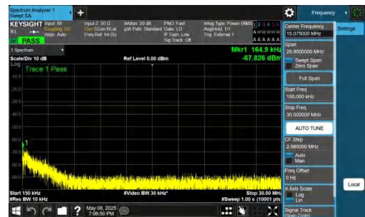
NTNV-n78(3700-3800)-PC2-30-60-M-DFT-QPSK-Inner_1RB_Left- 0.15-30-PASS
