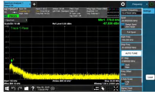
NTNV-n78(3700-3800)-PC2-30-60-H-DFT-BPSK-Inner_1RB_Left 0.15-30-PASS
