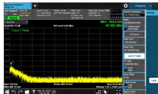
NTNV-n78(3700-3800)-PC2-30-60-M-DFT-BPSK-Inner_1RB_Left- 0.15-30-PASS
