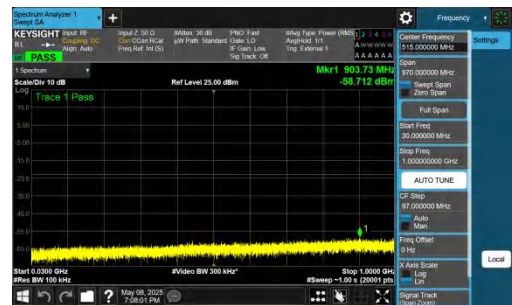
NTNV-n78(3700-3800)-PC2-30-60-M-DFT-QPSK-Inner_1RB_Righ t-30-1000-PASS
