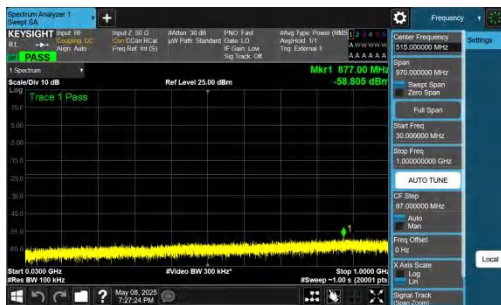
NTNV-n78(3700-3800)-PC2-30-80-L-DFT-BPSK-Inner_1RB_Left- 30-1000-PASS
