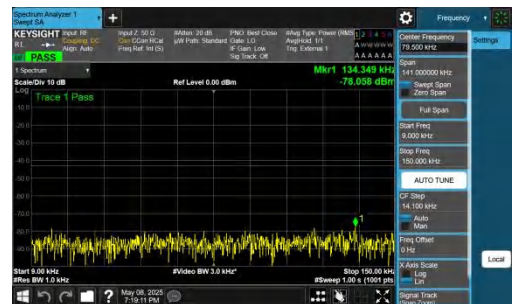
NTNV-n78(3700-3800)-PC2-30-70-M-DFT-BPSK-Inner_1RB_Right t-0.009-0.15-PASS
