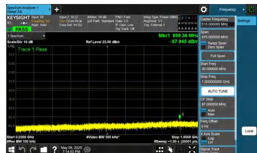
NTNV-n78(3700-3800)-PC2-30-70-L-DFT-BPSK-Inner_1RB_Right-30-1000-PASS
