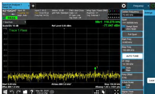
NTNV-n78(3700-3800)-PC2-30-80-M-DFT-BPSK-Inner_1RB_Left -0.009-0.15-PASS
