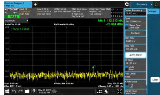
NTNV-n78(3700-3800)-PC2-30-70-L-DFT-QPSK-Inner_1RB_Right -0.009-0.15-PASS
