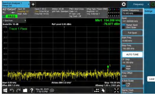
NTNV-n78(3700-3800)-PC2-30-70-M-DFT-BPSK-Inner_1RB_Left -0.009-0.15-PASS
