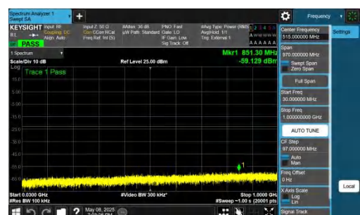
NTNV-n78(3700-3800)-PC2-30-60-L-DFT-QPSK-Inner_1RB_Right -30-1000-PASS
