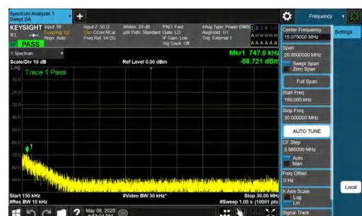
NTNV-n78(3700-3800)-PC2-30-50-M-DFT-QPSK-Inner_1RB_Left- 0.15-30-PASS
