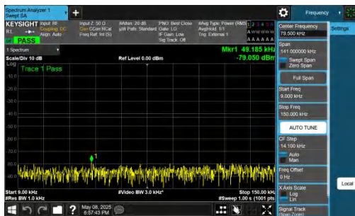
NTNV-n78(3700-3800)-PC2-30-50-H-DFT-QPSK-Inner_1RB_Left -0.009-0.15-PASS
