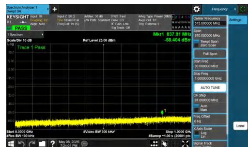
NTNV-n78(3700-3800)-PC2-30-70-H-DFT-BPSK-Inner_1RB_Right t-30-1000-PASS
