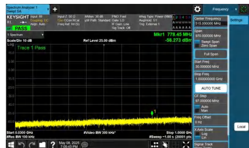
NTNV-n78(3700-3800)-PC2-30-60-M-DFT-BPSK-Inner_1RB_Right t-30-1000-PASS
