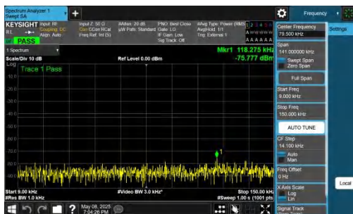
NTNV-n78(3700-3800)-PC2-30-60-M-DFT-BPSK-Inner_1RB_Left -0.009-0.15-PASS
