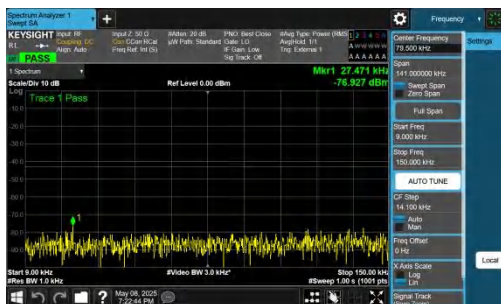
NTNV-n78(3700-3800)-PC2-30-70-H-DFT-BPSK-Inner_1RB_Left -0.009-0.15-PASS
