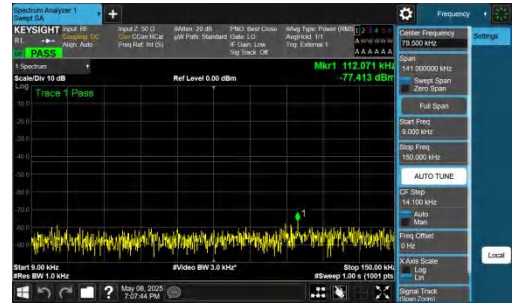
NTNV-n78(3700-3800)-PC2-30-60-M-DFT-QPSK-Inner_1RB_Righ t-0.009-0.15-PASS
