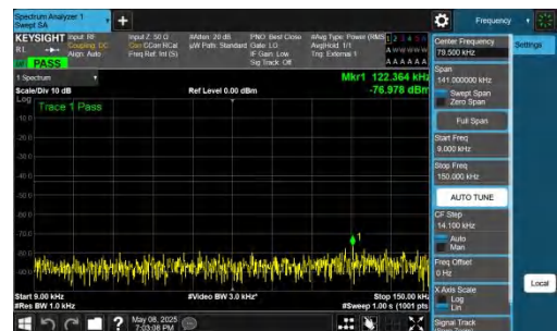
NTNV-n78(3700-3800)-PC2-30-60-L-DFT-QPSK-Inner_1RB_Right -0.009-0.15-PASS
