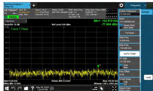
NTNV-n78(3700-3800)-PC2-30-70-H-DFT-BPSK-Inner_1RB_Right t-0.009-0.15-PASS
