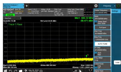
NTNV-n78(3700-3800)-PC2-30-50-M-DFT-QPSK-Inner_1RB_Right t-30-1000-PASS
