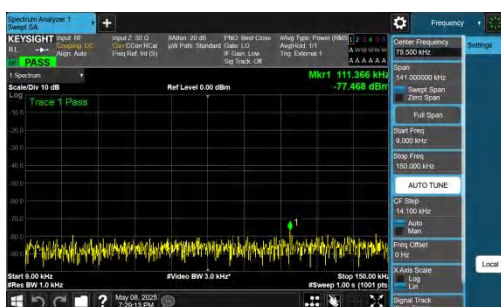
NTNV-n78(3700-3800)-PC2-30-80-L-DFT-QPSK-Inner_1RB_Left -0.009-0.15-PASS
