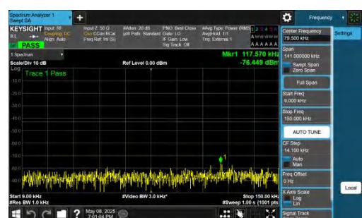
NTNV-n78(3700-3800)-PC2-30-60-L-DFT-BPSK-Inner_1RB_Right-0.009-0.15-PASS
