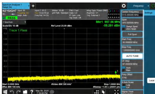
NTNV-n78(3700-3800)-PC2-30-70-L-DFT-QPSK-Inner_1RB_Left -30-1000-PASS
