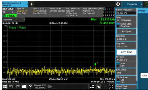
NTNV-n78(3700-3800)-PC2-30-60-L-DFT-BPSK-Inner_1RB_Left-0.009-0.15-PASS
