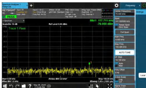
NTNV-n78(3700-3800)-PC2-30-70-L-DFT-BPSK-Inner_1RB_Left- 0.009-0.15-PASS
