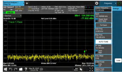
NTNV-n78(3700-3800)-PC2-30-70-H-DFT-QPSK-Inner_1RB_Right t-0.009-0.15-PASS
