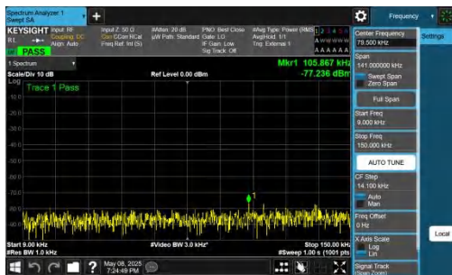
NTNV-n78(3700-3800)-PC2-30-70-H-DFT-QPSK-Inner_1RB_Left -0.009-0.15-PASS
