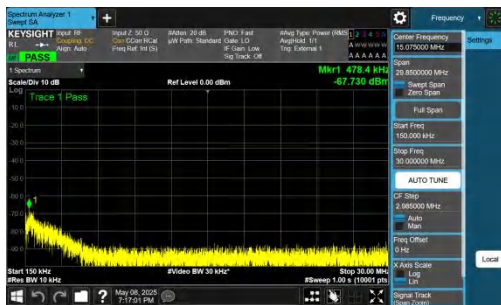
NTNV-n78(3700-3800)-PC2-30-70-L-DFT-QPSK-Inner_1RB_Rig ht-0.15-30-PASS
