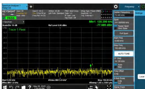
NTNV-n78(3700-3800)-PC2-30-70-M-DFT-QPSK-Inner_1RB_Lef t-0.009-0.15-PASS
