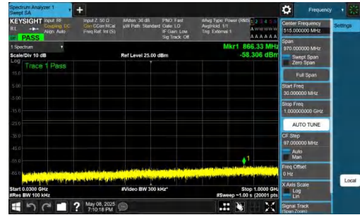
NTNV-n78(3700-3800)-PC2-30-60-H-DFT-BPSK-Inner_1RB_Righ t-30-1000-PASS
