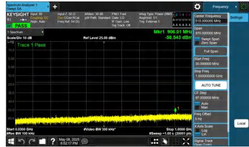
NTNV-n78(3700-3800)-PC2-30-50-M-DFT-BPSK-Inner_1RB_Rig t-30-1000-PASS
