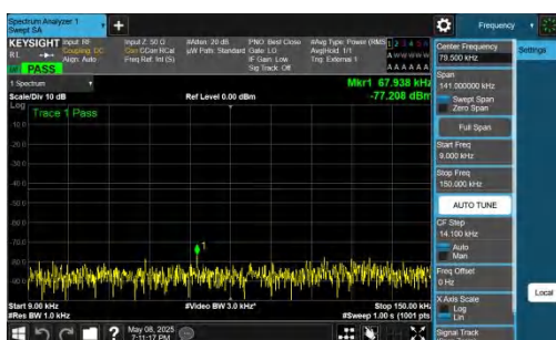
NTNV-n78(3700-3800)-PC2-30-60-H-DFT-QPSK-Inner_1RB_Left -0.009-0.15-PASS
