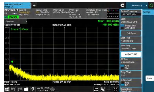
NTNV-n78(3700-3800)-PC2-30-70-H-DFT-QPSK-Inner_1RB_Left- 0.15-30-PASS
