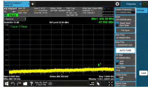
NTNV-n78(3700-3800)-PC2-30-70-M-DFT-BPSK-Inner_1RB_Rig t-30-1000-PASS
