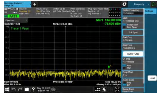
NTNV-n78(3700-3800)-PC2-30-50-H-DFT-QPSK-Inner_1RB_Right t-0.009-0.15-PASS
