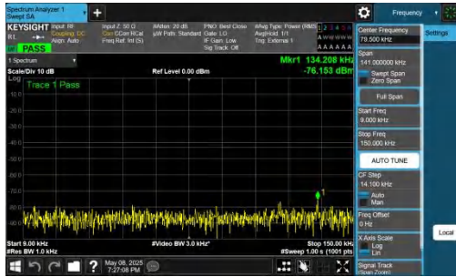
NTNV-n78(3700-3800)-PC2-30-80-L-DFT-BPSK-Inner_1RB_Left- 0.009-0.15-PASS
