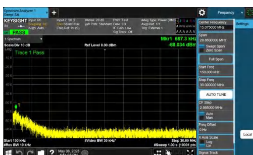
NTNV-n78(3700-3800)-PC2-30-50-M-DFT-QPSK-Inner_1RB_Rig ht-0.15-30-PASS
