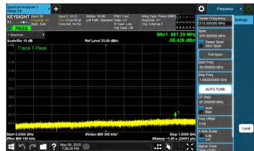
NTNV-n78(3700-3800)-PC2-30-70-H-DFT-QPSK-Inner_1RB_Right t-30-1000-PASS
