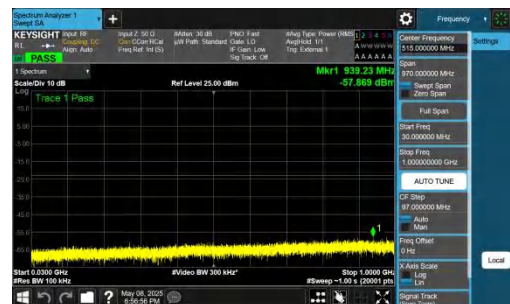
NTNV-n78(3700-3800)-PC2-30-50-H-DFT-BPSK-Inner_1RB_Right t-30-1000-PASS
