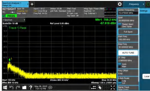
NTNV-n78(3700-3800)-PC2-30-60-L-DFT-BPSK-Inner_1RB_Rig ht-0.15-30-PASS
