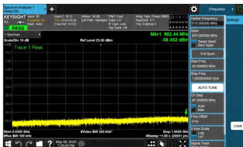
NTNV-n78(3700-3800)-PC2-30-70-H-DFT-QPSK-Inner_1RB_Left -30-1000-PASS
