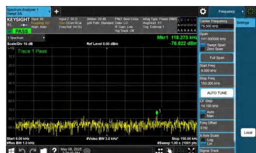
NTNV-n78(3700-3800)-PC2-30-80-L-DFT-BPSK-Inner_1RB_Right -0.009-0.15-PASS
