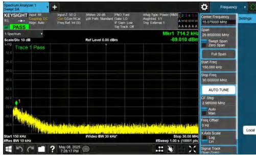
NTNV-n78(3700-3800)-PC2-30-80-L-DFT-BPSK-Inner_1RB_Rig ht-0.15-30-PASS
