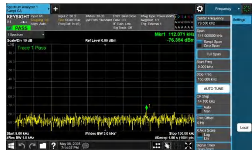
NTNV-n78(3700-3800)-PC2-30-70-L-DFT-BPSK-Inner_1RB_Right-0.009-0.15-PASS
