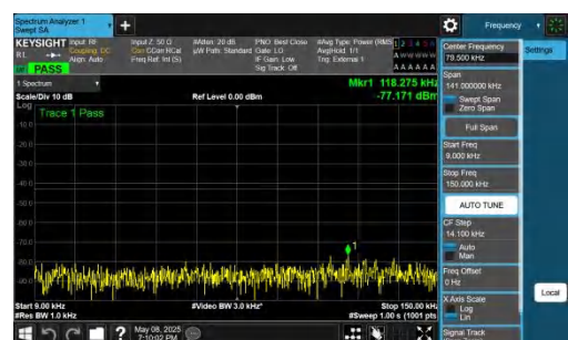
NTNV-n78(3700-3800)-PC2-30-60-H-DFT-BPSK-Inner_1RB_Right t-0.009-0.15-PASS
