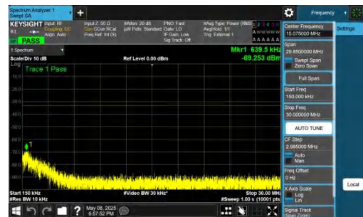
NTNV-n78(3700-3800)-PC2-30-50-H-DFT-QPSK-Inner_1RB_Left- 0.15-30-PASS
