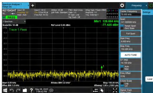
NTNV-n78(3700-3800)-PC2-30-60-M-DFT-QPSK-Inner_1RB_Lef t-0.009-0.15-PASS
