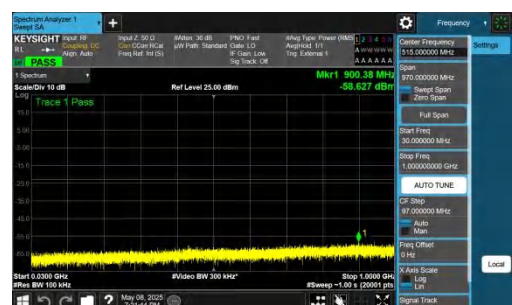
NTNV-n78(3700-3800)-PC2-30-70-M-DFT-QPSK-Inner_1RB_Right t-30-1000-PASS
