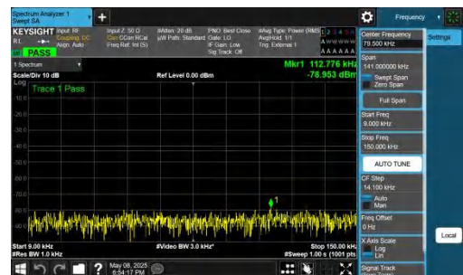
NTNV-n78(3700-3800)-PC2-30-50-M-DFT-QPSK-Inner_1RB_Right t-0.009-0.15-PASS
