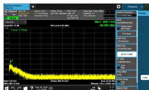
NTNV-n78(3700-3800)-PC2-30-60-H-DFT-QPSK-Inner_1RB_Left 0.15-30-PASS
