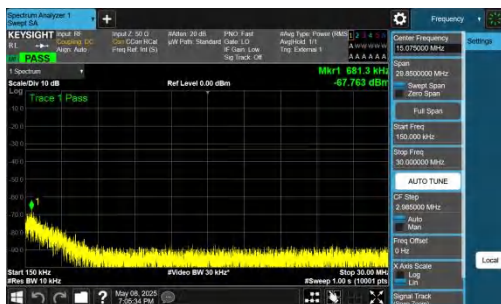
NTNV-n78(3700-3800)-PC2-30-60-M-DFT-BPSK-Inner_1RB_Right ht-0.15-30-PASS
