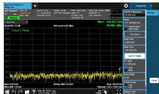
NTNV-n78(3700-3800)-PC2-30-70-M-DFT-QPSK-Inner_1RB_Right t-0.009-0.15-PASS
