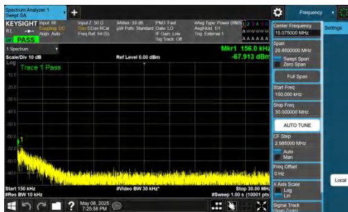
NTNV-n78(3700-3800)-PC2-30-70-H-DFT-QPSK-Inner_1RB_Right ht-0.15-30-PASS
