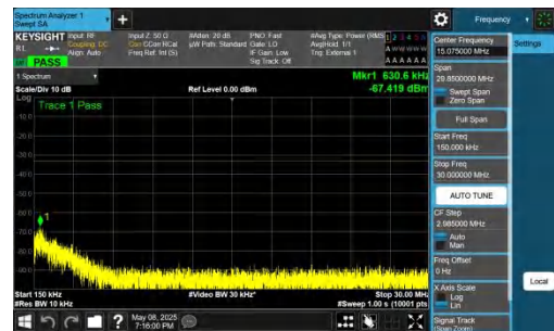
NTNV-n78(3700-3800)-PC2-30-70-L-DFT-QPSK-Inner_1RB_Left- 0.15-30-PASS
