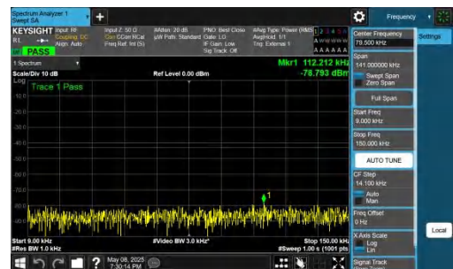
NTNV-n78(3700-3800)-PC2-30-80-L-DFT-QPSK-Inner_1RB_Right -0.009-0.15-PASS
