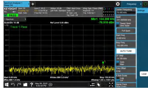
NTNV-n78(3700-3800)-PC2-30-40-M-DFT-QPSK-Inner_1RB_Righ t-0.009-0.15-PASS
