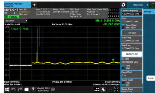
NTVN-n78(3700-3800)-PC2-30-30-M-DFT-QPSK-Inner_1RB_Righ t-3000-6000-PASS
