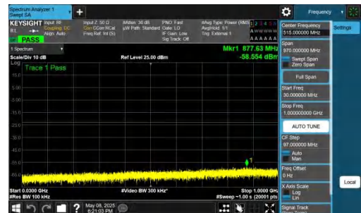
NTNV-n78(3700-3800)-PC2-30-30-L-DFT-BPSK-Inner_1RB_Right -30-1000-PASS
