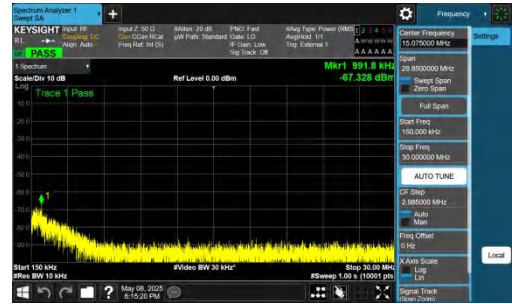
NTNV-n78(3700-3800)-PC2-30-20-H-DFT-BPSK-Inner_1RB_Left 0.15-30-PASS
