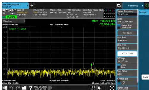
NTNV-n78(3700-3800)-PC2-30-30-L-DFT-BPSK-Inner_1RB_Left- 0.009-0.15-PASS
