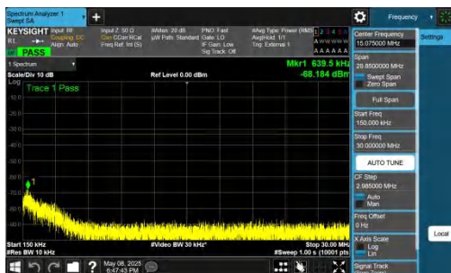
NTNV-n78(3700-3800)-PC2-30-50-L-DFT-BPSK-Inner_1RB_Rig ht-0.15-30-PASS
