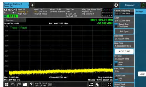
NTNV-n78(3700-3800)-PC2-30-40-M-DFT-QPSK-Inner_1RB_Righ t-30-1000-PASS
