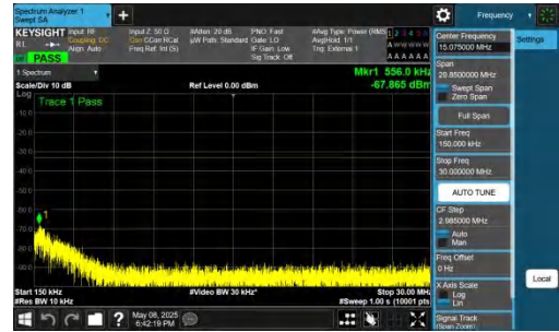
NTNV-n78(3700-3800)-PC2-30-40-H-DFT-BPSK-Inner_1RB_Left 0.15-30-PASS
