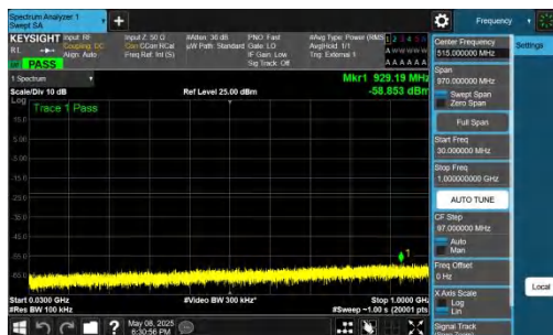
NTNV-n78(3700-3800)-PC2-30-30-H-DFT-QPSK-Inner_1RB_Left -30-1000-PASS
