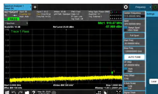
NTNV-n78(3700-3800)-PC2-30-40-L-DFT-QPSK-Inner_1RB_Right -30-1000-PASS
