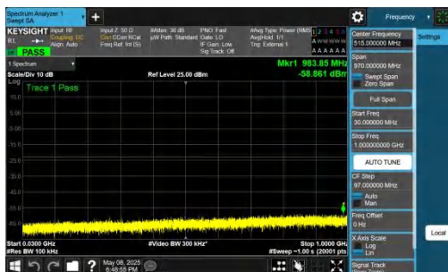
NTNV-n78(3700-3800)-PC2-30-50-L-DFT-QPSK-Inner_1RB_Left -30-1000-PASS
