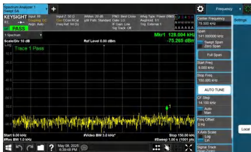
NTNV-n78(3700-3800)-PC2-30-40-M-DFT-QPSK-Inner_1RB_Lef t-0.009-0.15-PASS
