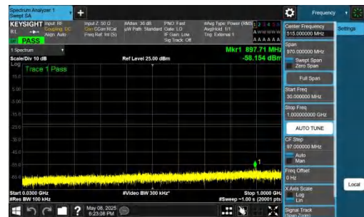
NTNV-n78(3700-3800)-PC2-30-30-L-DFT-QPSK-Inner_1RB_Right -30-1000-PASS
