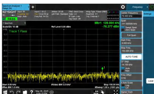
NTNV-n78(3700-3800)-PC2-30-40-H-DFT-QPSK-Inner_1RB_Left -0.009-0.15-PASS
