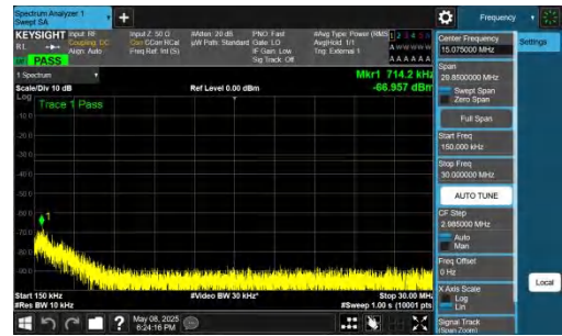
NTVN-n78(3700-3800)-PC2-30-30-M-DFT-BPSK-Inner_1RB_Left 0.15-30-PASS
