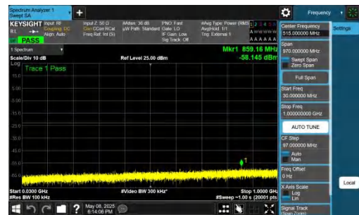
NTNV-n78(3700-3800)-PC2-30-20-M-DFT-QPSK-Inner_1RB_Righ t-30-1000-PASS
