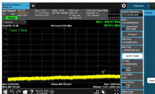
NTNV-n78(3700-3800)-PC2-30-20-M-DFT-QPSK-Inner_1RB_Lef t-30-1000-PASS
