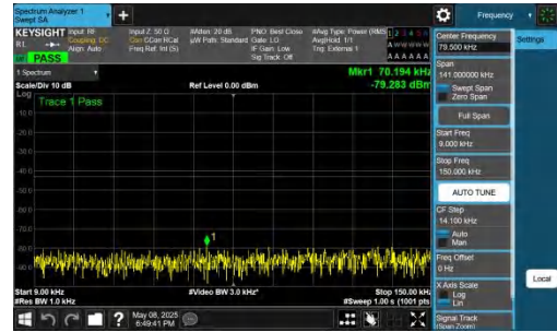
NTNV-n78(3700-3800)-PC2-30-50-L-DFT-QPSK-Inner_1RB_Right -0.009-0.15-PASS
