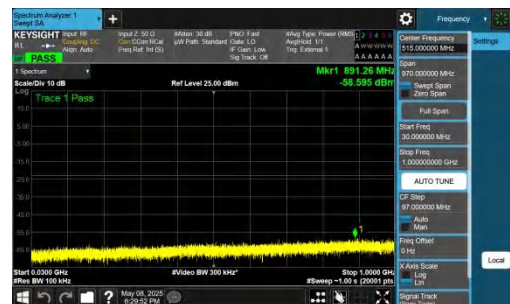
NTNV-n78(3700-3800)-PC2-30-30-H-DFT-BPSK-Inner_1RB_Right t-30-1000-PASS
