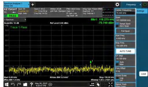
NTNV-n78(3700-3800)-PC2-30-30-L-DFT-BPSK-Inner_1RB_Right -0.009-0.15-PASS
