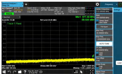
NTNV-n78(3700-3800)-PC2-30-20-H-DFT-BPSK-Inner_1RB_Left -30-1000-PASS
