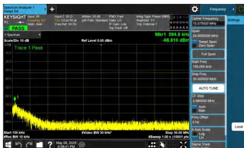
NTNV-n78(3700-3800)-PC2-30-40-M-DFT-BPSK-Inner_1RB_Rig ht-0.15-30-PASS
