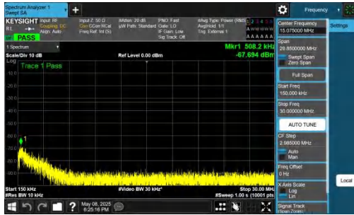
NTNV-n78(3700-3800)-PC2-30-30-M-DFT-BPSK-Inner_1RB_Rig ht-0.15-30-PASS
