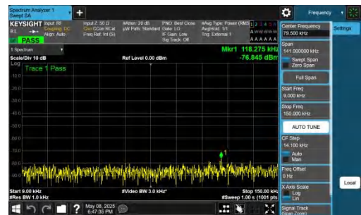
NTNV-n78(3700-3800)-PC2-30-50-L-DFT-BPSK-Inner_1RB_Right -0.009-0.15-PASS
