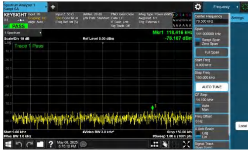
NTNV-n78(3700-3800)-PC2-30-20-H-DFT-BPSK-Inner_1RB_Left -0.009-0.15-PASS
