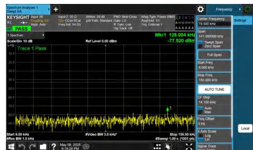
NTNV-n78(3700-3800)-PC2-30-20-H-DFT-QPSK-Inner_1RB_Right t-0.009-0.15-PASS
