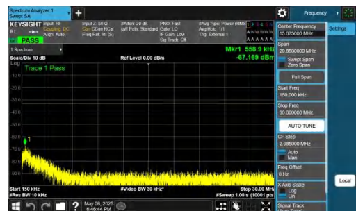
NTNV-n78(3700-3800)-PC2-30-50-L-DFT-BPSK-Inner_1RB_Left- 0.15-30-PASS
