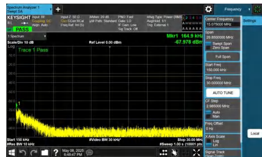
NTNV-n78(3700-3800)-PC2-30-50-L-DFT-QPSK-Inner_1RB_Left- 0.15-30-PASS
