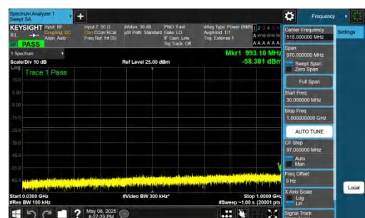
NTNV-n78(3700-3800)-PC2-30-30-M-DFT-QPSK-Inner_1RB_Right t-30-1000-PASS
