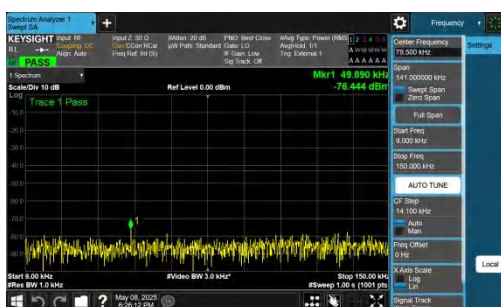
NTNV-n78(3700-3800)-PC2-30-30-M-DFT-QPSK-Inner_1RB_Lef t-0.009-0.15-PASS
