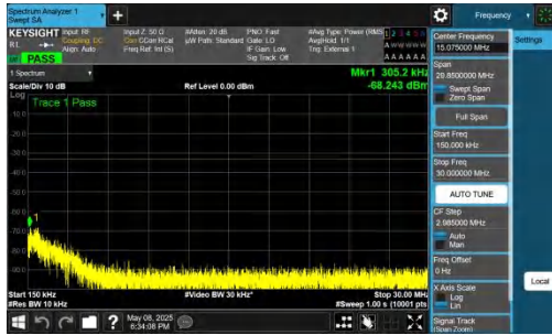
NTNV-n78(3700-3800)-PC2-30-40-L-DFT-BPSK-Inner_1RB_Rig ht-0.15-30-PASS
