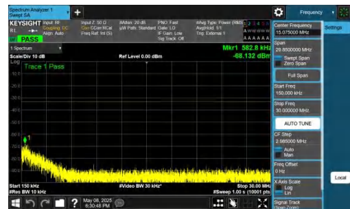
NTNV-n78(3700-3800)-PC2-30-30-H-DFT-QPSK-Inner_1RB_Left- 0.15-30-PASS
