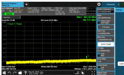
NTNV-n78(3700-3800)-PC2-30-50-M-DFT-BPSK-Inner_1RB_Left -30-1000-PASS
