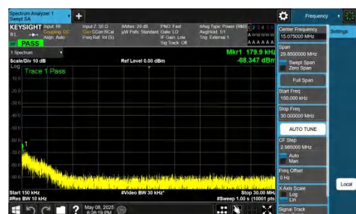
NTNV-n78(3700-3800)-PC2-30-30-M-DFT-QPSK-Inner_1RB_Left- 0.15-30-PASS
