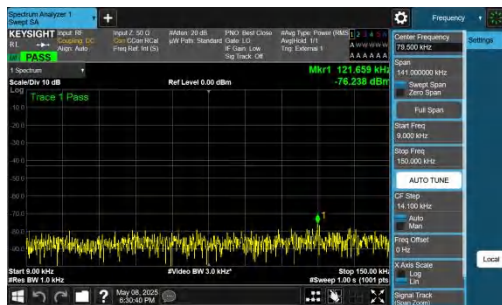
NTNV-n78(3700-3800)-PC2-30-30-H-DFT-QPSK-Inner_1RB_Left -0.009-0.15-PASS
