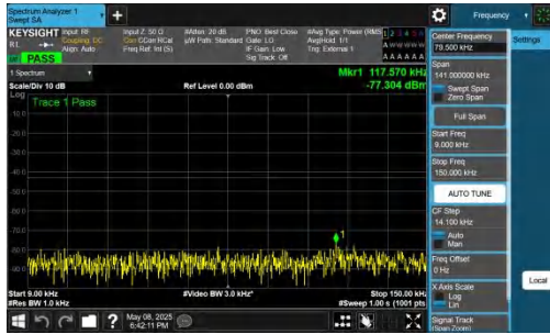
NTNV-n78(3700-3800)-PC2-30-40-H-DFT-BPSK-Inner_1RB_Left -0.009-0.15-PASS
