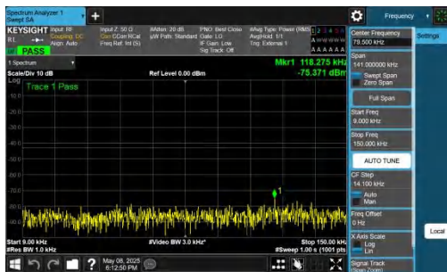
NTNV-n78(3700-3800)-PC2-30-20-M-DFT-QPSK-Inner_1RB_Lef t-0.009-0.15-PASS
