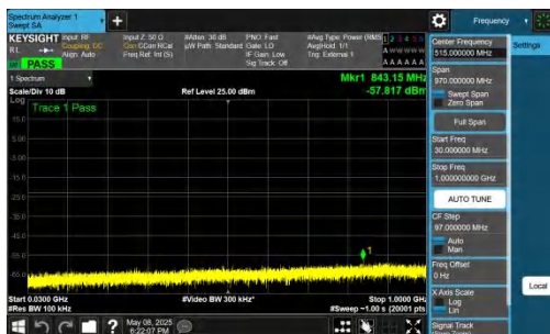
NTNV-n78(3700-3800)-PC2-30-30-L-DFT-QPSK-Inner_1RB_Left -30-1000-PASS
