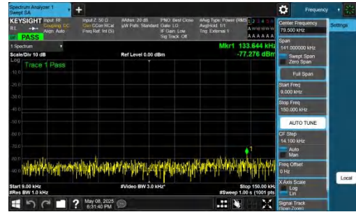
NTNV-n78(3700-3800)-PC2-30-30-H-DFT-QPSK-Inner_1RB_Right t-0.009-0.15-PASS
