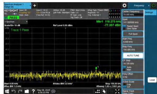
NTNV-n78(3700-3800)-PC2-30-40-M-DFT-BPSK-Inner_1RB_Right t-0.009-0.15-PASS
