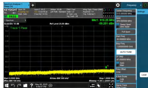
NTNV-n78(3700-3800)-PC2-30-50-L-DFT-QPSK-Inner_1RB_Right -30-1000-PASS
