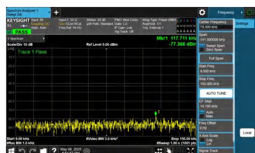
NTNV-n78(3700-3800)-PC2-30-50-M-DFT-BPSK-Inner_1RB_Right t-0.009-0.15-PASS
