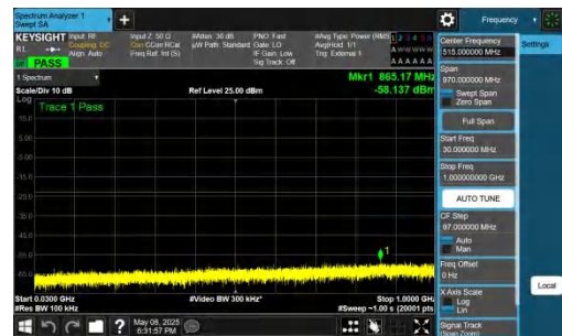
NTNV-n78(3700-3800)-PC2-30-30-H-DFT-QPSK-Inner_1RB_Right t-30-1000-PASS
