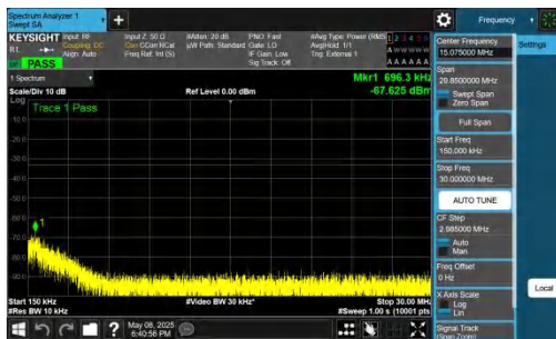
NTNV-n78(3700-3800)-PC2-30-40-M-DFT-QPSK-Inner_1RB_Rig ht-0.15-30-PASS
