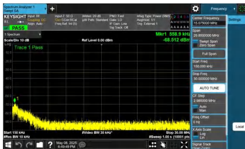
NTNV-n78(3700-3800)-PC2-30-50-L-DFT-QPSK-Inner_1RB_Rig ht-0.15-30-PASS
