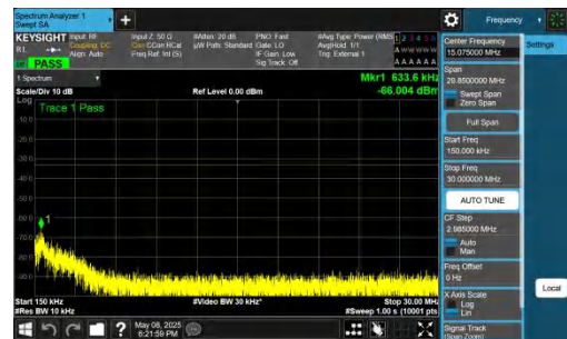
NTNV-n78(3700-3800)-PC2-30-30-L-DFT-QPSK-Inner_1RB_Left- 0.15-30-PASS
