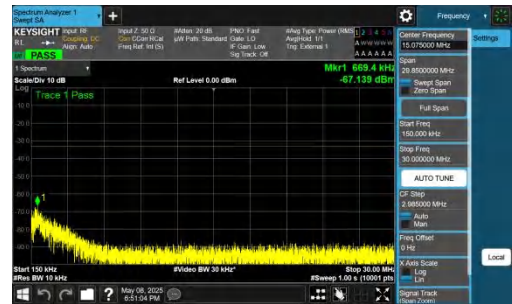
NTNV-n78(3700-3800)-PC2-30-50-M-DFT-BPSK-Inner_1RB_Left 0.15-30-PASS
