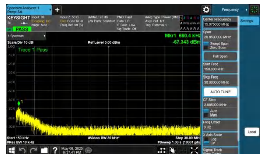
NTNV-n78(3700-3800)-PC2-30-40-M-DFT-BPSK-Inner_1RB_Left 0.15-30-PASS
