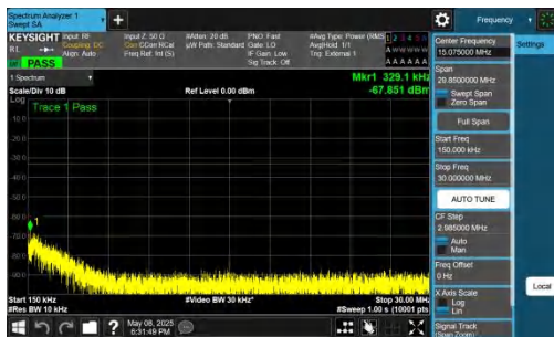
NTNV-n78(3700-3800)-PC2-30-30-H-DFT-QPSK-Inner_1RB_Right ht-0.15-30-PASS
