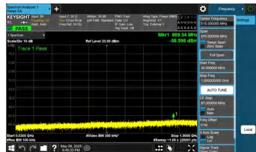
NTNV-n78(3700-3800)-PC2-30-40-H-DFT-QPSK-Inner_1RB_Right t=30-1000-PASS
