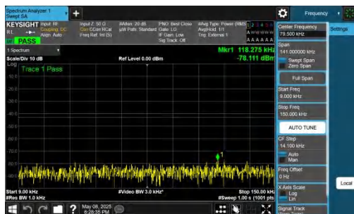
NTVN-n78(3700-3800)-PC2-30-30-H-DFT-BPSK-Inner_1RB_Left -0.009-0.15-PASS
