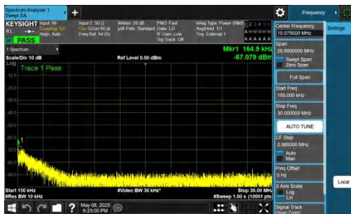
NTNV-n78(3700-3800)-PC2-30-30-L-DFT-QPSK-Inner_1RB_Rig ht-0.15-30-PASS
