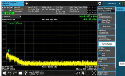
NTNV-n78(3700-3800)-PC2-30-40-H-DFT-BPSK-Inner_1RB_Rig ht-0.15-30-PASS
