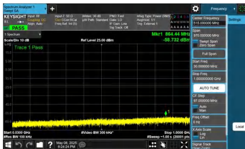
NTVN-n78(3700-3800)-PC2-30-30-M-DFT-BPSK-Inner_1RB_Left -30-1000-PASS
