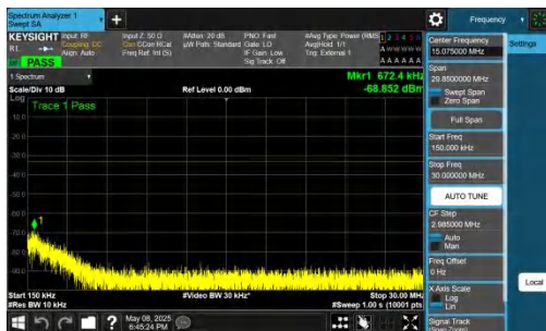
NTNV-n78(3700-3800)-PC2-30-40-H-DFT-QPSK-Inner_1RB_Rig ht=0.15-30-PASS
