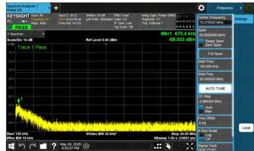
NTNV-n78(3700-3800)-PC2-30-40-L-DFT-BPSK-Inner_1RB_Left-0.15-30-PASS
