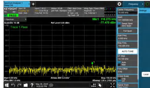
NTNV-n78(3700-3800)-PC2-30-30-L-DFT-QPSK-Inner_1RB_Right -0.009-0.15-PASS
