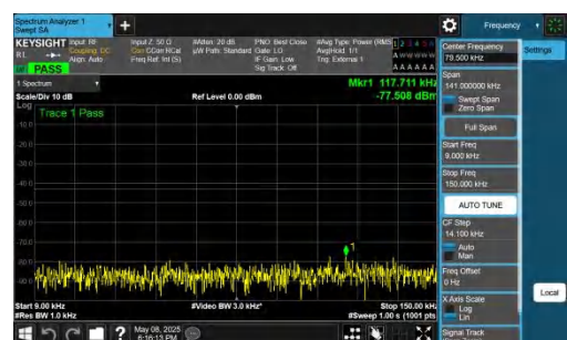
NTNV-n78(3700-3800)-PC2-30-20-H-DFT-BPSK-Inner_1RB_Right t-0.009-0.15-PASS
