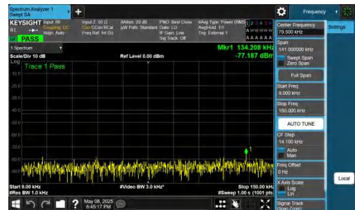
NTNV-n78(3700-3800)-PC2-30-40-H-DFT-QPSK-Inner_1RB_Right t=0.009-0.15-PASS
