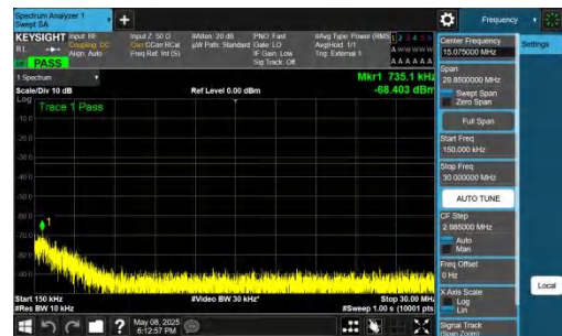
NTNV-n78(3700-3800)-PC2-30-20-M-DFT-QPSK-Inner_1RB_Left- 0.15-30-PASS
