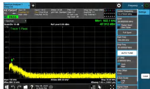
NTNV-n78(3700-3800)-PC2-30-30-L-DFT-BPSK-Inner_1RB_Left- 0.15-30-PASS
