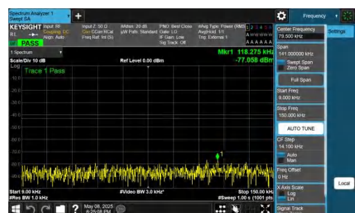
NTVN-n78(3700-3800)-PC2-30-30-M-DFT-BPSK-Inner_1RB_Right t-0.009-0.15-PASS
