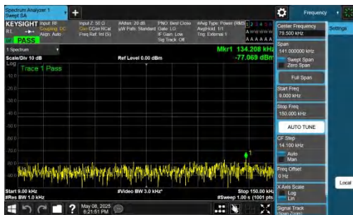
NTNV-n78(3700-3800)-PC2-30-30-L-DFT-QPSK-Inner_1RB_Left -0.009-0.15-PASS
