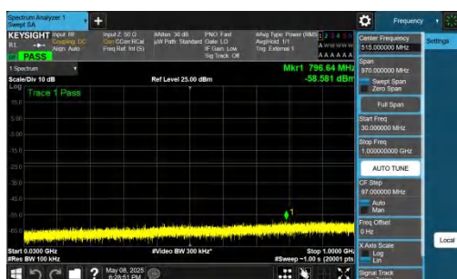
NTVN-n78(3700-3800)-PC2-30-30-H-DFT-BPSK-Inner_1RB_Left -30-1000-PASS
