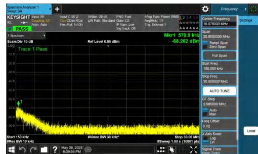
NTNV-n78(3700-3800)-PC2-30-40-M-DFT-QPSK-Inner_1RB_Left- 0.15-30-PASS
