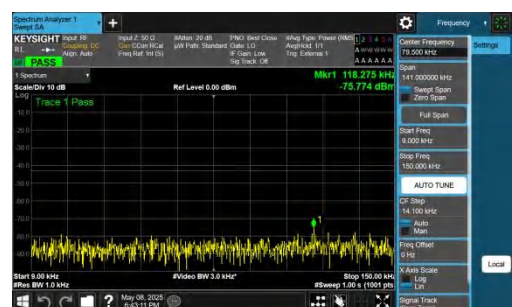
NTNV-n78(3700-3800)-PC2-30-40-H-DFT-BPSK-Inner_1RB_Right t-0.009-0.15-PASS
