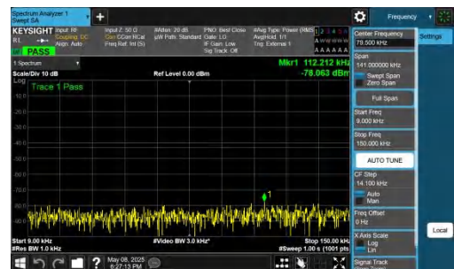
NTNV-n78(3700-3800)-PC2-30-30-M-DFT-QPSK-Inner_1RB_Right t-0.009-0.15-PASS
