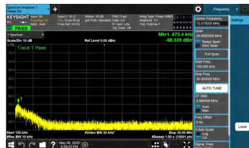
NTVN-n78(3700-3800)-PC2-30-30-H-DFT-BPSK-Inner_1RB_Left- 0.15-30-PASS
