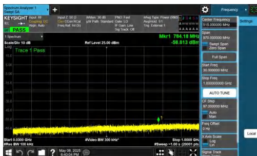
NTNV-n78(3700-3800)-PC2-30-40-M-DFT-QPSK-Inner_1RB_Lef t-30-1000-PASS
