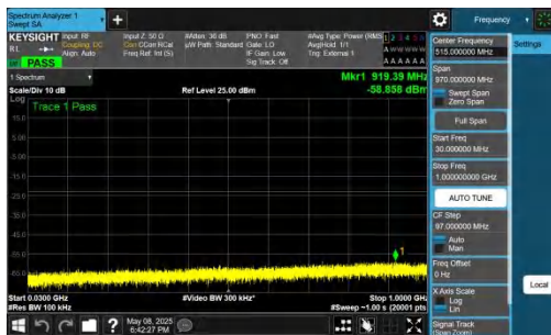
NTNV-n78(3700-3800)-PC2-30-40-H-DFT-BPSK-Inner_1RB_Left -30-1000-PASS
