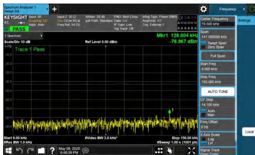
NTNV-n78(3700-3800)-PC2-30-50-L-DFT-QPSK-Inner_1RB_Left -0.009-0.15-PASS
