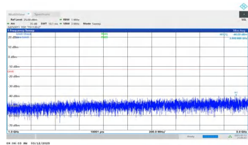
NTNV-n78(3450-3550)-PC2-30-80-H-DFT-BPSK-Inner_1RB_Left 1000-3000-PASS
