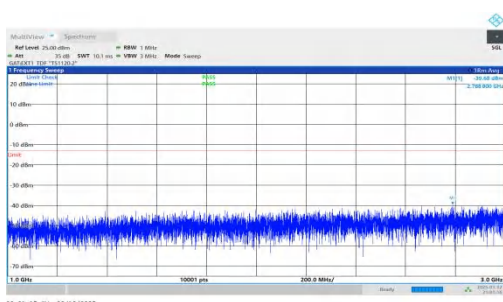
NTNV-n78(3450-3550)-PC2-30-80-M-DFT-BPSK-Inner_1RB_Rig ht-1000-3000-PASS
