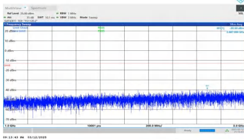
NTNV-n78(3450-3550)-PC2-30-90-L-DFT-BPSK-Inner_1RB_Rig ht-1000-3000-PASS
