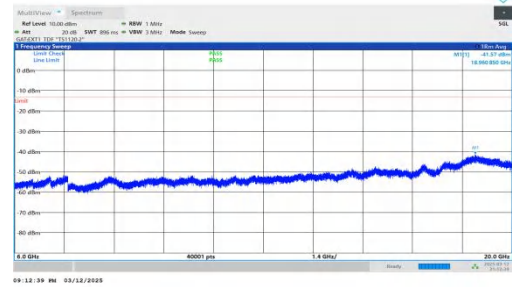
NTNV-n78(3450-3550)-PC2-30-90-L-DFT-BPSK-Inner_1RB_Left-6000-20000-PASS
