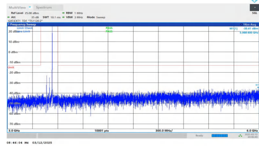
NTNV-n78(3450-3550)-PC2-30-70-M-DFT-QPSK-Inner_1RB_Righ t-3000-6000-PASS
