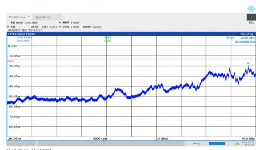
NTNV-n78(3450-3550)-PC2-30-90-L-DFT-QPSK-Inner_1RB_Right -20000-40000-PASS
