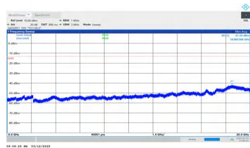
NTNV-n78(3450-3550)-PC2-30-80-H-DFT-BPSK-Inner_1RB_Left 6000-20000-PASS
