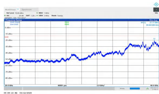
NTNV-n78(3450-3550)-PC2-30-80-H-DFT-BPSK-Inner_1RB_Righ t-20000-40000-PASS
