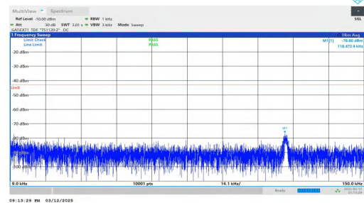
NTNV-n78(3450-3550)-PC2-30-90-L-DFT-BPSK-Inner_1RB_Right-0.009-0.15-PASS
