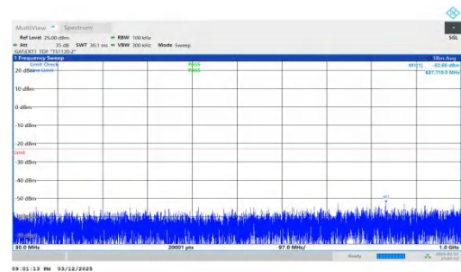
NTNV-n78(3450-3550)-PC2-30-80-M-DFT-BPSK-Inner_1RB_Right t-30-1000-PASS
