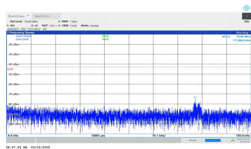
NTNV-n78(3450-3550)-PC2-30-80-L-DFT-QPSK-Inner_1RB_Right -0.009-0.15-PASS
