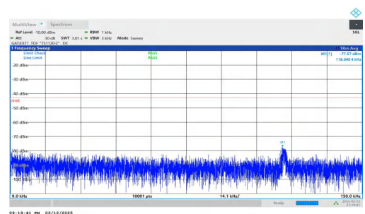
NTNV-n78(3450-3550)-PC2-30-90-M-DFT-BPSK-Inner_1RB_Right t-0.009-0.15-PASS
