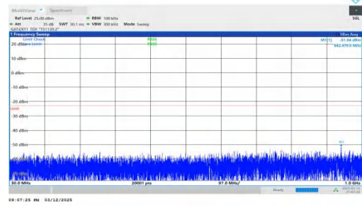
NTNV-n78(3450-3550)-PC2-30-80-H-DFT-BPSK-Inner_1RB_Righ t-30-1000-PASS
