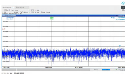
NTNV-n78(3450-3550)-PC2-30-80-M-DFT-QPSK-Inner_1RB_Rig ht-0.15-30-PASS
