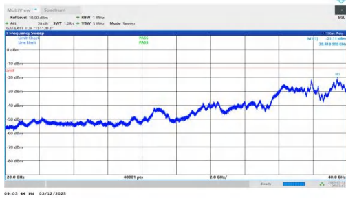
NTNV-n78(3450-3550)-PC2-30-80-M-DFT-QPSK-Inner_1RB_Lef t-20000-40000-PASS
