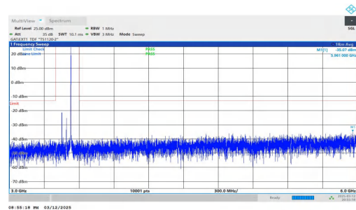
NTNV-n78(3450-3550)-PC2-30-80-L-DFT-BPSK-Inner_1RB_Right -3000-6000-PASS
