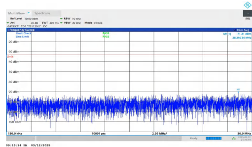
NTNV-n78(3450-3550)-PC2-30-90-L-DFT-QPSK-Inner_1RB_Left- 0.15-30-PASS
