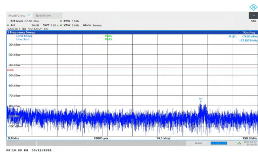
NTNV-n78(3450-3550)-PC2-30-80-H-DFT-QPSK-Inner_1RB_Right t=0.009-0.15-PASS
