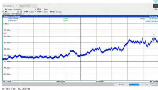
NTNV-n78(3450-3550)-PC2-30-80-L-DFT-BPSK-Inner_1RB_Left- 20000-40000-PASS
