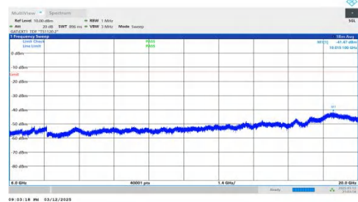
NTNV-n78(3450-3550)-PC2-30-80-M-DFT-QPSK-Inner_1RB_Left- 6000-20000-PASS
