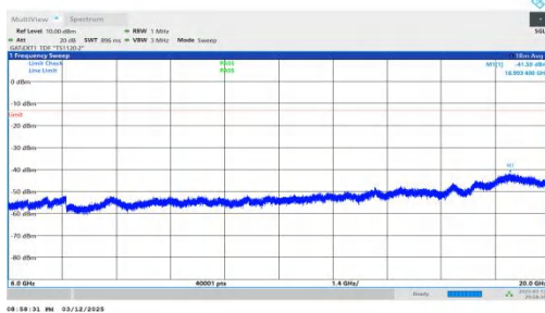
NTNV-n78(3450-3550)-PC2-30-80-L-DFT-QPSK-Inner_1RB_Rig ht-6000-20000-PASS
