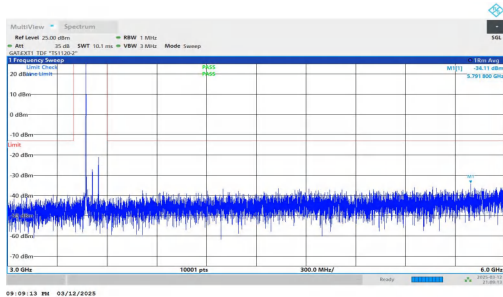
NTNV-n78(3450-3550)-PC2-30-80-H-DFT-QPSK-Inner_1RB_Left -3000-6000-PASS
