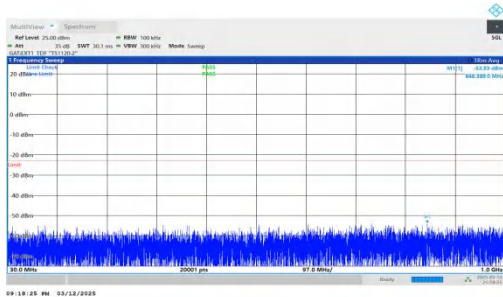
NTNV-n78(3450-3550)-PC2-30-90-M-DFT-BPSK-Inner_1RB_Left -30-1000-PASS
