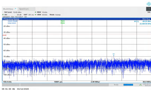
NTNV-n78(3450-3550)-PC2-30-70-H-DFT-QPSK-Inner_1RB_Right ht.0.15-30-PASS
