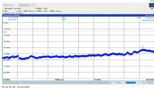
NTNV-n78(3450-3550)-PC2-30-80-M-DFT-QPSK-Inner_1RB_Rig ht-6000-20000-PASS
