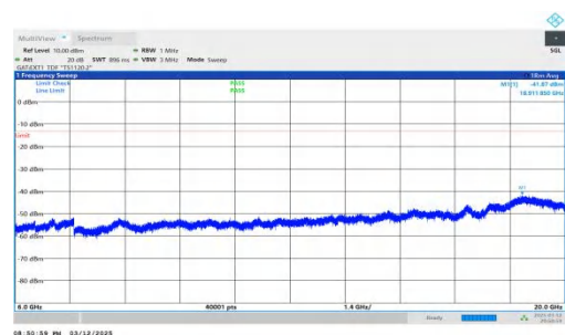
NTNV-n78(3450-3550)-PC2-30-70-H-DFT-QPSK-Inner_1RB_Left- 6000-20000-PASS
