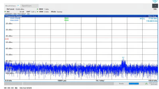
NTNV-n78(3450-3550)-PC2-30-80-L-DFT-BPSK-Inner_1RB_Right -0.009-0.15-PASS
