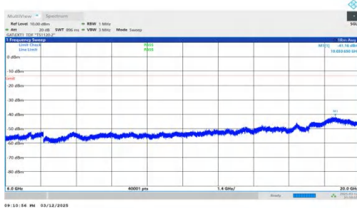
NTNV-n78(3450-3550)-PC2-30-80-H-DFT-QPSK-Inner_1RB_Rig ht-6000-20000-PASS
