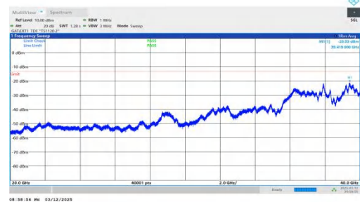
NTNV-n78(3450-3550)-PC2-30-80-L-DFT-QPSK-Inner_1RB_Right -20000-40000-PASS
