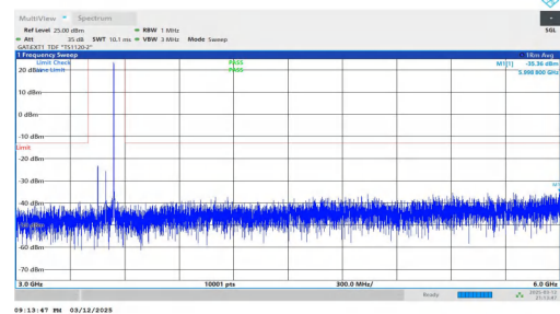
NTNV-n78(3450-3550)-PC2-30-90-L-DFT-BPSK-Inner_1RB_Right-3000-6000-PASS
