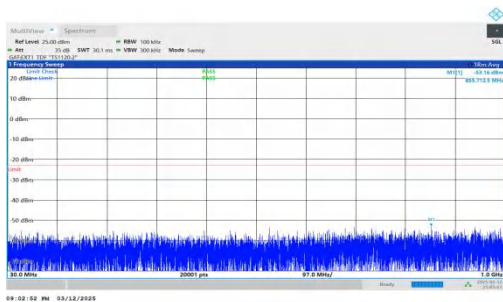
NTNV-n78(3450-3550)-PC2-30-80-M-DFT-QPSK-Inner_1RB_Lef t-30-1000-PASS
