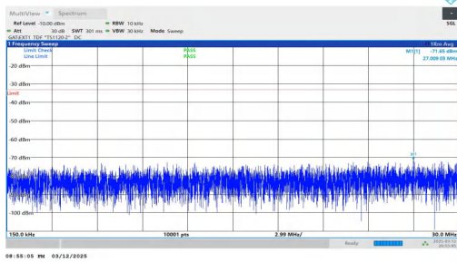
NTNV-n78(3450-3550)-PC2-30-80-L-DFT-BPSK-Inner_1RB_Rig ht-0.15-30-PASS
