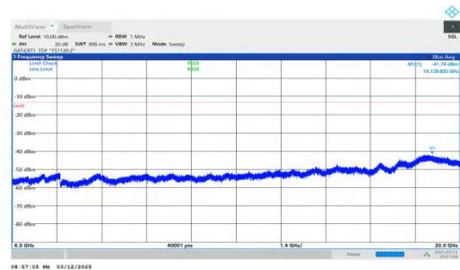
NTNV-n78(3450-3550)-PC2-30-80-L-DFT-QPSK-Inner_1RB_Left- 6000-20000-PASS
