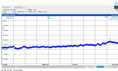
NTNV-n78(3450-3550)-PC2-30-80-L-DFT-BPSK-Inner_1RB_Rig ht-6000-20000-PASS
