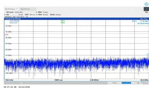
NTNV-n78(3450-3550)-PC2-30-70-H-DFT-BPSK-Inner_1RB_Left- 0.15-30-PASS
