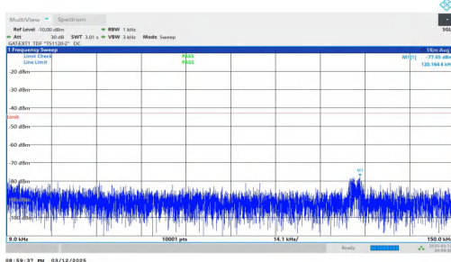
NTNV-n78(3450-3550)-PC2-30-80-M-DFT-BPSK-Inner_1RB_Left -0.009-0.15-PASS
