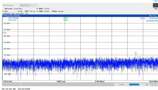
NTNV-n78(3450-3550)-PC2-30-80-H-DFT-QPSK-Inner_1RB_Rig ht=0.15-30-PASS
