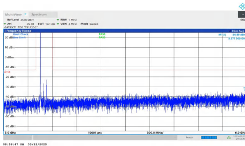
NTNV-n78(3450-3550)-PC2-30-80-L-DFT-QPSK-Inner_1RB_Left -3000-6000-PASS
