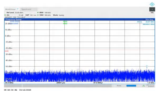
NTNV-n78(3450-3550)-PC2-30-70-H-DFT-BPSK-Inner_1RB_Right t-30-1000-PASS
