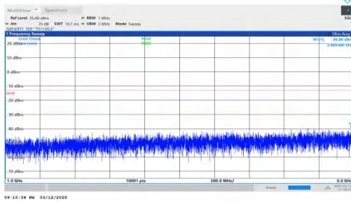
NTNV-n78(3450-3550)-PC2-30-80-H-DFT-QPSK-Inner_1RB_Rig ht-1000-3000-PASS
