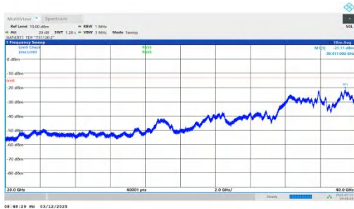
NTNV-n78(3450-3550)-PC2-30-70-H-DFT-BPSK-Inner_1RB_Left -20000-40000-PASS
