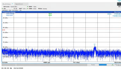
NTNV-n78(3450-3550)-PC2-30-80-H-DFT-QPSK-Inner_1RB_Left -0.009-0.15-PASS
