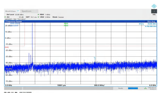
NTNV-n78(3450-3550)-PC2-30-70-H-DFT-BPSK-Inner_1RB_Right t-3000-6000-PASS
