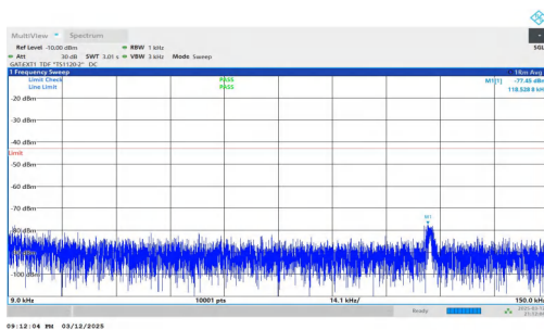
NTNV-n78(3450-3550)-PC2-30-90-L-DFT-BPSK-Inner_1RB_Left- 0.009-0.15-PASS
