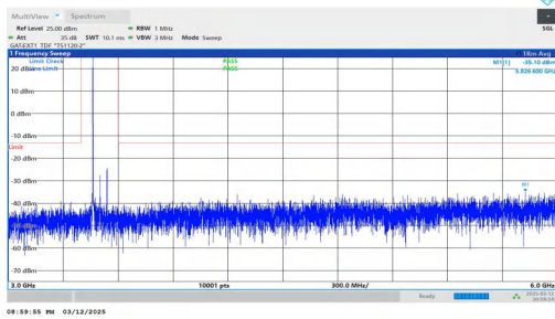
NTNV-n78(3450-3550)-PC2-30-80-M-DFT-BPSK-Inner_1RB_Left -3000-6000-PASS
