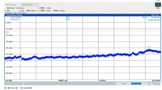
NTNV-n78(3450-3550)-PC2-30-70-H-DFT-BPSK-Inner_1RB_Left 6000-20000-PASS
