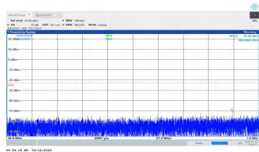
NTNV-n78(3450-3550)-PC2-30-80-M-DFT-QPSK-Inner_1RB_Righ t-30-1000-PASS
