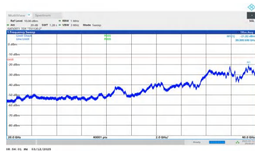
NTNV-n78(3450-3550)-PC2-30-80-L-DFT-BPSK-Inner_1RB_Right -20000-40000-PASS
