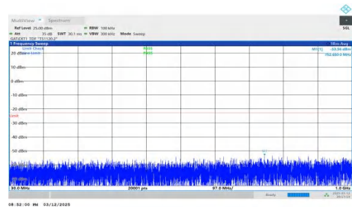
NTNV-n78(3450-3550)-PC2-30-70-H-DFT-QPSK-Inner_1RB_Right t.30-1000-PASS
