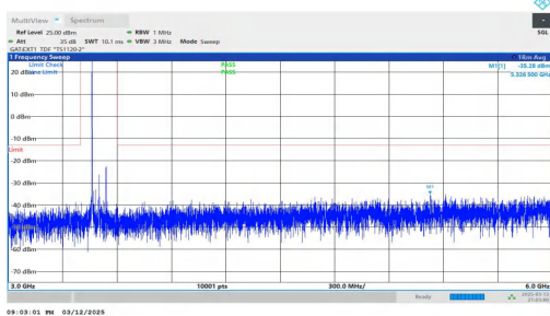
NTNV-n78(3450-3550)-PC2-30-80-M-DFT-QPSK-Inner_1RB_Lef t-3000-6000-PASS
