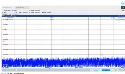
NTNV-n78(3450-3550)-PC2-30-90-L-DFT-QPSK-Inner_1RB_Left -30-1000-PASS
