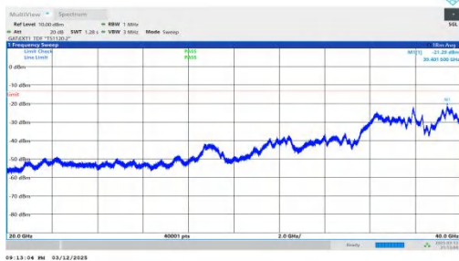
NTNV-n78(3450-3550)-PC2-30-90-L-DFT-BPSK-Inner_1RB_Left-20000-40000-PASS
