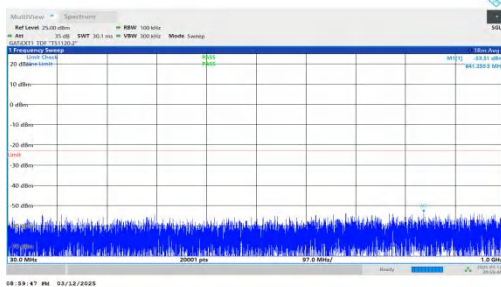
NTNV-n78(3450-3550)-PC2-30-80-M-DFT-BPSK-Inner_1RB_Left -30-1000-PASS
