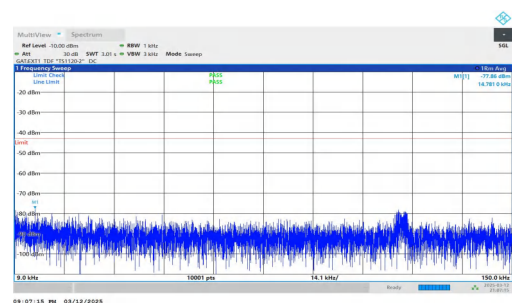
NTNV-n78(3450-3550)-PC2-30-80-H-DFT-BPSK-Inner_1RB_Right t-0.009-0.15-PASS
