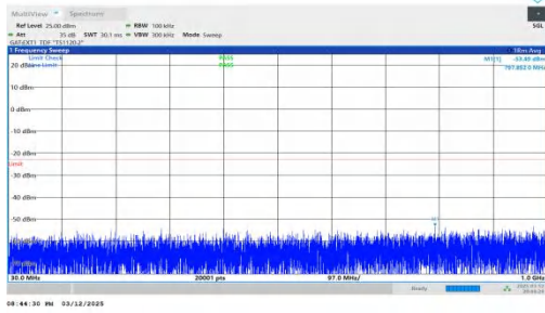
NTNV-n78(3450-3550)-PC2-30-70-M-DFT-QPSK-Inner_1RB_Lef t-30-1000-PASS
