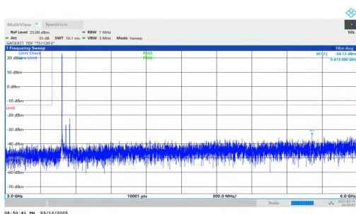
NTNV-n78(3450-3550)-PC2-30-70-H-DFT-QPSK-Inner_1RB_Left -3000-6000-PASS
