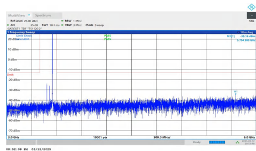
NTNV-n78(3450-3550)-PC2-30-70-H-DFT-QPSK-Inner_1RB_Right t.3000-6000-PASS
