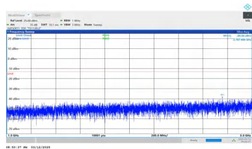
NTNV-n78(3450-3550)-PC2-30-70-H-DFT-QPSK-Inner_1RB_Left- 1000-3000-PASS
