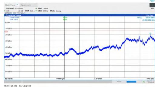
NTNV-n78(3450-3550)-PC2-30-80-M-DFT-QPSK-Inner_1RB_Righ t-20000-40000-PASS
