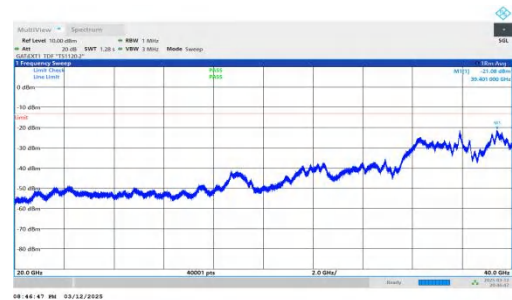
NTNV-n78(3450-3550)-PC2-30-70-M-DFT-QPSK-Inner_1RB_Righ t-20000-40000-PASS
