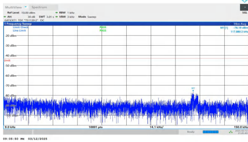
NTNV-n78(3450-3550)-PC2-30-80-H-DFT-BPSK-Inner_1RB_Left -0.009-0.15-PASS
