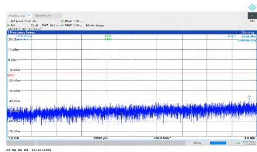
NTNV-n78(3450-3550)-PC2-30-80-M-DFT-QPSK-Inner_1RB_Left- 1000-3000-PASS
