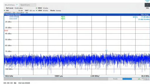
NTNV-n78(3450-3550)-PC2-30-80-H-DFT-QPSK-Inner_1RB_Left 0.15-30-PASS
