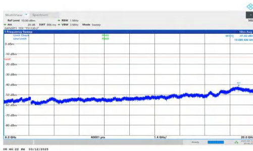
NTNV-n78(3450-3550)-PC2-30-70-M-DFT-QPSK-Inner_1RB_Rig ht-6000-20000-PASS
