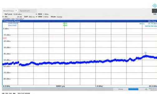
NTNV-n78(3450-3550)-PC2-30-70-H-DFT-QPSK-Inner_1RB_Right ht.6000-20000-PASS
