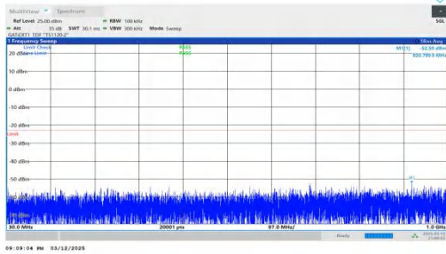
NTNV-n78(3450-3550)-PC2-30-80-H-DFT-QPSK-Inner_1RB_Left -30-1000-PASS
