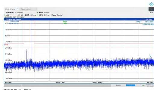
NTNV-n78(3450-3550)-PC2-30-90-L-DFT-QPSK-Inner_1RB_Right -3000-6000-PASS
