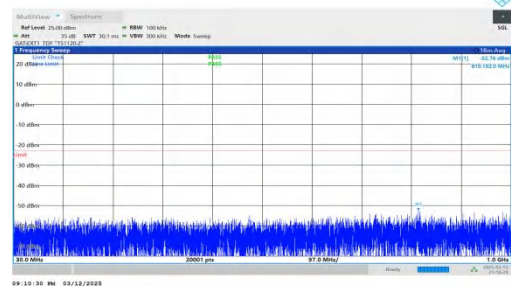
NTNV-n78(3450-3550)-PC2-30-80-H-DFT-QPSK-Inner_1RB_Right t=30-1000-PASS
