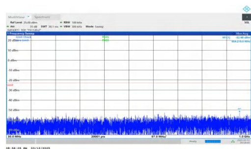
NTNV-n78(3450-3550)-PC2-30-80-L-DFT-QPSK-Inner_1RB_Right -30-1000-PASS
