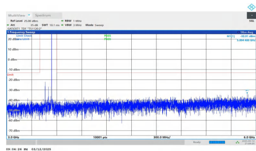
NTNV-n78(3450-3550)-PC2-30-80-M-DFT-QPSK-Inner_1RB_Righ t-3000-6000-PASS
