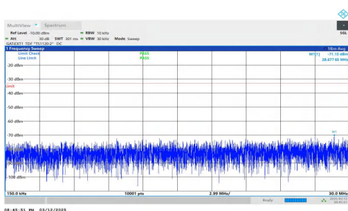
NTNV-n78(3450-3550)-PC2-30-70-M-DFT-QPSK-Inner_1RB_Rig ht-0.15-30-PASS
