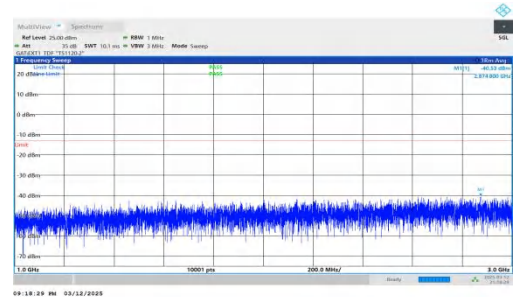
NTNV-n78(3450-3550)-PC2-30-90-M-DFT-BPSK-Inner_1RB_Left 1000-3000-PASS
