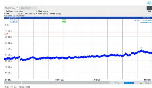
NTNV-n78(3450-3550)-PC2-30-80-H-DFT-QPSK-Inner_1RB_Left 6000-20000-PASS
