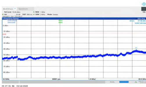
NTNV-n78(3450-3550)-PC2-30-80-H-DFT-BPSK-Inner_1RB_Rig ht-6000-20000-PASS
