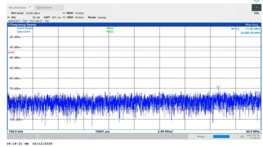
NTNV-n78(3450-3550)-PC2-30-90-M-DFT-BPSK-Inner_1RB_Left 0.15-30-PASS
