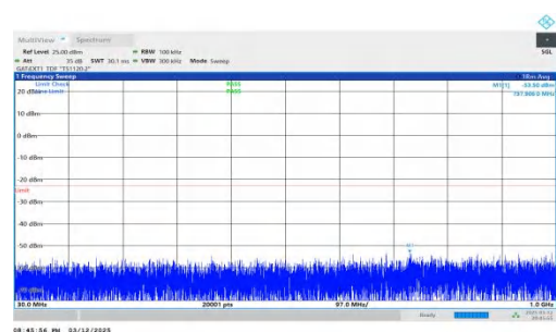
NTNV-n78(3450-3550)-PC2-30-70-M-DFT-QPSK-Inner_1RB_Right t-30-1000-PASS
