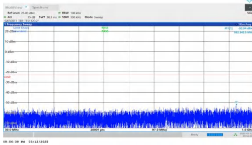
NTNV-n78(3450-3550)-PC2-30-80-L-DFT-QPSK-Inner_1RB_Left -30-1000-PASS
