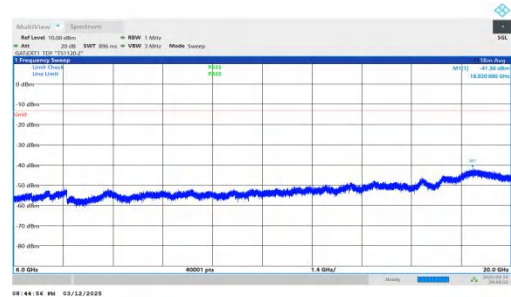
NTNV-n78(3450-3550)-PC2-30-70-M-DFT-QPSK-Inner_1RB_Left- 6000-20000-PASS
