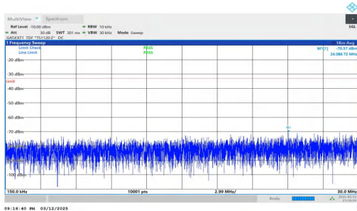
NTNV-n78(3450-3550)-PC2-30-90-L-DFT-QPSK-Inner_1RB_Rig ht-0.15-30-PASS
