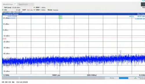
NTNV-n78(3450-3550)-PC2-30-80-L-DFT-QPSK-Inner_1RB_Rig ht-1000-3000-PASS
