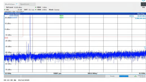
NTNV-n78(3450-3550)-PC2-30-80-H-DFT-QPSK-Inner_1RB_Righ t-3000-6000-PASS
