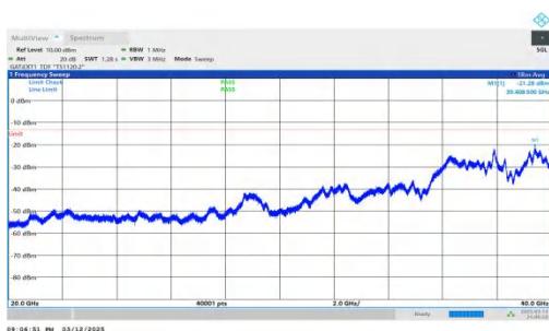
NTNV-n78(3450-3550)-PC2-30-80-H-DFT-BPSK-Inner_1RB_Left -20000-40000-PASS
