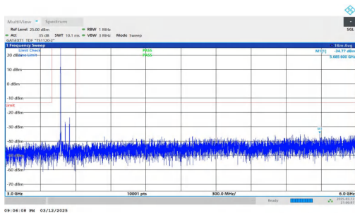
NTNV-n78(3450-3550)-PC2-30-80-H-DFT-BPSK-Inner_1RB_Left -3000-6000-PASS
