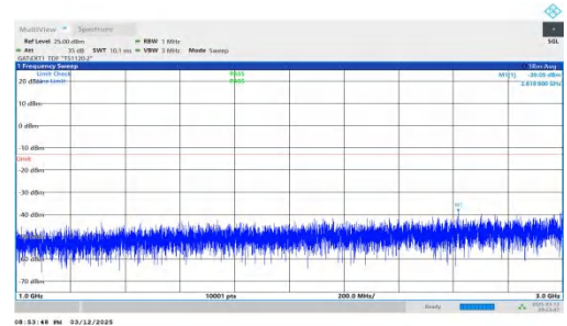
NTNV-n78(3450-3550)-PC2-30-80-L-DFT-BPSK-Inner_1RB_Left- 1000-3000-PASS
