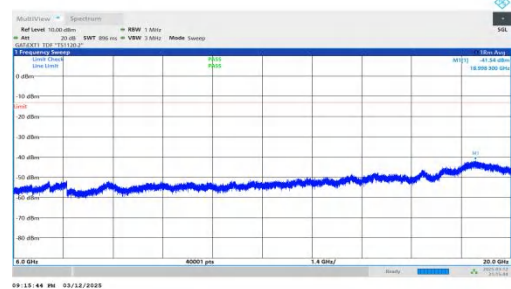
NTNV-n78(3450-3550)-PC2-30-90-L-DFT-QPSK-Inner_1RB_Left- 6000-20000-PASS
