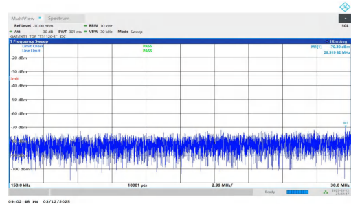
NTNV-n78(3450-3550)-PC2-30-80-M-DFT-QPSK-Inner_1RB_Left- 0.15-30-PASS
