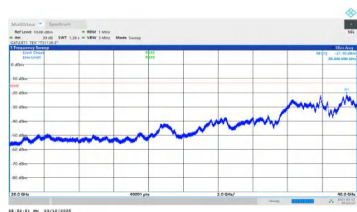
NTNV-n78(3450-3550)-PC2-30-70-H-DFT-QPSK-Inner_1RB_Right t.20000-40000-PASS
