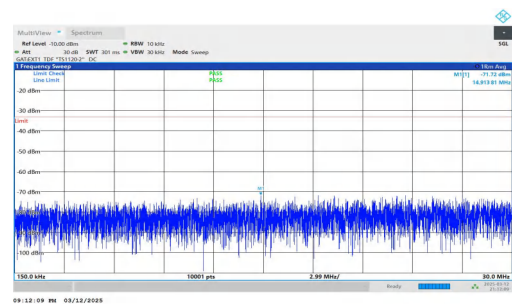
NTNV-n78(3450-3550)-PC2-30-90-L-DFT-BPSK-Inner_1RB_Left- 0.15-30-PASS
