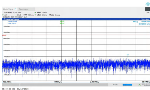
NTNV-n78(3450-3550)-PC2-30-70-H-DFT-BPSK-Inner_1RB_Right ht-0.15-30-PASS
