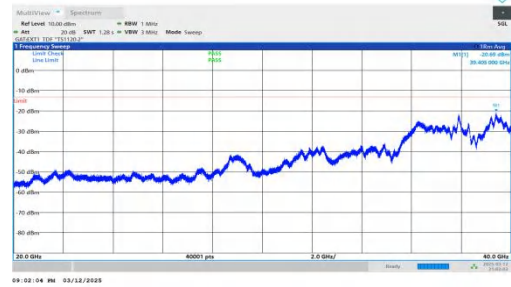
NTNV-n78(3450-3550)-PC2-30-80-M-DFT-BPSK-Inner_1RB_Righ t-20000-40000-PASS
