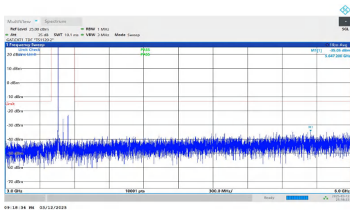
NTNV-n78(3450-3550)-PC2-30-90-M-DFT-BPSK-Inner_1RB_Left -3000-6000-PASS
