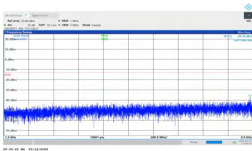
NTNV-n78(3450-3550)-PC2-30-80-M-DFT-QPSK-Inner_1RB_Rig ht-1000-3000-PASS
