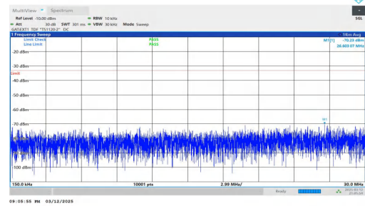
NTNV-n78(3450-3550)-PC2-30-80-H-DFT-BPSK-Inner_1RB_Left 0.15-30-PASS
