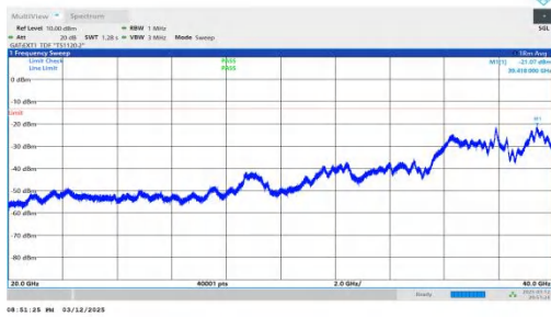
NTNV-n78(3450-3550)-PC2-30-70-H-DFT-QPSK-Inner_1RB_Left -20000-40000-PASS
