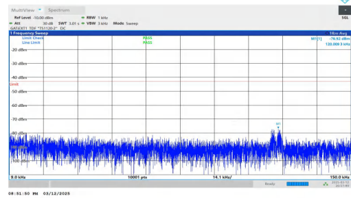
NTNV-n78(3450-3550)-PC2-30-70-H-DFT-QPSK-Inner_1RB_Right t.009-0.15-PASS
