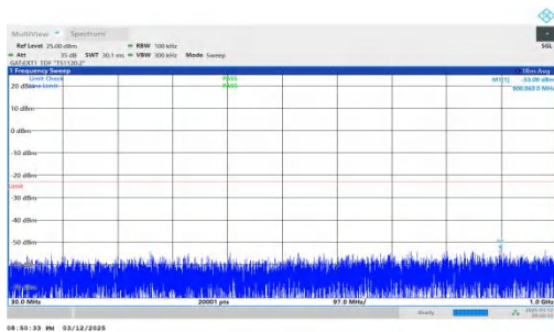
NTNV-n78(3450-3550)-PC2-30-70-H-DFT-QPSK-Inner_1RB_Left -30-1000-PASS
