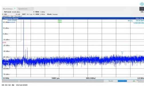
NTNV-n78(3450-3550)-PC2-30-80-L-DFT-BPSK-Inner_1RB_Left- 3000-6000-PASS
