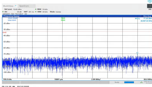
NTNV-n78(3450-3550)-PC2-30-90-L-DFT-BPSK-Inner_1RB_Rig ht-0.15-30-PASS
