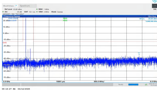
NTNV-n78(3450-3550)-PC2-30-90-L-DFT-QPSK-Inner_1RB_Left -3000-6000-PASS
