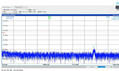
NTNV-n78(3450-3550)-PC2-30-70-H-DFT-BPSK-Inner_1RB_Left -0.009-0.15-PASS
