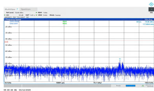
NTNV-n78(3450-3550)-PC2-30-70-M-DFT-QPSK-Inner_1RB_Right t-0.009-0.15-PASS
