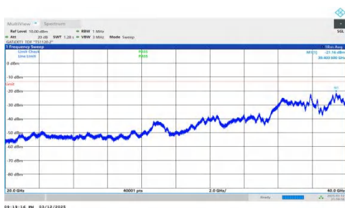
NTNV-n78(3450-3550)-PC2-30-90-M-DFT-BPSK-Inner_1RB_Left -20000-40000-PASS
