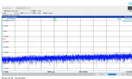
NTNV-n78(3450-3550)-PC2-30-70-H-DFT-QPSK-Inner_1RB_Right ht.1000-3000-PASS
