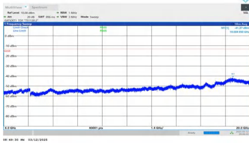
NTNV-n78(3450-3550)-PC2-30-70-H-DFT-BPSK-Inner_1RB_Rig ht-6000-20000-PASS
