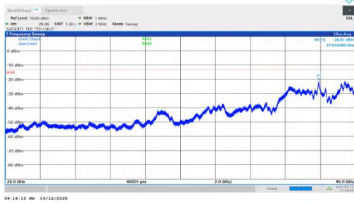
NTNV-n78(3450-3550)-PC2-30-90-L-DFT-QPSK-Inner_1RB_Left -20000-40000-PASS
