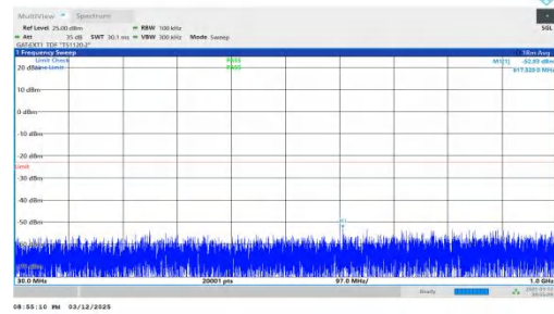
NTNV-n78(3450-3550)-PC2-30-80-L-DFT-BPSK-Inner_1RB_Right -30-1000-PASS
