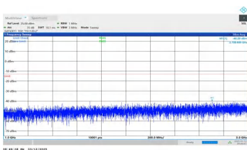
NTNV-n78(3450-3550)-PC2-30-70-H-DFT-BPSK-Inner_1RB_Right ht-1000-3000-PASS
