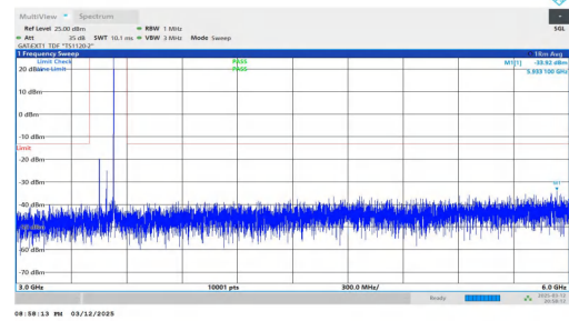
NTNV-n78(3450-3550)-PC2-30-80-L-DFT-QPSK-Inner_1RB_Right -3000-6000-PASS
