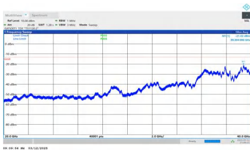
NTNV-n78(3450-3550)-PC2-30-80-H-DFT-QPSK-Inner_1RB_Left -20000-40000-PASS
