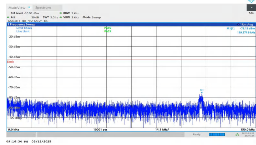
NTNV-n78(3450-3550)-PC2-30-90-L-DFT-QPSK-Inner_1RB_Right -0.009-0.15-PASS
