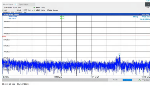
NTNV-n78(3450-3550)-PC2-30-90-M-DFT-BPSK-Inner_1RB_Left -0.009-0.15-PASS
