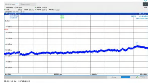
NTNV-n78(3450-3550)-PC2-30-80-M-DFT-BPSK-Inner_1RB_Left 6000-20000-PASS
