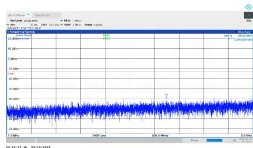
NTNV-n78(3450-3550)-PC2-30-90-L-DFT-QPSK-Inner_1RB_Left- 1000-3000-PASS
