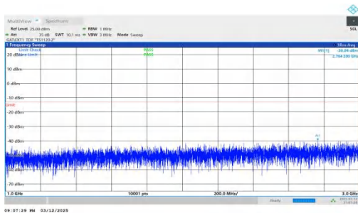
NTNV-n78(3450-3550)-PC2-30-80-H-DFT-BPSK-Inner_1RB_Rig ht-1000-3000-PASS
