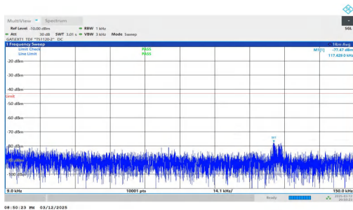
NTNV-n78(3450-3550)-PC2-30-70-H-DFT-QPSK-Inner_1RB_Left -0.009-0.15-PASS
