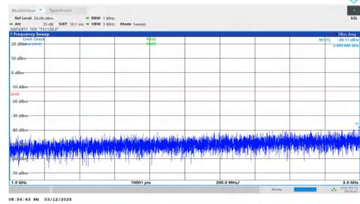
NTNV-n78(3450-3550)-PC2-30-80-L-DFT-QPSK-Inner_1RB_Left- 1000-3000-PASS
