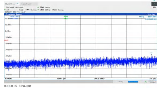
NTNV-n78(3450-3550)-PC2-30-80-H-DFT-QPSK-Inner_1RB_Left 1000-3000-PASS
