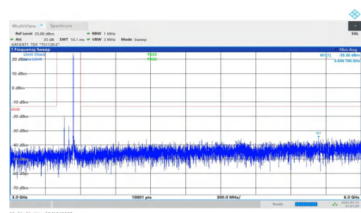
NTNV-n78(3450-3550)-PC2-30-80-M-DFT-BPSK-Inner_1RB_Right t-3000-6000-PASS
