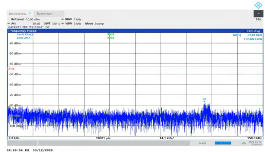
NTNV-n78(3450-3550)-PC2-30-70-H-DFT-BPSK-Inner_1RB_Right t-0.009-0.15-PASS
