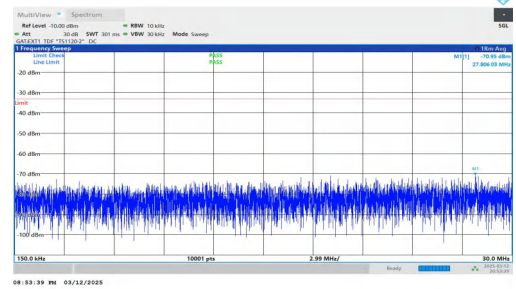
NTNV-n78(3450-3550)-PC2-30-80-L-DFT-BPSK-Inner_1RB_Left- 0.15-30-PASS
