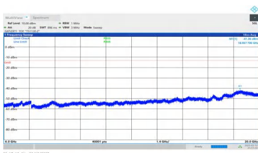
NTNV-n78(3450-3550)-PC2-30-90-L-DFT-QPSK-Inner_1RB_Rig ht-6000-20000-PASS
