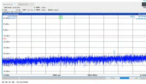
NTNV-n78(3450-3550)-PC2-30-70-M-DFT-QPSK-Inner_1RB_Rig ht-1000-3000-PASS
