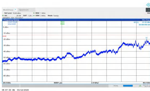
NTNV-n78(3450-3550)-PC2-30-80-L-DFT-QPSK-Inner_1RB_Left -20000-40000-PASS
