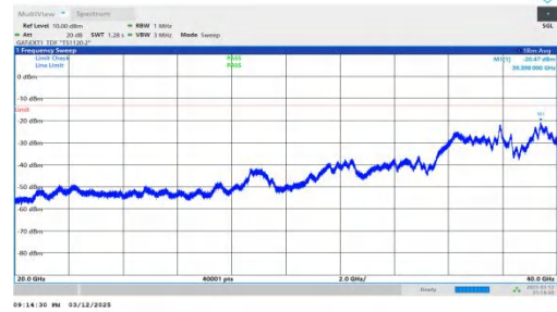
NTNV-n78(3450-3550)-PC2-30-90-L-DFT-BPSK-Inner_1RB_Right -20000-40000-PASS
