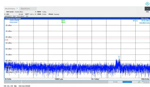
NTNV-n78(3450-3550)-PC2-30-80-M-DFT-BPSK-Inner_1RB_Right t-0.009-0.15-PASS
