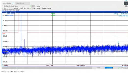
NTNV-n78(3450-3550)-PC2-30-90-L-DFT-BPSK-Inner_1RB_Left-3000-6000-PASS
