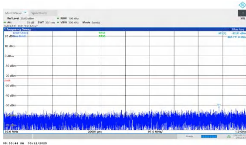
NTNV-n78(3450-3550)-PC2-30-80-L-DFT-BPSK-Inner_1RB_Left- 30-1000-PASS
