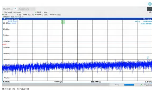
NTNV-n78(3450-3550)-PC2-30-80-L-DFT-BPSK-Inner_1RB_Rig ht-1000-3000-PASS
