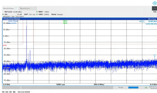
NTNV-n78(3450-3550)-PC2-30-70-M-DFT-QPSK-Inner_1RB_Lef t-3000-6000-PASS
