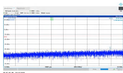
NTNV-n78(3450-3550)-PC2-30-70-H-DFT-BPSK-Inner_1RB_Left- 1000-3000-PASS
