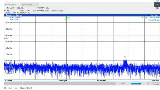
NTNV-n78(3450-3550)-PC2-30-80-M-DFT-QPSK-Inner_1RB_Righ t-0.009-0.15-PASS
