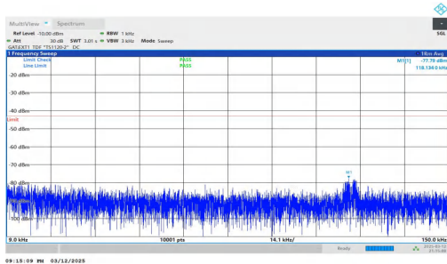
NTNV-n78(3450-3550)-PC2-30-90-L-DFT-QPSK-Inner_1RB_Left -0.009-0.15-PASS
