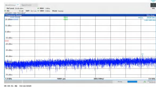
NTNV-n78(3450-3550)-PC2-30-80-M-DFT-BPSK-Inner_1RB_Left- 1000-3000-PASS
