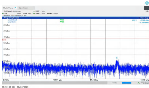
NTNV-n78(3450-3550)-PC2-30-80-M-DFT-QPSK-Inner_1RB_Lef t-0.009-0.15-PASS
