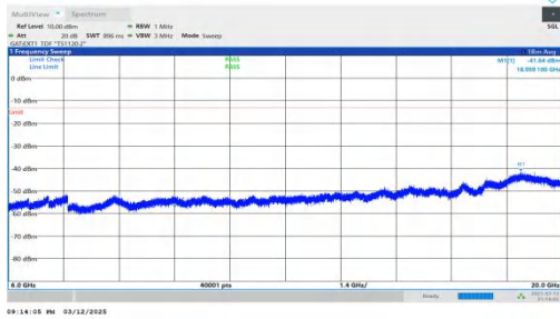
NTNV-n78(3450-3550)-PC2-30-90-L-DFT-BPSK-Inner_1RB_Rig ht-6000-20000-PASS
