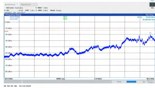
NTNV-n78(3450-3550)-PC2-30-70-H-DFT-BPSK-Inner_1RB_Righ t-20000-40000-PASS
