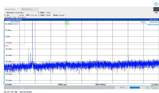
NTNV-n78(3450-3550)-PC2-30-80-H-DFT-BPSK-Inner_1RB_Righ t-3000-6000-PASS
