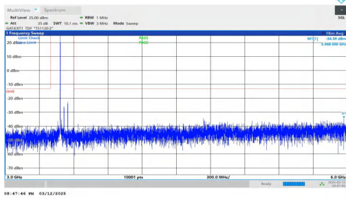
NTNV-n78(3450-3550)-PC2-30-70-H-DFT-BPSK-Inner_1RB_Left -3000-6000-PASS
