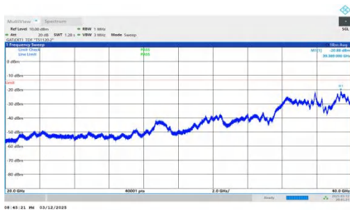
NTNV-n78(3450-3550)-PC2-30-70-M-DFT-QPSK-Inner_1RB_Lef t-20000-40000-PASS
