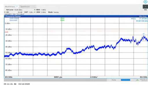
NTNV-n78(3450-3550)-PC2-30-80-H-DFT-QPSK-Inner_1RB_Righ t-20000-40000-PASS
