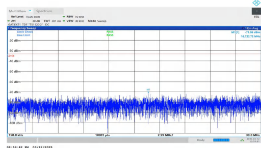
NTNV-n78(3450-3550)-PC2-30-80-M-DFT-BPSK-Inner_1RB_Left- 0.15-30-PASS
