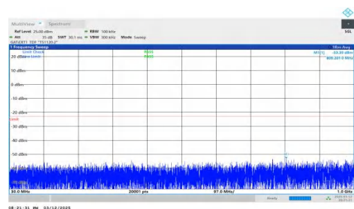
NTNV-n78(3450-3550)-PC2-30-60-L-DFT-QPSK-Inner_1RB_Right -30-1000-PASS
