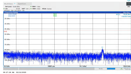
NTNV-n78(3450-3550)-PC2-30-60-M-DFT-QPSK-Inner_1RB_Righ t-0.009-0.15-PASS
