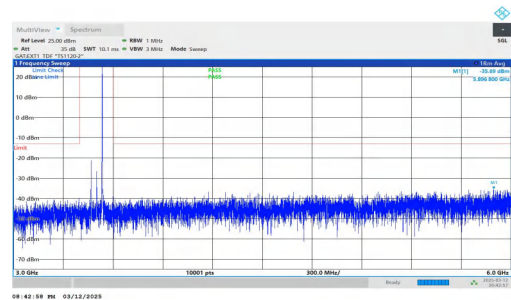
NTNV-n78(3450-3550)-PC2-30-70-M-DFT-BPSK-Inner_1RB_Righ t-3000-6000-PASS
