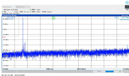
NTNV-n78(3450-3550)-PC2-30-60-H-DFT-QPSK-Inner_1RB_Left -3000-6000-PASS
