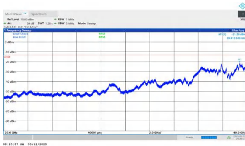
NTNV-n78(3450-3550)-PC2-30-60-L-DFT-QPSK-Inner_1RB_Left -20000-40000-PASS
