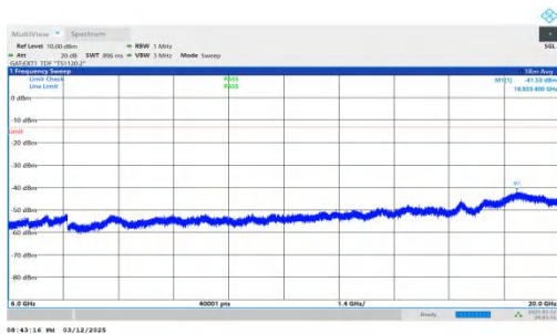
NTNV-n78(3450-3550)-PC2-30-70-M-DFT-BPSK-Inner_1RB_Rig ht-6000-20000-PASS
