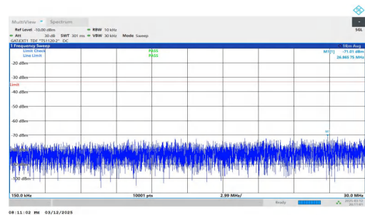
NTNV-n78(3450-3550)-PC2-30-50-H-DFT-BPSK-Inner_1RB_Left- 0.15-30-PASS
