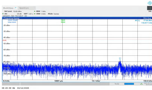
NTNV-n78(3450-3550)-PC2-30-60-M-DFT-QPSK-Inner_1RB_Lef t-0.009-0.15-PASS
