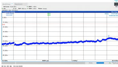
NTNV-n78(3450-3550)-PC2-30-60-L-DFT-QPSK-Inner_1RB_Rig ht-6000-20000-PASS
