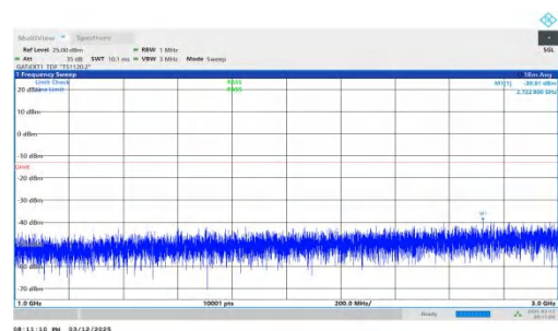
NTNV-n78(3450-3550)-PC2-30-50-H-DFT-BPSK-Inner_1RB_Left- 1000-3000-PASS
