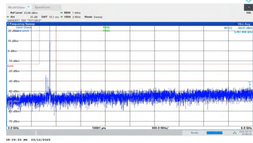
NTNV-n78(3450-3550)-PC2-30-50-M-DFT-QPSK-Inner_1RB_Righ t-3000-6000-PASS
