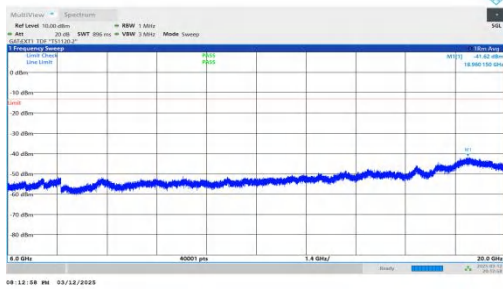
NTNV-n78(3450-3550)-PC2-30-50-H-DFT-BPSK-Inner_1RB_Rig ht-6000-20000-PASS
