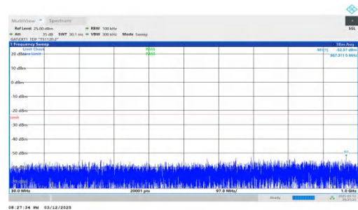
NTNV-n78(3450-3550)-PC2-30-60-M-DFT-QPSK-Inner_1RB_Righ t-30-1000-PASS
