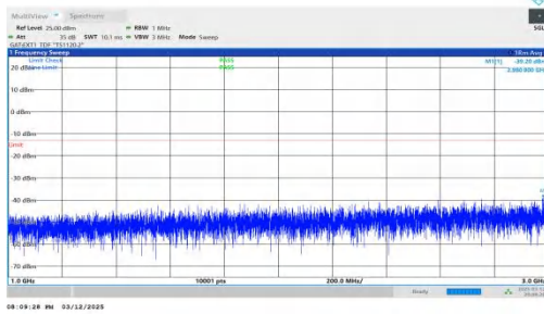
NTNV-n78(3450-3550)-PC2-30-50-M-DFT-QPSK-Inner_1RB_Rig ht-1000-3000-PASS
