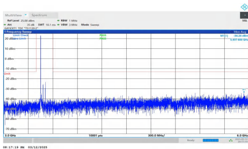
NTNV-n78(3450-3550)-PC2-30-60-L-DFT-BPSK-Inner_1RB_Left- 3000-6000-PASS
