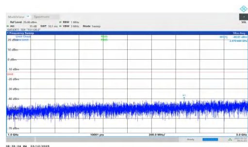
NTVN-n78(3450-3550)-PC2-30-70-L-DFT-BPSK-Inner_1RB_Left- 1000-3000-PASS
