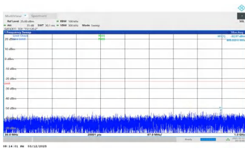
NTNV-n78(3450-3550)-PC2-30-50-H-DFT-QPSK-Inner_1RB_Left -30-1000-PASS
