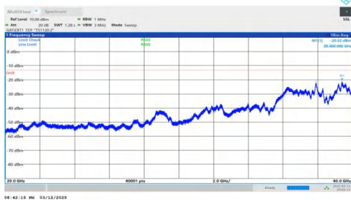
NTNV-n78(3450-3550)-PC2-30-70-M-DFT-BPSK-Inner_1RB_Left -20000-40000-PASS
