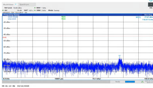
NTNV-n78(3450-3550)-PC2-30-70-M-DFT-BPSK-Inner_1RB_Left -0.009-0.15-PASS
