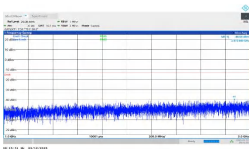
NTNV-n78(3450-3550)-PC2-30-50-H-DFT-QPSK-Inner_1RB_Right ht-1000-3000-PASS
