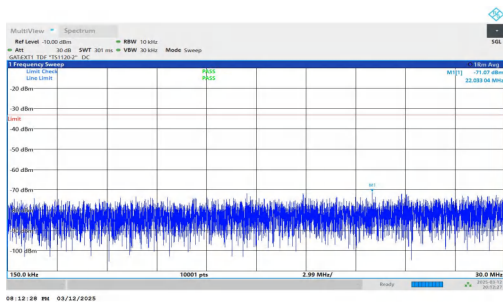
NTNV-n78(3450-3550)-PC2-30-50-H-DFT-BPSK-Inner_1RB_Rig ht-0.15-30-PASS
