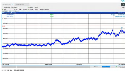
NTNV-n78(3450-3550)-PC2-30-60-L-DFT-BPSK-Inner_1RB_Left- 20000-40000-PASS
