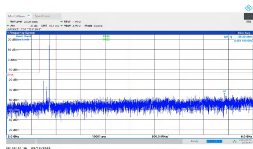
NTNV-n78(3450-3550)-PC2-30-70-L-DFT-QPSK-Inner_1RB_Right -3000-6000-PASS
