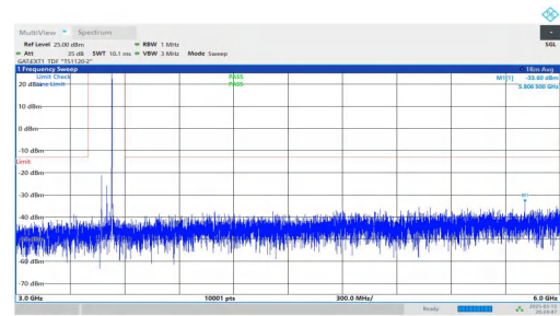
NTNV-n78(3450-3550)-PC2-30-60-M-DFT-BPSK-Inner_1RB_Right t-3000-6000-PASS
