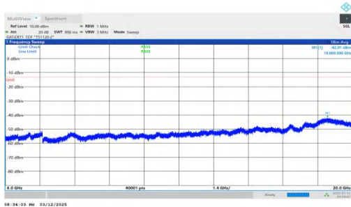
NTVN-n78(3450-3550)-PC2-30-60-H-DFT-QPSK-Inner_1RB_Rig ht-6000-20000-PASS
