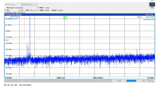
NTNV-n78(3450-3550)-PC2-30-60-L-DFT-QPSK-Inner_1RB_Right -3000-6000-PASS
