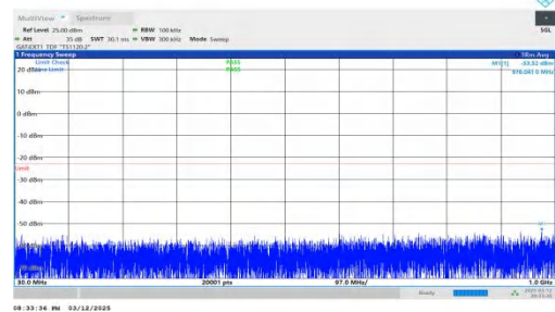
NTNV-n78(3450-3550)-PC2-30-60-H-DFT-QPSK-Inner_1RB_Right t-30-1000-PASS
