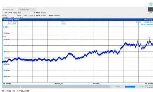
NTNV-n78(3450-3550)-PC2-30-60-H-DFT-QPSK-Inner_1RB_Left -20000-40000-PASS
