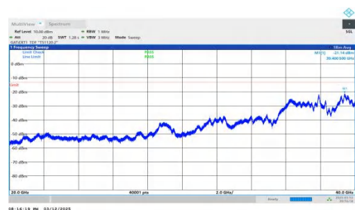
NTNV-n78(3450-3550)-PC2-30-50-H-DFT-QPSK-Inner_1RB_Right t-20000-40000-PASS
