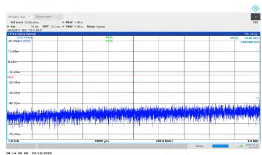
NTNV-n78(3450-3550)-PC2-30-50-H-DFT-QPSK-Inner_1RB_Left- 1000-3000-PASS
