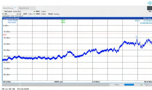
NTNV-n78(3450-3550)-PC2-30-50-H-DFT-BPSK-Inner_1RB_Left -20000-40000-PASS
