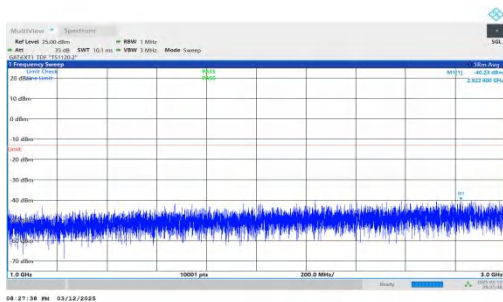
NTNV-n78(3450-3550)-PC2-30-60-M-DFT-QPSK-Inner_1RB_Rig ht-1000-3000-PASS
