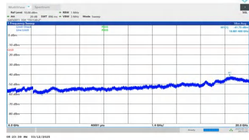
NTNV-n78(3450-3550)-PC2-30-60-M-DFT-BPSK-Inner_1RB_Left 6000-20000-PASS
