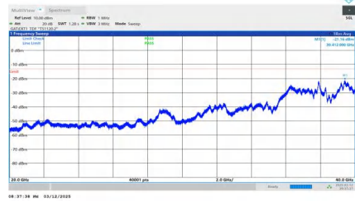
NTNV-n78(3450-3550)-PC2-30-70-L-DFT-BPSK-Inner_1RB_Right -20000-40000-PASS
