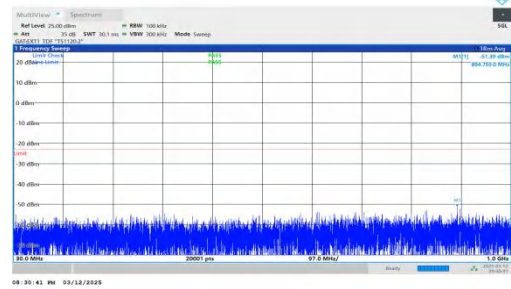
NTNV-n78(3450-3550)-PC2-30-60-H-DFT-BPSK-Inner_1RB_Righ t-30-1000-PASS
