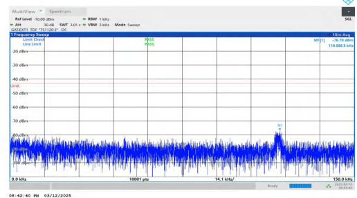
NTNV-n78(3450-3550)-PC2-30-70-M-DFT-BPSK-Inner_1RB_Right t-0.009-0.15-PASS
