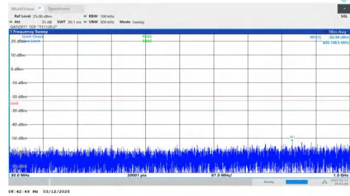
NTNV-n78(3450-3550)-PC2-30-70-M-DFT-BPSK-Inner_1RB_Righ t-30-1000-PASS
