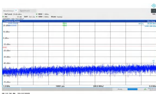
NTNV-n78(3450-3550)-PC2-30-50-H-DFT-BPSK-Inner_1RB_Rig ht-1000-3000-PASS
