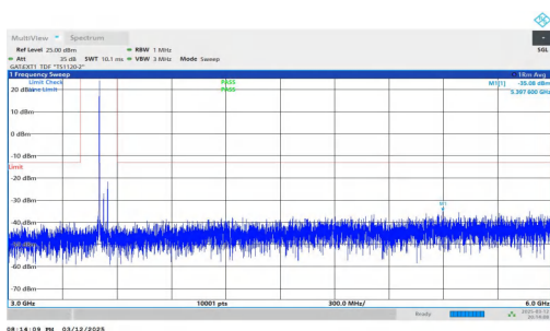
NTNV-n78(3450-3550)-PC2-30-50-H-DFT-QPSK-Inner_1RB_Left -3000-6000-PASS
