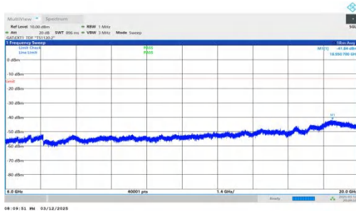
NTNV-n78(3450-3550)-PC2-30-50-M-DFT-QPSK-Inner_1RB_Rig ht-6000-20000-PASS
