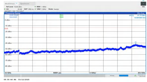
NTNV-n78(3450-3550)-PC2-30-70-L-DFT-BPSK-Inner_1RB_Left-6000-20000-PASS
