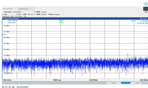
NTNV-n78(3450-3550)-PC2-30-60-M-DFT-QPSK-Inner_1RB_Rig ht-0.15-30-PASS
