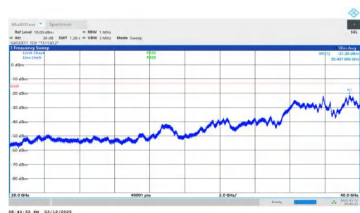
NTNV-n78(3450-3550)-PC2-30-70-L-DFT-QPSK-Inner_1RB_Right -20000-40000-PASS
