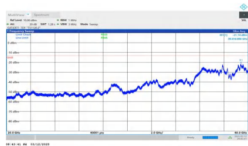
NTNV-n78(3450-3550)-PC2-30-70-M-DFT-BPSK-Inner_1RB_Righ t-20000-40000-PASS
