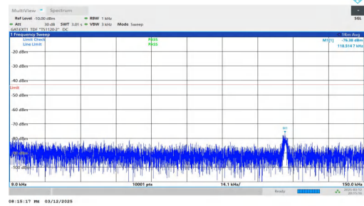
NTNV-n78(3450-3550)-PC2-30-50-H-DFT-QPSK-Inner_1RB_Right t.009-0.15-PASS
