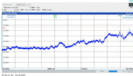
NTNV-n78(3450-3550)-PC2-30-70-L-DFT-BPSK-Inner_1RB_Left-20000-40000-PASS
