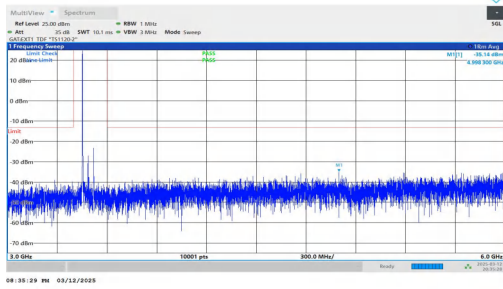
NTNV-n78(3450-3550)-PC2-30-70-L-DFT-BPSK-Inner_1RB_Left-3000-6000-PASS
