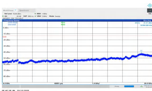
NTNV-n78(3450-3550)-PC2-30-70-L-DFT-QPSK-Inner_1RB_Rig ht-6000-20000-PASS
