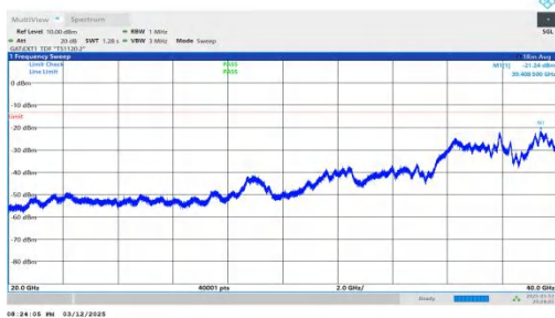
NTNV-n78(3450-3550)-PC2-30-60-M-DFT-BPSK-Inner_1RB_Left -20000-40000-PASS
