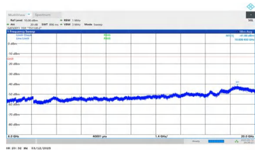
NTNV-n78(3450-3550)-PC2-30-60-L-DFT-QPSK-Inner_1RB_Left- 6000-20000-PASS
