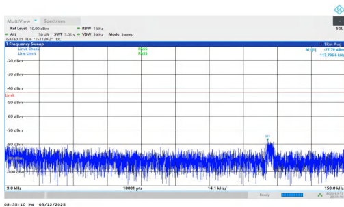
NTVN-n78(3450-3550)-PC2-30-70-L-DFT-BPSK-Inner_1RB_Left- 0.009-0.15-PASS
