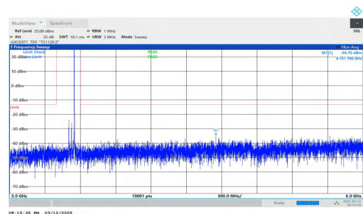
NTNV-n78(3450-3550)-PC2-30-50-H-DFT-QPSK-Inner_1RB_Right t-3000-6000-PASS
