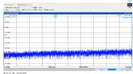
NTNV-n78(3450-3550)-PC2-30-60-M-DFT-BPSK-Inner_1RB_Left- 1000-3000-PASS
