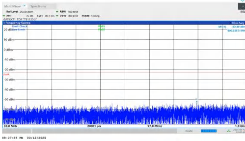
NTNV-n78(3450-3550)-PC2-30-50-M-DFT-QPSK-Inner_1RB_Lef t-30-1000-PASS
