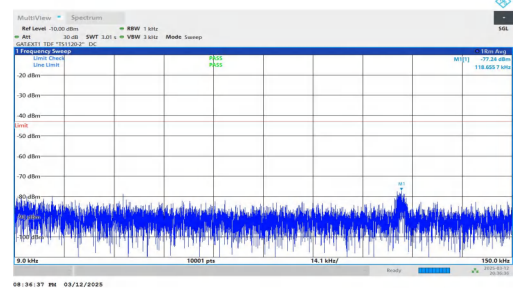
NTNV-n78(3450-3550)-PC2-30-70-L-DFT-BPSK-Inner_1RB_Right-0.009-0.15-PASS
