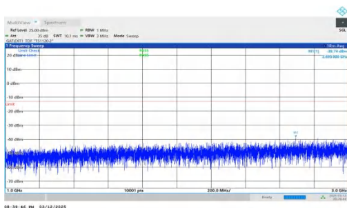
NTNV-n78(3450-3550)-PC2-30-70-L-DFT-QPSK-Inner_1RB_Rig ht-1000-3000-PASS
