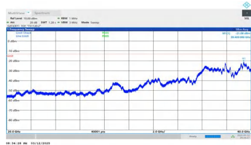
NTVN-n78(3450-3550)-PC2-30-60-H-DFT-QPSK-Inner_1RB_Righ t-20000-40000-PASS
