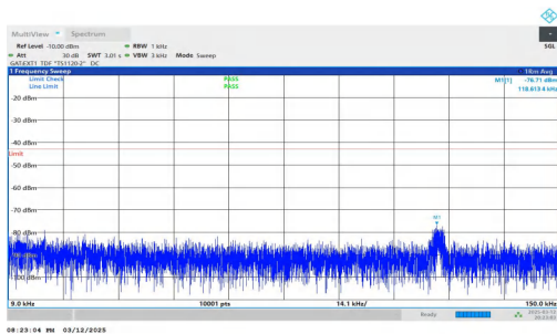
NTNV-n78(3450-3550)-PC2-30-60-M-DFT-BPSK-Inner_1RB_Left -0.009-0.15-PASS
