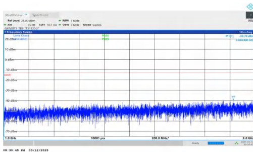
NTNV-n78(3450-3550)-PC2-30-60-H-DFT-BPSK-Inner_1RB_Rig ht-1000-3000-PASS
