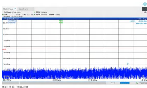
NTNV-n78(3450-3550)-PC2-30-60-M-DFT-QPSK-Inner_1RB_Lef t-30-1000-PASS
