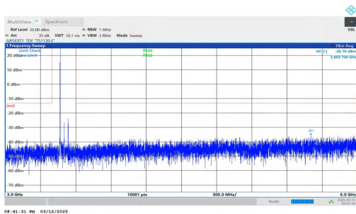
NTNV-n78(3450-3550)-PC2-30-70-M-DFT-BPSK-Inner_1RB_Left -3000-6000-PASS
