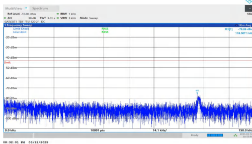
NTNV-n78(3450-3550)-PC2-30-60-H-DFT-QPSK-Inner_1RB_Left -0.009-0.15-PASS
