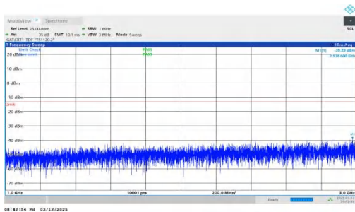
NTNV-n78(3450-3550)-PC2-30-70-M-DFT-BPSK-Inner_1RB_Rig ht-1000-3000-PASS
