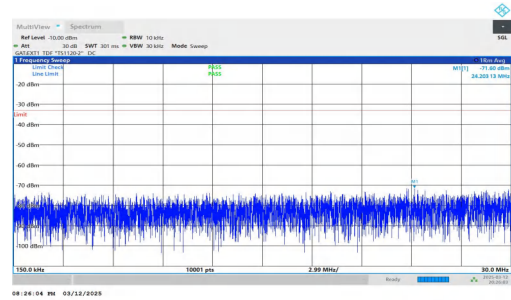
NTNV-n78(3450-3550)-PC2-30-60-M-DFT-QPSK-Inner_1RB_Left- 0.15-30-PASS
