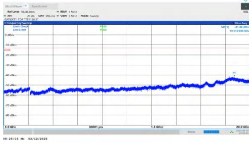
NTNV-n78(3450-3550)-PC2-30-60-M-DFT-BPSK-Inner_1RB_Rig ht-6000-20000-PASS
