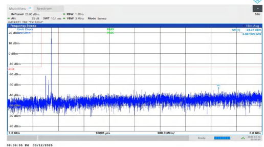
NTNV-n78(3450-3550)-PC2-30-70-L-DFT-BPSK-Inner_1RB_Right-3000-6000-PASS
