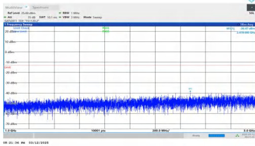
NTNV-n78(3450-3550)-PC2-30-60-L-DFT-QPSK-Inner_1RB_Rig ht-1000-3000-PASS
