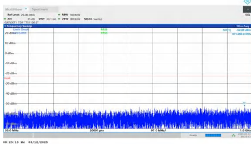
NTNV-n78(3450-3550)-PC2-30-60-M-DFT-BPSK-Inner_1RB_Left -30-1000-PASS
