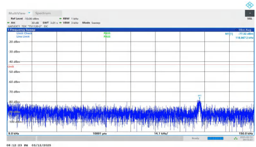
NTNV-n78(3450-3550)-PC2-30-50-H-DFT-BPSK-Inner_1RB_Right t-0.009-0.15-PASS
