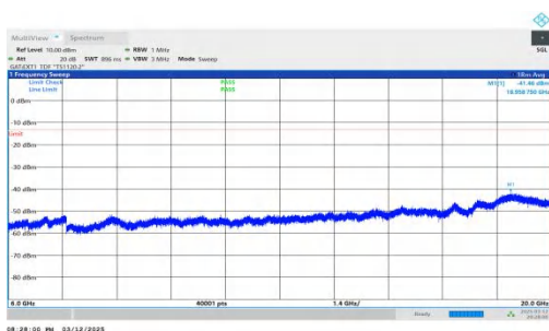
NTNV-n78(3450-3550)-PC2-30-60-M-DFT-QPSK-Inner_1RB_Rig ht-6000-20000-PASS
