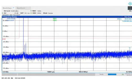
NTNV-n78(3450-3550)-PC2-30-60-H-DFT-BPSK-Inner_1RB_Left -3000-6000-PASS
