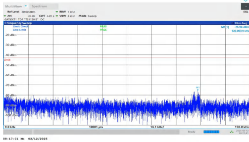
NTNV-n78(3450-3550)-PC2-30-60-L-DFT-BPSK-Inner_1RB_Left- 0.009-0.15-PASS
