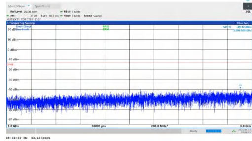
NTNV-n78(3450-3550)-PC2-30-50-M-DFT-QPSK-Inner_1RB_Left- 1000-3000-PASS
