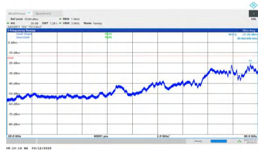
NTNV-n78(3450-3550)-PC2-30-50-M-DFT-QPSK-Inner_1RB_Righ t-20000-40000-PASS
