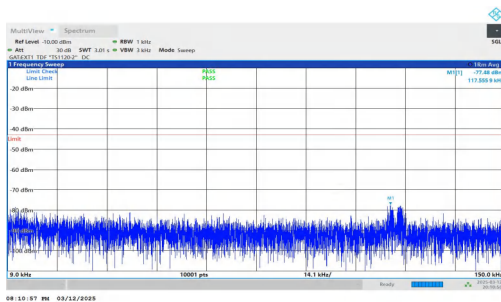
NTNV-n78(3450-3550)-PC2-30-50-H-DFT-BPSK-Inner_1RB_Left -0.009-0.15-PASS
