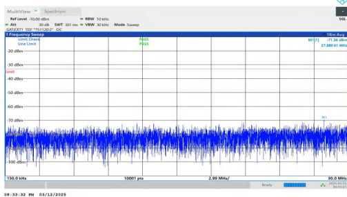
NTNV-n78(3450-3550)-PC2-30-60-H-DFT-QPSK-Inner_1RB_Rig ht-0.15-30-PASS
