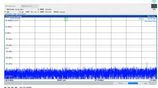
NTNV-n78(3450-3550)-PC2-30-70-L-DFT-BPSK-Inner_1RB_Right-30-1000-PASS
