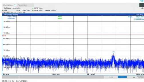
NTNV-n78(3450-3550)-PC2-30-70-L-DFT-QPSK-Inner_1RB_Left -0.009-0.15-PASS
