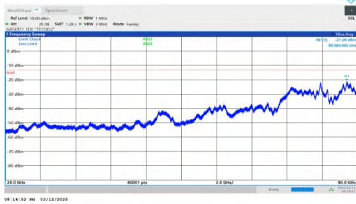
NTNV-n78(3450-3550)-PC2-30-50-H-DFT-QPSK-Inner_1RB_Left -20000-40000-PASS
