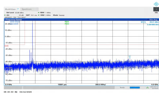
NTNV-n78(3450-3550)-PC2-30-60-H-DFT-BPSK-Inner_1RB_Righ t-3000-6000-PASS
