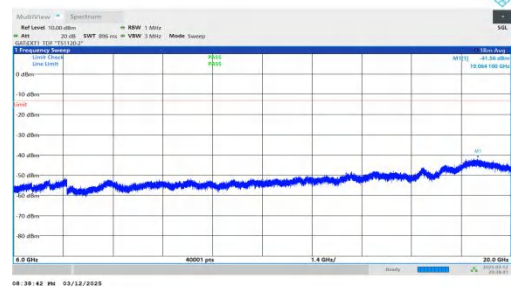
NTNV-n78(3450-3550)-PC2-30-70-L-DFT-QPSK-Inner_1RB_Left- 6000-20000-PASS
