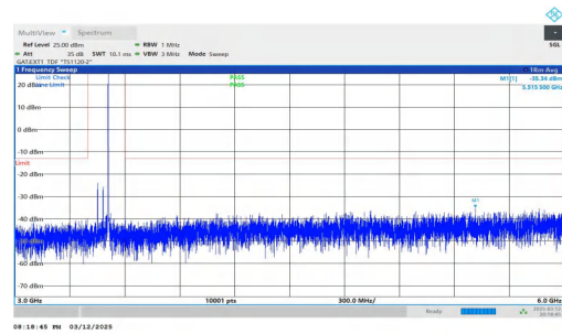
NTNV-n78(3450-3550)-PC2-30-60-L-DFT-BPSK-Inner_1RB_Right -3000-6000-PASS
