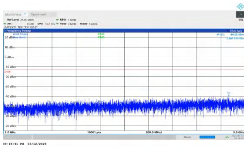
NTNV-n78(3450-3550)-PC2-30-60-L-DFT-BPSK-Inner_1RB_Rig ht-1000-3000-PASS
