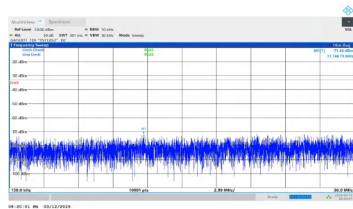
NTNV-n78(3450-3550)-PC2-30-60-L-DFT-QPSK-Inner_1RB_Left- 0.15-30-PASS
