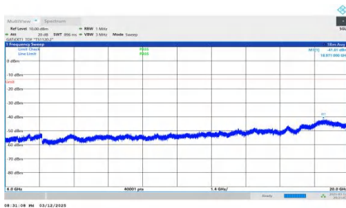
NTNV-n78(3450-3550)-PC2-30-60-H-DFT-BPSK-Inner_1RB_Rig ht-6000-20000-PASS
