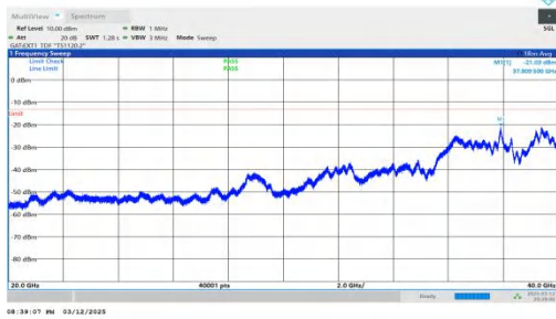
NTNV-n78(3450-3550)-PC2-30-70-L-DFT-QPSK-Inner_1RB_Left -20000-40000-PASS
