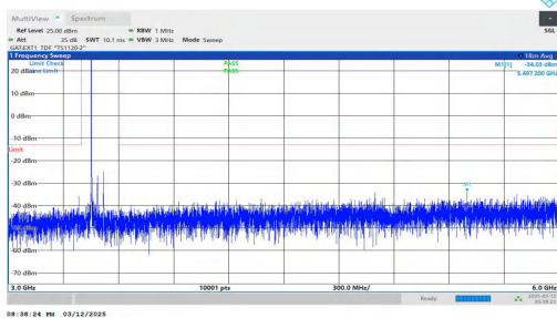
NTNV-n78(3450-3550)-PC2-30-70-L-DFT-QPSK-Inner_1RB_Left -3000-6000-PASS
