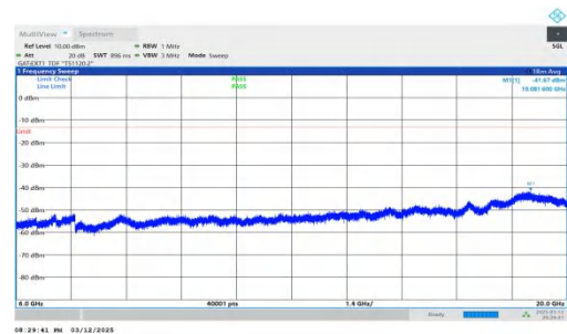
NTNV-n78(3450-3550)-PC2-30-60-H-DFT-BPSK-Inner_1RB_Left 6000-20000-PASS
