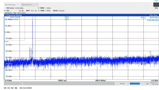
NTVN-n78(3450-3550)-PC2-30-60-H-DFT-QPSK-Inner_1RB_Righ t-3000-6000-PASS
