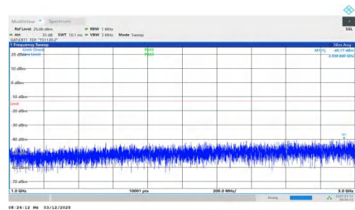
NTNV-n78(3450-3550)-PC2-30-60-M-DFT-QPSK-Inner_1RB_Left- 1000-3000-PASS
