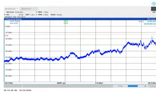
NTNV-n78(3450-3550)-PC2-30-60-L-DFT-BPSK-Inner_1RB_Right -20000-40000-PASS
