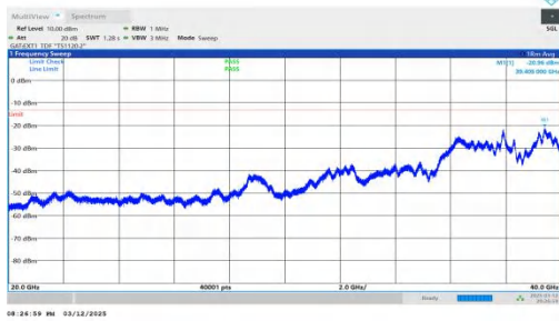
NTNV-n78(3450-3550)-PC2-30-60-M-DFT-QPSK-Inner_1RB_Lef t-20000-40000-PASS
