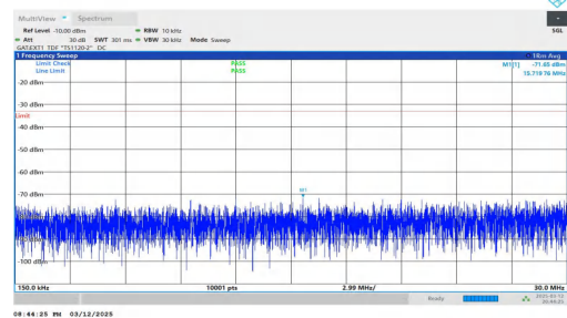
NTNV-n78(3450-3550)-PC2-30-70-M-DFT-QPSK-Inner_1RB_Left- 0.15-30-PASS
