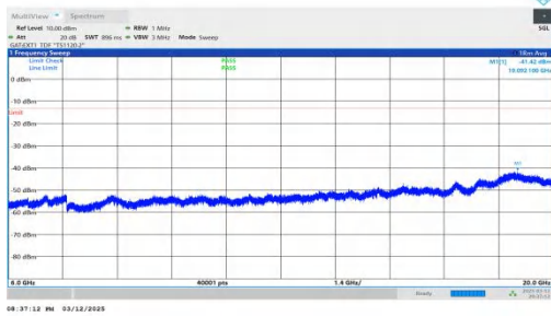
NTNV-n78(3450-3550)-PC2-30-70-L-DFT-BPSK-Inner_1RB_Rig ht-6000-20000-PASS
