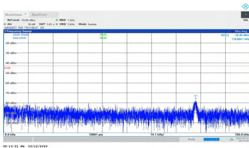
NTNV-n78(3450-3550)-PC2-30-50-H-DFT-QPSK-Inner_1RB_Left -0.009-0.15-PASS
