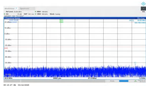
NTNV-n78(3450-3550)-PC2-30-50-H-DFT-QPSK-Inner_1RB_Right t-30-1000-PASS
