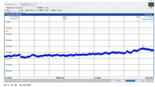
NTNV-n78(3450-3550)-PC2-30-50-H-DFT-BPSK-Inner_1RB_Left- 6000-20000-PASS
