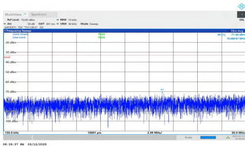
NTNV-n78(3450-3550)-PC2-30-70-L-DFT-QPSK-Inner_1RB_Rig ht-0.15-30-PASS
