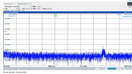
NTNV-n78(3450-3550)-PC2-30-70-L-DFT-QPSK-Inner_1RB_Right -0.009-0.15-PASS
