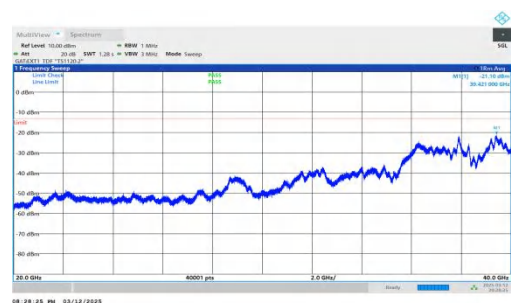
NTNV-n78(3450-3550)-PC2-30-60-M-DFT-QPSK-Inner_1RB_Righ t-20000-40000-PASS
