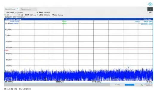
NTNV-n78(3450-3550)-PC2-30-50-H-DFT-BPSK-Inner_1RB_Right t-30-1000-PASS
