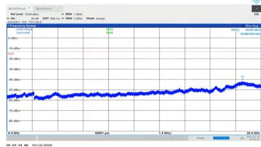
NTNV-n78(3450-3550)-PC2-30-60-M-DFT-QPSK-Inner_1RB_Left- 6000-20000-PASS
