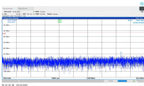
NTNV-n78(3450-3550)-PC2-30-50-H-DFT-QPSK-Inner_1RB_Right ht-0.15-30-PASS
