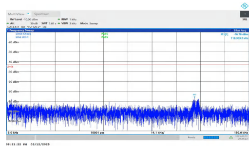
NTNV-n78(3450-3550)-PC2-30-60-L-DFT-QPSK-Inner_1RB_Right -0.009-0.15-PASS
