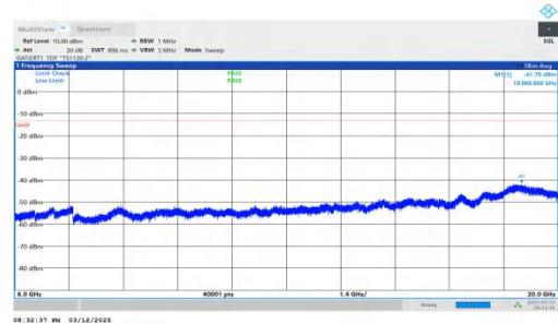
NTNV-n78(3450-3550)-PC2-30-60-H-DFT-QPSK-Inner_1RB_Left 6000-20000-PASS
