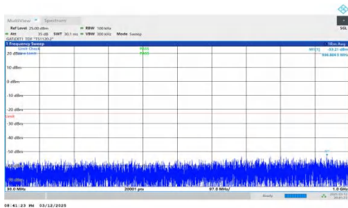
NTNV-n78(3450-3550)-PC2-30-70-M-DFT-BPSK-Inner_1RB_Left -30-1000-PASS
