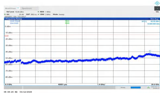
NTNV-n78(3450-3550)-PC2-30-50-M-DFT-QPSK-Inner_1RB_Left- 6000-20000-PASS
