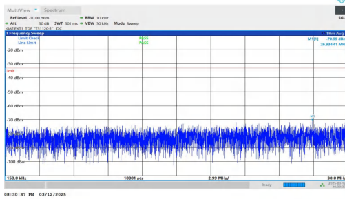
NTNV-n78(3450-3550)-PC2-30-60-H-DFT-BPSK-Inner_1RB_Rig ht-0.15-30-PASS
