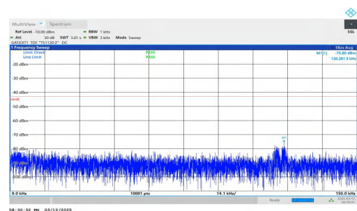
NTNV-n78(3450-3550)-PC2-30-60-H-DFT-BPSK-Inner_1RB_Right t-0.009-0.15-PASS
