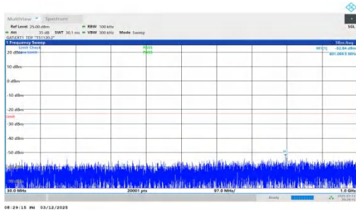
NTNV-n78(3450-3550)-PC2-30-60-H-DFT-BPSK-Inner_1RB_Left -30-1000-PASS
