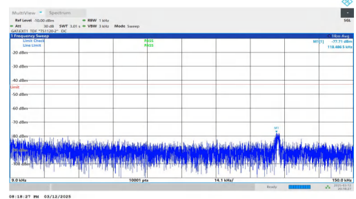
NTNV-n78(3450-3550)-PC2-30-60-L-DFT-BPSK-Inner_1RB_Right -0.009-0.15-PASS
