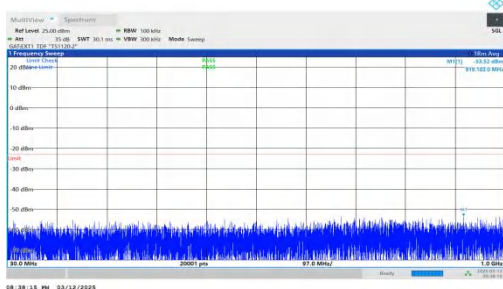
NTNV-n78(3450-3550)-PC2-30-70-L-DFT-QPSK-Inner_1RB_Left -30-1000-PASS
