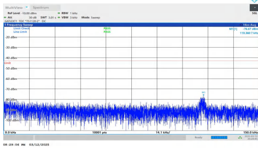
NTNV-n78(3450-3550)-PC2-30-60-H-DFT-BPSK-Inner_1RB_Left -0.009-0.15-PASS
