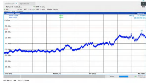
NTNV-n78(3450-3550)-PC2-30-60-M-DFT-BPSK-Inner_1RB_Righ t-20000-40000-PASS
