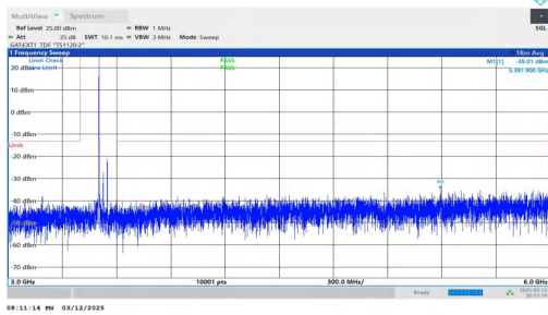
NTNV-n78(3450-3550)-PC2-30-50-H-DFT-BPSK-Inner_1RB_Left -3000-6000-PASS
