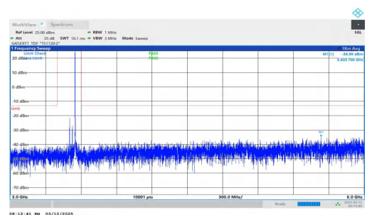
NTNV-n78(3450-3550)-PC2-30-50-H-DFT-BPSK-Inner_1RB_Right t-3000-6000-PASS
