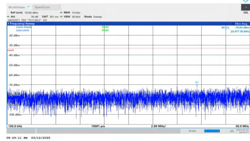
NTNV-n78(3450-3550)-PC2-30-60-H-DFT-BPSK-Inner_1RB_Left 0.15-30-PASS
