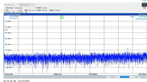
NTNV-n78(3450-3550)-PC2-30-60-H-DFT-QPSK-Inner_1RB_Left 0.15-30-PASS
