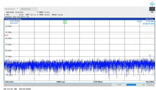
NTNV-n78(3450-3550)-PC2-30-50-H-DFT-QPSK-Inner_1RB_Left- 0.15-30-PASS
