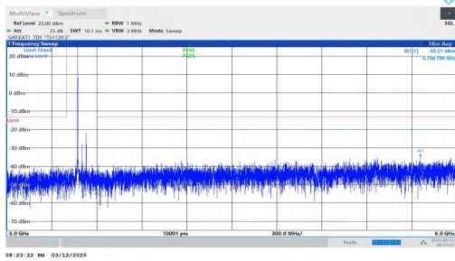
NTNV-n78(3450-3550)-PC2-30-60-M-DFT-BPSK-Inner_1RB_Left -3000-6000-PASS
