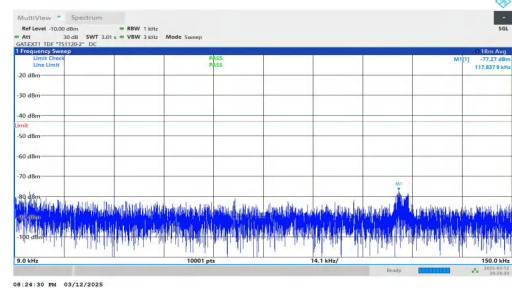
NTNV-n78(3450-3550)-PC2-30-60-M-DFT-BPSK-Inner_1RB_Right t-0.009-0.15-PASS
