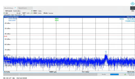
NTNV-n78(3450-3550)-PC2-30-60-H-DFT-QPSK-Inner_1RB_Right t-0.009-0.15-PASS
