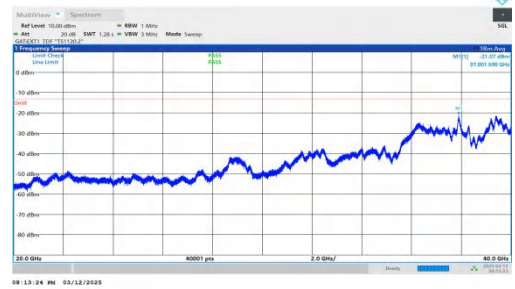
NTNV-n78(3450-3550)-PC2-30-50-H-DFT-BPSK-Inner_1RB_Righ t-20000-40000-PASS
