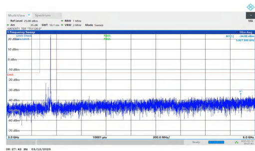
NTNV-n78(3450-3550)-PC2-30-60-M-DFT-QPSK-Inner_1RB_Righ t-3000-6000-PASS
