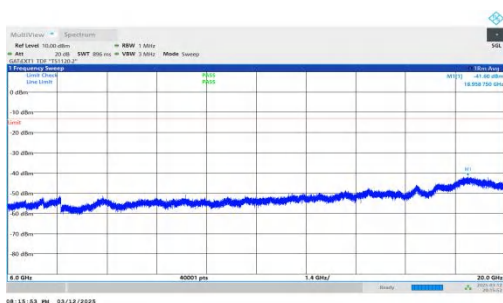
NTNV-n78(3450-3550)-PC2-30-50-H-DFT-QPSK-Inner_1RB_Right ht-6000-20000-PASS
