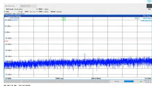
NTNV-n78(3450-3550)-PC2-30-70-L-DFT-QPSK-Inner_1RB_Left- 1000-3000-PASS
