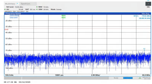
NTNV-n78(3450-3550)-PC2-30-60-L-DFT-BPSK-Inner_1RB_Left- 0.15-30-PASS
