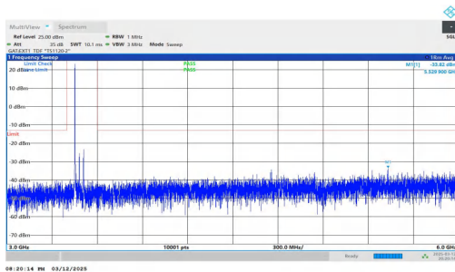
NTNV-n78(3450-3550)-PC2-30-60-L-DFT-QPSK-Inner_1RB_Left -3000-6000-PASS
