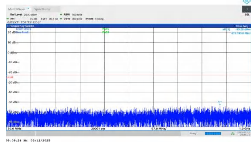
NTNV-n78(3450-3550)-PC2-30-50-M-DFT-QPSK-Inner_1RB_Right t-30-1000-PASS
