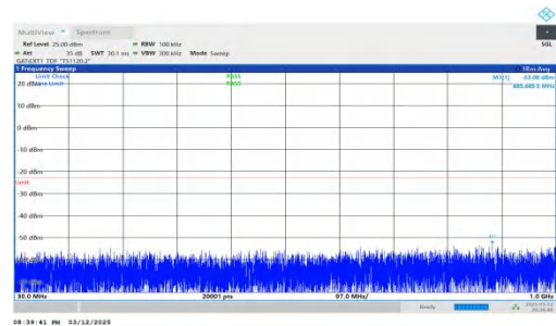
NTNV-n78(3450-3550)-PC2-30-70-L-DFT-QPSK-Inner_1RB_Right -30-1000-PASS
