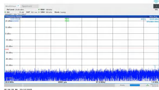
NTNV-n78(3450-3550)-PC2-30-60-M-DFT-BPSK-Inner_1RB_Right t-30-1000-PASS
