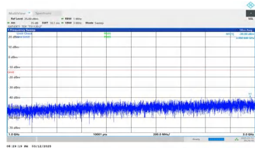
NTNV-n78(3450-3550)-PC2-30-60-H-DFT-BPSK-Inner_1RB_Left 1000-3000-PASS
