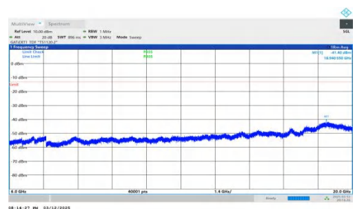
NTNV-n78(3450-3550)-PC2-30-50-H-DFT-QPSK-Inner_1RB_Left- 6000-20000-PASS
