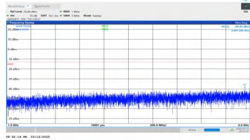
NTNV-n78(3450-3550)-PC2-30-60-H-DFT-QPSK-Inner_1RB_Left 1000-3000-PASS
