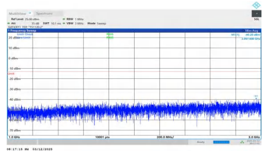
NTNV-n78(3450-3550)-PC2-30-60-L-DFT-BPSK-Inner_1RB_Left- 1000-3000-PASS
