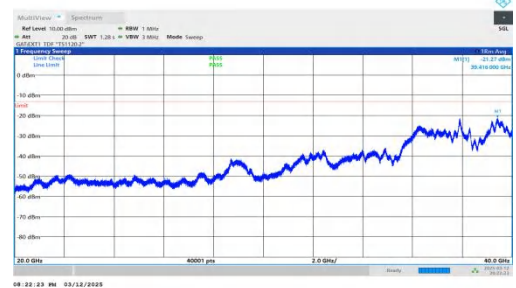
NTNV-n78(3450-3550)-PC2-30-60-L-DFT-QPSK-Inner_1RB_Right -20000-40000-PASS
