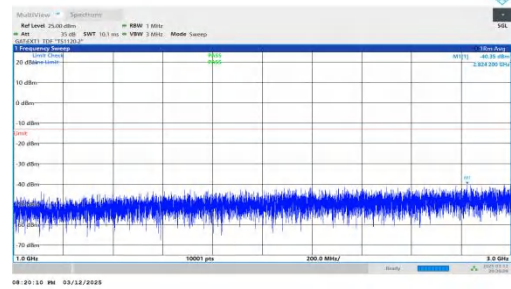
NTNV-n78(3450-3550)-PC2-30-60-L-DFT-QPSK-Inner_1RB_Left- 1000-3000-PASS
