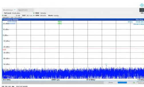
NTVN-n78(3450-3550)-PC2-30-70-L-DFT-BPSK-Inner_1RB_Left- 30-1000-PASS
