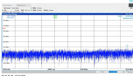
NTNV-n78(3450-3550)-PC2-30-60-M-DFT-BPSK-Inner_1RB_Rig ht-0.15-30-PASS
