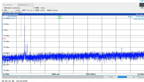
NTNV-n78(3450-3550)-PC2-30-60-M-DFT-QPSK-Inner_1RB_Lef t-3000-6000-PASS
