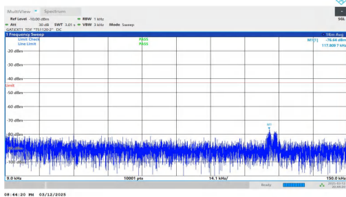
NTNV-n78(3450-3550)-PC2-30-70-M-DFT-QPSK-Inner_1RB_Lef t-0.009-0.15-PASS
