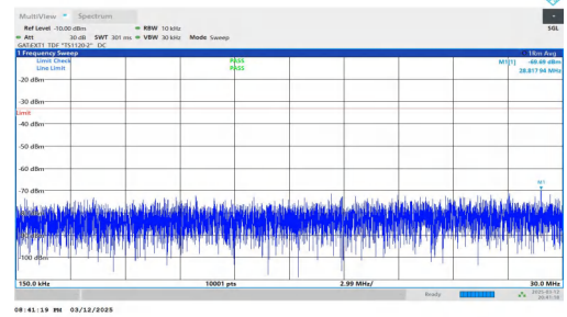
NTNV-n78(3450-3550)-PC2-30-70-M-DFT-BPSK-Inner_1RB_Left 0.15-30-PASS
