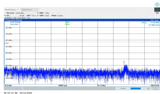
NTNV-n78(3450-3550)-PC2-30-50-M-DFT-QPSK-Inner_1RB_Right t-0.009-0.15-PASS
