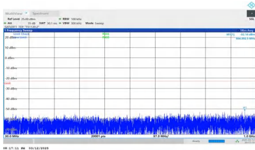
NTNV-n78(3450-3550)-PC2-30-60-L-DFT-BPSK-Inner_1RB_Left- 30-1000-PASS
