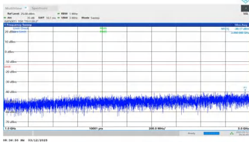
NTNV-n78(3450-3550)-PC2-30-70-L-DFT-BPSK-Inner_1RB_Rig ht-1000-3000-PASS
