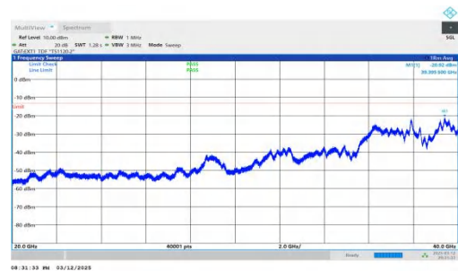
NTNV-n78(3450-3550)-PC2-30-60-H-DFT-BPSK-Inner_1RB_Righ t-20000-40000-PASS
