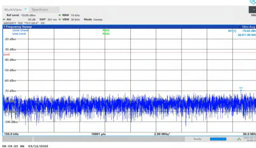
NTNV-n78(3450-3550)-PC2-30-50-M-DFT-QPSK-Inner_1RB_Rig ht-0.15-30-PASS
