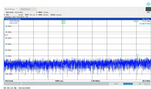
NTVN-n78(3450-3550)-PC2-30-70-L-DFT-BPSK-Inner_1RB_Left- 0.15-30-PASS
