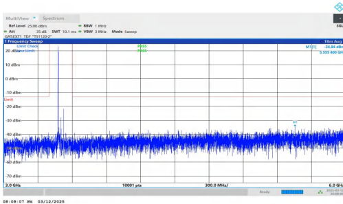
NTNV-n78(3450-3550)-PC2-30-50-M-DFT-QPSK-Inner_1RB_Lef t-3000-6000-PASS
