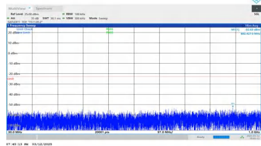
NTNV-n78(3450-3550)-PC2-30-40-L-DFT-QPSK-Inner_1RB_Right -30-1000-PASS
