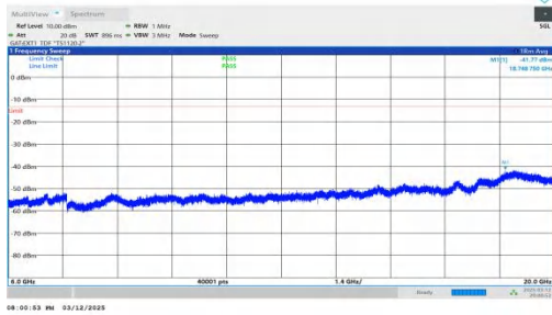
NTNV-n78(3450-3550)-PC2-30-50-L-DFT-BPSK-Inner_1RB_Rig ht-6000-20000-PASS
