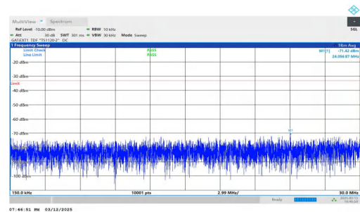
NTNV-n78(3450-3550)-PC2-30-40-M-DFT-BPSK-Inner_1RB_Left- 0.15-30-PASS
