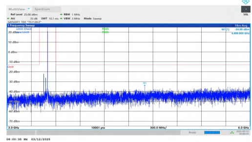
NTNV-n78(3450-3550)-PC2-30-50-L-DFT-BPSK-Inner_1RB_Right-3000-6000-PASS
