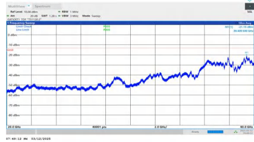
NTNV-n78(3450-3550)-PC2-30-40-M-DFT-BPSK-Inner_1RB_Righ t-20000-40000-PASS
