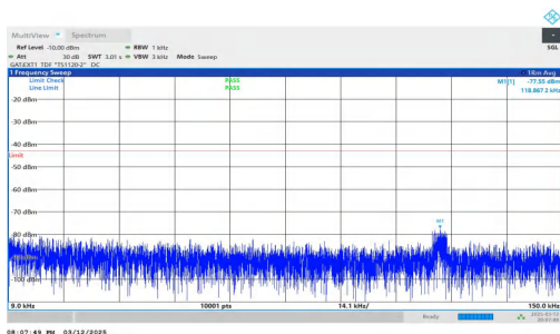
NTNV-n78(3450-3550)-PC2-30-50-M-DFT-QPSK-Inner_1RB_Lef t-0.009-0.15-PASS
