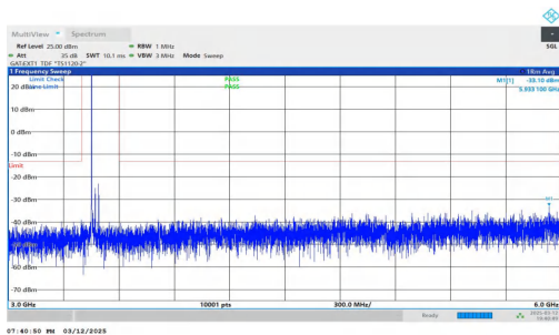
NTNV-n78(3450-3550)-PC2-30-40-L-DFT-BPSK-Inner_1RB_Left- 3000-6000-PASS
