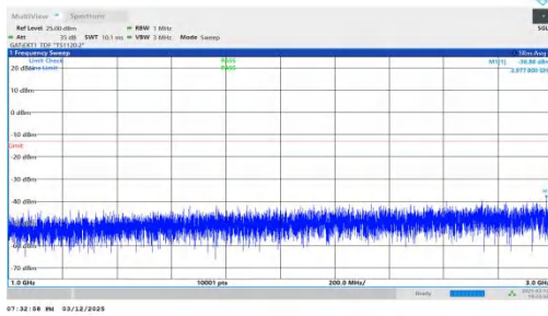
NTNV-n78(3450-3550)-PC2-30-30-M-DFT-QPSK-Inner_1RB_Rig ht-1000-3000-PASS
