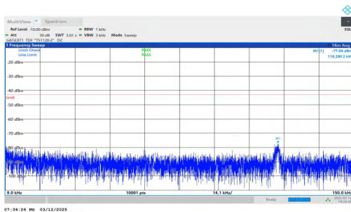
NTNV-n78(3450-3550)-PC2-30-30-H-DFT-BPSK-Inner_1RB_Left -0.009-0.15-PASS
