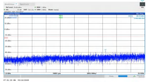
NTNV-n78(3450-3550)-PC2-30-30-M-DFT-QPSK-Inner_1RB_Left- 1000-3000-PASS
