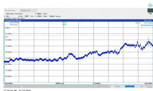
NTNV-n78(3450-3550)-PC2-30-40-M-DFT-QPSK-Inner_1RB_Righ t-20000-40000-PASS
