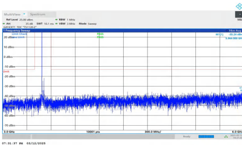
NTNV-n78(3450-3550)-PC2-30-30-M-DFT-QPSK-Inner_1RB_Lef t-3000-6000-PASS
