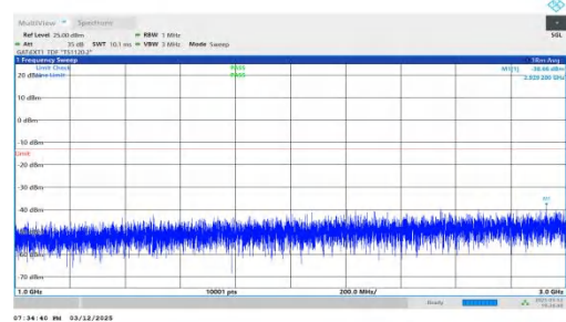
NTNV-n78(3450-3550)-PC2-30-30-H-DFT-BPSK-Inner_1RB_Left- 1000-3000-PASS
