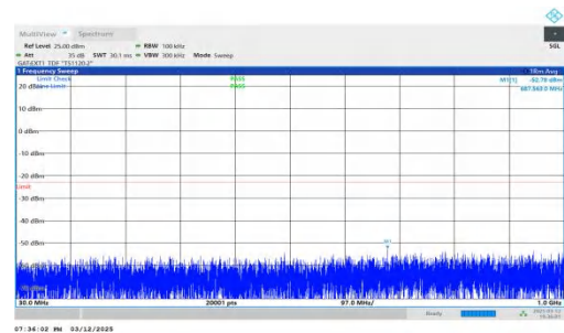
NTNV-n78(3450-3550)-PC2-30-30-H-DFT-BPSK-Inner_1RB_Right t-30-1000-PASS
