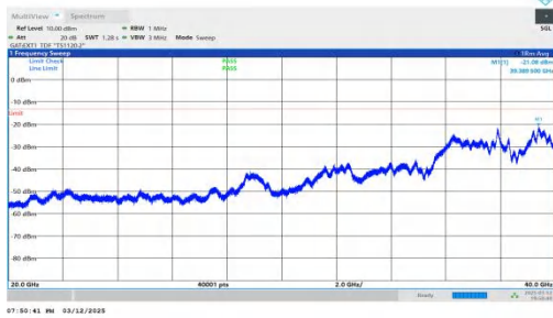
NTNV-n78(3450-3550)-PC2-30-40-M-DFT-QPSK-Inner_1RB_Lef t-20000-40000-PASS
