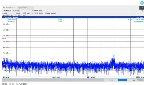
NTNV-n78(3450-3550)-PC2-30-50-L-DFT-QPSK-Inner_1RB_Left -0.009-0.15-PASS
