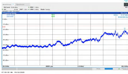
NTNV-n78(3450-3550)-PC2-30-50-L-DFT-BPSK-Inner_1RB_Left-20000-40000-PASS
