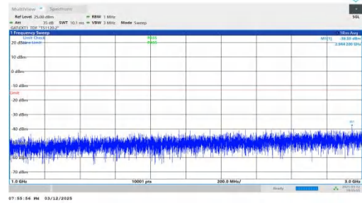
NTNV-n78(3450-3550)-PC2-30-40-H-DFT-QPSK-Inner_1RB_Left 1000-3000-PASS
