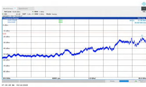
NTNV-n78(3450-3550)-PC2-30-30-H-DFT-BPSK-Inner_1RB_Left -20000-40000-PASS
