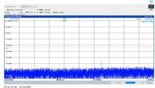
NTNV-n78(3450-3550)-PC2-30-50-L-DFT-BPSK-Inner_1RB_Right-30-1000-PASS
