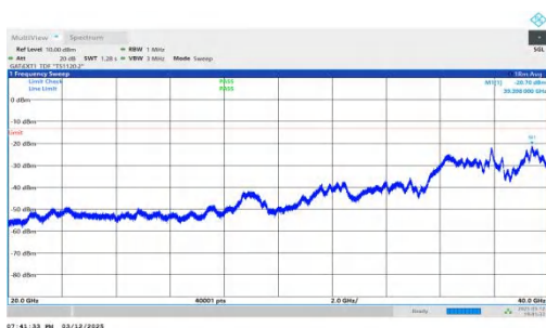
NTNV-n78(3450-3550)-PC2-30-40-L-DFT-BPSK-Inner_1RB_Left- 20000-40000-PASS
