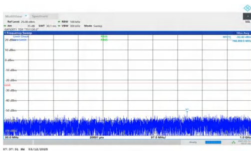
NTNV-n78(3450-3550)-PC2-30-30-H-DFT-QPSK-Inner_1RB_Left -30-1000-PASS
