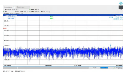
NTNV-n78(3450-3550)-PC2-30-30-H-DFT-QPSK-Inner_1RB_Left- 0.15-30-PASS
