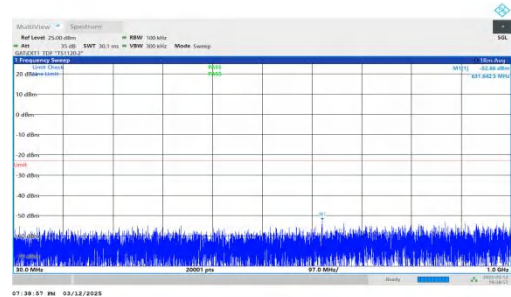
NTNV-n78(3450-3550)-PC2-30-30-H-DFT-QPSK-Inner_1RB_Right t-30-1000-PASS
