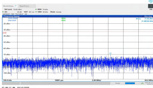
NTNV-n78(3450-3550)-PC2-30-40-M-DFT-BPSK-Inner_1RB_Rig ht-0.15-30-PASS
