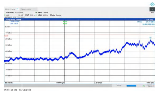
NTNV-n78(3450-3550)-PC2-30-40-H-DFT-BPSK-Inner_1RB_Righ t-20000-40000-PASS
