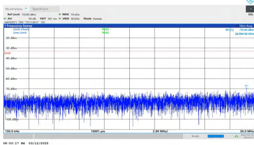
NTNV-n78(3450-3550)-PC2-30-50-L-DFT-QPSK-Inner_1RB_Rig ht-0.15-30-PASS
