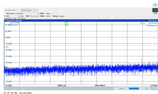
NTNV-n78(3450-3550)-PC2-30-30-H-DFT-QPSK-Inner_1RB_Left- 1000-3000-PASS
