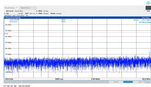
NTNV-n78(3450-3550)-PC2-30-40-M-DFT-QPSK-Inner_1RB_Left- 0.15-30-PASS
