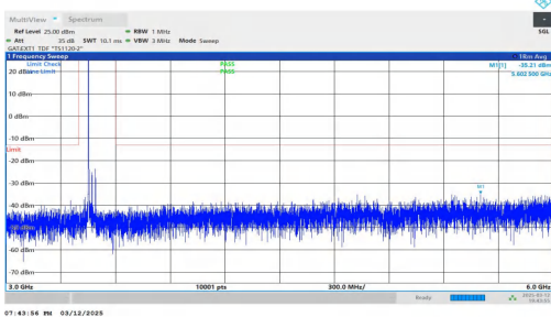
NTNV-n78(3450-3550)-PC2-30-40-L-DFT-QPSK-Inner_1RB_Left -3000-6000-PASS
