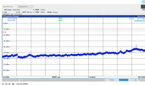
NTNV-n78(3450-3550)-PC2-30-30-M-DFT-QPSK-Inner_1RB_Rig ht-6000-20000-PASS
