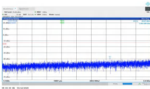
NTNV-n78(3450-3550)-PC2-30-50-M-DFT-BPSK-Inner_1RB_Rig ht-1000-3000-PASS
