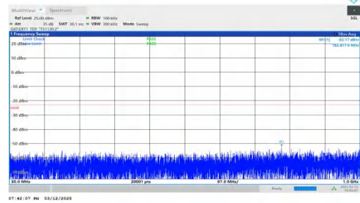
NTNV-n78(3450-3550)-PC2-30-40-L-DFT-BPSK-Inner_1RB_Right -30-1000-PASS
