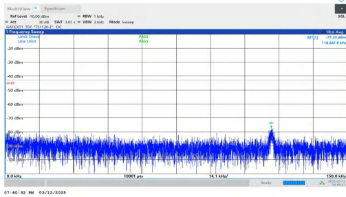
NTNV-n78(3450-3550)-PC2-30-40-L-DFT-BPSK-Inner_1RB_Left- 0.009-0.15-PASS
