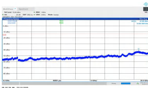
NTNV-n78(3450-3550)-PC2-30-50-M-DFT-BPSK-Inner_1RB_Rig ht-6000-20000-PASS
