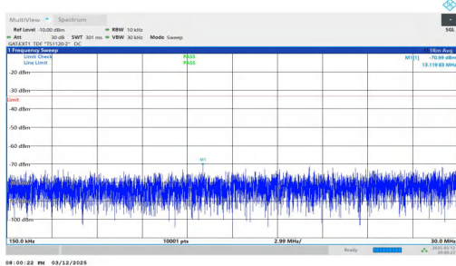
NTNV-n78(3450-3550)-PC2-30-50-L-DFT-BPSK-Inner_1RB_Rig ht-0.15-30-PASS
