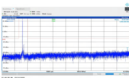
NTNV-n78(3450-3550)-PC2-30-40-M-DFT-QPSK-Inner_1RB_Lef t-3000-6000-PASS
