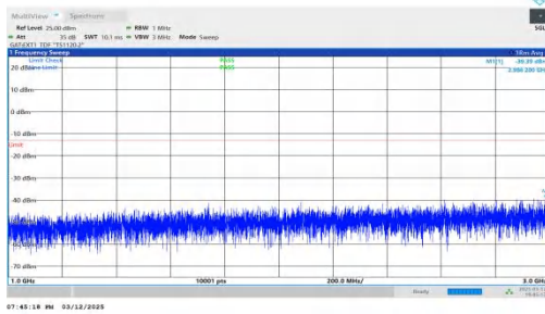
NTNV-n78(3450-3550)-PC2-30-40-L-DFT-QPSK-Inner_1RB_Rig ht-1000-3000-PASS
