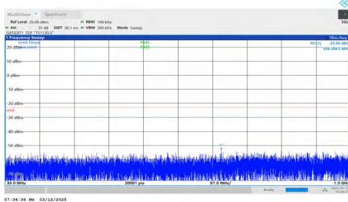
NTNV-n78(3450-3550)-PC2-30-30-H-DFT-BPSK-Inner_1RB_Left -30-1000-PASS
