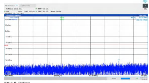
NTNV-n78(3450-3550)-PC2-30-40-M-DFT-BPSK-Inner_1RB_Right t-30-1000-PASS
