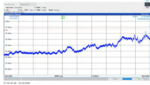
NTNV-n78(3450-3550)-PC2-30-30-H-DFT-BPSK-Inner_1RB_Righ t-20000-40000-PASS
