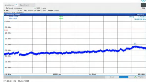
NTNV-n78(3450-3550)-PC2-30-40-L-DFT-QPSK-Inner_1RB_Left- 6000-20000-PASS
