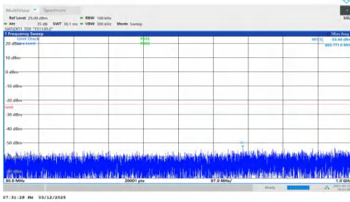
NTNV-n78(3450-3550)-PC2-30-30-M-DFT-QPSK-Inner_1RB_Lef t-30-1000-PASS
