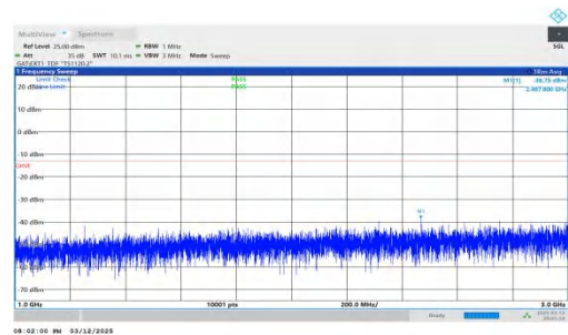
NTNV-n78(3450-3550)-PC2-30-50-L-DFT-QPSK-Inner_1RB_Left- 1000-3000-PASS
