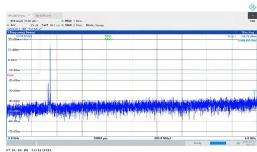
NTNV-n78(3450-3550)-PC2-30-40-M-DFT-QPSK-Inner_1RB_Righ t-3000-6000-PASS
