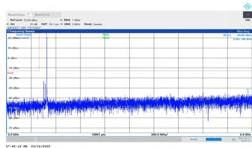
NTNV-n78(3450-3550)-PC2-30-40-L-DFT-BPSK-Inner_1RB_Right -3000-6000-PASS
