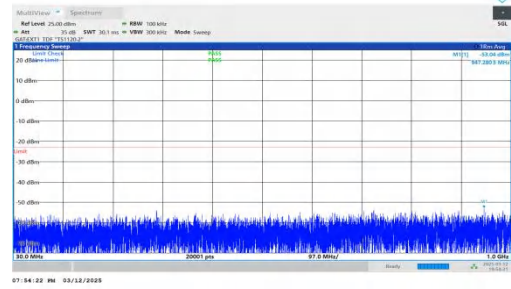
NTNV-n78(3450-3550)-PC2-30-40-H-DFT-BPSK-Inner_1RB_Righ t-30-1000-PASS
