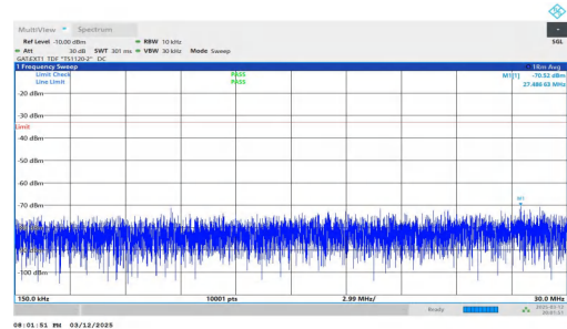
NTNV-n78(3450-3550)-PC2-30-50-L-DFT-QPSK-Inner_1RB_Left- 0.15-30-PASS
