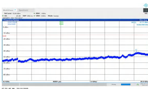
NTNV-n78(3450-3550)-PC2-30-40-M-DFT-QPSK-Inner_1RB_Rig ht-6000-20000-PASS
