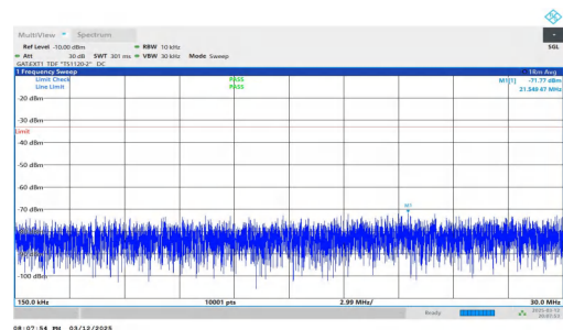
NTNV-n78(3450-3550)-PC2-30-50-M-DFT-QPSK-Inner_1RB_Left- 0.15-30-PASS
