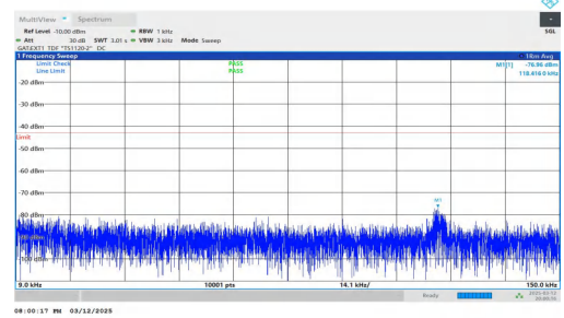
NTNV-n78(3450-3550)-PC2-30-50-L-DFT-BPSK-Inner_1RB_Right-0.009-0.15-PASS
