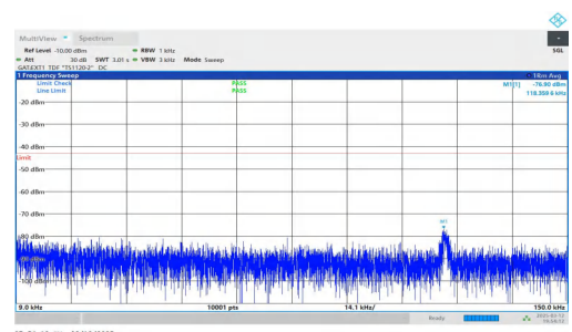
NTNV-n78(3450-3550)-PC2-30-40-H-DFT-BPSK-Inner_1RB_Right t-0.009-0.15-PASS
