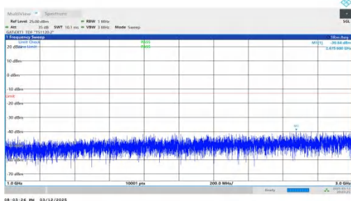
NTNV-n78(3450-3550)-PC2-30-50-L-DFT-QPSK-Inner_1RB_Rig ht-1000-3000-PASS
