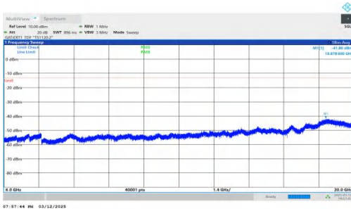
NTNV-n78(3450-3550)-PC2-30-40-H-DFT-QPSK-Inner_1RB_Rig ht-6000-20000-PASS
