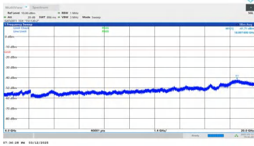
NTNV-n78(3450-3550)-PC2-30-30-H-DFT-BPSK-Inner_1RB_Rig ht-6000-20000-PASS
