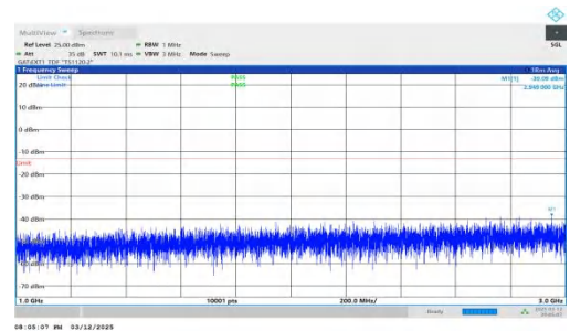
NTNV-n78(3450-3550)-PC2-30-50-M-DFT-BPSK-Inner_1RB_Left 1000-3000-PASS
