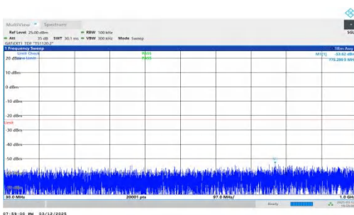
NTNV-n78(3450-3550)-PC2-30-50-L-DFT-BPSK-Inner_1RB_Left- 30-1000-PASS
