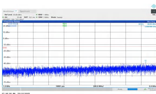
NTNV-n78(3450-3550)-PC2-30-30-H-DFT-BPSK-Inner_1RB_Right ht-1000-3000-PASS
