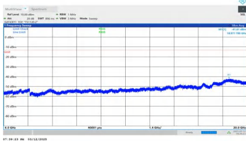
NTNV-n78(3450-3550)-PC2-30-30-H-DFT-QPSK-Inner_1RB_Right ht-6000-20000-PASS
