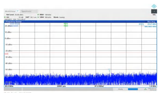
NTNV-n78(3450-3550)-PC2-30-30-M-DFT-QPSK-Inner_1RB_Right t-30-1000-PASS
