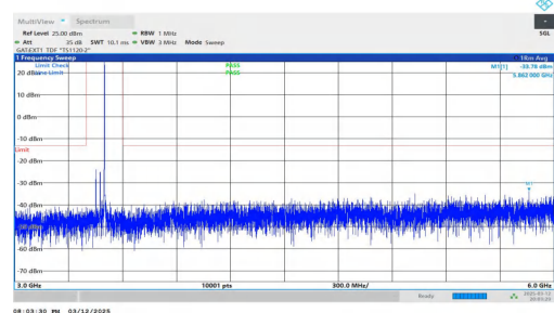
NTNV-n78(3450-3550)-PC2-30-50-L-DFT-QPSK-Inner_1RB_Right -3000-6000-PASS
