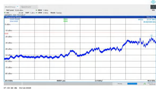
NTNV-n78(3450-3550)-PC2-30-30-M-DFT-QPSK-Inner_1RB_Righ t-20000-40000-PASS
