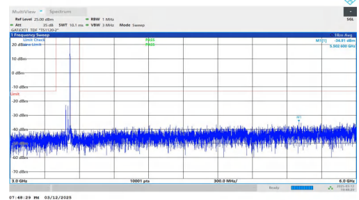
NTNV-n78(3450-3550)-PC2-30-40-M-DFT-BPSK-Inner_1RB_Right t-3000-6000-PASS
