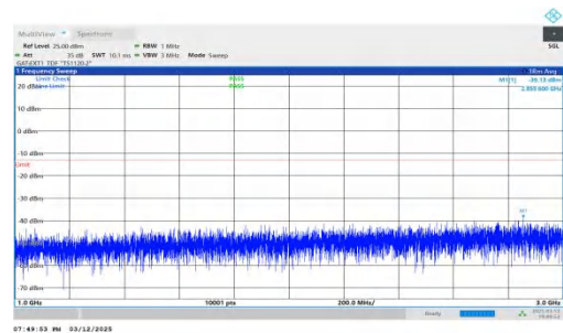
NTNV-n78(3450-3550)-PC2-30-40-M-DFT-QPSK-Inner_1RB_Left- 1000-3000-PASS
