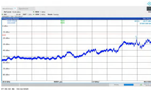
NTNV-n78(3450-3550)-PC2-30-40-H-DFT-QPSK-Inner_1RB_Left -20000-40000-PASS
