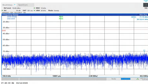
NTNV-n78(3450-3550)-PC2-30-40-L-DFT-QPSK-Inner_1RB_Rig ht-0.15-30-PASS
