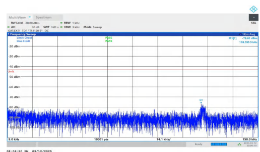
NTNV-n78(3450-3550)-PC2-30-50-M-DFT-BPSK-Inner_1RB_Right t-0.009-0.15-PASS
