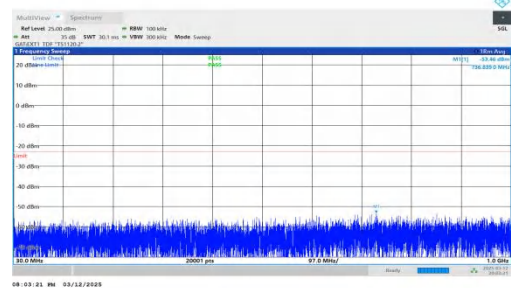
NTNV-n78(3450-3550)-PC2-30-50-L-DFT-QPSK-Inner_1RB_Right -30-1000-PASS
