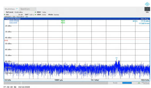
NTNV-n78(3450-3550)-PC2-30-30-M-DFT-QPSK-Inner_1RB_Right t-0.009-0.15-PASS
