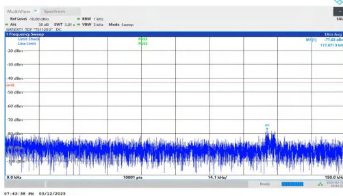
NTNV-n78(3450-3550)-PC2-30-40-L-DFT-QPSK-Inner_1RB_Left -0.009-0.15-PASS
