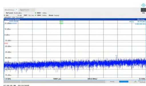
NTNV-n78(3450-3550)-PC2-30-50-L-DFT-BPSK-Inner_1RB_Left- 1000-3000-PASS
