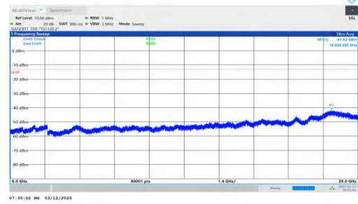
NTNV-n78(3450-3550)-PC2-30-30-H-DFT-BPSK-Inner_1RB_Left 6000-20000-PASS
