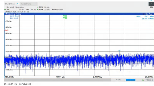
NTNV-n78(3450-3550)-PC2-30-40-L-DFT-BPSK-Inner_1RB_Left- 0.15-30-PASS
