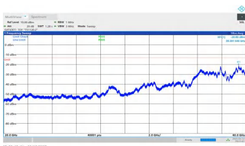
NTNV-n78(3450-3550)-PC2-30-40-H-DFT-BPSK-Inner_1RB_Left -20000-40000-PASS
