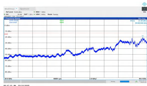
NTNV-n78(3450-3550)-PC2-30-50-M-DFT-BPSK-Inner_1RB_Righ t-20000-40000-PASS
