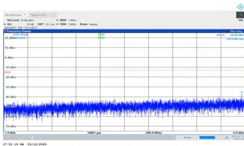
NTNV-n78(3450-3550)-PC2-30-40-M-DFT-QPSK-Inner_1RB_Rig ht-1000-3000-PASS
