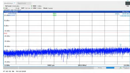
NTNV-n78(3450-3550)-PC2-30-40-L-DFT-QPSK-Inner_1RB_Left- 1000-3000-PASS
