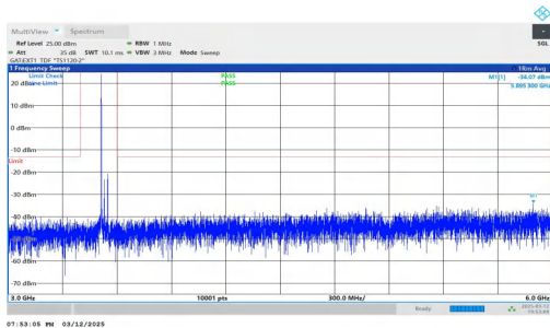
NTNV-n78(3450-3550)-PC2-30-40-H-DFT-BPSK-Inner_1RB_Left -3000-6000-PASS
