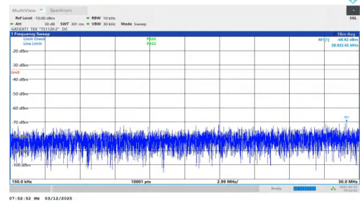
NTNV-n78(3450-3550)-PC2-30-40-H-DFT-BPSK-Inner_1RB_Left- 0.15-30-PASS
