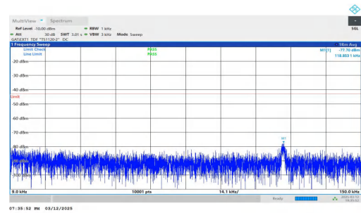
NTNV-n78(3450-3550)-PC2-30-30-H-DFT-BPSK-Inner_1RB_Right t-0.009-0.15-PASS
