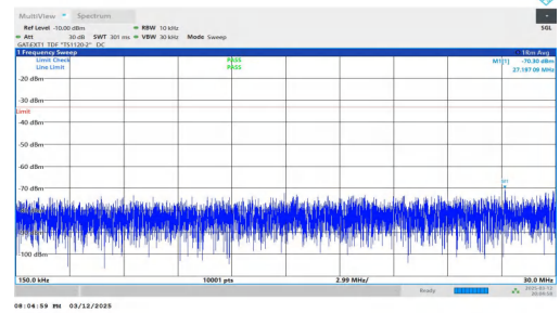
NTNV-n78(3450-3550)-PC2-30-50-M-DFT-BPSK-Inner_1RB_Left 0.15-30-PASS
