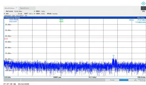
NTNV-n78(3450-3550)-PC2-30-40-H-DFT-QPSK-Inner_1RB_Right t-0.009-0.15-PASS
