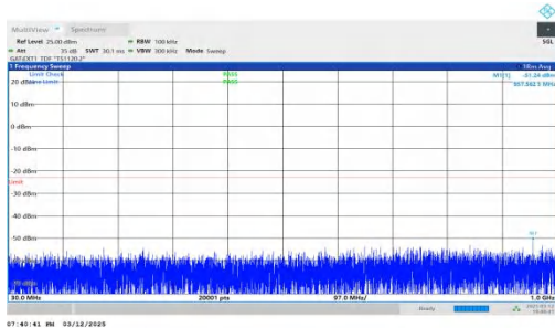
NTNV-n78(3450-3550)-PC2-30-40-L-DFT-BPSK-Inner_1RB_Left- 30-1000-PASS
