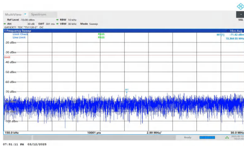
NTNV-n78(3450-3550)-PC2-30-40-M-DFT-QPSK-Inner_1RB_Rig ht-0.15-30-PASS
