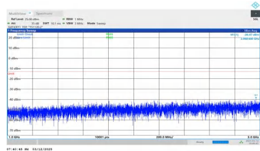
NTNV-n78(3450-3550)-PC2-30-40-L-DFT-BPSK-Inner_1RB_Left- 1000-3000-PASS
