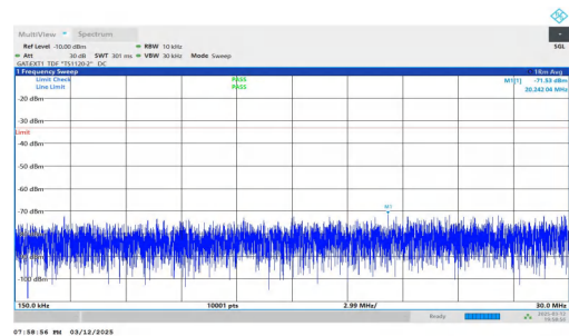
NTNV-n78(3450-3550)-PC2-30-50-L-DFT-BPSK-Inner_1RB_Left- 0.15-30-PASS
