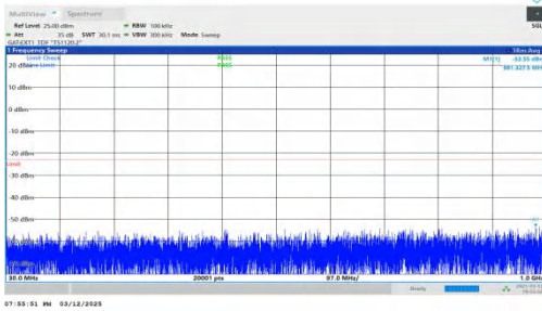
NTNV-n78(3450-3550)-PC2-30-40-H-DFT-QPSK-Inner_1RB_Left -30-1000-PASS
