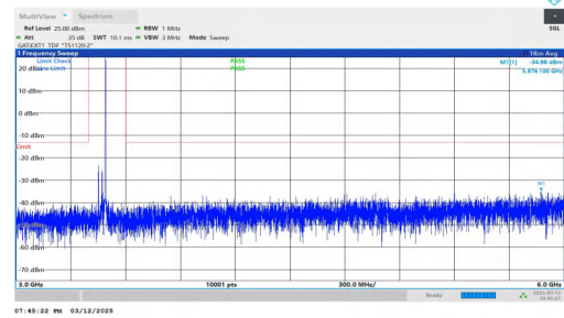
NTNV-n78(3450-3550)-PC2-30-40-L-DFT-QPSK-Inner_1RB_Right -3000-6000-PASS
