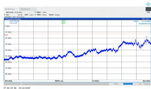
NTNV-n78(3450-3550)-PC2-30-40-L-DFT-BPSK-Inner_1RB_Right -20000-40000-PASS
