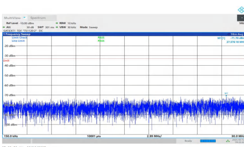
NTNV-n78(3450-3550)-PC2-30-30-M-DFT-QPSK-Inner_1RB_Rig ht-0.15-30-PASS
