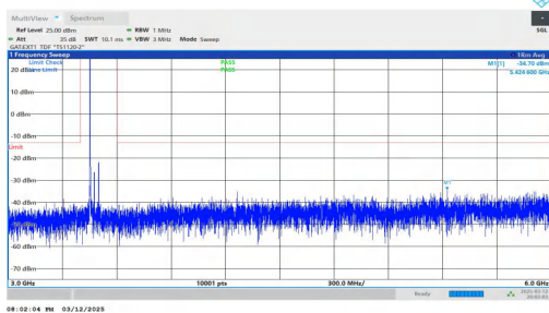
NTNV-n78(3450-3550)-PC2-30-50-L-DFT-QPSK-Inner_1RB_Left -3000-6000-PASS
