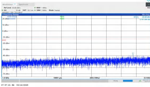
NTNV-n78(3450-3550)-PC2-30-40-H-DFT-QPSK-Inner_1RB_Rig ht-1000-3000-PASS
