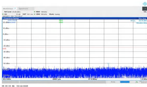
NTNV-n78(3450-3550)-PC2-30-50-M-DFT-BPSK-Inner_1RB_Left -30-1000-PASS
