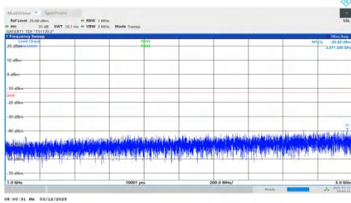
NTNV-n78(3450-3550)-PC2-30-50-L-DFT-BPSK-Inner_1RB_Rig ht-1000-3000-PASS
