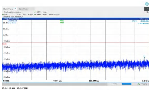
NTNV-n78(3450-3550)-PC2-30-40-H-DFT-BPSK-Inner_1RB_Rig ht-1000-3000-PASS
