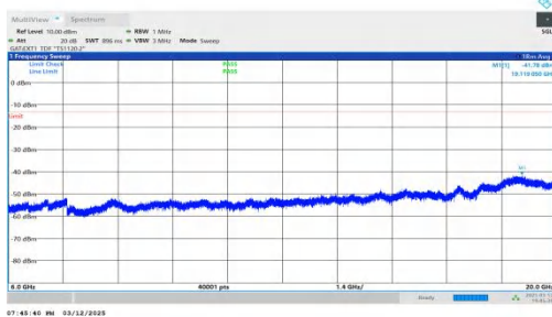
NTNV-n78(3450-3550)-PC2-30-40-L-DFT-QPSK-Inner_1RB_Rig ht-6000-20000-PASS
