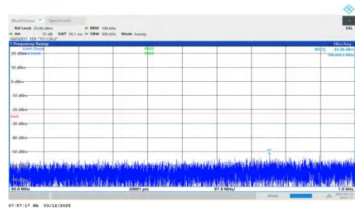
NTNV-n78(3450-3550)-PC2-30-40-H-DFT-QPSK-Inner_1RB_Right t-30-1000-PASS
