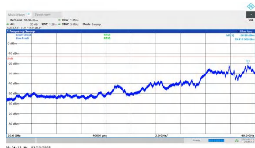
NTNV-n78(3450-3550)-PC2-30-50-L-DFT-QPSK-Inner_1RB_Right -20000-40000-PASS
