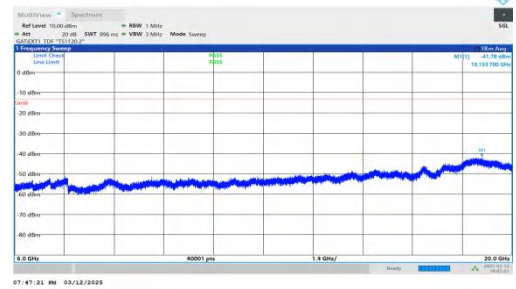
NTNV-n78(3450-3550)-PC2-30-40-M-DFT-BPSK-Inner_1RB_Left 6000-20000-PASS
