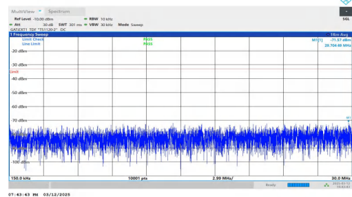
NTNV-n78(3450-3550)-PC2-30-40-L-DFT-QPSK-Inner_1RB_Left- 0.15-30-PASS
