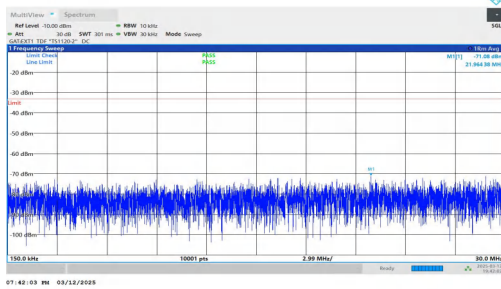
NTNV-n78(3450-3550)-PC2-30-40-L-DFT-BPSK-Inner_1RB_Rig ht-0.15-30-PASS
