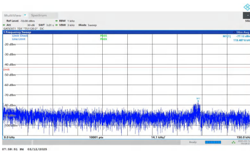
NTNV-n78(3450-3550)-PC2-30-50-L-DFT-BPSK-Inner_1RB_Left- 0.009-0.15-PASS
