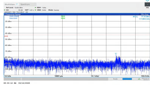
NTNV-n78(3450-3550)-PC2-30-50-L-DFT-QPSK-Inner_1RB_Right -0.009-0.15-PASS
