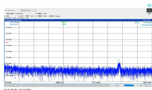
NTNV-n78(3450-3550)-PC2-30-40-L-DFT-BPSK-Inner_1RB_Right -0.009-0.15-PASS
