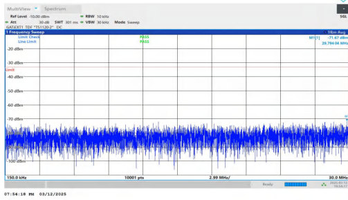
NTNV-n78(3450-3550)-PC2-30-40-H-DFT-BPSK-Inner_1RB_Rig ht-0.15-30-PASS
