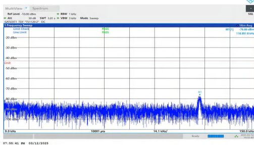
NTNV-n78(3450-3550)-PC2-30-40-H-DFT-QPSK-Inner_1RB_Left -0.009-0.15-PASS
