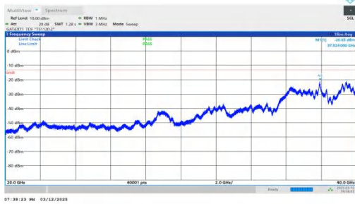
NTNV-n78(3450-3550)-PC2-30-30-H-DFT-QPSK-Inner_1RB_Left -20000-40000-PASS
