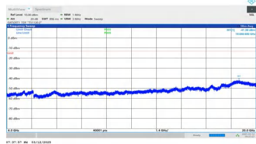
NTNV-n78(3450-3550)-PC2-30-30-H-DFT-QPSK-Inner_1RB_Left- 6000-20000-PASS
