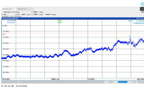
NTNV-n78(3450-3550)-PC2-30-30-M-DFT-QPSK-Inner_1RB_Lef t-20000-40000-PASS
