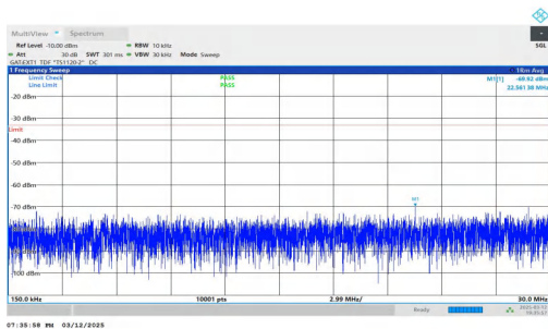
NTNV-n78(3450-3550)-PC2-30-30-H-DFT-BPSK-Inner_1RB_Right ht-0.15-30-PASS
