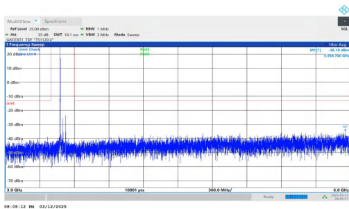
NTNV-n78(3450-3550)-PC2-30-50-M-DFT-BPSK-Inner_1RB_Left -3000-6000-PASS
