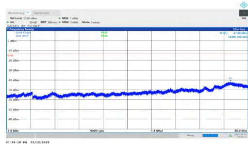
NTNV-n78(3450-3550)-PC2-30-40-H-DFT-QPSK-Inner_1RB_Left 6000-20000-PASS
