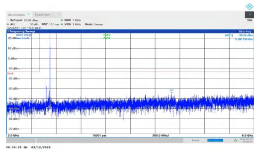
NTNV-n78(3450-3550)-PC2-30-50-M-DFT-BPSK-Inner_1RB_Righ t-3000-6000-PASS
