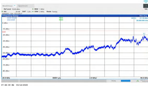
NTNV-n78(3450-3550)-PC2-30-40-L-DFT-QPSK-Inner_1RB_Left -20000-40000-PASS
