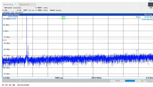
NTNV-n78(3450-3550)-PC2-30-40-M-DFT-BPSK-Inner_1RB_Left -3000-6000-PASS
