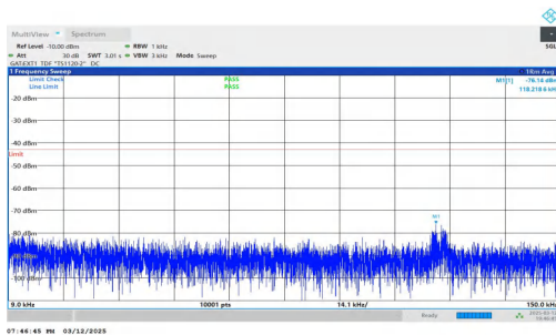
NTNV-n78(3450-3550)-PC2-30-40-M-DFT-BPSK-Inner_1RB_Left -0.009-0.15-PASS
