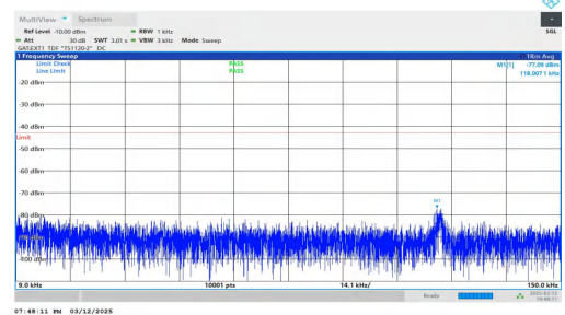
NTNV-n78(3450-3550)-PC2-30-40-M-DFT-BPSK-Inner_1RB_Right t-0.009-0.15-PASS
