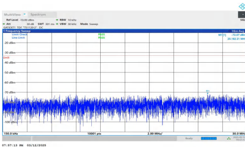
NTNV-n78(3450-3550)-PC2-30-40-H-DFT-QPSK-Inner_1RB_Rig ht-0.15-30-PASS
