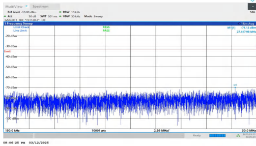
NTNV-n78(3450-3550)-PC2-30-50-M-DFT-BPSK-Inner_1RB_Rig ht-0.15-30-PASS
