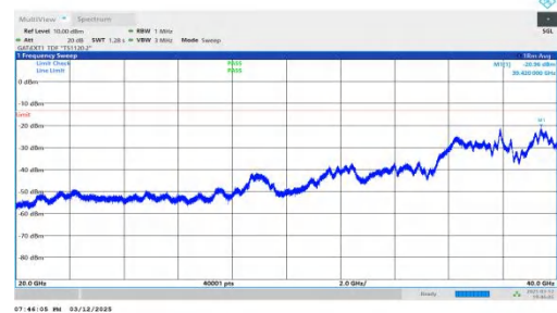
NTNV-n78(3450-3550)-PC2-30-40-L-DFT-QPSK-Inner_1RB_Right -20000-40000-PASS
