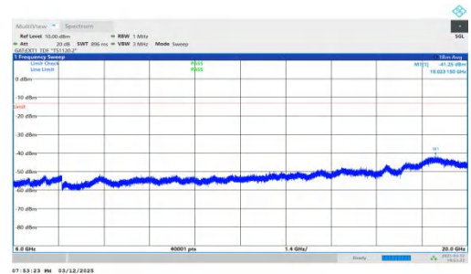
NTNV-n78(3450-3550)-PC2-30-40-H-DFT-BPSK-Inner_1RB_Left- 6000-20000-PASS
