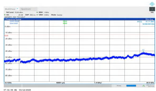
NTNV-n78(3450-3550)-PC2-30-30-M-DFT-QPSK-Inner_1RB_Left- 6000-20000-PASS
