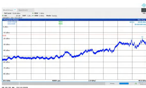
NTNV-n78(3450-3550)-PC2-30-50-M-DFT-BPSK-Inner_1RB_Left -20000-40000-PASS
