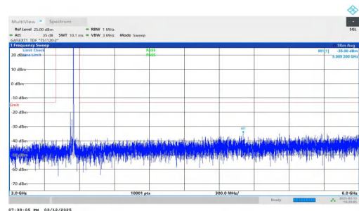
NTNV-n78(3450-3550)-PC2-30-30-H-DFT-QPSK-Inner_1RB_Right t-3000-6000-PASS
