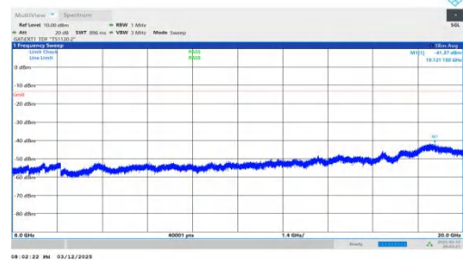
NTNV-n78(3450-3550)-PC2-30-50-L-DFT-QPSK-Inner_1RB_Left- 6000-20000-PASS
