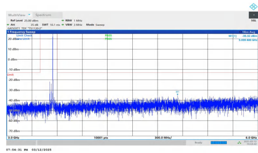
NTNV-n78(3450-3550)-PC2-30-40-H-DFT-BPSK-Inner_1RB_Righ t-3000-6000-PASS
