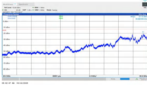
NTNV-n78(3450-3550)-PC2-30-50-L-DFT-QPSK-Inner_1RB_Left -20000-40000-PASS
