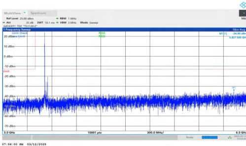
NTNV-n78(3450-3550)-PC2-30-40-H-DFT-QPSK-Inner_1RB_Left -3000-6000-PASS
