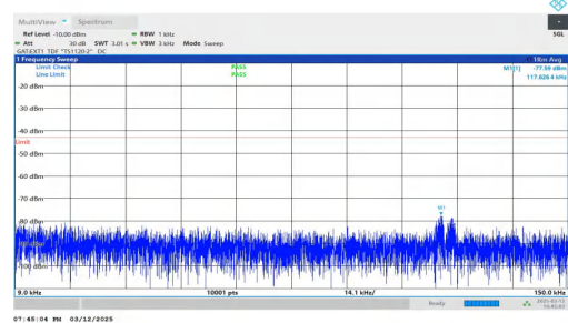
NTNV-n78(3450-3550)-PC2-30-40-L-DFT-QPSK-Inner_1RB_Right -0.009-0.15-PASS
