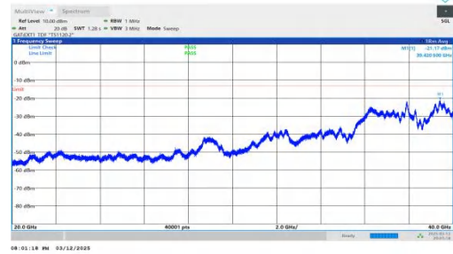
NTNV-n78(3450-3550)-PC2-30-50-L-DFT-BPSK-Inner_1RB_Right -20000-40000-PASS
