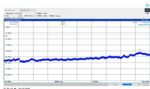
NTNV-n78(3450-3550)-PC2-30-40-M-DFT-QPSK-Inner_1RB_Left- 6000-20000-PASS
