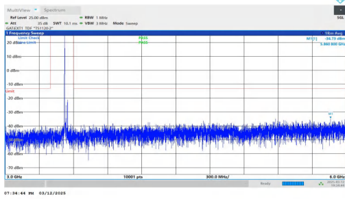
NTNV-n78(3450-3550)-PC2-30-30-H-DFT-BPSK-Inner_1RB_Left -3000-6000-PASS
