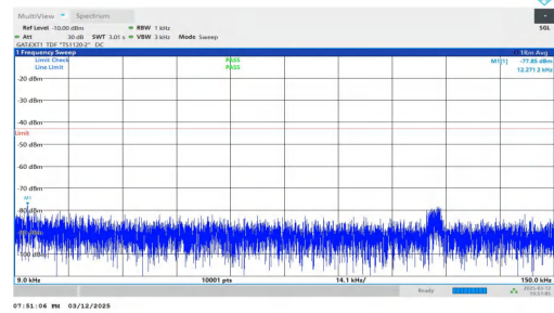
NTNV-n78(3450-3550)-PC2-30-40-M-DFT-QPSK-Inner_1RB_Righ t-0.009-0.15-PASS
