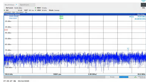
NTNV-n78(3450-3550)-PC2-30-40-H-DFT-QPSK-Inner_1RB_Left 0.15-30-PASS
