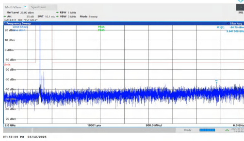
NTNV-n78(3450-3550)-PC2-30-50-L-DFT-BPSK-Inner_1RB_Left-3000-6000-PASS
