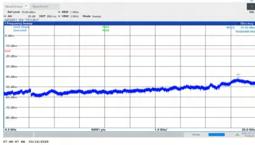
NTNV-n78(3450-3550)-PC2-30-40-M-DFT-BPSK-Inner_1RB_Rig ht-6000-20000-PASS
