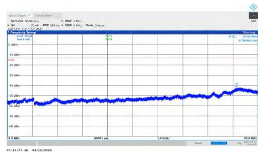
NTNV-n78(3450-3550)-PC2-30-40-L-DFT-BPSK-Inner_1RB_Left- 6000-20000-PASS
