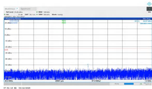
NTNV-n78(3450-3550)-PC2-30-40-M-DFT-QPSK-Inner_1RB_Righ t-30-1000-PASS
