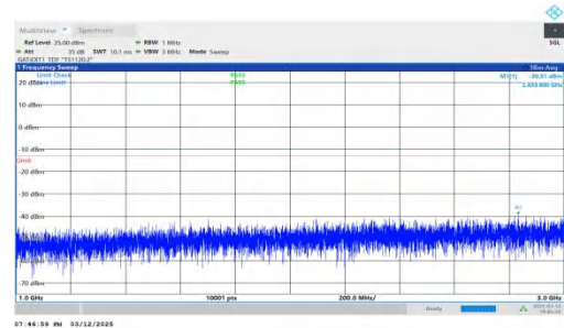
NTNV-n78(3450-3550)-PC2-30-40-M-DFT-BPSK-Inner_1RB_Left- 1000-3000-PASS
