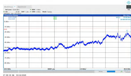
NTNV-n78(3450-3550)-PC2-30-40-H-DFT-QPSK-Inner_1RB_Righ t-20000-40000-PASS
