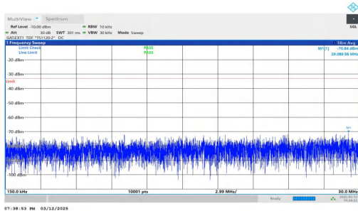
NTNV-n78(3450-3550)-PC2-30-30-H-DFT-QPSK-Inner_1RB_Right ht.0.15-30-PASS
