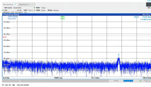
NTNV-n78(3450-3550)-PC2-30-40-H-DFT-BPSK-Inner_1RB_Left -0.009-0.15-PASS
