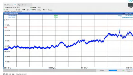
NTNV-n78(3450-3550)-PC2-30-30-H-DFT-QPSK-Inner_1RB_Right t-20000-40000-PASS
