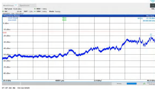
NTNV-n78(3450-3550)-PC2-30-40-M-DFT-BPSK-Inner_1RB_Left -20000-40000-PASS
