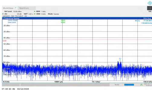
NTNV-n78(3450-3550)-PC2-30-40-M-DFT-QPSK-Inner_1RB_Lef t-0.009-0.15-PASS
