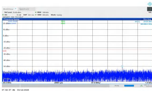
NTNV-n78(3450-3550)-PC2-30-40-H-DFT-BPSK-Inner_1RB_Left -30-1000-PASS
