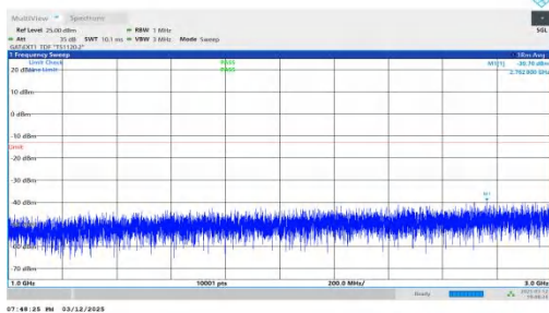
NTNV-n78(3450-3550)-PC2-30-40-M-DFT-BPSK-Inner_1RB_Rig ht-1000-3000-PASS
