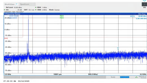
NTNV-n78(3450-3550)-PC2-30-30-M-DFT-QPSK-Inner_1RB_Righ t-3000-6000-PASS
