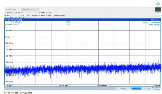
NTNV-n78(3450-3550)-PC2-30-40-H-DFT-BPSK-Inner_1RB_Left- 1000-3000-PASS
