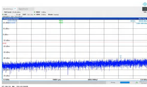
NTNV-n78(3450-3550)-PC2-30-30-H-DFT-QPSK-Inner_1RB_Right ht-1000-3000-PASS
