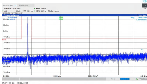
NTNV-n78(3450-3550)-PC2-30-30-H-DFT-QPSK-Inner_1RB_Left -3000-6000-PASS
