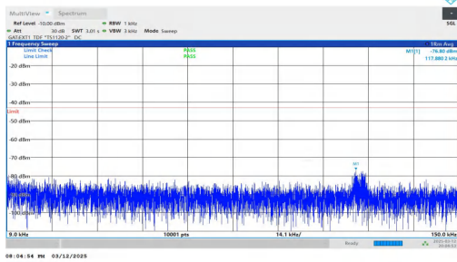
NTNV-n78(3450-3550)-PC2-30-50-M-DFT-BPSK-Inner_1RB_Left -0.009-0.15-PASS
