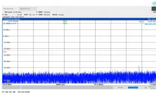
NTNV-n78(3450-3550)-PC2-30-40-M-DFT-BPSK-Inner_1RB_Left -30-1000-PASS
