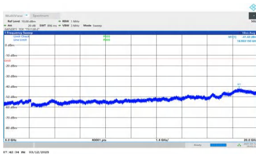
NTNV-n78(3450-3550)-PC2-30-40-L-DFT-BPSK-Inner_1RB_Rig ht-6000-20000-PASS
