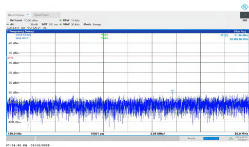
NTNV-n78(3450-3550)-PC2-30-30-H-DFT-BPSK-Inner_1RB_Left- 0.15-30-PASS
