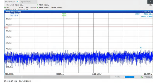
NTNV-n78(3450-3550)-PC2-30-20-L-DFT-BPSK-Inner_1RB_Left- 0.15-30-PASS
