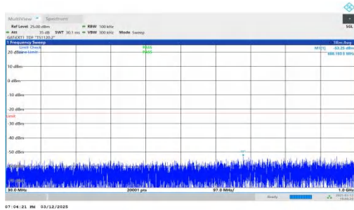
NTNV-n78(3450-3550)-PC2-30-20-L-DFT-BPSK-Inner_1RB_Left- 30-1000-PASS
