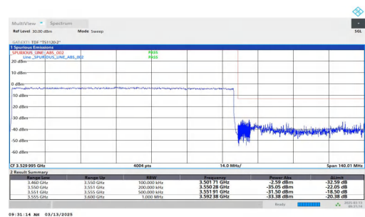
NTNV-n78(3450-3550)-PC2-30-90-H-DFT-BPSK-Outer_Full-PASS
