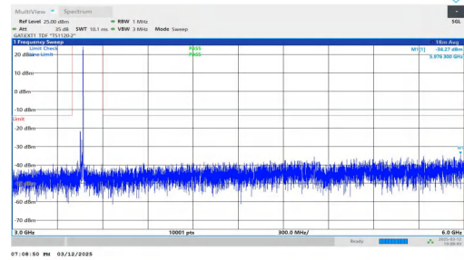
NTNV-n78(3450-3550)-PC2-30-20-L-DFT-QPSK-Inner_1RB_Right -3000-6000-PASS
