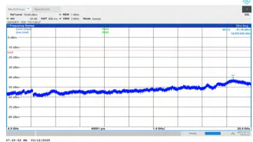
NTNV-n78(3450-3550)-PC2-30-30-L-DFT-QPSK-Inner_1RB_Left- 6000-20000-PASS
