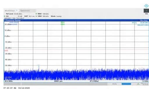
NTNV-n78(3450-3550)-PC2-30-20-H-DFT-QPSK-Inner_1RB_Right t-30-1000-PASS
