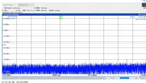
NTNV-n78(3450-3550)-PC2-30-20-M-DFT-BPSK-Inner_1RB_Left -30-1000-PASS
