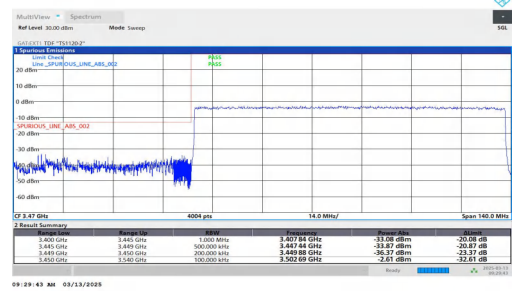
NTNV-n78(3450-3550)-PC2-30-90-L-DFT-BPSK-Outer_Full-PASS
