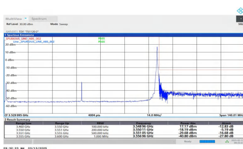
NTNV-n78(3450-3550)-PC2-30-90-H-DFT-QPSK-Edge_1RB_Right-PASS
