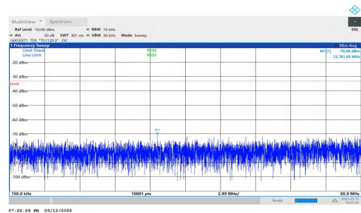
NTNV-n78(3450-3550)-PC2-30-30-L-DFT-BPSK-Inner_1RB_Left- 0.15-30-PASS
