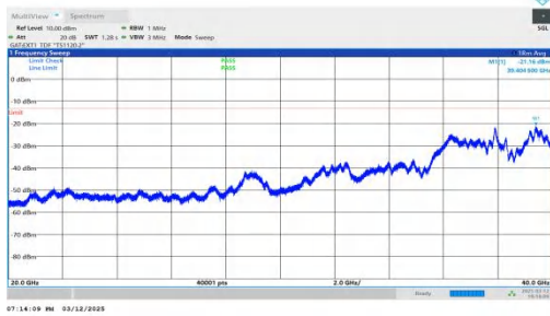
NTNV-n78(3450-3550)-PC2-30-20-M-DFT-QPSK-Inner_1RB_Lef t-20000-40000-PASS
