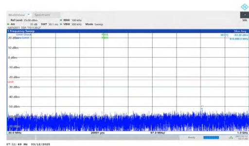
NTNV-n78(3450-3550)-PC2-30-20-M-DFT-BPSK-Inner_1RB_Right t-30-1000-PASS
