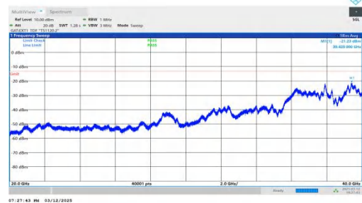
NTNV-n78(3450-3550)-PC2-30-30-L-DFT-QPSK-Inner_1RB_Right -20000-40000-PASS
