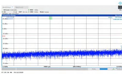
NTNV-n78(3450-3550)-PC2-30-30-M-DFT-BPSK-Inner_1RB_Rig ht-1000-3000-PASS
