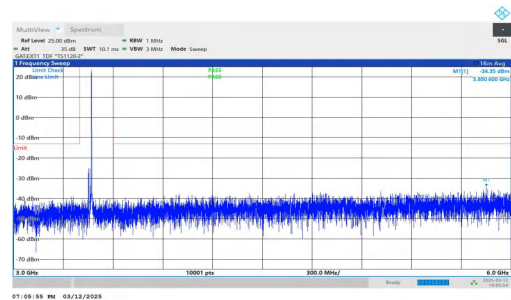
NTNV-n78(3450-3550)-PC2-30-20-L-DFT-BPSK-Inner_1RB_Right -3000-6000-PASS
