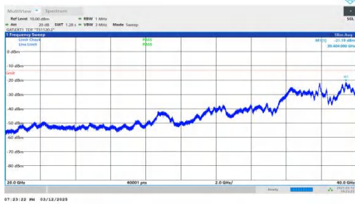
NTNV-n78(3450-3550)-PC2-30-30-L-DFT-BPSK-Inner_1RB_Left-20000-40000-PASS
