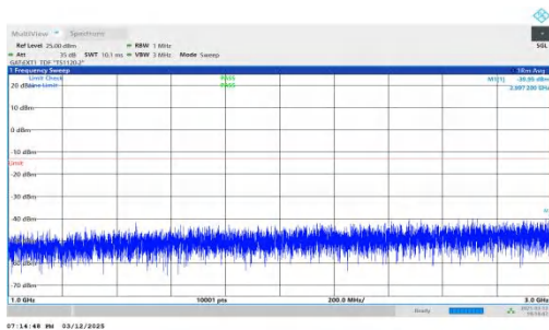
NTNV-n78(3450-3550)-PC2-30-20-M-DFT-QPSK-Inner_1RB_Rig ht-1000-3000-PASS
