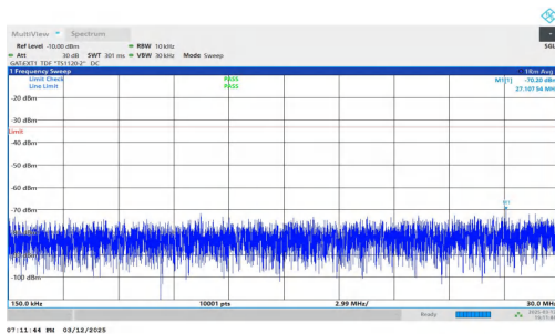
NTNV-n78(3450-3550)-PC2-30-20-M-DFT-BPSK-Inner_1RB_Rig ht-0.15-30-PASS
