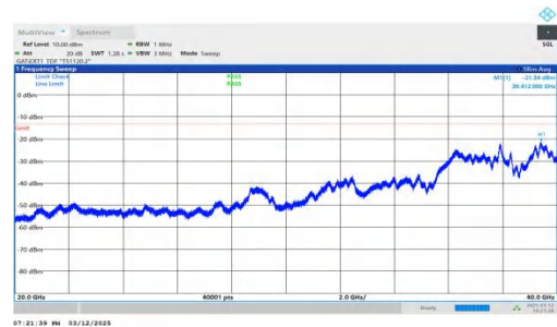
NTNV-n78(3450-3550)-PC2-30-20-H-DFT-QPSK-Inner_1RB_Righ t-20000-40000-PASS
