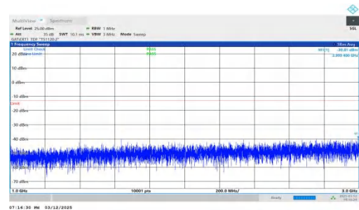
NTNV-n78(3450-3550)-PC2-30-20-H-DFT-BPSK-Inner_1RB_Left 1000-3000-PASS
