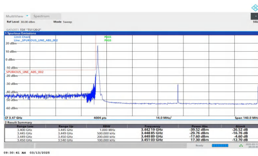
NTNV-n78(3450-3550)-PC2-30-90-L-DFT-QPSK-Edge_1RB_Left-PASS
