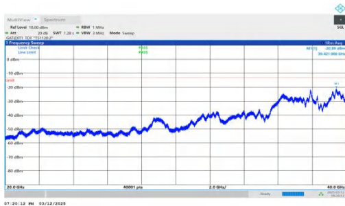
NTNV-n78(3450-3550)-PC2-30-20-H-DFT-QPSK-Inner_1RB_Left -20000-40000-PASS
