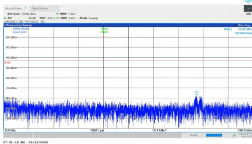
NTNV-n78(3450-3550)-PC2-30-30-M-DFT-QPSK-Inner_1RB_Lef t-0.009-0.15-PASS
