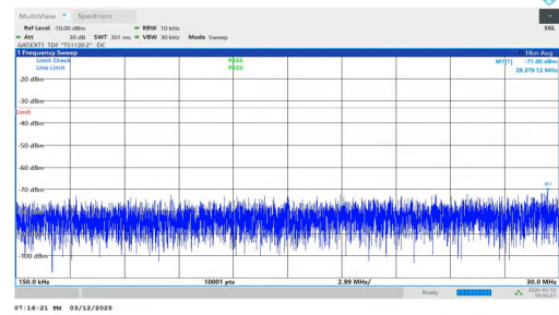
NTNV-n78(3450-3550)-PC2-30-20-H-DFT-BPSK-Inner_1RB_Left 0.15-30-PASS
