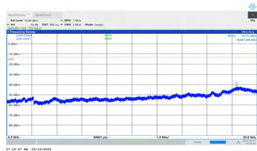
NTNV-n78(3450-3550)-PC2-30-20-H-DFT-QPSK-Inner_1RB_Left 6000-20000-PASS
