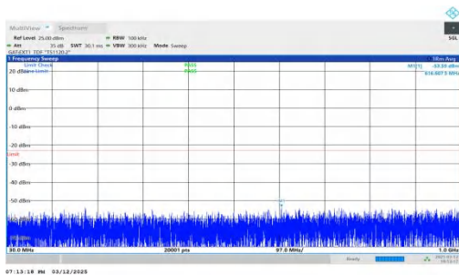
NTNV-n78(3450-3550)-PC2-30-20-M-DFT-QPSK-Inner_1RB_Lef t-30-1000-PASS
