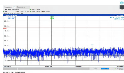
NTNV-n78(3450-3550)-PC2-30-20-M-DFT-BPSK-Inner_1RB_Left- 0.15-30-PASS
