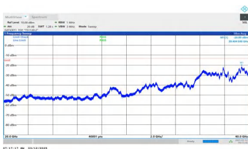
NTNV-n78(3450-3550)-PC2-30-20-H-DFT-BPSK-Inner_1RB_Left -20000-40000-PASS
