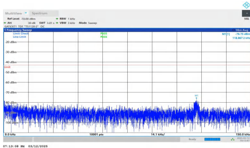
NTNV-n78(3450-3550)-PC2-30-20-M-DFT-QPSK-Inner_1RB_Lef t-0.009-0.15-PASS
