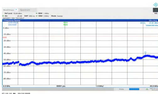
NTNV-n78(3450-3550)-PC2-30-20-M-DFT-QPSK-Inner_1RB_Rig ht-6000-20000-PASS
