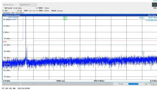
NTNV-n78(3450-3550)-PC2-30-30-L-DFT-BPSK-Inner_1RB_Left-3000-6000-PASS
