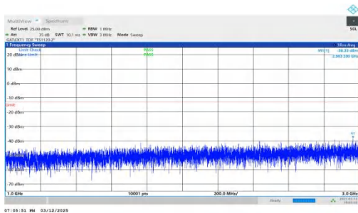
NTNV-n78(3450-3550)-PC2-30-20-L-DFT-BPSK-Inner_1RB_Rig ht-1000-3000-PASS
