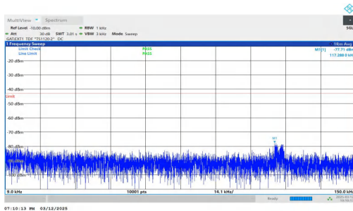
NTNV-n78(3450-3550)-PC2-30-20-M-DFT-BPSK-Inner_1RB_Left -0.009-0.15-PASS
