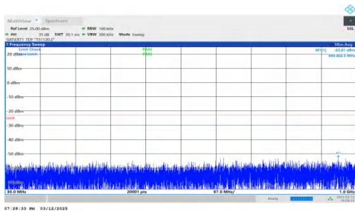
NTNV-n78(3450-3550)-PC2-30-30-M-DFT-BPSK-Inner_1RB_Left -30-1000-PASS
