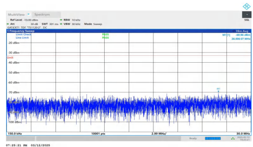
NTNV-n78(3450-3550)-PC2-30-30-L-DFT-QPSK-Inner_1RB_Left- 0.15-30-PASS
