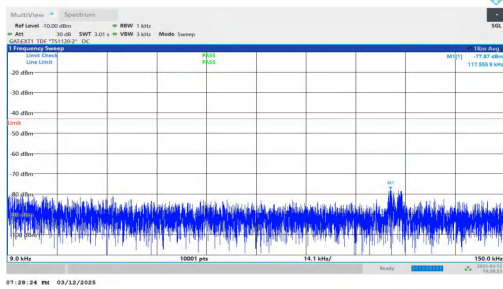
NTNV-n78(3450-3550)-PC2-30-30-M-DFT-BPSK-Inner_1RB_Left -0.009-0.15-PASS
