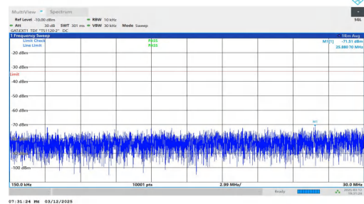
NTNV-n78(3450-3550)-PC2-30-30-M-DFT-QPSK-Inner_1RB_Left- 0.15-30-PASS
