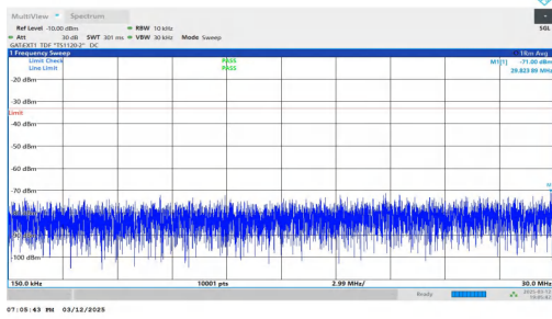
NTNV-n78(3450-3550)-PC2-30-20-L-DFT-BPSK-Inner_1RB_Rig ht-0.15-30-PASS
