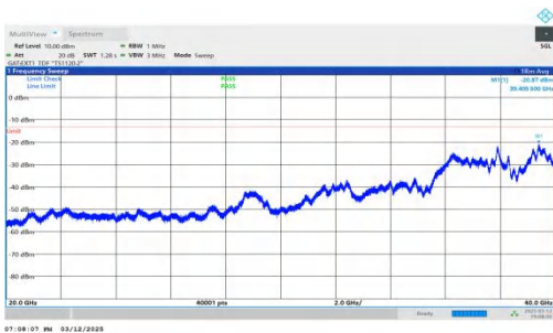
NTNV-n78(3450-3550)-PC2-30-20-L-DFT-QPSK-Inner_1RB_Left -20000-40000-PASS
