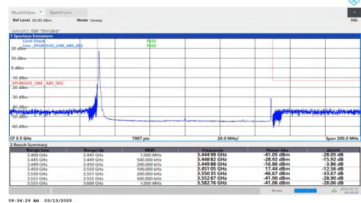
NTNV-n78(3450-3550)-PC2-30-100-L-DFT-QPSK-Edge_1RB_Lef t-PASS
