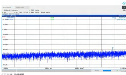
NTNV-n78(3450-3550)-PC2-30-20-H-DFT-BPSK-Inner_1RB_Rig ht-1000-3000-PASS
