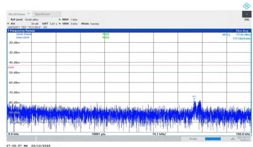
NTNV-n78(3450-3550)-PC2-30-20-L-DFT-BPSK-Inner_1RB_Right -0.009-0.15-PASS
