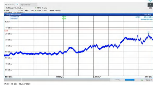
NTNV-n78(3450-3550)-PC2-30-20-L-DFT-QPSK-Inner_1RB_Right -20000-40000-PASS
