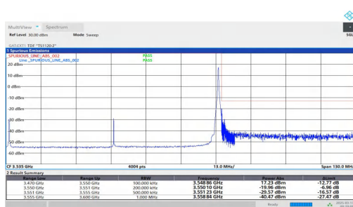
NTNV-n78(3450-3550)-PC2-30-80-H-DFT-QPSK-Edge_1RB_Right-PASS
