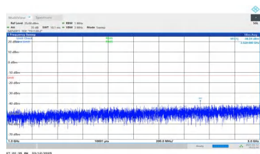
NTNV-n78(3450-3550)-PC2-30-30-L-DFT-BPSK-Inner_1RB_Left- 1000-3000-PASS
