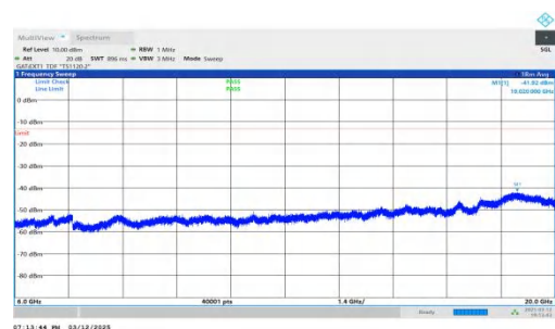
NTNV-n78(3450-3550)-PC2-30-20-M-DFT-QPSK-Inner_1RB_Left- 6000-20000-PASS
