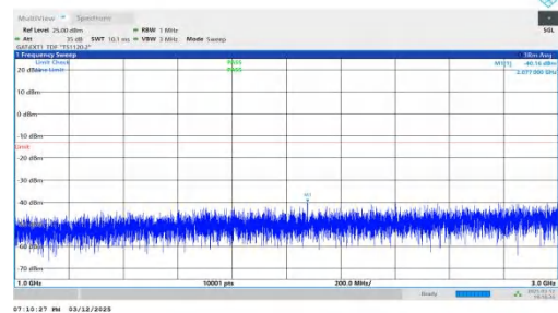
NTNV-n78(3450-3550)-PC2-30-20-M-DFT-BPSK-Inner_1RB_Left- 1000-3000-PASS
