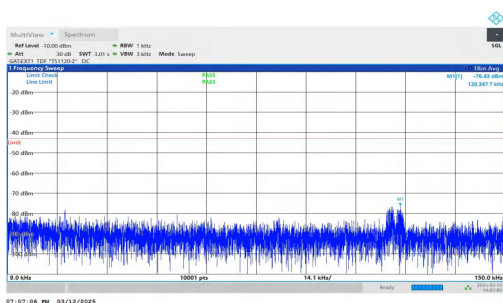
NTNV-n78(3450-3550)-PC2-30-20-L-DFT-QPSK-Inner_1RB_Left -0.009-0.15-PASS
