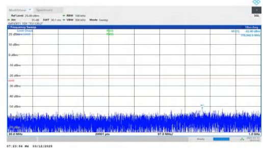
NTNV-n78(3450-3550)-PC2-30-30-L-DFT-BPSK-Inner_1RB_Right-30-1000-PASS
