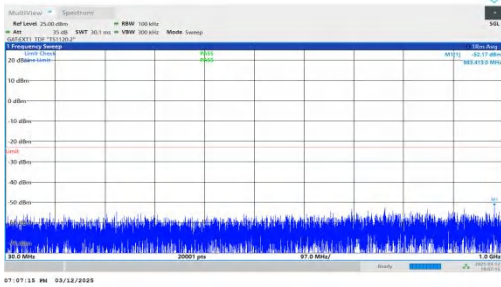
NTNV-n78(3450-3550)-PC2-30-20-L-DFT-QPSK-Inner_1RB_Left -30-1000-PASS
