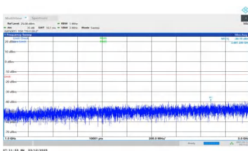
NTNV-n78(3450-3550)-PC2-30-20-M-DFT-BPSK-Inner_1RB_Rig ht-1000-3000-PASS
