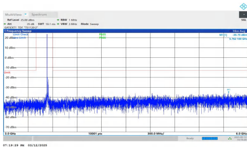
NTNV-n78(3450-3550)-PC2-30-20-H-DFT-QPSK-Inner_1RB_Left -3000-6000-PASS
