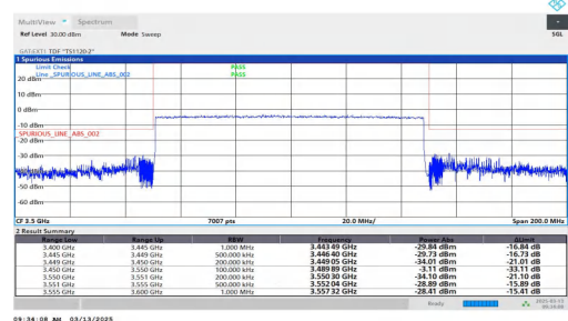
NTNV-n78(3450-3550)-PC2-30-100-L-DFT-QPSK-Outer_Full-PA SS
