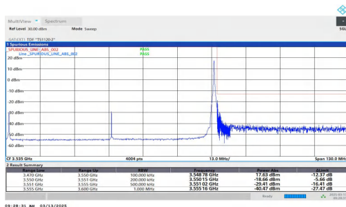
NTNV-n78(3450-3550)-PC2-30-80-H-DFT-BPSK-Edge_1RB_Right-PASS
