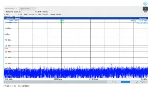
NTNV-n78(3450-3550)-PC2-30-20-M-DFT-QPSK-Inner_1RB_Righ t-30-1000-PASS
