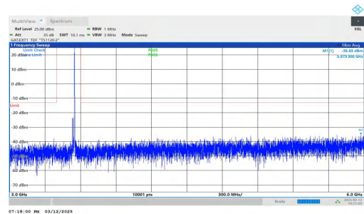
NTNV-n78(3450-3550)-PC2-30-20-H-DFT-BPSK-Inner_1RB_Righ t-3000-6000-PASS
