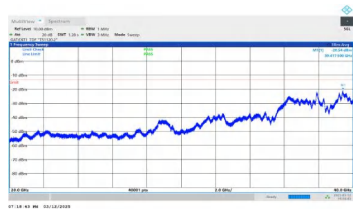
NTNV-n78(3450-3550)-PC2-30-20-H-DFT-BPSK-Inner_1RB_Righ t-20000-40000-PASS
