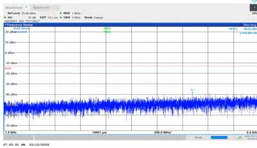
NTNV-n78(3450-3550)-PC2-30-20-H-DFT-QPSK-Inner_1RB_Rig ht-1000-3000-PASS
