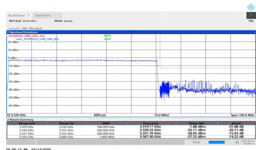
NTNV-n78(3450-3550)-PC2-30-80-H-DFT-BPSK-Outer_Full-PASS
