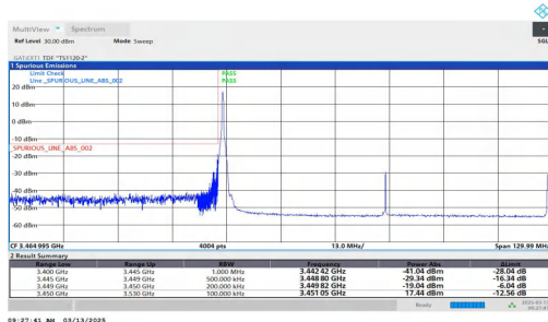
NTNV-n78(3450-3550)-PC2-30-80-L-DFT-QPSK-Edge_1RB_Left-PASS
