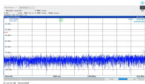
NTNV-n78(3450-3550)-PC2-30-20-M-DFT-QPSK-Inner_1RB_Left- 0.15-30-PASS
