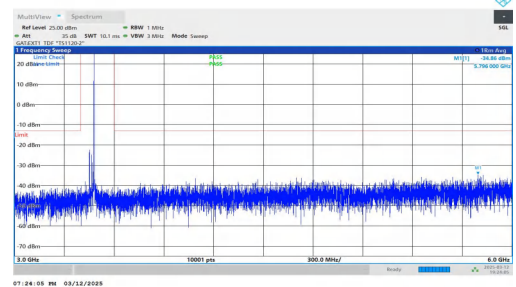
NTNV-n78(3450-3550)-PC2-30-30-L-DFT-BPSK-Inner_1RB_Right-3000-6000-PASS
