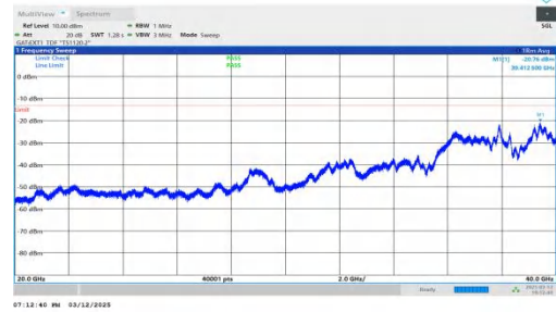
NTNV-n78(3450-3550)-PC2-30-20-M-DFT-BPSK-Inner_1RB_Righ t-20000-40000-PASS
