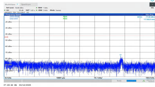
NTNV-n78(3450-3550)-PC2-30-30-L-DFT-QPSK-Inner_1RB_Right -0.009-0.15-PASS
