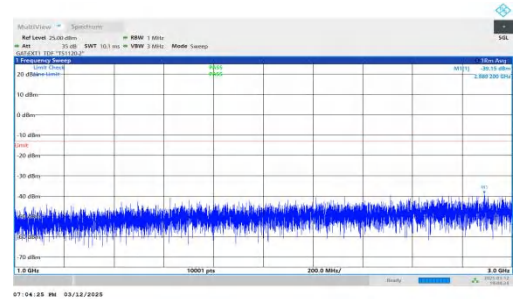
NTNV-n78(3450-3550)-PC2-30-20-L-DFT-BPSK-Inner_1RB_Left- 1000-3000-PASS
