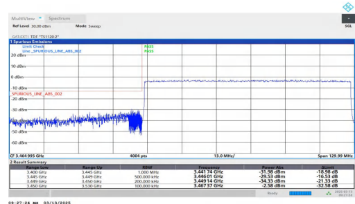
NTNV-n78(3450-3550)-PC2-30-80-L-DFT-QPSK-Outer_Full-PASS
