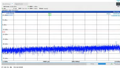
NTNV-n78(3450-3550)-PC2-30-30-L-DFT-BPSK-Inner_1RB_Rig ht-1000-3000-PASS
