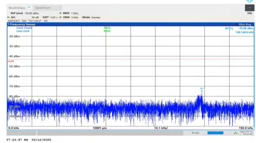
NTNV-n78(3450-3550)-PC2-30-30-L-DFT-BPSK-Inner_1RB_Right-0.009-0.15-PASS
