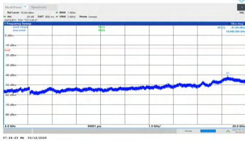
NTNV-n78(3450-3550)-PC2-30-30-L-DFT-BPSK-Inner_1RB_Rig ht-6000-20000-PASS
