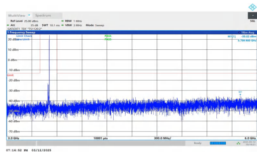
NTNV-n78(3450-3550)-PC2-30-20-M-DFT-QPSK-Inner_1RB_Righ t-3000-6000-PASS
