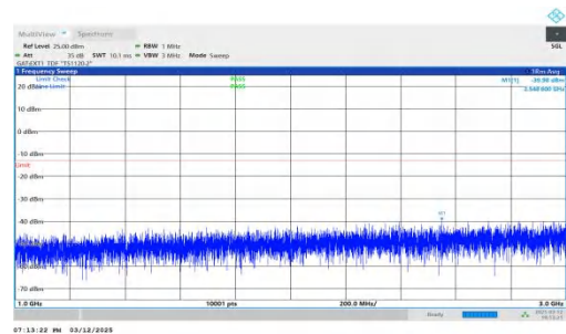
NTNV-n78(3450-3550)-PC2-30-20-M-DFT-QPSK-Inner_1RB_Left- 1000-3000-PASS
