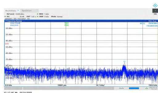
NTNV-n78(3450-3550)-PC2-30-20-H-DFT-BPSK-Inner_1RB_Right t-0.009-0.15-PASS
