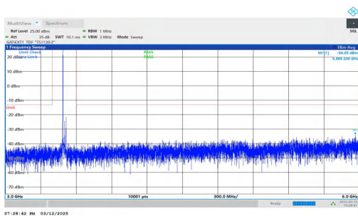
NTNV-n78(3450-3550)-PC2-30-30-M-DFT-BPSK-Inner_1RB_Left -3000-6000-PASS
