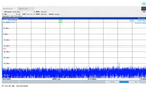
NTNV-n78(3450-3550)-PC2-30-20-H-DFT-BPSK-Inner_1RB_Left -30-1000-PASS
