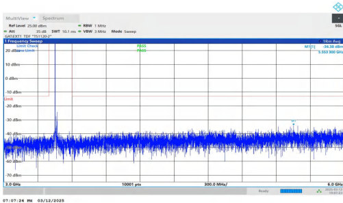
NTNV-n78(3450-3550)-PC2-30-20-L-DFT-QPSK-Inner_1RB_Left -3000-6000-PASS
