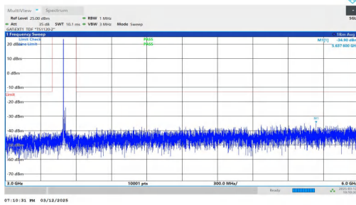
NTNV-n78(3450-3550)-PC2-30-20-M-DFT-BPSK-Inner_1RB_Left -3000-6000-PASS
