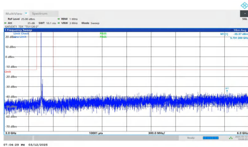
NTNV-n78(3450-3550)-PC2-30-20-L-DFT-BPSK-Inner_1RB_Left- 3000-6000-PASS
