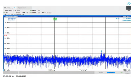
NTNV-n78(3450-3550)-PC2-30-20-L-DFT-QPSK-Inner_1RB_Right -0.009-0.15-PASS
