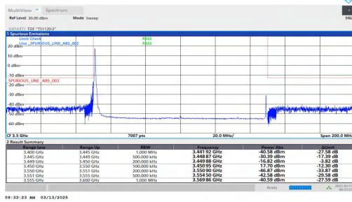
NTNV-n78(3450-3550)-PC2-30-100-L-DFT-BPSK-Edge_1RB_Left -PASS
