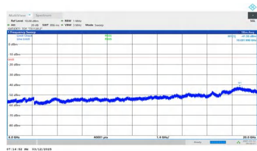
NTNV-n78(3450-3550)-PC2-30-20-H-DFT-BPSK-Inner_1RB_Left 6000-20000-PASS
