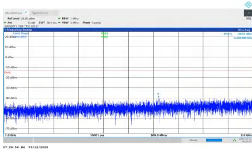
NTNV-n78(3450-3550)-PC2-30-30-L-DFT-QPSK-Inner_1RB_Rig ht-1000-3000-PASS
