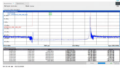
NTNV-n78(3450-3550)-PC2-30-100-L-DFT-BPSK-Edge_1RB_Rig ht-PASS
