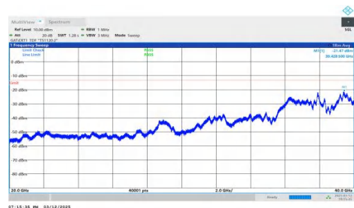
NTNV-n78(3450-3550)-PC2-30-20-M-DFT-QPSK-Inner_1RB_Righ t-20000-40000-PASS
