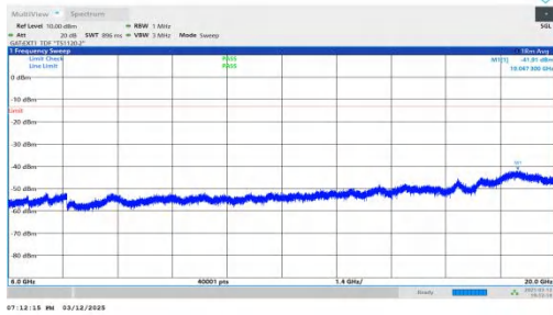
NTNV-n78(3450-3550)-PC2-30-20-M-DFT-BPSK-Inner_1RB_Rig ht-6000-20000-PASS
