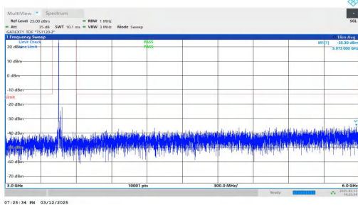
NTNV-n78(3450-3550)-PC2-30-30-L-DFT-QPSK-Inner_1RB_Left -3000-6000-PASS
