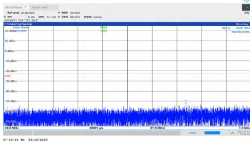
NTNV-n78(3450-3550)-PC2-30-20-H-DFT-QPSK-Inner_1RB_Left -30-1000-PASS
