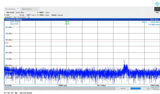
NTNV-n78(3450-3550)-PC2-30-20-H-DFT-QPSK-Inner_1RB_Right t-0.009-0.15-PASS
