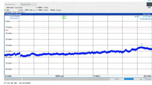
NTNV-n78(3450-3550)-PC2-30-20-M-DFT-BPSK-Inner_1RB_Left 6000-20000-PASS
