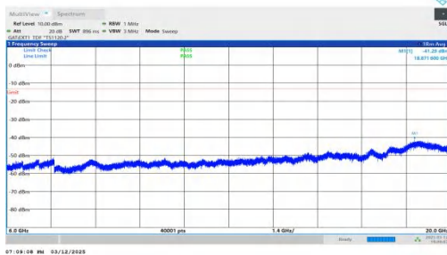
NTNV-n78(3450-3550)-PC2-30-20-L-DFT-QPSK-Inner_1RB_Rig ht-6000-20000-PASS
