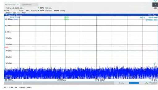
NTNV-n78(3450-3550)-PC2-30-20-H-DFT-BPSK-Inner_1RB_Righ t-30-1000-PASS
