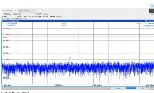
NTNV-n78(3450-3550)-PC2-30-20-L-DFT-QPSK-Inner_1RB_Rig ht-0.15-30-PASS
