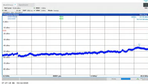
NTNV-n78(3450-3550)-PC2-30-30-L-DFT-QPSK-Inner_1RB_Rig ht-6000-20000-PASS
