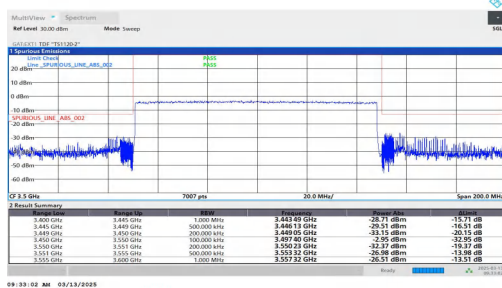
NTNV-n78(3450-3550)-PC2-30-100-L-DFT-BPSK-Outer_Full-PAS S
