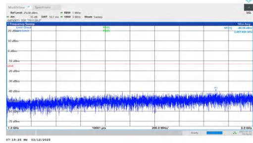
NTNV-n78(3450-3550)-PC2-30-20-H-DFT-QPSK-Inner_1RB_Left 1000-3000-PASS
