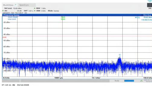
NTNV-n78(3450-3550)-PC2-30-20-H-DFT-QPSK-Inner_1RB_Left -0.009-0.15-PASS
