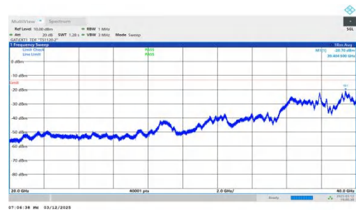
NTNV-n78(3450-3550)-PC2-30-20-L-DFT-BPSK-Inner_1RB_Right -20000-40000-PASS
