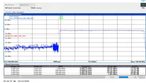
NTNV-n78(3450-3550)-PC2-30-80-L-DFT-BPSK-Outer_Full-PASS
