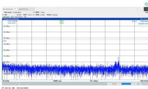
NTNV-n78(3450-3550)-PC2-30-30-L-DFT-BPSK-Inner_1RB_Left- 0.009-0.15-PASS
