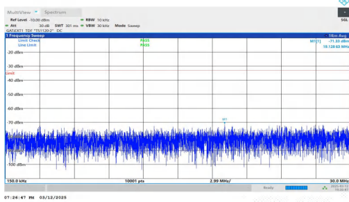
NTNV-n78(3450-3550)-PC2-30-30-L-DFT-QPSK-Inner_1RB_Rig ht-0.15-30-PASS
