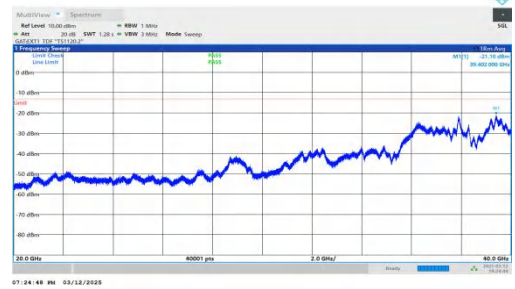
NTNV-n78(3450-3550)-PC2-30-30-L-DFT-BPSK-Inner_1RB_Right -20000-40000-PASS
