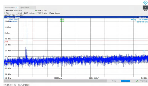
NTNV-n78(3450-3550)-PC2-30-30-L-DFT-QPSK-Inner_1RB_Right -3000-6000-PASS
