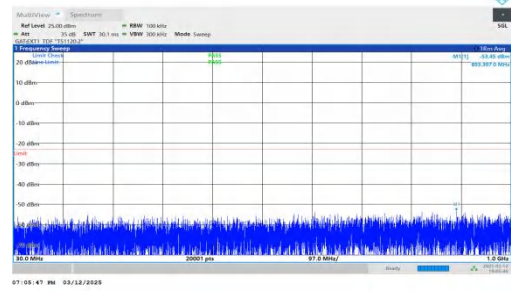
NTNV-n78(3450-3550)-PC2-30-20-L-DFT-BPSK-Inner_1RB_Right -30-1000-PASS
