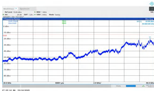
NTNV-n78(3450-3550)-PC2-30-20-L-DFT-BPSK-Inner_1RB_Left- 20000-40000-PASS
