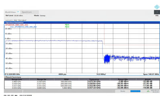
NTNV-n78(3450-3550)-PC2-30-90-H-DFT-QPSK-Outer_Full-PASS
