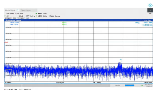
NTNV-n78(3450-3550)-PC2-30-30-M-DFT-BPSK-Inner_1RB_Right t-0.009-0.15-PASS
