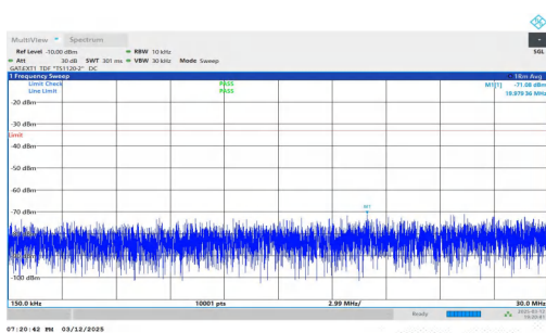
NTNV-n78(3450-3550)-PC2-30-20-H-DFT-QPSK-Inner_1RB_Rig ht-0.15-30-PASS
