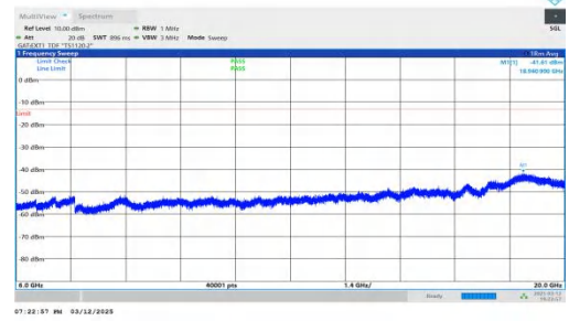
NTNV-n78(3450-3550)-PC2-30-30-L-DFT-BPSK-Inner_1RB_Left-6000-20000-PASS
