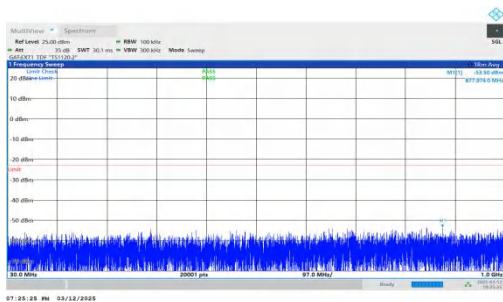
NTNV-n78(3450-3550)-PC2-30-30-L-DFT-QPSK-Inner_1RB_Left -30-1000-PASS
