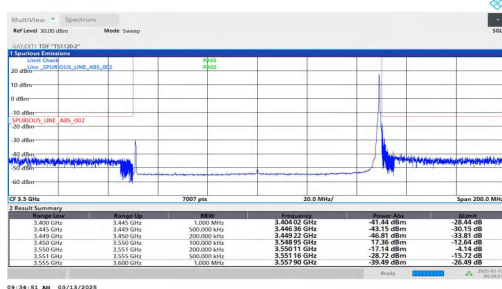
NTNV-n78(3450-3550)-PC2-30-100-L-DFT-QPSK-Edge_1RB_Rig ht-PASS
