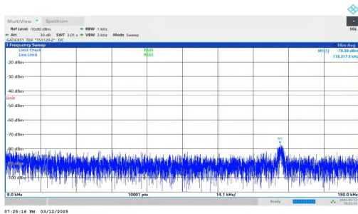
NTNV-n78(3450-3550)-PC2-30-30-L-DFT-QPSK-Inner_1RB_Left -0.009-0.15-PASS
