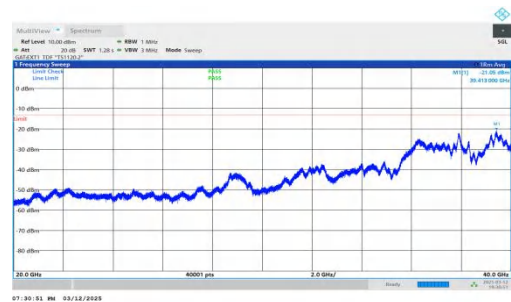
NTNV-n78(3450-3550)-PC2-30-30-M-DFT-BPSK-Inner_1RB_Righ t-20000-40000-PASS
