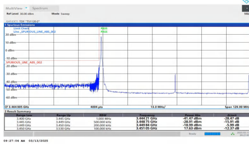
NTNV-n78(3450-3550)-PC2-30-80-L-DFT-BPSK-Edge_1RB_Left-PASS
