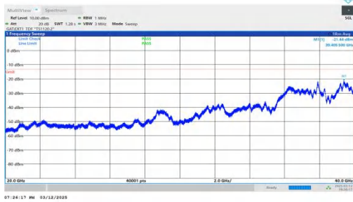
NTNV-n78(3450-3550)-PC2-30-30-L-DFT-QPSK-Inner_1RB_Left -20000-40000-PASS
