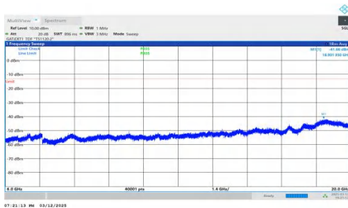
NTNV-n78(3450-3550)-PC2-30-20-H-DFT-QPSK-Inner_1RB_Rig ht-6000-20000-PASS
