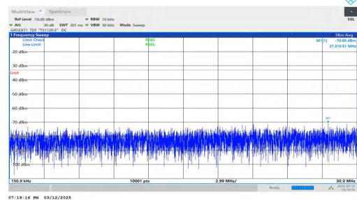
NTNV-n78(3450-3550)-PC2-30-20-H-DFT-QPSK-Inner_1RB_Left 0.15-30-PASS
