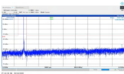
NTNV-n78(3450-3550)-PC2-30-20-H-DFT-BPSK-Inner_1RB_Left -3000-6000-PASS
