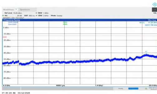
NTNV-n78(3450-3550)-PC2-30-30-M-DFT-BPSK-Inner_1RB_Rig ht-6000-20000-PASS
