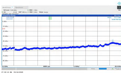
NTNV-n78(3450-3550)-PC2-30-20-L-DFT-BPSK-Inner_1RB_Rig ht-6000-20000-PASS
