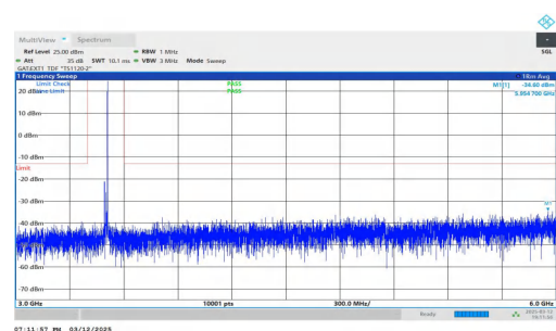
NTNV-n78(3450-3550)-PC2-30-20-M-DFT-BPSK-Inner_1RB_Right t-3000-6000-PASS
