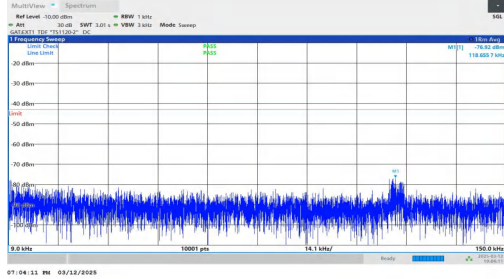
NTNV-n78(3450-3550)-PC2-30-20-L-DFT-BPSK-Inner_1RB_Left- 0.009-0.15-PASS
