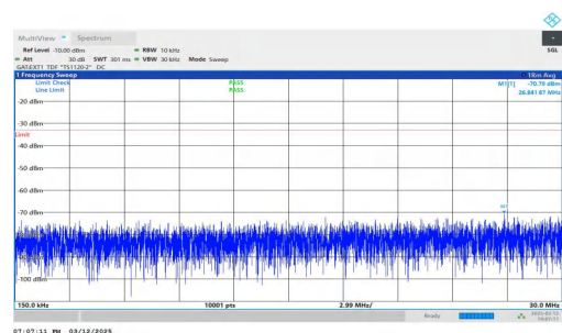
NTNV-n78(3450-3550)-PC2-30-20-L-DFT-QPSK-Inner_1RB_Left- 0.15-30-PASS
