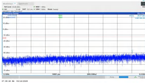
NTNV-n78(3450-3550)-PC2-30-20-L-DFT-QPSK-Inner_1RB_Rig ht-1000-3000-PASS
