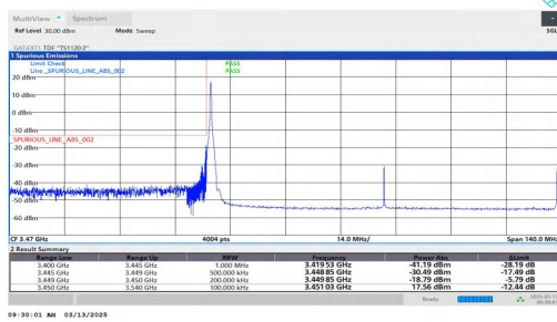
NTNV-n78(3450-3550)-PC2-30-90-L-DFT-BPSK-Edge_1RB_Left-PASS
