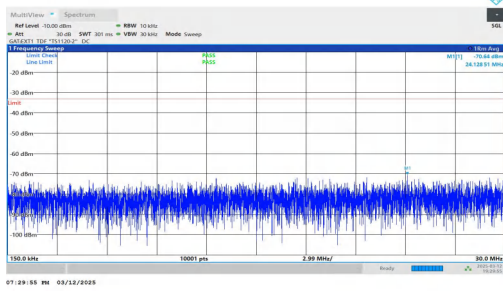
NTNV-n78(3450-3550)-PC2-30-30-M-DFT-BPSK-Inner_1RB_Rig ht-0.15-30-PASS
