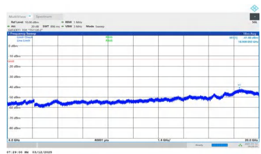
NTNV-n78(3450-3550)-PC2-30-30-M-DFT-BPSK-Inner_1RB_Left 6000-20000-PASS
