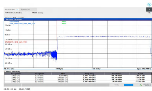
NTNV-n78(3450-3550)-PC2-30-90-L-DFT-QPSK-Outer_Full-PASS
