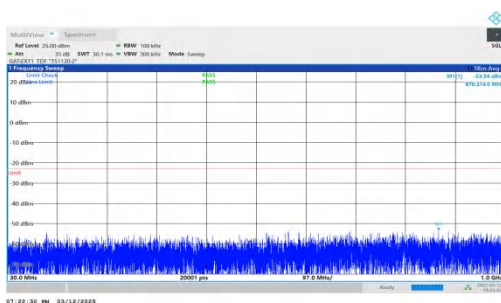
NTNV-n78(3450-3550)-PC2-30-30-L-DFT-BPSK-Inner_1RB_Left- 30-1000-PASS
