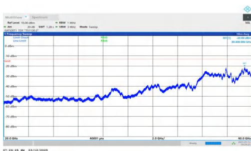
NTNV-n78(3450-3550)-PC2-30-30-M-DFT-BPSK-Inner_1RB_Left -20000-40000-PASS
