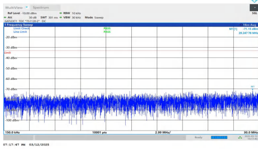
NTNV-n78(3450-3550)-PC2-30-20-H-DFT-BPSK-Inner_1RB_Rig ht-0.15-30-PASS
