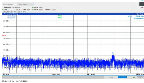
NTNV-n78(3450-3550)-PC2-30-20-H-DFT-BPSK-Inner_1RB_Left -0.009-0.15-PASS
