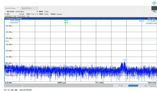
NTNV-n78(3450-3550)-PC2-30-20-M-DFT-BPSK-Inner_1RB_Right t-0.009-0.15-PASS
