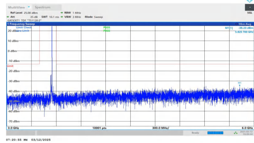
NTNV-n78(3450-3550)-PC2-30-20-H-DFT-QPSK-Inner_1RB_Righ t-3000-6000-PASS
