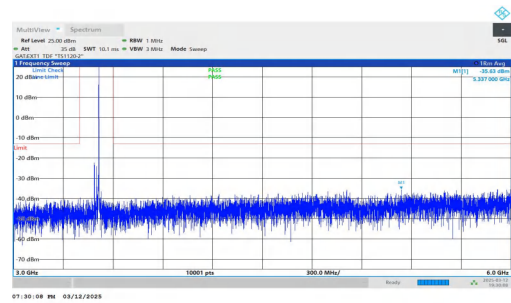
NTNV-n78(3450-3550)-PC2-30-30-M-DFT-BPSK-Inner_1RB_Righ t-3000-6000-PASS
