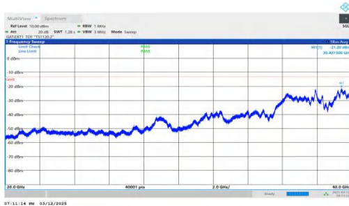
NTNV-n78(3450-3550)-PC2-30-20-M-DFT-BPSK-Inner_1RB_Left -20000-40000-PASS
