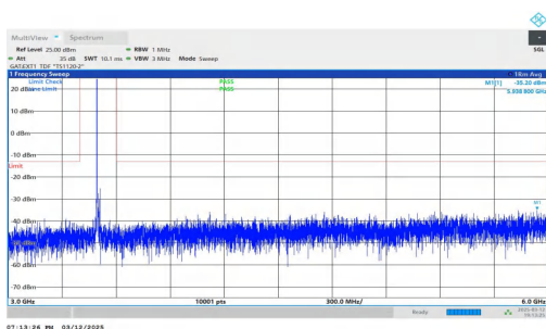
NTNV-n78(3450-3550)-PC2-30-20-M-DFT-QPSK-Inner_1RB_Lef t-3000-6000-PASS
