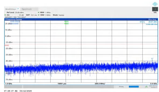
NTNV-n78(3450-3550)-PC2-30-30-M-DFT-BPSK-Inner_1RB_Left 1000-3000-PASS
