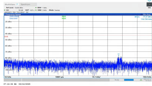
NTNV-n78(3450-3550)-PC2-30-20-M-DFT-QPSK-Inner_1RB_Righ t-0.009-0.15-PASS
