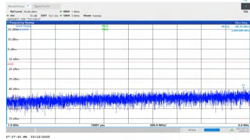
NTNV-n78(3450-3550)-PC2-30-20-L-DFT-QPSK-Inner_1RB_Left- 1000-3000-PASS
