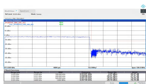
NTNV-n78(3450-3550)-PC2-30-80-H-DFT-QPSK-Outer_Full-PASS
