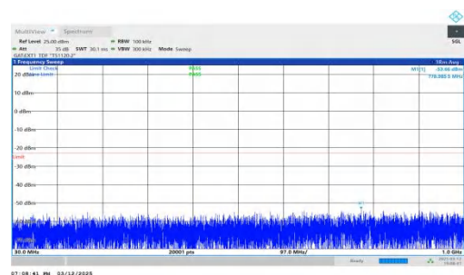
NTNV-n78(3450-3550)-PC2-30-20-L-DFT-QPSK-Inner_1RB_Right -30-1000-PASS
