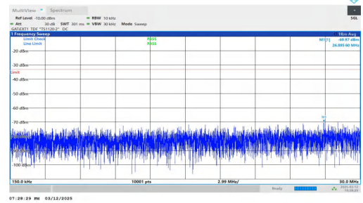
NTNV-n78(3450-3550)-PC2-30-30-M-DFT-BPSK-Inner_1RB_Left 0.15-30-PASS
