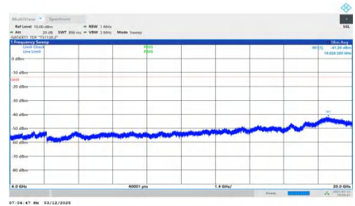
NTNV-n78(3450-3550)-PC2-30-20-L-DFT-BPSK-Inner_1RB_Left- 6000-20000-PASS
