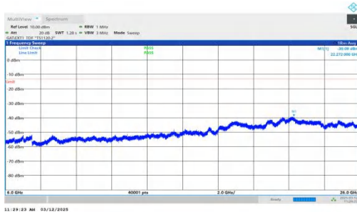
NTNV-n77(3700-3980)-PC2-30-40-H-DFT-QPSK-Inner_1RB_Rig ht-6000-26000-PASS
