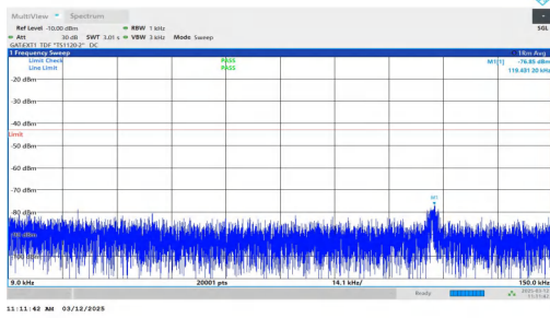
NTNV-n77(3700-3980)-PC2-30-40-L-DFT-BPSK-Inner_1RB_Left- 0.009-0.15-PASS
