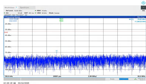
NTNV-n77(3700-3980)-PC2-30-30-L-DFT-QPSK-Inner_1RB_Left- 0.15-30-PASS
