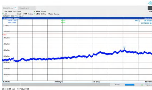
NTNV-n77(3700-3980)-PC2-30-30-M-DFT-QPSK-Inner_1RB_Rig ht-6000-26000-PASS
