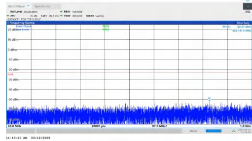
NTNV-n77(3700-3980)-PC2-30-40-L-DFT-BPSK-Inner_1RB_Right -30-1000-PASS
