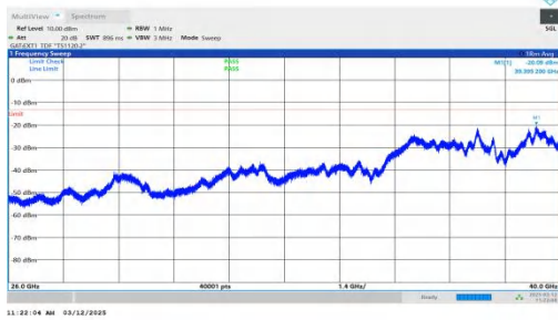
NTNV-n77(3700-3980)-PC2-30-40-M-DFT-QPSK-Inner_1RB_Lef t-26000-40000-PASS
