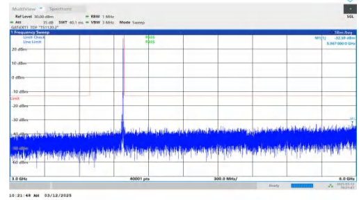
NTNV-n77(3700-3980)-PC2-30-20-H-DFT-QPSK-Inner_1RB_Righ t-3000-6000-PASS
