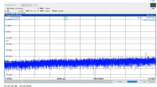
NTNV-n77(3700-3980)-PC2-30-30-L-DFT-BPSK-Inner_1RB_Left- 1000-3000-PASS
