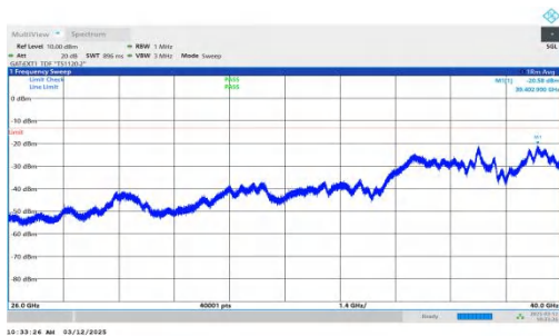
NTNV-n77(3700-3980)-PC2-30-30-M-DFT-QPSK-Inner_1RB_Lef t-26000-40000-PASS
