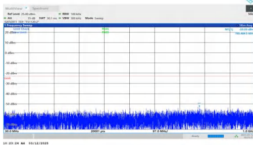
NTNV-n77(3700-3980)-PC2-30-30-L-DFT-BPSK-Inner_1RB_Left- 30-1000-PASS
