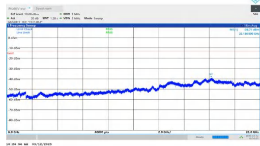
NTNV-n77(3700-3980)-PC2-30-30-L-DFT-QPSK-Inner_1RB_Left- 6000-26000-PASS
