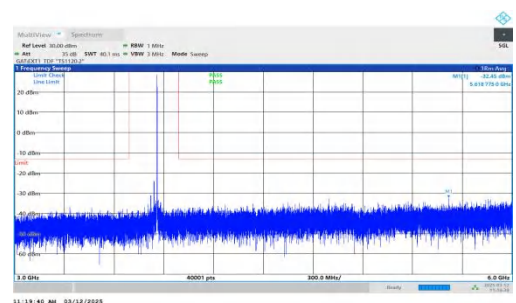
NTNV-n77(3700-3980)-PC2-30-40-M-DFT-BPSK-Inner_1RB_Right t-3000-6000-PASS
