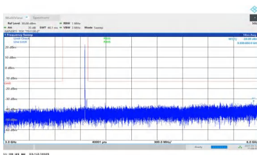
NTNV-n77(3700-3980)-PC2-30-30-H-DFT-QPSK-Inner_1RB_Left -3000-6000-PASS
