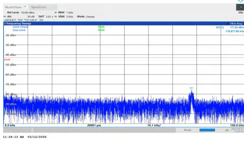
NTNV-n77(3700-3980)-PC2-30-40-H-DFT-BPSK-Inner_1RB_Left -0.009-0.15-PASS
