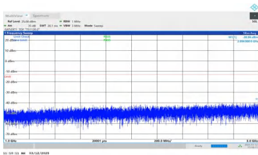
NTNV-n77(3700-3980)-PC2-30-30-H-DFT-QPSK-Inner_1RB_Right ht.1000-3000-PASS
