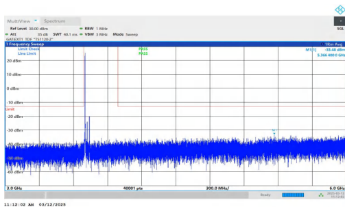
NTNV-n77(3700-3980)-PC2-30-40-L-DFT-BPSK-Inner_1RB_Left- 3000-6000-PASS
