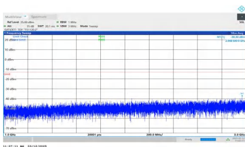
NTNV-n77(3700-3980)-PC2-30-30-H-DFT-BPSK-Inner_1RB_Right ht-1000-3000-PASS
