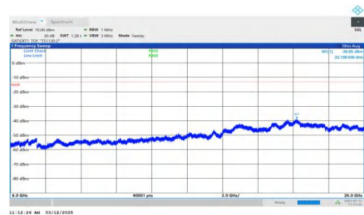
NTNV-n77(3700-3980)-PC2-30-40-L-DFT-BPSK-Inner_1RB_Left- 6000-26000-PASS
