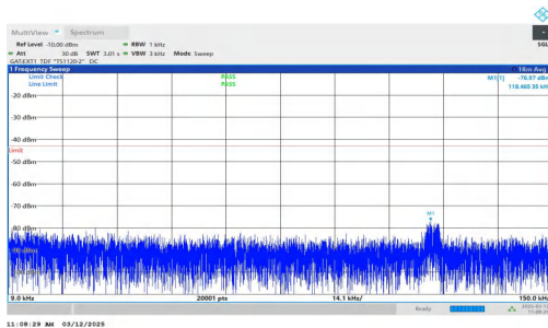
NTNV-n77(3700-3980)-PC2-30-30-H-DFT-QPSK-Inner_1RB_Left -0.009-0.15-PASS
