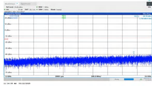
NTNV-n77(3700-3980)-PC2-30-40-L-DFT-QPSK-Inner_1RB_Left- 1000-3000-PASS
