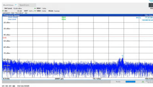
NTNV-n77(3700-3980)-PC2-30-30-M-DFT-QPSK-Inner_1RB_Lef t-0.009-0.15-PASS
