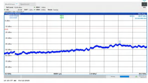
NTNV-n77(3700-3980)-PC2-30-30-L-DFT-BPSK-Inner_1RB_Left-6000-26000-PASS
