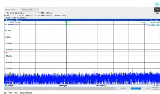
NTNV-n77(3700-3980)-PC2-30-30-H-DFT-BPSK-Inner_1RB_Right t-30-1000-PASS
