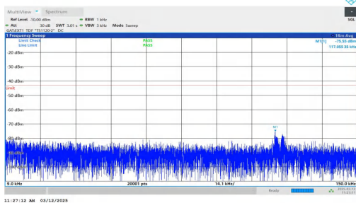
NTNV-n77(3700-3980)-PC2-30-40-H-DFT-QPSK-Inner_1RB_Left -0.009-0.15-PASS
