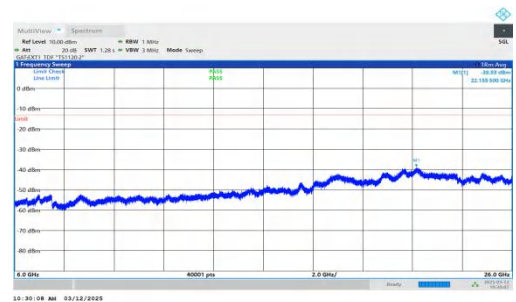
NTNV-n77(3700-3980)-PC2-30-30-M-DFT-BPSK-Inner_1RB_Left 6000-26000-PASS
