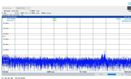
NTNV-n77(3700-3980)-PC2-30-60-L-DFT-BPSK-Inner_1RB_Left- 0.009-0.15-PASS
