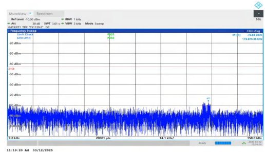
NTNV-n77(3700-3980)-PC2-30-40-M-DFT-BPSK-Inner_1RB_Right t-0.009-0.15-PASS
