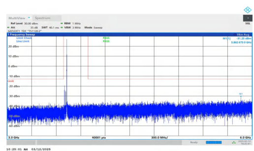
NTNV-n77(3700-3980)-PC2-30-30-L-DFT-BPSK-Inner_1RB_Right-3000-6000-PASS
