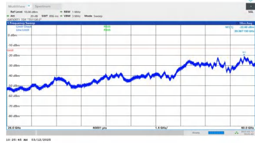
NTNV-n77(3700-3980)-PC2-30-30-L-DFT-BPSK-Inner_1RB_Right -26000-40000-PASS
