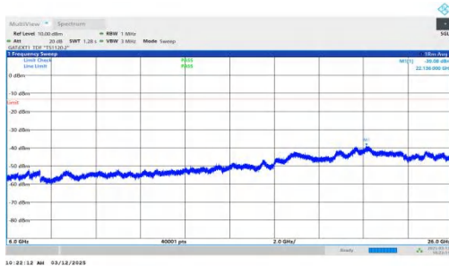
NTNV-n77(3700-3980)-PC2-30-20-H-DFT-QPSK-Inner_1RB_Rig ht-6000-26000-PASS
