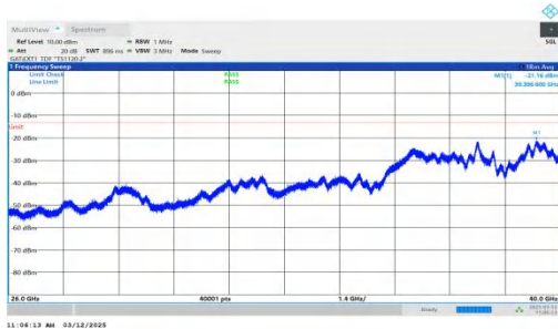
NTNV-n77(3700-3980)-PC2-30-30-H-DFT-BPSK-Inner_1RB_Left -26000-40000-PASS
