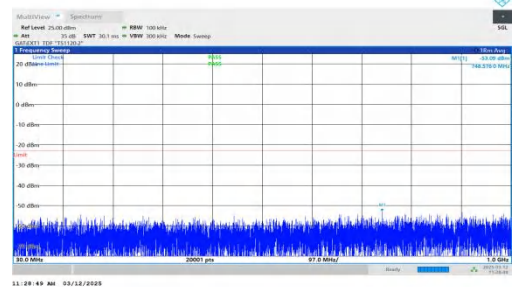
NTNV-n77(3700-3980)-PC2-30-40-H-DFT-QPSK-Inner_1RB_Right t-30-1000-PASS
