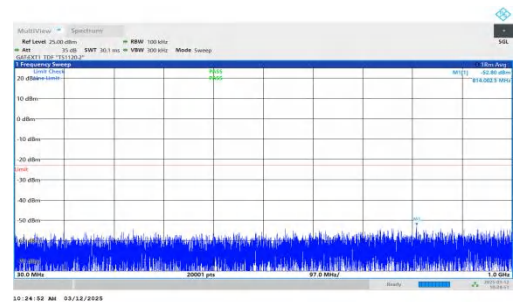
NTNV-n77(3700-3980)-PC2-30-30-L-DFT-BPSK-Inner_1RB_Right-30-1000-PASS
