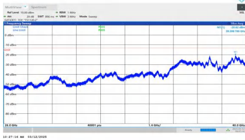
NTNV-n77(3700-3980)-PC2-30-30-L-DFT-QPSK-Inner_1RB_Left -26000-40000-PASS
