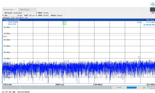
NTNV-n77(3700-3980)-PC2-30-30-H-DFT-BPSK-Inner_1RB_Right ht-0.15-30-PASS
