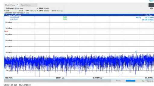
NTNV-n77(3700-3980)-PC2-30-30-M-DFT-QPSK-Inner_1RB_Left- 0.15-30-PASS
