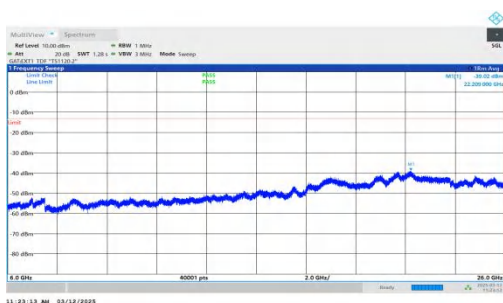
NTNV-n77(3700-3980)-PC2-30-40-M-DFT-QPSK-Inner_1RB_Rig ht-6000-26000-PASS
