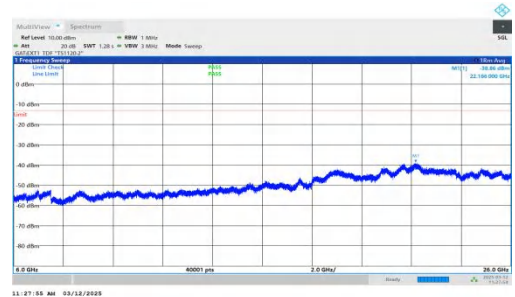
NTNV-n77(3700-3980)-PC2-30-40-H-DFT-QPSK-Inner_1RB_Left 6000-26000-PASS
