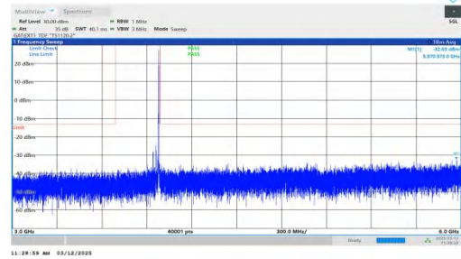
NTNV-n77(3700-3980)-PC2-30-40-H-DFT-QPSK-Inner_1RB_Righ t-3000-6000-PASS
