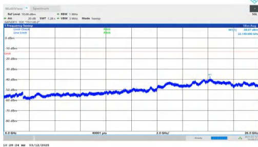
NTNV-n77(3700-3980)-PC2-30-30-L-DFT-QPSK-Inner_1RB_Rig ht-6000-26000-PASS
