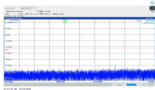
NTNV-n77(3700-3980)-PC2-30-30-L-DFT-QPSK-Inner_1RB_Right -30-1000-PASS
