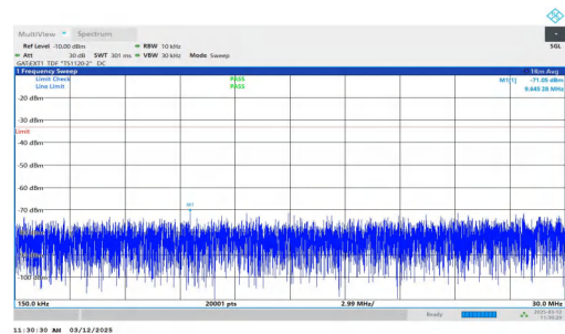
NTNV-n77(3700-3980)-PC2-30-60-L-DFT-BPSK-Inner_1RB_Left- 0.15-30-PASS
