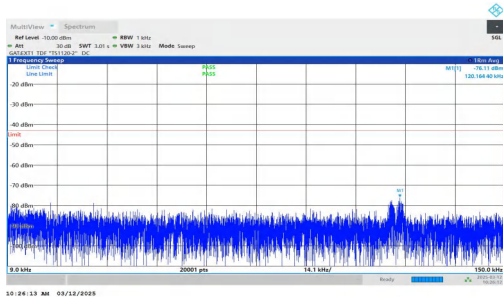
NTNV-n77(3700-3980)-PC2-30-30-L-DFT-QPSK-Inner_1RB_Left -0.009-0.15-PASS
