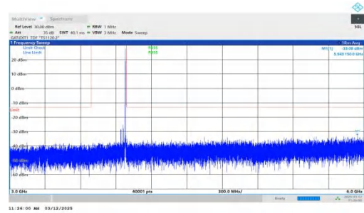
NTNV-n77(3700-3980)-PC2-30-40-H-DFT-BPSK-Inner_1RB_Righ t-3000-6000-PASS
