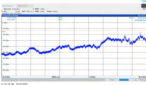
NTNV-n77(3700-3980)-PC2-30-40-L-DFT-QPSK-Inner_1RB_Left -26000-40000-PASS
