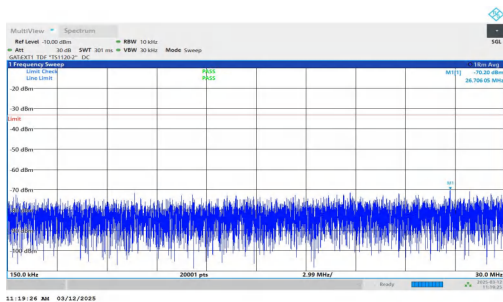
NTNV-n77(3700-3980)-PC2-30-40-M-DFT-BPSK-Inner_1RB_Right ht-0.15-30-PASS
