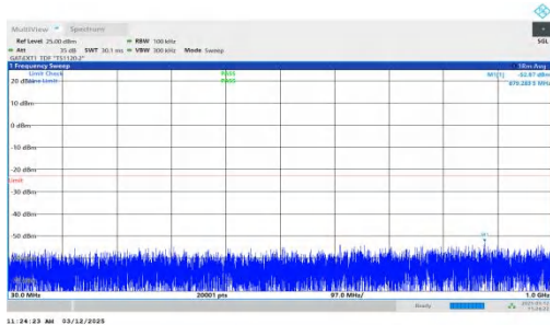
NTNV-n77(3700-3980)-PC2-30-40-H-DFT-BPSK-Inner_1RB_Left -30-1000-PASS
