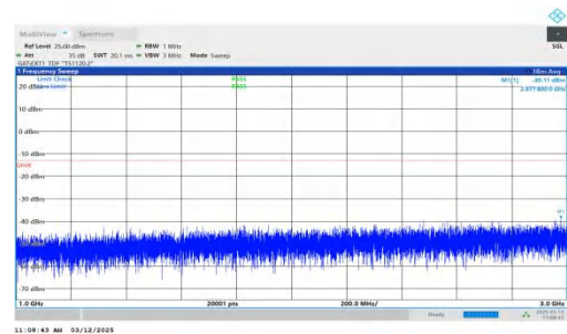
NTNV-n77(3700-3980)-PC2-30-30-H-DFT-QPSK-Inner_1RB_Left- 1000-3000-PASS
