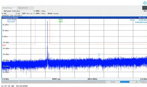
NTNV-n77(3700-3980)-PC2-30-40-H-DFT-QPSK-Inner_1RB_Left -3000-6000-PASS
