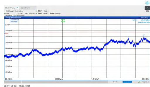
NTNV-n77(3700-3980)-PC2-30-40-L-DFT-QPSK-Inner_1RB_Right -26000-40000-PASS
