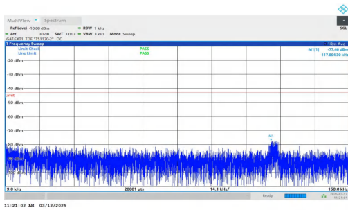
NTNV-n77(3700-3980)-PC2-30-40-M-DFT-QPSK-Inner_1RB_Lef t-0.009-0.15-PASS
