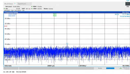
NTNV-n77(3700-3980)-PC2-30-40-H-DFT-BPSK-Inner_1RB_Left 0.15-30-PASS
