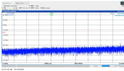
NTNV-n77(3700-3980)-PC2-30-20-H-DFT-QPSK-Inner_1RB_Rig ht-1000-3000-PASS
