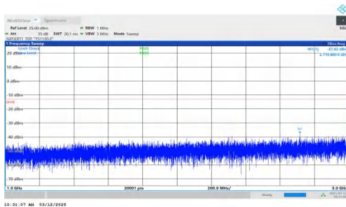
NTNV-n77(3700-3980)-PC2-30-30-M-DFT-BPSK-Inner_1RB_Rig ht-1000-3000-PASS
