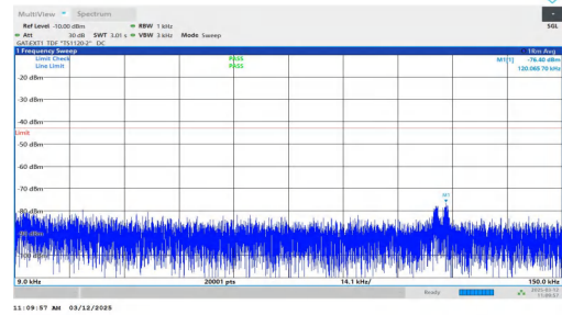
NTNV-n77(3700-3980)-PC2-30-30-H-DFT-QPSK-Inner_1RB_Right t.0.009-0.15-PASS
