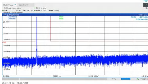
NTNV-n77(3700-3980)-PC2-30-30-L-DFT-QPSK-Inner_1RB_Left -3000-6000-PASS
