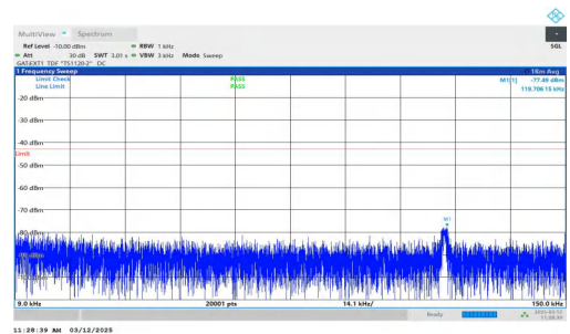
NTNV-n77(3700-3980)-PC2-30-40-H-DFT-QPSK-Inner_1RB_Right t-0.009-0.15-PASS
