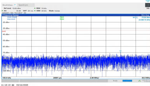
NTNV-n77(3700-3980)-PC2-30-40-L-DFT-QPSK-Inner_1RB_Rig ht-0.15-30-PASS
