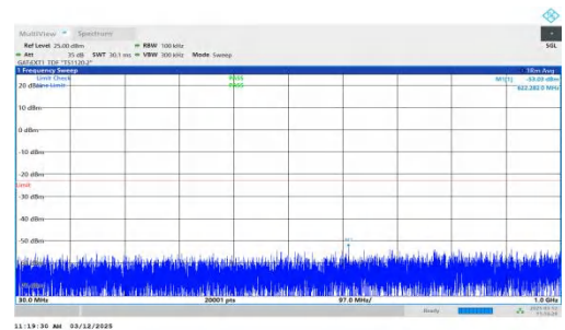
NTNV-n77(3700-3980)-PC2-30-40-M-DFT-BPSK-Inner_1RB_Right t-30-1000-PASS
