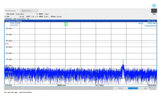
NTNV-n77(3700-3980)-PC2-30-30-M-DFT-BPSK-Inner_1RB_Right t-0.009-0.15-PASS
