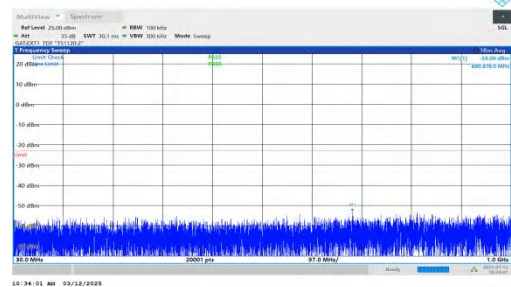
NTNV-n77(3700-3980)-PC2-30-30-M-DFT-QPSK-Inner_1RB_Right t-30-1000-PASS
