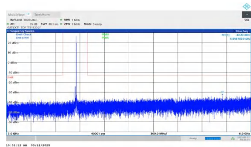
NTNV-n77(3700-3980)-PC2-30-30-M-DFT-BPSK-Inner_1RB_Righ t-3000-6000-PASS
