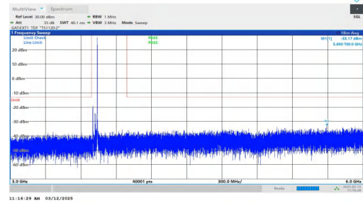
NTNV-n77(3700-3980)-PC2-30-40-L-DFT-QPSK-Inner_1RB_Right -3000-6000-PASS
