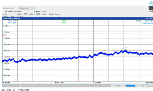
NTNV-n77(3700-3980)-PC2-30-40-L-DFT-QPSK-Inner_1RB_Rig ht-6000-26000-PASS
