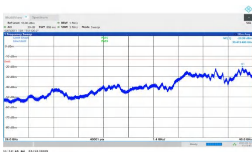
NTNV-n77(3700-3980)-PC2-30-40-L-DFT-BPSK-Inner_1RB_Left- 26000-40000-PASS
