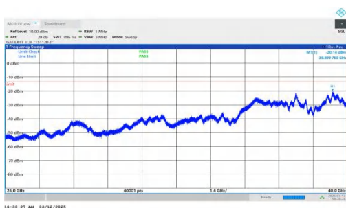
NTNV-n77(3700-3980)-PC2-30-30-M-DFT-BPSK-Inner_1RB_Left -26000-40000-PASS
