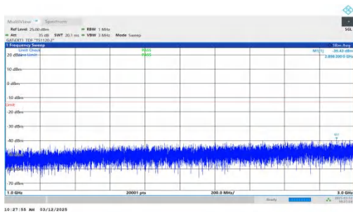
NTNV-n77(3700-3980)-PC2-30-30-L-DFT-QPSK-Inner_1RB_Rig ht-1000-3000-PASS
