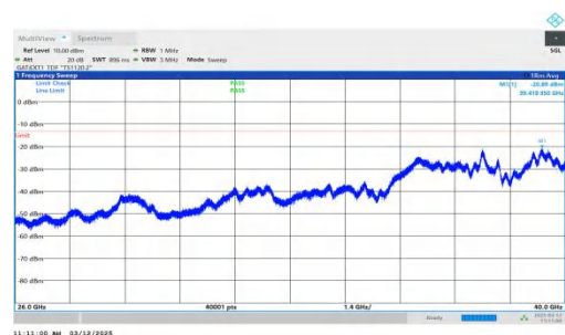
NTNV-n77(3700-3980)-PC2-30-30-H-DFT-QPSK-Inner_1RB_Right t.26000-40000-PASS
