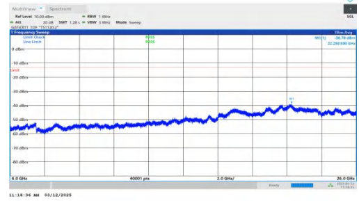
NTNV-n77(3700-3980)-PC2-30-40-M-DFT-BPSK-Inner_1RB_Left 6000-26000-PASS
