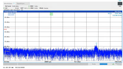
NTNV-n77(3700-3980)-PC2-30-40-M-DFT-QPSK-Inner_1RB_Righ t-0.009-0.15-PASS
