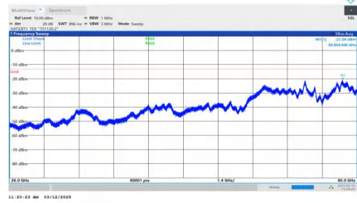
NTNV-n77(3700-3980)-PC2-30-40-M-DFT-BPSK-Inner_1RB_Righ t-26000-40000-PASS
