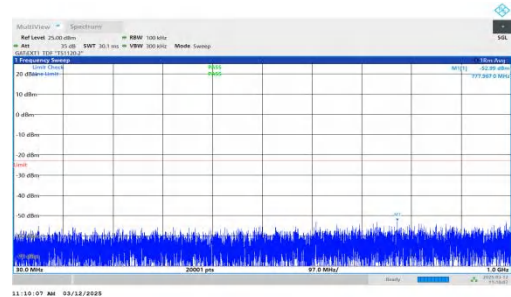
NTNV-n77(3700-3980)-PC2-30-30-H-DFT-QPSK-Inner_1RB_Right t.30-1000-PASS
