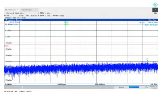
NTNV-n77(3700-3980)-PC2-30-30-H-DFT-BPSK-Inner_1RB_Left- 1000-3000-PASS
