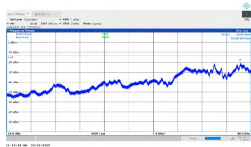
NTNV-n77(3700-3980)-PC2-30-40-H-DFT-BPSK-Inner_1RB_Righ t-26000-40000-PASS
