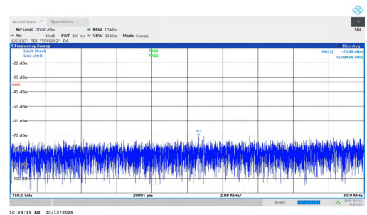
NTNV-n77(3700-3980)-PC2-30-30-L-DFT-BPSK-Inner_1RB_Left- 0.15-30-PASS
