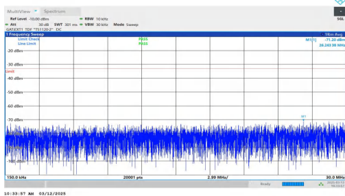
NTNV-n77(3700-3980)-PC2-30-30-M-DFT-QPSK-Inner_1RB_Rig ht-0.15-30-PASS
