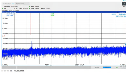
NTNV-n77(3700-3980)-PC2-30-30-L-DFT-BPSK-Inner_1RB_Left-3000-6000-PASS
