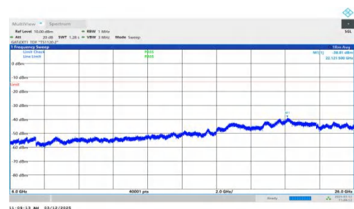
NTNV-n77(3700-3980)-PC2-30-30-H-DFT-QPSK-Inner_1RB_Left- 6000-26000-PASS
