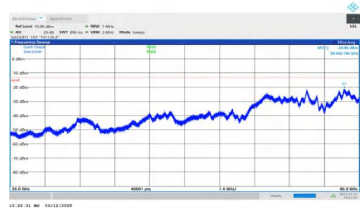
NTNV-n77(3700-3980)-PC2-30-20-H-DFT-QPSK-Inner_1RB_Righ t-26000-40000-PASS
