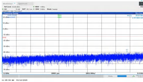
NTNV-n77(3700-3980)-PC2-30-40-H-DFT-QPSK-Inner_1RB_Rig ht-1000-3000-PASS
