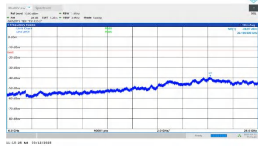
NTNV-n77(3700-3980)-PC2-30-40-L-DFT-QPSK-Inner_1RB_Left- 6000-26000-PASS
