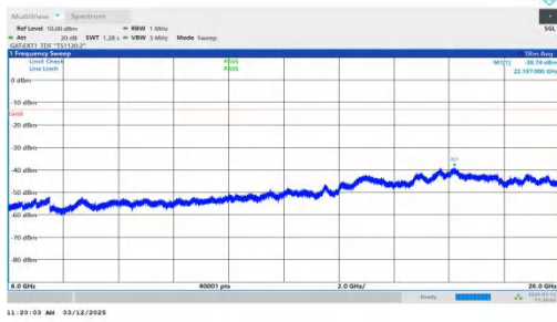
NTNV-n77(3700-3980)-PC2-30-40-M-DFT-BPSK-Inner_1RB_Rig ht-6000-26000-PASS
