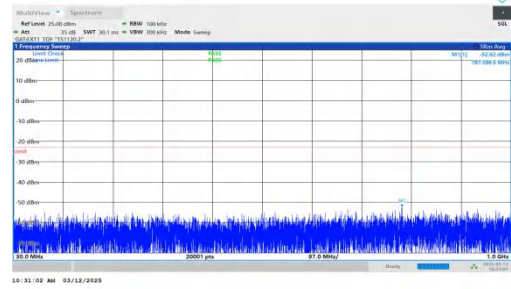
NTNV-n77(3700-3980)-PC2-30-30-M-DFT-BPSK-Inner_1RB_Righ t-30-1000-PASS
