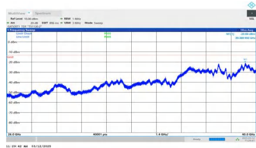
NTNV-n77(3700-3980)-PC2-30-40-H-DFT-QPSK-Inner_1RB_Righ t-26000-40000-PASS
