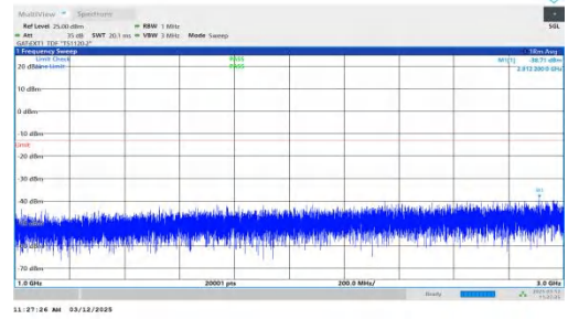
NTNV-n77(3700-3980)-PC2-30-40-H-DFT-QPSK-Inner_1RB_Left 1000-3000-PASS
