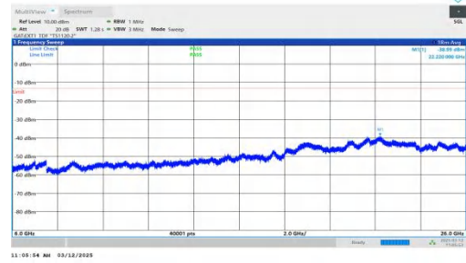
NTNV-n77(3700-3980)-PC2-30-30-H-DFT-BPSK-Inner_1RB_Left 6000-26000-PASS
