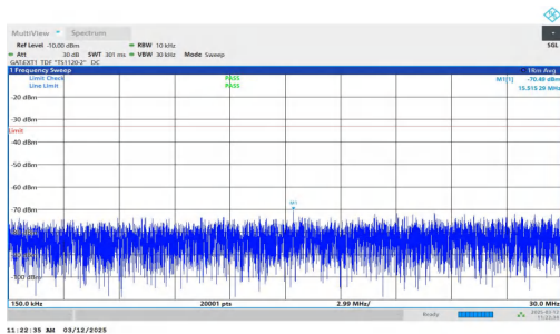
NTNV-n77(3700-3980)-PC2-30-40-M-DFT-QPSK-Inner_1RB_Rig ht-0.15-30-PASS
