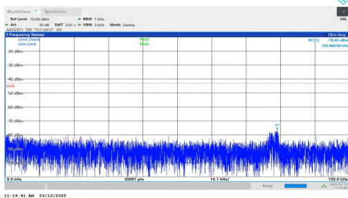
NTNV-n77(3700-3980)-PC2-30-40-L-DFT-QPSK-Inner_1RB_Left -0.009-0.15-PASS
