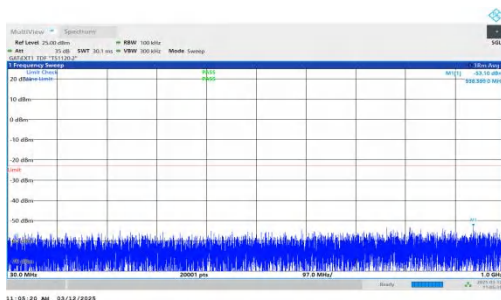
NTNV-n77(3700-3980)-PC2-30-30-H-DFT-BPSK-Inner_1RB_Left -30-1000-PASS
