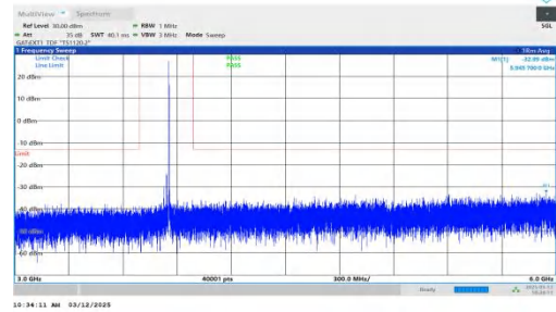
NTNV-n77(3700-3980)-PC2-30-30-M-DFT-QPSK-Inner_1RB_Righ t-3000-6000-PASS
