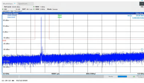
NTNV-n77(3700-3980)-PC2-30-40-M-DFT-BPSK-Inner_1RB_Left -3000-6000-PASS
