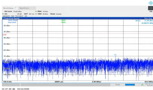
NTNV-n77(3700-3980)-PC2-30-30-L-DFT-QPSK-Inner_1RB_Rig ht-0.15-30-PASS
