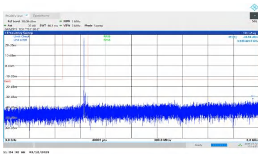
NTNV-n77(3700-3980)-PC2-30-40-H-DFT-BPSK-Inner_1RB_Left -3000-6000-PASS
