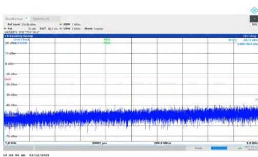
NTNV-n77(3700-3980)-PC2-30-30-L-DFT-BPSK-Inner_1RB_Rig ht-1000-3000-PASS
