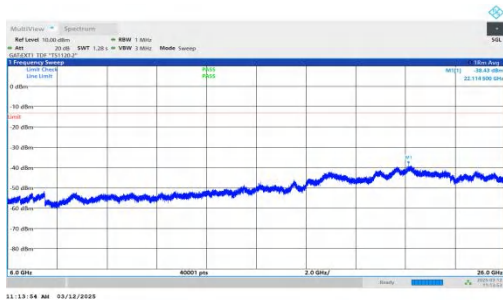
NTNV-n77(3700-3980)-PC2-30-40-L-DFT-BPSK-Inner_1RB_Rig ht-6000-26000-PASS
