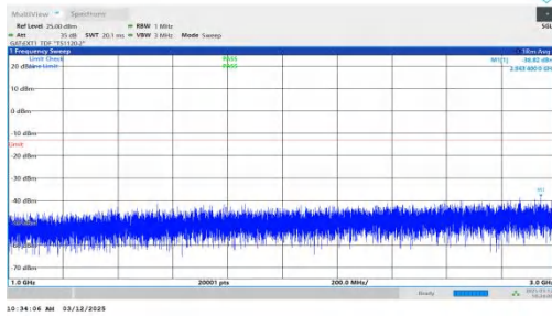
NTNV-n77(3700-3980)-PC2-30-30-M-DFT-QPSK-Inner_1RB_Rig ht-1000-3000-PASS
