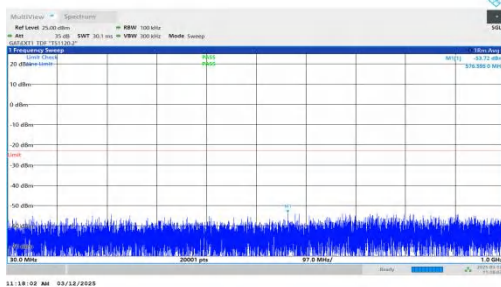
NTNV-n77(3700-3980)-PC2-30-40-M-DFT-BPSK-Inner_1RB_Left -30-1000-PASS
