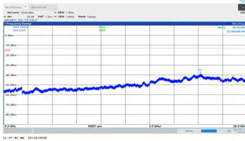
NTNV-n77(3700-3980)-PC2-30-30-H-DFT-BPSK-Inner_1RB_Rig ht-6000-26000-PASS
