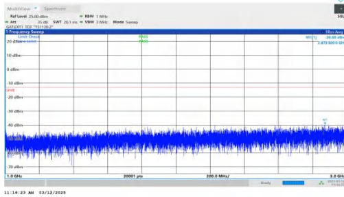
NTNV-n77(3700-3980)-PC2-30-40-L-DFT-QPSK-Inner_1RB_Rig ht-1000-3000-PASS
