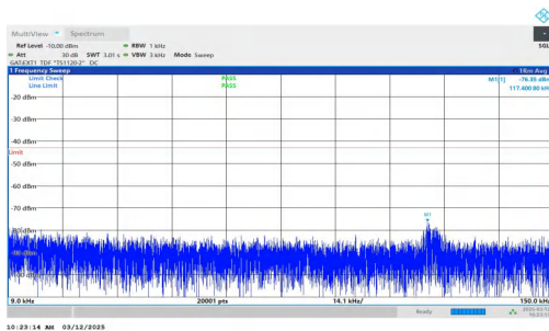
NTNV-n77(3700-3980)-PC2-30-30-L-DFT-BPSK-Inner_1RB_Left- 0.009-0.15-PASS
