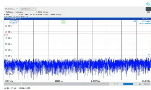
NTNV-n77(3700-3980)-PC2-30-40-M-DFT-QPSK-Inner_1RB_Left- 0.15-30-PASS
