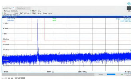
NTNV-n77(3700-3980)-PC2-30-30-M-DFT-BPSK-Inner_1RB_Left -3000-6000-PASS
