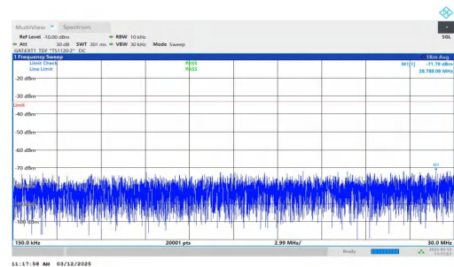
NTNV-n77(3700-3980)-PC2-30-40-M-DFT-BPSK-Inner_1RB_Left- 0.15-30-PASS
