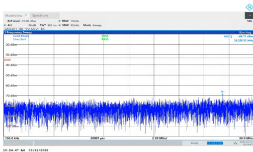
NTNV-n77(3700-3980)-PC2-30-30-L-DFT-BPSK-Inner_1RB_Rig ht-0.15-30-PASS
