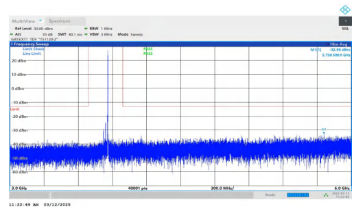
NTNV-n77(3700-3980)-PC2-30-40-M-DFT-QPSK-Inner_1RB_Righ t-3000-6000-PASS
