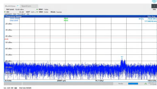
NTNV-n77(3700-3980)-PC2-30-40-L-DFT-QPSK-Inner_1RB_Right -0.009-0.15-PASS
