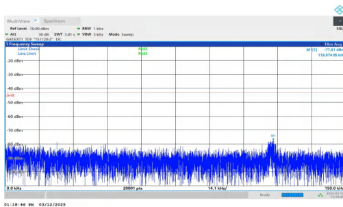
NTNV-n77(3700-3980)-PC2-30-30-H-DFT-BPSK-Inner_1RB_Left -0.009-0.15-PASS
