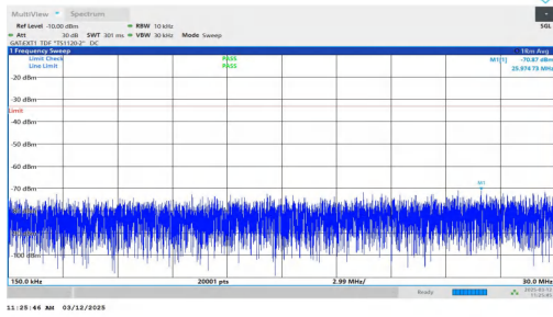
NTNV-n77(3700-3980)-PC2-30-40-H-DFT-BPSK-Inner_1RB_Rig ht-0.15-30-PASS
