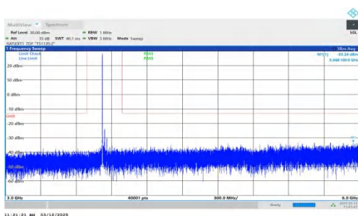
NTNV-n77(3700-3980)-PC2-30-40-M-DFT-QPSK-Inner_1RB_Lef t-3000-6000-PASS
