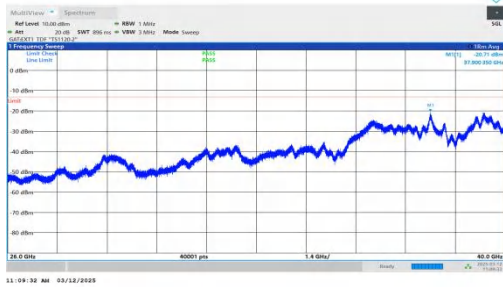
NTNV-n77(3700-3980)-PC2-30-30-H-DFT-QPSK-Inner_1RB_Left -26000-40000-PASS
