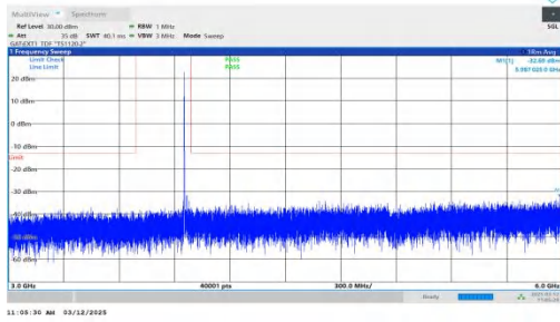
NTNV-n77(3700-3980)-PC2-30-30-H-DFT-BPSK-Inner_1RB_Left -3000-6000-PASS
