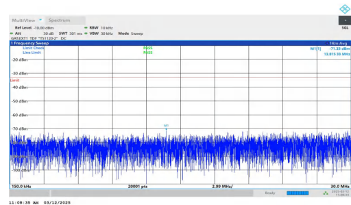
NTNV-n77(3700-3980)-PC2-30-30-H-DFT-QPSK-Inner_1RB_Left- 0.15-30-PASS
