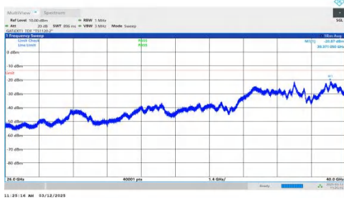
NTNV-n77(3700-3980)-PC2-30-40-H-DFT-BPSK-Inner_1RB_Left -26000-40000-PASS
