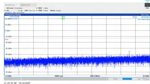
NTNV-n77(3700-3980)-PC2-30-40-M-DFT-BPSK-Inner_1RB_Left- 1000-3000-PASS
