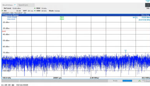
NTNV-n77(3700-3980)-PC2-30-40-H-DFT-QPSK-Inner_1RB_Rig ht-0.15-30-PASS
