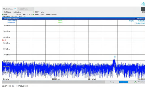
NTNV-n77(3700-3980)-PC2-30-40-M-DFT-BPSK-Inner_1RB_Left -0.009-0.15-PASS
