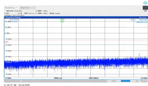
NTNV-n77(3700-3980)-PC2-30-40-H-DFT-BPSK-Inner_1RB_Left 1000-3000-PASS
