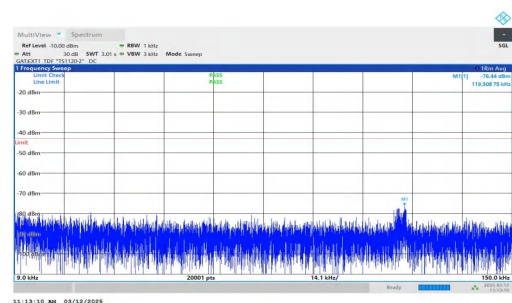
NTNV-n77(3700-3980)-PC2-30-40-L-DFT-BPSK-Inner_1RB_Right -0.009-0.15-PASS
