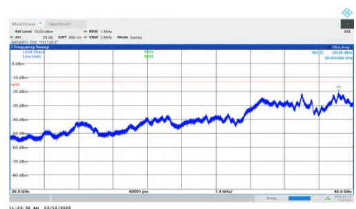
NTNV-n77(3700-3980)-PC2-30-40-M-DFT-QPSK-Inner_1RB_Righ t-26000-40000-PASS
