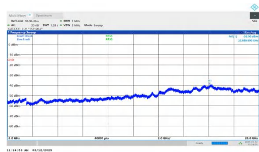
NTNV-n77(3700-3980)-PC2-30-40-H-DFT-BPSK-Inner_1RB_Left 6000-26000-PASS
