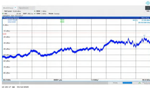
NTNV-n77(3700-3980)-PC2-30-30-L-DFT-BPSK-Inner_1RB_Left-26000-40000-PASS
