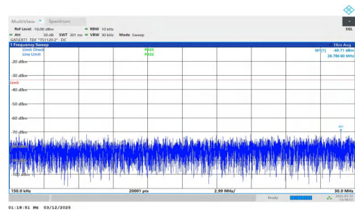
NTNV-n77(3700-3980)-PC2-30-30-H-DFT-BPSK-Inner_1RB_Left- 0.15-30-PASS
