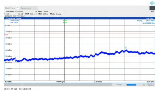
NTNV-n77(3700-3980)-PC2-30-30-M-DFT-QPSK-Inner_1RB_Left- 6000-26000-PASS
