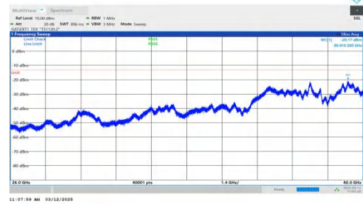
NTNV-n77(3700-3980)-PC2-30-30-H-DFT-BPSK-Inner_1RB_Righ t-26000-40000-PASS
