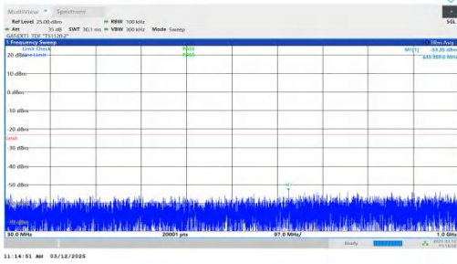
NTNV-n77(3700-3980)-PC2-30-40-L-DFT-QPSK-Inner_1RB_Left -30-1000-PASS
