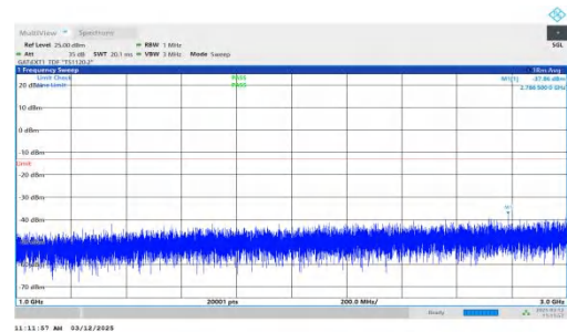
NTNV-n77(3700-3980)-PC2-30-40-L-DFT-BPSK-Inner_1RB_Left- 1000-3000-PASS
