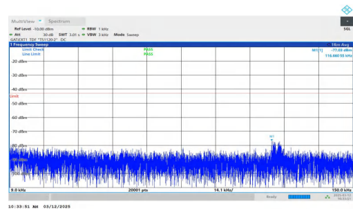
NTNV-n77(3700-3980)-PC2-30-30-M-DFT-QPSK-Inner_1RB_Right t-0.009-0.15-PASS
