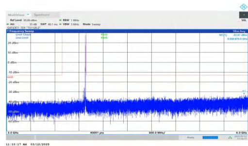
NTNV-n77(3700-3980)-PC2-30-30-H-DFT-QPSK-Inner_1RB_Right t.3000-6000-PASS
