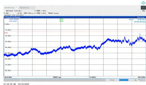
NTNV-n77(3700-3980)-PC2-30-30-M-DFT-QPSK-Inner_1RB_Righ t-26000-40000-PASS
