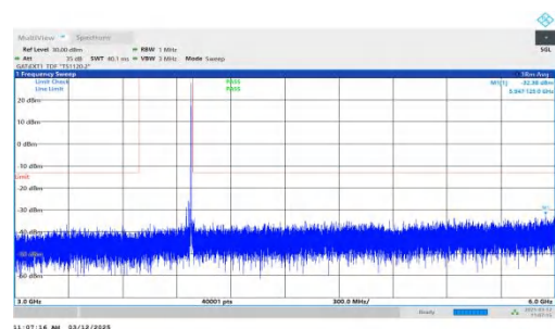
NTNV-n77(3700-3980)-PC2-30-30-H-DFT-BPSK-Inner_1RB_Right t-3000-6000-PASS
