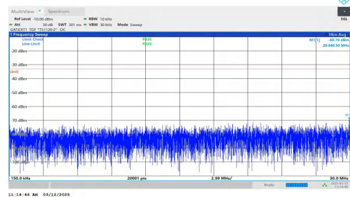
NTNV-n77(3700-3980)-PC2-30-40-L-DFT-QPSK-Inner_1RB_Left- 0.15-30-PASS
