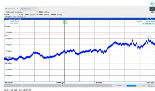
NTNV-n77(3700-3980)-PC2-30-40-L-DFT-BPSK-Inner_1RB_Right -26000-40000-PASS
