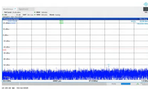
NTNV-n77(3700-3980)-PC2-30-30-L-DFT-QPSK-Inner_1RB_Left -30-1000-PASS
