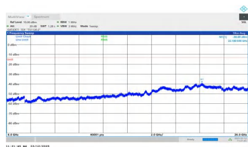
NTNV-n77(3700-3980)-PC2-30-40-M-DFT-QPSK-Inner_1RB_Left- 6000-26000-PASS
