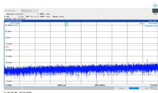
NTNV-n77(3700-3980)-PC2-30-60-L-DFT-BPSK-Inner_1RB_Left- 1000-3000-PASS
