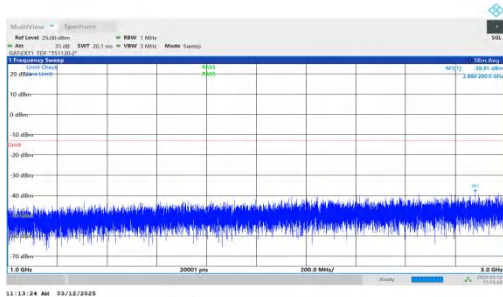
NTNV-n77(3700-3980)-PC2-30-40-L-DFT-BPSK-Inner_1RB_Rig ht-1000-3000-PASS
