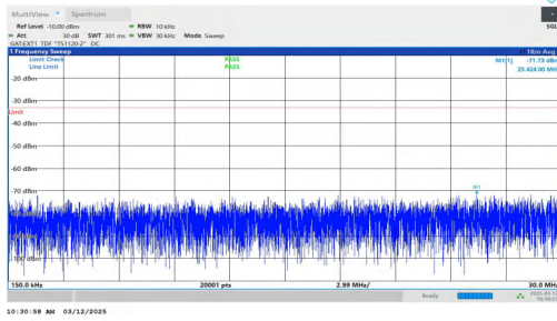
NTNV-n77(3700-3980)-PC2-30-30-M-DFT-BPSK-Inner_1RB_Rig ht-0.15-30-PASS
