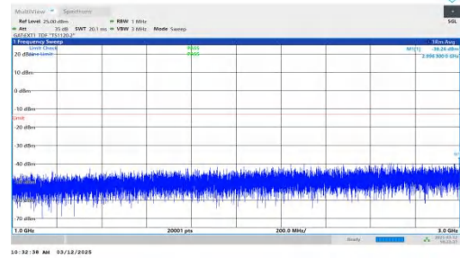
NTNV-n77(3700-3980)-PC2-30-30-M-DFT-QPSK-Inner_1RB_Left- 1000-3000-PASS
