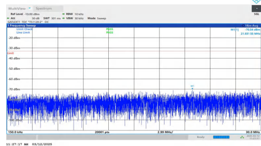
NTNV-n77(3700-3980)-PC2-30-40-H-DFT-QPSK-Inner_1RB_Left 0.15-30-PASS
