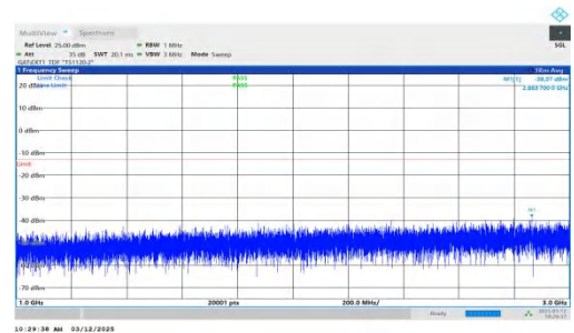
NTNV-n77(3700-3980)-PC2-30-30-M-DFT-BPSK-Inner_1RB_Left 1000-3000-PASS
