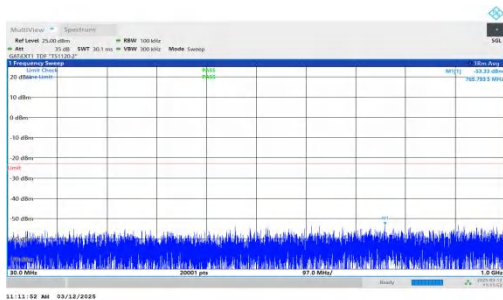
NTNV-n77(3700-3980)-PC2-30-40-L-DFT-BPSK-Inner_1RB_Left- 30-1000-PASS
