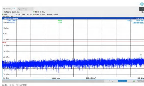
NTNV-n77(3700-3980)-PC2-30-40-M-DFT-QPSK-Inner_1RB_Rig ht-1000-3000-PASS
