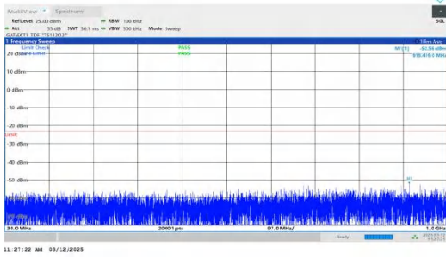
NTNV-n77(3700-3980)-PC2-30-40-H-DFT-QPSK-Inner_1RB_Left -30-1000-PASS
