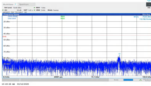
NTNV-n77(3700-3980)-PC2-30-30-M-DFT-BPSK-Inner_1RB_Left -0.009-0.15-PASS
