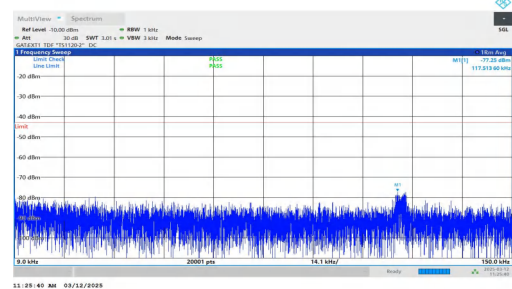
NTNV-n77(3700-3980)-PC2-30-40-H-DFT-BPSK-Inner_1RB_Right t-0.009-0.15-PASS
