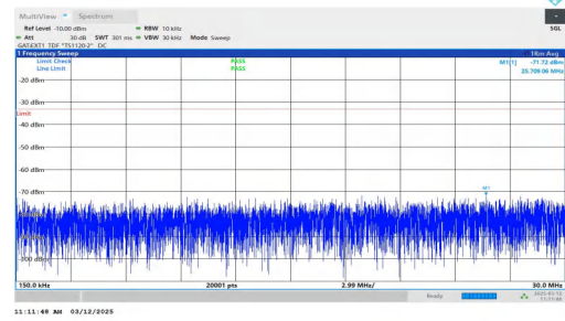
NTNV-n77(3700-3980)-PC2-30-40-L-DFT-BPSK-Inner_1RB_Left- 0.15-30-PASS
