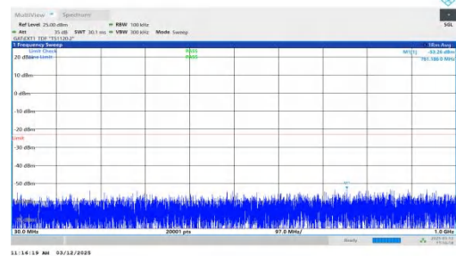
NTNV-n77(3700-3980)-PC2-30-40-L-DFT-QPSK-Inner_1RB_Right -30-1000-PASS
