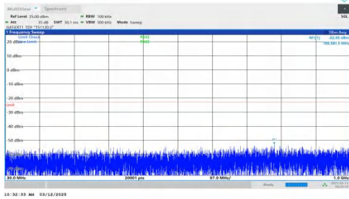
NTNV-n77(3700-3980)-PC2-30-30-M-DFT-QPSK-Inner_1RB_Lef t-30-1000-PASS
