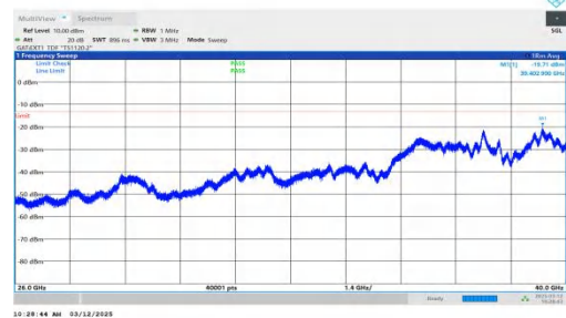
NTNV-n77(3700-3980)-PC2-30-30-L-DFT-QPSK-Inner_1RB_Right -26000-40000-PASS
