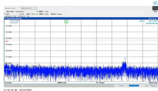
NTNV-n77(3700-3980)-PC2-30-30-H-DFT-BPSK-Inner_1RB_Right t-0.009-0.15-PASS
