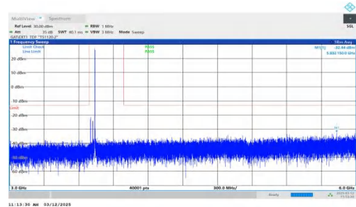
NTNV-n77(3700-3980)-PC2-30-40-L-DFT-BPSK-Inner_1RB_Right -3000-6000-PASS
