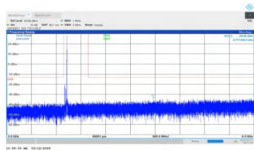
NTNV-n77(3700-3980)-PC2-30-30-L-DFT-QPSK-Inner_1RB_Right -3000-6000-PASS
