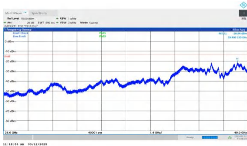
NTNV-n77(3700-3980)-PC2-30-40-M-DFT-BPSK-Inner_1RB_Left -26000-40000-PASS
