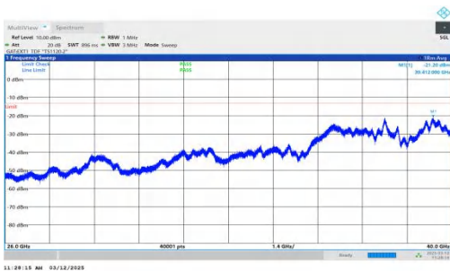
NTNV-n77(3700-3980)-PC2-30-40-H-DFT-QPSK-Inner_1RB_Left -26000-40000-PASS
