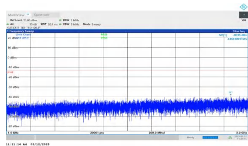
NTNV-n77(3700-3980)-PC2-30-40-M-DFT-QPSK-Inner_1RB_Left- 1000-3000-PASS
