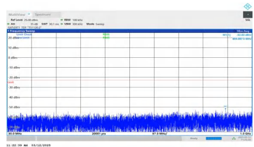
NTNV-n77(3700-3980)-PC2-30-40-M-DFT-QPSK-Inner_1RB_Righ t-30-1000-PASS
