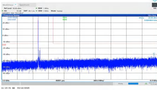
NTNV-n77(3700-3980)-PC2-30-40-L-DFT-QPSK-Inner_1RB_Left -3000-6000-PASS
