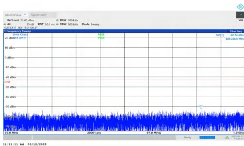
NTNV-n77(3700-3980)-PC2-30-40-M-DFT-QPSK-Inner_1RB_Lef t-30-1000-PASS
