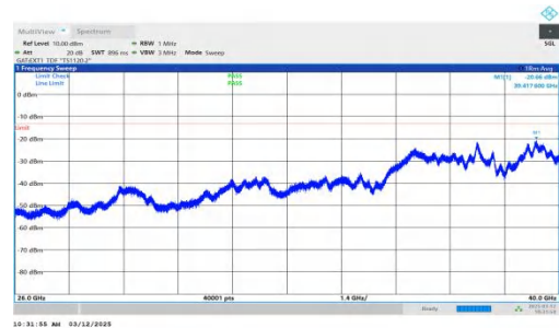
NTNV-n77(3700-3980)-PC2-30-30-M-DFT-BPSK-Inner_1RB_Righ t-26000-40000-PASS
