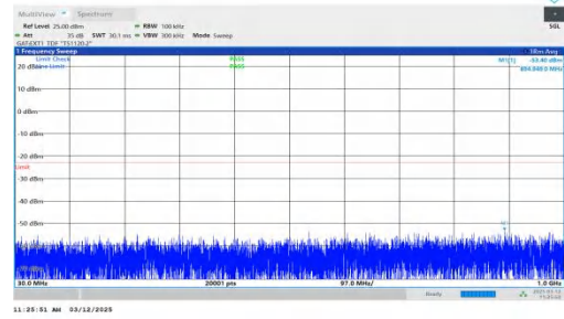
NTNV-n77(3700-3980)-PC2-30-40-H-DFT-BPSK-Inner_1RB_Righ t-30-1000-PASS
