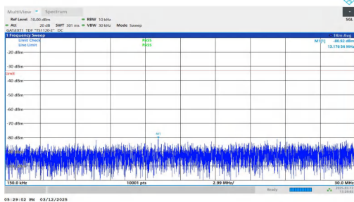
NTNV-n77(3450-3550)-PC2-30-80-L-DFT-QPSK-Inner_1RB_Rig ht-0.15-30-PASS
