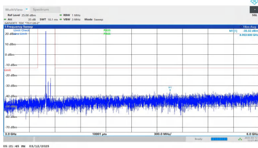
NTNV-n77(3450-3550)-PC2-30-60-H-DFT-QPSK-Inner_1RB_Left -3000-6000-PASS
