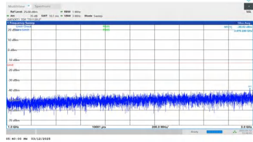
NTNV-n77(3450-3550)-PC2-30-80-H-DFT-QPSK-Inner_1RB_Left 1000-3000-PASS
