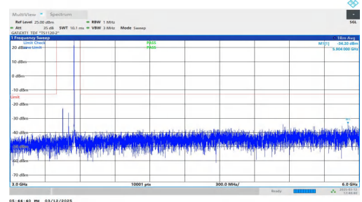
NTNV-n77(3450-3550)-PC2-30-100-L-DFT-BPSK-Inner_1RB_Rig ht-3000-6000-PASS
