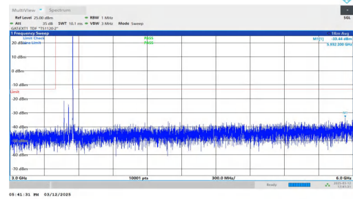
NTNV-n77(3450-3550)-PC2-30-80-H-DFT-QPSK-Inner_1RB_Righ t-3000-6000-PASS
