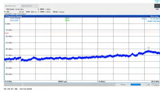
NTNV-n77(3450-3550)-PC2-30-60-L-DFT-QPSK-Inner_1RB_Left- 6000-20000-PASS
