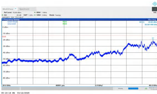
NTNV-n77(3450-3550)-PC2-30-60-M-DFT-QPSK-Inner_1RB_Lef t-20000-40000-PASS
