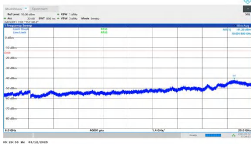
NTNV-n77(3450-3550)-PC2-30-80-L-DFT-QPSK-Inner_1RB_Rig ht-6000-20000-PASS
