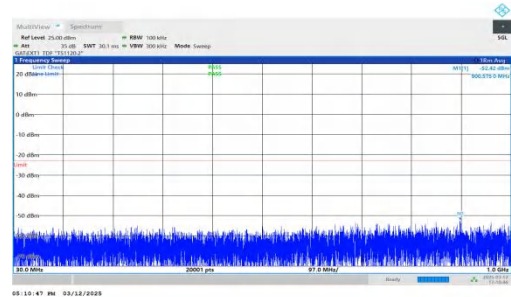
NTNV-n77(3450-3550)-PC2-30-60-L-DFT-QPSK-Inner_1RB_Right -30-1000-PASS
