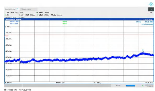
NTNV-n77(3450-3550)-PC2-30-80-L-DFT-BPSK-Inner_1RB_Left- 6000-20000-PASS
