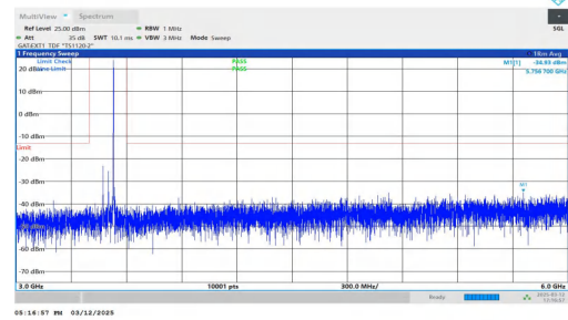
NTNV-n77(3450-3550)-PC2-30-60-M-DFT-QPSK-Inner_1RB_Righ t-3000-6000-PASS
