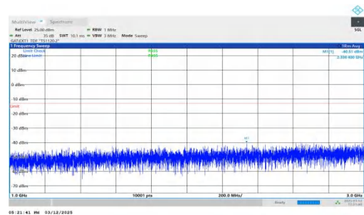
NTNV-n77(3450-3550)-PC2-30-60-H-DFT-QPSK-Inner_1RB_Left- 1000-3000-PASS
