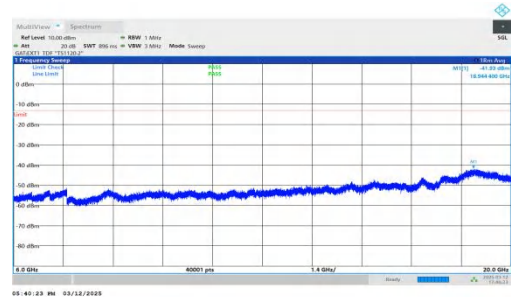
NTNV-n77(3450-3550)-PC2-30-80-H-DFT-QPSK-Inner_1RB_Left 6000-20000-PASS
