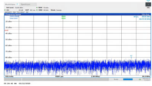
NTNV-n77(3450-3550)-PC2-30-80-L-DFT-BPSK-Inner_1RB_Left- 0.15-30-PASS
