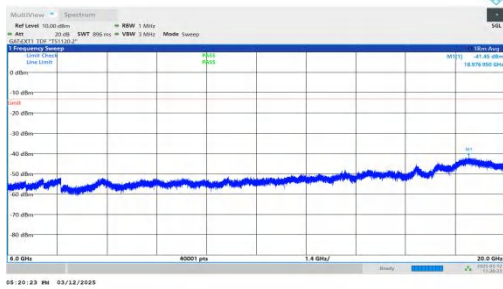
NTNV-n77(3450-3550)-PC2-30-60-H-DFT-BPSK-Inner_1RB_Rig ht-6000-20000-PASS
