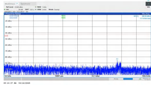
NTNV-n77(3450-3550)-PC2-30-60-L-DFT-QPSK-Inner_1RB_Right -0.009-0.15-PASS
