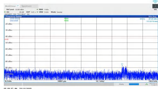
NTNV-n77(3450-3550)-PC2-30-80-L-DFT-QPSK-Inner_1RB_Right -0.009-0.15-PASS
