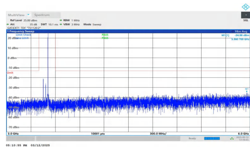
NTNV-n77(3450-3550)-PC2-30-60-L-DFT-QPSK-Inner_1RB_Right -3000-6000-PASS
