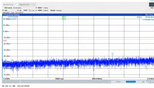
NTNV-n77(3450-3550)-PC2-30-80-L-DFT-QPSK-Inner_1RB_Rig ht-1000-3000-PASS
