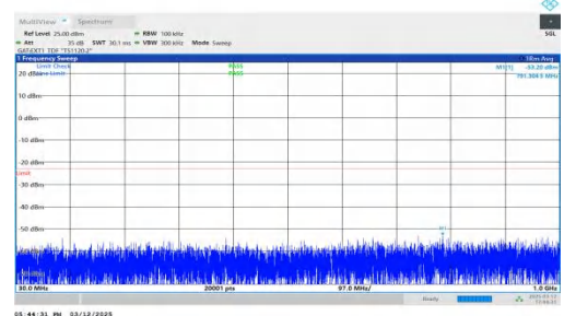
NTNV-n77(3450-3550)-PC2-30-100-L-DFT-BPSK-Inner_1RB_Rig ht-30-1000-PASS
