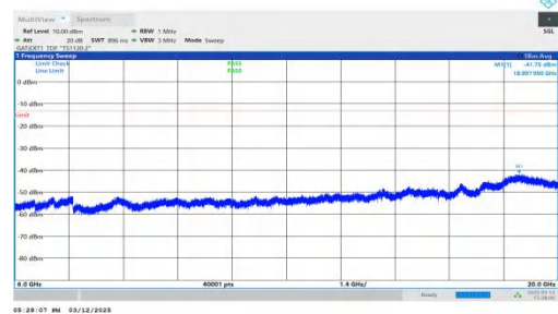
NTNV-n77(3450-3550)-PC2-30-80-L-DFT-QPSK-Inner_1RB_Left- 6000-20000-PASS
