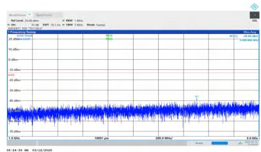
NTNV-n77(3450-3550)-PC2-30-80-L-DFT-BPSK-Inner_1RB_Left- 1000-3000-PASS
