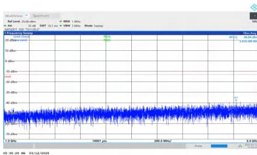
NTNV-n77(3450-3550)-PC2-30-80-M-DFT-QPSK-Inner_1RB_Rig ht-1000-3000-PASS
