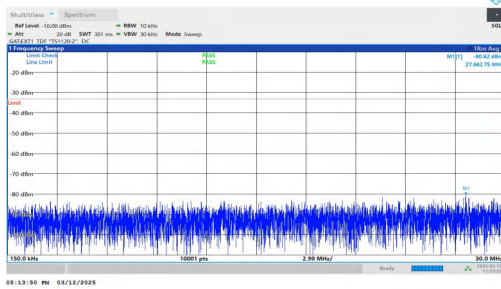
NTNV-n77(3450-3550)-PC2-30-60-M-DFT-BPSK-Inner_1RB_Rig ht-0.15-30-PASS
