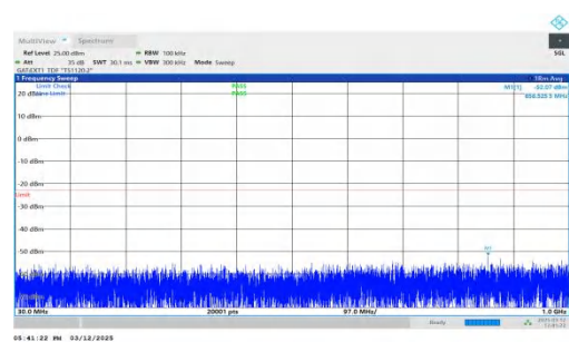
NTNV-n77(3450-3550)-PC2-30-80-H-DFT-QPSK-Inner_1RB_Right t-30-1000-PASS
