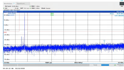
NTNV-n77(3450-3550)-PC2-30-80-L-DFT-QPSK-Inner_1RB_Right -3000-6000-PASS
