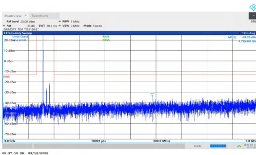
NTNV-n77(3450-3550)-PC2-30-80-H-DFT-BPSK-Inner_1RB_Left -3000-6000-PASS
