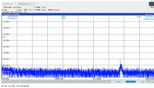
NTNV-n77(3450-3550)-PC2-30-60-M-DFT-BPSK-Inner_1RB_Left -0.009-0.15-PASS
