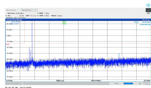
NTNV-n77(3450-3550)-PC2-30-60-H-DFT-BPSK-Inner_1RB_Right t=3000-6000-PASS
