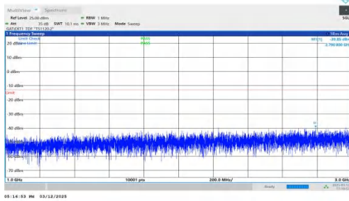
NTNV-n77(3450-3550)-PC2-30-60-M-DFT-QPSK-Inner_1RB_Rig ht-1000-3000-PASS
