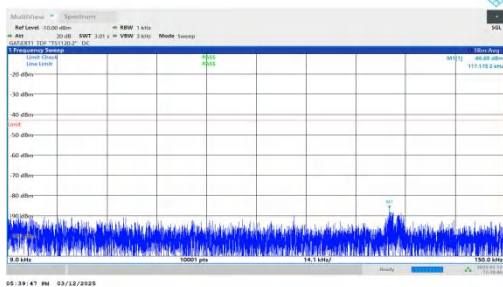
NTNV-n77(3450-3550)-PC2-30-80-H-DFT-QPSK-Inner_1RB_Left -0.009-0.15-PASS
