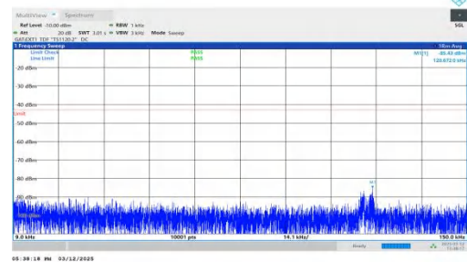
NTNV-n77(3450-3550)-PC2-30-80-H-DFT-BPSK-Inner_1RB_Right t-0.009-0.15-PASS
