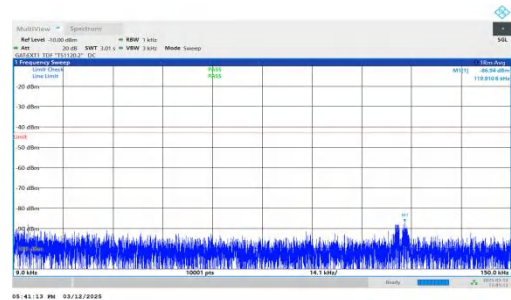
NTNV-n77(3450-3550)-PC2-30-80-H-DFT-QPSK-Inner_1RB_Right t-0.009-0.15-PASS
