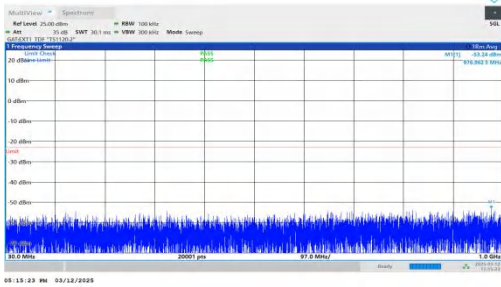
NTNV-n77(3450-3550)-PC2-30-60-M-DFT-QPSK-Inner_1RB_Lef t-30-1000-PASS
