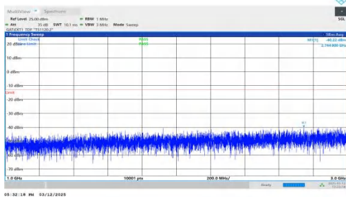
NTNV-n77(3450-3550)-PC2-30-80-M-DFT-BPSK-Inner_1RB_Rig ht-1000-3000-PASS
