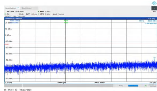
NTNV-n77(3450-3550)-PC2-30-80-H-DFT-BPSK-Inner_1RB_Left 1000-3000-PASS
