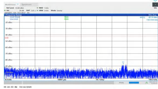
NTNV-n77(3450-3550)-PC2-30-60-H-DFT-QPSK-Inner_1RB_Right t.009-0.15-PASS
