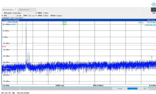
NTNV-n77(3450-3550)-PC2-30-60-M-DFT-BPSK-Inner_1RB_Left -3000-6000-PASS
