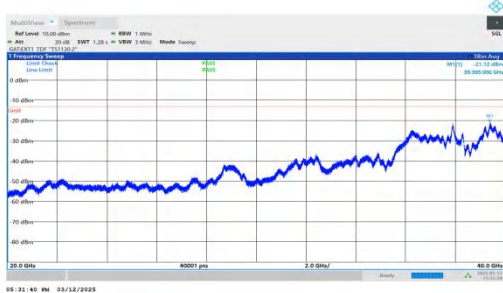
NTNV-n77(3450-3550)-PC2-30-80-M-DFT-BPSK-Inner_1RB_Left -20000-40000-PASS
