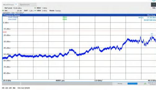
NTNV-n77(3450-3550)-PC2-30-60-H-DFT-QPSK-Inner_1RB_Left -20000-40000-PASS
