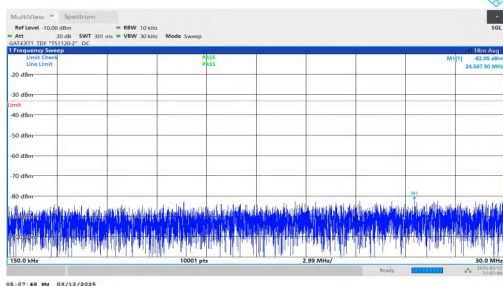
NTNV-n77(3450-3550)-PC2-30-60-L-DFT-BPSK-Inner_1RB_Rig ht-0.15-30-PASS
