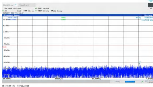
NTNV-n77(3450-3550)-PC2-30-80-M-DFT-BPSK-Inner_1RB_Left -30-1000-PASS
