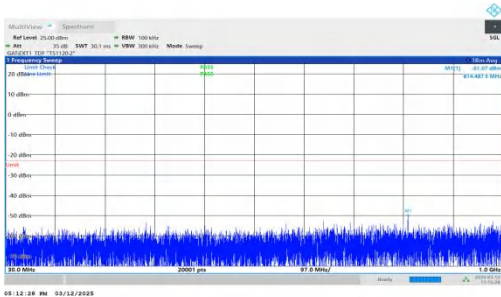
NTNV-n77(3450-3550)-PC2-30-60-M-DFT-BPSK-Inner_1RB_Left -30-1000-PASS
