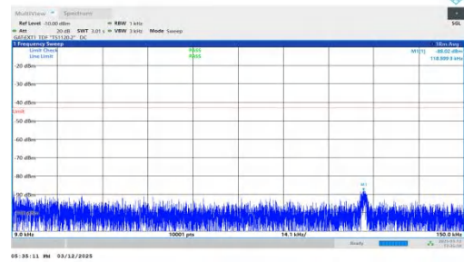
NTNV-n77(3450-3550)-PC2-30-80-M-DFT-QPSK-Inner_1RB_Righ t-0.009-0.15-PASS
