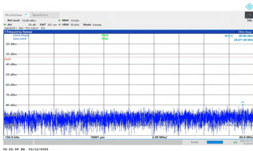
NTNV-n77(3450-3550)-PC2-30-60-H-DFT-QPSK-Inner_1RB_Right ht.0.15-30-PASS
