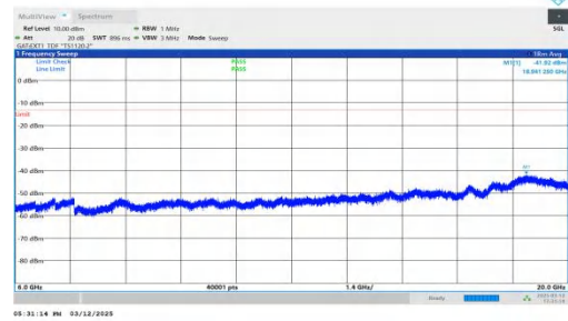
NTNV-n77(3450-3550)-PC2-30-80-M-DFT-BPSK-Inner_1RB_Left 6000-20000-PASS
