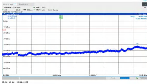
NTNV-n77(3450-3550)-PC2-30-80-M-DFT-BPSK-Inner_1RB_Rig ht-6000-20000-PASS
