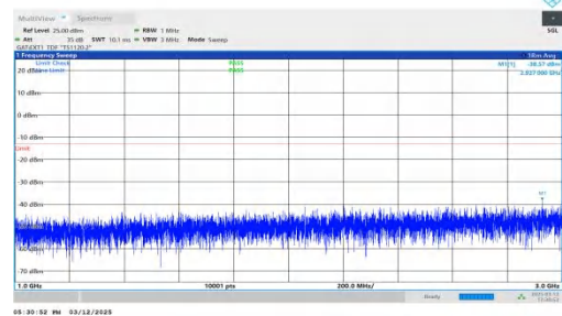
NTNV-n77(3450-3550)-PC2-30-80-M-DFT-BPSK-Inner_1RB_Left- 1000-3000-PASS
