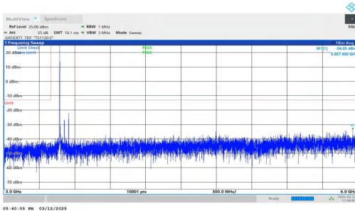
NTNV-n77(3450-3550)-PC2-30-80-H-DFT-QPSK-Inner_1RB_Left -3000-6000-PASS
