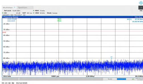
NTNV-n77(3450-3550)-PC2-30-60-L-DFT-QPSK-Inner_1RB_Rig ht-0.15-30-PASS
