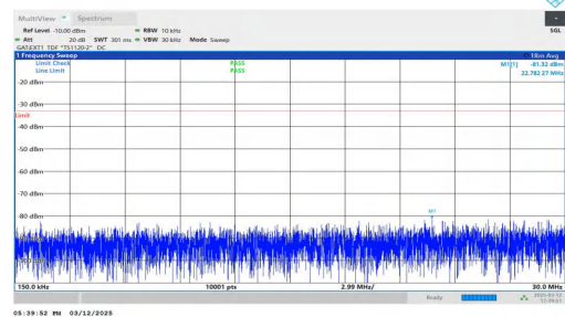
NTNV-n77(3450-3550)-PC2-30-80-H-DFT-QPSK-Inner_1RB_Left 0.15-30-PASS
