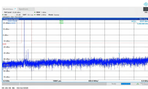
NTNV-n77(3450-3550)-PC2-30-80-L-DFT-BPSK-Inner_1RB_Left- 3000-6000-PASS
