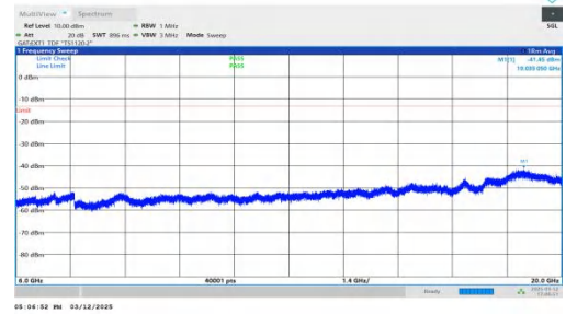
NTNV-n77(3450-3550)-PC2-30-60-L-DFT-BPSK-Inner_1RB_Left-6000-20000-PASS
