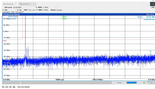
NTNV-n77(3450-3550)-PC2-30-60-L-DFT-BPSK-Inner_1RB_Left-3000-6000-PASS
