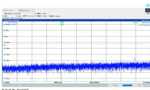
NTNV-n77(3450-3550)-PC2-30-60-H-DFT-BPSK-Inner_1RB_Right ht=1000-3000-PASS
