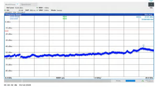
NTNV-n77(3450-3550)-PC2-30-100-L-DFT-BPSK-Inner_1RB_Left -6000-20000-PASS
