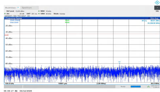
NTNV-n77(3450-3550)-PC2-30-60-L-DFT-QPSK-Inner_1RB_Left- 0.15-30-PASS
