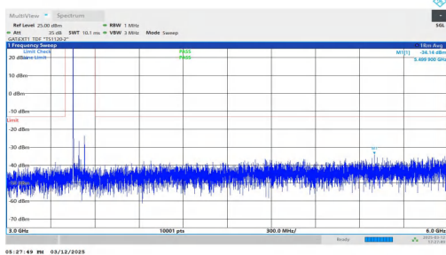
NTNV-n77(3450-3550)-PC2-30-80-L-DFT-QPSK-Inner_1RB_Left -3000-6000-PASS
