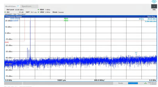
NTNV-n77(3450-3550)-PC2-30-60-L-DFT-BPSK-Inner_1RB_Right-3000-6000-PASS
