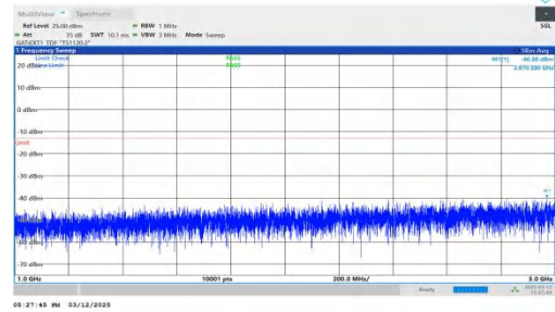
NTNV-n77(3450-3550)-PC2-30-80-L-DFT-QPSK-Inner_1RB_Left- 1000-3000-PASS
