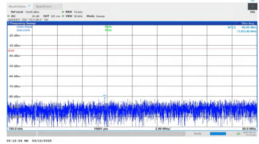
NTNV-n77(3450-3550)-PC2-30-60-M-DFT-BPSK-Inner_1RB_Left 0.15-30-PASS
