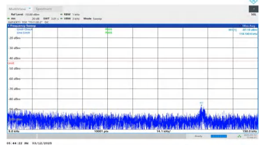
NTNV-n77(3450-3550)-PC2-30-100-L-DFT-BPSK-Inner_1RB_Rig ht-0.009-0.15-PASS
