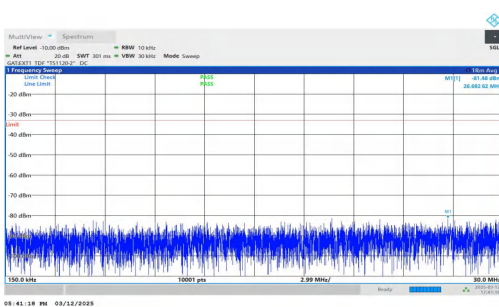
NTNV-n77(3450-3550)-PC2-30-80-H-DFT-QPSK-Inner_1RB_Rig ht-0.15-30-PASS
