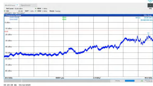
NTNV-n77(3450-3550)-PC2-30-80-L-DFT-QPSK-Inner_1RB_Right -20000-40000-PASS
