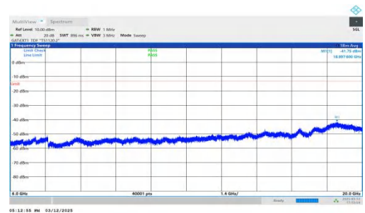
NTNV-n77(3450-3550)-PC2-30-60-M-DFT-BPSK-Inner_1RB_Left 6000-20000-PASS
