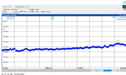
NTNV-n77(3450-3550)-PC2-30-60-M-DFT-QPSK-Inner_1RB_Rig ht-6000-20000-PASS
