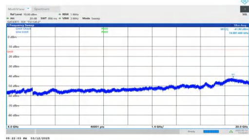
NTNV-n77(3450-3550)-PC2-30-60-H-DFT-QPSK-Inner_1RB_Left- 6000-20000-PASS
