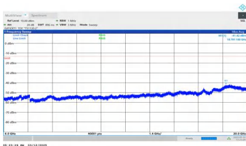
NTNV-n77(3450-3550)-PC2-30-60-H-DFT-QPSK-Inner_1RB_Right ht.6000-20000-PASS
