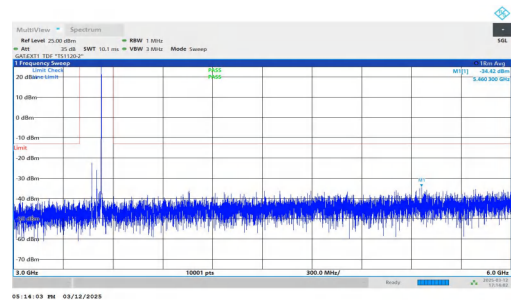
NTNV-n77(3450-3550)-PC2-30-60-M-DFT-BPSK-Inner_1RB_Righ t-3000-6000-PASS
