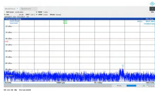
NTNV-n77(3450-3550)-PC2-30-60-M-DFT-QPSK-Inner_1RB_Right t-0.009-0.15-PASS
