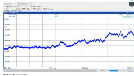
NTNV-n77(3450-3550)-PC2-30-60-L-DFT-BPSK-Inner_1RB_Right -20000-40000-PASS
