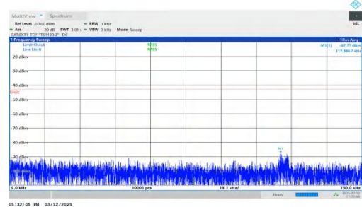
NTNV-n77(3450-3550)-PC2-30-80-M-DFT-BPSK-Inner_1RB_Right t-0.009-0.15-PASS
