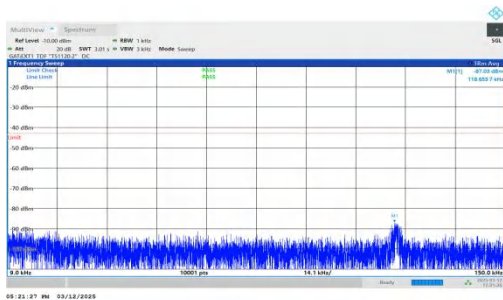
NTNV-n77(3450-3550)-PC2-30-60-H-DFT-QPSK-Inner_1RB_Left -0.009-0.15-PASS
