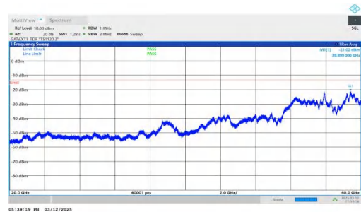
NTNV-n77(3450-3550)-PC2-30-80-H-DFT-BPSK-Inner_1RB_Righ t-20000-40000-PASS
