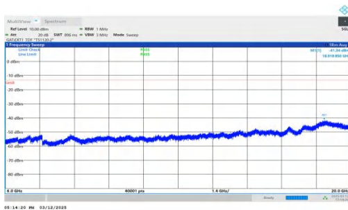
NTNV-n77(3450-3550)-PC2-30-60-M-DFT-BPSK-Inner_1RB_Rig ht-6000-20000-PASS
