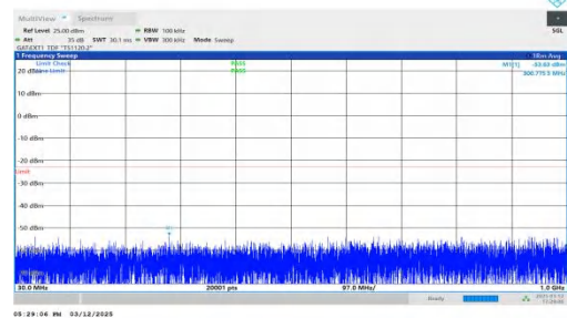
NTNV-n77(3450-3550)-PC2-30-80-L-DFT-QPSK-Inner_1RB_Right -30-1000-PASS
