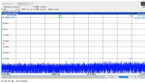
NTNV-n77(3450-3550)-PC2-30-80-H-DFT-QPSK-Inner_1RB_Left -30-1000-PASS
