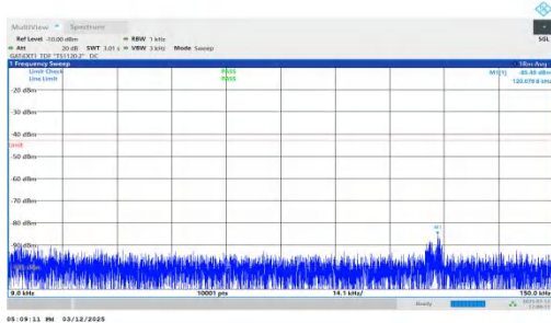
NTNV-n77(3450-3550)-PC2-30-60-L-DFT-QPSK-Inner_1RB_Left -0.009-0.15-PASS
