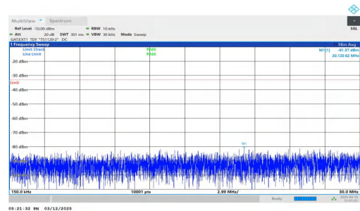
NTNV-n77(3450-3550)-PC2-30-60-H-DFT-QPSK-Inner_1RB_Left- 0.15-30-PASS
