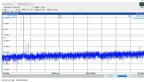
NTNV-n77(3450-3550)-PC2-30-100-L-DFT-BPSK-Inner_1RB_Lef t-3000-6000-PASS
