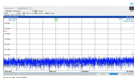
NTNV-n77(3450-3550)-PC2-30-60-M-DFT-QPSK-Inner_1RB_Left- 0.15-30-PASS
