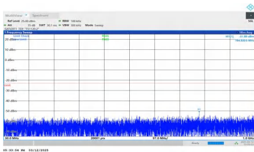
NTNV-n77(3450-3550)-PC2-30-80-M-DFT-QPSK-Inner_1RB_Lef t-30-1000-PASS
