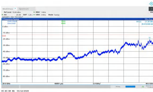
NTNV-n77(3450-3550)-PC2-30-80-H-DFT-QPSK-Inner_1RB_Left -20000-40000-PASS
