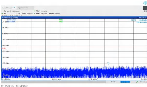
NTNV-n77(3450-3550)-PC2-30-80-H-DFT-BPSK-Inner_1RB_Left -30-1000-PASS
