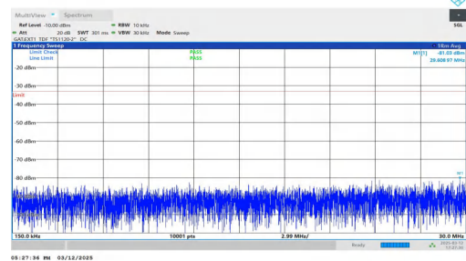
NTNV-n77(3450-3550)-PC2-30-80-L-DFT-QPSK-Inner_1RB_Left- 0.15-30-PASS
