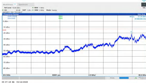
NTNV-n77(3450-3550)-PC2-30-60-L-DFT-BPSK-Inner_1RB_Left-20000-40000-PASS
