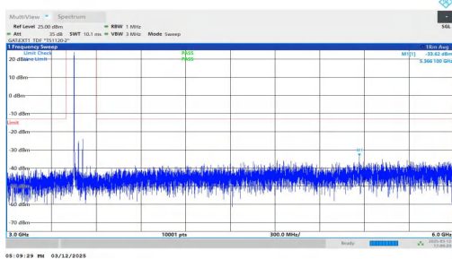
NTNV-n77(3450-3550)-PC2-30-60-L-DFT-QPSK-Inner_1RB_Left -3000-6000-PASS
