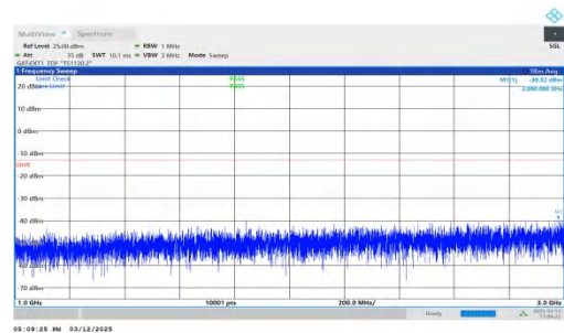
NTNV-n77(3450-3550)-PC2-30-60-L-DFT-QPSK-Inner_1RB_Left- 1000-3000-PASS
