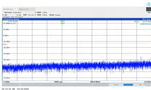
NTNV-n77(3450-3550)-PC2-30-60-L-DFT-QPSK-Inner_1RB_Rig ht-1000-3000-PASS
