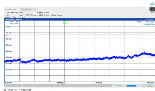
NTNV-n77(3450-3550)-PC2-30-80-H-DFT-BPSK-Inner_1RB_Left 6000-20000-PASS
