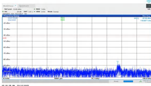
NTNV-n77(3450-3550)-PC2-30-80-M-DFT-BPSK-Inner_1RB_Left -0.009-0.15-PASS
