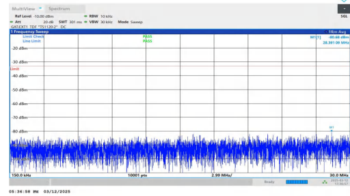
NTNV-n77(3450-3550)-PC2-30-80-H-DFT-BPSK-Inner_1RB_Left 0.15-30-PASS
