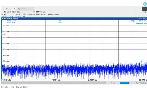
NTNV-n77(3450-3550)-PC2-30-60-M-DFT-QPSK-Inner_1RB_Rig ht-0.15-30-PASS
