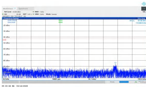
NTNV-n77(3450-3550)-PC2-30-80-M-DFT-QPSK-Inner_1RB_Lef t-0.009-0.15-PASS
