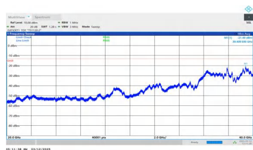
NTNV-n77(3450-3550)-PC2-30-60-L-DFT-QPSK-Inner_1RB_Right -20000-40000-PASS
