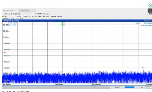
NTNV-n77(3450-3550)-PC2-30-60-H-DFT-BPSK-Inner_1RB_Left -30-1000-PASS
