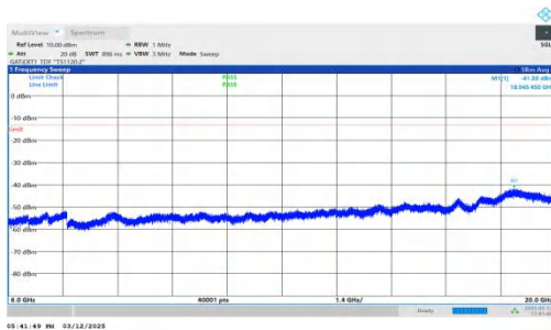
NTNV-n77(3450-3550)-PC2-30-80-H-DFT-QPSK-Inner_1RB_Rig ht-6000-20000-PASS
