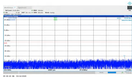
NTNV-n77(3450-3550)-PC2-30-80-M-DFT-QPSK-Inner_1RB_Righ t-30-1000-PASS
