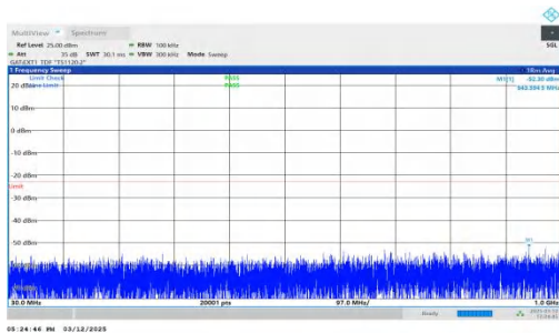
NTNV-n77(3450-3550)-PC2-30-80-L-DFT-BPSK-Inner_1RB_Left- 30-1000-PASS
