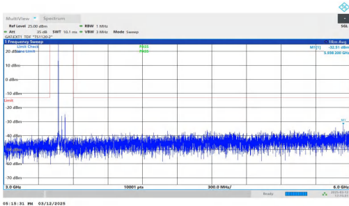
NTNV-n77(3450-3550)-PC2-30-60-M-DFT-QPSK-Inner_1RB_Lef t-3000-6000-PASS
