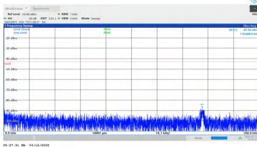
NTNV-n77(3450-3550)-PC2-30-80-L-DFT-QPSK-Inner_1RB_Left -0.009-0.15-PASS
