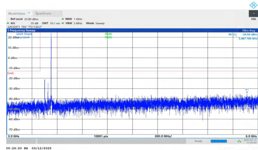
NTNV-n77(3450-3550)-PC2-30-80-L-DFT-BPSK-Inner_1RB_Right -3000-6000-PASS
