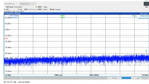
NTNV-n77(3450-3550)-PC2-30-60-M-DFT-QPSK-Inner_1RB_Left- 1000-3000-PASS
