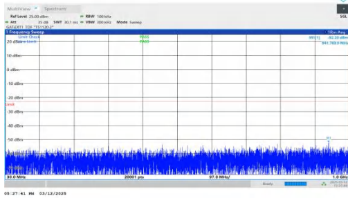
NTNV-n77(3450-3550)-PC2-30-80-L-DFT-QPSK-Inner_1RB_Left -30-1000-PASS
