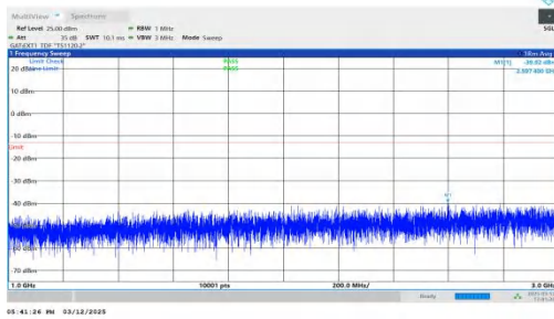
NTNV-n77(3450-3550)-PC2-30-80-H-DFT-QPSK-Inner_1RB_Rig ht-1000-3000-PASS
