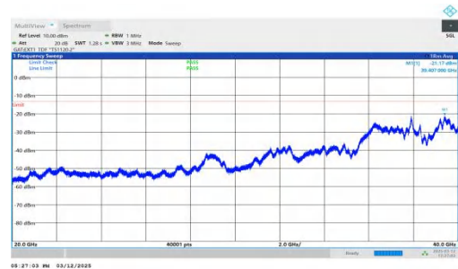
NTNV-n77(3450-3550)-PC2-30-80-L-DFT-BPSK-Inner_1RB_Right -20000-40000-PASS
