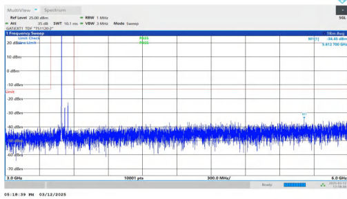
NTNV-n77(3450-3550)-PC2-30-60-H-DFT-BPSK-Inner_1RB_Left -3000-6000-PASS
