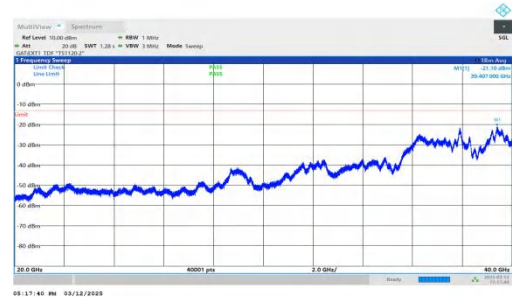
NTNV-n77(3450-3550)-PC2-30-60-M-DFT-QPSK-Inner_1RB_Righ t-20000-40000-PASS
