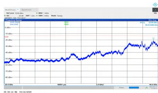
NTNV-n77(3450-3550)-PC2-30-80-M-DFT-QPSK-Inner_1RB_Righ t-20000-40000-PASS
