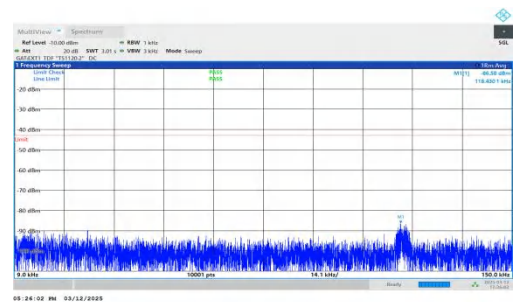
NTNV-n77(3450-3550)-PC2-30-80-L-DFT-BPSK-Inner_1RB_Right -0.009-0.15-PASS
