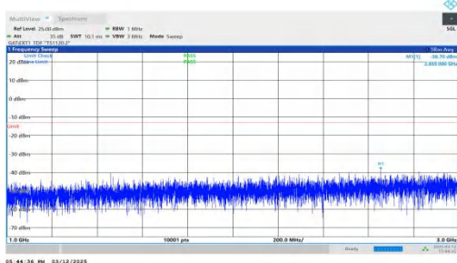
NTNV-n77(3450-3550)-PC2-30-100-L-DFT-BPSK-Inner_1RB_Ri ght-1000-3000-PASS
