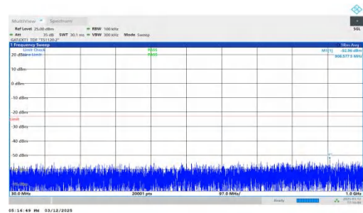
NTNV-n77(3450-3550)-PC2-30-60-M-DFT-QPSK-Inner_1RB_Right t-30-1000-PASS
