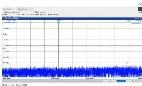
NTNV-n77(3450-3550)-PC2-30-100-L-DFT-BPSK-Inner_1RB_Lef t-30-1000-PASS
