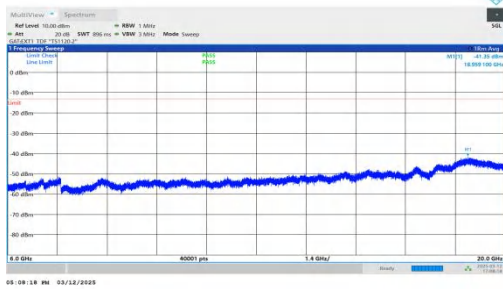
NTNV-n77(3450-3550)-PC2-30-60-L-DFT-BPSK-Inner_1RB_Rig ht-6000-20000-PASS
