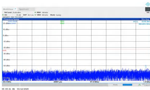
NTNV-n77(3450-3550)-PC2-30-60-L-DFT-QPSK-Inner_1RB_Left -30-1000-PASS
