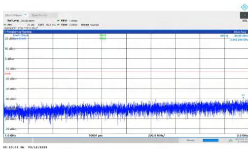
NTNV-n77(3450-3550)-PC2-30-60-H-DFT-QPSK-Inner_1RB_Right ht.1000-3000-PASS
