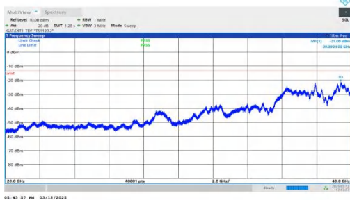
NTNV-n77(3450-3550)-PC2-30-100-L-DFT-BPSK-Inner_1RB_Lef t-20000-40000-PASS
