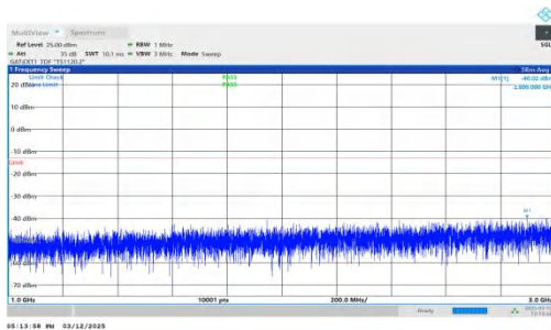
NTNV-n77(3450-3550)-PC2-30-60-M-DFT-BPSK-Inner_1RB_Rig ht-1000-3000-PASS
