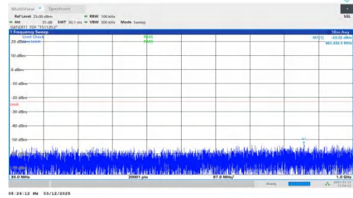
NTNV-n77(3450-3550)-PC2-30-80-L-DFT-BPSK-Inner_1RB_Right -30-1000-PASS
