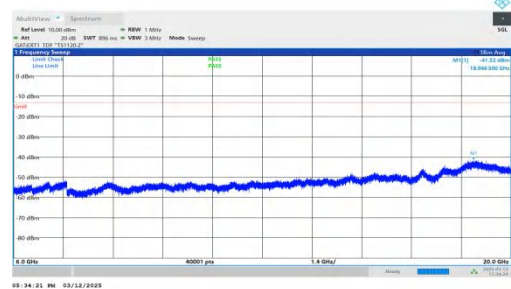
NTNV-n77(3450-3550)-PC2-30-80-M-DFT-QPSK-Inner_1RB_Left- 6000-20000-PASS
