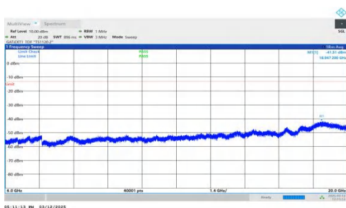
NTNV-n77(3450-3550)-PC2-30-60-L-DFT-QPSK-Inner_1RB_Rig ht-6000-20000-PASS
