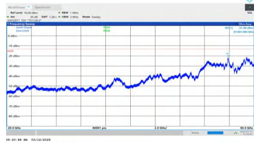
NTNV-n77(3450-3550)-PC2-30-60-H-DFT-BPSK-Inner_1RB_Righ t-20000-40000-PASS
