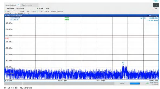
NTNV-n77(3450-3550)-PC2-30-60-M-DFT-BPSK-Inner_1RB_Right t-0.009-0.15-PASS
