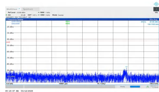
NTNV-n77(3450-3550)-PC2-30-60-H-DFT-BPSK-Inner_1RB_Right t=0.009-0.15-PASS
