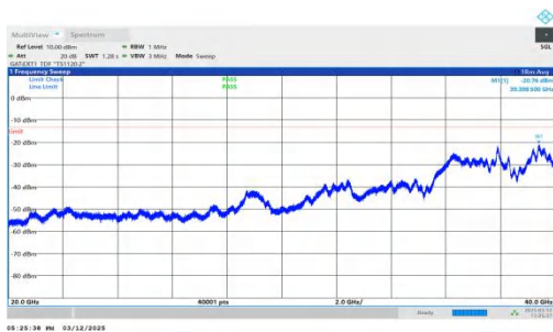
NTNV-n77(3450-3550)-PC2-30-80-L-DFT-BPSK-Inner_1RB_Left- 20000-40000-PASS
