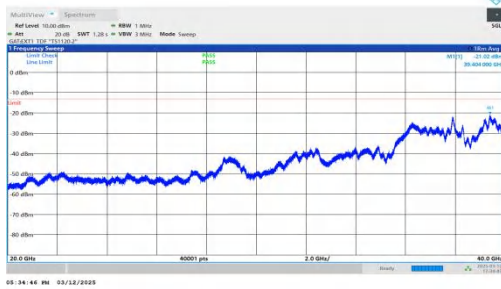
NTNV-n77(3450-3550)-PC2-30-80-M-DFT-QPSK-Inner_1RB_Lef t-20000-40000-PASS
