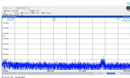
NTNV-n77(3450-3550)-PC2-30-60-H-DFT-BPSK-Inner_1RB_Left -0.009-0.15-PASS
