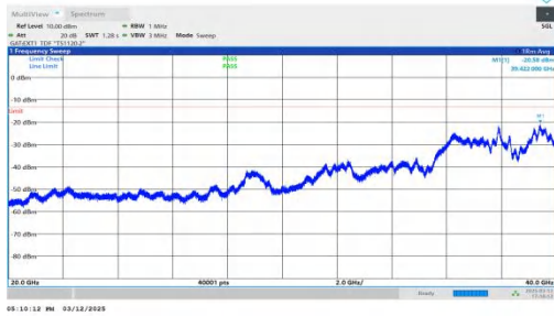
NTNV-n77(3450-3550)-PC2-30-60-L-DFT-QPSK-Inner_1RB_Left -20000-40000-PASS
