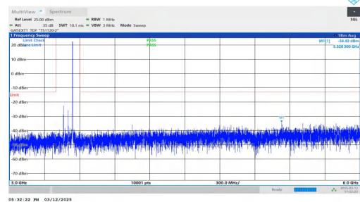
NTNV-n77(3450-3550)-PC2-30-80-M-DFT-BPSK-Inner_1RB_Right t-3000-6000-PASS
