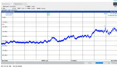
NTNV-n77(3450-3550)-PC2-30-60-M-DFT-BPSK-Inner_1RB_Left -20000-40000-PASS
