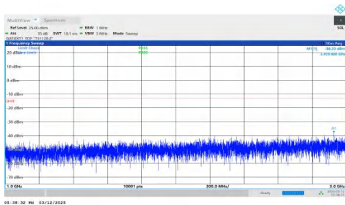
NTNV-n77(3450-3550)-PC2-30-80-H-DFT-BPSK-Inner_1RB_Rig ht-1000-3000-PASS
