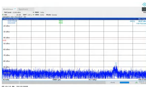
NTNV-n77(3450-3550)-PC2-30-60-M-DFT-QPSK-Inner_1RB_Lef t-0.009-0.15-PASS
