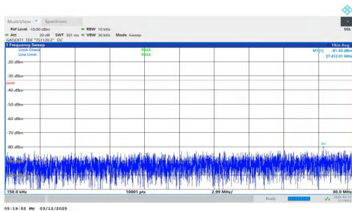
NTNV-n77(3450-3550)-PC2-30-60-H-DFT-BPSK-Inner_1RB_Right ht=0.15-30-PASS
