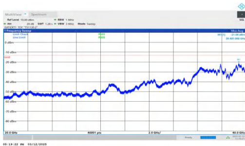
NTNV-n77(3450-3550)-PC2-30-60-H-DFT-BPSK-Inner_1RB_Left -20000-40000-PASS
