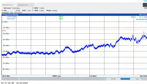
NTNV-n77(3450-3550)-PC2-30-80-H-DFT-BPSK-Inner_1RB_Left -20000-40000-PASS
