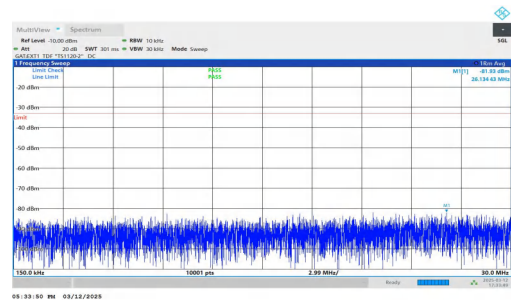
NTNV-n77(3450-3550)-PC2-30-80-M-DFT-QPSK-Inner_1RB_Left- 0.15-30-PASS
