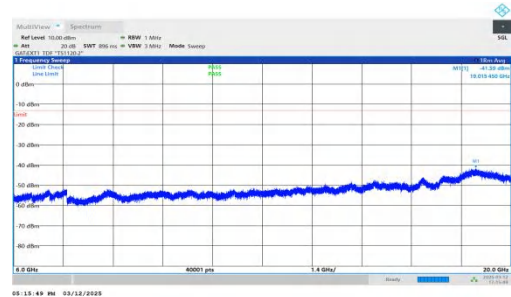
NTNV-n77(3450-3550)-PC2-30-60-M-DFT-QPSK-Inner_1RB_Left- 6000-20000-PASS
