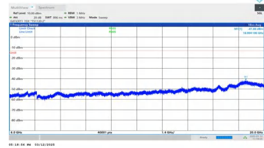
NTNV-n77(3450-3550)-PC2-30-60-H-DFT-BPSK-Inner_1RB_Left 6000-20000-PASS
