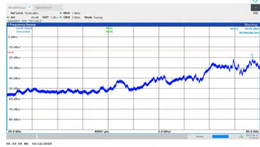
NTNV-n77(3450-3550)-PC2-30-80-M-DFT-BPSK-Inner_1RB_Righ t-20000-40000-PASS
