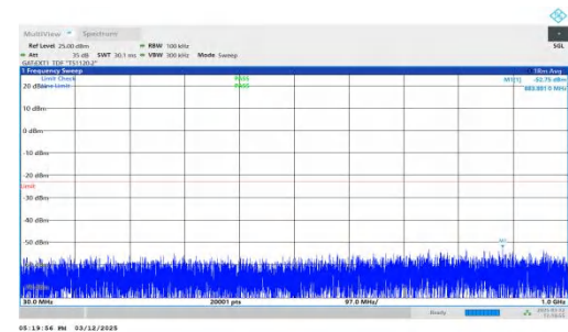
NTNV-n77(3450-3550)-PC2-30-60-H-DFT-BPSK-Inner_1RB_Right t=30-1000-PASS
