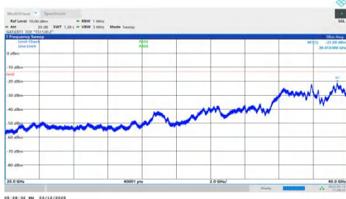
NTNV-n77(3450-3550)-PC2-30-80-L-DFT-QPSK-Inner_1RB_Left -20000-40000-PASS
