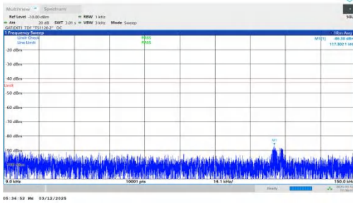
NTNV-n77(3450-3550)-PC2-30-80-H-DFT-BPSK-Inner_1RB_Left -0.009-0.15-PASS
