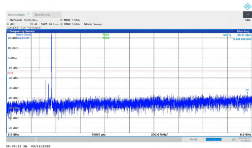
NTNV-n77(3450-3550)-PC2-30-80-H-DFT-BPSK-Inner_1RB_Righ t-3000-6000-PASS
