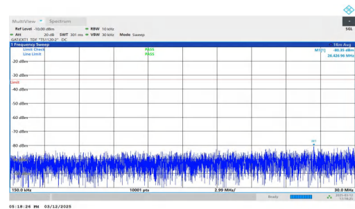
NTNV-n77(3450-3550)-PC2-30-60-H-DFT-BPSK-Inner_1RB_Left- 0.15-30-PASS
