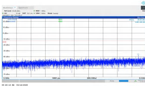
NTNV-n77(3450-3550)-PC2-30-80-L-DFT-BPSK-Inner_1RB_Rig ht-1000-3000-PASS
