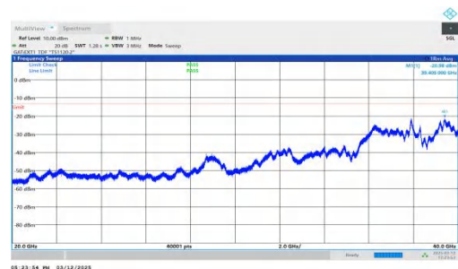
NTNV-n77(3450-3550)-PC2-30-60-H-DFT-QPSK-Inner_1RB_Right t.20000-40000-PASS
