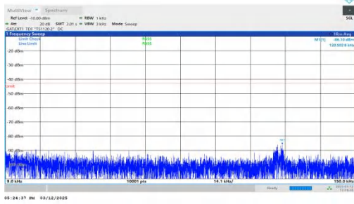
NTNV-n77(3450-3550)-PC2-30-80-L-DFT-BPSK-Inner_1RB_Left- 0.009-0.15-PASS
