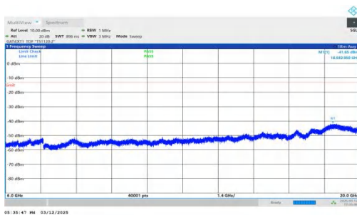
NTNV-n77(3450-3550)-PC2-30-80-M-DFT-QPSK-Inner_1RB_Rig ht-6000-20000-PASS
