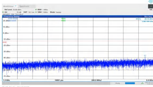
NTNV-n77(3450-3550)-PC2-30-60-L-DFT-BPSK-Inner_1RB_Rig ht-1000-3000-PASS
