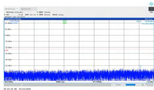
NTNV-n77(3450-3550)-PC2-30-60-H-DFT-QPSK-Inner_1RB_Right t.30-1000-PASS
