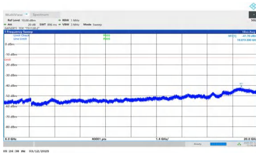
NTNV-n77(3450-3550)-PC2-30-80-L-DFT-BPSK-Inner_1RB_Rig ht-6000-20000-PASS
