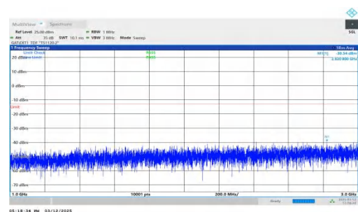
NTNV-n77(3450-3550)-PC2-30-60-H-DFT-BPSK-Inner_1RB_Left- 1000-3000-PASS
