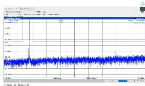
NTNV-n77(3450-3550)-PC2-30-60-H-DFT-QPSK-Inner_1RB_Right t.3000-6000-PASS
