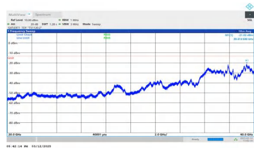
NTNV-n77(3450-3550)-PC2-30-80-H-DFT-QPSK-Inner_1RB_Righ t-20000-40000-PASS
