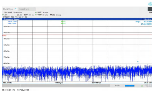
NTNV-n77(3450-3550)-PC2-30-80-M-DFT-QPSK-Inner_1RB_Rig ht-0.15-30-PASS
