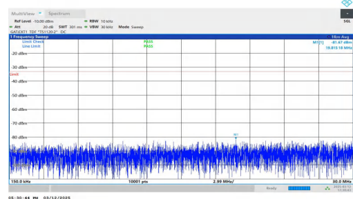
NTNV-n77(3450-3550)-PC2-30-80-M-DFT-BPSK-Inner_1RB_Left- 0.15-30-PASS
