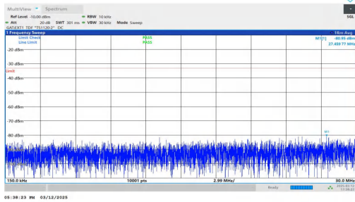
NTNV-n77(3450-3550)-PC2-30-80-H-DFT-BPSK-Inner_1RB_Rig ht-0.15-30-PASS
