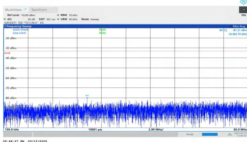
NTNV-n77(3450-3550)-PC2-30-100-L-DFT-BPSK-Inner_1RB_Ri ght-0.15-30-PASS
