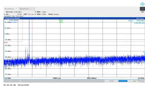
NTNV-n77(3450-3550)-PC2-30-80-M-DFT-QPSK-Inner_1RB_Righ t-3000-6000-PASS
