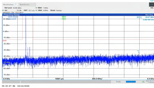
NTNV-n77(3450-3550)-PC2-30-80-M-DFT-BPSK-Inner_1RB_Left -3000-6000-PASS
