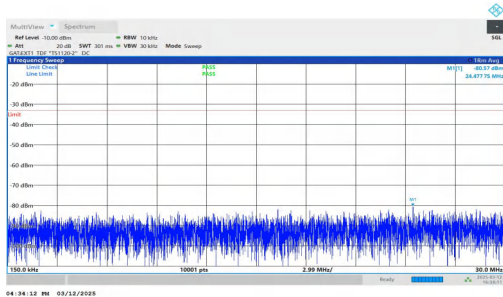
NTNV-n77(3450-3550)-PC2-30-30-L-DFT-QPSK-Inner_1RB_Rig ht-0.15-30-PASS
