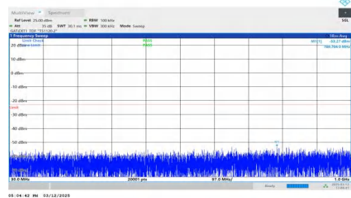
NTNV-n77(3450-3550)-PC2-30-40-H-DFT-QPSK-Inner_1RB_Right t-30-1000-PASS
