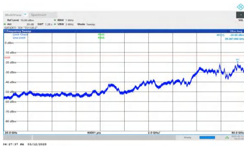
NTNV-n77(3450-3550)-PC2-30-20-H-DFT-QPSK-Inner_1RB_Left -20000-40000-PASS
