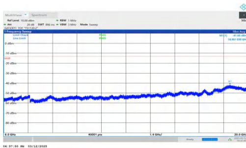
NTNV-n77(3450-3550)-PC2-30-30-M-DFT-BPSK-Inner_1RB_Rig ht-6000-20000-PASS
