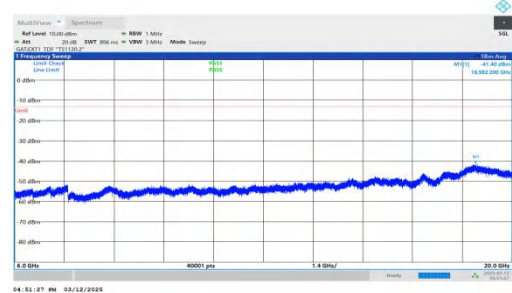
NTNV-n77(3450-3550)-PC2-30-40-L-DFT-QPSK-Inner_1RB_Left- 6000-20000-PASS
