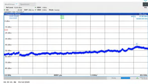
NTNV-n77(3450-3550)-PC2-30-30-L-DFT-BPSK-Inner_1RB_Left-6000-20000-PASS
