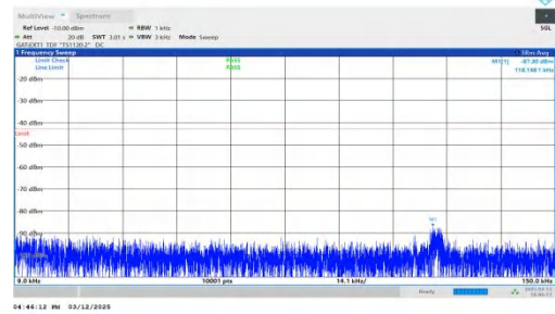
NTNV-n77(3450-3550)-PC2-30-30-H-DFT-QPSK-Inner_1RB_Right t.009-0.15-PASS
