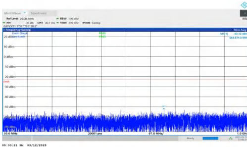
NTNV-n77(3450-3550)-PC2-30-40-H-DFT-BPSK-Inner_1RB_Left -30-1000-PASS
