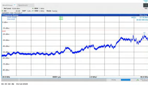
NTNV-n77(3450-3550)-PC2-30-30-L-DFT-BPSK-Inner_1RB_Left-20000-40000-PASS
