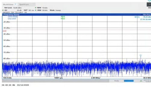
NTNV-n77(3450-3550)-PC2-30-40-L-DFT-BPSK-Inner_1RB_Rig ht-0.15-30-PASS
