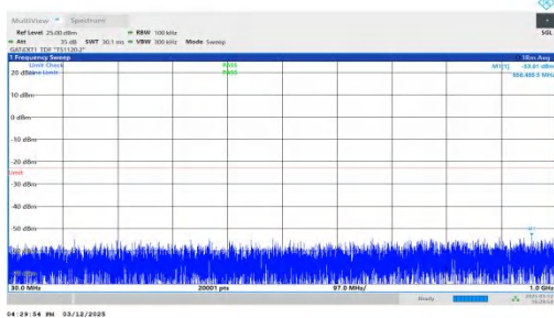
NTNV-n77(3450-3550)-PC2-30-30-L-DFT-BPSK-Inner_1RB_Left- 30-1000-PASS
