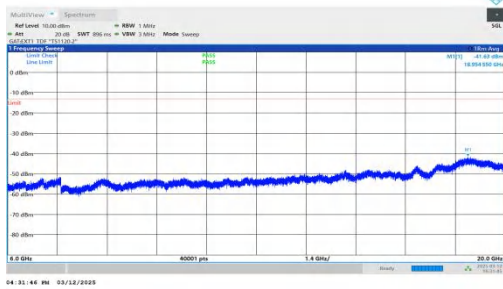
NTNV-n77(3450-3550)-PC2-30-30-L-DFT-BPSK-Inner_1RB_Rig ht-6000-20000-PASS
