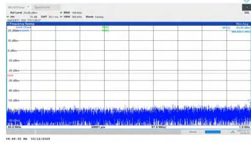
NTNV-n77(3450-3550)-PC2-30-40-L-DFT-BPSK-Inner_1RB_Right -30-1000-PASS
