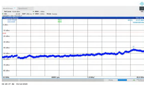
NTNV-n77(3450-3550)-PC2-30-20-H-DFT-QPSK-Inner_1RB_Rig ht-6000-20000-PASS
