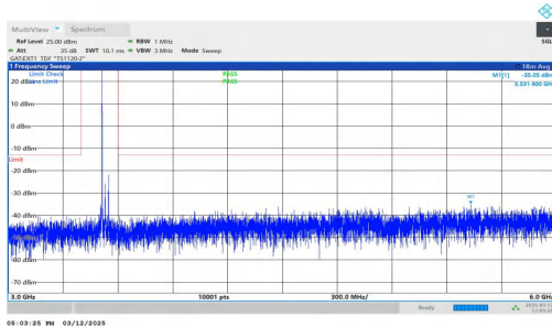
NTNV-n77(3450-3550)-PC2-30-40-H-DFT-QPSK-Inner_1RB_Left -3000-6000-PASS
