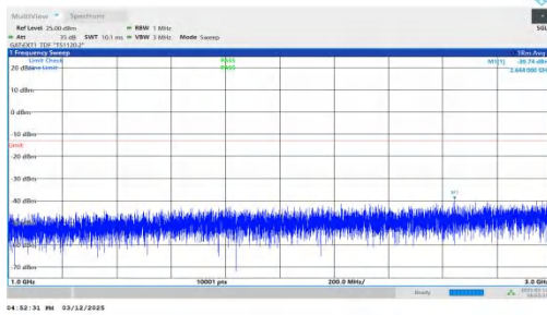
NTNV-n77(3450-3550)-PC2-30-40-L-DFT-QPSK-Inner_1RB_Rig ht-1000-3000-PASS
