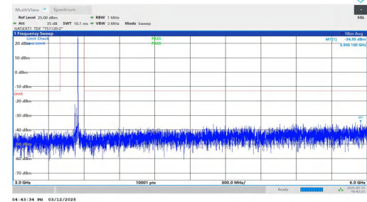
NTNV-n77(3450-3550)-PC2-30-30-H-DFT-BPSK-Inner_1RB_Right t-3000-6000-PASS
