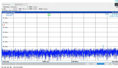
NTNV-n77(3450-3550)-PC2-30-40-H-DFT-QPSK-Inner_1RB_Rig ht-0.15-30-PASS
