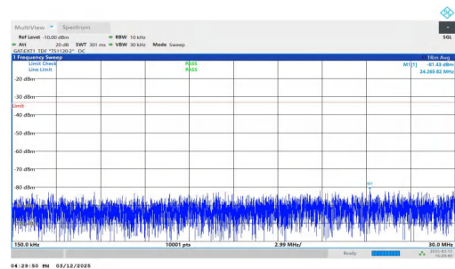
NTNV-n77(3450-3550)-PC2-30-30-L-DFT-BPSK-Inner_1RB_Left- 0.15-30-PASS
