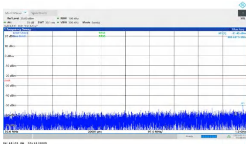
NTNV-n77(3450-3550)-PC2-30-40-L-DFT-BPSK-Inner_1RB_Left- 30-1000-PASS
