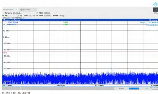
NTNV-n77(3450-3550)-PC2-30-40-M-DFT-QPSK-Inner_1RB_Lef t-30-1000-PASS
