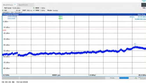
NTNV-n77(3450-3550)-PC2-30-40-M-DFT-QPSK-Inner_1RB_Rig ht-6000-20000-PASS
