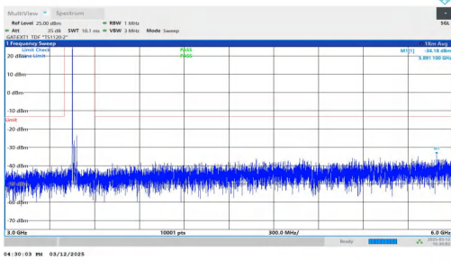
NTNV-n77(3450-3550)-PC2-30-30-L-DFT-BPSK-Inner_1RB_Left-3000-6000-PASS
