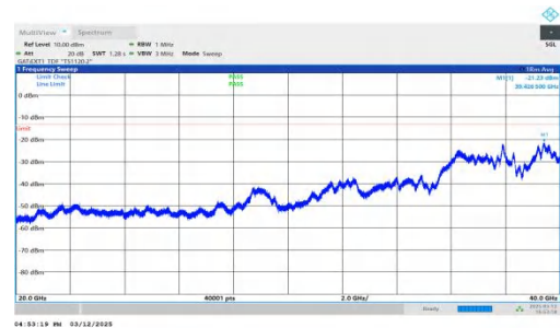
NTNV-n77(3450-3550)-PC2-30-40-L-DFT-QPSK-Inner_1RB_Right -20000-40000-PASS
