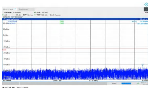
NTNV-n77(3450-3550)-PC2-30-40-M-DFT-BPSK-Inner_1RB_Left -30-1000-PASS
