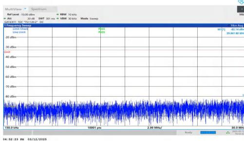
NTNV-n77(3450-3550)-PC2-30-40-L-DFT-QPSK-Inner_1RB_Rig ht-0.15-30-PASS
