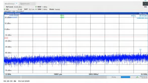
NTNV-n77(3450-3550)-PC2-30-20-H-DFT-QPSK-Inner_1RB_Left 1000-3000-PASS
