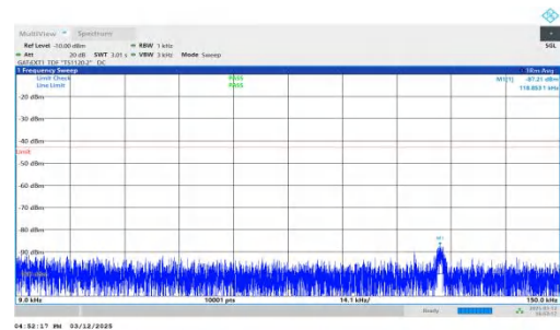
NTNV-n77(3450-3550)-PC2-30-40-L-DFT-QPSK-Inner_1RB_Right -0.009-0.15-PASS
