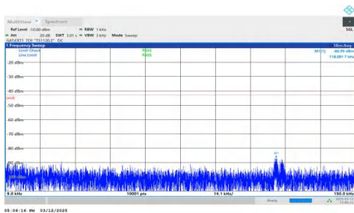
NTNV-n77(3450-3550)-PC2-30-60-L-DFT-BPSK-Inner_1RB_Left- 0.009-0.15-PASS
