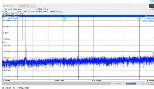
NTNV-n77(3450-3550)-PC2-30-30-L-DFT-QPSK-Inner_1RB_Left -3000-6000-PASS
