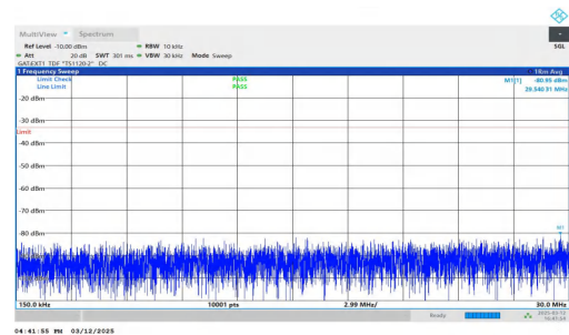
NTNV-n77(3450-3550)-PC2-30-30-H-DFT-BPSK-Inner_1RB_Left- 0.15-30-PASS
