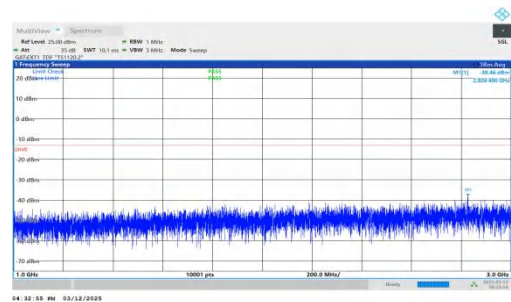
NTNV-n77(3450-3550)-PC2-30-30-L-DFT-QPSK-Inner_1RB_Left- 1000-3000-PASS
