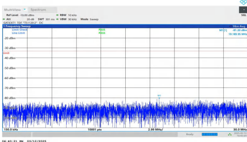
NTNV-n77(3450-3550)-PC2-30-30-H-DFT-BPSK-Inner_1RB_Rig ht-0.15-30-PASS
