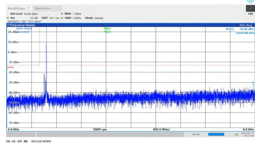
NTNV-n77(3450-3550)-PC2-30-30-L-DFT-BPSK-Inner_1RB_Right-3000-6000-PASS
