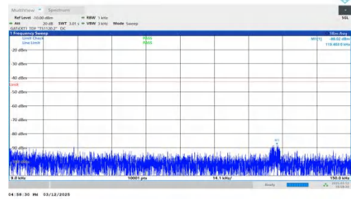
NTNV-n77(3450-3550)-PC2-30-40-M-DFT-QPSK-Inner_1RB_Righ t-0.009-0.15-PASS
