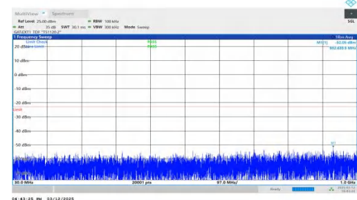
NTNV-n77(3450-3550)-PC2-30-30-H-DFT-BPSK-Inner_1RB_Right t-30-1000-PASS
