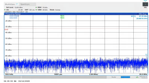
NTNV-n77(3450-3550)-PC2-30-30-M-DFT-BPSK-Inner_1RB_Left 0.15-30-PASS
