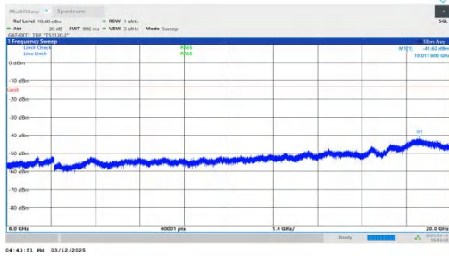
NTNV-n77(3450-3550)-PC2-30-30-H-DFT-BPSK-Inner_1RB_Rig ht-6000-20000-PASS
