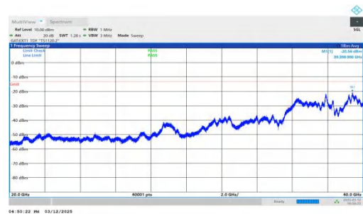
NTNV-n77(3450-3550)-PC2-30-40-L-DFT-BPSK-Inner_1RB_Right -20000-40000-PASS
