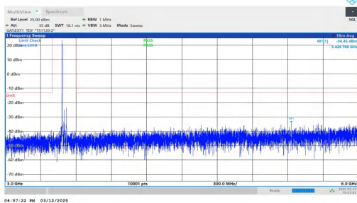
NTNV-n77(3450-3550)-PC2-30-40-M-DFT-QPSK-Inner_1RB_Lef t-3000-6000-PASS
