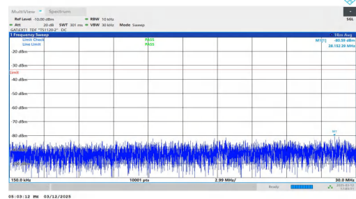
NTNV-n77(3450-3550)-PC2-30-40-H-DFT-QPSK-Inner_1RB_Left 0.15-30-PASS
