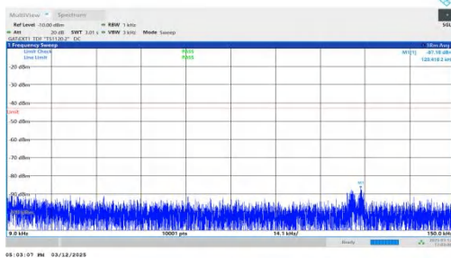
NTNV-n77(3450-3550)-PC2-30-40-H-DFT-QPSK-Inner_1RB_Left -0.009-0.15-PASS
