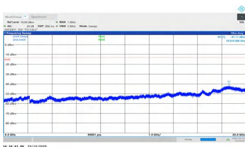
NTNV-n77(3450-3550)-PC2-30-30-L-DFT-QPSK-Inner_1RB_Rig ht-6000-20000-PASS
