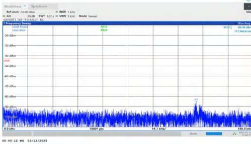
NTNV-n77(3450-3550)-PC2-30-40-H-DFT-BPSK-Inner_1RB_Left -0.009-0.15-PASS
