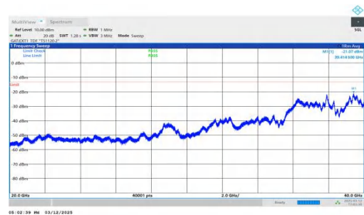
NTNV-n77(3450-3550)-PC2-30-40-H-DFT-BPSK-Inner_1RB_Righ t-20000-40000-PASS
