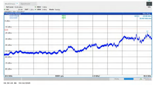
NTNV-n77(3450-3550)-PC2-30-40-M-DFT-BPSK-Inner_1RB_Righ t-20000-40000-PASS
