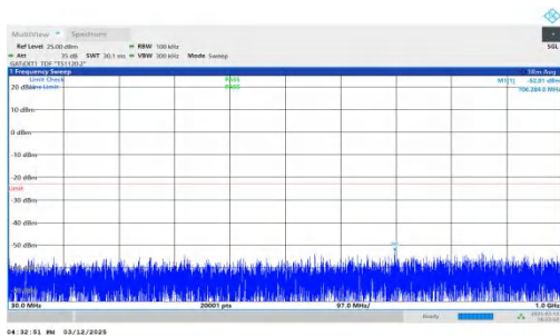
NTNV-n77(3450-3550)-PC2-30-30-L-DFT-QPSK-Inner_1RB_Left -30-1000-PASS
