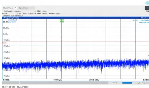
NTNV-n77(3450-3550)-PC2-30-30-M-DFT-BPSK-Inner_1RB_Rig ht-1000-3000-PASS
