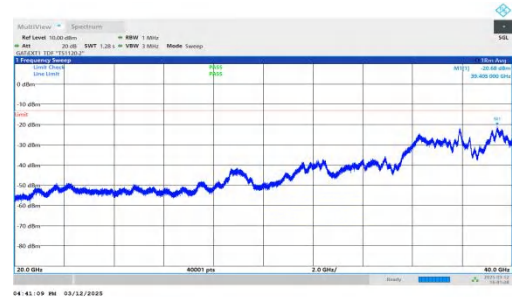
NTNV-n77(3450-3550)-PC2-30-30-M-DFT-QPSK-Inner_1RB_Righ t-20000-40000-PASS
