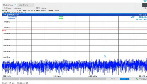
NTNV-n77(3450-3550)-PC2-30-20-H-DFT-QPSK-Inner_1RB_Rig ht-0.15-30-PASS
