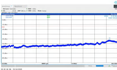
NTNV-n77(3450-3550)-PC2-30-30-M-DFT-QPSK-Inner_1RB_Rig ht-6000-20000-PASS
