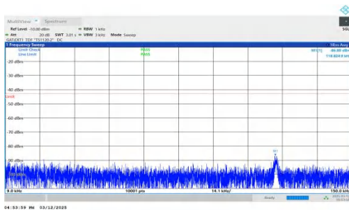
NTNV-n77(3450-3550)-PC2-30-40-M-DFT-BPSK-Inner_1RB_Left -0.009-0.15-PASS
