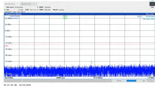
NTNV-n77(3450-3550)-PC2-30-30-M-DFT-BPSK-Inner_1RB_Righ t-30-1000-PASS
