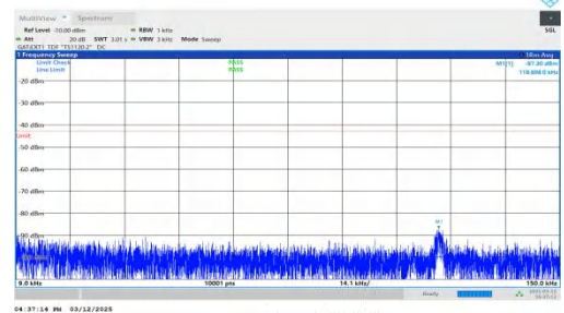
NTNV-n77(3450-3550)-PC2-30-30-M-DFT-BPSK-Inner_1RB_Right t-0.009-0.15-PASS
