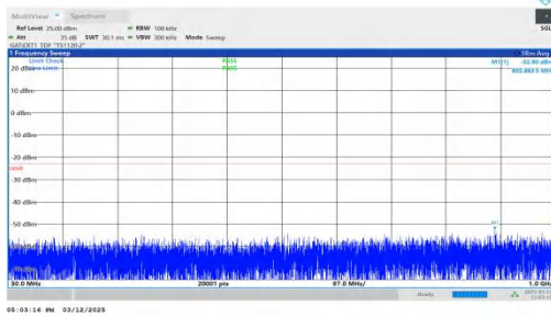
NTNV-n77(3450-3550)-PC2-30-40-H-DFT-QPSK-Inner_1RB_Left -30-1000-PASS
