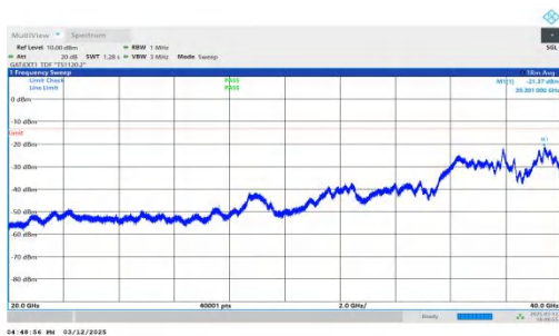
NTNV-n77(3450-3550)-PC2-30-40-L-DFT-BPSK-Inner_1RB_Left- 20000-40000-PASS
