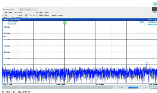
NTNV-n77(3450-3550)-PC2-30-40-M-DFT-QPSK-Inner_1RB_Rig ht-0.15-30-PASS
