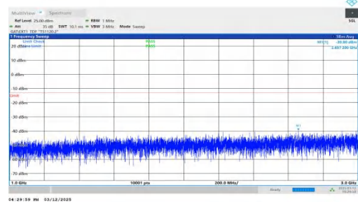
NTNV-n77(3450-3550)-PC2-30-30-L-DFT-BPSK-Inner_1RB_Left- 1000-3000-PASS
