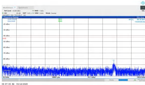
NTNV-n77(3450-3550)-PC2-30-40-M-DFT-QPSK-Inner_1RB_Lef t-0.009-0.15-PASS
