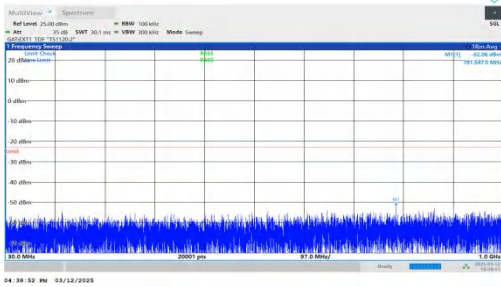
NTNV-n77(3450-3550)-PC2-30-30-M-DFT-QPSK-Inner_1RB_Lef t-30-1000-PASS
