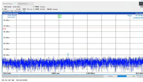
NTNV-n77(3450-3550)-PC2-30-40-H-DFT-BPSK-Inner_1RB_Rig ht-0.15-30-PASS
