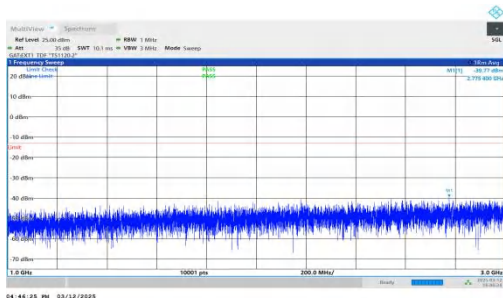
NTNV-n77(3450-3550)-PC2-30-30-H-DFT-QPSK-Inner_1RB_Right ht-1000-3000-PASS
