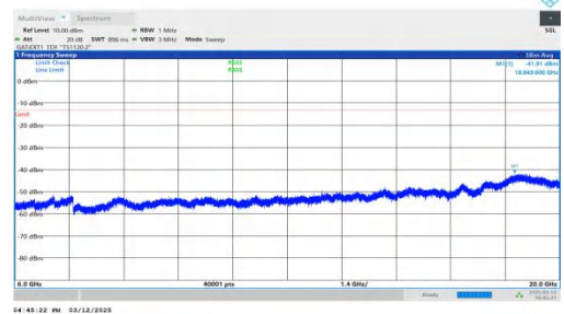
NTNV-n77(3450-3550)-PC2-30-30-H-DFT-QPSK-Inner_1RB_Left- 6000-20000-PASS
