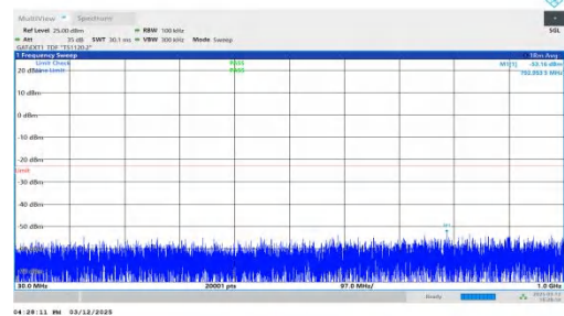
NTNV-n77(3450-3550)-PC2-30-20-H-DFT-QPSK-Inner_1RB_Right t-30-1000-PASS
