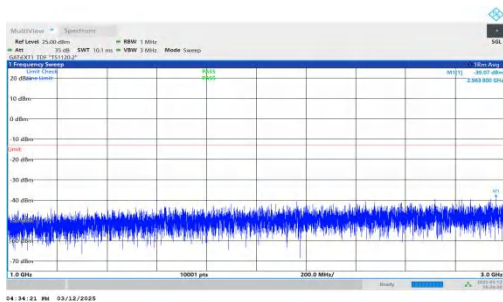
NTNV-n77(3450-3550)-PC2-30-30-L-DFT-QPSK-Inner_1RB_Rig ht-1000-3000-PASS
