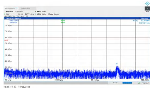
NTNV-n77(3450-3550)-PC2-30-30-M-DFT-QPSK-Inner_1RB_Right t-0.009-0.15-PASS
