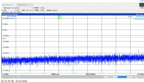
NTNV-n77(3450-3550)-PC2-30-30-L-DFT-BPSK-Inner_1RB_Rig ht-1000-3000-PASS
