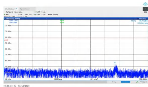
NTNV-n77(3450-3550)-PC2-30-40-H-DFT-QPSK-Inner_1RB_Right t-0.009-0.15-PASS
