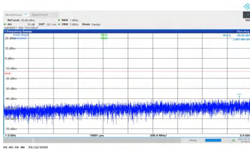
NTNV-n77(3450-3550)-PC2-30-40-L-DFT-BPSK-Inner_1RB_Rig ht-1000-3000-PASS
