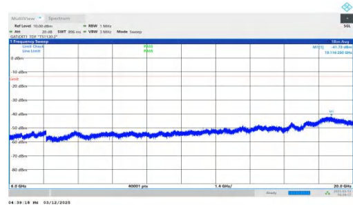
NTNV-n77(3450-3550)-PC2-30-30-M-DFT-QPSK-Inner_1RB_Left- 6000-20000-PASS
