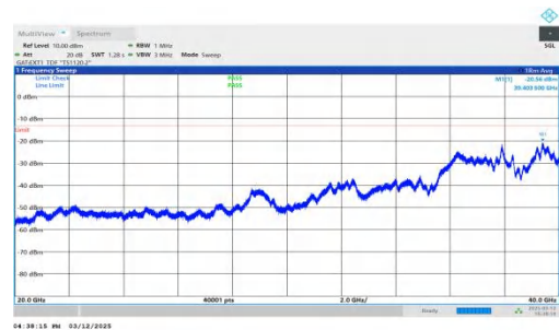
NTNV-n77(3450-3550)-PC2-30-30-M-DFT-BPSK-Inner_1RB_Righ t-20000-40000-PASS
