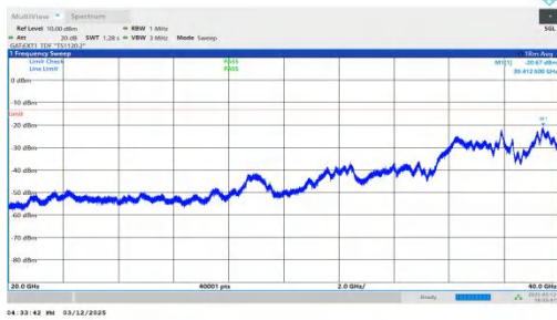
NTNV-n77(3450-3550)-PC2-30-30-L-DFT-QPSK-Inner_1RB_Left -20000-40000-PASS
