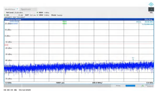
NTNV-n77(3450-3550)-PC2-30-30-H-DFT-QPSK-Inner_1RB_Left- 1000-3000-PASS
