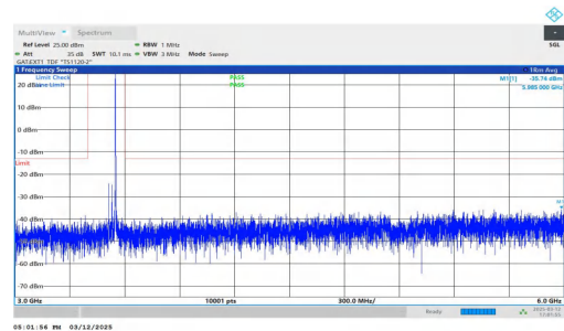
NTNV-n77(3450-3550)-PC2-30-40-H-DFT-BPSK-Inner_1RB_Righ t-3000-6000-PASS
