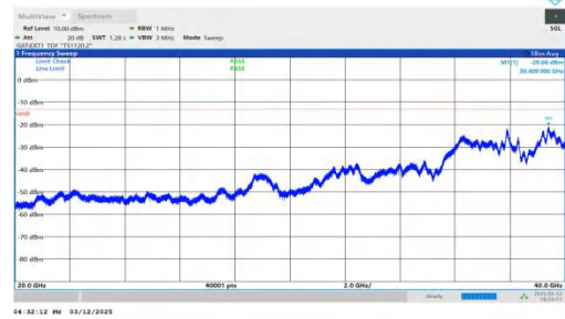
NTNV-n77(3450-3550)-PC2-30-30-L-DFT-BPSK-Inner_1RB_Right -20000-40000-PASS
