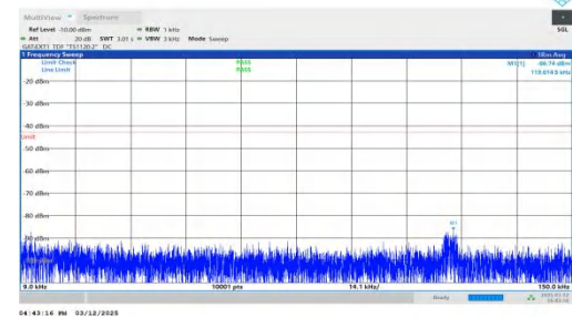
NTNV-n77(3450-3550)-PC2-30-30-H-DFT-BPSK-Inner_1RB_Right t-0.009-0.15-PASS
