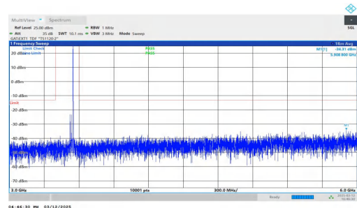
NTNV-n77(3450-3550)-PC2-30-30-H-DFT-QPSK-Inner_1RB_Right t-3000-6000-PASS
