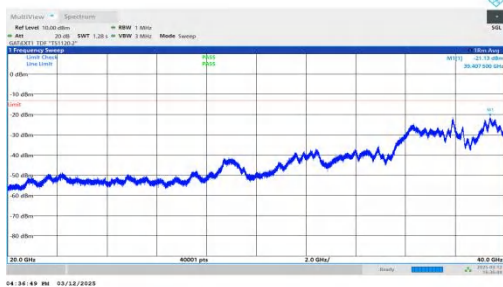
NTNV-n77(3450-3550)-PC2-30-30-M-DFT-BPSK-Inner_1RB_Left -20000-40000-PASS
