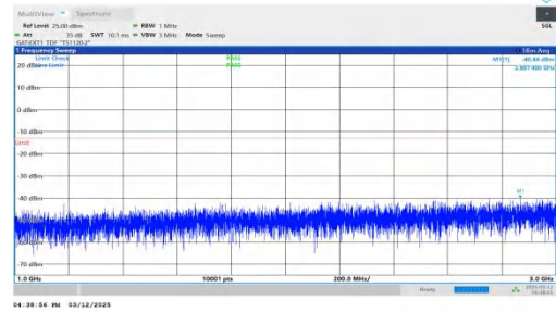
NTNV-n77(3450-3550)-PC2-30-30-M-DFT-QPSK-Inner_1RB_Left- 1000-3000-PASS
