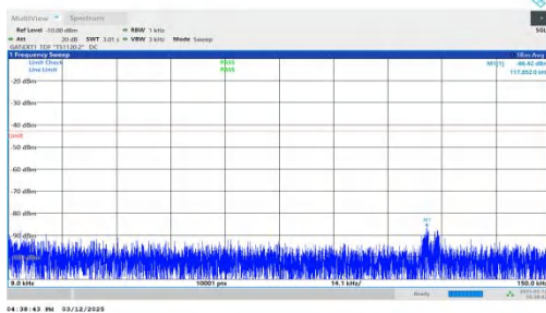
NTNV-n77(3450-3550)-PC2-30-30-M-DFT-QPSK-Inner_1RB_Lef t-0.009-0.15-PASS
