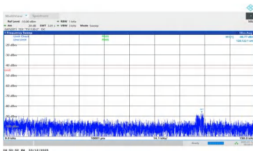
NTNV-n77(3450-3550)-PC2-30-40-L-DFT-QPSK-Inner_1RB_Left -0.009-0.15-PASS
