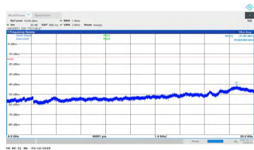
NTNV-n77(3450-3550)-PC2-30-40-L-DFT-BPSK-Inner_1RB_Left- 6000-20000-PASS
