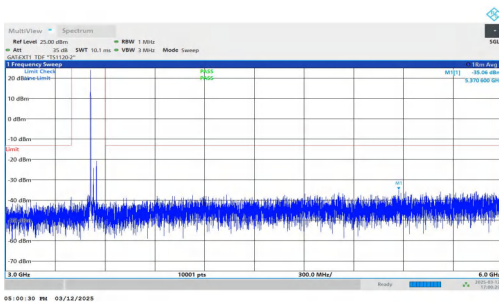
NTNV-n77(3450-3550)-PC2-30-40-H-DFT-BPSK-Inner_1RB_Left -3000-6000-PASS
