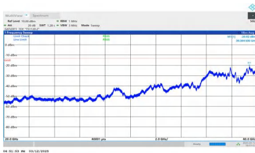
NTNV-n77(3450-3550)-PC2-30-40-L-DFT-QPSK-Inner_1RB_Left -20000-40000-PASS
