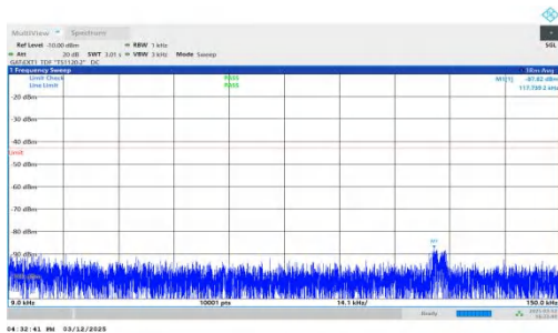
NTNV-n77(3450-3550)-PC2-30-30-L-DFT-QPSK-Inner_1RB_Left -0.009-0.15-PASS
