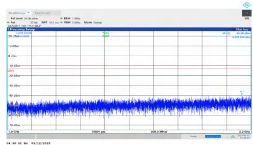
NTNV-n77(3450-3550)-PC2-30-30-M-DFT-BPSK-Inner_1RB_Left 1000-3000-PASS
