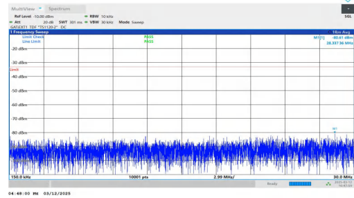
NTNV-n77(3450-3550)-PC2-30-40-L-DFT-BPSK-Inner_1RB_Left- 0.15-30-PASS
