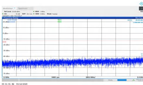
NTNV-n77(3450-3550)-PC2-30-40-H-DFT-BPSK-Inner_1RB_Rig ht-1000-3000-PASS
