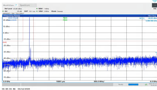
NTNV-n77(3450-3550)-PC2-30-30-H-DFT-QPSK-Inner_1RB_Left -3000-6000-PASS
