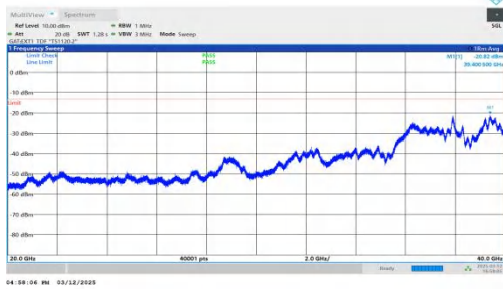
NTNV-n77(3450-3550)-PC2-30-40-M-DFT-QPSK-Inner_1RB_Lef t-20000-40000-PASS
