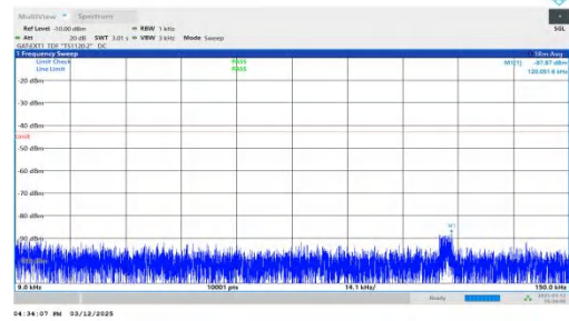
NTNV-n77(3450-3550)-PC2-30-30-L-DFT-QPSK-Inner_1RB_Right -0.009-0.15-PASS
