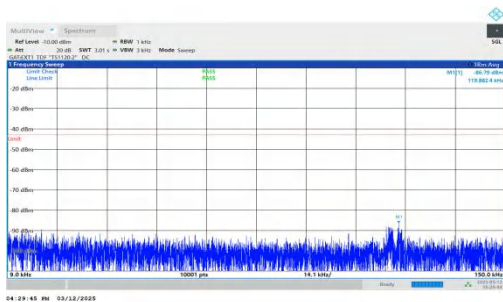
NTNV-n77(3450-3550)-PC2-30-30-L-DFT-BPSK-Inner_1RB_Left- 0.009-0.15-PASS
