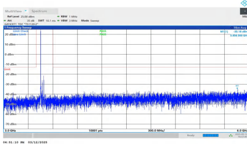
NTNV-n77(3450-3550)-PC2-30-40-L-DFT-QPSK-Inner_1RB_Left -3000-6000-PASS
