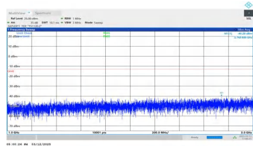
NTNV-n77(3450-3550)-PC2-30-40-H-DFT-BPSK-Inner_1RB_Left- 1000-3000-PASS
