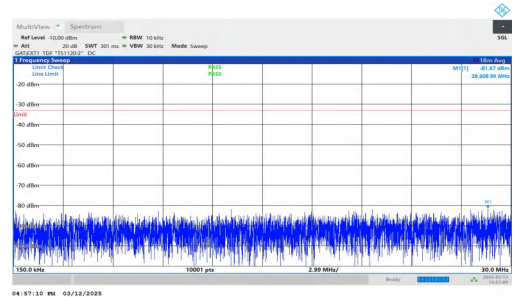
NTNV-n77(3450-3550)-PC2-30-40-M-DFT-QPSK-Inner_1RB_Left- 0.15-30-PASS
