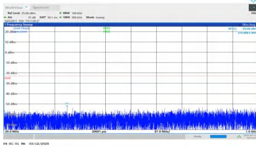
NTNV-n77(3450-3550)-PC2-30-40-L-DFT-QPSK-Inner_1RB_Left -30-1000-PASS
