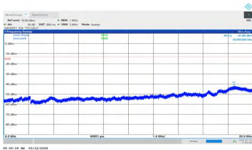
NTNV-n77(3450-3550)-PC2-30-40-H-DFT-QPSK-Inner_1RB_Rig ht-6000-20000-PASS
