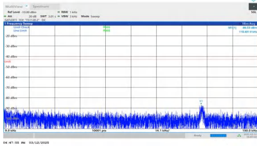
NTNV-n77(3450-3550)-PC2-30-40-L-DFT-BPSK-Inner_1RB_Left- 0.009-0.15-PASS
