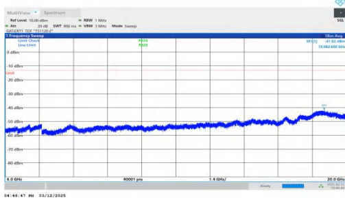
NTNV-n77(3450-3550)-PC2-30-30-H-DFT-QPSK-Inner_1RB_Right ht-6000-20000-PASS
