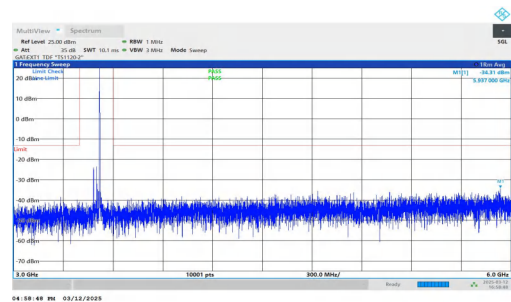
NTNV-n77(3450-3550)-PC2-30-40-M-DFT-QPSK-Inner_1RB_Righ t-3000-6000-PASS
