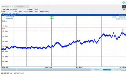
NTNV-n77(3450-3550)-PC2-30-40-M-DFT-BPSK-Inner_1RB_Left -20000-40000-PASS
