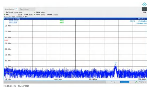
NTNV-n77(3450-3550)-PC2-30-40-L-DFT-BPSK-Inner_1RB_Right -0.009-0.15-PASS
