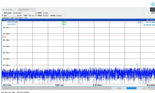
NTNV-n77(3450-3550)-PC2-30-40-M-DFT-BPSK-Inner_1RB_Rig ht-0.15-30-PASS
