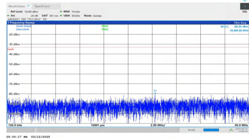
NTNV-n77(3450-3550)-PC2-30-40-H-DFT-BPSK-Inner_1RB_Left- 0.15-30-PASS
