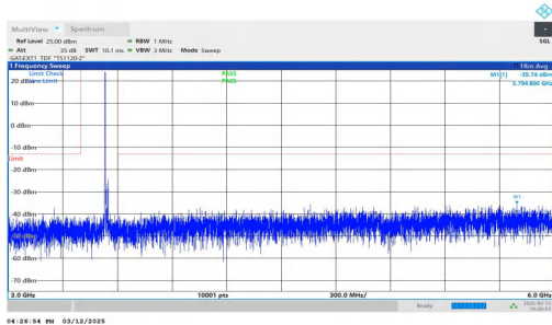
NTNV-n77(3450-3550)-PC2-30-20-H-DFT-QPSK-Inner_1RB_Left -3000-6000-PASS
