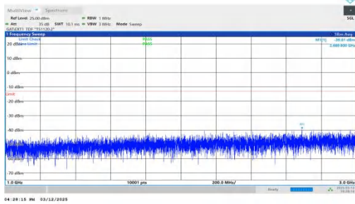
NTNV-n77(3450-3550)-PC2-30-20-H-DFT-QPSK-Inner_1RB_Rig ht-1000-3000-PASS
