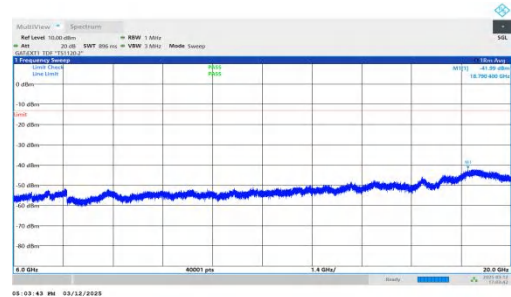
NTNV-n77(3450-3550)-PC2-30-40-H-DFT-QPSK-Inner_1RB_Left 6000-20000-PASS
