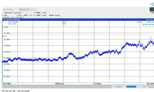
NTNV-n77(3450-3550)-PC2-30-40-H-DFT-QPSK-Inner_1RB_Left -20000-40000-PASS
