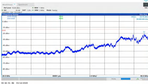
NTNV-n77(3450-3550)-PC2-30-30-H-DFT-BPSK-Inner_1RB_Left -20000-40000-PASS
