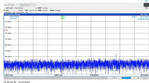
NTNV-n77(3450-3550)-PC2-30-30-M-DFT-QPSK-Inner_1RB_Left- 0.15-30-PASS
