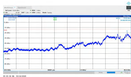
NTNV-n77(3450-3550)-PC2-30-40-H-DFT-QPSK-Inner_1RB_Righ t-20000-40000-PASS
