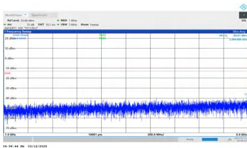
NTNV-n77(3450-3550)-PC2-30-40-M-DFT-QPSK-Inner_1RB_Rig ht-1000-3000-PASS
