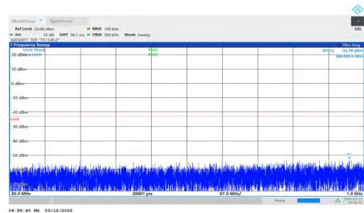
NTNV-n77(3450-3550)-PC2-30-40-M-DFT-QPSK-Inner_1RB_Righ t-30-1000-PASS
