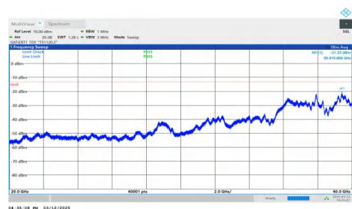
NTNV-n77(3450-3550)-PC2-30-30-L-DFT-QPSK-Inner_1RB_Right -20000-40000-PASS
