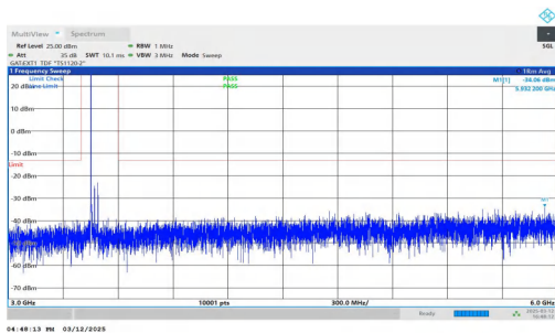
NTNV-n77(3450-3550)-PC2-30-40-L-DFT-BPSK-Inner_1RB_Left- 3000-6000-PASS
