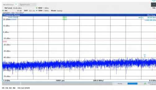
NTNV-n77(3450-3550)-PC2-30-40-H-DFT-QPSK-Inner_1RB_Rig ht-1000-3000-PASS
