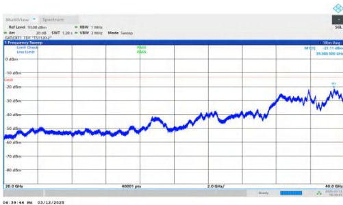
NTNV-n77(3450-3550)-PC2-30-30-M-DFT-QPSK-Inner_1RB_Lef t-20000-40000-PASS
