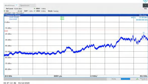
NTNV-n77(3450-3550)-PC2-30-30-H-DFT-QPSK-Inner_1RB_Right t-20000-40000-PASS
