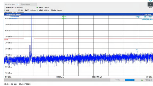
NTNV-n77(3450-3550)-PC2-30-40-H-DFT-QPSK-Inner_1RB_Righ t-3000-6000-PASS
