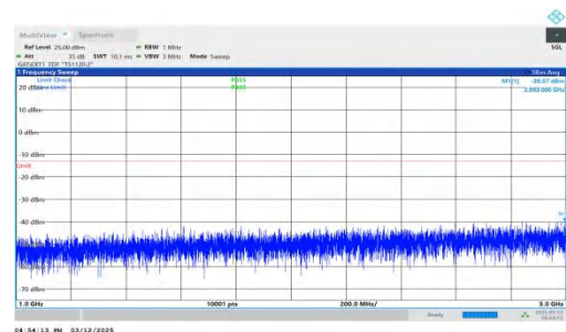
NTNV-n77(3450-3550)-PC2-30-40-M-DFT-BPSK-Inner_1RB_Left- 1000-3000-PASS
