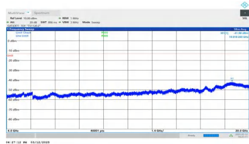
NTNV-n77(3450-3550)-PC2-30-20-H-DFT-QPSK-Inner_1RB_Left 6000-20000-PASS
