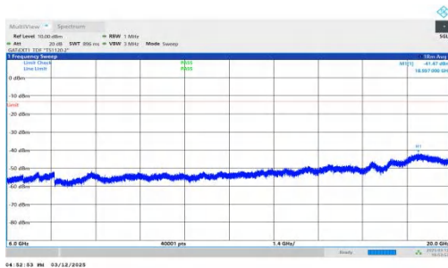
NTNV-n77(3450-3550)-PC2-30-40-L-DFT-QPSK-Inner_1RB_Rig ht-6000-20000-PASS
