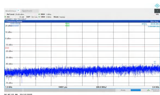
NTNV-n77(3450-3550)-PC2-30-30-H-DFT-BPSK-Inner_1RB_Left- 1000-3000-PASS
