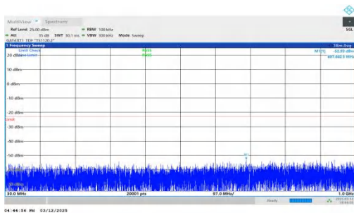
NTNV-n77(3450-3550)-PC2-30-30-H-DFT-QPSK-Inner_1RB_Left -30-1000-PASS
