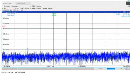
NTNV-n77(3450-3550)-PC2-30-30-M-DFT-BPSK-Inner_1RB_Rig ht-0.15-30-PASS
