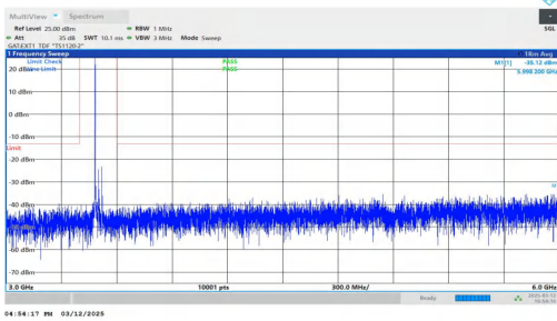
NTNV-n77(3450-3550)-PC2-30-40-M-DFT-BPSK-Inner_1RB_Left -3000-6000-PASS
