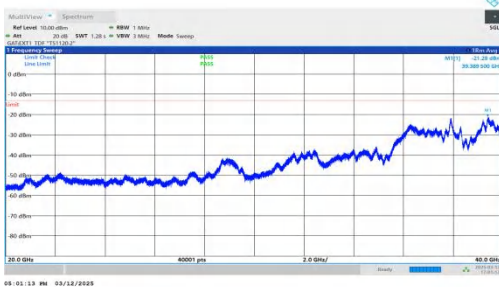
NTNV-n77(3450-3550)-PC2-30-40-H-DFT-BPSK-Inner_1RB_Left -20000-40000-PASS
