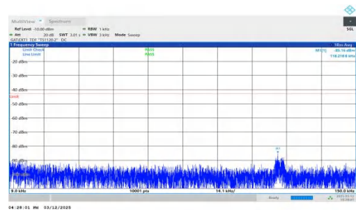
NTNV-n77(3450-3550)-PC2-30-20-H-DFT-QPSK-Inner_1RB_Right t-0.009-0.15-PASS
