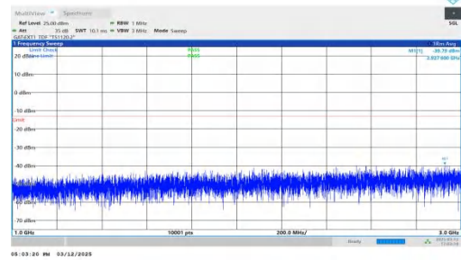
NTNV-n77(3450-3550)-PC2-30-40-H-DFT-QPSK-Inner_1RB_Left 1000-3000-PASS
