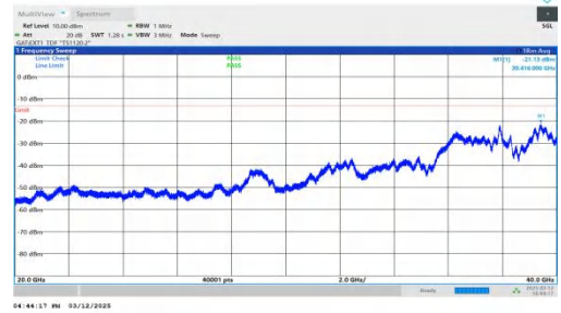
NTNV-n77(3450-3550)-PC2-30-30-H-DFT-BPSK-Inner_1RB_Righ t-20000-40000-PASS
