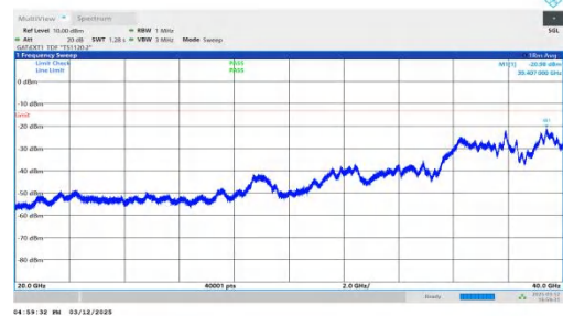
NTNV-n77(3450-3550)-PC2-30-40-M-DFT-QPSK-Inner_1RB_Righ t-20000-40000-PASS
