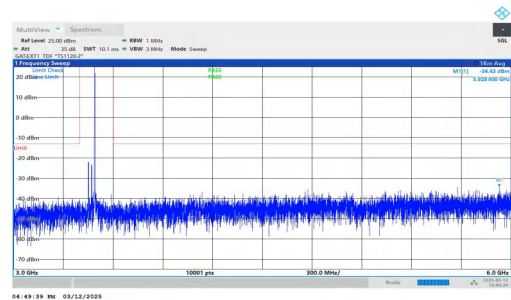
NTNV-n77(3450-3550)-PC2-30-40-L-DFT-BPSK-Inner_1RB_Right -3000-6000-PASS
