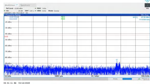
NTNV-n77(3450-3550)-PC2-30-30-L-DFT-BPSK-Inner_1RB_Right-0.009-0.15-PASS
