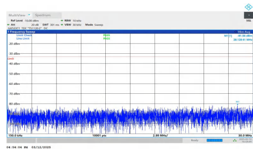
NTNV-n77(3450-3550)-PC2-30-40-M-DFT-BPSK-Inner_1RB_Left- 0.15-30-PASS
