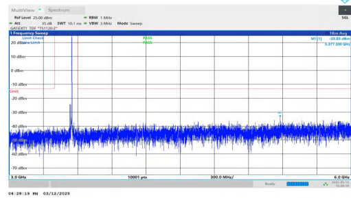
NTNV-n77(3450-3550)-PC2-30-20-H-DFT-QPSK-Inner_1RB_Righ t-3000-6000-PASS
