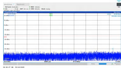
NTNV-n77(3450-3550)-PC2-30-40-L-DFT-QPSK-Inner_1RB_Right -30-1000-PASS
