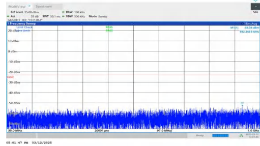
NTNV-n77(3450-3550)-PC2-30-40-H-DFT-BPSK-Inner_1RB_Righ t-30-1000-PASS
