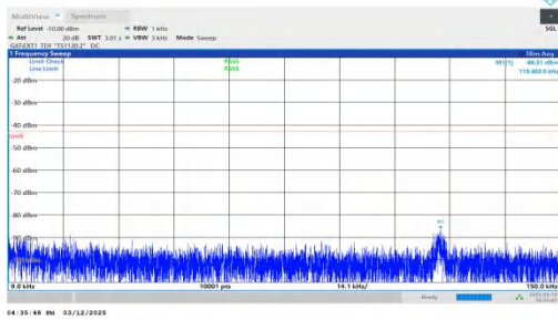
NTNV-n77(3450-3550)-PC2-30-30-M-DFT-BPSK-Inner_1RB_Left -0.009-0.15-PASS
