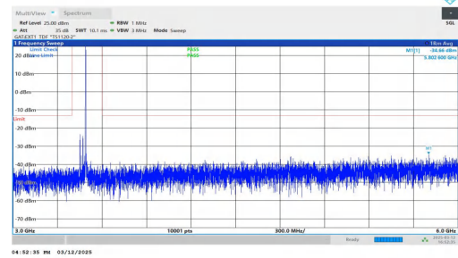
NTNV-n77(3450-3550)-PC2-30-40-L-DFT-QPSK-Inner_1RB_Right -3000-6000-PASS
