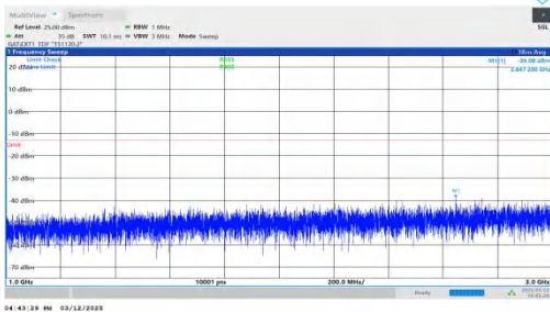
NTNV-n77(3450-3550)-PC2-30-30-H-DFT-BPSK-Inner_1RB_Rig ht-1000-3000-PASS
