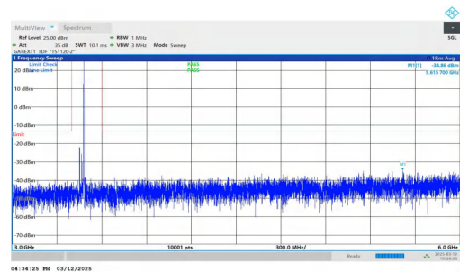
NTNV-n77(3450-3550)-PC2-30-30-L-DFT-QPSK-Inner_1RB_Right -3000-6000-PASS
