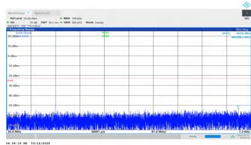
NTNV-n77(3450-3550)-PC2-30-30-L-DFT-QPSK-Inner_1RB_Right -30-1000-PASS
