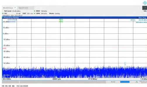
NTNV-n77(3450-3550)-PC2-30-30-M-DFT-BPSK-Inner_1RB_Left -30-1000-PASS
