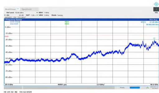
NTNV-n77(3450-3550)-PC2-30-20-H-DFT-QPSK-Inner_1RB_Righ t-20000-40000-PASS
