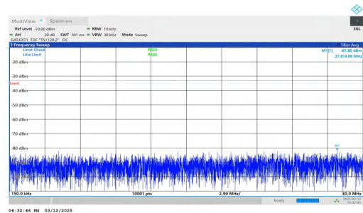
NTNV-n77(3450-3550)-PC2-30-30-L-DFT-QPSK-Inner_1RB_Left- 0.15-30-PASS
