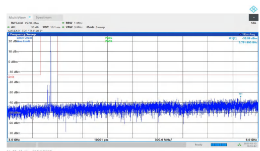
NTNV-n77(3450-3550)-PC2-30-40-M-DFT-BPSK-Inner_1RB_Right t-3000-6000-PASS
