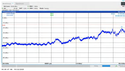
NTNV-n77(3450-3550)-PC2-30-30-H-DFT-QPSK-Inner_1RB_Left -20000-40000-PASS
