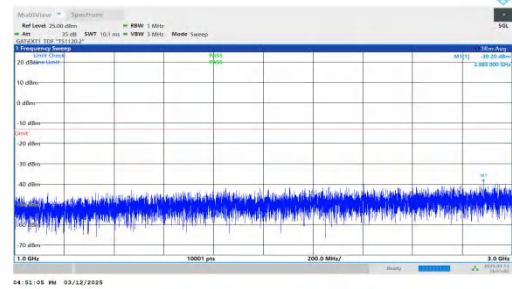
NTNV-n77(3450-3550)-PC2-30-40-L-DFT-QPSK-Inner_1RB_Left- 1000-3000-PASS
