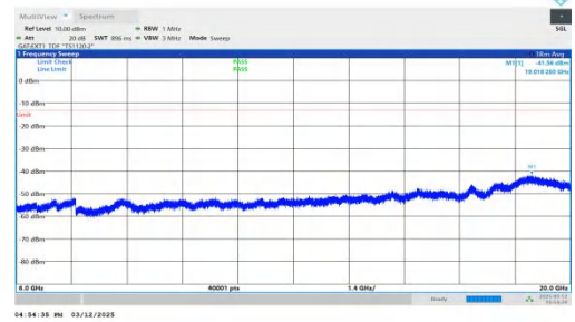
NTNV-n77(3450-3550)-PC2-30-40-M-DFT-BPSK-Inner_1RB_Left 6000-20000-PASS
