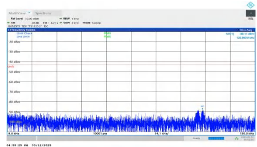
NTNV-n77(3450-3550)-PC2-30-40-M-DFT-BPSK-Inner_1RB_Right t-0.009-0.15-PASS
