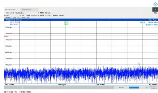
NTNV-n77(3450-3550)-PC2-30-60-L-DFT-BPSK-Inner_1RB_Left- 0.15-30-PASS
