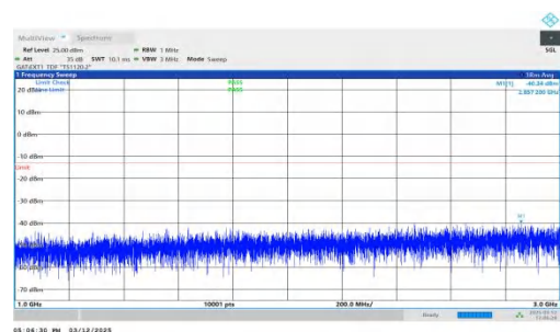
NTNV-n77(3450-3550)-PC2-30-60-L-DFT-BPSK-Inner_1RB_Left- 1000-3000-PASS
