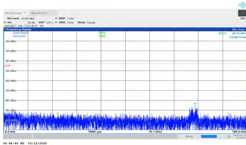
NTNV-n77(3450-3550)-PC2-30-30-H-DFT-QPSK-Inner_1RB_Left -0.009-0.15-PASS
