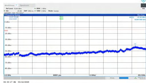
NTNV-n77(3450-3550)-PC2-30-30-L-DFT-QPSK-Inner_1RB_Left- 6000-20000-PASS
