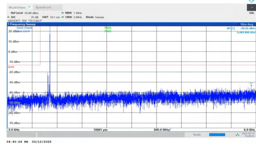
NTNV-n77(3450-3550)-PC2-30-30-M-DFT-QPSK-Inner_1RB_Righ t-3000-6000-PASS
