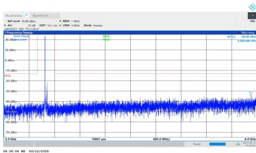
NTNV-n77(3450-3550)-PC2-30-30-M-DFT-BPSK-Inner_1RB_Left -3000-6000-PASS
