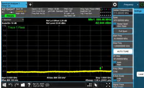
NTVN-n70-PC3-15-15-M-DFT-BPSK-Inner_1RB_Right-30-1000-PAS
