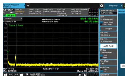
NTNV-n70-PC3-15-15-L-DFT-BPSK-Inner_1RB_Right-0.15-30-PASS
