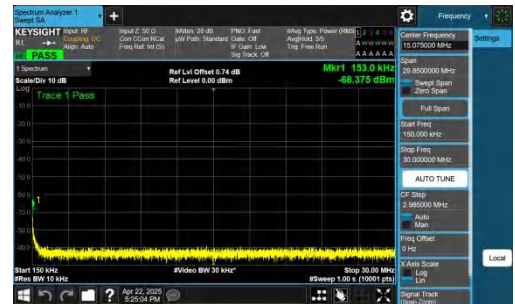
NTNV-n70-PC3-15-15-H-DFT-BPSK-Inner_1RB_Left-0.15-30-PASS
