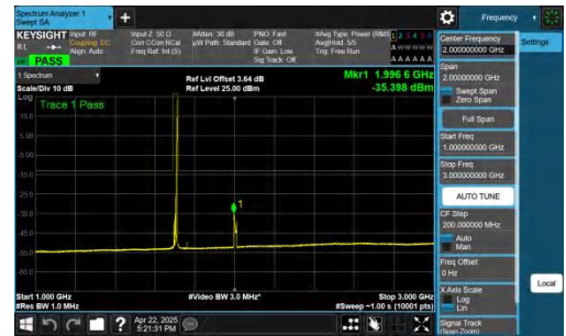
NTVN-n70-PC3-15-15-M-DFT-BPSK-Inner_1RB_Right-1000-3000-PA
