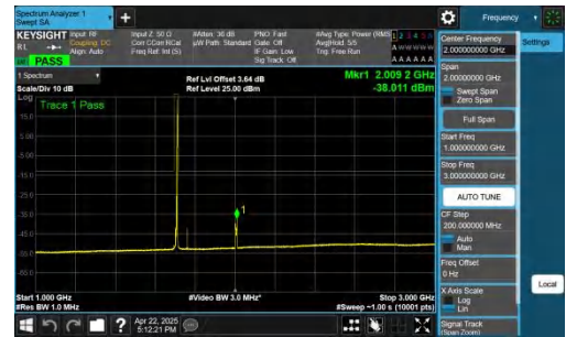
NTNV-n70-PC3-15-10-H-DFT-BPSK-Inner_1RB_Right-1000-3000-PAS
