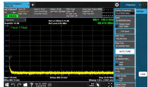
NTVN-n70-PC3-15-15-M-DFT-QPSK-Inner_1RB_Left-0.15-30-PASS
