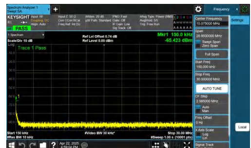
NTNV-n70-PC3-15-5-H-DFT-QPSK-Inner_1RB_Left-0.15-30-PASS
