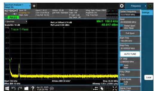
NTNV-n70-PC3-15-15-H-DFT-QPSK-Inner_1RB_Right-0.15-30-PASS
