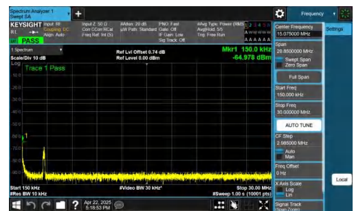
NTNV-n70-PC3-15-15-L-DFT-QPSK-Inner_1RB_Right-0.15-30-PASS
