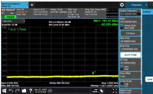
NTNV-n70-PC3-15-10-H-DFT-BPSK-Inner_1RB_Right-30-1000-PAS
