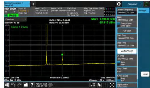
NTNV-n70-PC3-15-15-H-DFT-BPSK-Inner_1RB_Right-1000-3000-PAS
