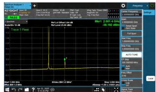
NTNV-n70-PC3-15-10-H-DFT-QPSK-Inner_1RB_Right-1000-3000-PA
