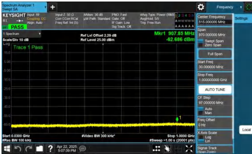
NTVN-n70-PC3-15-10-M-DFT-BPSK-Inner_1RB_Right-30-1000-PAS
