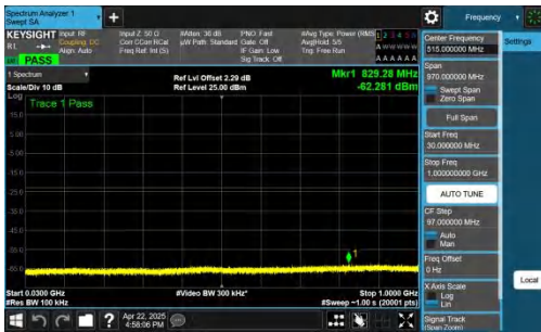
NTNV-n70-PC3-15-5-H-DFT-BPSK-Inner_1RB_Right-30-1000-PASS
