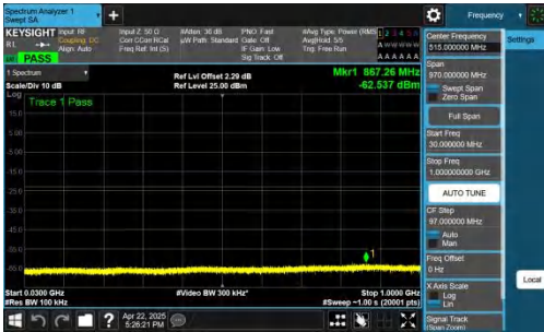
NTNV-n70-PC3-15-15-H-DFT-BPSK-Inner_1RB_Right-30-1000-PAS
