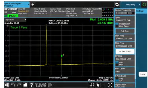
NTNV-n70-PC3-15-5-H-DFT-BPSK-Inner_1RB_Right-1000-3000-PASS S
