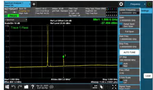
NTVN-n70-PC3-15-10-M-DFT-BPSK-Inner_1RB_Right-1000-3000-PA
