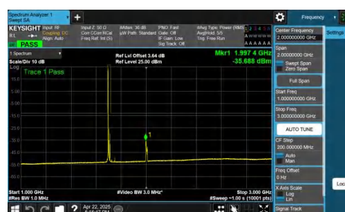
NTNV-n70-PC3-15-15-L-DFT-BPSK-Inner_1RB_Left-1000-3000-PASS
