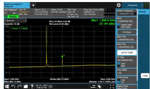
NTNV-n70-PC3-15-10-M-DFT-BPSK-Inner_1RB_Left-1000-3000-PAS S
