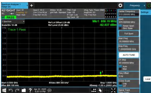
NTNV-n70-PC3-15-15-M-DFT-BPSK-Inner_1RB_Left-30-1000-PASS
