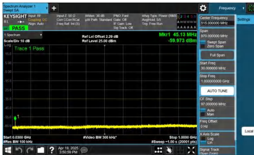
NTNV-n41-PC2-30-30-M-DFT-BPSK-Inner_1RB_Right-30-1000-PAS
