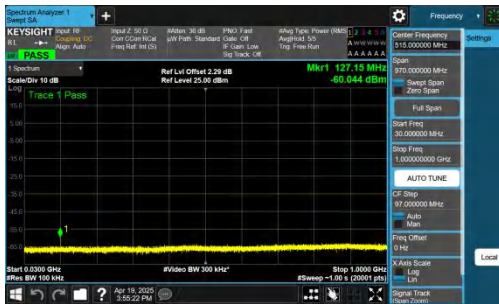
NTNV-n41-PC2-30-30-H-DFT-BPSK-Inner_1RB_Right-30-1000-PAS
