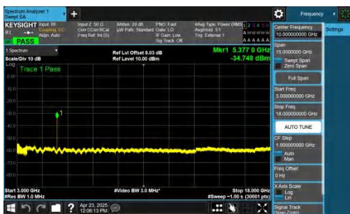
NTNV-n41-PC2-30-40-H-DFT-BPSK-Inner_1RB_Right-3000-18000-P
