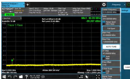
NTNV-n41-PC2-30-40-H-DFT-BPSK-Inner_1RB_Left-30-1000-PASS
