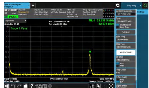
NTNV-n41-PC2-30-20-M-DFT-QPSK-Inner_1RB_Left-0.15-30-PASS
