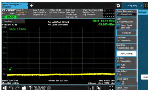
NTNV-n41-PC2-30-50-M-DFT-QPSK-Inner_1RB_Right-30-1000-PAS S
