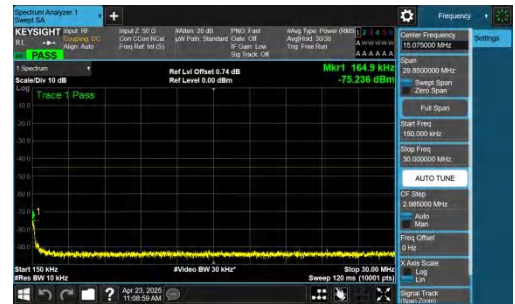
NTNV-n41-PC2-30-20-H-DFT-BPSK-Inner_1RB_Left-0.15-30-PASS
