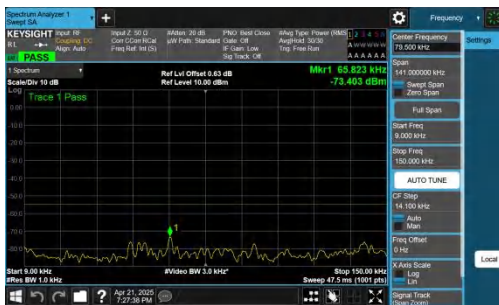
NTNV-n41-PC2-30-30-L-DFT-QPSK-Inner_1RB_Right-0.009-0.15-PA SS
