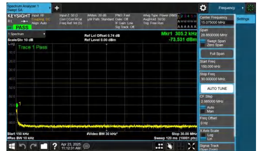
NTNV-n41-PC2-30-40-L-DFT-BPSK-Inner_1RB_Left-0.15-30-PASS
