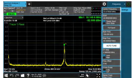
NTNV-n41-PC2-30-30-M-DFT-BPSK-Inner_1RB_Left-0.15-30-PASS
