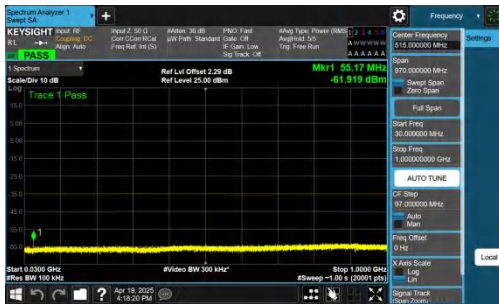
NTNV-n41-PC2-30-50-M-DFT-BPSK-Inner_1RB_Right-30-1000-PAS
