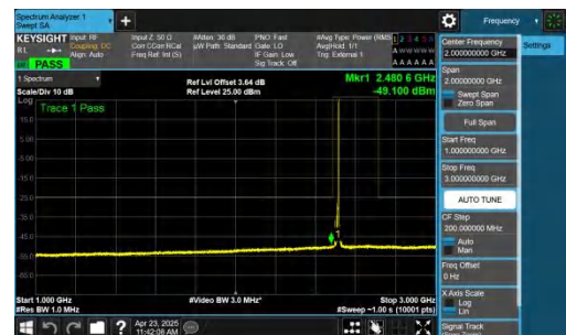
NTNV-n41-PC2-30-20-L-DFT-QPSK-Inner_1RB_Right-1000-3000-PAS S
