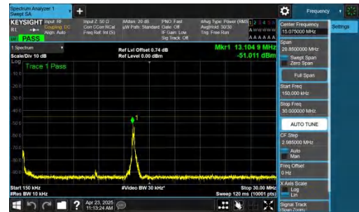
NTNV-n41-PC2-30-40-M-DFT-BPSK-Inner_1RB_Left-0.15-30-PASS
