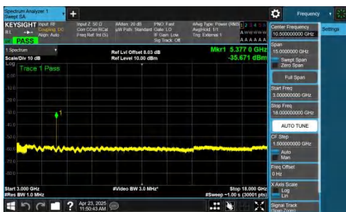
NTNV-n41-PC2-30-20-H-DFT-BPSK-Inner_1RB_Right-3000-18000-P
