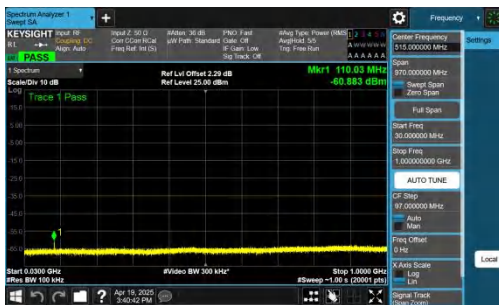
NTNV-n41-PC2-30-20-H-DFT-BPSK-Inner_1RB_Left-30-1000-PASS
