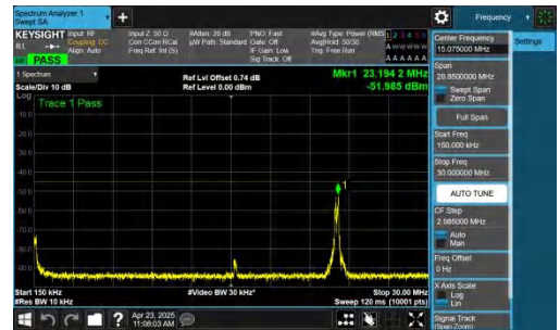
NTNV-n41-PC2-30-20-M-DFT-BPSK-Inner_1RB_Left-0.15-30-PASS
