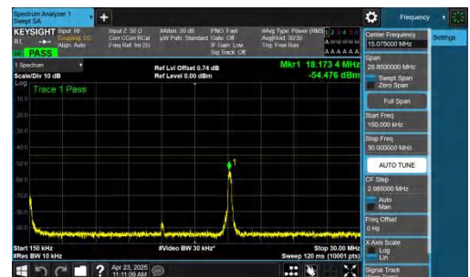
NTNV-n41-PC2-30-30-M-DFT-QPSK-Inner_1RB_Left-0.15-30-PASS
