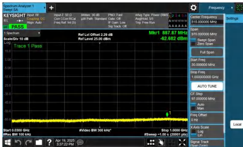
NTNV-n41-PC2-30-20-M-DFT-BPSK-Inner_1RB_Right-30-1000-PAS
