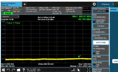
NTNV-n41-PC2-30-30-L-DFT-BPSK-Inner_1RB_Left-30-1000-PASS
