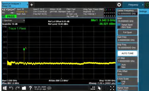
NTNV-n41-PC2-30-20-H-DFT-QPSK-Inner_1RB_Left-3000-18000-PA SS
