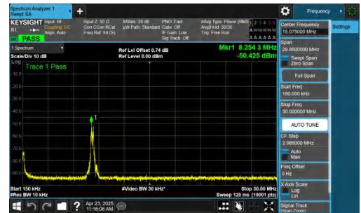
NTNV-n41-PC2-30-50-M-DFT-BPSK-Inner_1RB_Left-0.15-30-PASS
