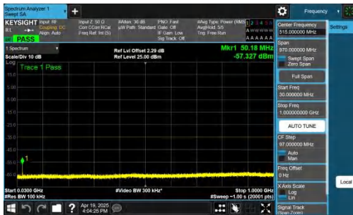
NTNV-n41-PC2-30-40-M-DFT-BPSK-Inner_1RB_Right-30-1000-PAS
