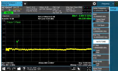
NTNV-n41-PC2-30-30-L-DFT-QPSK-Inner_1RB_Left-3000-18000-PA SS
