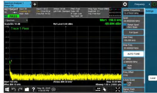
NTNV-n26(824-849)-PC3-15-15-L-DFT-BPSK-Inner_1RB_Left-0.15-30-PASS
