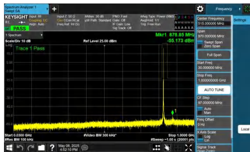
NTNV-n26(824-849)-PC3-15-20-H-DFT-BPSK-Inner_1RB_Left-30-1000-PASS
