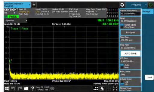
NTNV-n26(824-849)-PC3-15-20-M-DFT-BPSK-Inner_1RB_Left-0. 15-30-PASS
