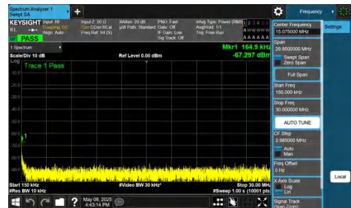
NTNV-n26(824-849)-PC3-15-15-M-DFT-QPSK-Inner_1RB_Left-0.15-30-PASS
