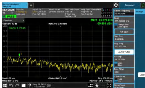
NTNV-n26(824-849)-PC3-15-10-L-DFT-QPSK-Inner_1RB_Right- 0.009-0.15-PASS
