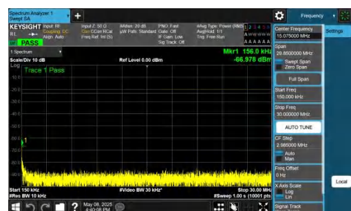
NTNV-n26(824-849)-PC3-15-15-L-DFT-BPSK-Inner_1RB_Right-0.15-30-PASS
