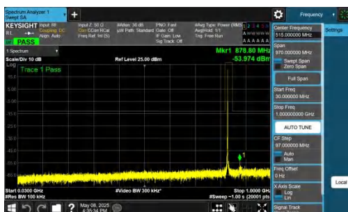
NTNV-n26(824-849)-PC3-15-10-M-DFT-QPSK-Inner_1RB_Left-30-1000-PASS
