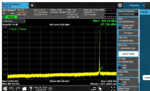
NTNV-n26(824-849)-PC3-15-5-H-DFT-QPSK-Inner_1RB_Left-30 -1000-PASS
