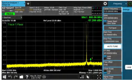
NTNV-n26(824-849)-PC3-15-15-L-DFT-BPSK-Inner_1RB_Right-30-1000-PASS
