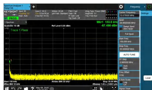
NTNV-n26(824-849)-PC3-15-20-H-DFT-BPSK-Inner_1RB_Right-0.15-30-PASS
