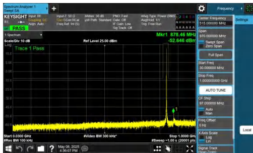
NTNV-n26(824-849)-PC3-15-10-M-DFT-QPSK-Inner_1RB_Right- 30-1000-PASS
