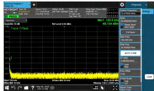
NTNV-n26(824-849)-PC3-15-20-M-DFT-QPSK-Inner_1RB_Right- 0.15-30-PASS
