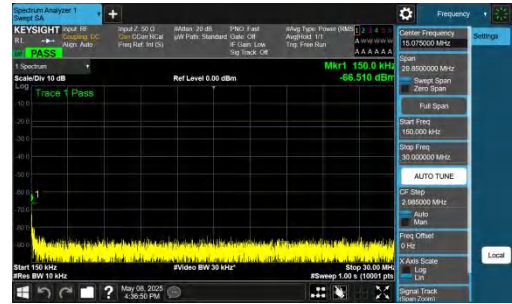
NTNV-n26(824-849)-PC3-15-10-H-DFT-BPSK-Inner_1RB_Left-0.15-30-PASS
