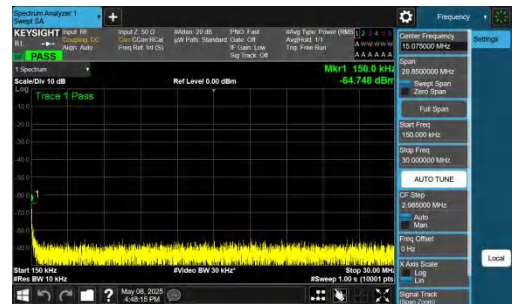
NTNV-n26(824-849)-PC3-15-20-L-DFT-QPSK-Inner_1RB_Left-0.15-30-PASS
