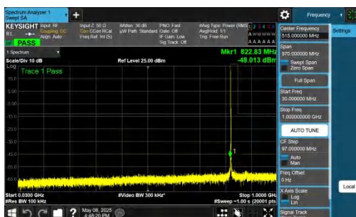
NTNV-n26(824-849)-PC3-15-20-L-DFT-QPSK-Inner_1RB_Left-30-1000-PASS
