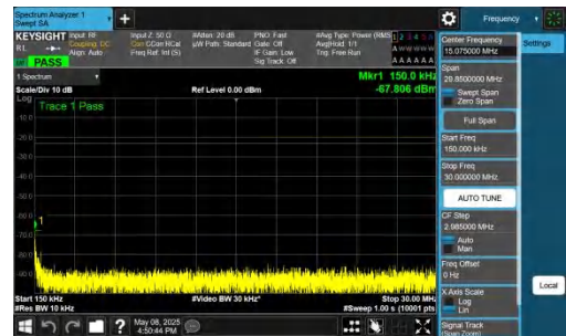
NTNV-n26(824-849)-PC3-15-20-M-DFT-QPSK-Inner_1RB_Left-0.15-30-PASS
