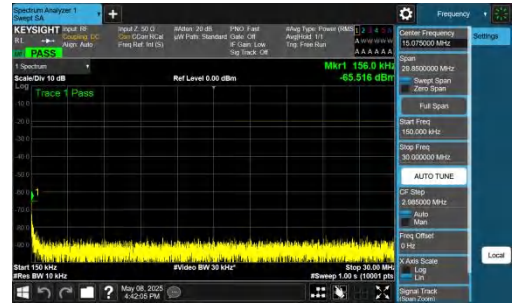
NTNV-n26(824-849)-PC3-15-15-M-DFT-BPSK-Inner_1RB_Left-0.15-30-PASS
