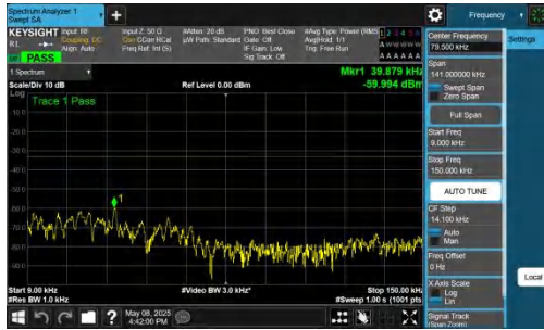
NTNV-n26(824-849)-PC3-15-15-M-DFT-BPSK-Inner_1RB_Left-0.009-0.15-PASS
