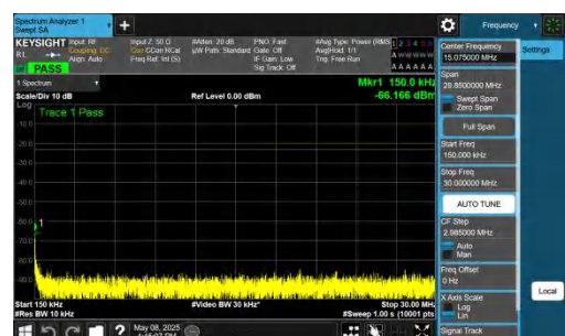
NTNV-n26(824-849)-PC3-15-15-H-DFT-BPSK-Inner_1RB_Right-0.15-30-PASS
