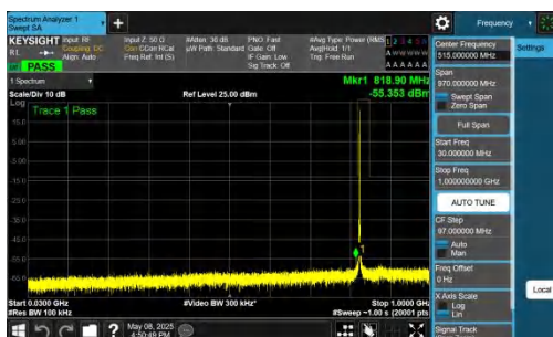
NTNV-n26(824-849)-PC3-15-20-M-DFT-QPSK-Inner_1RB_Left-30-1000-PASS
