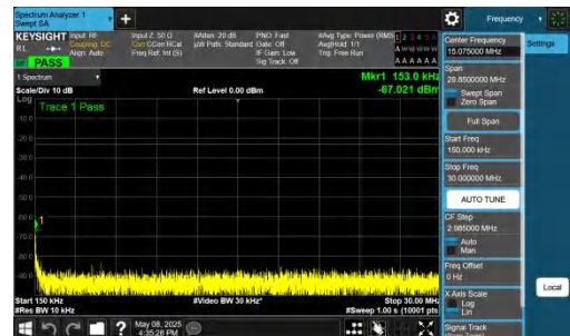
NTNV-n26(824-849)-PC3-15-10-M-DFT-QPSK-Inner_1RB_Left-0.15-30-PASS
