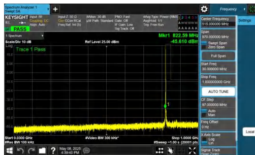
NTNV-n26(824-849)-PC3-15-15-L-DFT-BPSK-Inner_1RB_Left-30-1000-PASS
