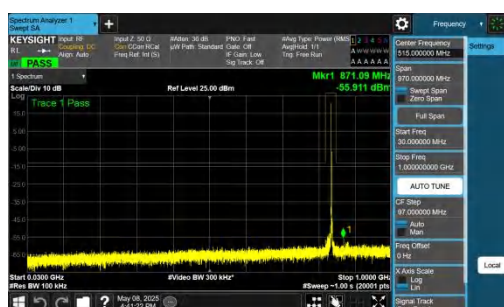
NTNV-n26(824-849)-PC3-15-15-L-DFT-QPSK-Inner_1RB_Right-30-1000-PASS
