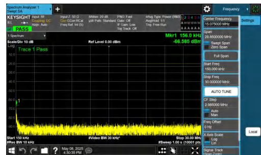
NTNV-n26(824-849)-PC3-15-5-H-DFT-QPSK-Inner_1RB_Right-0. 15-30-PASS
