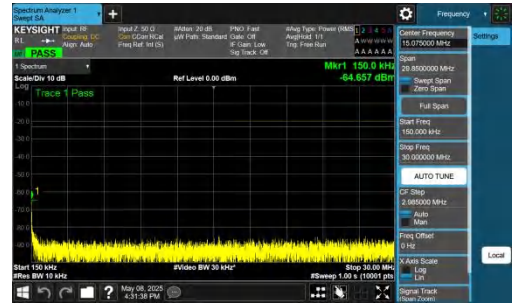
NTNV-n26(824-849)-PC3-15-10-L-DFT-BPSK-Inner_1RB_Left-0.15-30-PASS
