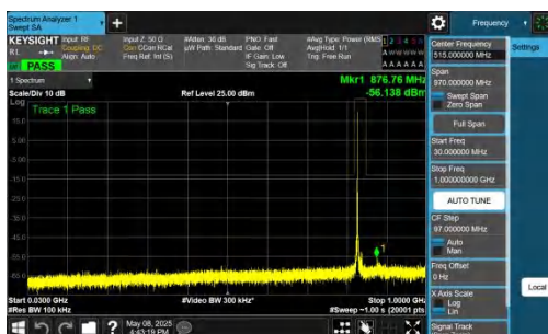
NTNV-n26(824-849)-PC3-15-15-M-DFT-QPSK-Inner_1RB_Left-30-1000-PASS
