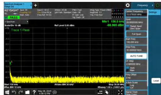
NTNV-n26(824-849)-PC3-15-10-H-DFT-QPSK-Inner_1RB_Left-0.15-30-PASS
