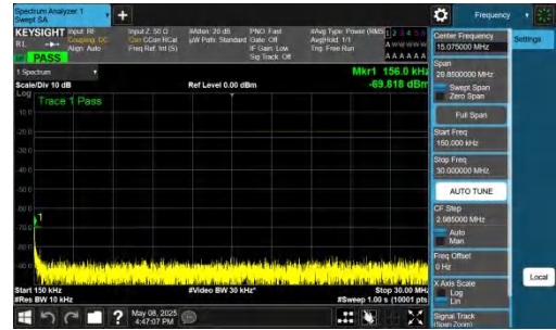
NTNV-n26(824-849)-PC3-15-20-L-DFT-BPSK-Inner_1RB_Left-0.15-30-PASS
