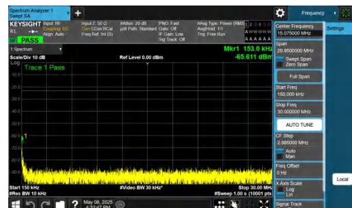
NTNV-n26(824-849)-PC3-15-10-L-DFT-QPSK-Inner_1RB_Left-0.15-30-PASS
