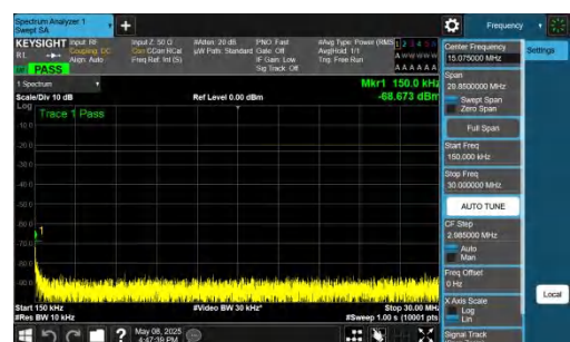
NTNV-n26(824-849)-PC3-15-20-L-DFT-BPSK-Inner_1RB_Right-0.15-30-PASS
