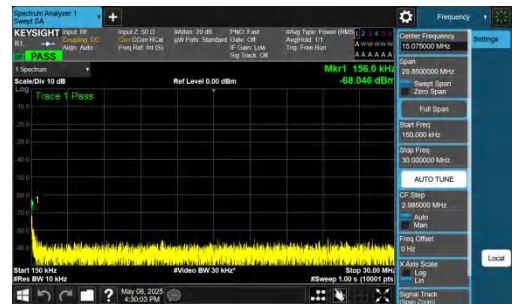
NTNV-n26(824-849)-PC3-15-5-H-DFT-QPSK-Inner_1RB_Left-0.1 5-30-PASS
