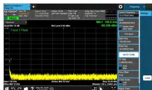
NTNV-n26(824-849)-PC3-15-10-H-DFT-BPSK-Inner_1RB_Right-0.15-30-PASS
