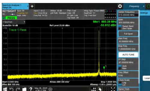
NTNV-n26(824-849)-PC3-15-10-H-DFT-QPSK-Inner_1RB_Left-30-1000-PASS
