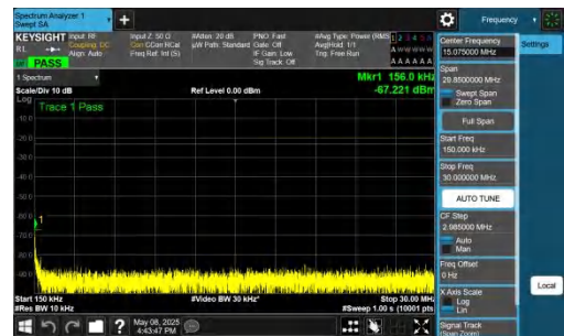
NTNV-n26(824-849)-PC3-15-15-M-DFT-QPSK-Inner_1RB_Right- 0.15-30-PASS
