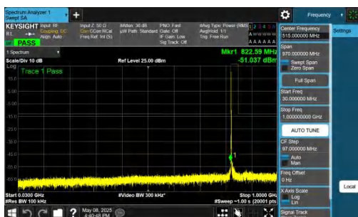
NTNV-n26(824-849)-PC3-15-15-L-DFT-QPSK-Inner_1RB_Left-30-1000-PASS
