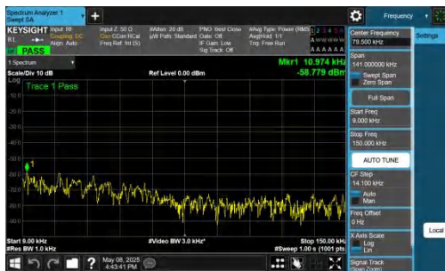
NTNV-n26(824-849)-PC3-15-15-M-DFT-QPSK-Inner_1RB_Right- 0.009-0.15-PASS
