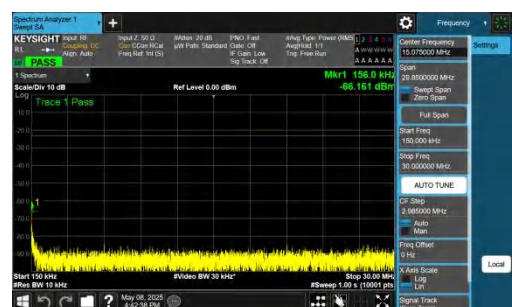
NTNV-n26(824-849)-PC3-15-15-M-DFT-BPSK-Inner_1RB_Right-0.15-30-PASS
