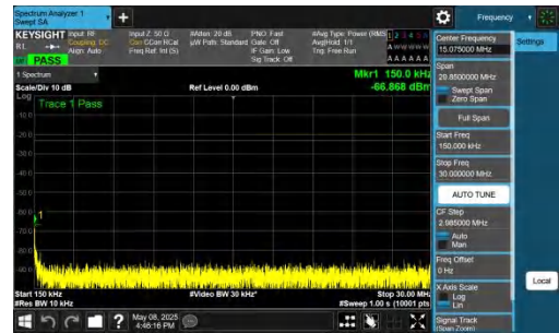
NTNV-n26(824-849)-PC3-15-15-H-DFT-QPSK-Inner_1RB_Right-0 .15-30-PASS
