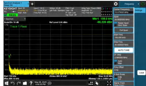
NTNV-n26(824-849)-PC3-15-15-H-DFT-BPSK-Inner_1RB_Left-0.15-30-PASS
