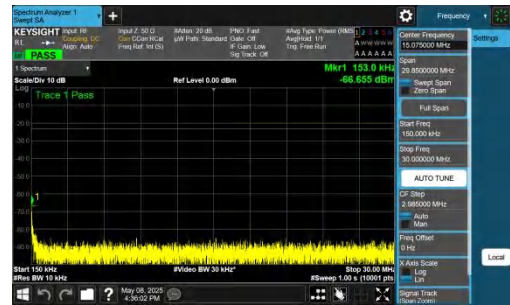
NTNV-n26(824-849)-PC3-15-10-M-DFT-QPSK-Inner_1RB_Right- 0.15-30-PASS
