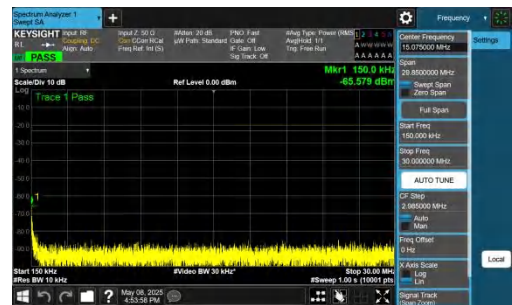
NTNV-n26(824-849)-PC3-15-20-H-DFT-QPSK-Inner_1RB_Right-0 .15-30-PASS
