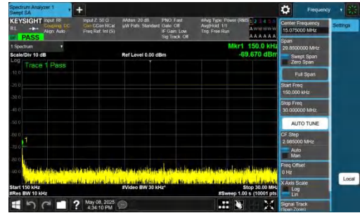
NTNV-n26(824-849)-PC3-15-10-M-DFT-BPSK-Inner_1RB_Left-0.15-30-PASS
