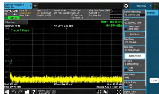
NTNV-n26(824-849)-PC3-15-15-H-DFT-QPSK-Inner_1RB_Left-0.15-30-PASS
