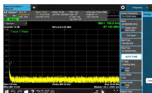
NTNV-n26(824-849)-PC3-15-15-L-DFT-QPSK-Inner_1RB_Right-0 .15-30-PASS
