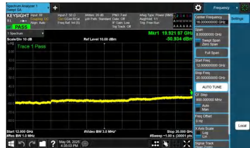
NTNV-n26(824-849)-PC3-15-10-M-DFT-BPSK-Inner_1RB_Right-12000-20000-PASS
