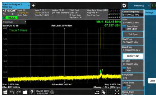
NTNV-n26(824-849)-PC3-15-20-M-DFT-BPSK-Inner_1RB_Left-3 0-1000-PASS
