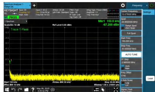
NTNV-n26(824-849)-PC3-15-10-M-DFT-BPSK-Inner_1RB_Right-0.15-30-PASS
