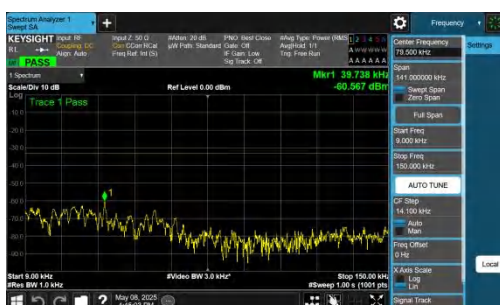
NTNV-n26(824-849)-PC3-15-15-H-DFT-BPSK-Inner_1RB_Right-0.009-0.15-PASS
