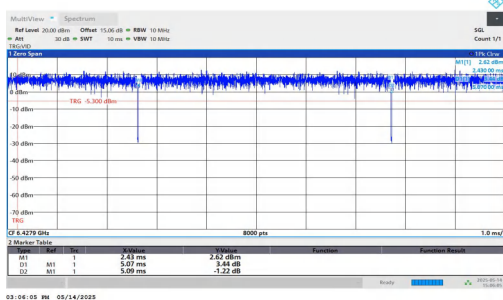
NTNV-11AX20MIMO-Ant1-6435-106Tone-RU53
