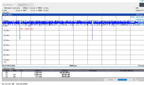
NTNV-11AX20MIMO-Ant1-6475-106Tone-RU53
