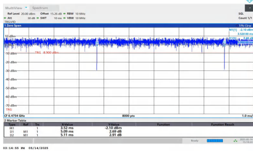
NTNV-11AX20MIMO-Ant1-6475-52Tone-RU39
