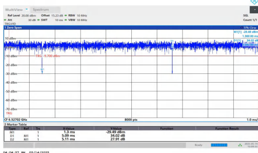
NTNV-11AX20MIMO-Ant1-6535-52Tone-RU37
