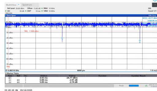
NTNV-11AX20MIMO-Ant2-6875-106Tone-RU54
