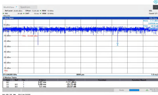
NTNV-11AX20MIMO-Ant1-6855-52Tone-RU40
