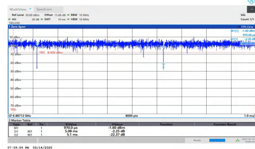
NTNV-11AX20MIMO-Ant2-6895-52Tone-RU37
