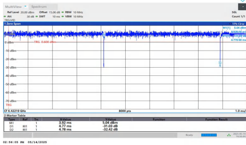
NTNV-11AX20MIMO-Ant1-6435-26Tone-RU0
