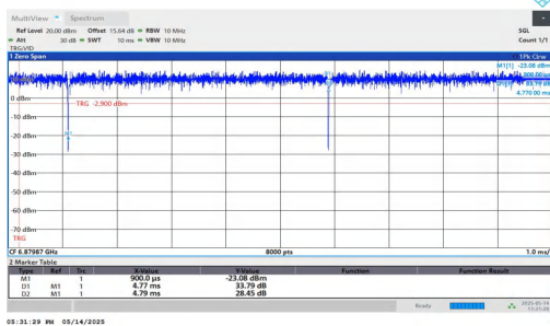
NTNV-11AX20MIMO-Ant1-6895-26Tone-RU0
