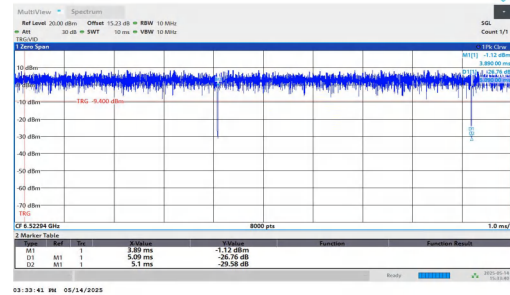
NTNV-11AX20MIMO-Ant2-6515-52Tone-RU40
