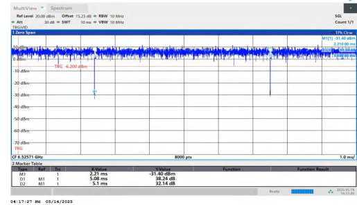
NTNV-11AX20MIMO-Ant2-6535-106Tone-RU53
