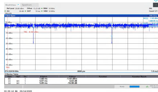
NTNV-11AX20MIMO-Ant2-6515-106Tone-RU54
