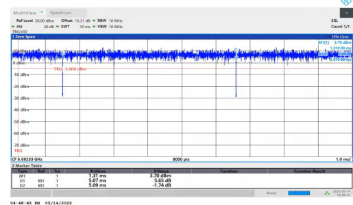
NTNV-11AX20MIMO-Ant2-6695-106Tone-RU53
