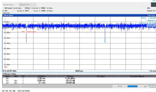
NTNV-11AX20MIMO-Ant1-6435-52Tone-RU37
