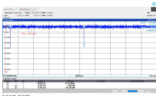
NTNV-11AX20MIMO-Ant1-6875-26Tone-RU8
