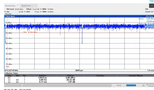
NTNV-11AX20MIMO-Ant2-6535-52Tone-RU37
