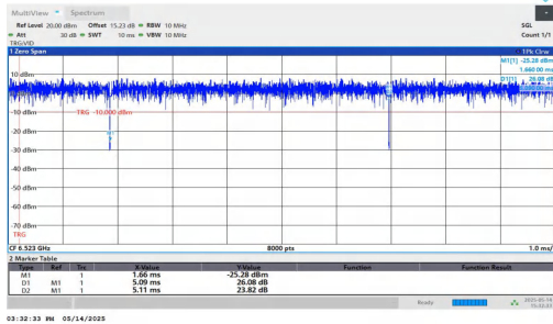
NTNV-11AX20MIMO-Ant1-6515-52Tone-RU40
