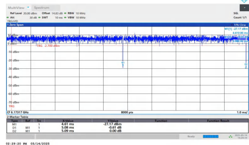
NTNV-11AX20MIMO-Ant2-6175-106Tone-RU53
