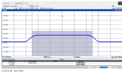
11AX160MIMO-Ant1-6185-Center-6258.3374-OFF-PASS
