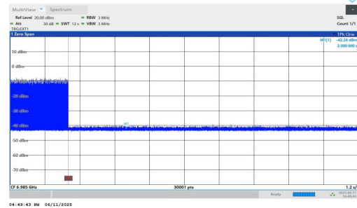
11AX160MIMO-Ant1-6985-High-7058.386-OFF-PASS
