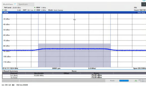
11AX160MIMO-Ant1-6185-Low-6111.1324-Minimal
