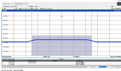
11AX160MIMO-Ant1-6665-Center-6738.9118-Minimal
