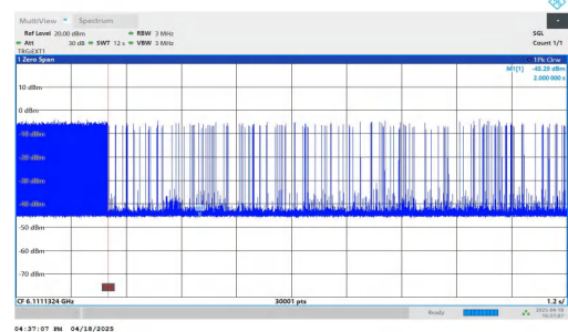
11AX160MIMO-Ant1-6185-Center-6185-Minimal
