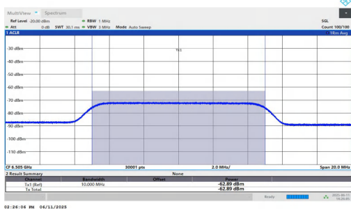
11AX160MIMO-Ant1-6505-High-6578.4549-Minimal
