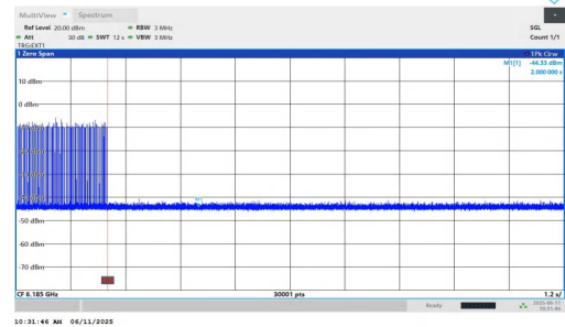
11AX160MIMO-Ant1-6185-Center-6258.3374-OFF-PASS
