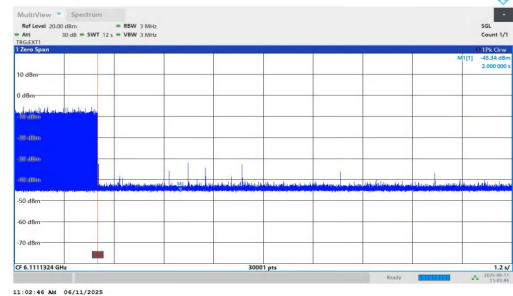
11AX160MIMO-Ant1-6185-Low-6111.1324-Minimal
