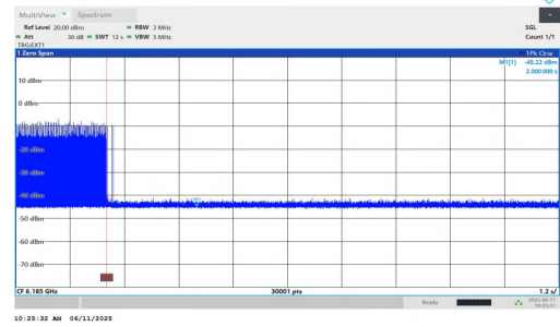
11AX160MIMO-Ant1-6185-Center-6111.1324-Minimal
