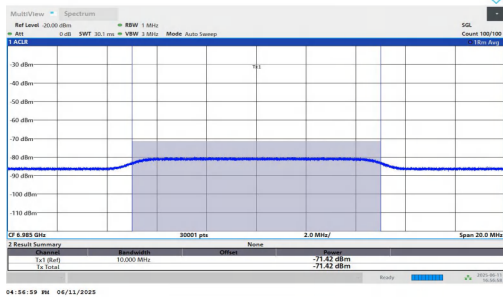
11AX160MIMO-Ant1-6985-High-7058.386-OFF-PASS
