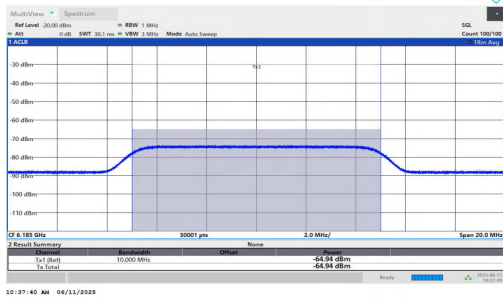
11AX160MIMO-Ant1-6185-Center-6111.1324-Minimal
