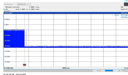
11AX160MIMO-Ant1-6985-High-7058.386-Minimal
