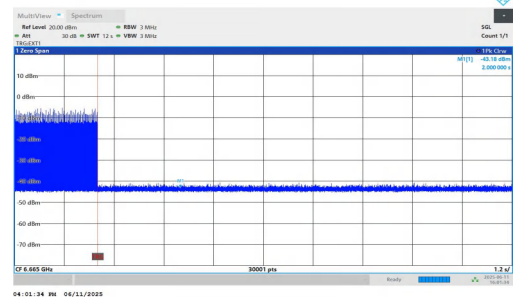
11AX160MIMO-Ant1-6665-Center-6738.9118-Minimal
