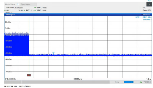
11AX160MIMO-Ant1-6665-Center-6738.9118-OFF-PASS
