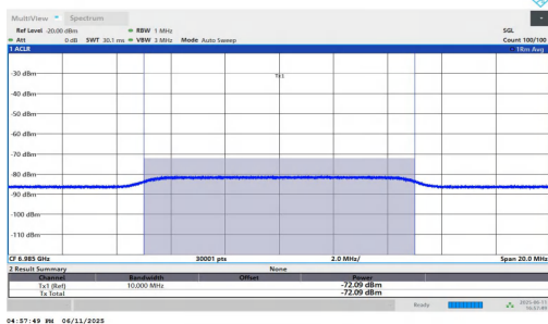
11AX160MIMO-Ant1-6985-High-7058.386-Minimal
