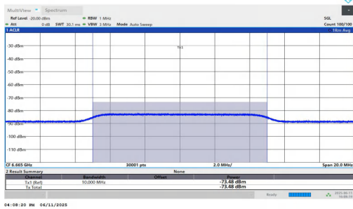
11AX160MIMO-Ant1-6665-Center-6738.9118-OFF-PASS
