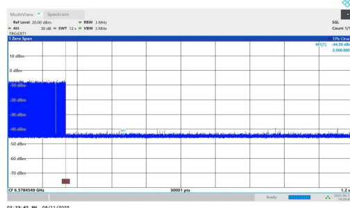
11AX160MIMO-Ant1-6505-Low-6431.1682-Minimal
