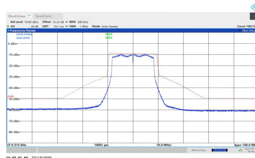
NTNV-11A-CDD-Ant2-6535-PASS
