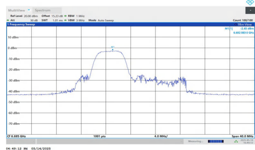
11AX20MIMO-Ant2-6695-106Tone-RU53-PASS
