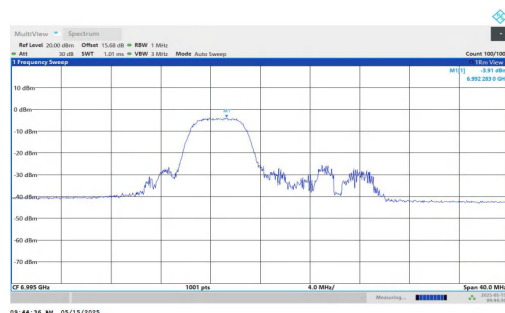
11AX20MIMO-Ant2-6995-106Tone-RU53-PASS
