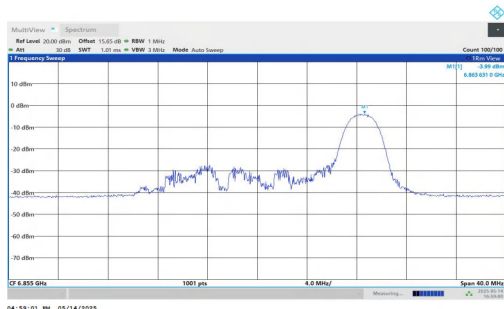
11AX20MIMO-Ant1-6855-52Tone-RU40-PASS
