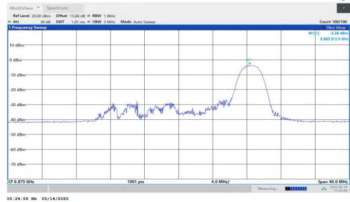
11AX20MIMO-Ant2-6875-52Tone-RU40-PASS
