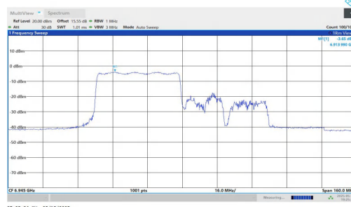
11AX80MIMO-Ant2-7025-484Tone-RU66-PASS
