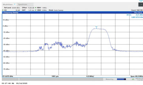
11AX20MIMO-Ant1-6875-106Tone-RU54-PASS
