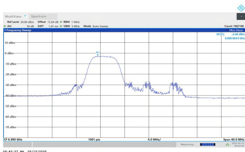
11AX20MIMO-Ant1-6995-106Tone-RU53-PASS
