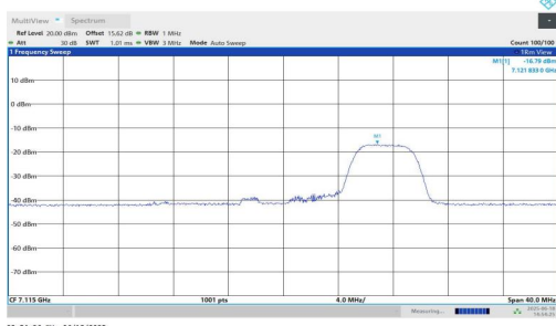
11AX20MIMO-Ant1-7115-106Tone-RU54-PASS
