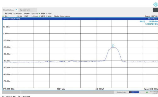
11AX20MIMO-Ant1-7115-52Tone-RU40-PASS
