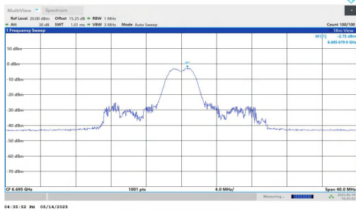
11AX20MIMO-Ant1-6695-52Tone-RU39-PASS
