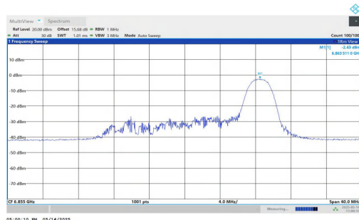
11AX20MIMO-Ant2-6855-52Tone-RU40-PASS
