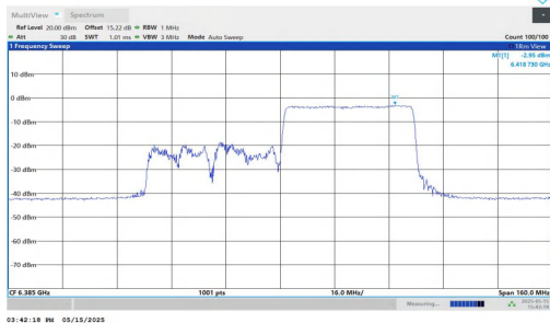
11AX80MIMO-Ant1-6465-484Tone-RU65-PASS
