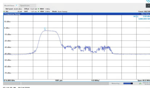
11AX20MIMO-Ant2-6895-106Tone-RU53-PASS
