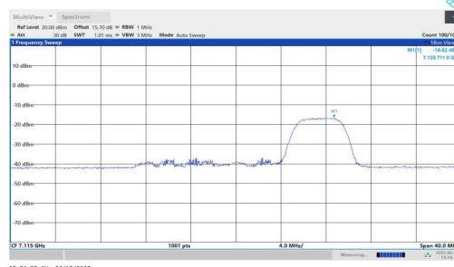
11AX20MIMO-Ant2-7115-106Tone-RU54-PASS
