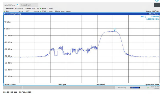
11AX20MIMO-Ant2-6875-106Tone-RU54-PASS
