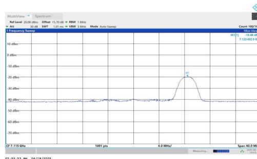
11AX20MIMO-Ant2-7115-52Tone-RU40-PASS
