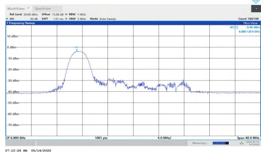
11AX20MIMO-Ant2-6895-52Tone-RU37-PASS
