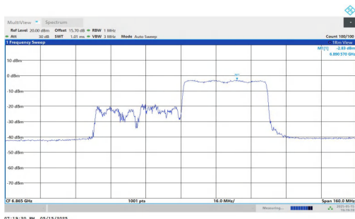
11AX80MIMO-Ant1-6945-484Tone-RU65-PASS
