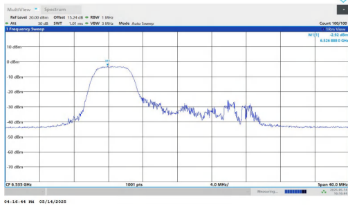
11AX20MIMO-Ant1-6535-106Tone-RU53-PASS
