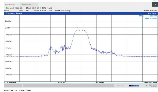
11AX20MIMO-Ant2-6695-52Tone-RU39-PASS
