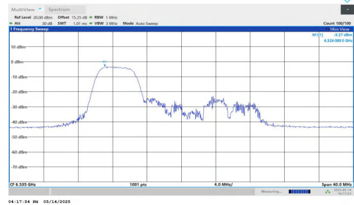
11AX20MIMO-Ant2-6535-106Tone-RU53-PASS
