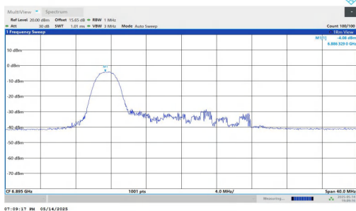
11AX20MIMO-Ant1-6895-52Tone-RU37-PASS
