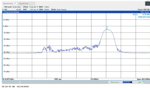
11AX20MIMO-Ant1-6875-52Tone-RU40-PASS
