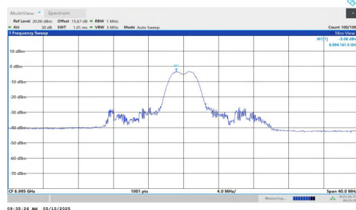
11AX20MIMO-Ant2-6995-52Tone-RU39-PASS
