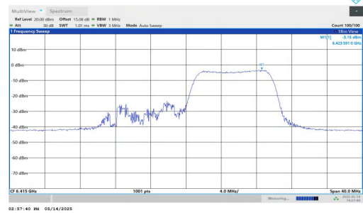
11AX20MIMO-Ant2-6435-26Tone-RU0-PASS
