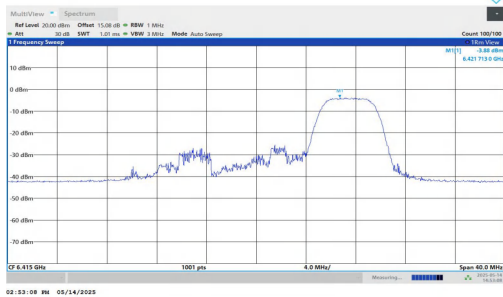
11AX20MIMO-Ant1-6415-106Tone-RU54-PASS
