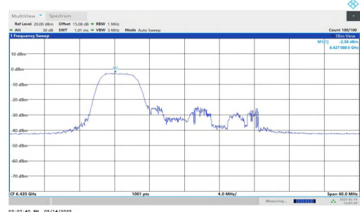
11AX20MIMO-Ant2-6435-106Tone-RU53-PASS
