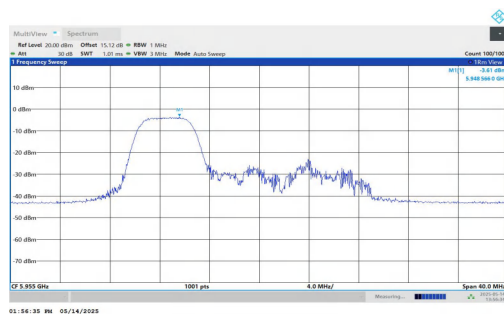
11AX20MIMO-Ant2-5955-106Tone-RU53-PASS
