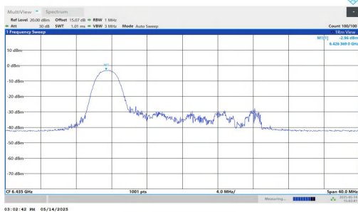
11AX20MIMO-Ant1-6435-52Tone-RU37-PASS
