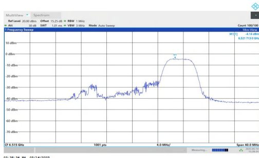
11AX20MIMO-Ant1-6515-106Tone-RU54-PASS
