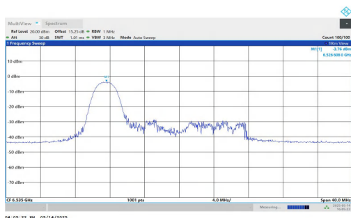
11AX20MIMO-Ant1-6535-52Tone-RU37-PASS
