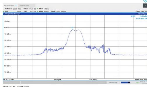
11AX20MIMO-Ant2-6175-52Tone-RU39-PASS
