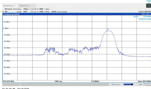
11AX20MIMO-Ant1-6515-52Tone-RU40-PASS
