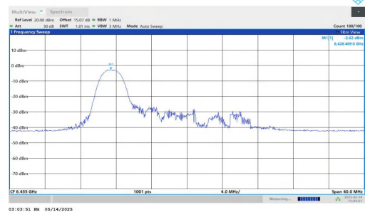
11AX20MIMO-Ant2-6435-52Tone-RU37-PASS
