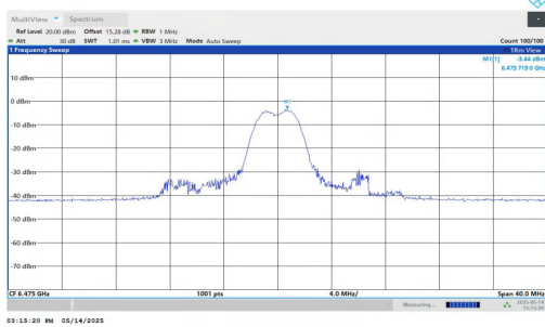
11AX20MIMO-Ant1-6475-52Tone-RU39-PASS
