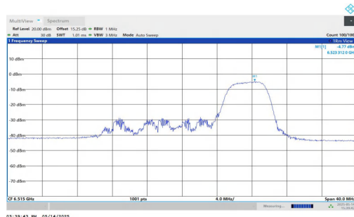
11AX20MIMO-Ant2-6515-106Tone-RU54-PASS
