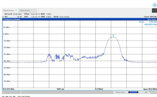
11AX20MIMO-Ant1-6415-52Tone-RU40-PASS
