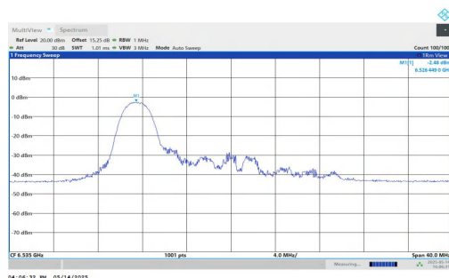
11AX20MIMO-Ant2-6535-52Tone-RU37-PASS
