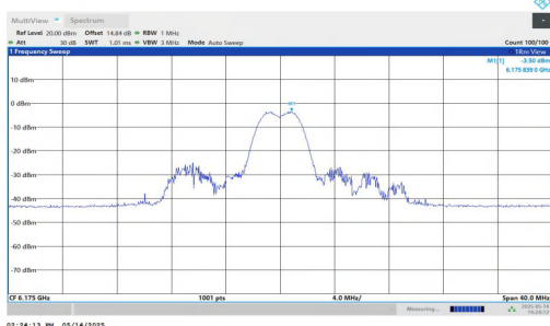
11AX20MIMO-Ant1-6175-52Tone-RU39-PASS
