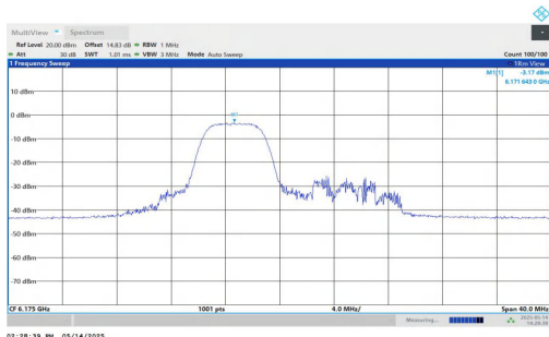
11AX20MIMO-Ant1-6175-106Tone-RU53-PASS
