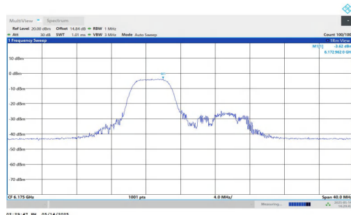
11AX20MIMO-Ant2-6175-106Tone-RU53-PASS
