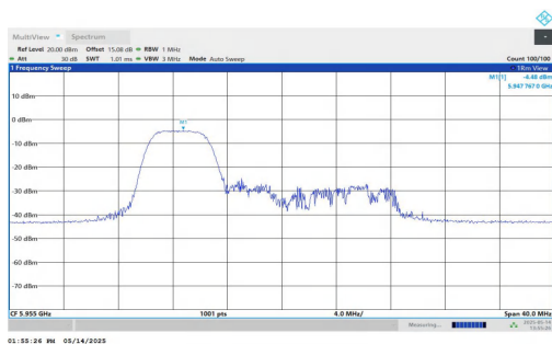
11AX20MIMO-Ant1-5955-106Tone-RU53-PASS
