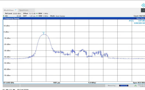
11AX20MIMO-Ant2-5955-52Tone-RU37-PASS
