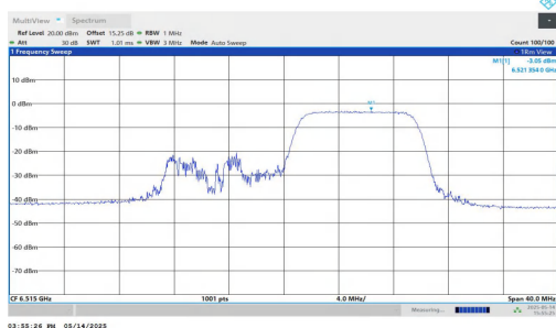
11AX20MIMO-Ant1-6535-26Tone-RU0-PASS
