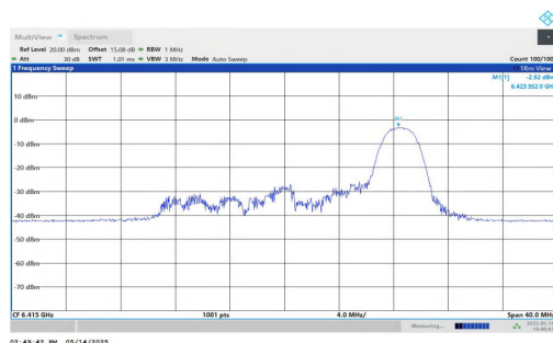
11AX20MIMO-Ant2-6415-52Tone-RU40-PASS
