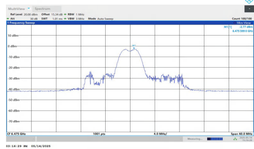
11AX20MIMO-Ant2-6475-52Tone-RU39-PASS
