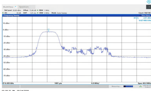
11AX20MIMO-Ant1-6435-106Tone-RU53-PASS
