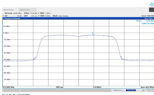
11AX20MIMO-Ant1-6875-PASS
