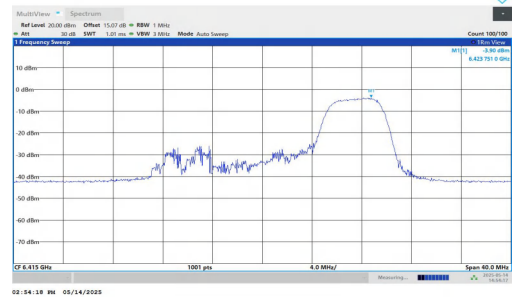
11AX20MIMO-Ant2-6415-106Tone-RU54-PASS
