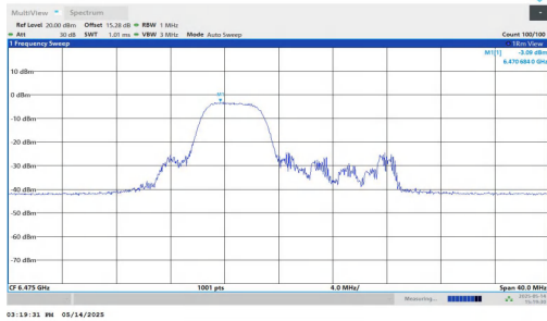
11AX20MIMO-Ant1-6475-106Tone-RU53-PASS
