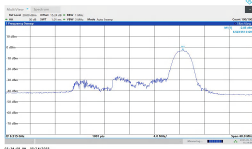
11AX20MIMO-Ant2-6515-52Tone-RU40-PASS
