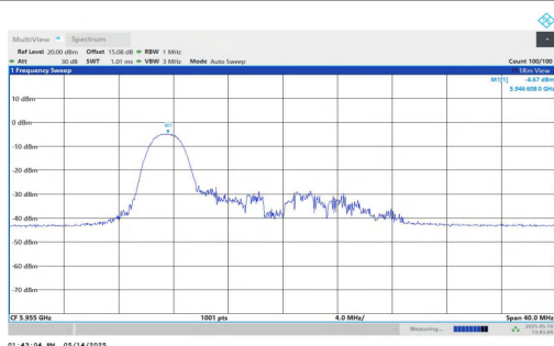
11AX20MIMO-Ant1-5955-52Tone-RU37-PASS
