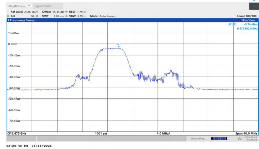
11AX20MIMO-Ant2-6475-106Tone-RU53-PASS
