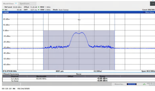
11AX20MIMO-Ant1-6475-52Tone-RU39-PASS
