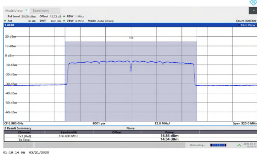
11AX160MIMO-Ant1-6985-PASS
