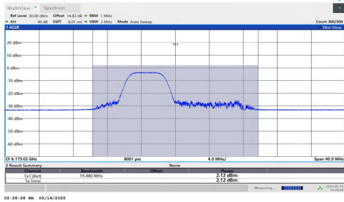
11AX20MIMO-Ant1-6175-106Tone-RU53-PASS
