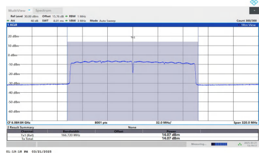
11AX160MIMO-Ant2-6985-PASS
