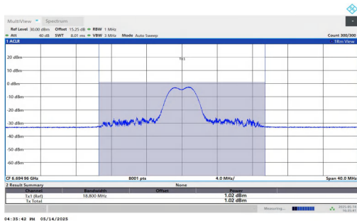
11AX20MIMO-Ant1-6695-52Tone-RU39-PASS
