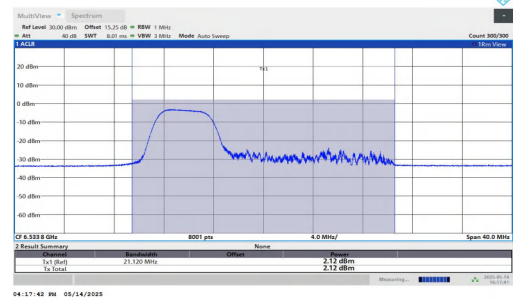
11AX20MIMO-Ant2-6535-106Tone-RU53-PASS
