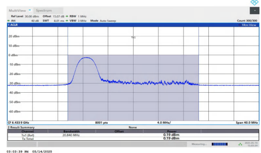
11AX20MIMO-Ant2-6435-52Tone-RU37-PASS
