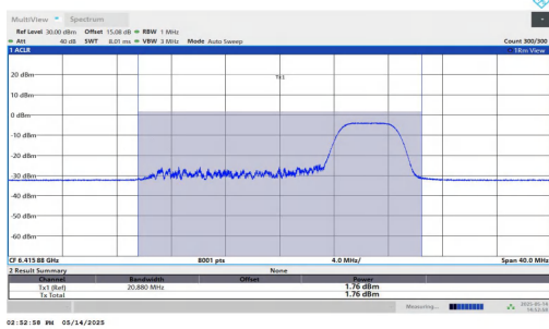
11AX20MIMO-Ant1-6415-106Tone-RU54-PASS
