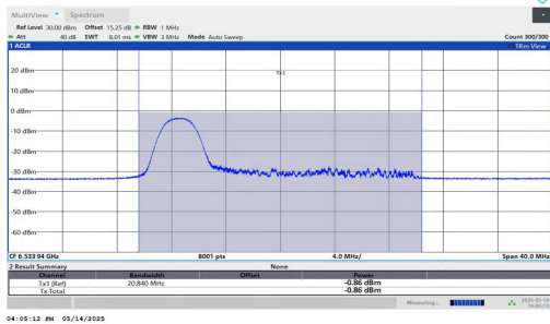
11AX20MIMO-Ant1-6535-52Tone-RU37-PASS
