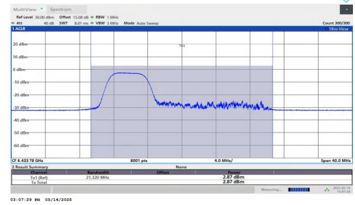
11AX20MIMO-Ant2-6435-106Tone-RU53-PASS
