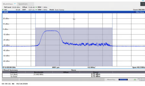
11AX20MIMO-Ant1-6435-106Tone-RU53-PASS
