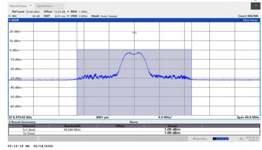
11AX20MIMO-Ant2-6475-52Tone-RU39-PASS
