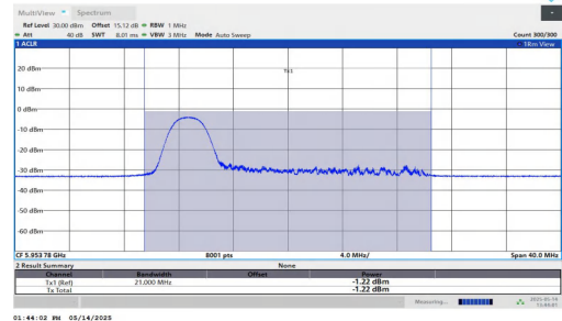
11AX20MIMO-Ant2-5955-52Tone-RU37-PASS
