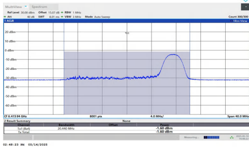
11AX20MIMO-Ant1-6415-52Tone-RU40-PASS
