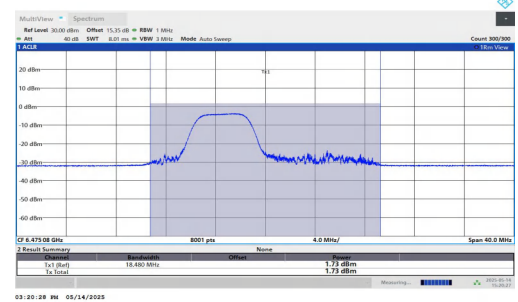
11AX20MIMO-Ant2-6475-106Tone-RU53-PASS
