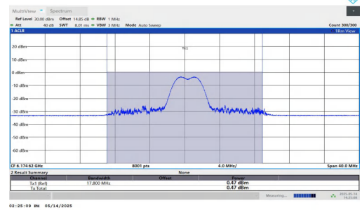
11AX20MIMO-Ant2-6175-52Tone-RU39-PASS
