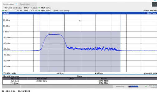
11AX20MIMO-Ant1-5955-106Tone-RU53-PASS
