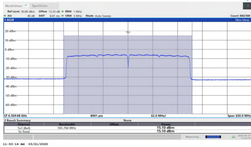
11AX160MIMO-Ant1-6665-PASS
