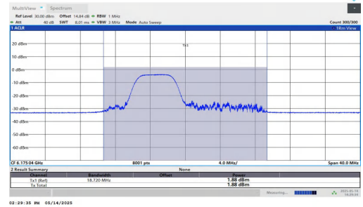
11AX20MIMO-Ant2-6175-106Tone-RU53-PASS
