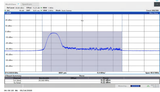
11AX20MIMO-Ant2-6535-52Tone-RU37-PASS
