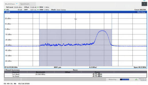
11AX20MIMO-Ant2-6415-52Tone-RU40-PASS
