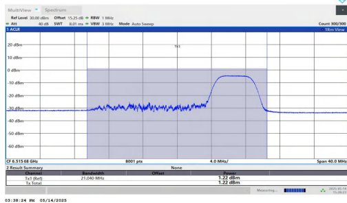
11AX20MIMO-Ant1-6515-106Tone-RU54-PASS
