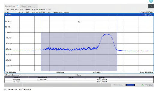
11AX20MIMO-Ant2-6515-52Tone-RU40-PASS
