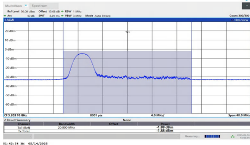
11AX20MIMO-Ant1-5955-52Tone-RU37-PASS
