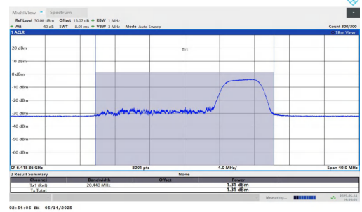
11AX20MIMO-Ant2-6415-106Tone-RU54-PASS
