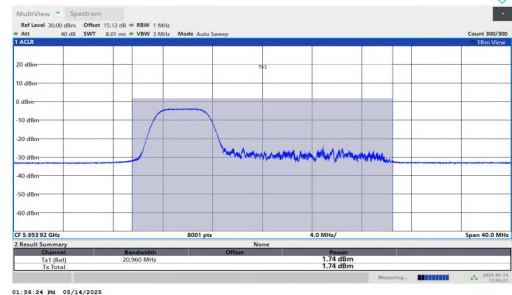
11AX20MIMO-Ant2-5955-106Tone-RU53-PASS
