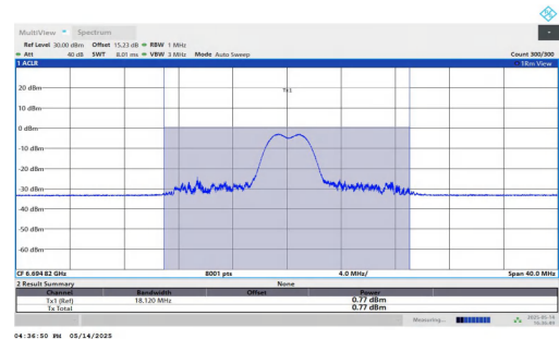
11AX20MIMO-Ant2-6695-52Tone-RU39-PASS
