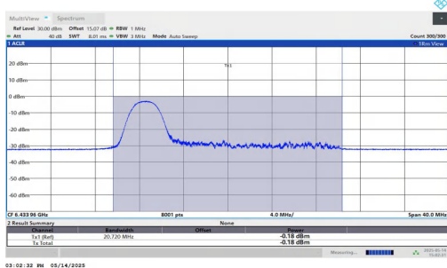
11AX20MIMO-Ant1-6435-52Tone-RU37-PASS
