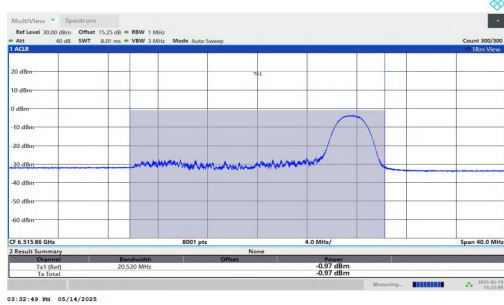
11AX20MIMO-Ant1-6515-52Tone-RU40-PASS
