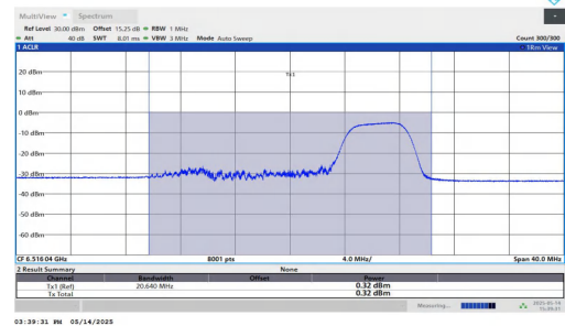
11AX20MIMO-Ant2-6515-106Tone-RU54-PASS
