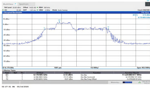
11AX20MIMO-Ant1-6175-106Tone-RU53-PASS
