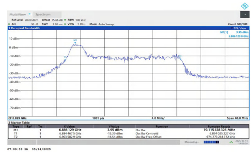
11AX20MIMO-Ant2-6895-52Tone-RU37-PASS
