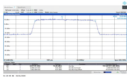
11AX160MIMO-Ant2-6985-PASS
