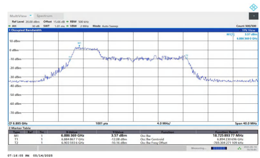
11AX20MIMO-Ant2-6895-106Tone-RU53-PASS
