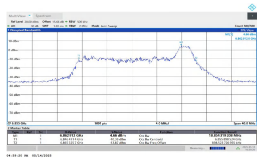
11AX20MIMO-Ant2-6855-52Tone-RU40-PASS
