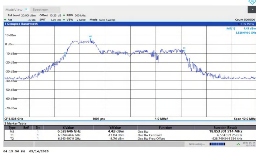
11AX20MIMO-Ant1-6535-106Tone-RU53-PASS
