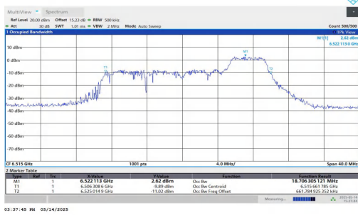
11AX20MIMO-Ant1-6515-106Tone-RU54-PASS
