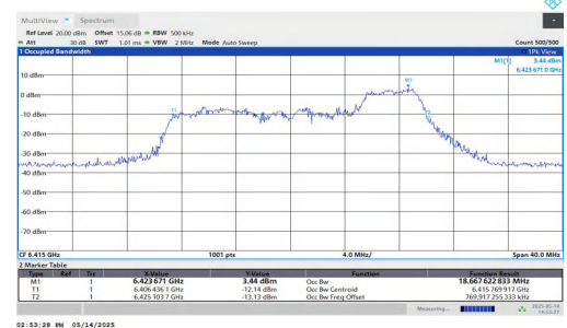
11AX20MIMO-Ant2-6415-106Tone-RU54-PASS
