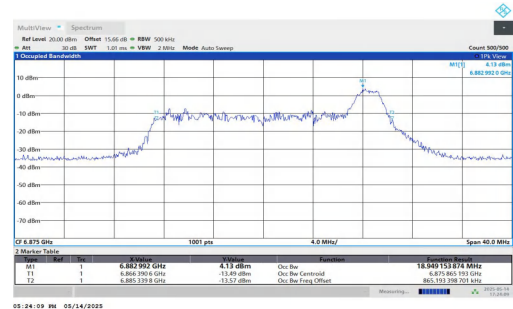
11AX20MIMO-Ant2-6875-52Tone-RU40-PASS
