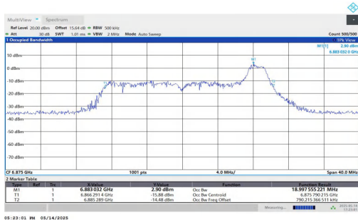
11AX20MIMO-Ant1-6875-52Tone-RU40-PASS
