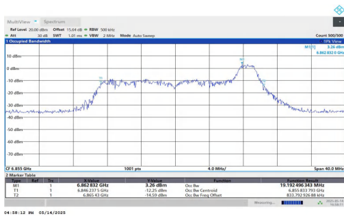
11AX20MIMO-Ant1-6855-52Tone-RU40-PASS
