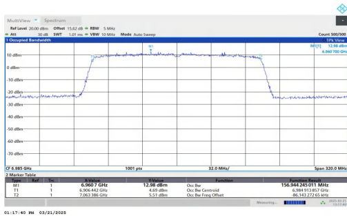
11AX160MIMO-Ant1-6985-PASS
