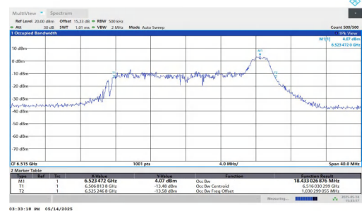
11AX20MIMO-Ant2-6515-52Tone-RU40-PASS
