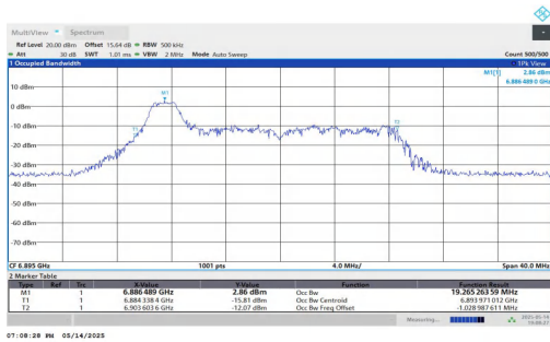
11AX20MIMO-Ant1-6895-52Tone-RU37-PASS
