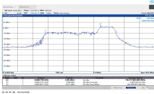
11AX20MIMO-Ant1-6855-106Tone-RU54-PASS
