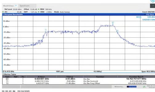
11AX20MIMO-Ant1-6415-106Tone-RU54-PASS
