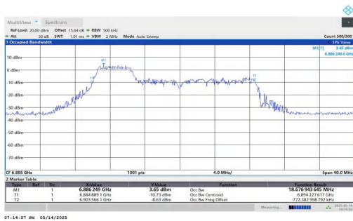
11AX20MIMO-Ant1-6895-106Tone-RU53-PASS
