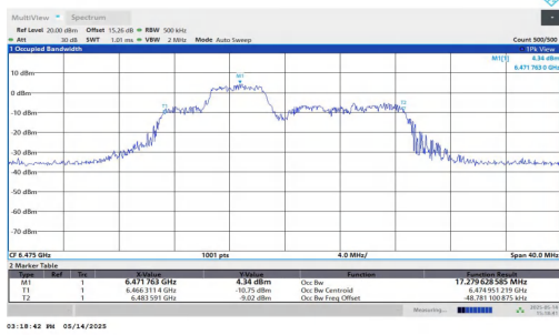
11AX20MIMO-Ant1-6475-106Tone-RU53-PASS
