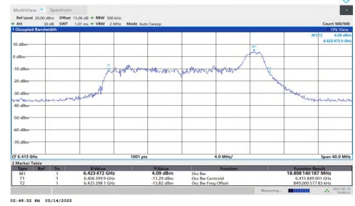
11AX20MIMO-Ant2-6415-52Tone-RU40-PASS
