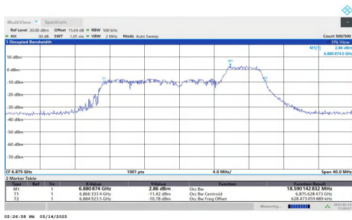
11AX20MIMO-Ant1-6875-106Tone-RU54-PASS
