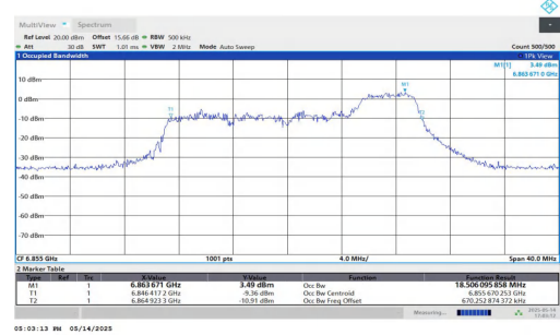
11AX20MIMO-Ant2-6855-106Tone-RU54-PASS
