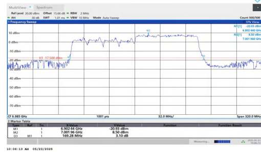
11AX160MIMO-Ant2-6985-996Tone-RU68
