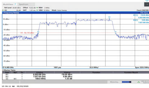
11AX160MIMO-Ant1-6985-996Tone-RU68
