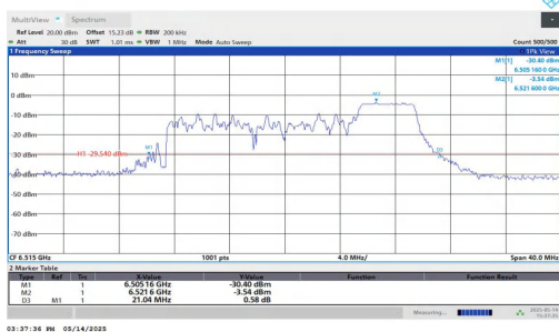
11AX20MIMO-Ant1-6515-106Tone-RU54
