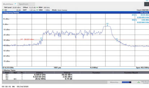
11AX20MIMO-Ant1-6515-52Tone-RU40
