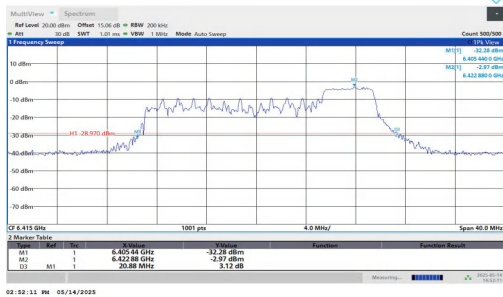
11AX20MIMO-Ant1-6415-106Tone-RU54
