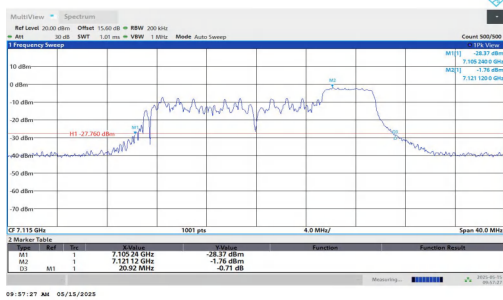
11AX20MIMO-Ant1-7115-106Tone-RU54
