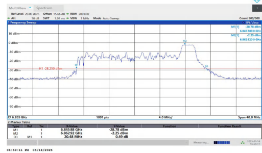
11AX20MIMO-Ant2-6855-52Tone-RU40
