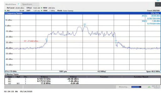
11AX20MIMO-Ant2-6175-52Tone-RU39
