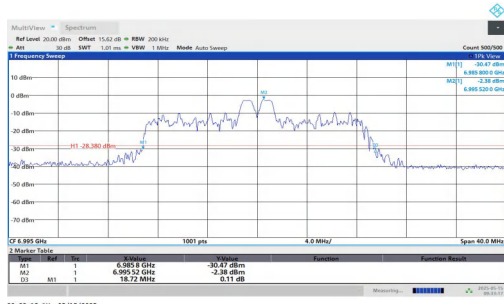
11AX20MIMO-Ant1-6995-52Tone-RU39
