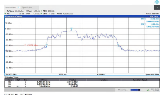
11AX20MIMO-Ant2-6475-106Tone-RU53
