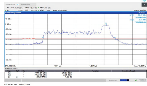
11AX20MIMO-Ant2-7115-52Tone-RU40
