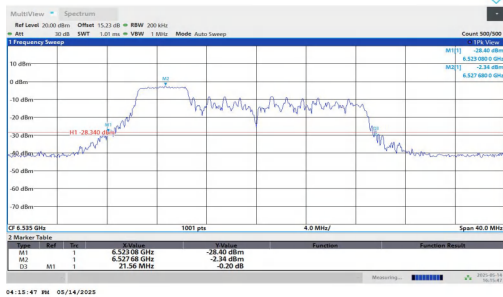
11AX20MIMO-Ant1-6535-106Tone-RU53
