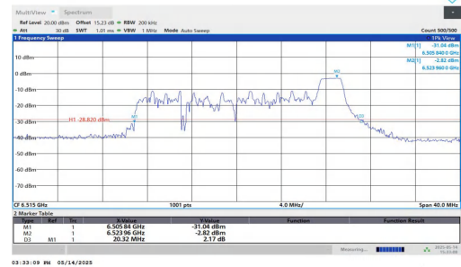
11AX20MIMO-Ant2-6515-52Tone-RU40
