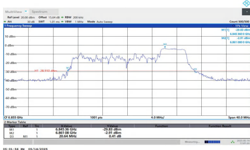
11AX20MIMO-Ant1-6855-106Tone-RU54
