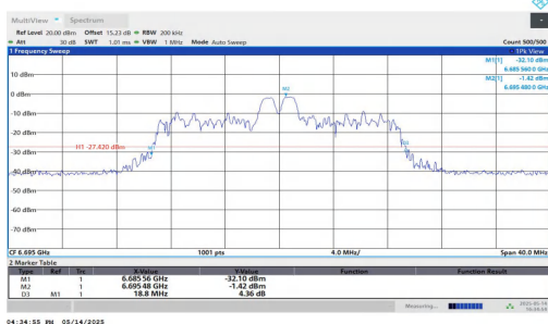
11AX20MIMO-Ant1-6695-52Tone-RU39
