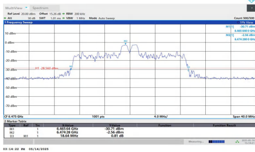
11AX20MIMO-Ant1-6475-52Tone-RU39
