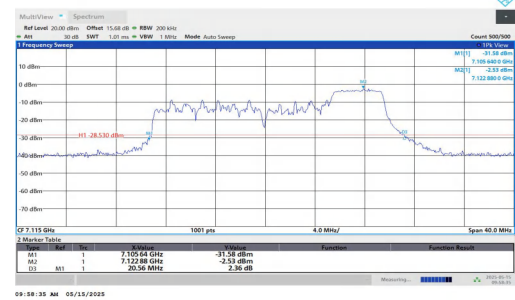
11AX20MIMO-Ant2-7115-106Tone-RU54
