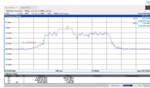
11AX20MIMO-Ant2-6695-106Tone-RU53
