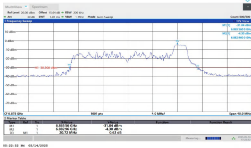
11AX20MIMO-Ant1-6875-52Tone-RU40
