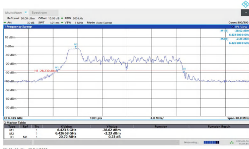
11AX20MIMO-Ant1-6435-52Tone-RU37
