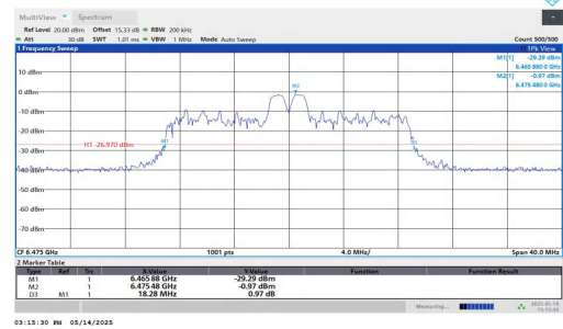
11AX20MIMO-Ant2-6475-52Tone-RU39
