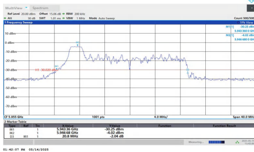
11AX20MIMO-Ant1-5955-52Tone-RU37
