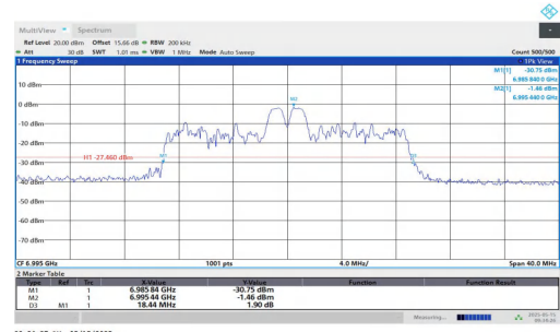
11AX20MIMO-Ant2-6995-52Tone-RU39
