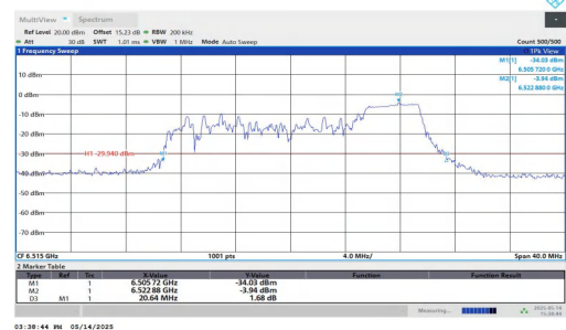
11AX20MIMO-Ant2-6515-106Tone-RU54
