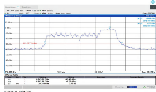
11AX20MIMO-Ant2-6855-106Tone-RU54
