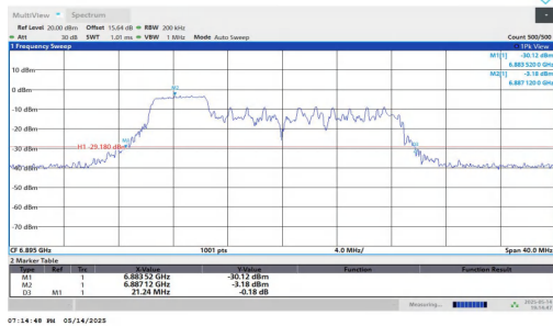
11AX20MIMO-Ant1-6895-106Tone-RU53
