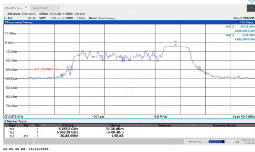
11AX20MIMO-Ant1-6875-106Tone-RU54
