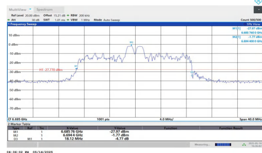
11AX20MIMO-Ant2-6695-52Tone-RU39
