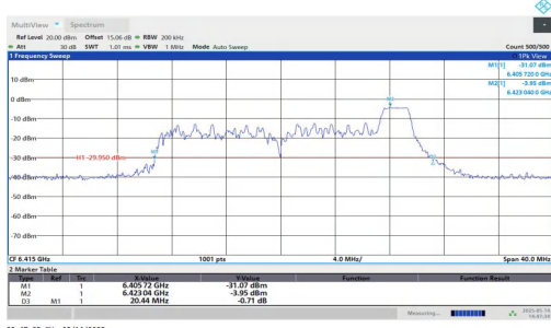
11AX20MIMO-Ant1-6415-52Tone-RU40
