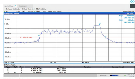
11AX20MIMO-Ant2-6415-52Tone-RU40
