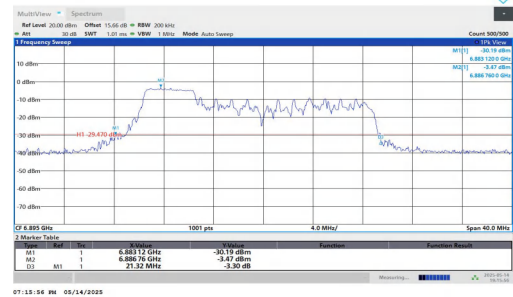
11AX20MIMO-Ant2-6895-106Tone-RU53
