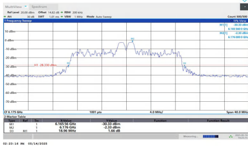
11AX20MIMO-Ant1-6175-52Tone-RU39
