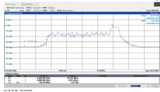
11AX20MIMO-Ant2-6875-52Tone-RU40
