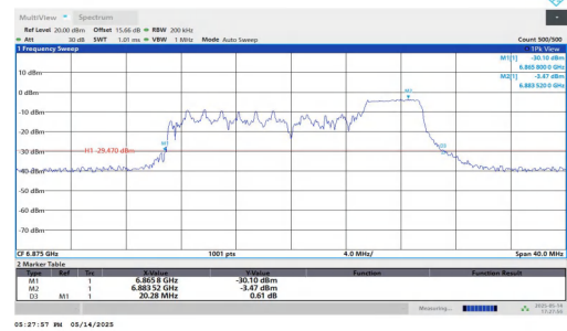
11AX20MIMO-Ant2-6875-106Tone-RU54
