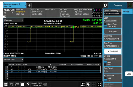
NTNV-11AX20MIMO-Ant2-5700-106Tone-RU54
