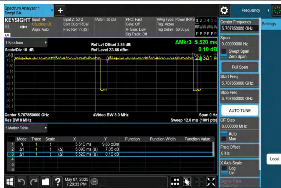
NTNV-11AX20MIMO-Ant1-5700-52Tone-RU40
