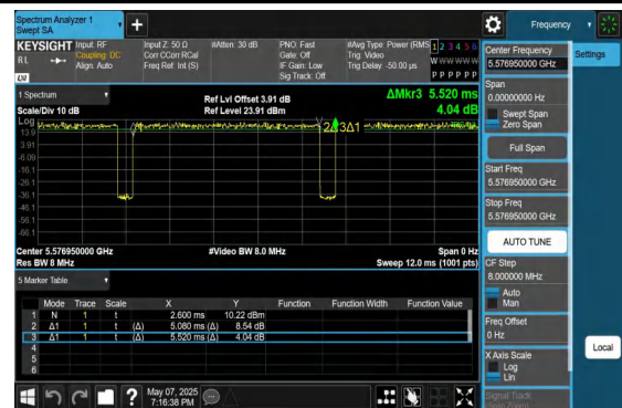
NTNV-11AX20MIMO-Ant2-5580-106Tone-RU53
