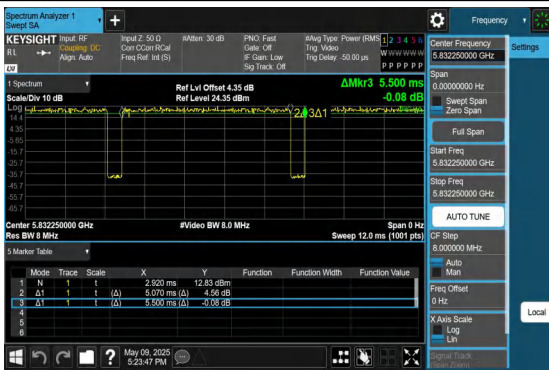
NTVN-11AX20MIMO-Ant1-5825-106Tone-RU54
