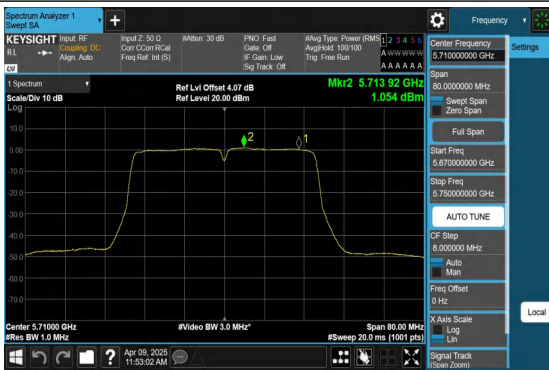
11AC40MIMO-Ant1-5710_UNII-3-PASS
