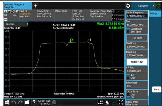
11AC40MIMO-Ant2-5710_UNII-3-PASS
