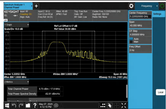
11AX20MIMO-Ant2-5220-106Tone-RU53-PASS
