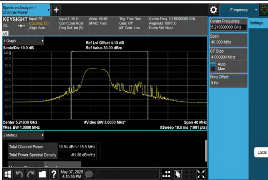
11AX20MIMO-Ant1-5220-106Tone-RU53-PASS
