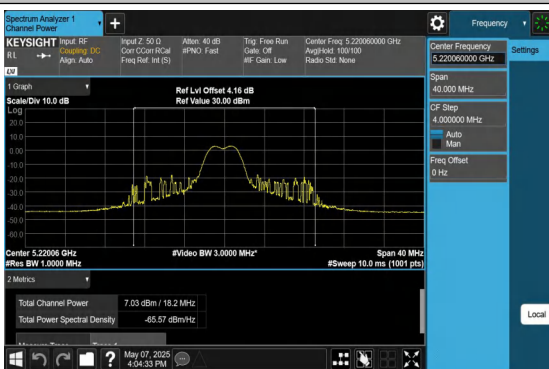
11AX20MIMO-Ant1-5220-52Tone-RU39-PASS
