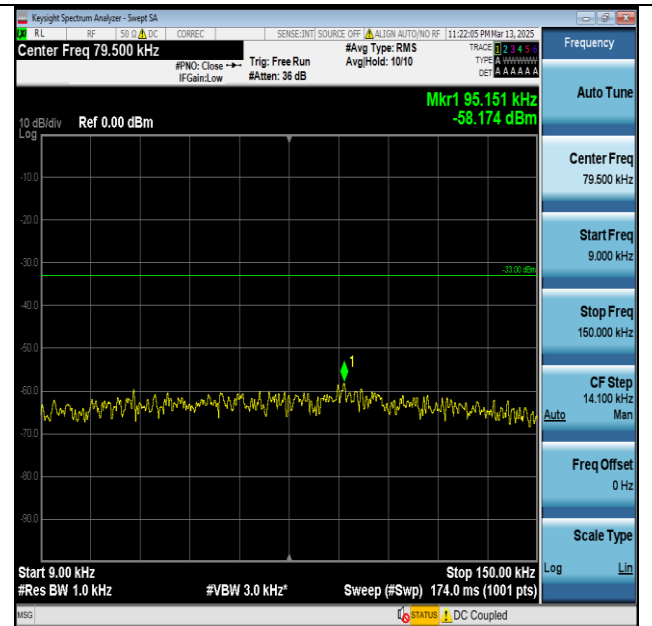
Band26(824-849)-15MHz-QPSK-26915-1RB#0- 0.009~0.15-PASS
