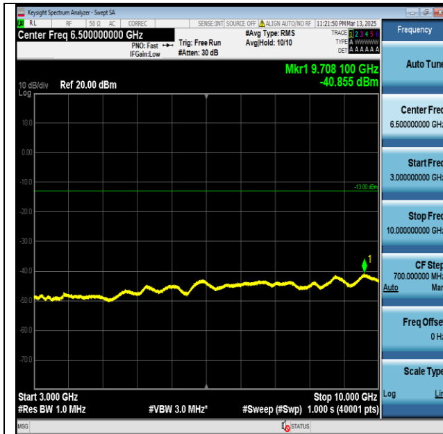
Band26(824-849)-15MHz-QPSK-26865-1RB#0- 3000~10000-PASS
