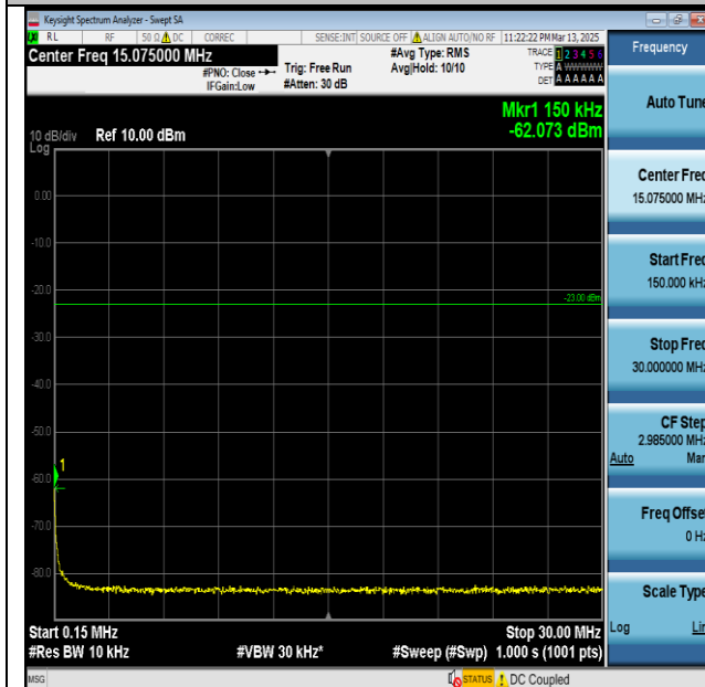
Band26(824-849)-15MHz-QPSK-26915-1RB#0-0.15~30- PASS
