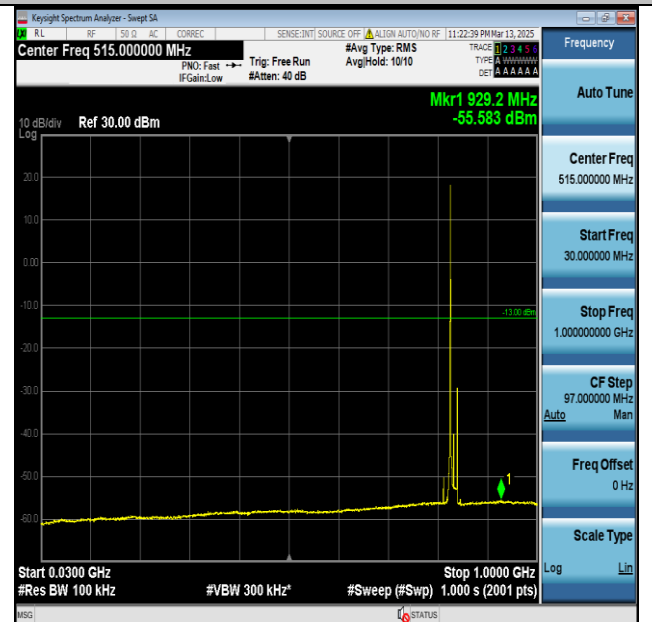
Band26(824-849)-15MHz-QPSK-26915-1RB#0-30~1000- PASS
