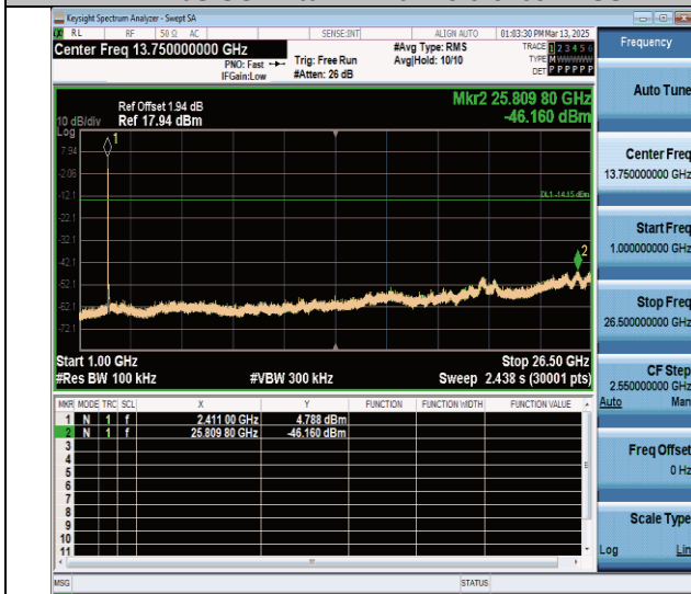
11n20SISO-Ant0-2412-1000-26500-PASS
