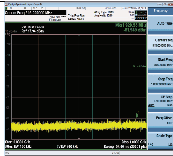
11n20SISO-Ant0-2412-30-1000-PASS
