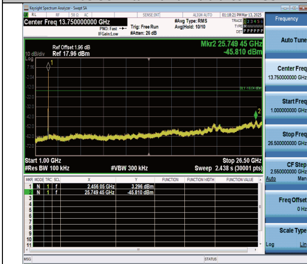
11n20SISO-Ant0-2462-1000-26500-PASS
