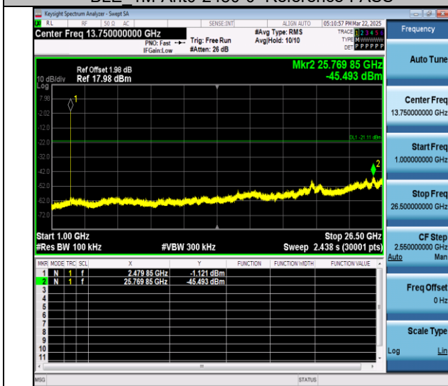
BLE_1M-Ant0-2480-1000~26500-PASS
