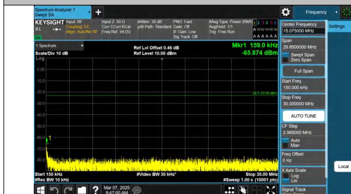
Band71-15MHz-QPSK-133397-1RB#74-0.15~30-PASS
