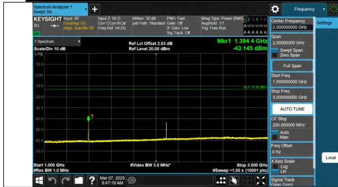
Band71-15MHz-QPSK-133397-1RB#74-1000~3000-PASS
