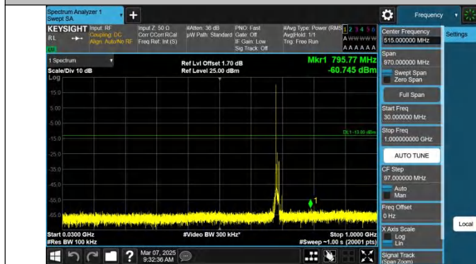
Band71-10MHz-QPSK-133422-1RB#0-30~1000-PASS
