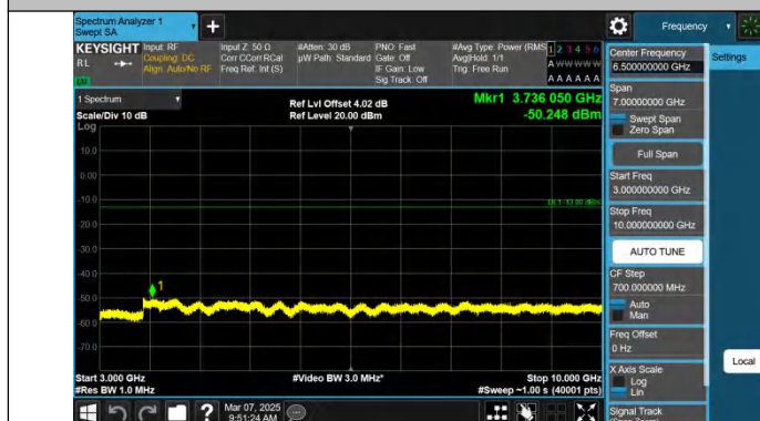
Band71-20MHz-QPSK-133222-1RB#0-3000~10000-PASS
