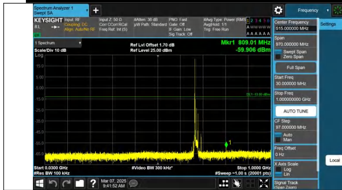
Band71-15MHz-QPSK-133297-1RB#0-30~1000-PASS
