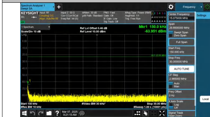
Band71-5MHz-QPSK-133447-1RB#24-0.15~30-PASS
