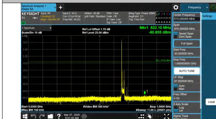
Band71-20MHz-QPSK-133222-1RB#0-30~1000-PASS
