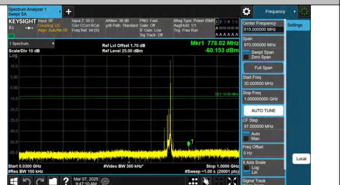
Band71-15MHz-QPSK-133397-1RB#74-30~1000-PASS
