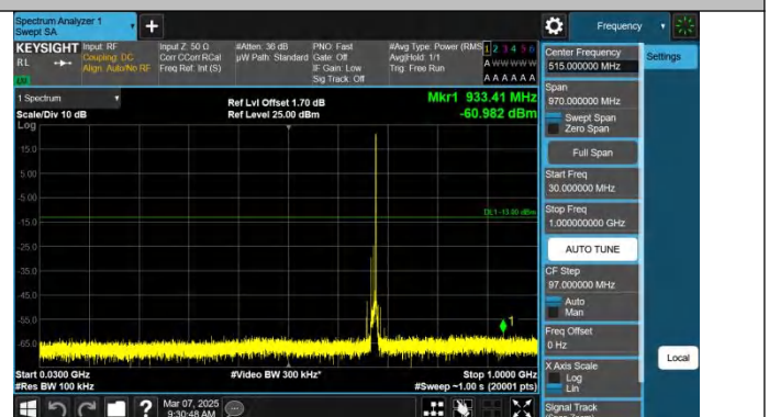
Band71-10MHz-QPSK-133297-1RB#49-30~1000-PASS
