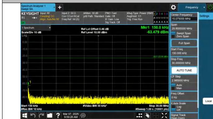
Band71-20MHz-QPSK-133372-1RB#99-0.15~30-PASS
