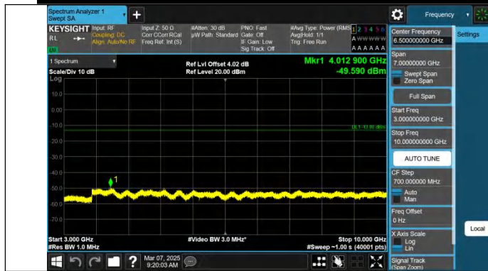
Band71-5MHz-QPSK-133447-1RB#0-3000~10000-PASS
