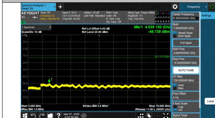
Band71-10MHz-QPSK-133422-1RB#0-3000~10000-PASS
