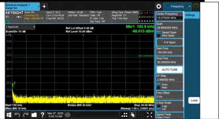
Band71-15MHz-QPSK-133397-1RB#0-0.15~30-PASS
