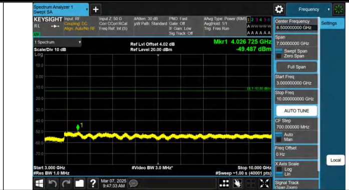
Band71-15MHz-QPSK-133397-1RB#74-3000~10000-PASS
