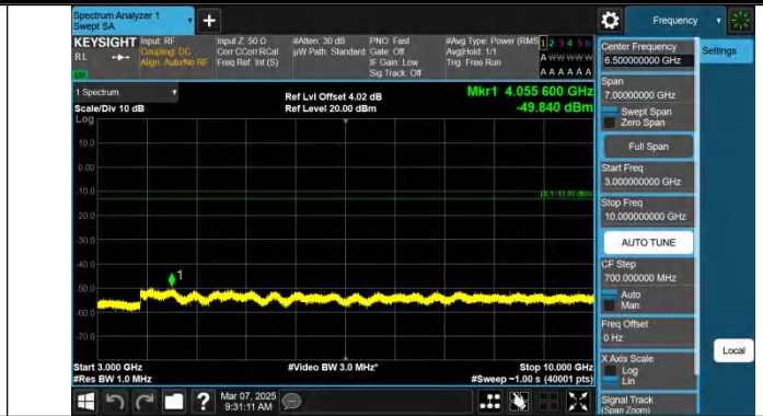
Band71-10MHz-QPSK-133297-1RB#49-3000~10000-PASS
