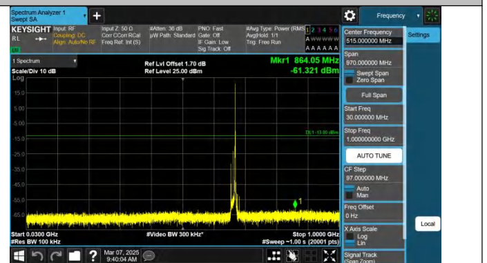
Band71-15MHz-QPSK-133197-1RB#74-30~1000-PASS
