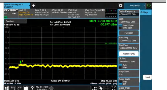
Band71-15MHz-QPSK-133297-1RB#74-3000~10000-PASS
