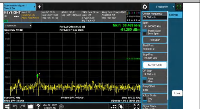
Band71-10MHz-QPSK-133297-1RB#49-0.009~0.15-PASS
