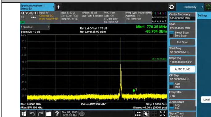
Band71-10MHz-QPSK-133297-1RB#0-30~1000-PASS
