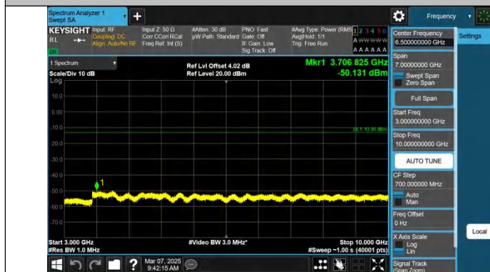
Band71-15MHz-QPSK-133297-1RB#0-3000~10000-PASS
