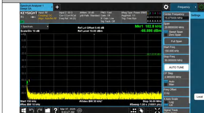
Band71-15MHz-QPSK-133297-1RB#74-0.15~30-PASS
