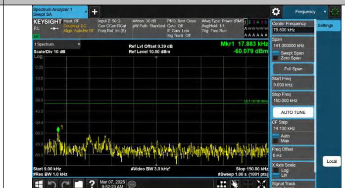
Band71-20MHz-QPSK-133222-1RB#99-0.009~0.15-PASS
