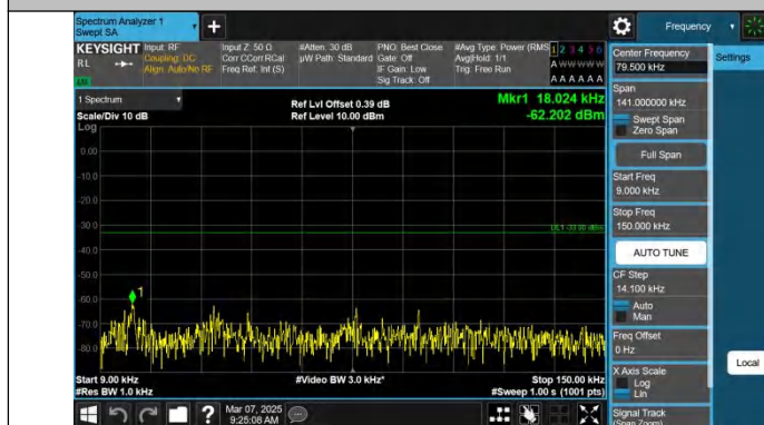
Band71-10MHz-QPSK-133172-1RB#0-0.009~0.15-PASS
