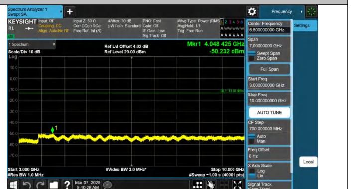
Band71-15MHz-QPSK-133197-1RB#74-3000~10000-PASS
