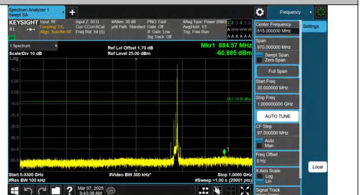
Band71-15MHz-QPSK-133297-1RB#74-30~1000-PASS
