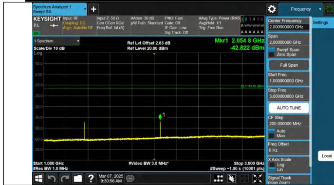
Band71-10MHz-QPSK-133297-1RB#49-1000~3000-PASS
