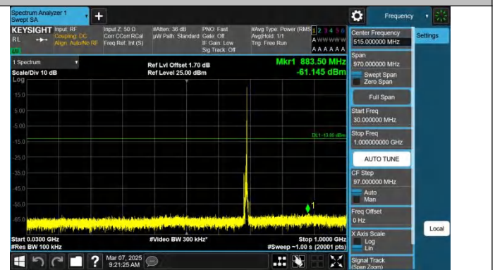
Band71-5MHz-QPSK-133447-1RB#24-30~1000-PASS
