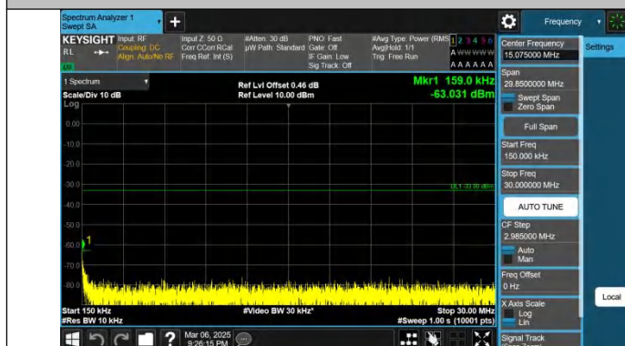
Band66-3MHz-QPSK-132322-1RB#14-0.15~30-PASS
