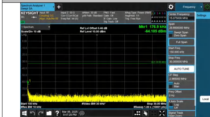
Band66-15MHz-QPSK-132597-1RB#74-0.15~30-PASS
