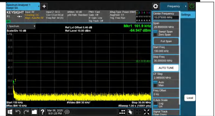
Band66-20MHz-QPSK-132322-1RB#0-0.15~30-PASS
