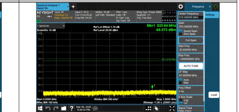
Band66-10MHz-QPSK-132322-1RB#49-30~1000-PASS
