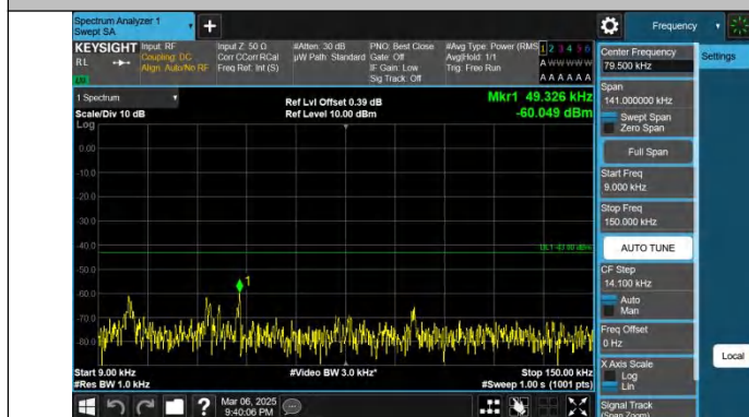
Band66-10MHz-QPSK-132622-1RB#0-0.009~0.15-PASS
