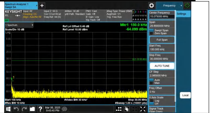
Band66-15MHz-QPSK-132047-1RB#0-0.15~30-PASS
