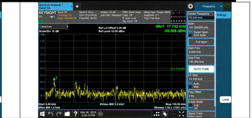
Band66-10MHz-QPSK-132322-1RB#49-0.009~0.15-PASS
