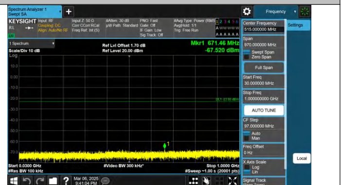
Band66-10MHz-QPSK-132622-1RB#49-30~1000-PASS
