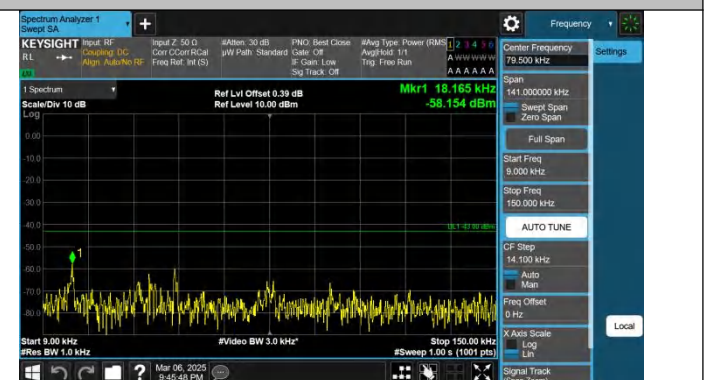
Band66-15MHz-QPSK-132322-1RB#74-0.009~0.15-PASS
