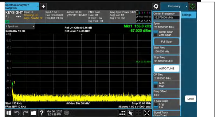
Band66-5MHz-QPSK-132647-1RB#0-0.15~30-PASS
