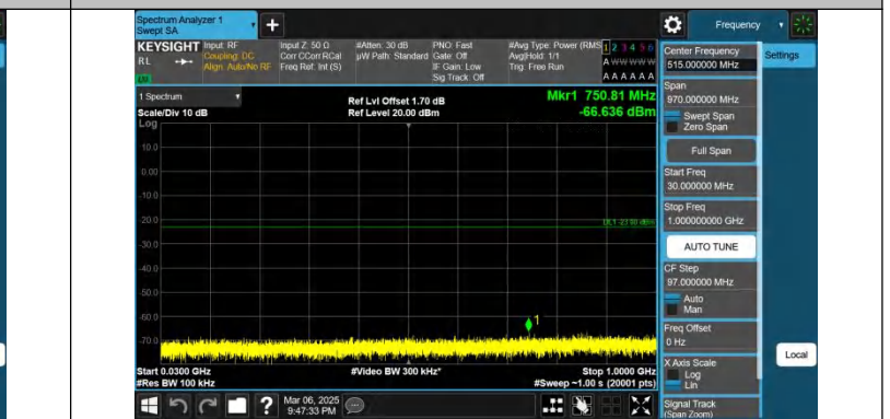
Band66-15MHz-QPSK-132597-1RB#74-30~1000-PASS
