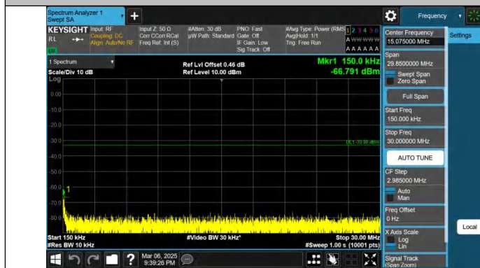
Band66-10MHz-QPSK-132322-1RB#49-0.15~30-PASS
