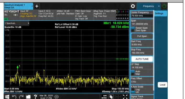
Band66-15MHz-QPSK-132047-1RB#74-0.009~0.15-PASS
