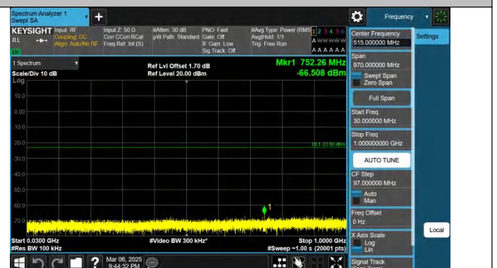
Band66-15MHz-QPSK-132047-1RB#74-30~1000-PASS
