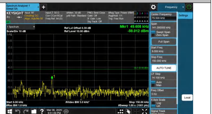
Band66-20MHz-QPSK-132322-1RB#99-0.009~0.15-PASS
