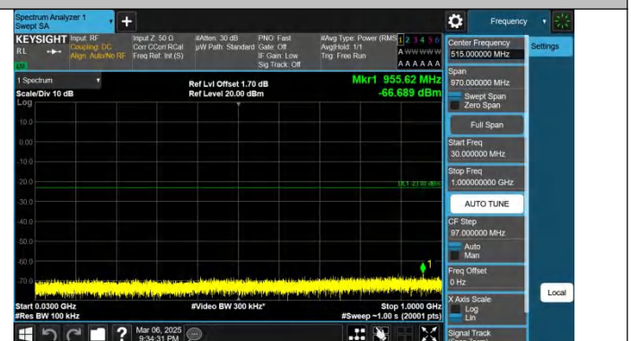
Band66-5MHz-QPSK-132647-1RB#24-30~1000-PASS
