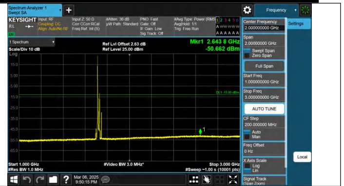
Band66-20MHz-QPSK-132072-1RB#0-1000~3000-PASS
