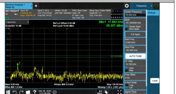
Band66-3MHz-QPSK-132657-1RB#14-0.009~0.15-PASS
