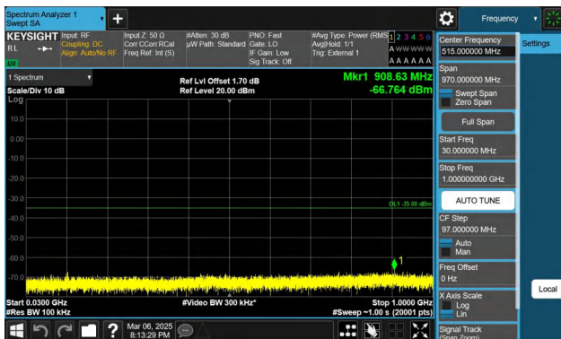
Band41-15MHz-QPSK-39725-1RB#0-30~1000-PASS
