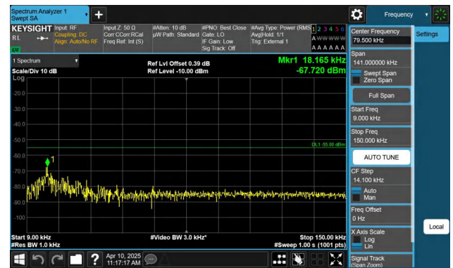
Band41-10MHz-QPSK-40620-1RB#49-0.009~0.15-PASS
