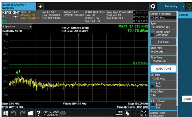
Band41-15MHz-QPSK-41515-1RB#0-0.009~0.15-PASS
