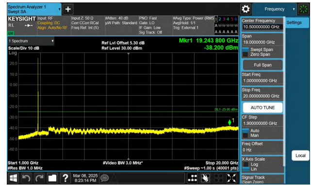
Band41-15MHz-QPSK-41515-1RB#0-1000~20000-PASS
