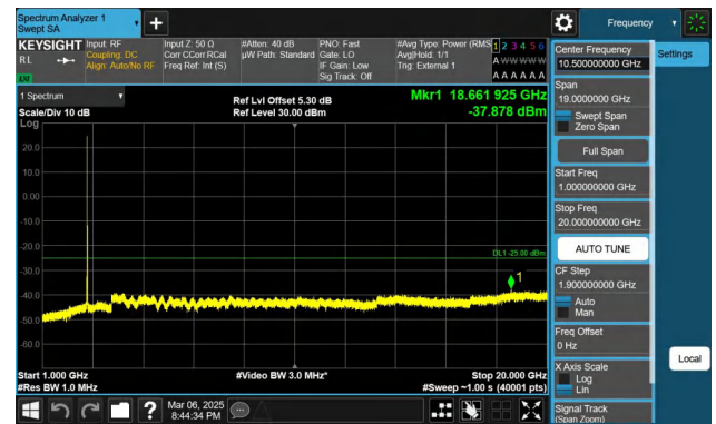
Band41-20MHz-QPSK-41490-1RB#0-1000~20000-PASS
