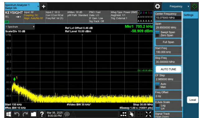
Band41-10MHz-QPSK-41540-1RB#0-0.15~30-PASS
