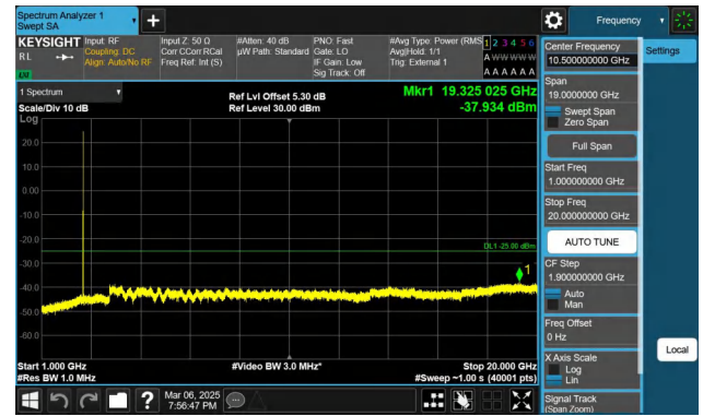
Band41-10MHz-QPSK-40620-1RB#0-1000~20000-PASS
