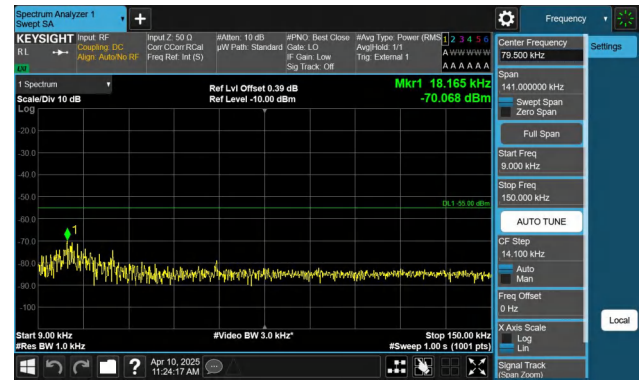
Band41-20MHz-QPSK-41490-1RB#99-0.009~0.15-PASS
