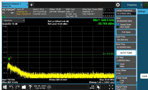
Band41-10MHz-QPSK-40620-1RB#49-0.15~30-PASS
