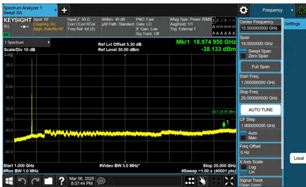
Band41-20MHz-QPSK-39750-1RB#99-1000~20000-PASS
