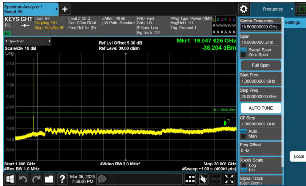
Band41-10MHz-QPSK-40620-1RB#49-1000~20000-PASS
