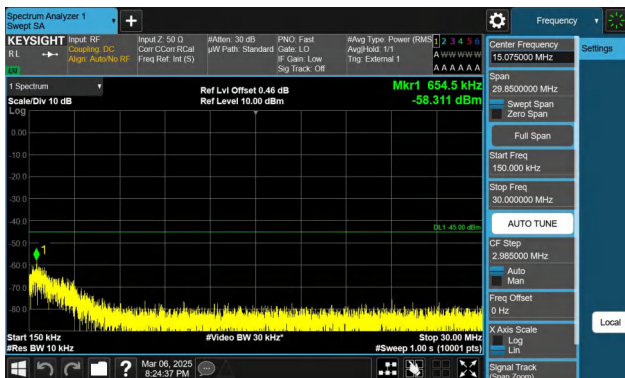
Band41-15MHz-QPSK-41515-1RB#74-0.15~30-PASS
