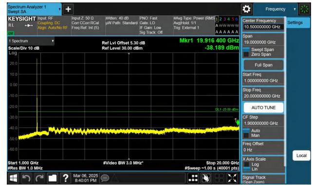
Band41-20MHz-QPSK-40620-1RB#0-1000~20000-PASS
