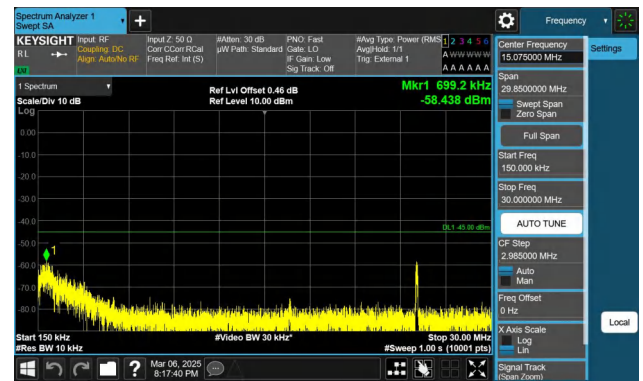
Band41-15MHz-QPSK-40620-1RB#0-0.15~30-PASS
