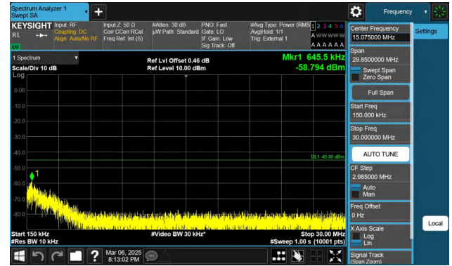
Band41-15MHz-QPSK-39725-1RB#0-0.15~30-PASS
