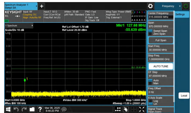
Band41-20MHz-QPSK-41490-1RB#99-30~1000-PASS
