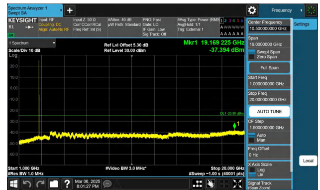
Band41-10MHz-QPSK-41540-1RB#0-1000~20000-PASS
