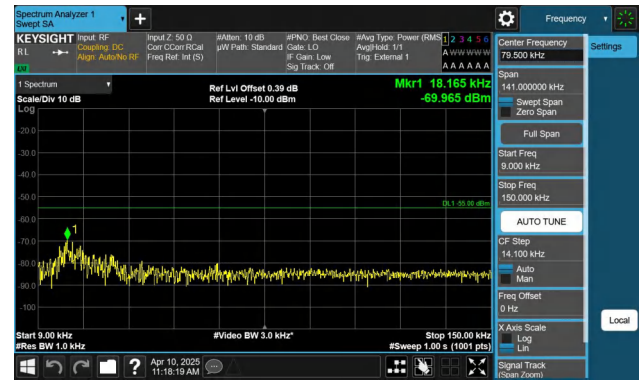
Band41-10MHz-QPSK-41540-1RB#49-0.009~0.15-PASS
