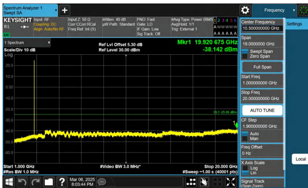
Band41-10MHz-QPSK-41540-1RB#49-1000~20000-PASS
