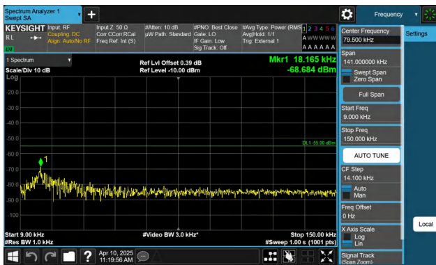
Band41-15MHz-QPSK-40620-1RB#0-0.009~0.15-PASS
