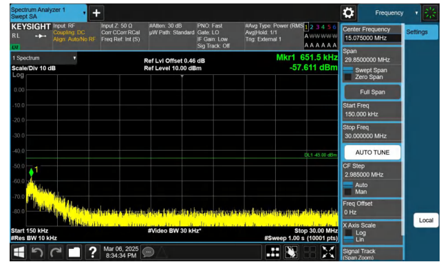
Band41-20MHz-QPSK-39750-1RB#0-0.15~30-PASS
