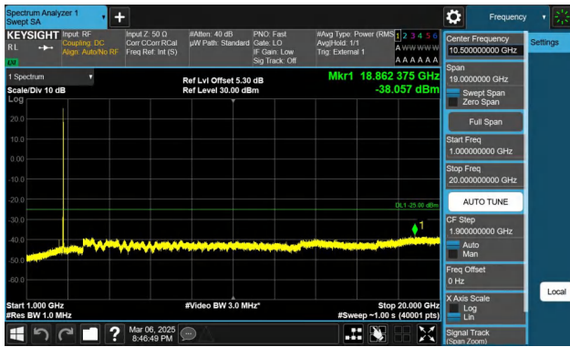
Band41-20MHz-QPSK-41490-1RB#99-1000~20000-PASS
