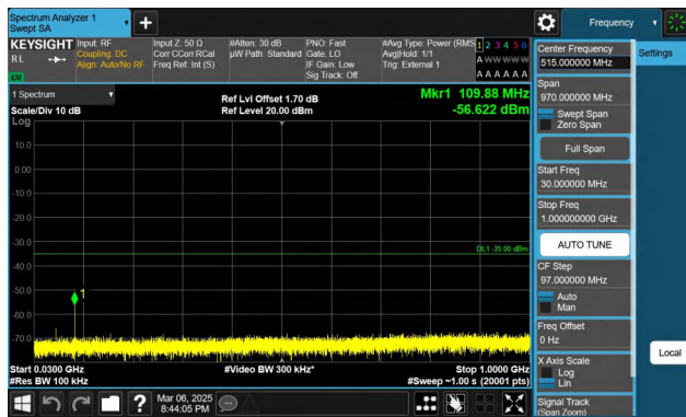
Band41-20MHz-QPSK-41490-1RB#0-30~1000-PASS
