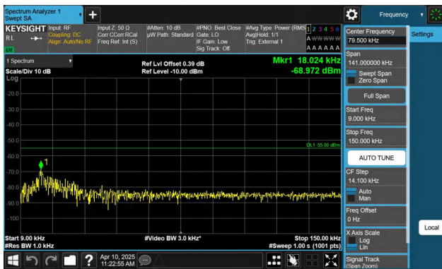
Band41-20MHz-QPSK-40620-1RB#0-0.009~0.15-PASS
