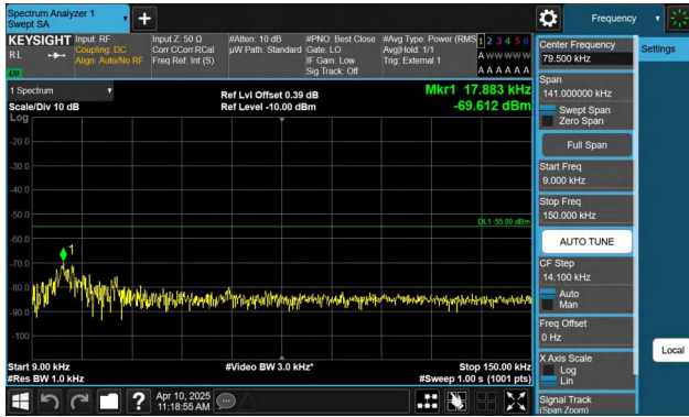
Band41-15MHz-QPSK-39725-1RB#0-0.009~0.15-PASS
