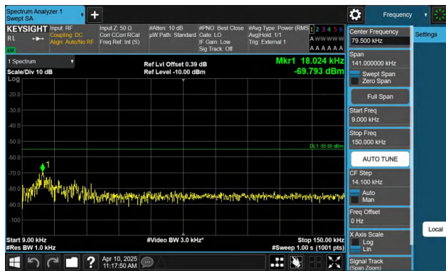
Band41-10MHz-QPSK-41540-1RB#0-0.009~0.15-PASS
