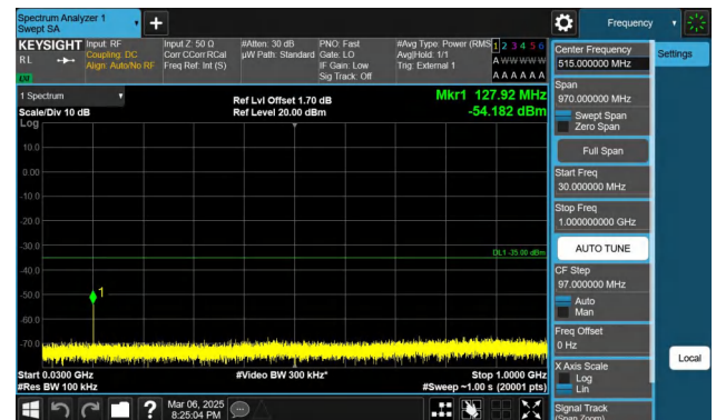
Band41-15MHz-QPSK-41515-1RB#74-30~1000-PASS
