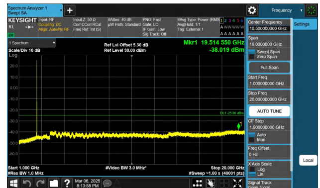
Band41-15MHz-QPSK-39725-1RB#0-1000~20000-PASS
