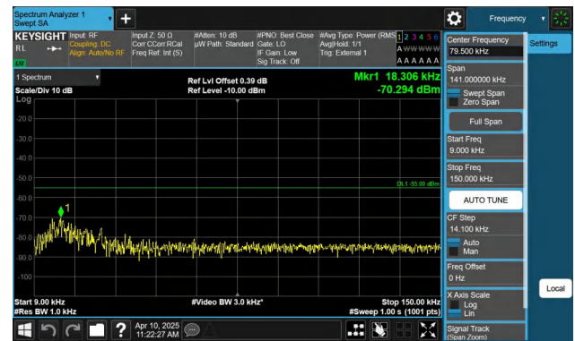
Band41-20MHz-QPSK-39750-1RB#99-0.009~0.15-PASS
