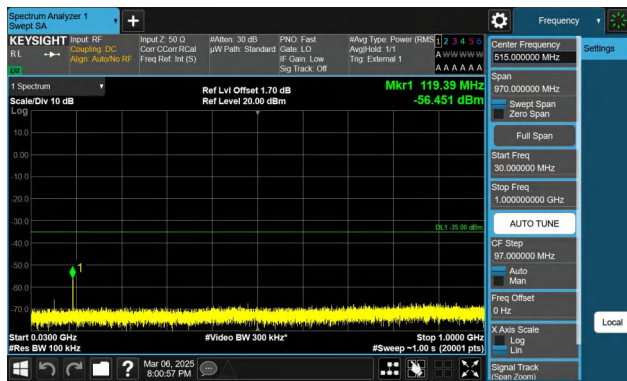
Band41-10MHz-QPSK-41540-1RB#0-30~1000-PASS
