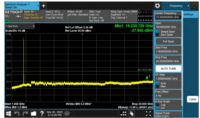
Band41-15MHz-QPSK-40620-1RB#0-1000~20000-PASS
