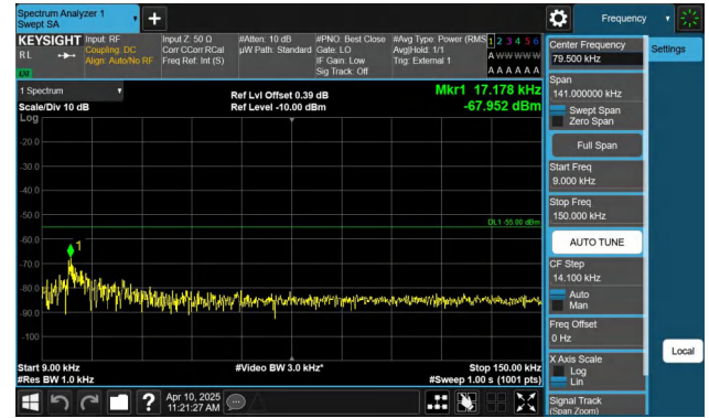
Band41-15MHz-QPSK-41515-1RB#74-0.009~0.15-PASS
