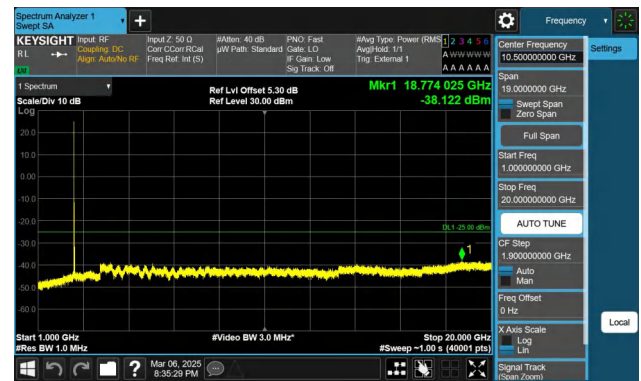
Band41-20MHz-QPSK-39750-1RB#0-1000~20000-PASS
