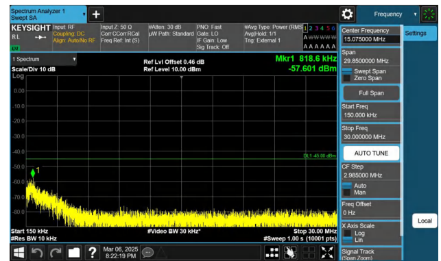
Band41-15MHz-QPSK-41515-1RB#0-0.15~30-PASS
