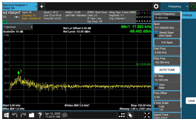
Band41-20MHz-QPSK-41490-1RB#0-0.009~0.15-PASS
