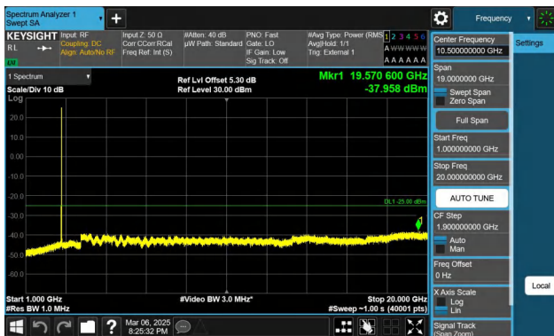
Band41-15MHz-QPSK-41515-1RB#74-1000~20000-PASS
