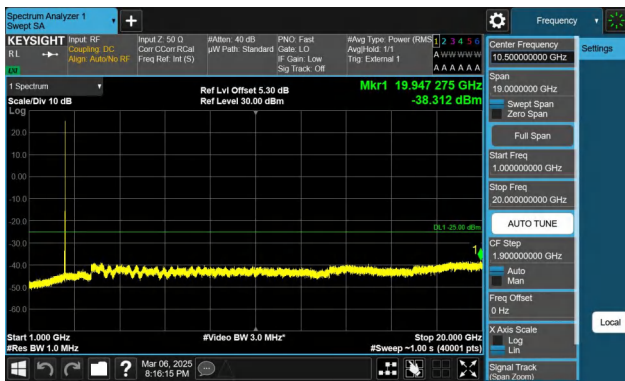
Band41-15MHz-QPSK-39725-1RB#74-1000~20000-PASS
