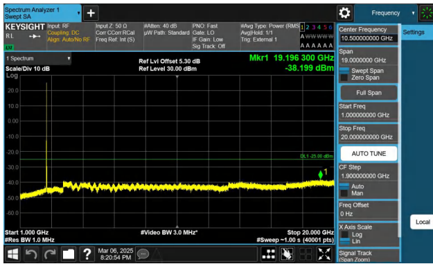
Band41-15MHz-QPSK-40620-1RB#74-1000~20000-PASS
