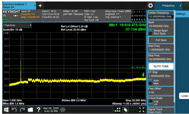
Band41-20MHz-QPSK-40620-1RB#99-1000~20000-PASS
