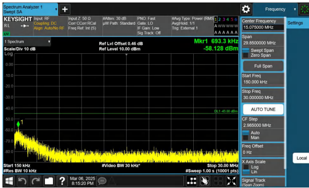
Band41-15MHz-QPSK-39725-1RB#74-0.15~30-PASS
