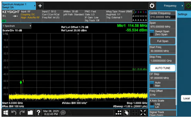
Band41-15MHz-QPSK-41515-1RB#0-30~1000-PASS
