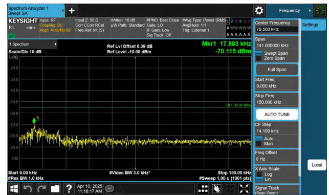
Band41-10MHz-QPSK-39700-1RB#49-0.009~0.15-PASS
