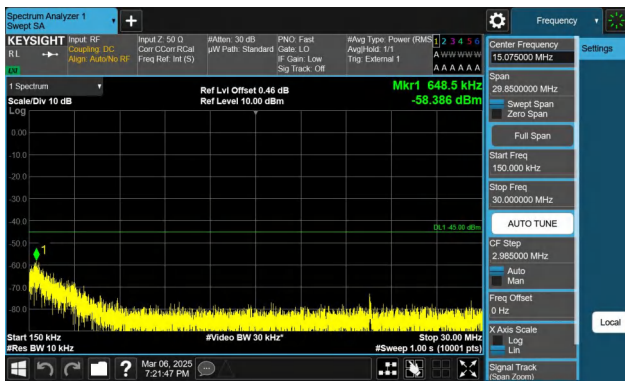
Band41-5MHz-QPSK-40620-1RB#24-0.15~30-PASS
