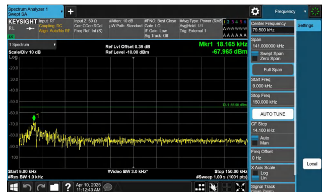
Band41-5MHz-QPSK-39675-1RB#24-0.009~0.15-PASS
