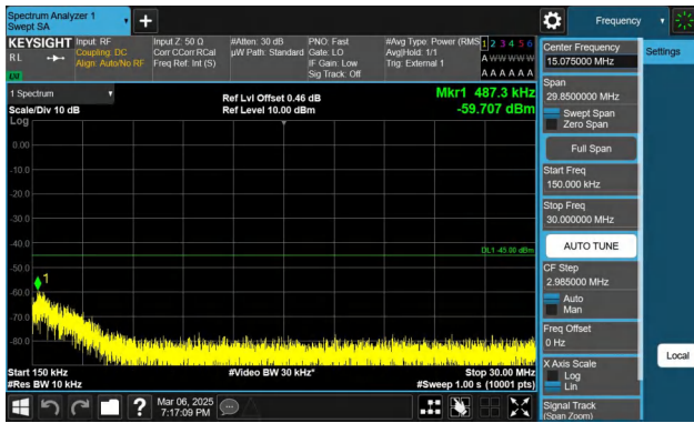
Band41-5MHz-QPSK-39675-1RB#24-0.15~30-PASS
