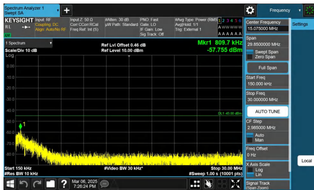
Band41-5MHz-QPSK-41565-1RB#24-0.15~30-PASS
