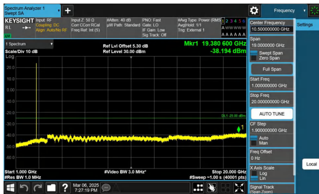
Band41-5MHz-QPSK-41565-1RB#24-1000~20000-PASS
