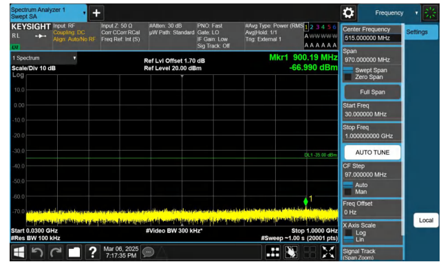
Band41-5MHz-QPSK-39675-1RB#24-30~1000-PASS
