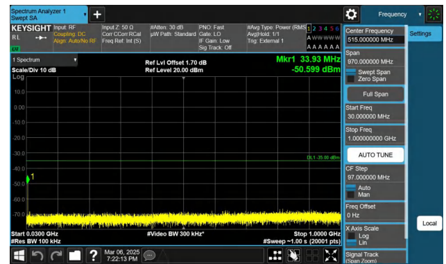
Band41-5MHz-QPSK-40620-1RB#24-30~1000-PASS
