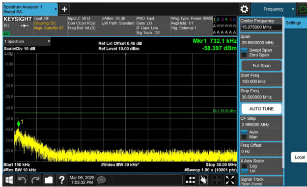
Band41-10MHz-QPSK-39700-1RB#49-0.15~30-PASS
