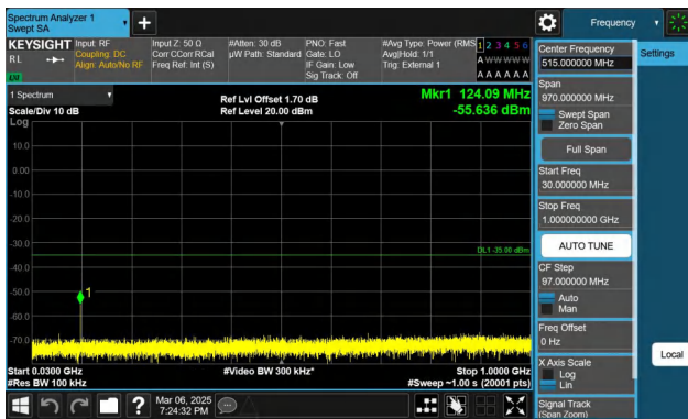
Band41-5MHz-QPSK-41565-1RB#0-30~1000-PASS
