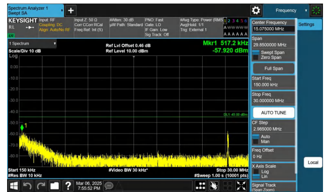
Band41-10MHz-QPSK-40620-1RB#0-0.15~30-PASS
