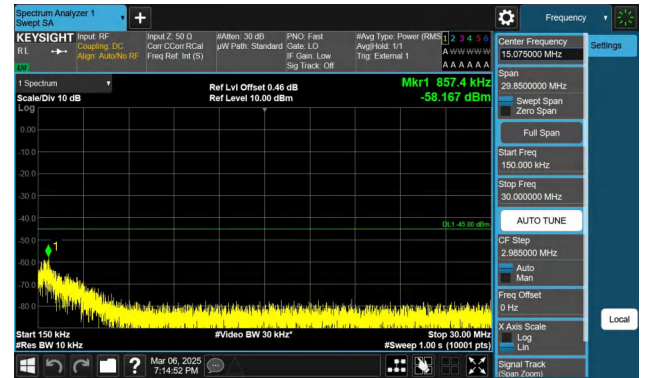
Band41-5MHz-QPSK-39675-1RB#0-0.15~30-PASS
