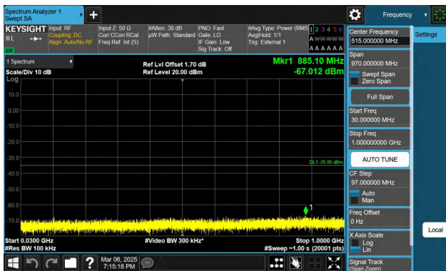
Band41-5MHz-QPSK-39675-1RB#0-30~1000-PASS
