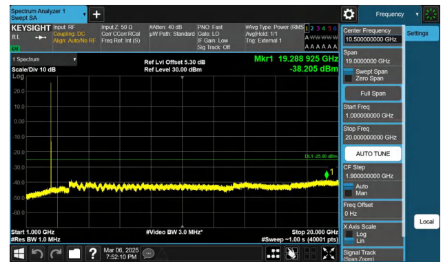
Band41-10MHz-QPSK-39700-1RB#0-1000~20000-PASS
