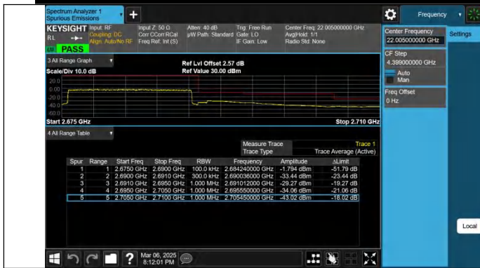
Band41-15MHz-QPSK-41515-75RB#0-PASS
