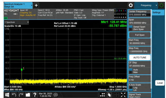
Band41-5MHz-QPSK-41565-1RB#24-30~1000-PASS
