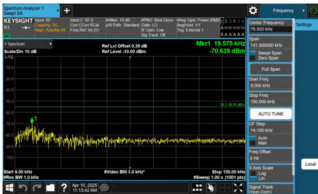
Band41-5MHz-QPSK-40620-1RB#0-0.009~0.15-PASS
