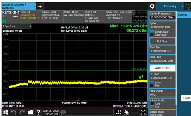
Band41-10MHz-QPSK-39700-1RB#49-1000~20000-PASS
