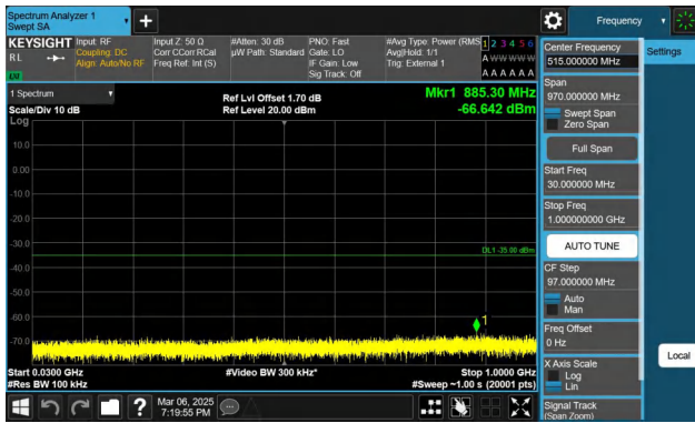
Band41-5MHz-QPSK-40620-1RB#0-30~1000-PASS
