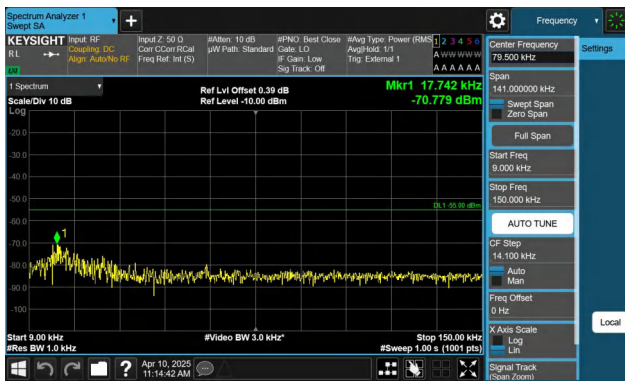
Band41-5MHz-QPSK-41565-1RB#0-0.009~0.15-PASS
