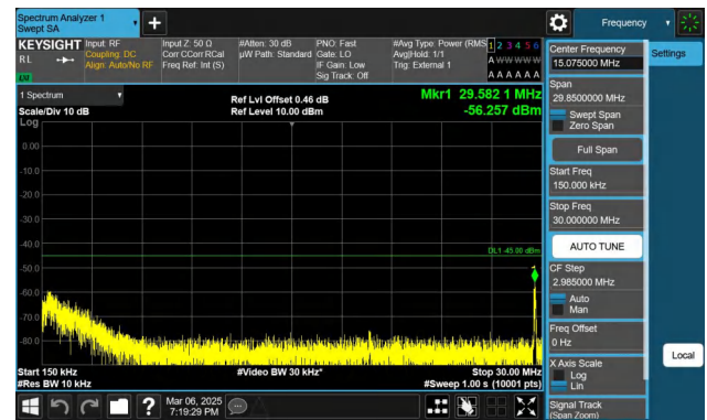
Band41-5MHz-QPSK-40620-1RB#0-0.15~30-PASS
