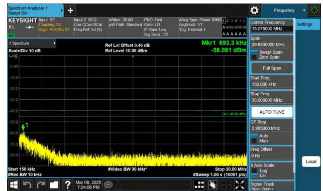
Band41-5MHz-QPSK-41565-1RB#0-0.15~30-PASS
