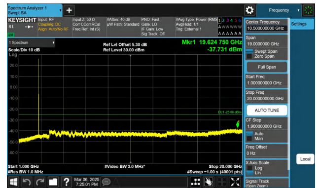
Band41-5MHz-QPSK-41565-1RB#0-1000~20000-PASS
