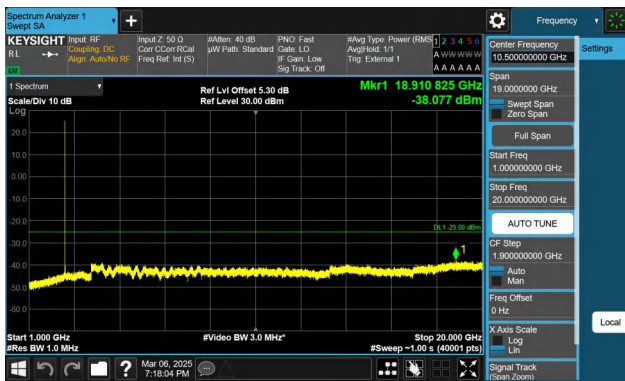
Band41-5MHz-QPSK-39675-1RB#24-1000~20000-PASS
