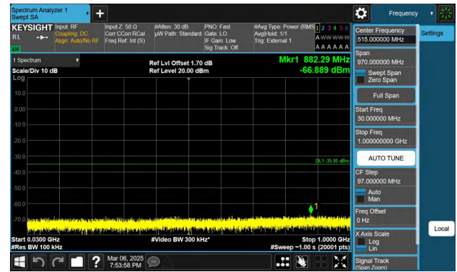
Band41-10MHz-QPSK-39700-1RB#49-30~1000-PASS
