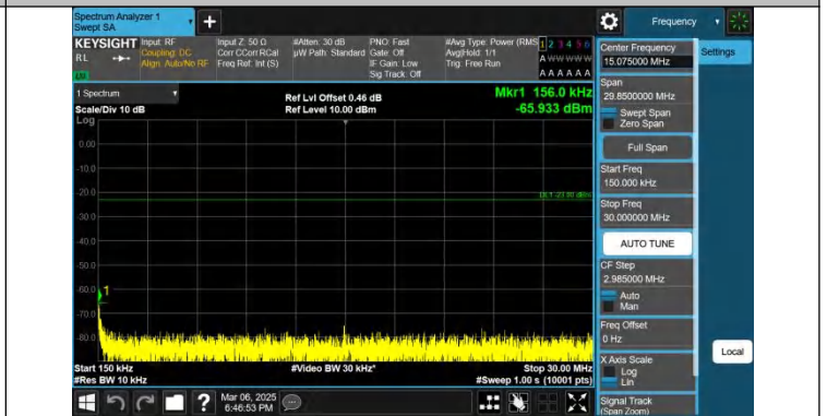
Band26(824-849)-5MHz-QPSK-26815-1RB#0-0.15~30-PASS
