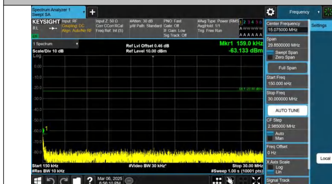
Band26(824-849)-10MHz-QPSK-26915-1RB#49-0.15~30-PASS
