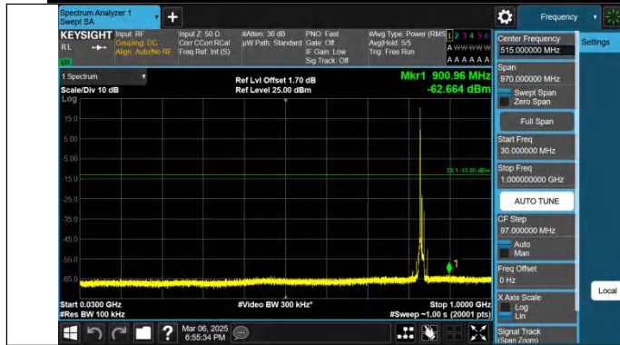
Band26(824-849)-10MHz-QPSK-26915-1RB#0-30~1000-PASS
