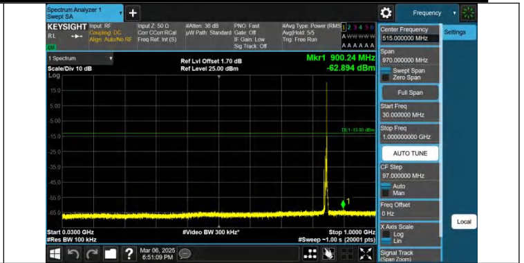
Band26(824-849)-5MHz-QPSK-27015-1RB#24-30~1000-PASS
