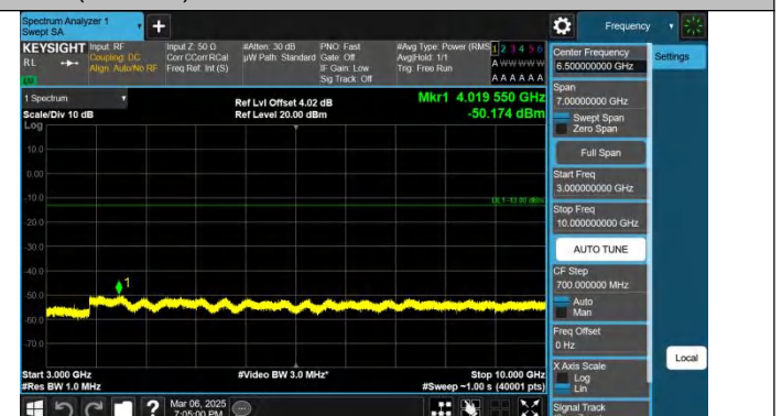
Band26(824-849)-15MHz-QPSK-26965-1RB#74-3000~10000-PASS
