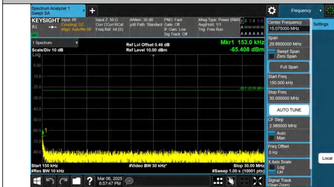
Band26(824-849)-10MHz-QPSK-26990-1RB#49-0.15~30-PASS
