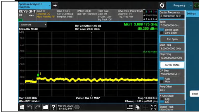
Band26(824-849)-3MHz-QPSK-27025-1RB#0-3000~10000-PASS
