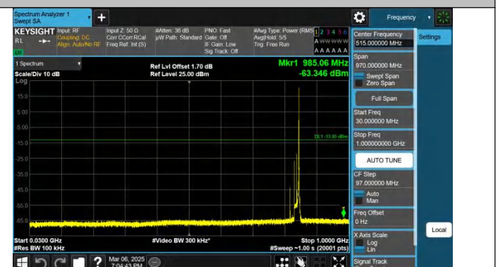
Band26(824-849)-15MHz-QPSK-26965-1RB#74-30~1000-PASS
