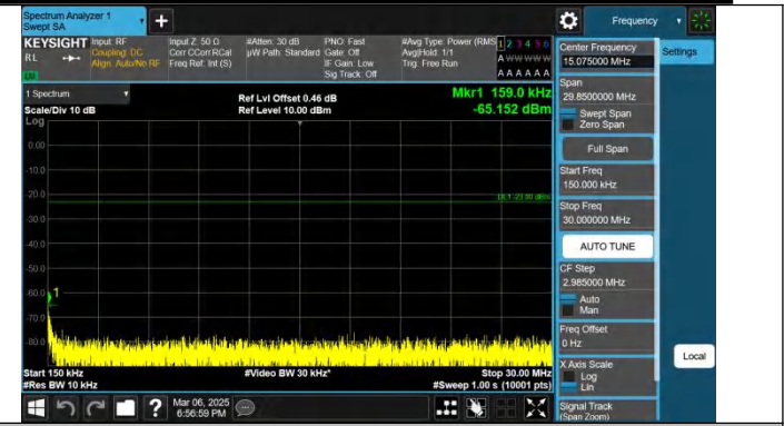
Band26(824-849)-10MHz-QPSK-26990-1RB#0-0.15~30-PASS
