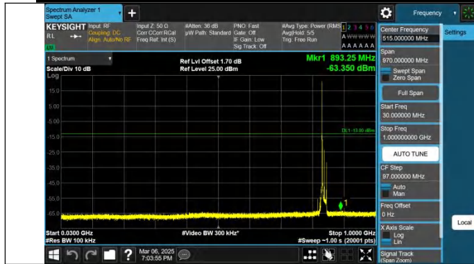
Band26(824-849)-15MHz-QPSK-26965-1RB#0-30~1000-PASS
