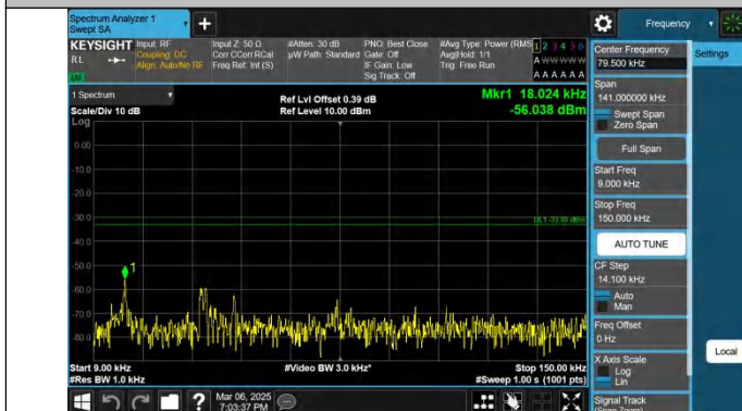
Band26(824-849)-15MHz-QPSK-26965-1RB#0-0.009~0.15-PASS
