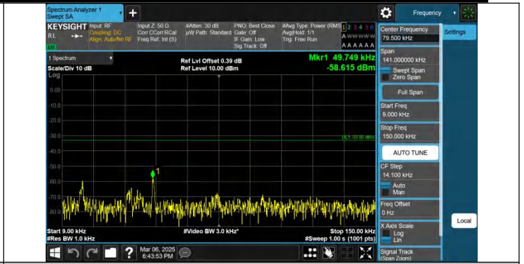
Band26(824-849)-3MHz-QPSK-27025-1RB#14-0.009~0.15-PASS
