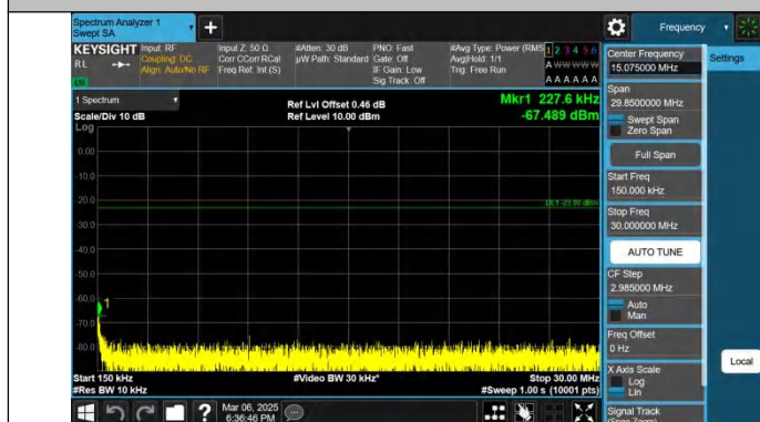
Band26(824-849)-1.4MHz-QPSK-27033-1RB#5-0.15~30-PASS
