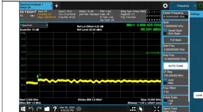
Band26(824-849)-10MHz-QPSK-26915-1RB#0-3000~10000-PASS
