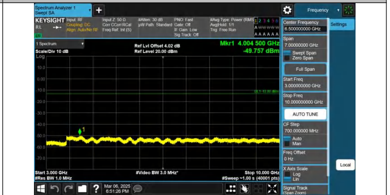
Band26(824-849)-5MHz-QPSK-27015-1RB#24-3000~10000-PASS
