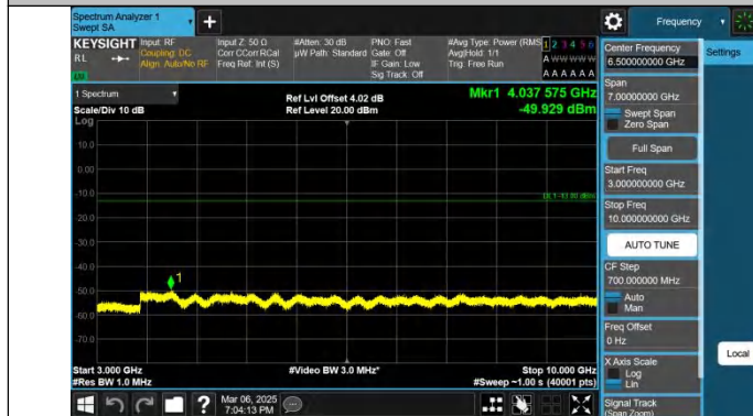
Band26(824-849)-15MHz-QPSK-26965-1RB#0-3000~10000-PASS
