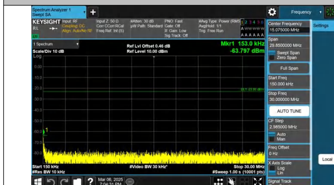
Band26(824-849)-15MHz-QPSK-26965-1RB#74-0.15~30-PASS
