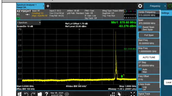
Band26(824-849)-10MHz-QPSK-26840-1RB#0-30~1000-PASS
