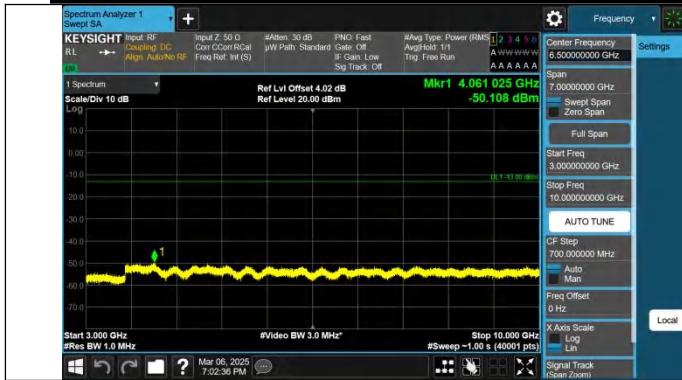
Band26(824-849)-15MHz-QPSK-26915-1RB#0-3000~10000-PAS S
