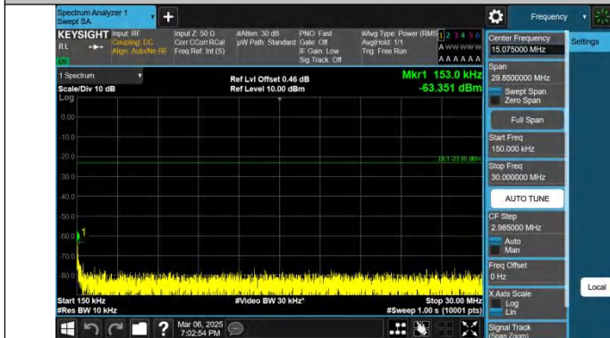
Band26(824-849)-15MHz-QPSK-26915-1RB#74-0.15~30-PASS
