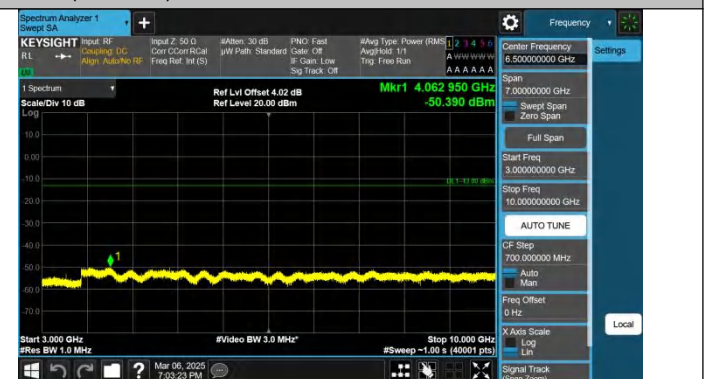
Band26(824-849)-15MHz-QPSK-26915-1RB#74-3000~10000-PAS S
