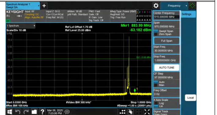
Band26(824-849)-15MHz-QPSK-26915-1RB#74-30~1000-PASS
