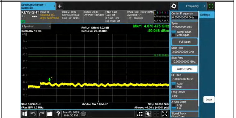
Band26(824-849)-3MHz-QPSK-27025-1RB#14-3000~10000-PASS
