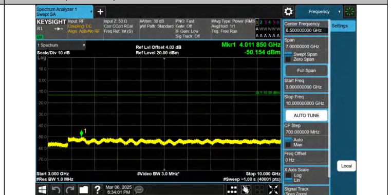
Band26(824-849)-1.4MHz-QPSK-26797-1RB#5-3000~10000-PASS
