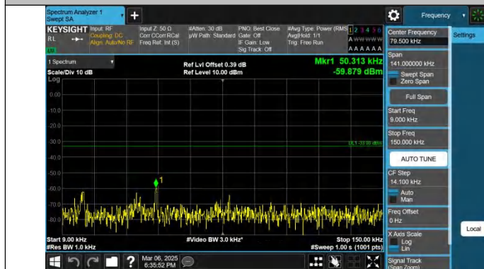
Band26(824-849)-1.4MHz-QPSK-27033-1RB#0-0.009~0.15-PASS
