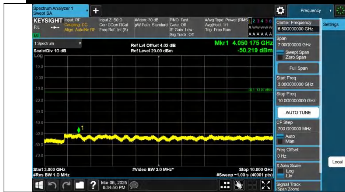
Band26(824-849)-1.4MHz-QPSK-26915-1RB#0-3000~10000-PASS
