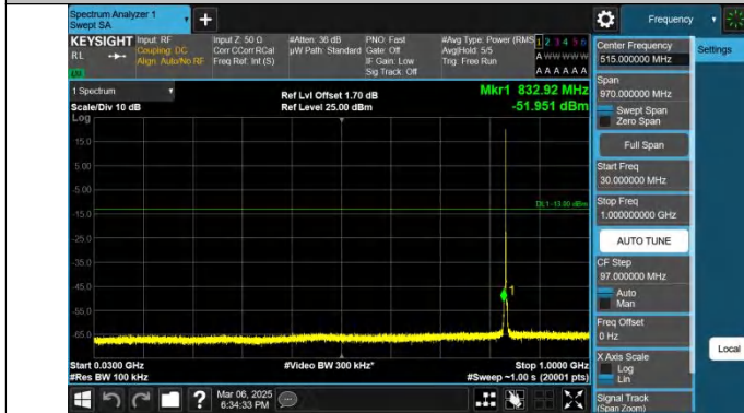
Band26(824-849)-1.4MHz-QPSK-26915-1RB#0-30~1000-PASS
