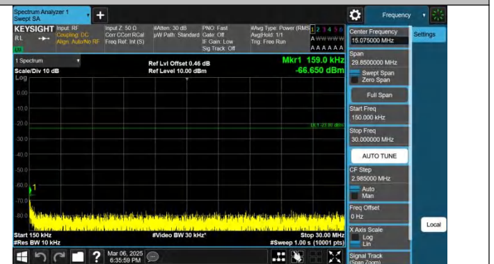
Band26(824-849)-1.4MHz-QPSK-27033-1RB#0-0.15~30-PASS
