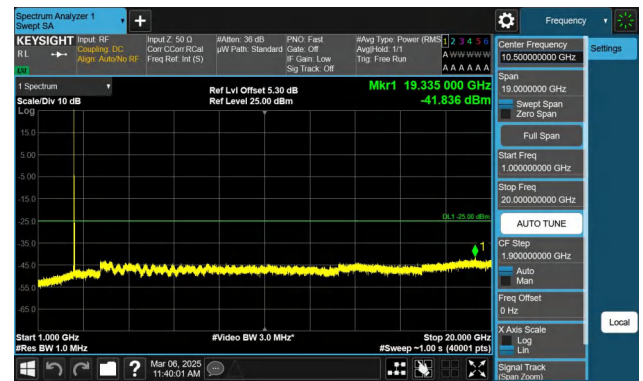
Band7-15MHz-QPSK-20825-1RB#0-1000~20000-PASS
