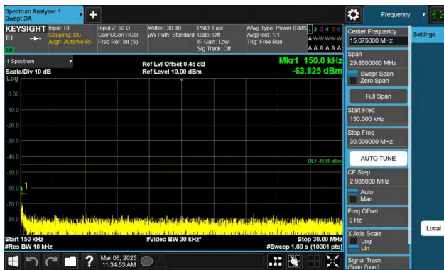
Band7-10MHz-QPSK-21100-1RB#49-0.15~30-PASS
