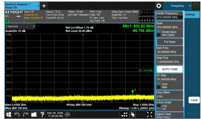
Band7-20MHz-QPSK-20850-1RB#99-30~1000-PASS
