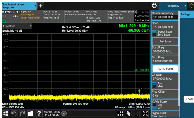
Band7-15MHz-QPSK-21100-1RB#0-30~1000-PASS
