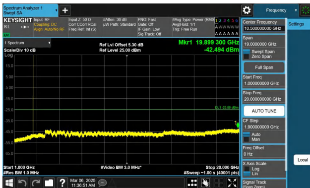
Band7-10MHz-QPSK-21400-1RB#49-1000~20000-PASS
