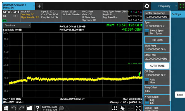
Band7-20MHz-QPSK-21100-1RB#99-1000~20000-PASS
