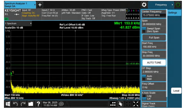
Band7-20MHz-QPSK-20850-1RB#0-0.15~30-PASS
