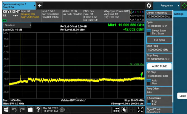
Band7-15MHz-QPSK-21100-1RB#74-1000~20000-PASS
