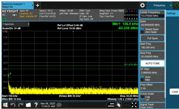
Band7-20MHz-QPSK-20850-1RB#99-0.15~30-PASS
