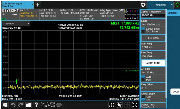
Band7-20MHz-QPSK-20850-1RB#0-0.009~0.15-PASS
