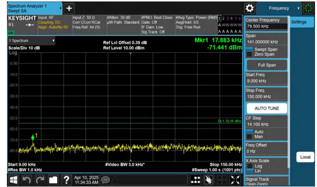
Band7-15MHz-QPSK-21375-1RB#74-0.009~0.15-PASS
