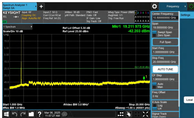
Band7-20MHz-QPSK-21350-1RB#99-1000~20000-PASS
