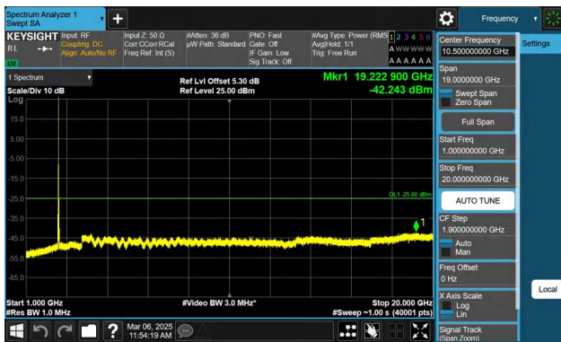
Band7-20MHz-QPSK-20850-1RB#99-1000~20000-PASS
