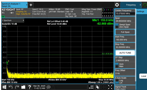
Band7-15MHz-QPSK-21100-1RB#74-0.15~30-PASS
