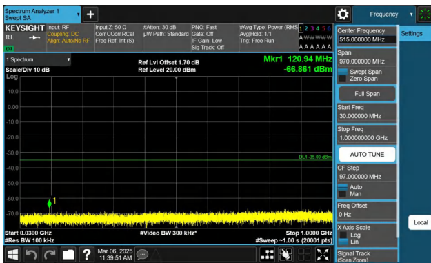
Band7-15MHz-QPSK-20825-1RB#0-30~1000-PASS
