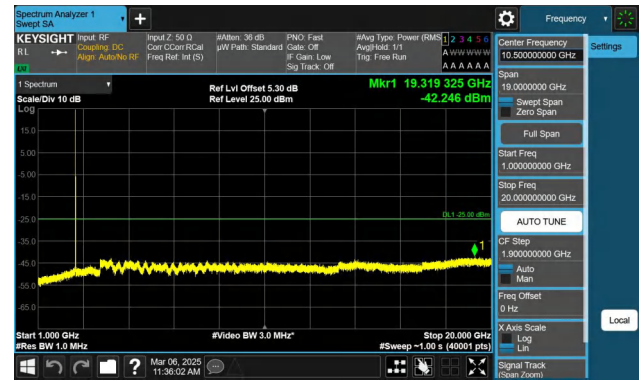
Band7-10MHz-QPSK-21400-1RB#0-1000~20000-PASS
