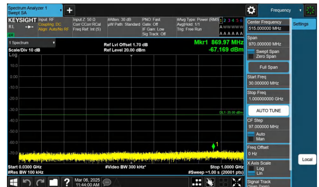
Band7-15MHz-QPSK-21375-1RB#74-30~1000-PASS
