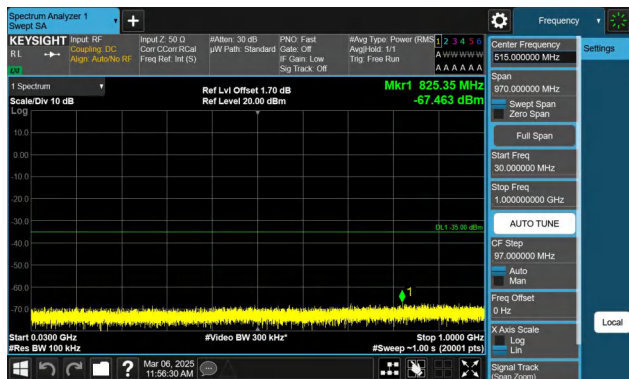
Band7-20MHz-QPSK-21350-1RB#0-30~1000-PASS
