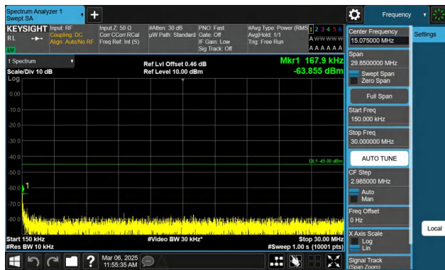
Band7-20MHz-QPSK-21100-1RB#99-0.15~30-PASS
