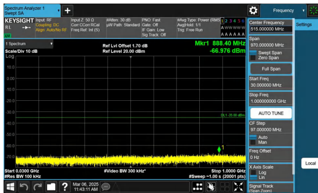
Band7-15MHz-QPSK-21375-1RB#0-30~1000-PASS
