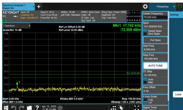
Band7-20MHz-QPSK-21350-1RB#0-0.009~0.15-PASS
