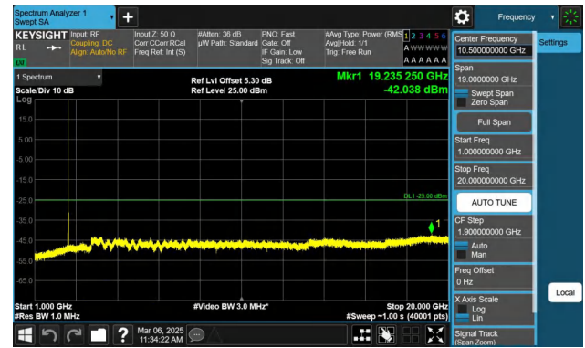
Band7-10MHz-QPSK-21100-1RB#0-1000~20000-PASS
