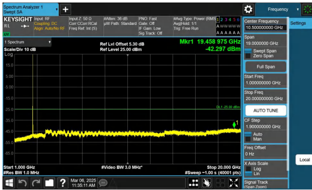
Band7-10MHz-QPSK-21100-1RB#49-1000~20000-PASS
