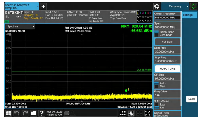
Band7-20MHz-QPSK-21100-1RB#99-30~1000-PASS
