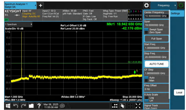
Band7-20MHz-QPSK-21100-1RB#0-1000~20000-PASS
