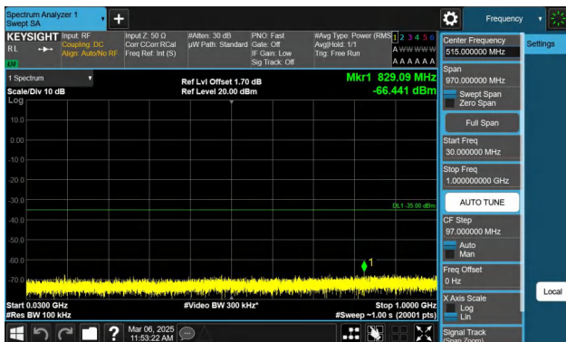
Band7-20MHz-QPSK-20850-1RB#0-30~1000-PASS
