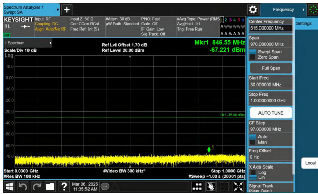
Band7-10MHz-QPSK-21400-1RB#0-30~1000-PASS
