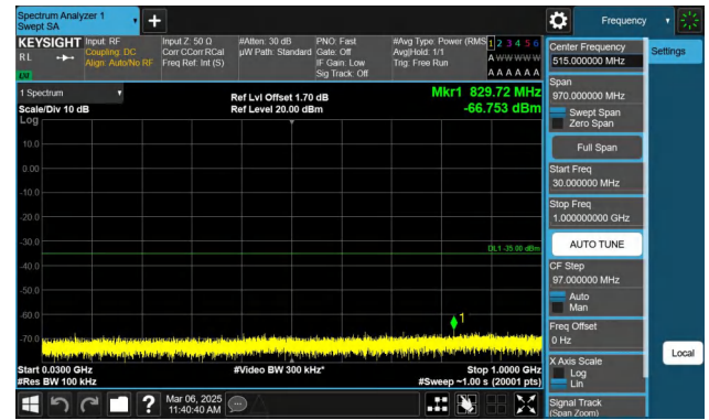
Band7-15MHz-QPSK-20825-1RB#74-30~1000-PASS
