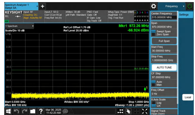
Band7-15MHz-QPSK-21100-1RB#74-30~1000-PASS
