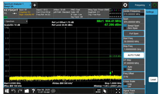
Band7-20MHz-QPSK-21350-1RB#99-30~1000-PASS
