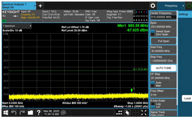
Band7-10MHz-QPSK-21100-1RB#0-30~1000-PASS
