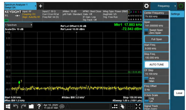
Band7-15MHz-QPSK-21100-1RB#74-0.009~0.15-PASS
