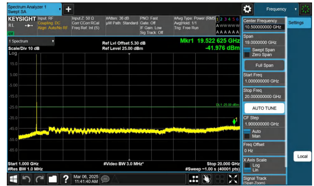
Band7-15MHz-QPSK-21100-1RB#0-1000~20000-PASS
