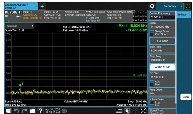
Band7-20MHz-QPSK-20850-1RB#99-0.009~0.15-PASS
