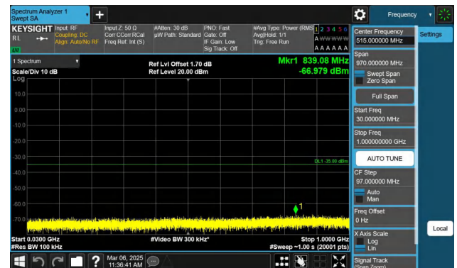
Band7-10MHz-QPSK-21400-1RB#49-30~1000-PASS
