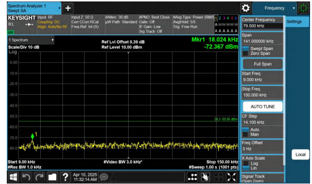
Band7-10MHz-QPSK-21400-1RB#49-0.009~0.15-PASS
