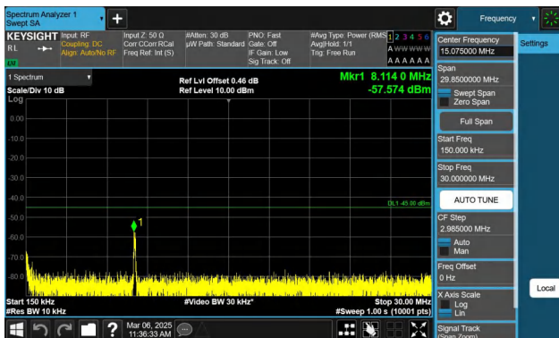
Band7-10MHz-QPSK-21400-1RB#49-0.15~30-PASS
