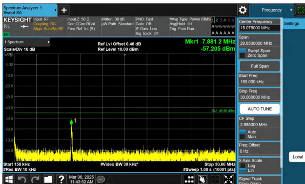
Band7-15MHz-QPSK-21375-1RB#74-0.15~30-PASS
