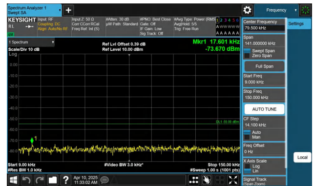
Band7-15MHz-QPSK-20825-1RB#74-0.009~0.15-PASS
