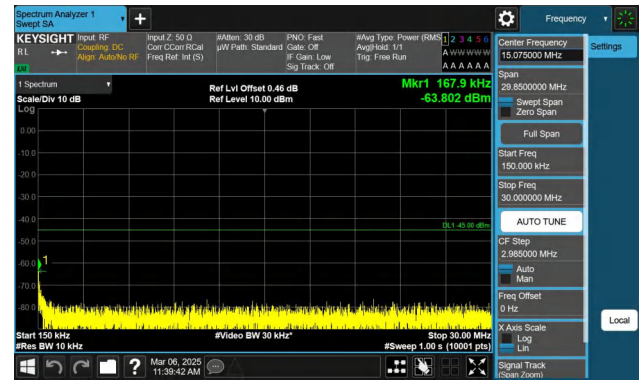
Band7-15MHz-QPSK-20825-1RB#0-0.15~30-PASS
