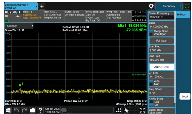
Band7-20MHz-QPSK-21100-1RB#99-0.009~0.15-PASS
