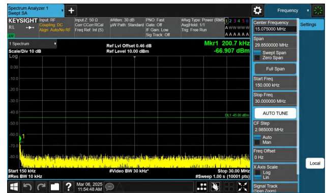
Band7-20MHz-QPSK-21100-1RB#0-0.15~30-PASS
