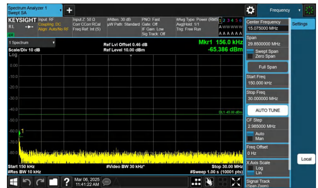
Band7-15MHz-QPSK-21100-1RB#0-0.15~30-PASS
