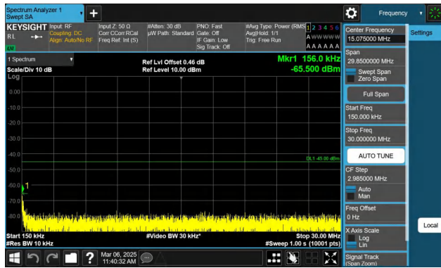
Band7-15MHz-QPSK-20825-1RB#74-0.15~30-PASS
