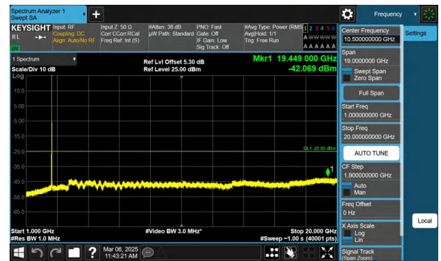
Band7-15MHz-QPSK-21375-1RB#0-1000~20000-PASS
