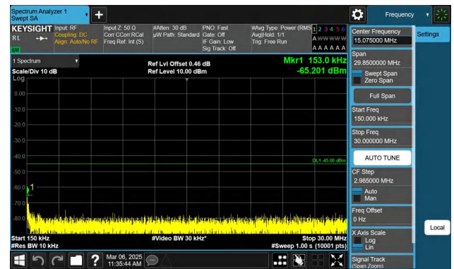
Band7-10MHz-QPSK-21400-1RB#0-0.15~30-PASS
