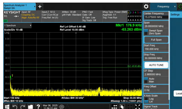
Band7-20MHz-QPSK-21350-1RB#0-0.15~30-PASS
