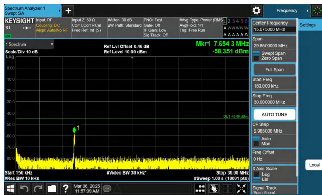
Band7-20MHz-QPSK-21350-1RB#99-0.15~30-PASS
