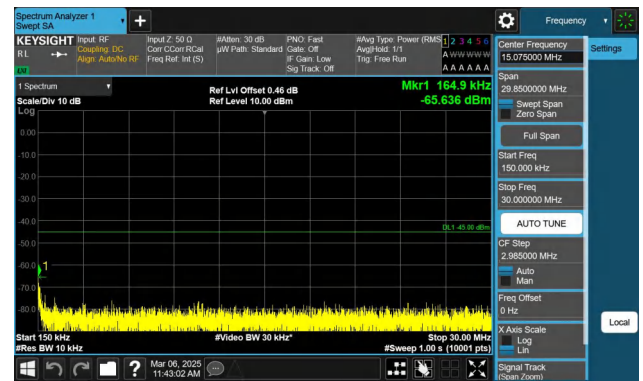
Band7-15MHz-QPSK-21375-1RB#0-0.15~30-PASS
