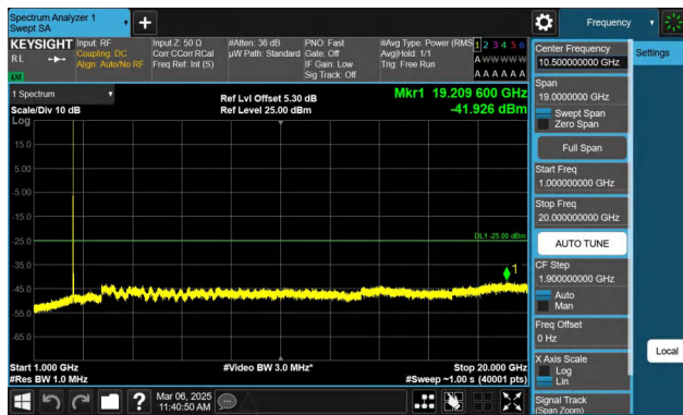
Band7-15MHz-QPSK-20825-1RB#74-1000~20000-PASS
