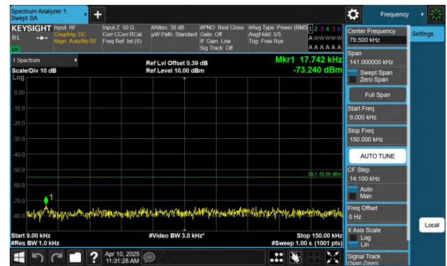
Band7-10MHz-QPSK-21100-1RB#49-0.009~0.15-PASS
