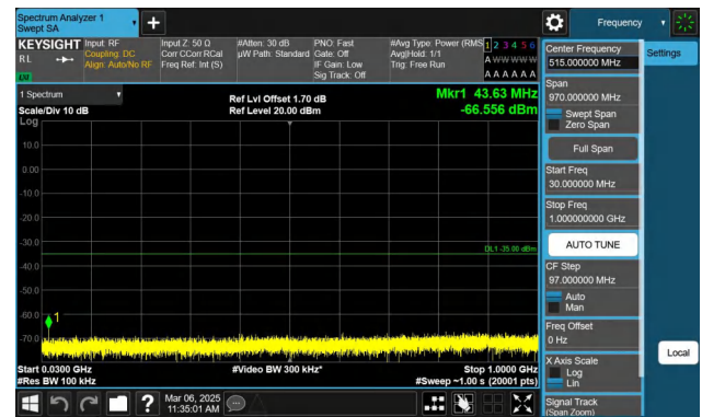
Band7-10MHz-QPSK-21100-1RB#49-30~1000-PASS
