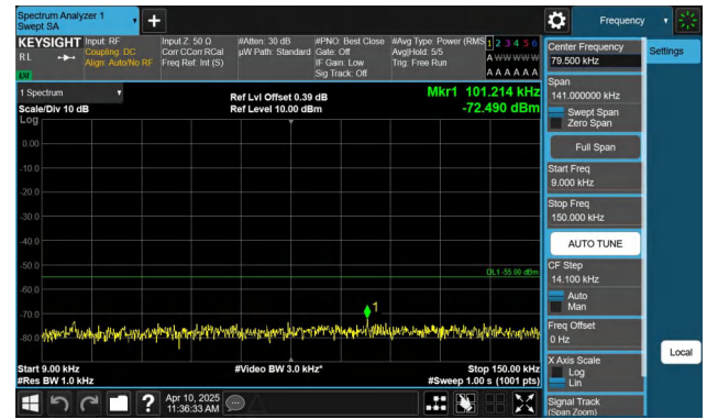
Band7-20MHz-QPSK-21350-1RB#99-0.009~0.15-PASS
