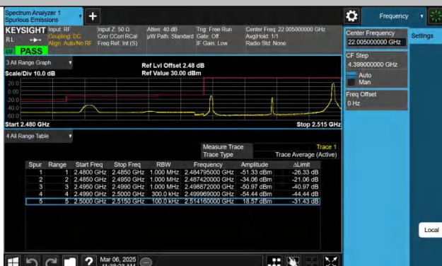
Band7-15MHz-QPSK-20825-1RB#74-PASS
