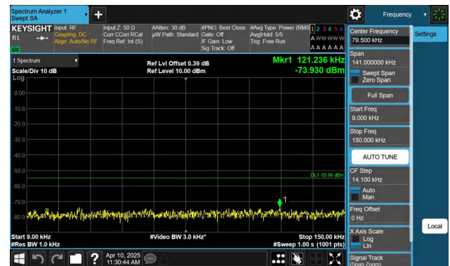
Band7-10MHz-QPSK-20800-1RB#49-0.009~0.15-PASS
