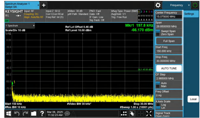
Band7-10MHz-QPSK-20800-1RB#0-0.15~30-PASS
