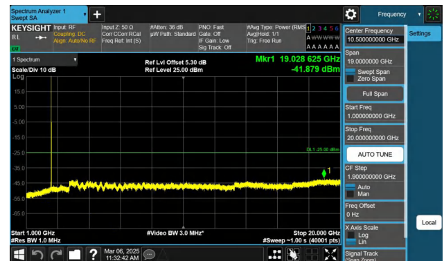
Band7-10MHz-QPSK-20800-1RB#0-1000~20000-PASS
