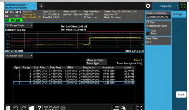
Band7-15MHz-QPSK-20825-75RB#0-PASS
