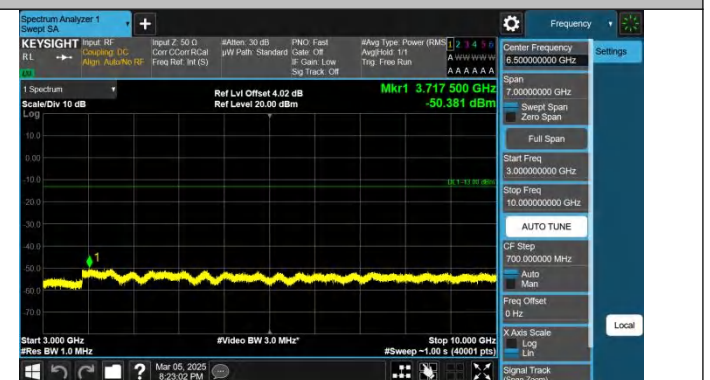
Band5-5MHz-QPSK-20425-1RB#24-3000~10000-PASS
