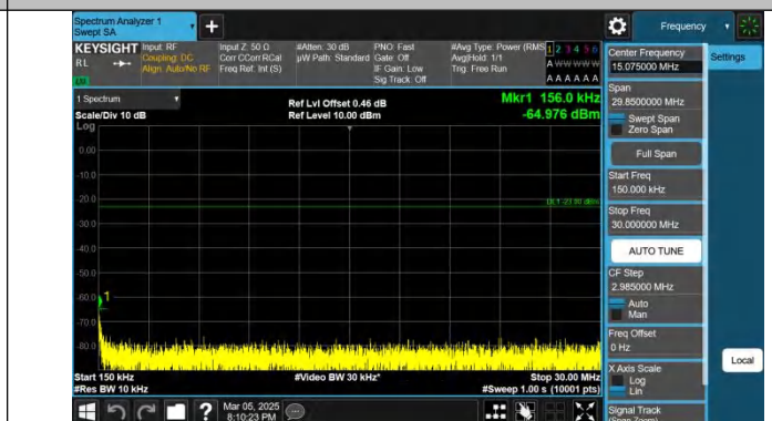
Band5-1.4MHz-QPSK-20643-1RB#0-0.15~30-PASS
