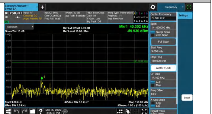
Band5-5MHz-QPSK-20625-1RB#24-0.009~0.15-PASS
