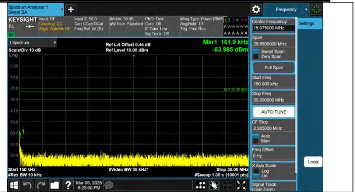
Band5-5MHz-QPSK-20625-1RB#0-0.15~30-PASS
