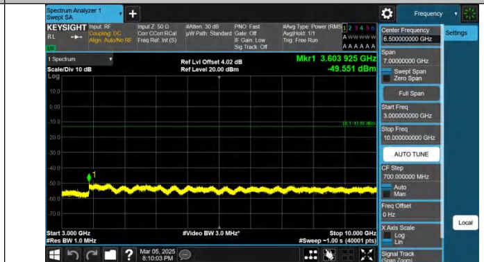
Band5-1.4MHz-QPSK-20525-1RB#5-3000~10000-PASS
