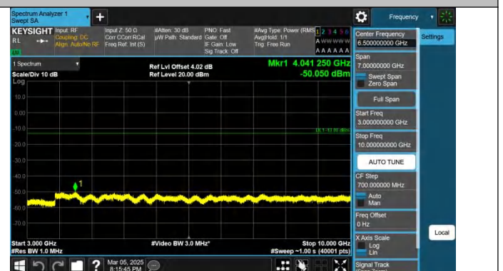
Band5-3MHz-QPSK-20415-1RB#14-3000~10000-PASS
