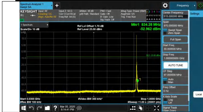
Band5-3MHz-QPSK-20415-1RB#0-30~1000-PASS
