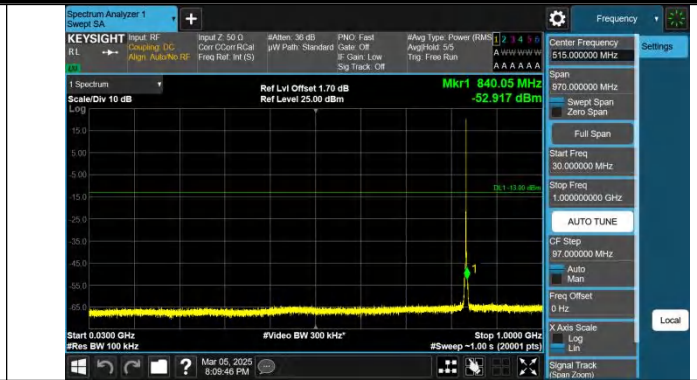
Band5-1.4MHz-QPSK-20525-1RB#5-30~1000-PASS
