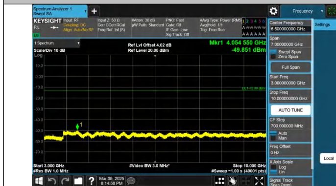
Band5-3MHz-QPSK-20415-1RB#0-3000~10000-PASS
