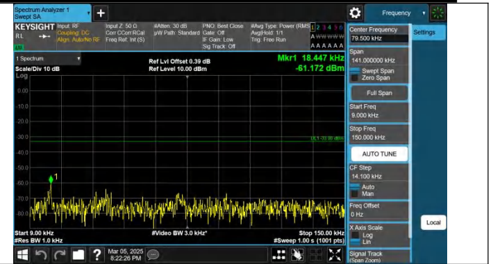
Band5-5MHz-QPSK-20425-1RB#24-0.009~0.15-PASS
