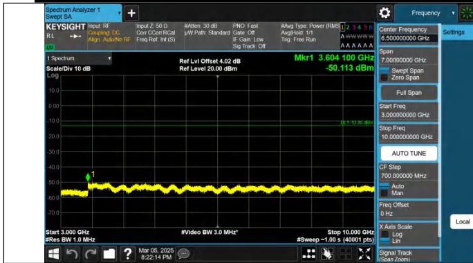
Band5-5MHz-QPSK-20425-1RB#0-3000~10000-PASS
