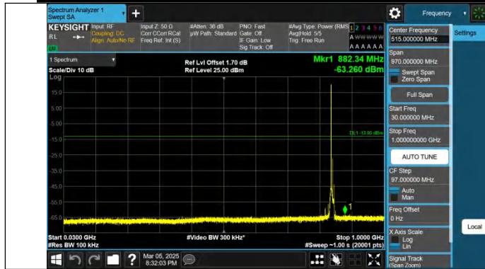
Band5-10MHz-QPSK-20600-1RB#0-30~1000-PASS
