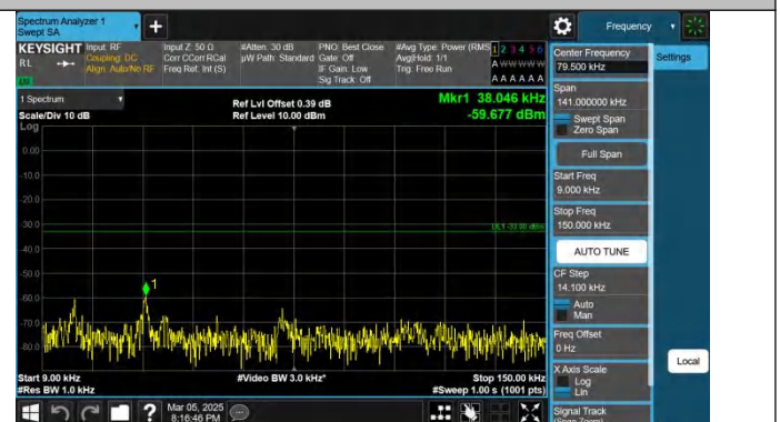
Band5-3MHz-QPSK-20525-1RB#14-0.009~0.15-PASS
