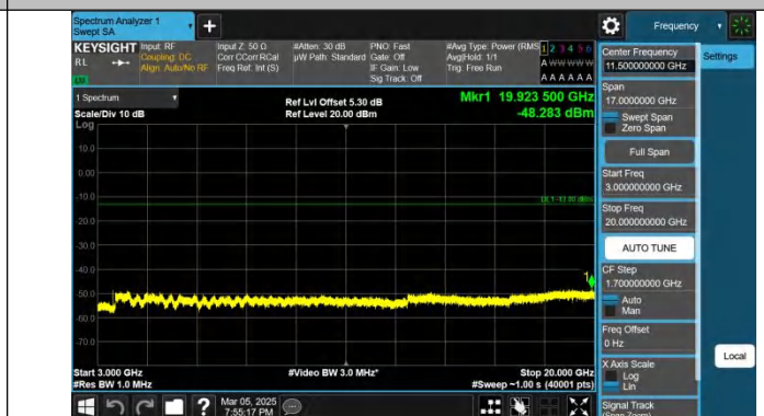
Band4-15MHz-QPSK-20325-1RB#74.3000~20000-PASS
