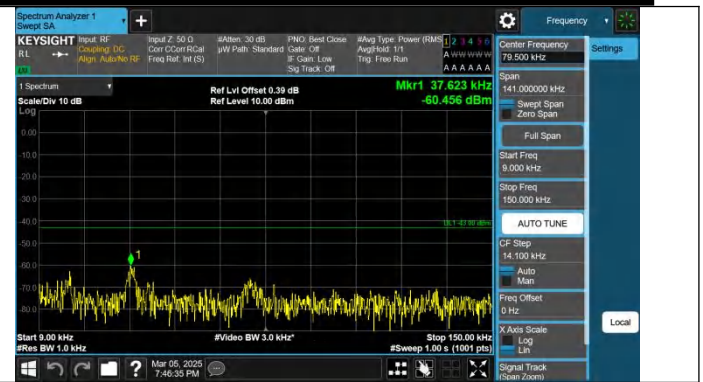
Band4-10MHz-QPSK-20175-1RB#49.0.009~0.15-PASS
