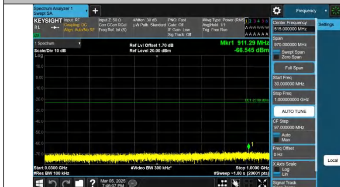
Band4-10MHz-QPSK-20175-1RB#0-30~1000-PASS
