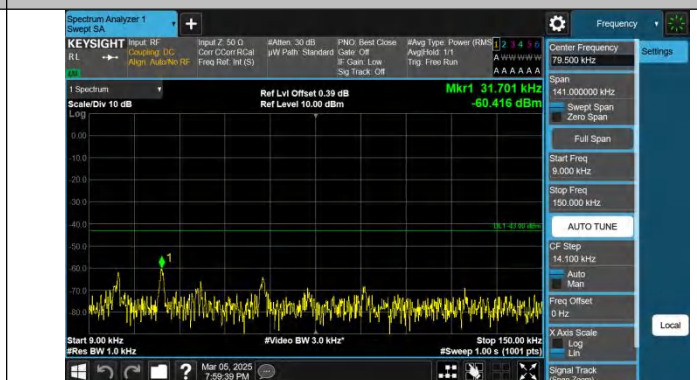
Band4-20MHz-QPSK-20175-1RB#99-0.009~0.15-PASS
