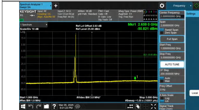
Band4-20MHz-QPSK-20300-1RB#99-1000~3000-PASS
