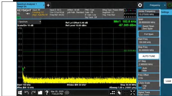
Band4-15MHz-QPSK-20175-1RB#74-0.15~30-PASS
