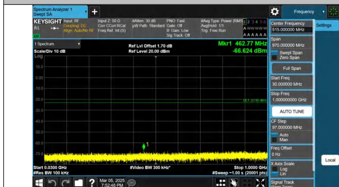
Band4-15MHz-QPSK-20175-1RB#0-30~1000-PASS
