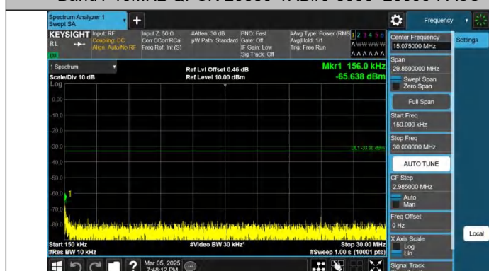
Band4-10MHz-QPSK-20350-1RB#49-0.15~30-PASS
