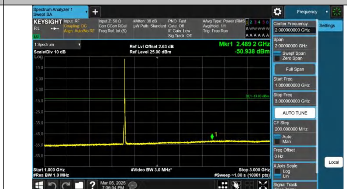
Band4-5MHz-QPSK-19975-1RB#0-1000~3000-PASS
