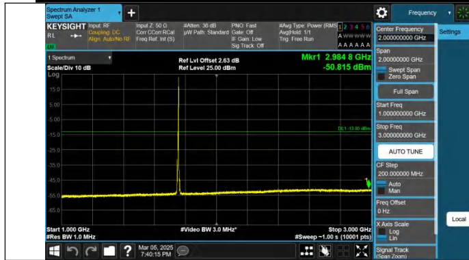
Band4-5MHz-QPSK-20375-1RB#24-1000~3000-PASS
