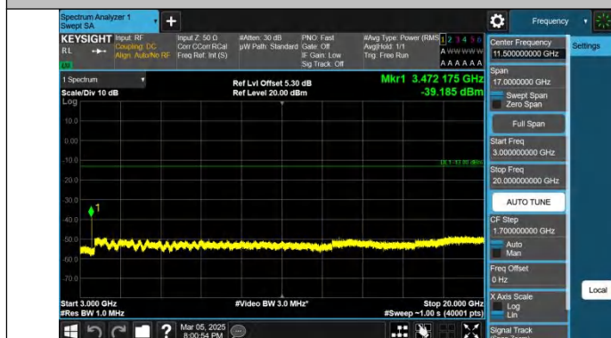
Band4-20MHz-QPSK-20300-1RB#0-3000~20000-PASS
