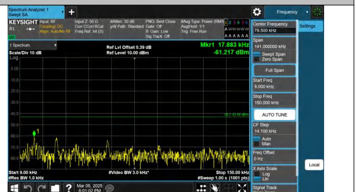
Band4-20MHz-QPSK-20300-1RB#99-0.009~0.15-PASS
