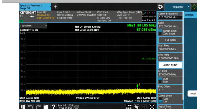
Band4-15MHz-QPSK-20325-1RB#0-30~1000-PASS
