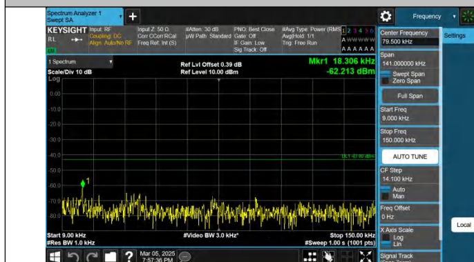
Band4-20MHz-QPSK-20050-1RB#0-0.009~0.15-PASS
