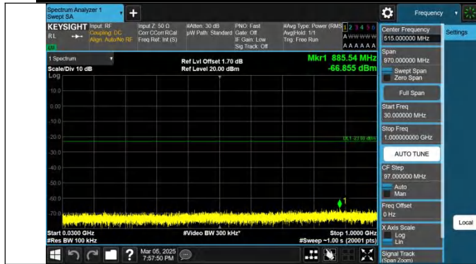
Band4-20MHz-QPSK-20050-1RB#0-30~1000-PASS
