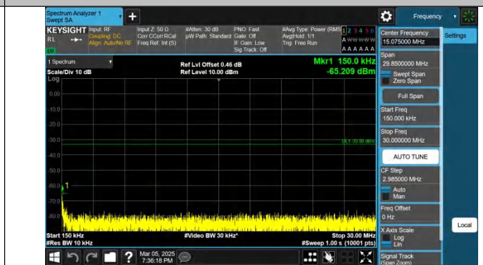
Band4-5MHz-QPSK-19975-1RB#0-0.15~30-PASS
