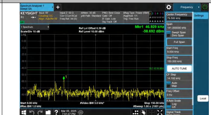
Band4-15MHz-QPSK-20025-1RB#74-0.009~0.15-PASS
