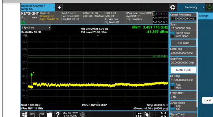
Band4-15MHz-QPSK-20175-1RB#0-3000~20000-PASS
