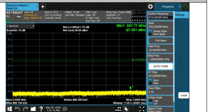
Band4-5MHz-QPSK-19975-1RB#24-30~1000-PASS
