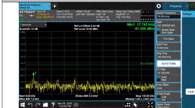
Band4-10MHz-QPSK-20175-1RB#0-0.009~0.15-PASS
