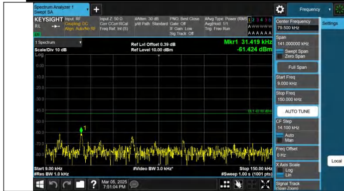
Band4-15MHz-QPSK-20025-1RB#0-0.009~0.15-PASS
