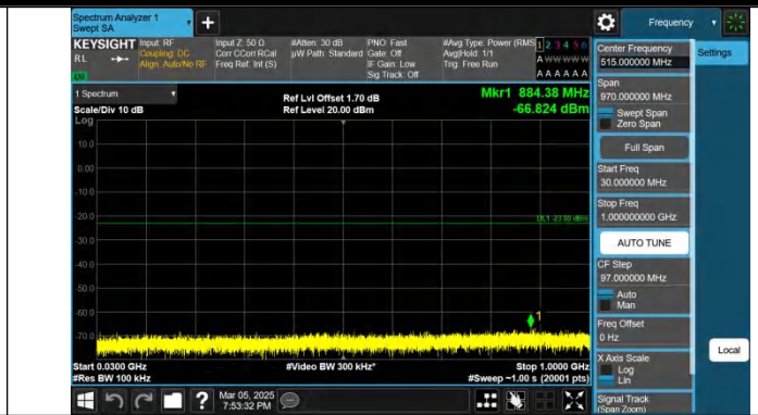
Band4-15MHz-QPSK-20175-1RB#74-30~1000-PASS
