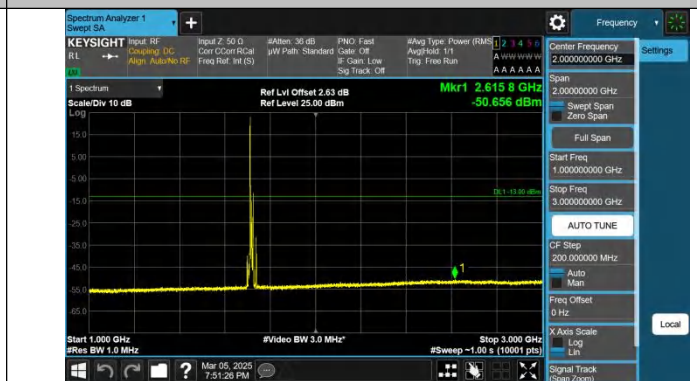
Band4-15MHz-QPSK-20025-1RB#0-1000~3000-PASS
