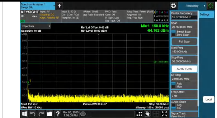
Band4-20MHz-QPSK-20175-1RB#0-0.15~30-PASS
