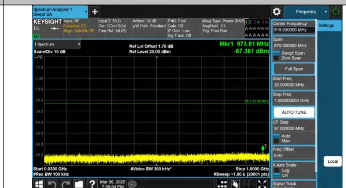
Band4-20MHz-QPSK-20175-1RB#99-30~1000-PASS
