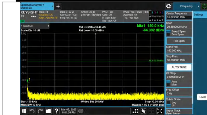
Band4-20MHz-QPSK-20300-1RB#99-0.15~30-PASS
