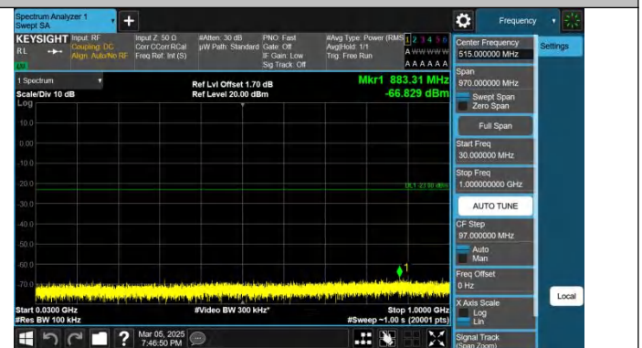
Band4-10MHz-QPSK-20175-1RB#49.30~1000-PASS
