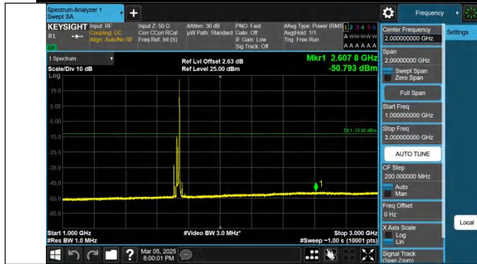
Band4-20MHz-QPSK-20175-1RB#99-1000~3000-PASS
