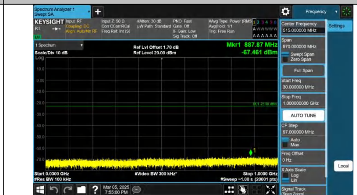
Band4-15MHz-QPSK-20325-1RB#74.30~1000-PASS
