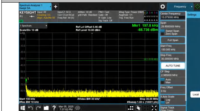
Band4-5MHz-QPSK-19975-1RB#24-0.15~30-PASS
