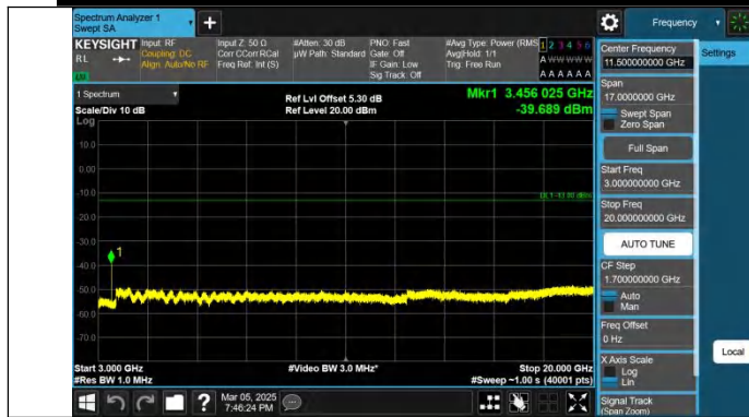
Band4-10MHz-QPSK-20175-1RB#0-3000~20000-PASS
