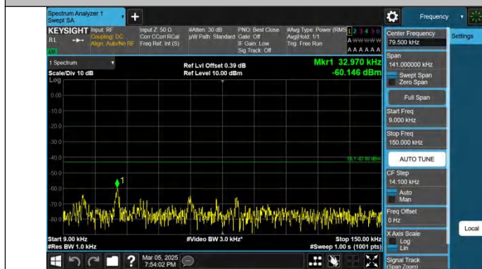
Band4-15MHz-QPSK-20325-1RB#0-0.009~0.15-PASS
