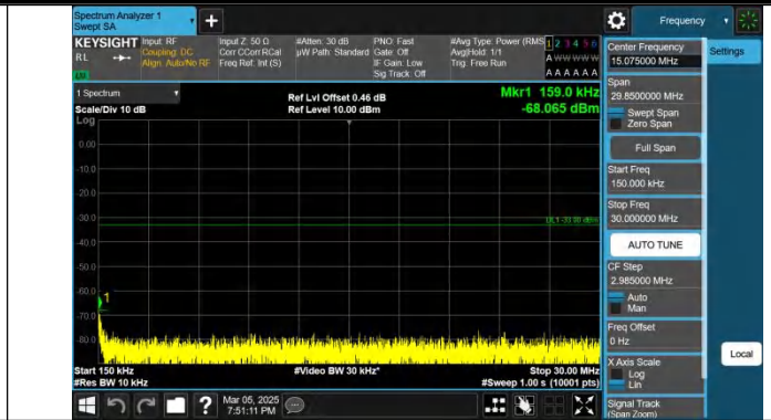
Band4-15MHz-QPSK-20025-1RB#0-0.15~30-PASS
