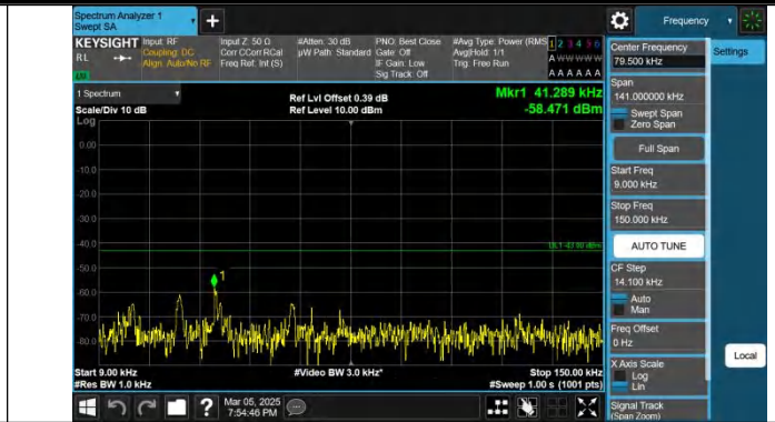
Band4-15MHz-QPSK-20325-1RB#74.0.009~0.15-PASS
