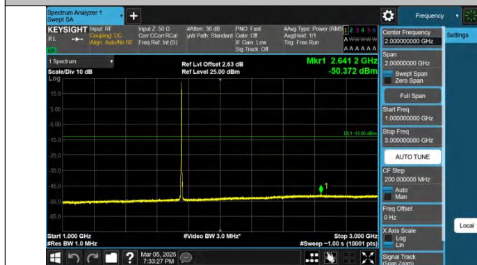
Band4-3MHz-QPSK-20385-1RB#14-1000~3000-PASS
