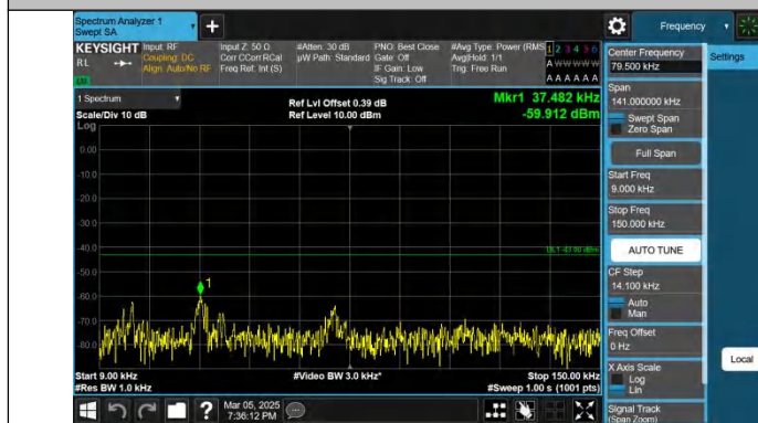
Band4-5MHz-QPSK-19975-1RB#0-0.009~0.15-PASS
