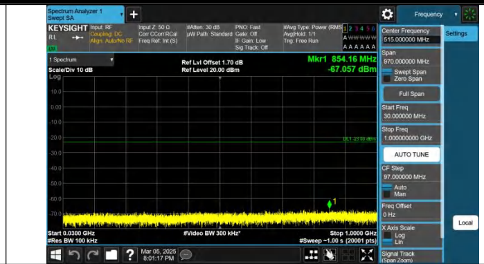
Band4-20MHz-QPSK-20300-1RB#99-30~1000-PASS
