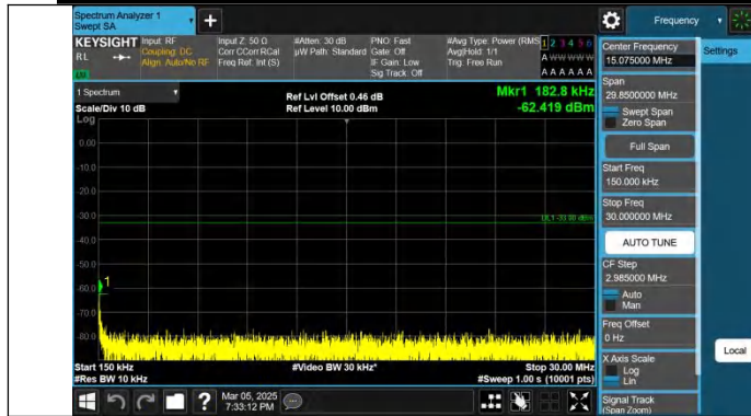
Band4-3MHz-QPSK-20385-1RB#14-0.15~30-PASS
