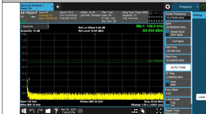
Band4-10MHz-QPSK-20175-1RB#49.0.15~30-PASS
