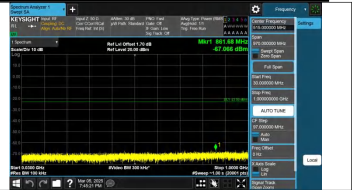
Band4-10MHz-QPSK-20000-1RB#49-30~1000-PASS
