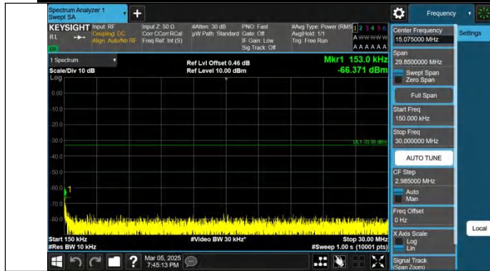
Band4-10MHz-QPSK-20000-1RB#49-0.15~30-PASS
