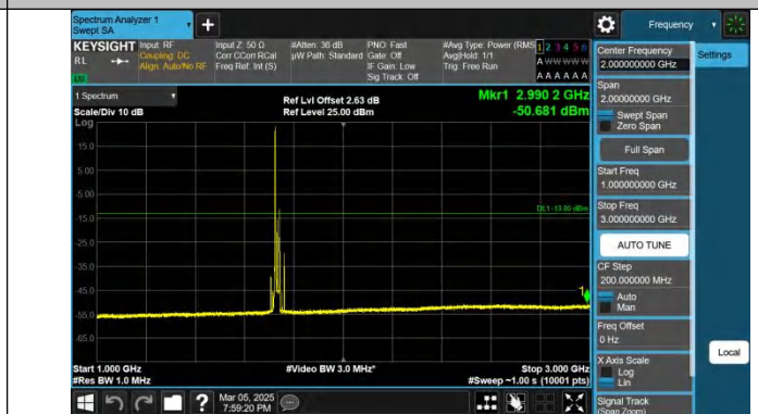
Band4-20MHz-QPSK-20175-1RB#0-1000~3000-PASS
