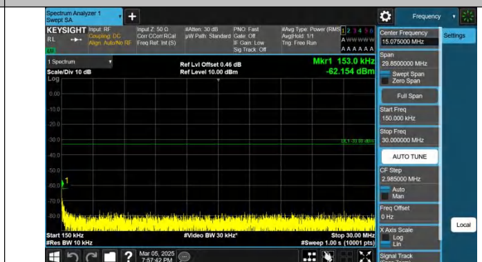
Band4-20MHz-QPSK-20050-1RB#0-0.15~30-PASS
