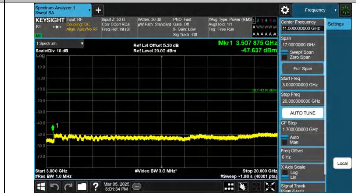
Band4-20MHz-QPSK-20300-1RB#99-3000~20000-PASS
