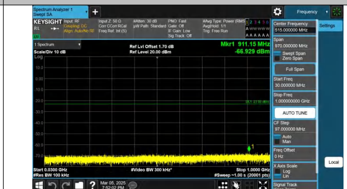
Band4-15MHz-QPSK-20025-1RB#74-30~1000-PASS
