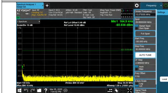
Band4-15MHz-QPSK-20325-1RB#74.0.15~30-PASS
