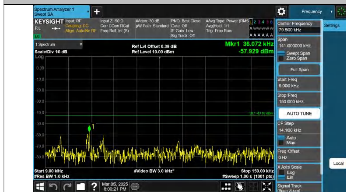
Band4-20MHz-QPSK-20300-1RB#0-0.009~0.15-PASS
