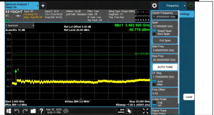
Band4-20MHz-QPSK-20175-1RB#99-3000~20000-PASS
