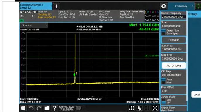
Band4-3MHz-QPSK-20175-1RB#14-1000~3000-PASS
