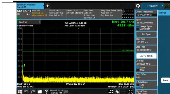
Band4-1.4MHz-QPSK-20175-1RB#5-0.15~30-PASS
