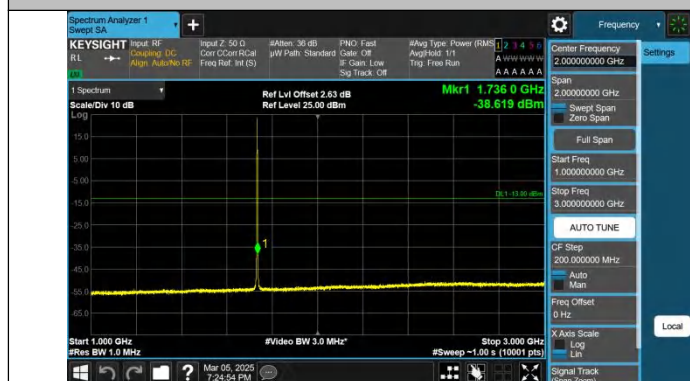
Band4-1.4MHz-QPSK-20175-1RB#5-1000~3000-PASS
