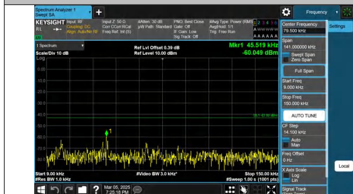
Band4-1.4MHz-QPSK-20393-1RB#0-0.009~0.15-PASS
