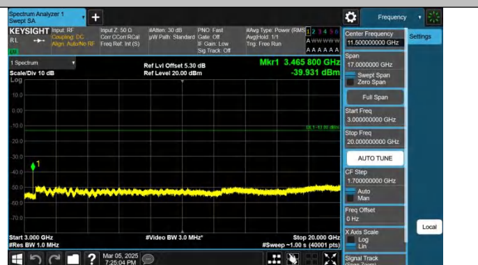
Band4-1.4MHz-QPSK-20175-1RB#5-3000~20000-PASS
