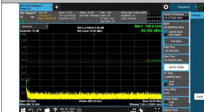
Band2-5MHz-QPSK-19175-1RB#24-0.15~30-PASS
