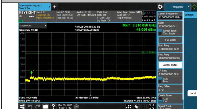
Band2-5MHz-QPSK-19175-1RB#0-3000~20000-PASS
