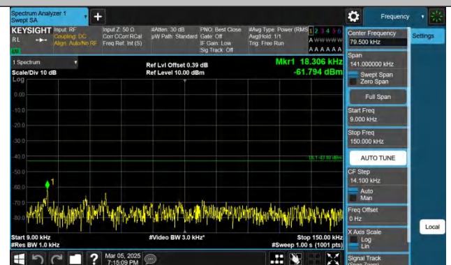
Band2-20MHz-QPSK-18900-1RB#99-0.009~0.15-PASS
