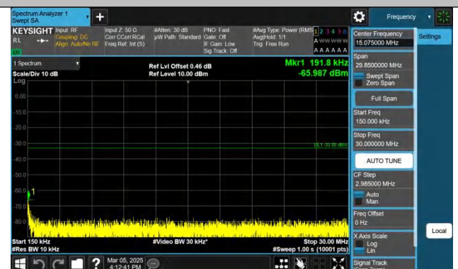
Band2-10MHz-QPSK-19150-1RB#0-0.15~30-PASS
