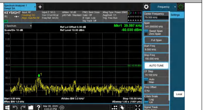
Band2-5MHz-QPSK-19175-1RB#24-0.009~0.15-PASS
