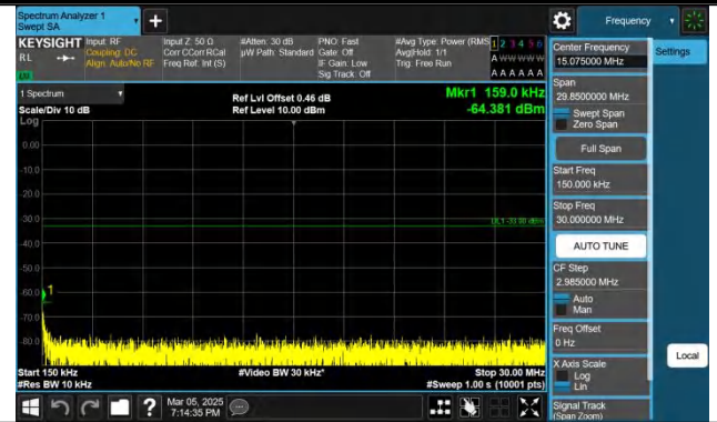
Band2-20MHz-QPSK-18900-1RB#0-0.15~30-PASS
