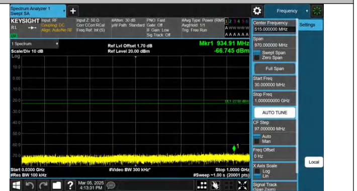
Band2-10MHz-QPSK-19150-1RB#49-30~1000-PASS
