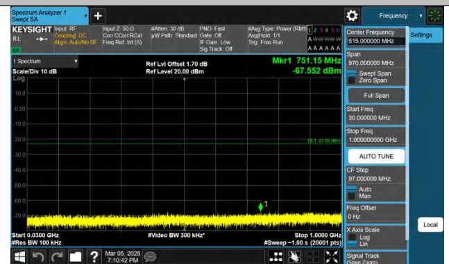
Band2-15MHz-QPSK-19125-1RB#74-30~1000-PASS
