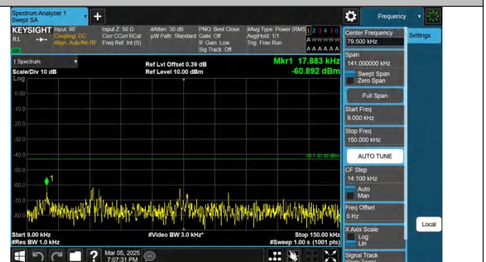
Band2-15MHz-QPSK-18675-1RB#74-0.009~0.15-PASS
