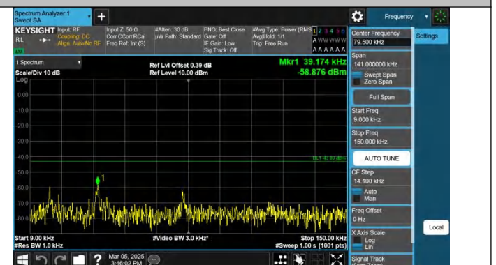
Band2-3MHz-QPSK-19185-1RB#14-0.009~0.15-PASS
