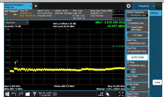
Band2-15MHz-QPSK-19125-1RB#74-3000~20000-PASS
