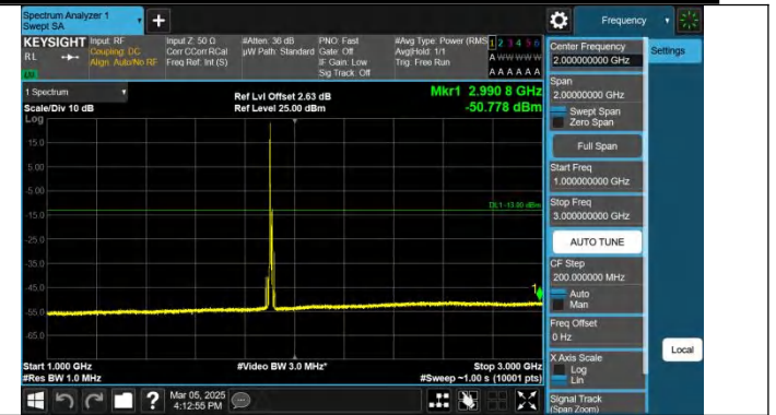
Band2-10MHz-QPSK-19150-1RB#0-1000~3000-PASS
