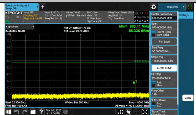
Band2-10MHz-QPSK-18900-1RB#49.30~1000-PASS
