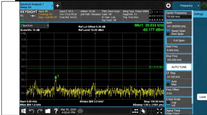
Band2-5MHz-QPSK-19175-1RB#0-0.009~0.15-PASS
