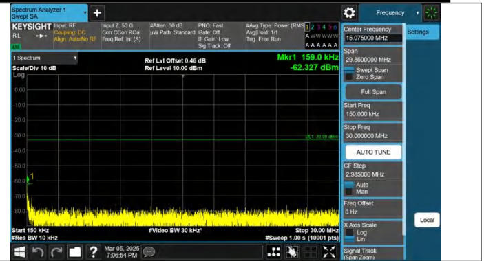
Band2-15MHz-QPSK-18675-1RB#0-0.15~30-PASS
