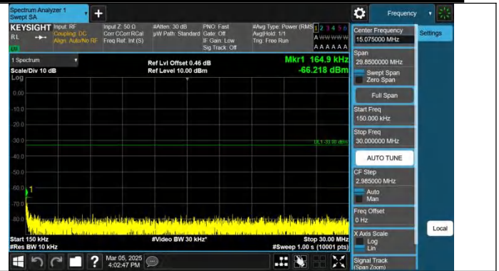
Band2-5MHz-QPSK-19175-1RB#0-0.15~30-PASS
