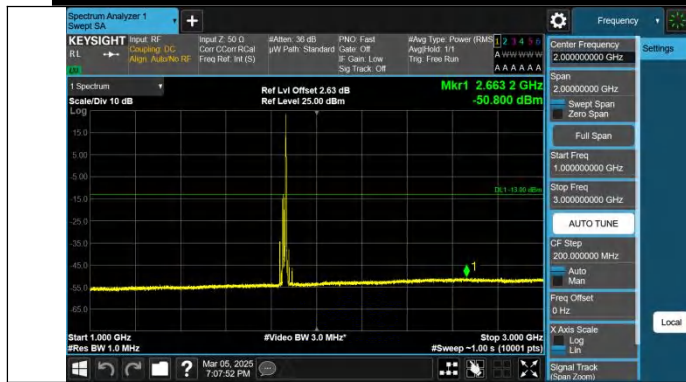
Band2-15MHz-QPSK-18675-1RB#74-1000~3000-PASS
