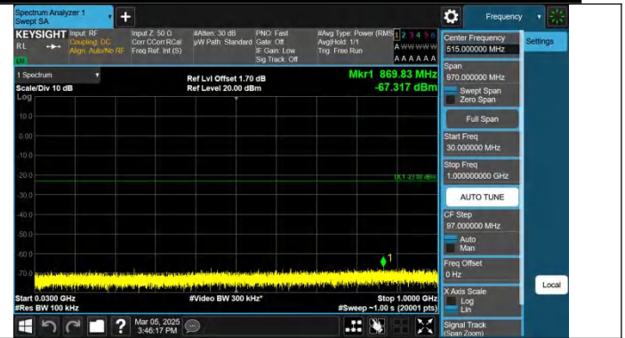
Band2-3MHz-QPSK-19185-1RB#14-30~1000-PASS
