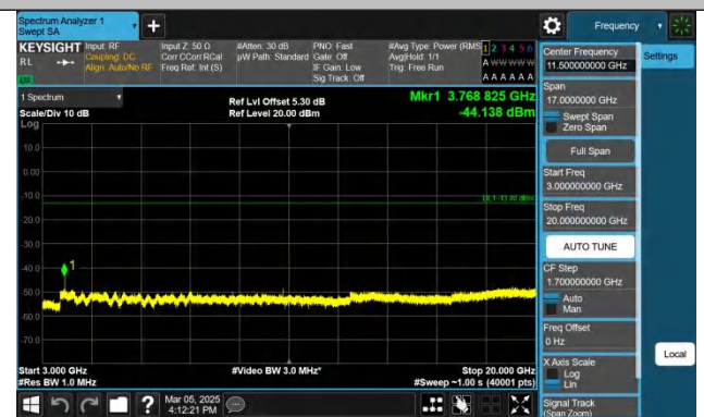
Band2-10MHz-QPSK-18900-1RB#49.3000~20000-PASS
