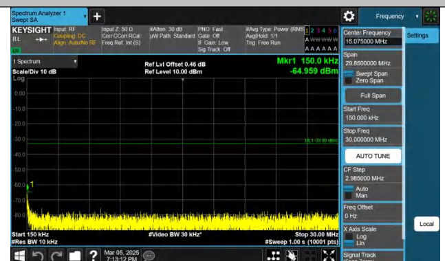
Band2-20MHz-QPSK-18700-1RB#0-0.15~30-PASS
